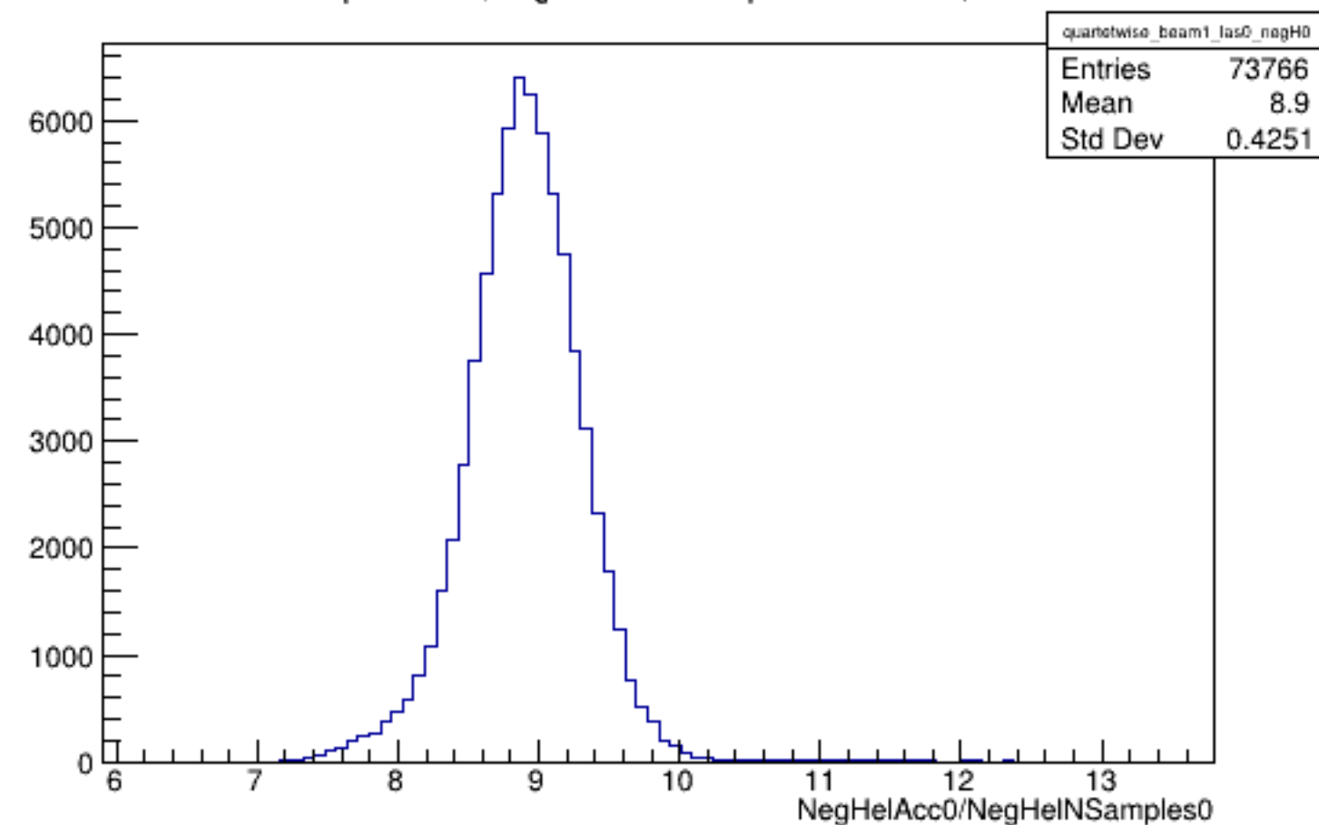
Run 4448 quartetwise, NegHelAcc0/NSamples0: Beam ON, Laser OFF
