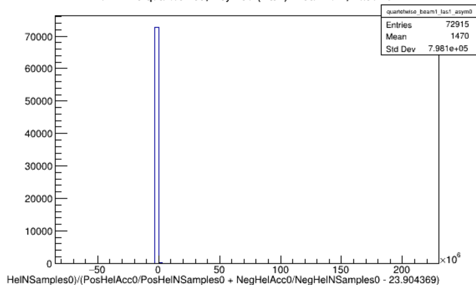
Run 4448 quartetwise, Asyms0 (Raw): Beam ON, Laser ON
