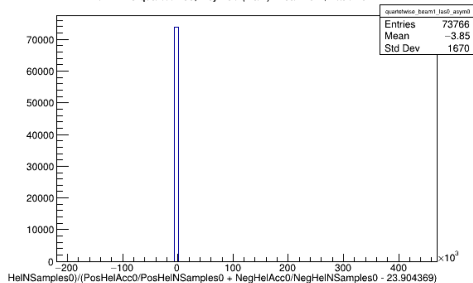
Run 4448 quartetwise, Asyms0 (Raw): Beam ON, Laser OFF
