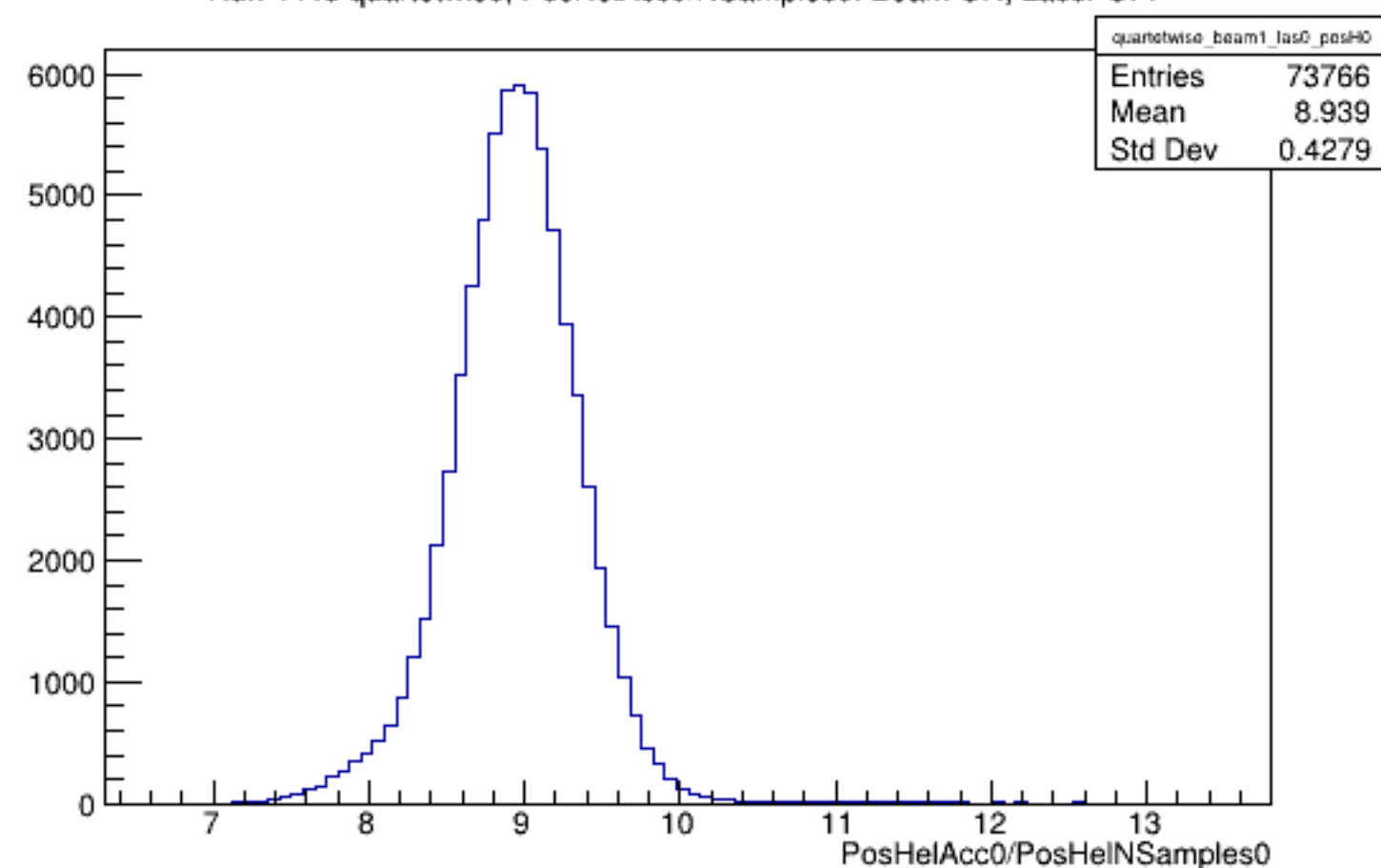
Run 4448 quartetwise, PosHelAcc0/NSamples0: Beam ON, Laser OFF
