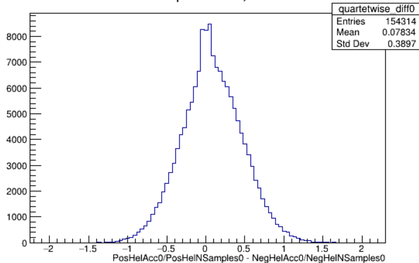
Run 4448 quartetwise, Diffs0: All
