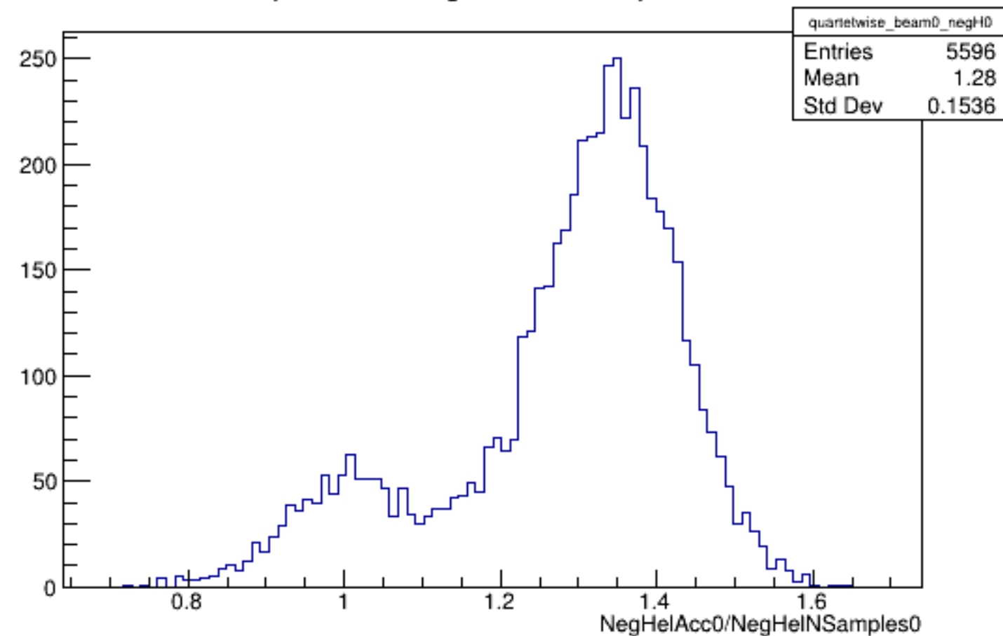
Run 4448 quartetwise, NegHelAcc0/NSamples0: Beam OFF
