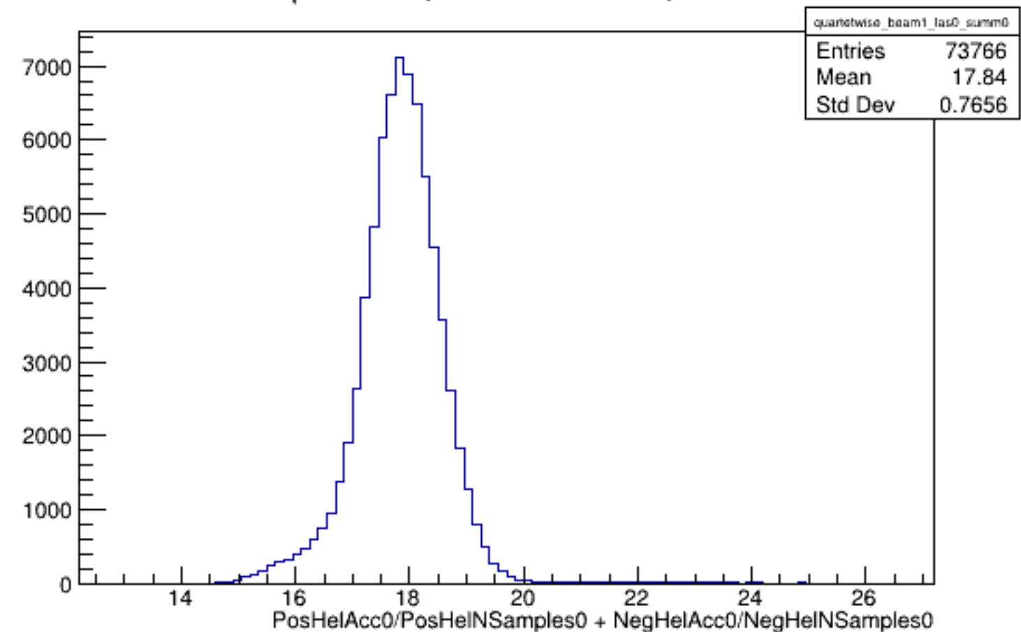
Run 4448 quartetwise, Sums0: Beam ON, Laser OFF
