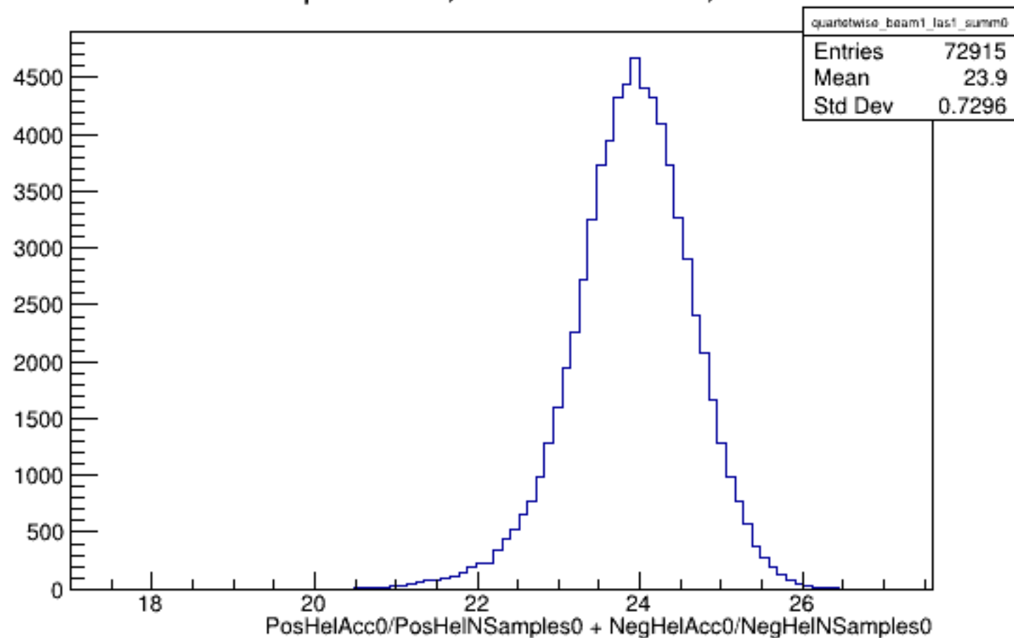
Run 4448 quartetwise, Sums0: Beam ON, Laser ON
