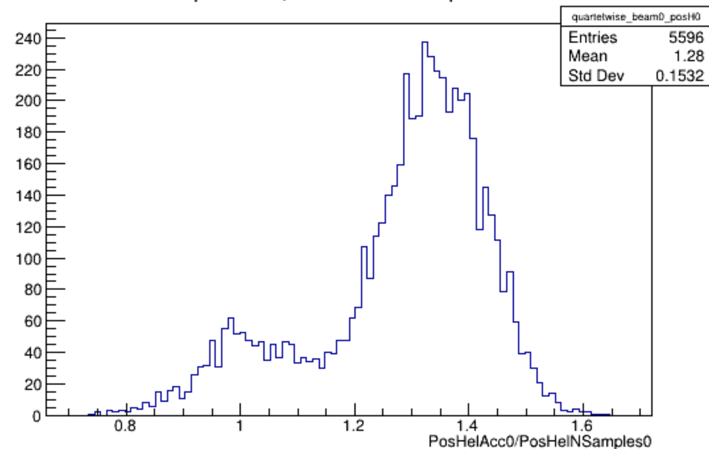
Run 4448 quartetwise, PosHelAcc0/NSamples0: Beam OFF
