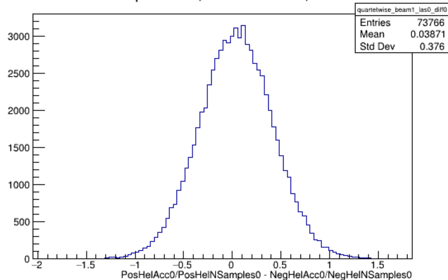
Run 4448 quartetwise, Diffs0: Beam ON, Laser OFF
