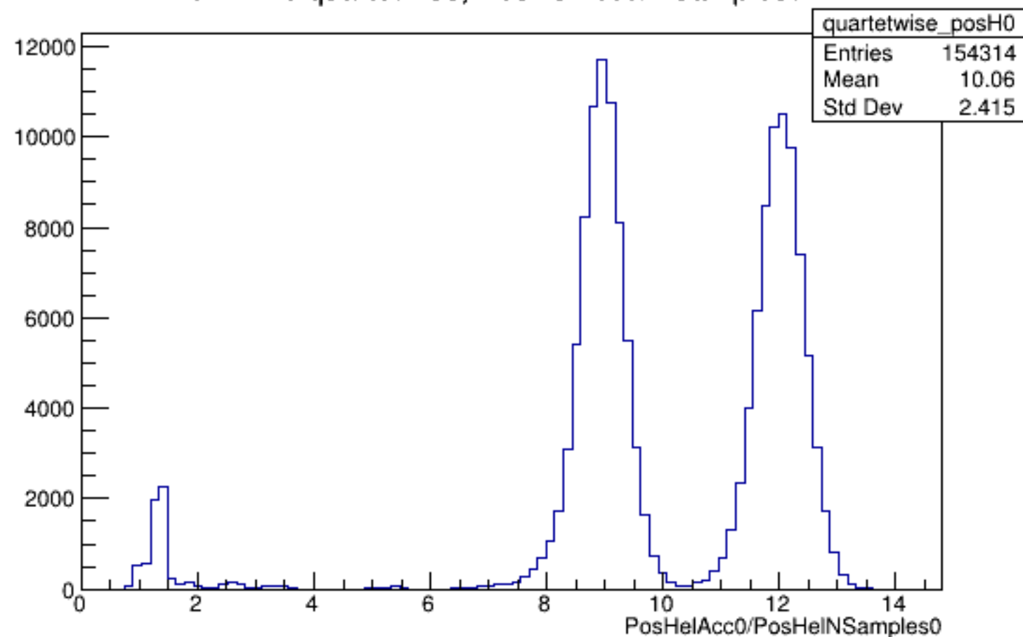
Run 4448 quartetwise, PosHelAcc0/NSamples0: All
