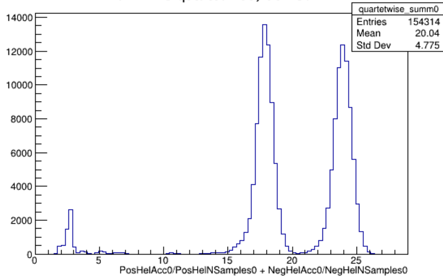
Run 4448 quartetwise, Sums0: All
