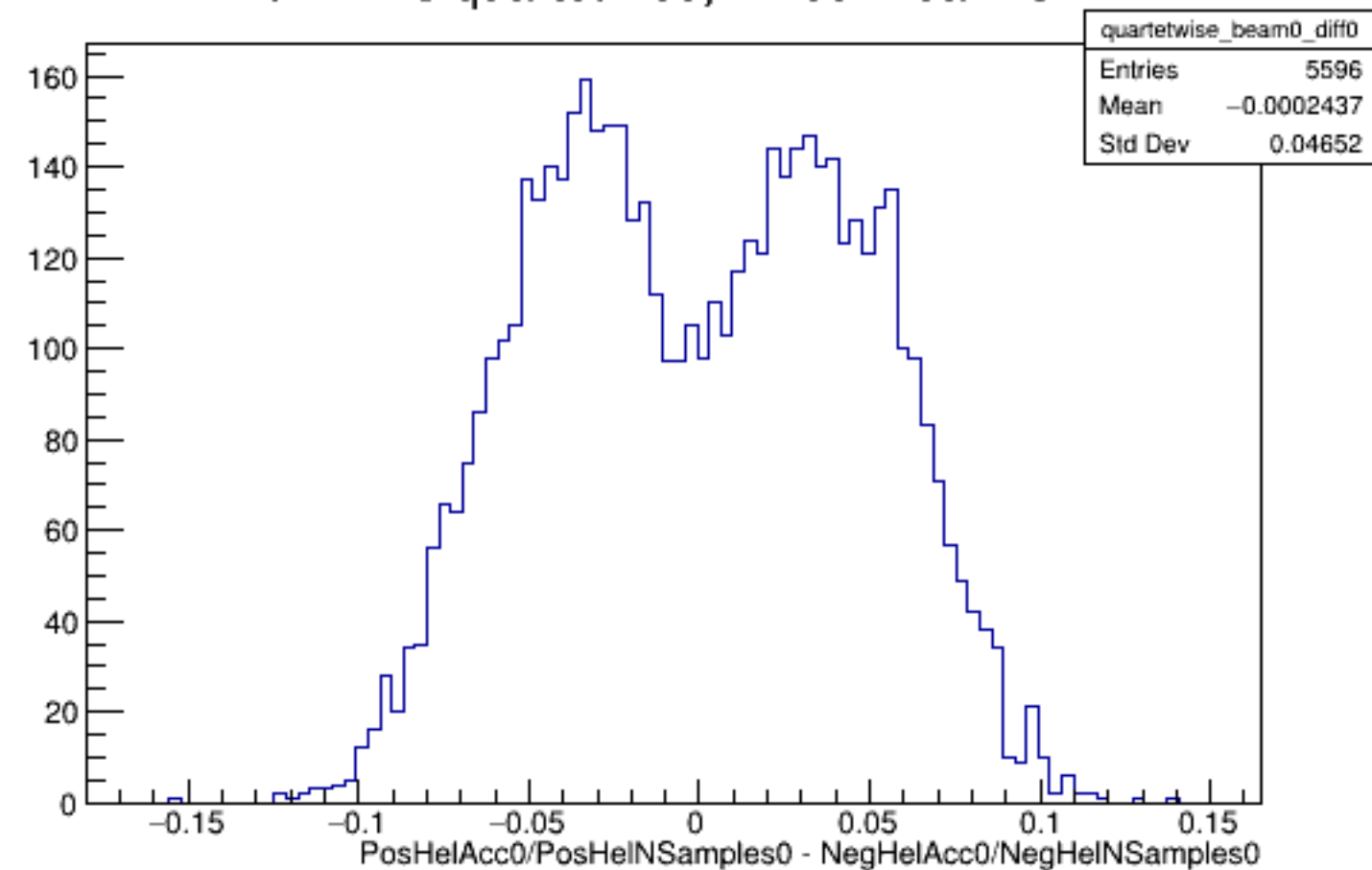
Run 4448 quartetwise, Diffs0: Beam OFF
