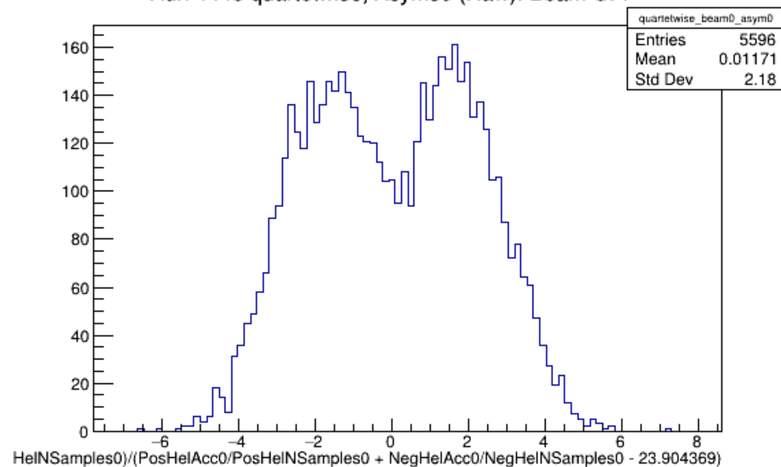
Run 4448 quartetwise, Asyms0 (Raw): Beam OFF
