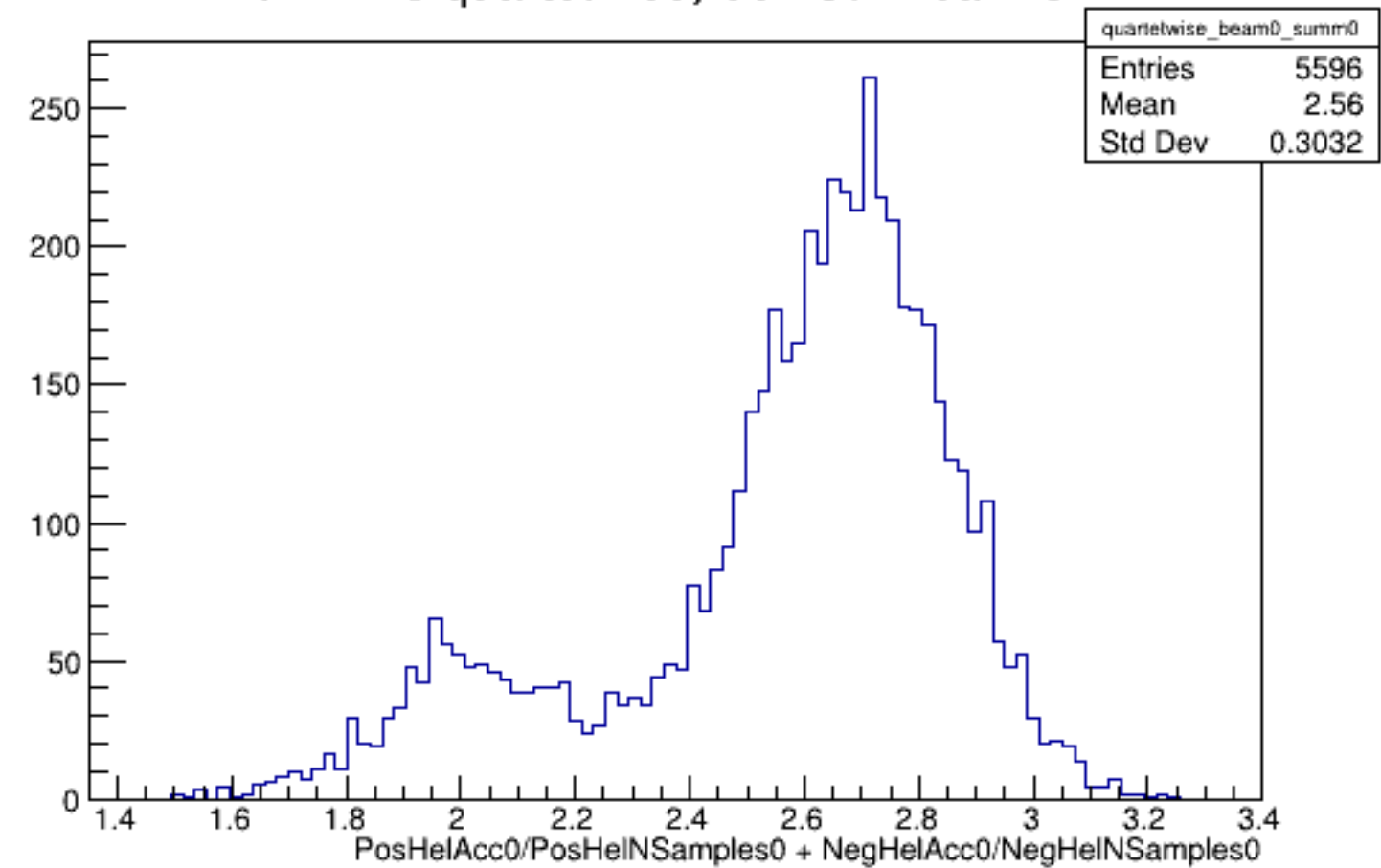
Run 4448 quartetwise, Sums0: Beam OFF
