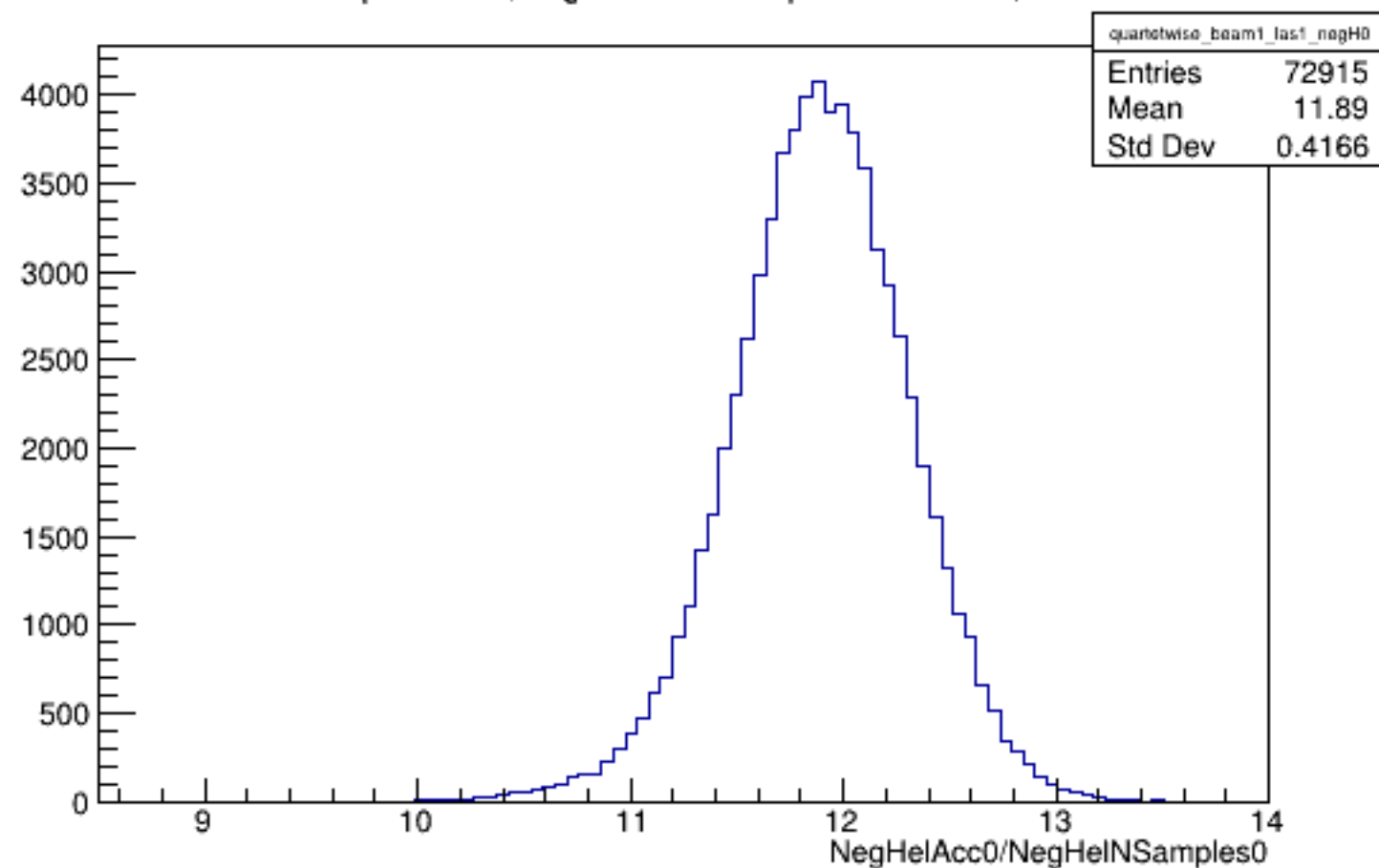
Run 4448 quartetwise, NegHelAcc0/NSamples0: Beam ON, Laser ON
