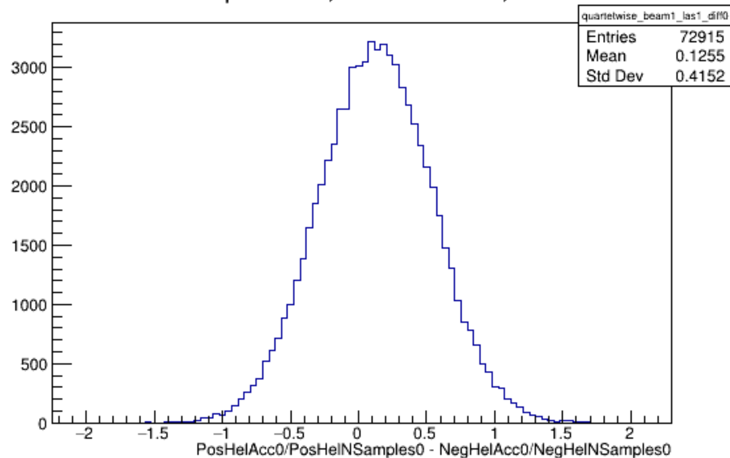
Run 4448 quartetwise, Diffs0: Beam ON, Laser ON
