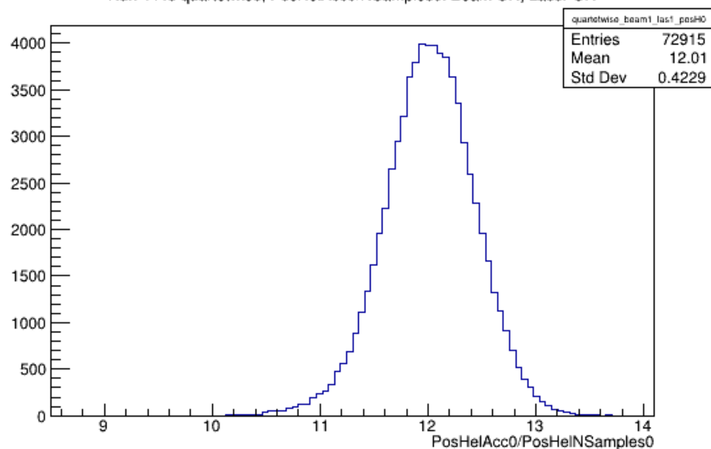
Run 4448 quartetwise, PosHelAcc0/NSamples0: Beam ON, Laser ON
