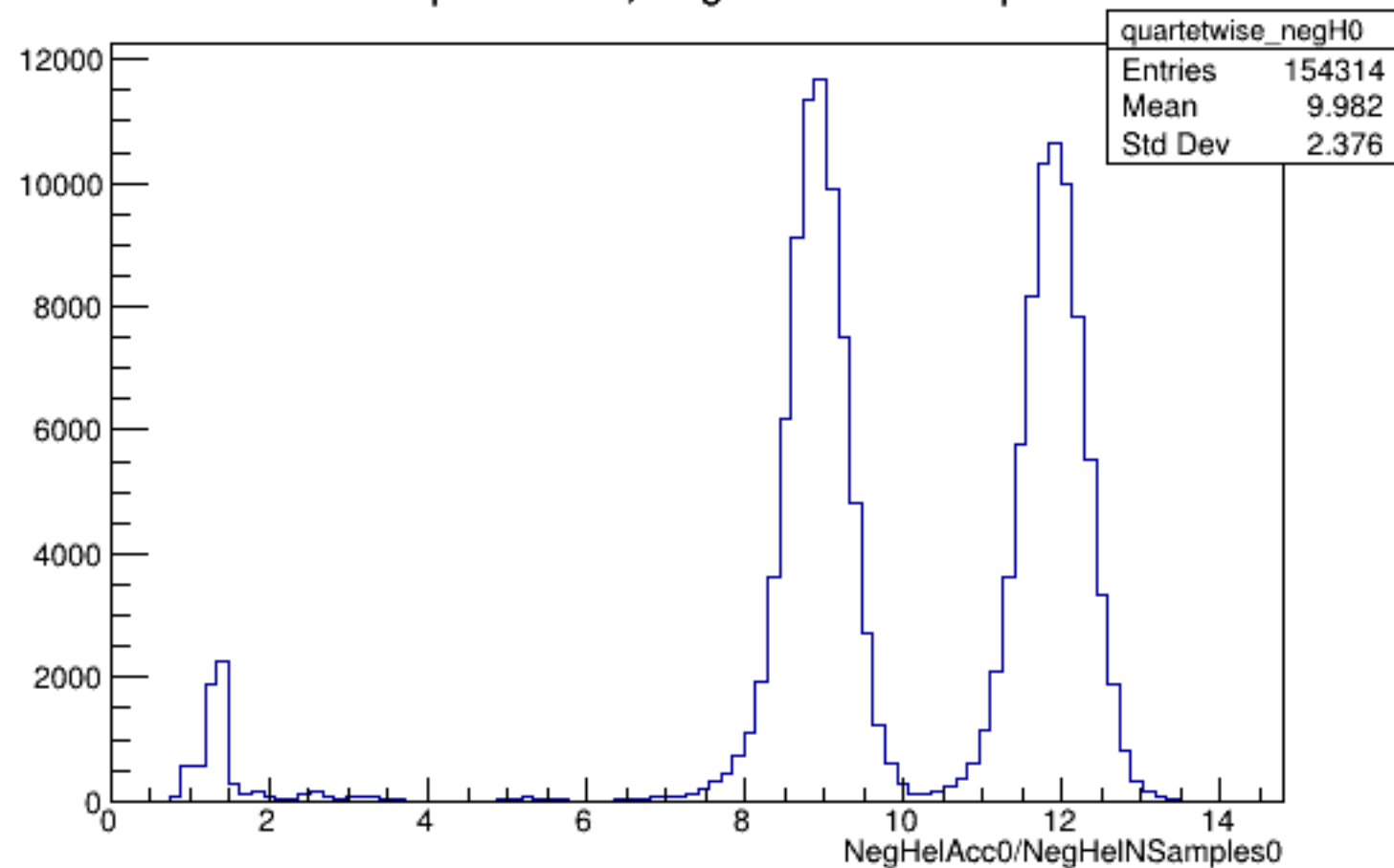
Run 4448 quartetwise, NegHelAcc0/NSamples0: All
