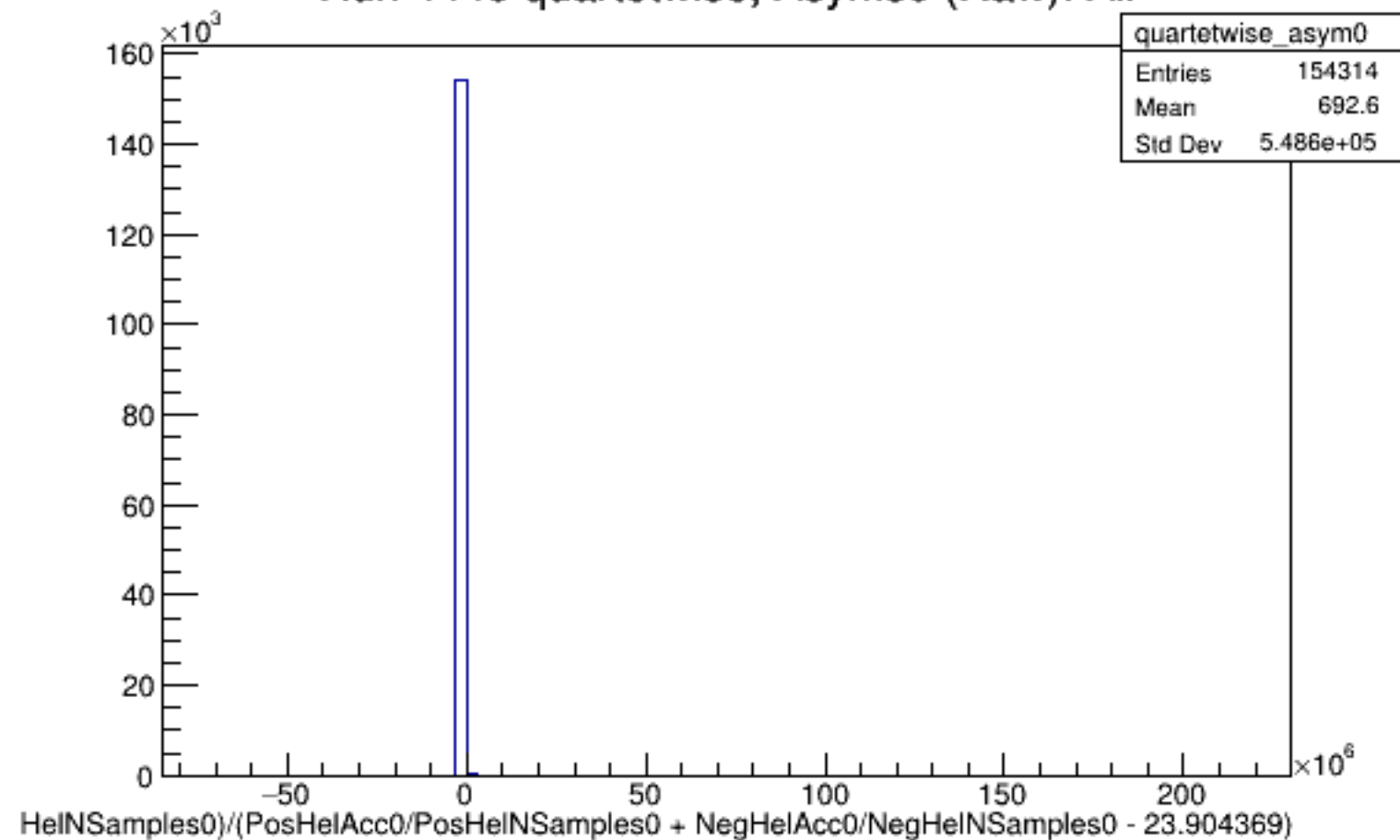
Run 4448 quartetwise, Asyms0 (Raw): All
