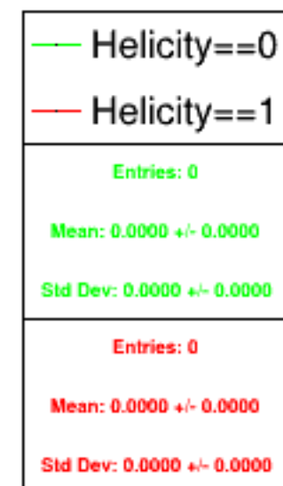
Run 4481 triggerwise, sums: Beam ON, Laser OFF
