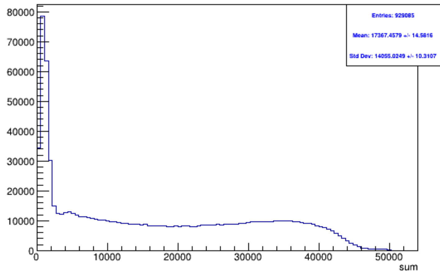
Run 4481 triggerwise, sums: All
