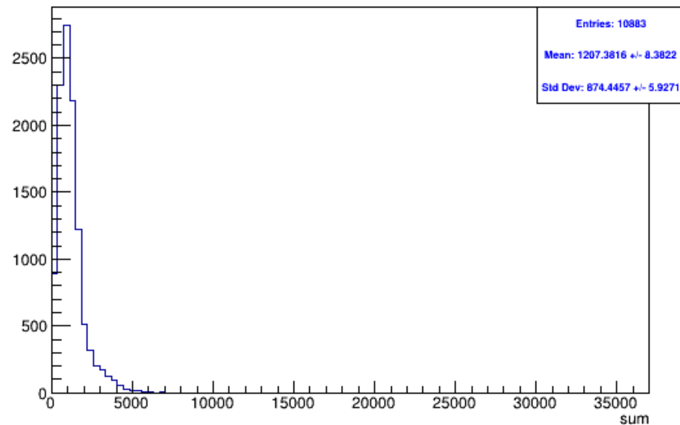
Run 4481 triggerwise, sums: Beam OFF
