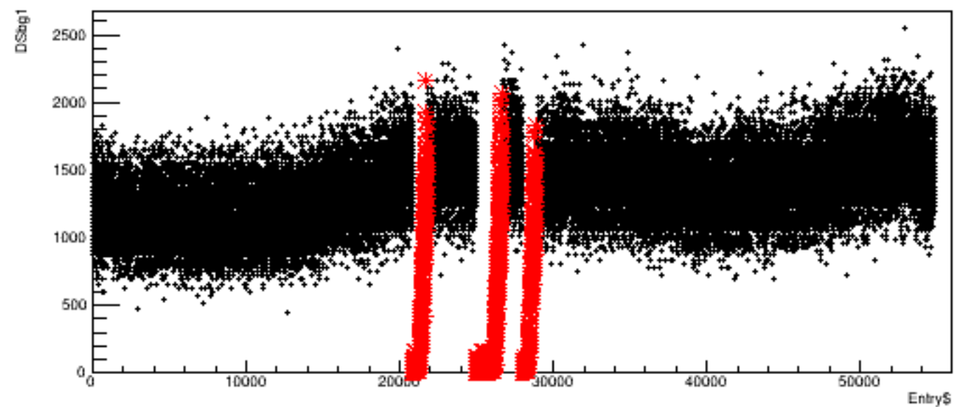
Run 4486, quartetwise: DSbg1 vs time
