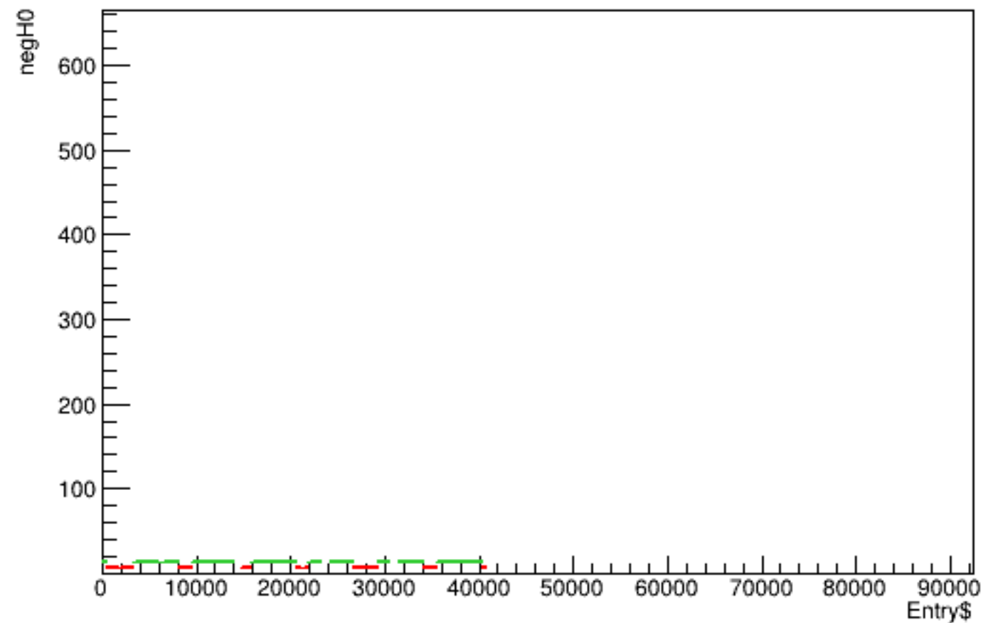
Run 4490 quartetwise, negH0 vs time
