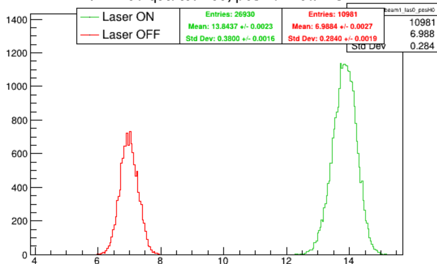
Run 4490 quartetwise, posH0: Beam ON
