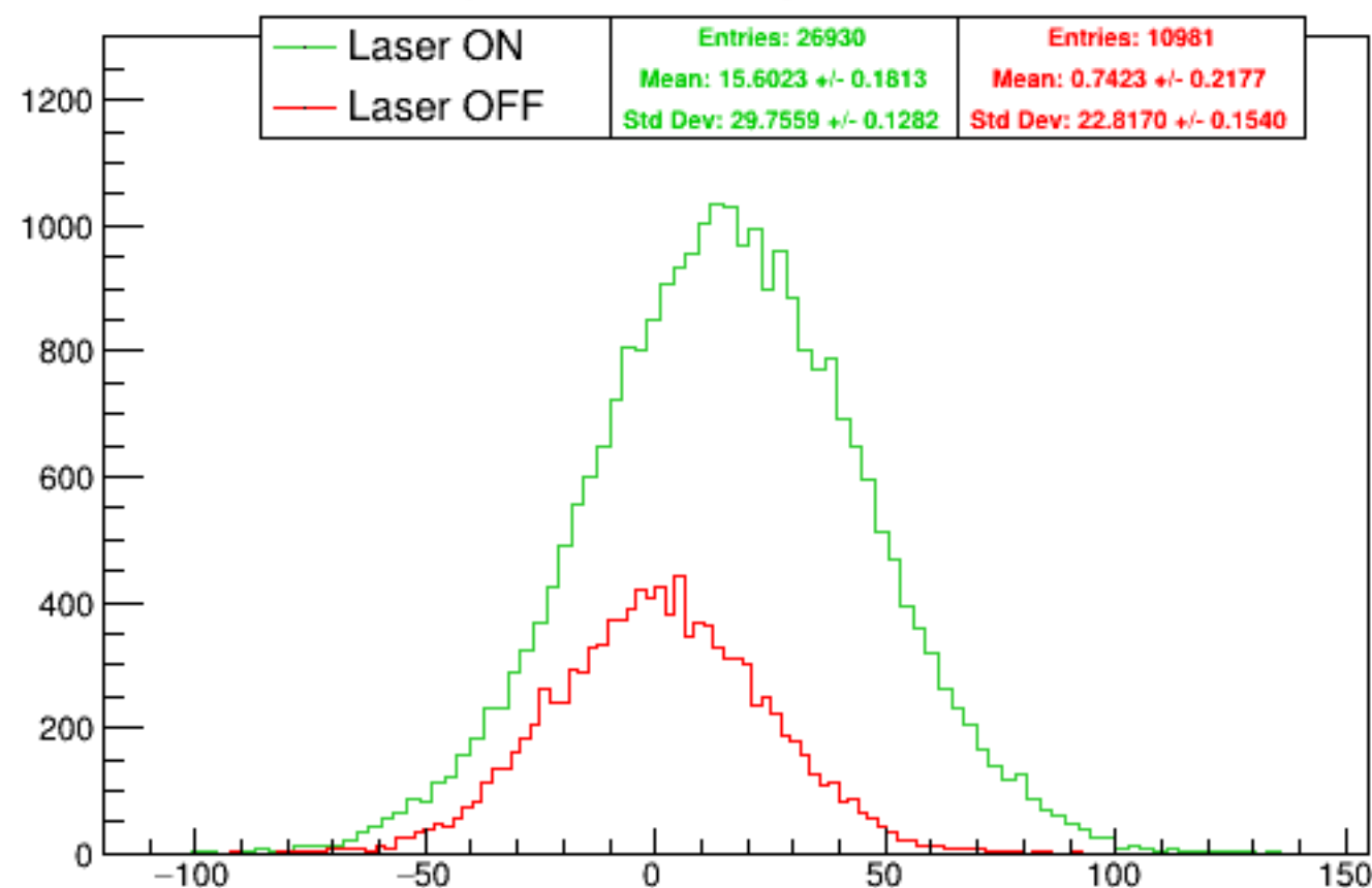
Run 4490 quartetwise, asym0sub: Beam ON
