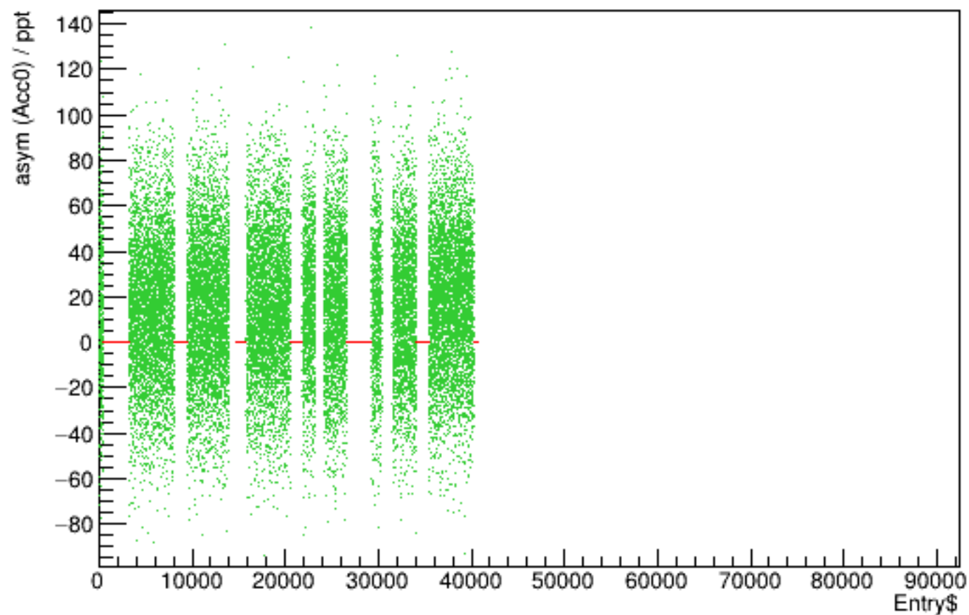
Run 4490 quartetwise, asym0sub vs time
