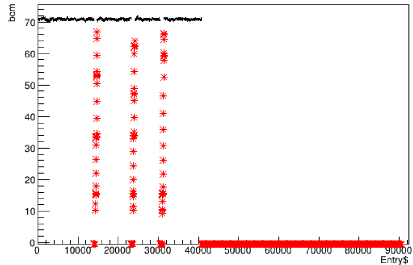
Run 4490 quartetwise, bcm vs time
