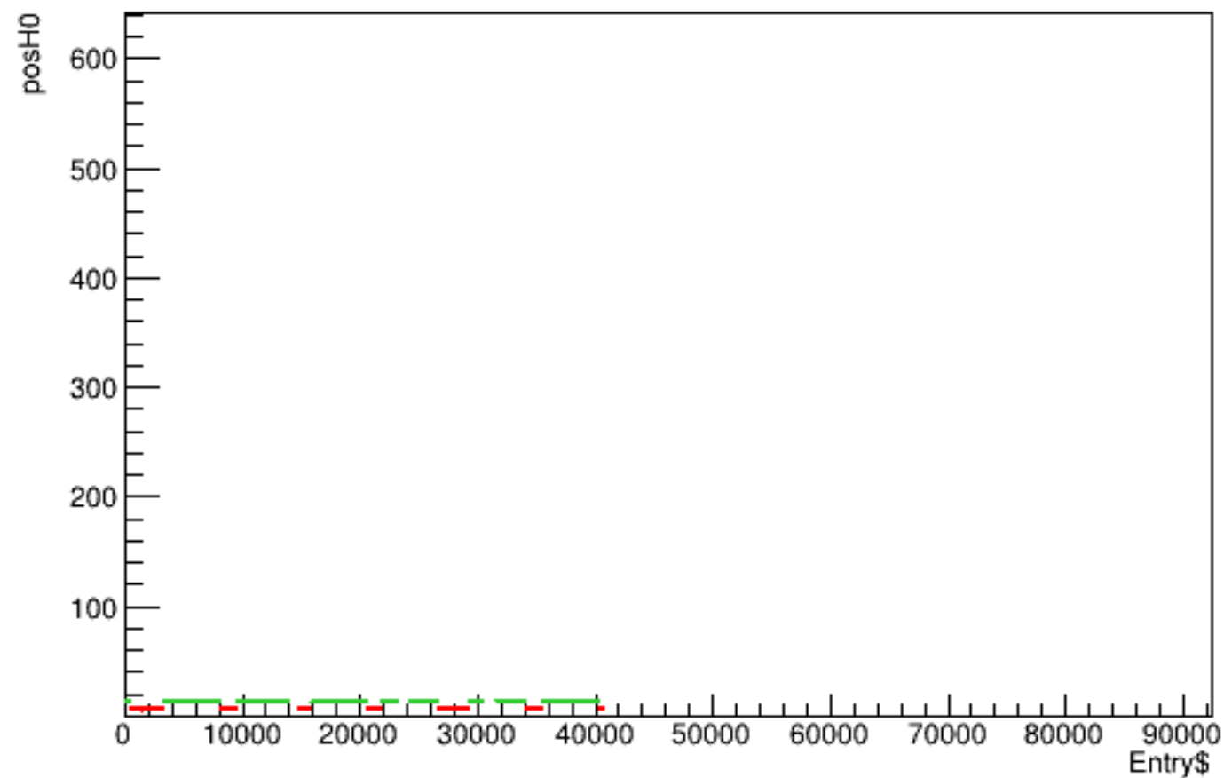
Run 4490 quartetwise, posH0 vs time
