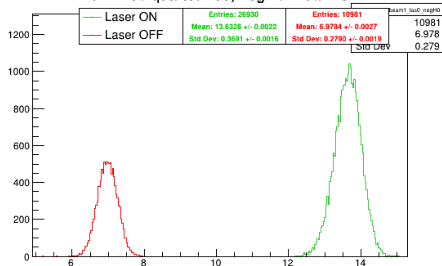
Run 4490 quartetwise, negH0: Beam ON
