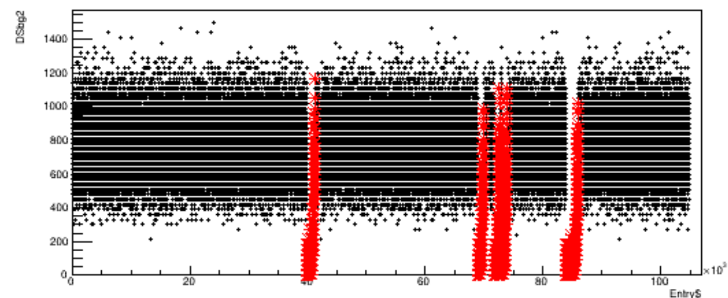
Run 4491, quartetwise: DSbg2 vs time
