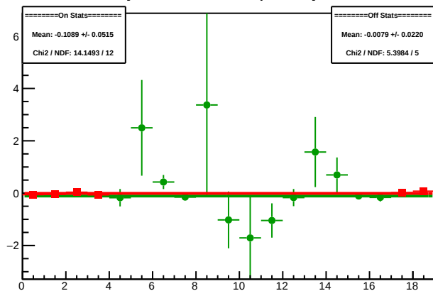
Cycle 4491.4: Multiplet Asyms
