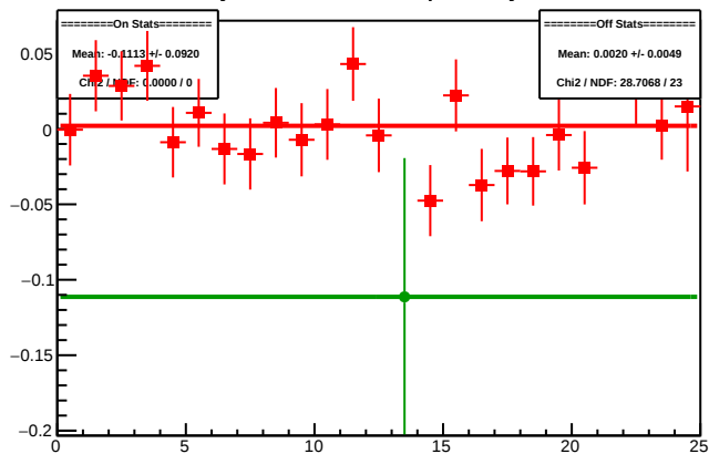
Cycle 4491.8: Multiplet Asyms
