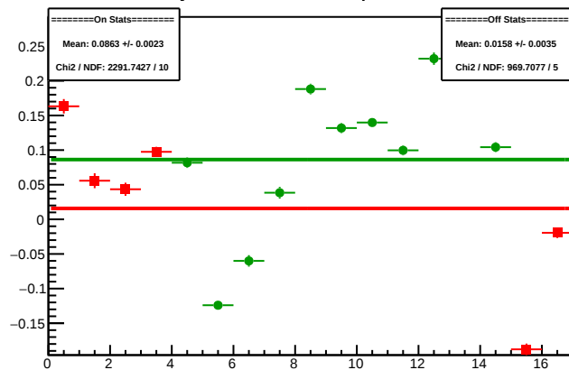
Cycle 4491.11: Multiplet Sums
