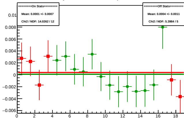
Cycle 4491.4: Multiplet Diffs
