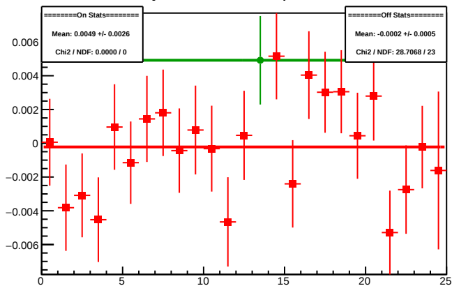
Cycle 4491.8: Multiplet Diffs
