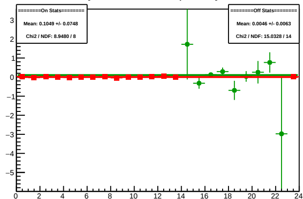
Cycle 4491.1: Multiplet Asyms
