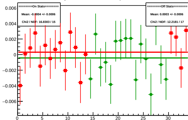
Cycle 4491.3: Multiplet Diffs
