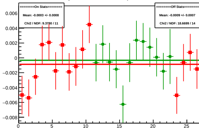
Cycle 4491.6: Multiplet Diffs
