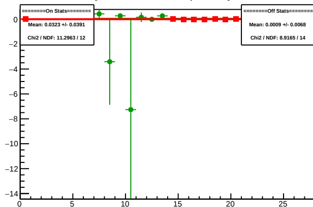
Cycle 4491.2: Multiplet Asyms
