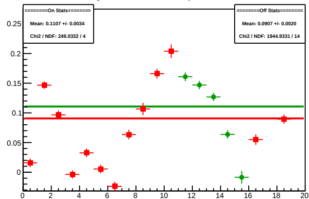
Cycle 4491.9: Multiplet Sums
