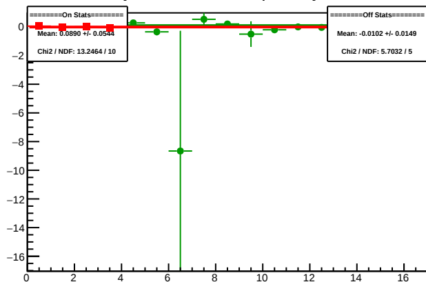
Cycle 4491.11: Multiplet Asyms
