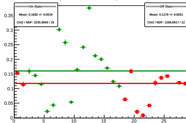
Cycle 4491.5: Multiplet Sums
