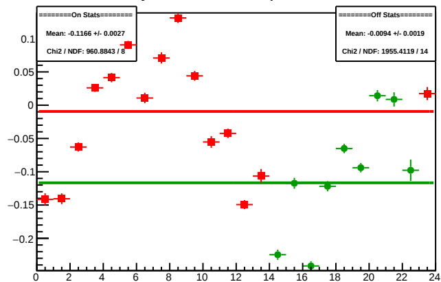
Cycle 4491.1: Multiplet Sums
