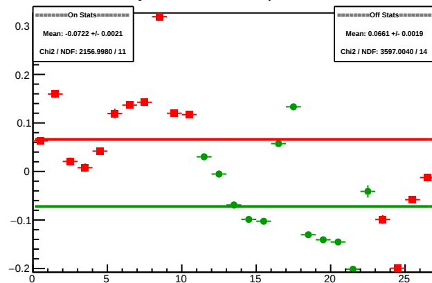
Cycle 4491.6: Multiplet Sums
