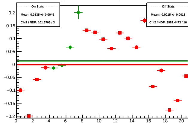
Cycle 4491.7: Multiplet Sums
