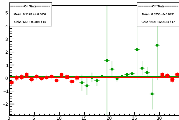
Cycle 4491.3: Multiplet Asyms
