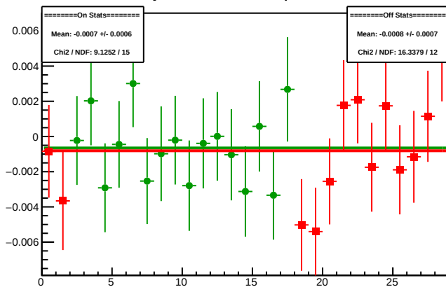
Cycle 4491.5: Multiplet Diffs
