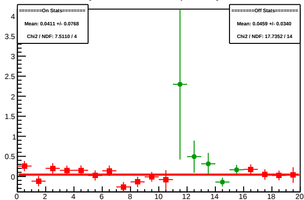
Cycle 4491.9: Multiplet Asyms
