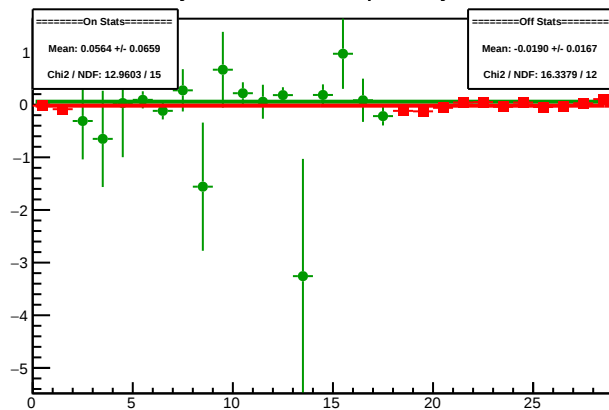
Cycle 4491.5: Multiplet Asyms
