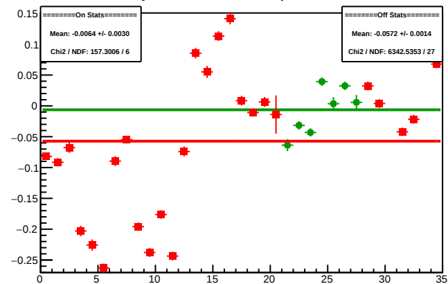
Cycle 4491.13: Multiplet Sums
