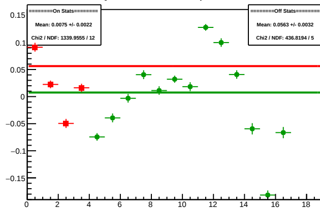
Cycle 4491.4: Multiplet Sums
