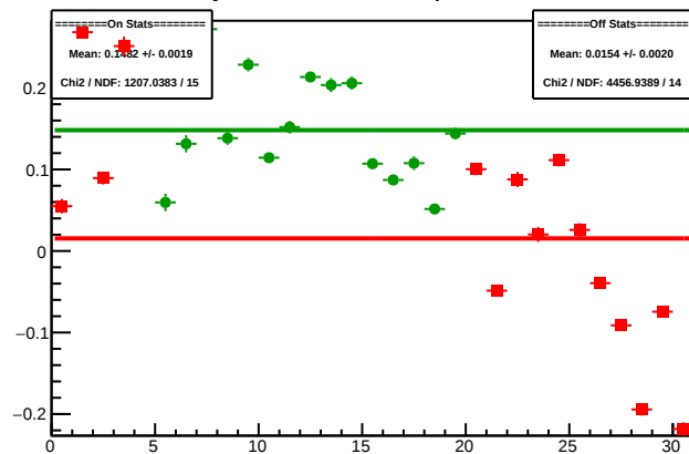
Cycle 4491.10: Multiplet Sums
