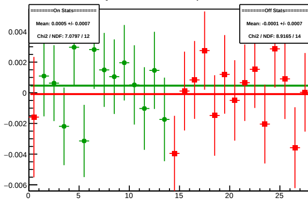
Cycle 4491.2: Multiplet Diffs
