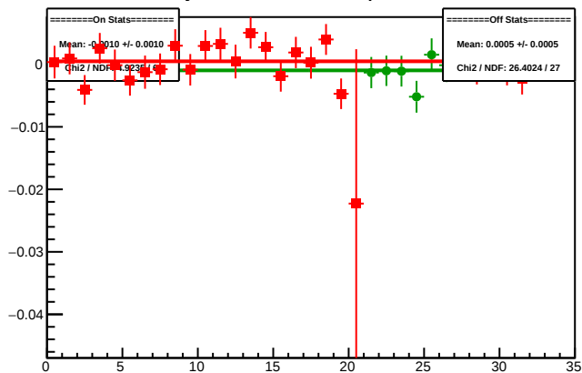
Cycle 4491.13: Multiplet Diffs
