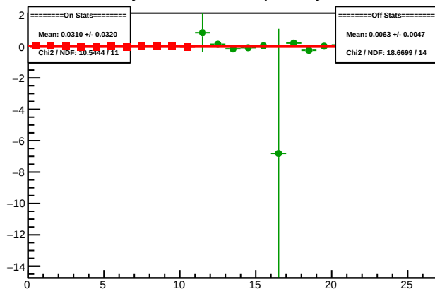
Cycle 4491.6: Multiplet Asyms
