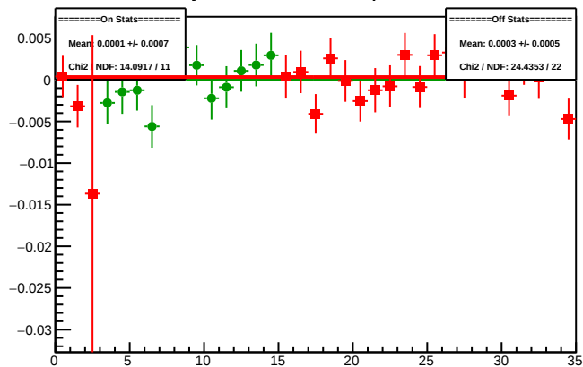
Cycle 4491.12: Multiplet Diffs
