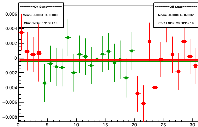
Cycle 4491.10: Multiplet Diffs
