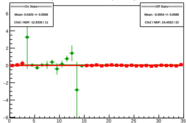
Cycle 4491.12: Multiplet Asyms
