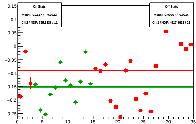
Cycle 4491.12: Multiplet Sums
