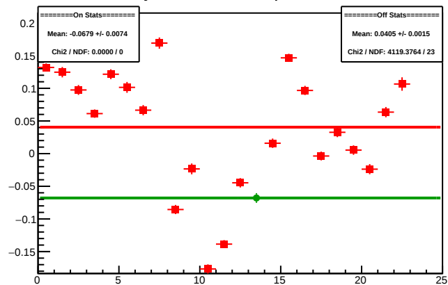
Cycle 4491.8: Multiplet Sums
