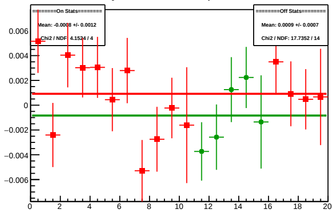
Cycle 4491.9: Multiplet Diffs
