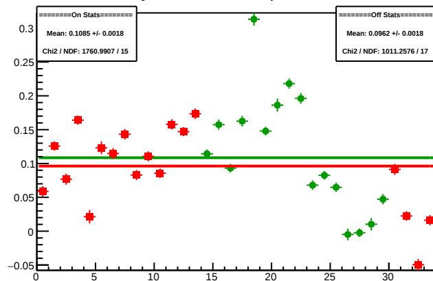
Cycle 4491.3: Multiplet Sums
