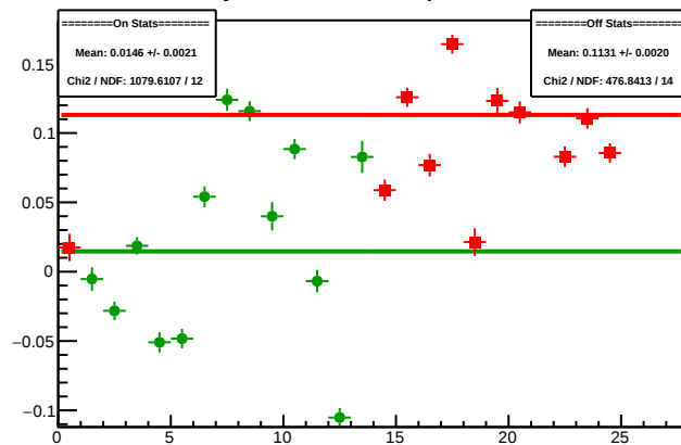
Cycle 4491.2: Multiplet Sums
