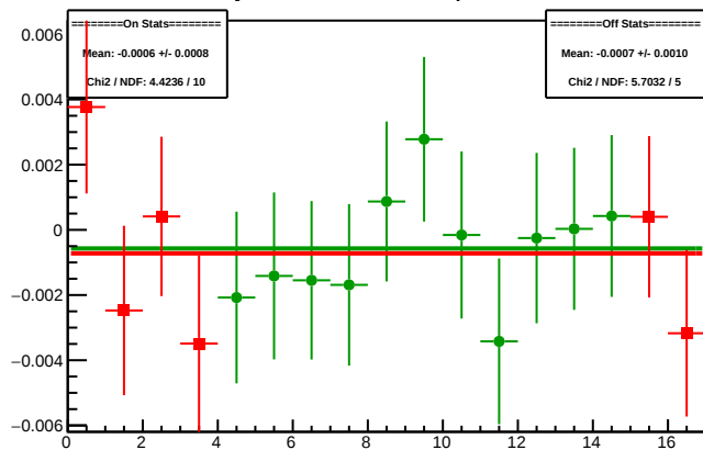
Cycle 4491.11: Multiplet Diffs
