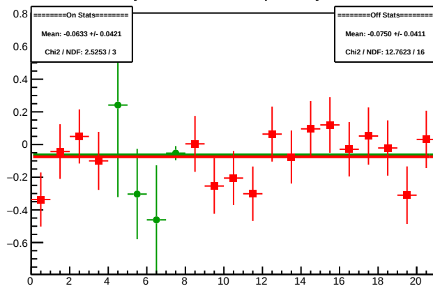
Cycle 4491.7: Multiplet Asyms
