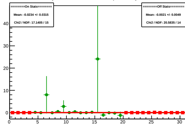
Cycle 4491.10: Multiplet Asyms
