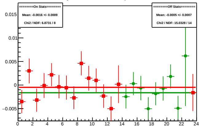
Cycle 4491.1: Multiplet Diffs
