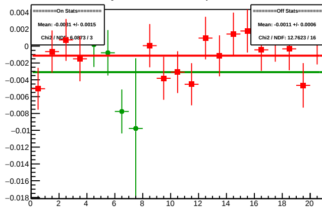
Cycle 4491.7: Multiplet Diffs
