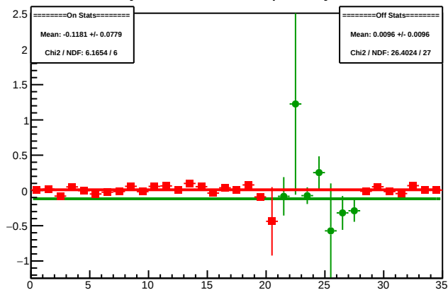
Cycle 4491.13: Multiplet Asyms
