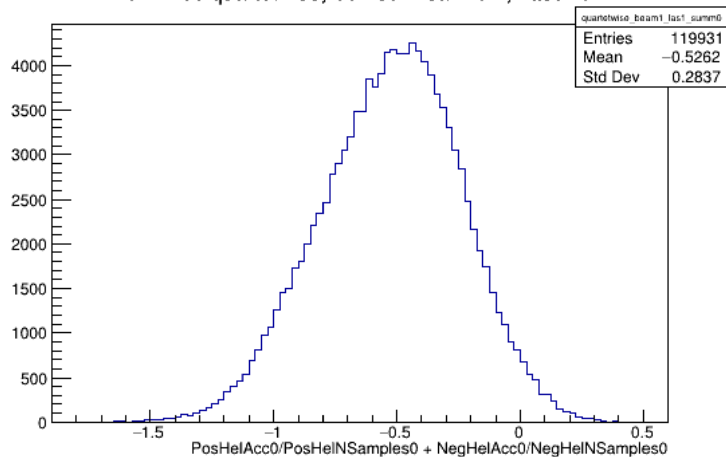
Run 4496 quartetwise, Sums0: Beam ON, Laser ON
