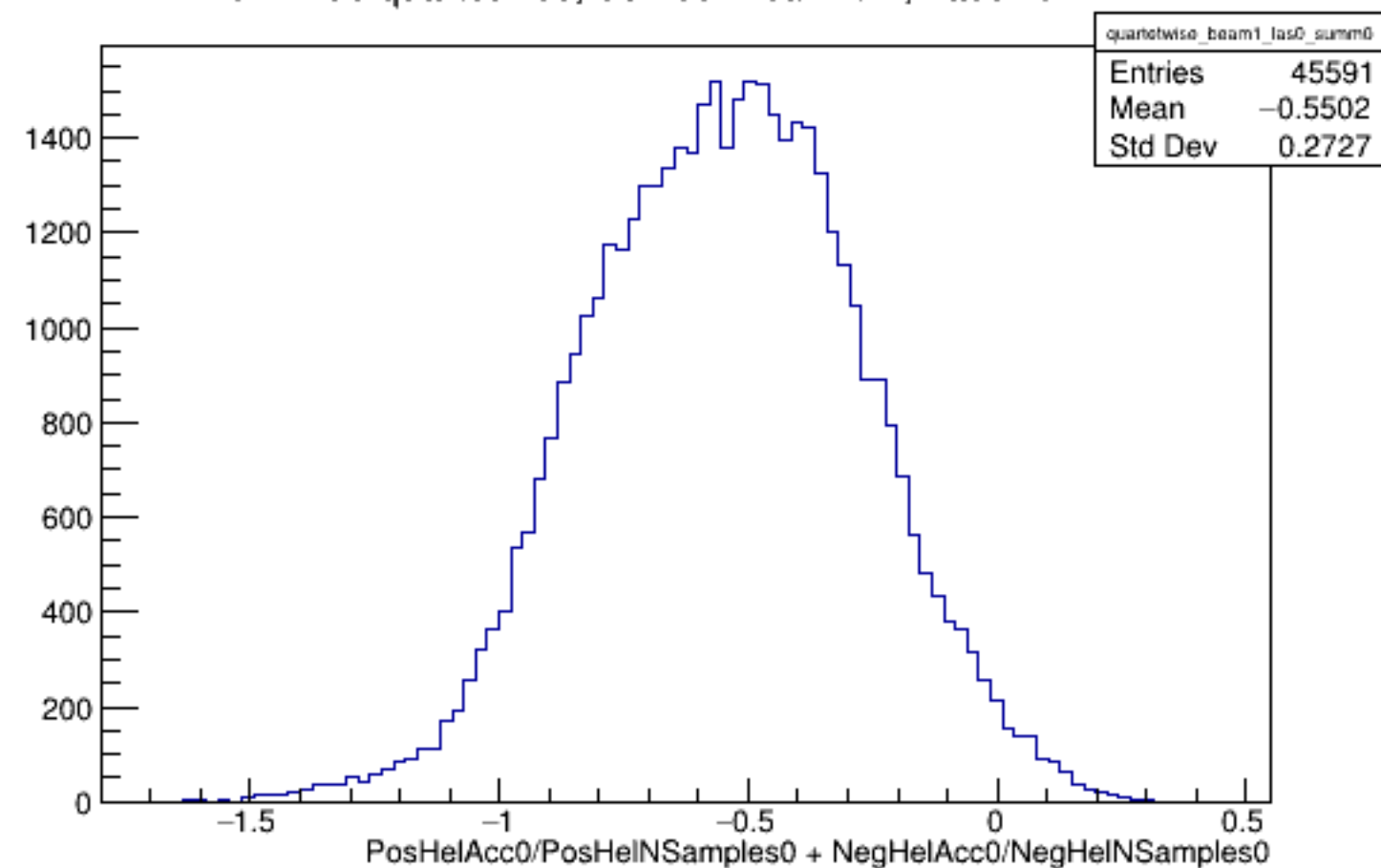
Run 4496 quartetwise, Sums0: Beam ON, Laser OFF
