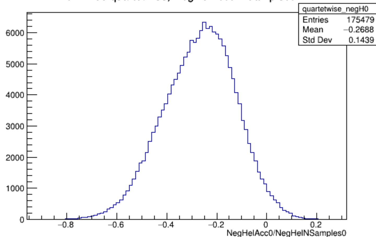
Run 4496 quartetwise, NegHelAcc0/NSamples0: All
