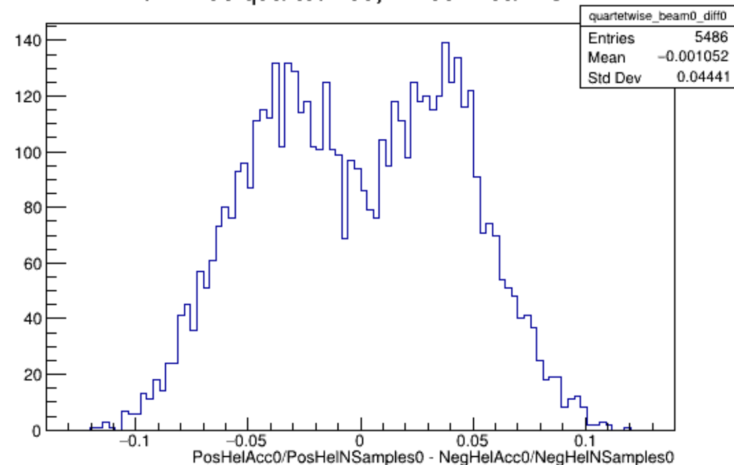
Run 4496 quartetwise, Diffs0: Beam OFF
