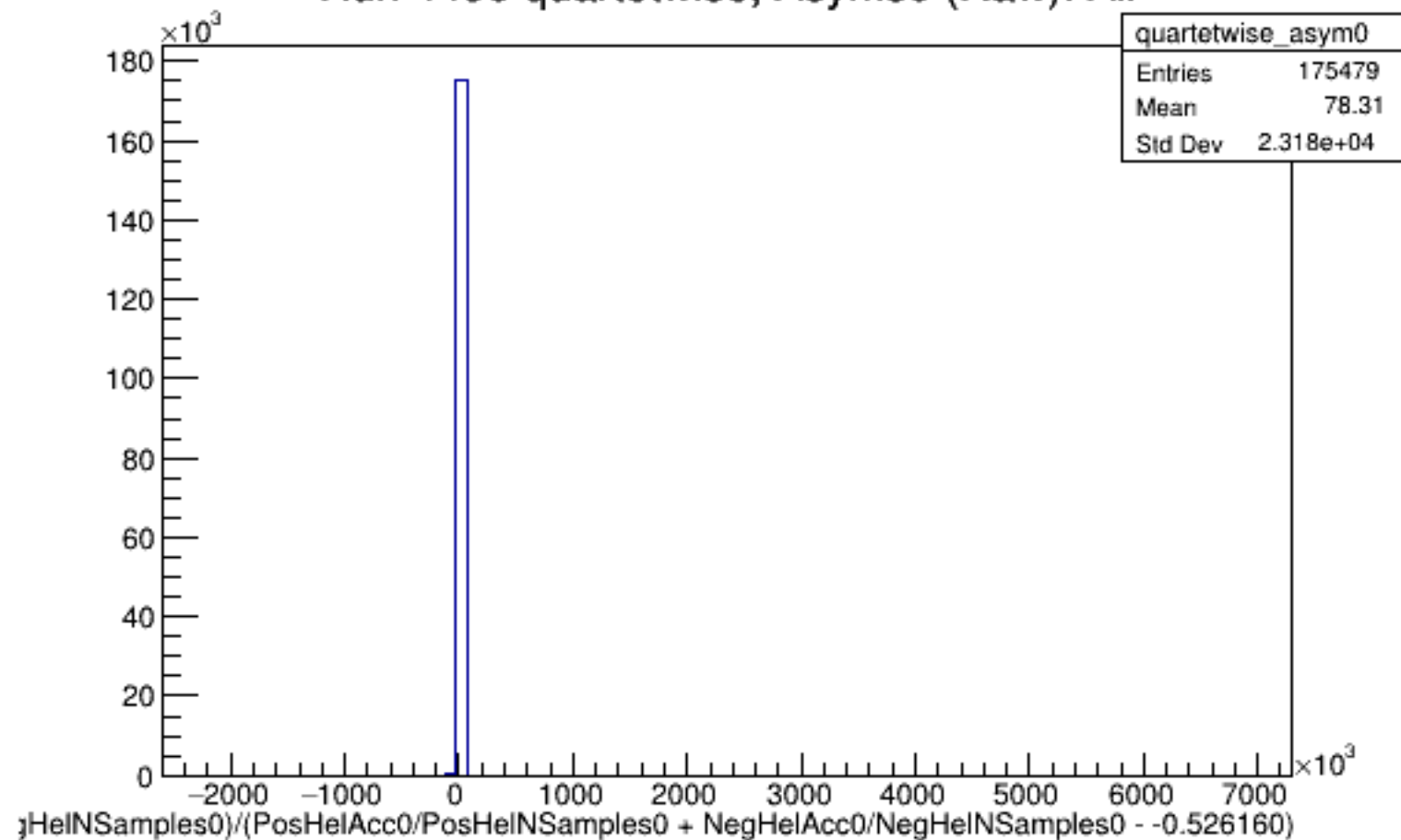
Run 4496 quartetwise, Asyms0 (Raw): All
