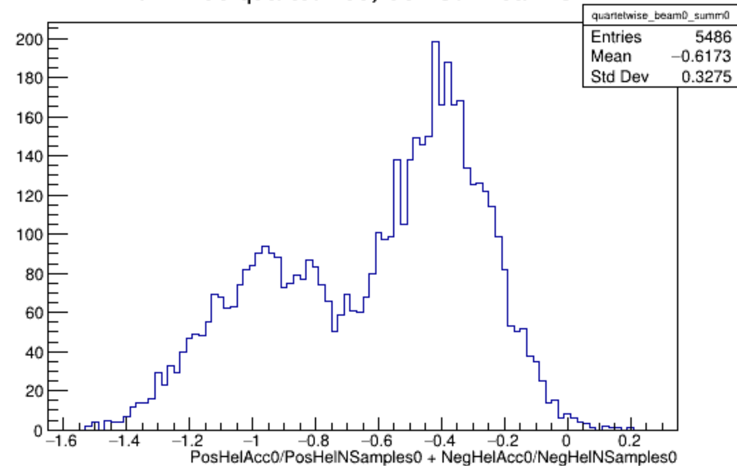
Run 4496 quartetwise, Sums0: Beam OFF
