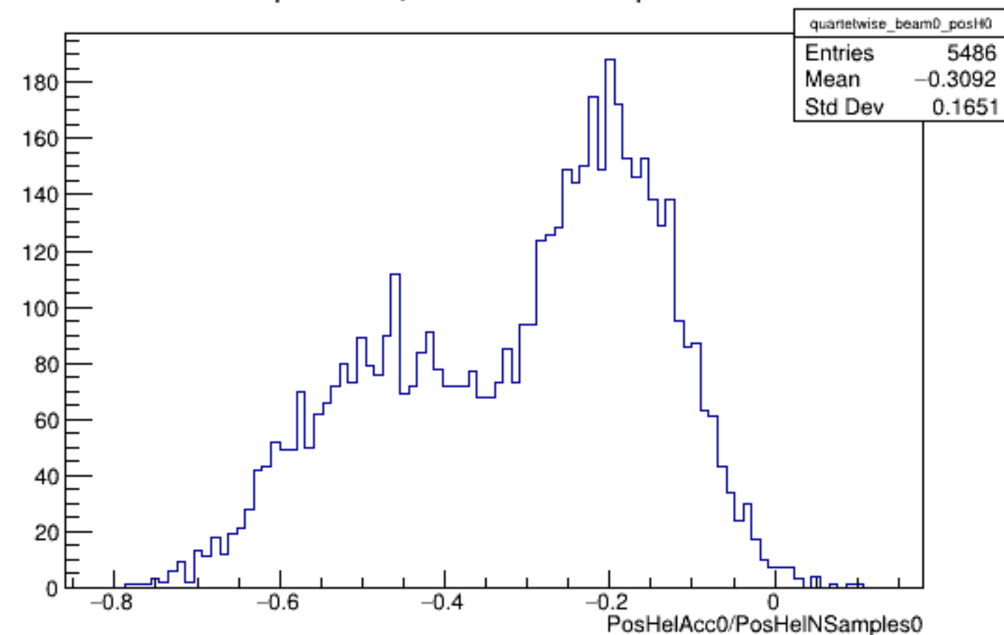
Run 4496 quartetwise, PosHelAcc0/NSamples0: Beam OFF
