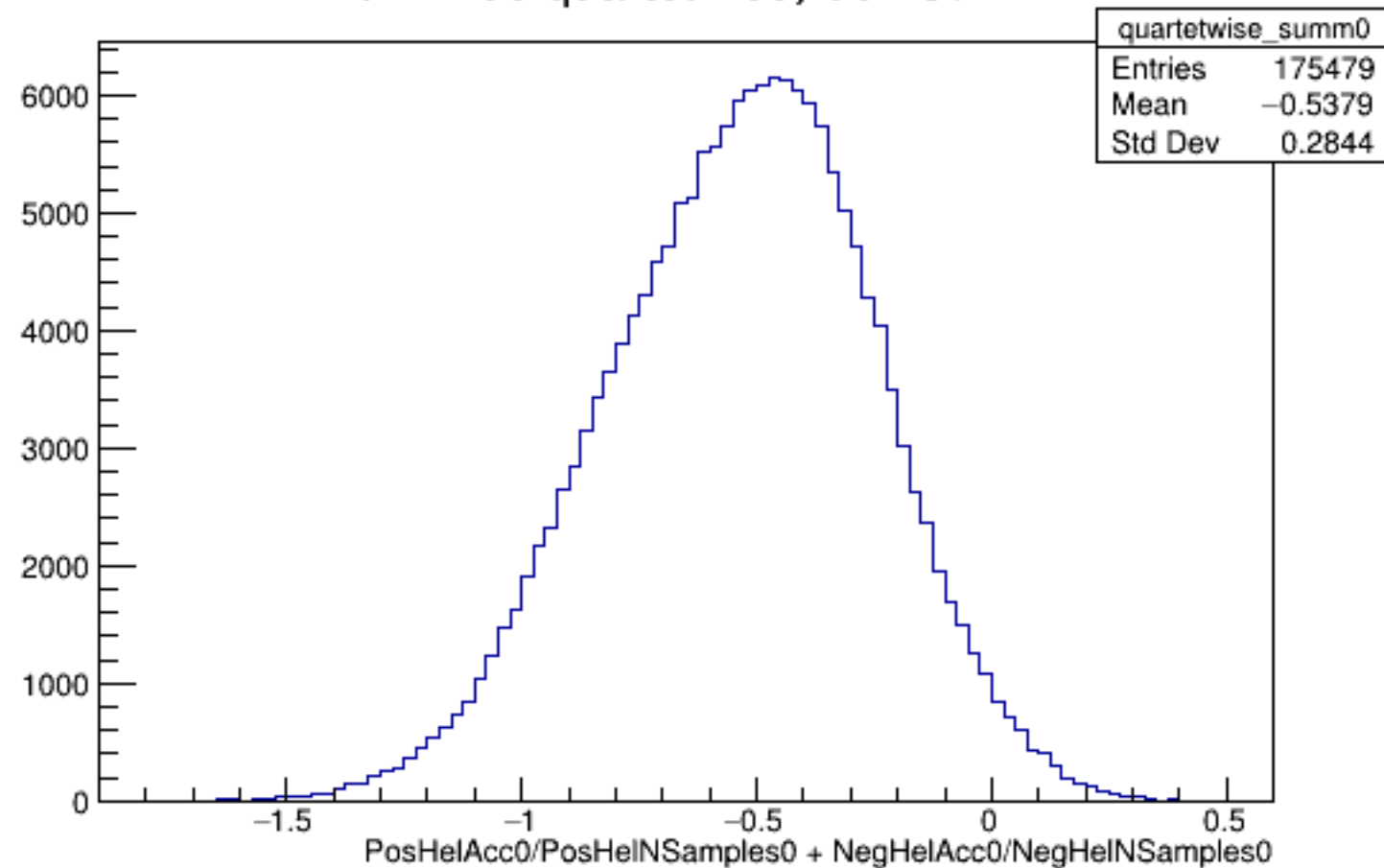
Run 4496 quartetwise, Sums0: All
