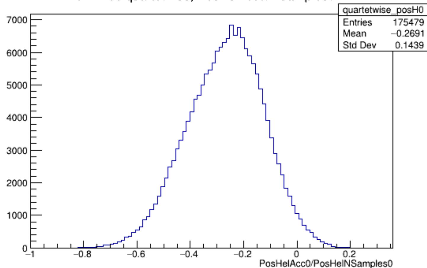
Run 4496 quartetwise, PosHelAcc0/NSamples0: All
