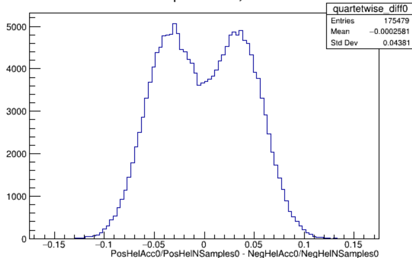
Run 4496 quartetwise, Diffs0: All
