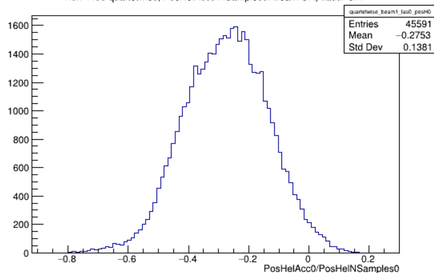
Run 4496 quartetwise, PosHelAcc0/NSamples0: Beam ON, Laser OFF
