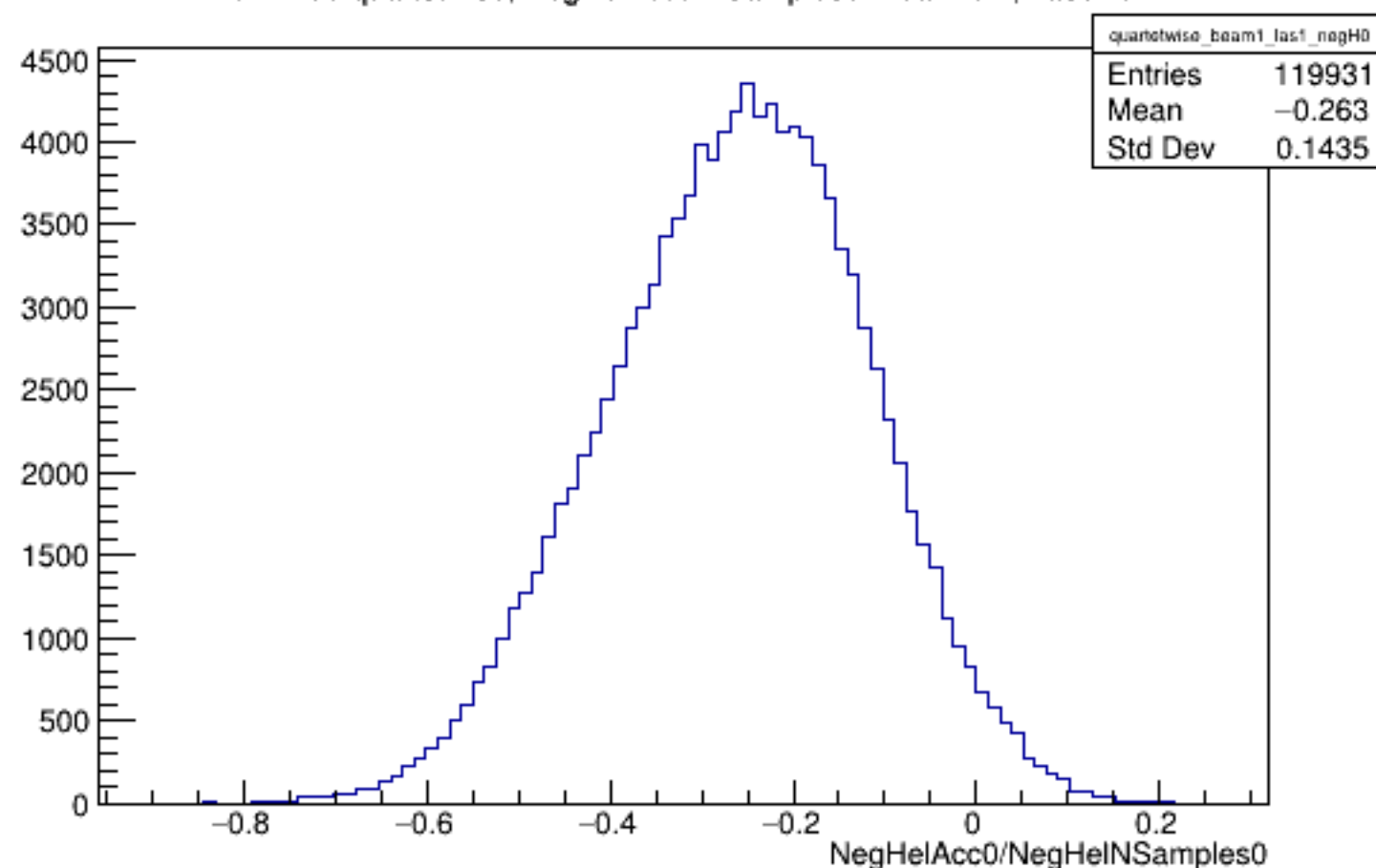
Run 4496 quartetwise, NegHelAcc0/NSamples0: Beam ON, Laser ON
