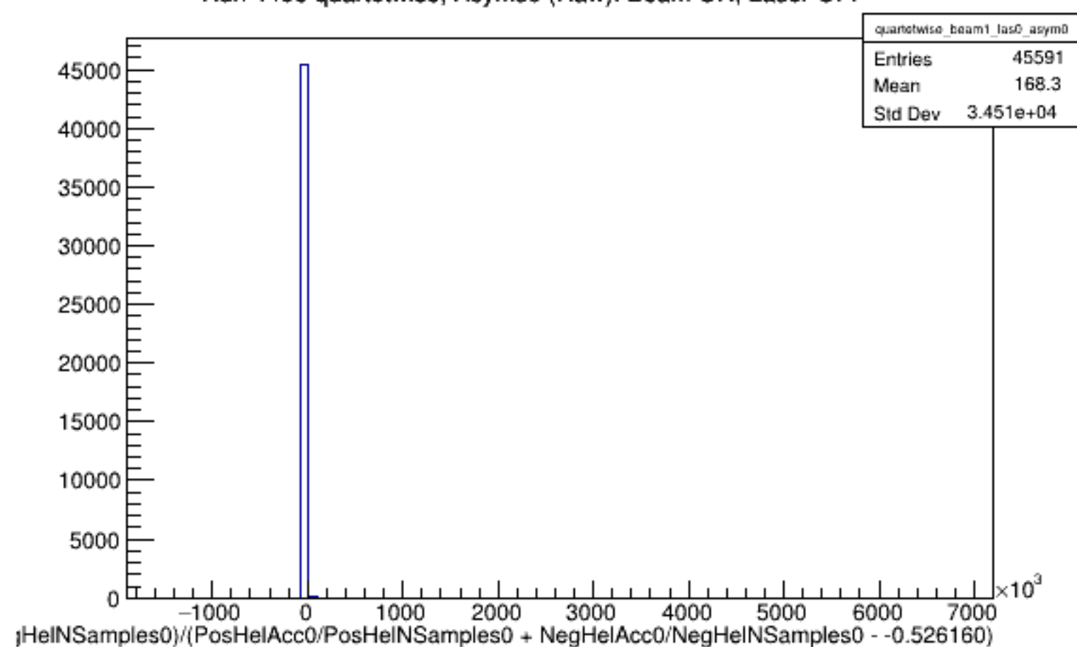
Run 4496 quartetwise, Asyms0 (Raw): Beam ON, Laser OFF
