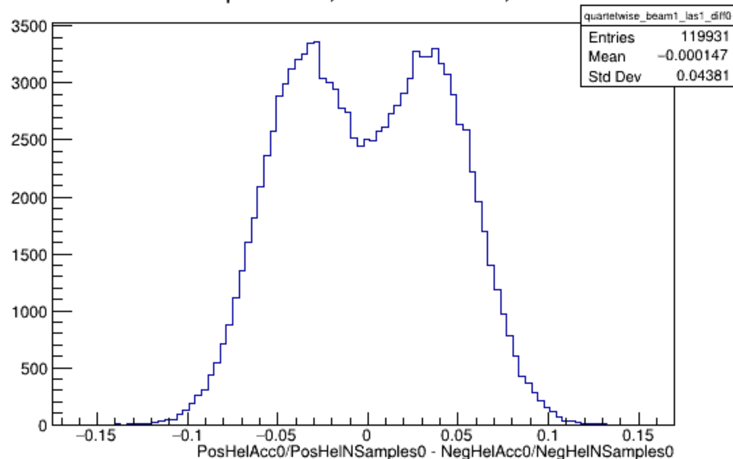
Run 4496 quartetwise, Diffs0: Beam ON, Laser ON
