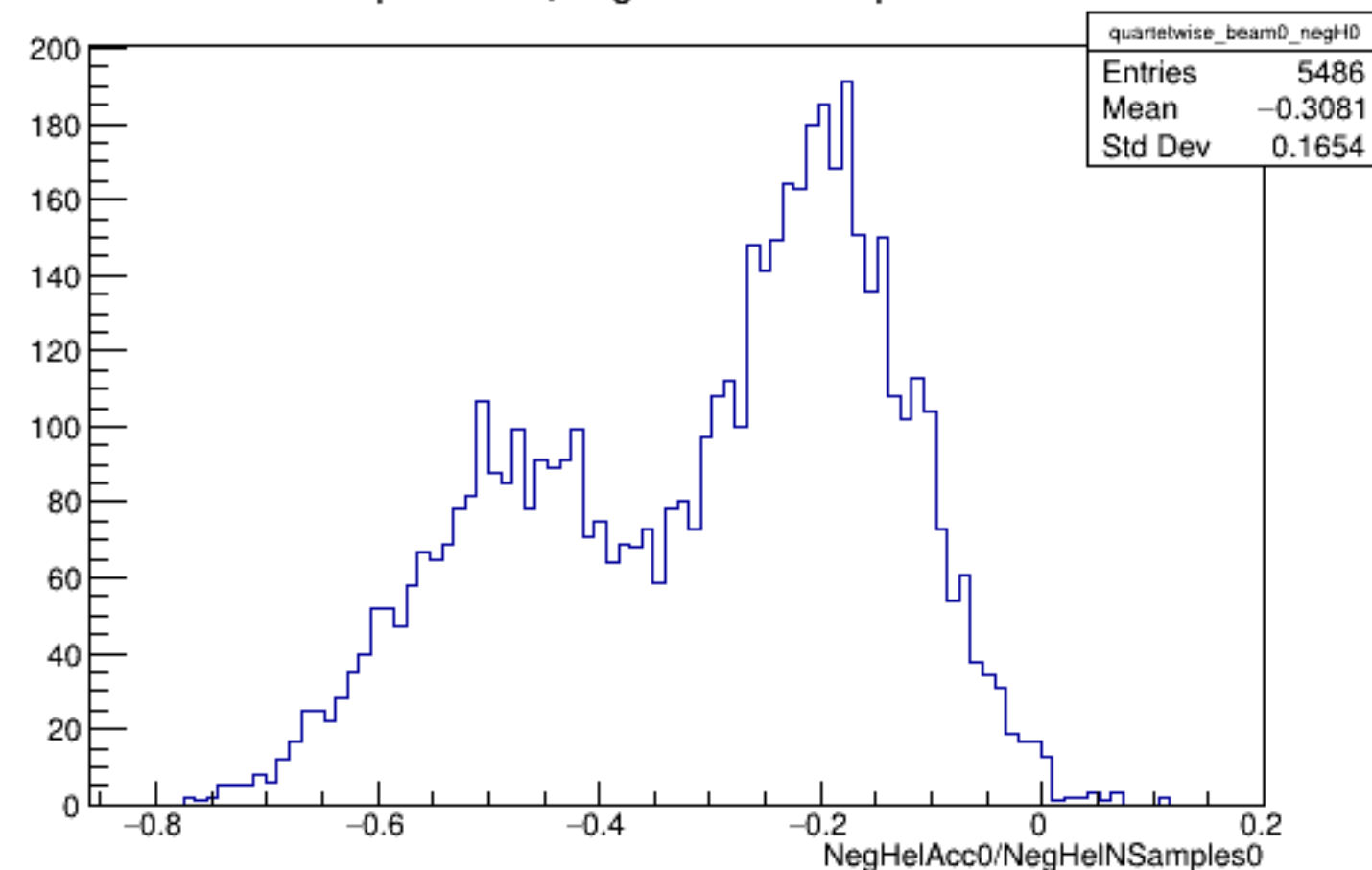
Run 4496 quartetwise, NegHelAcc0/NSamples0: Beam OFF
