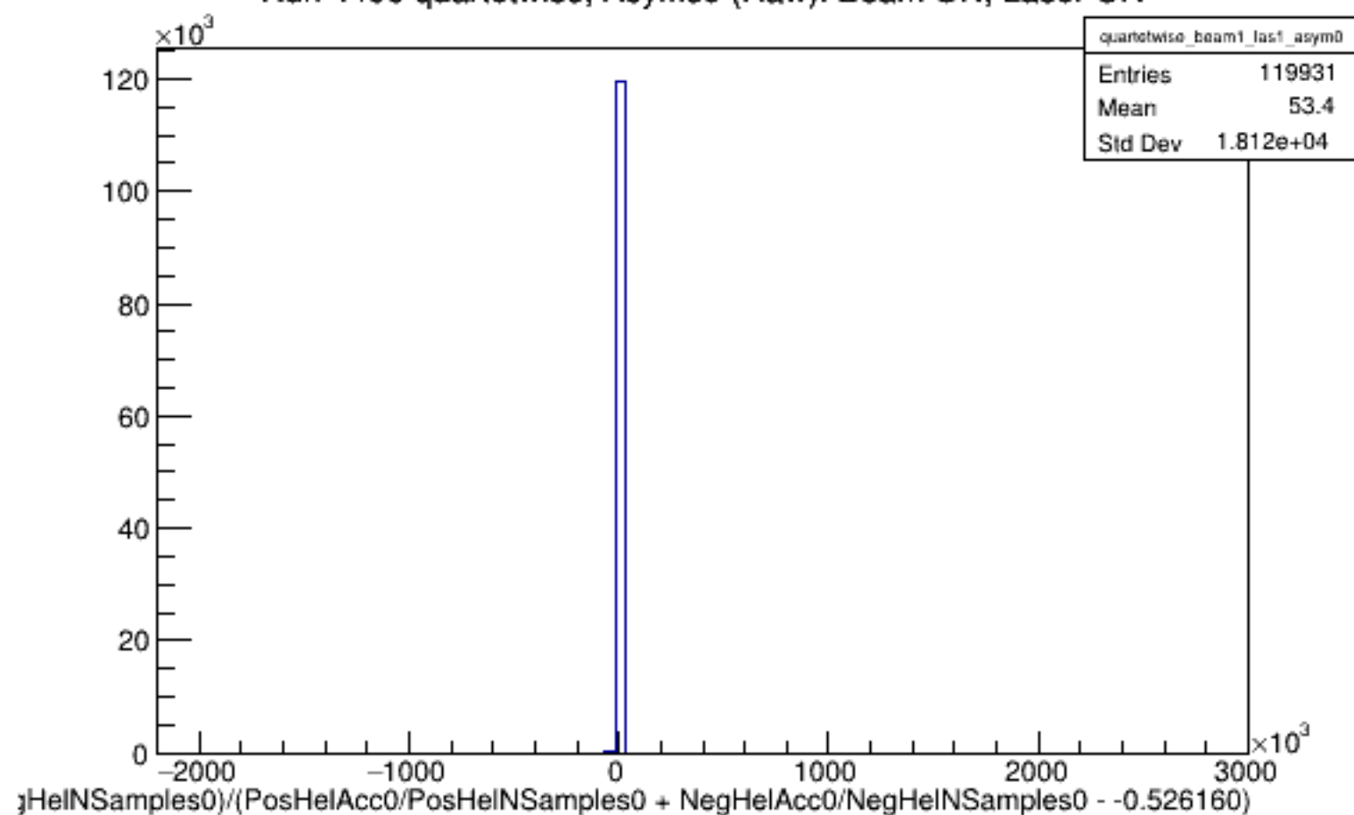
Run 4496 quartetwise, Asyms0 (Raw): Beam ON, Laser ON
