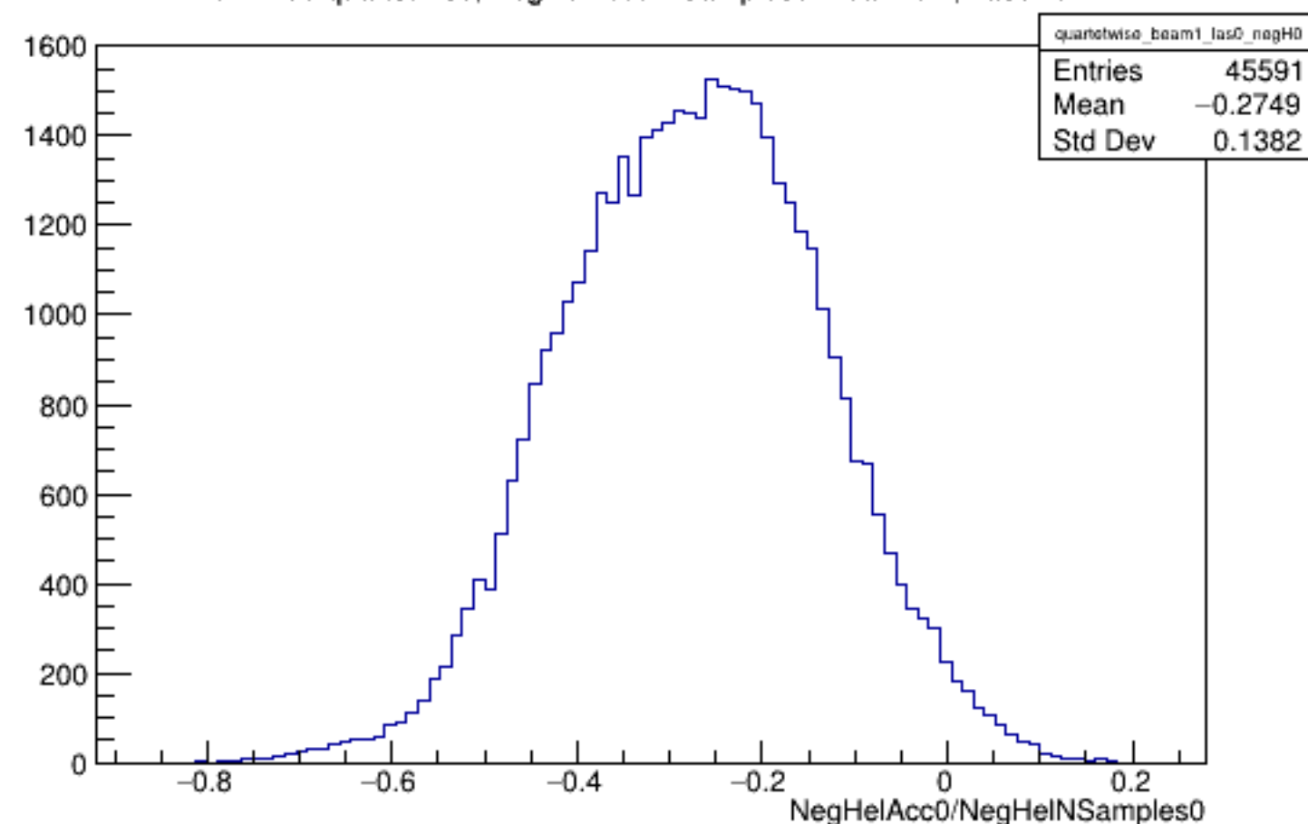
Run 4496 quartetwise, NegHelAcc0/NSamples0: Beam ON, Laser OFF
