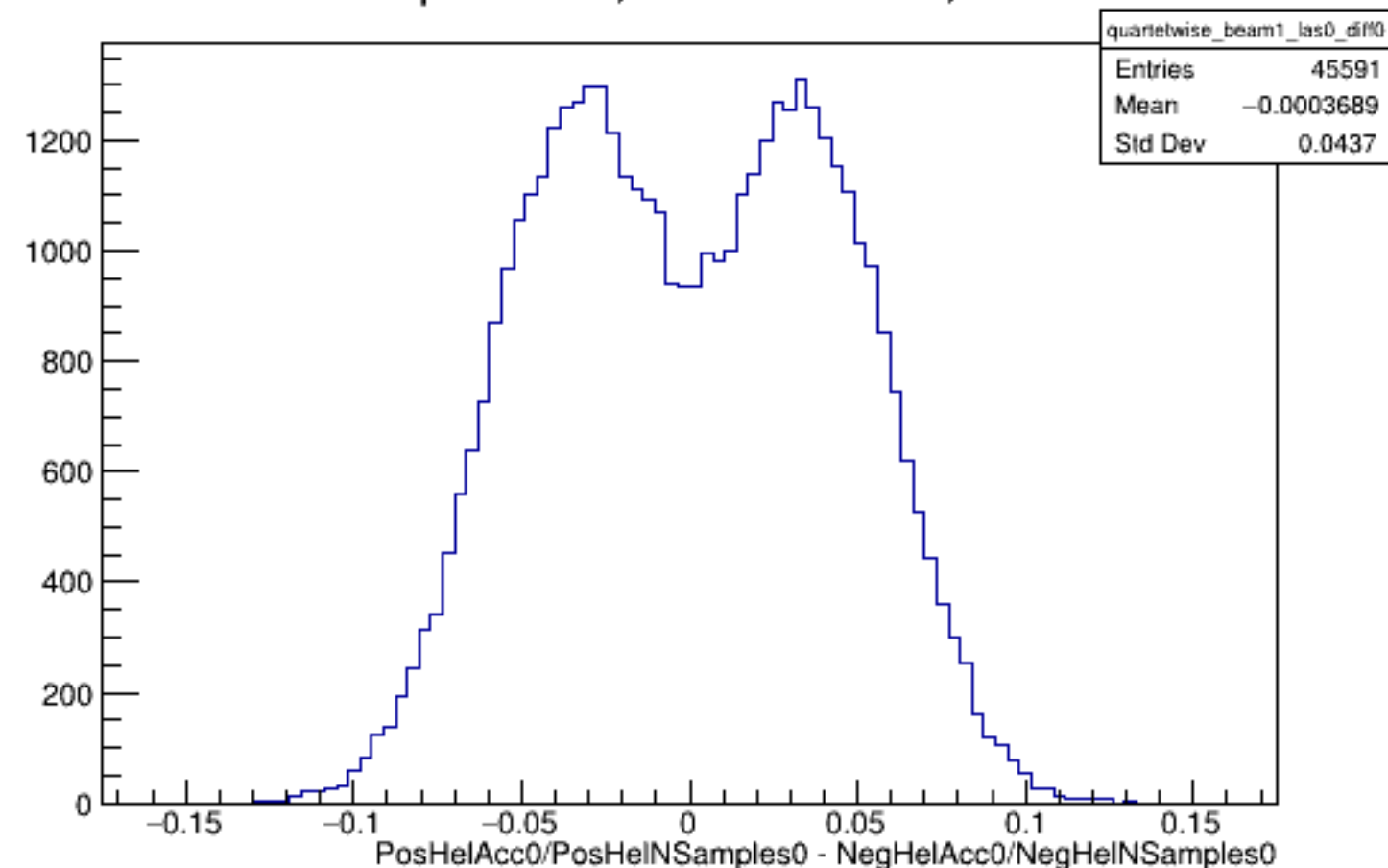
Run 4496 quartetwise, Diffs0: Beam ON, Laser OFF
