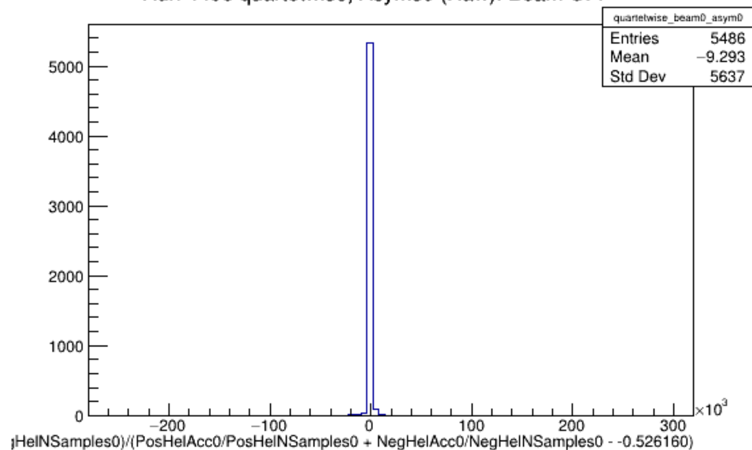
Run 4496 quartetwise, Asyms0 (Raw): Beam OFF
