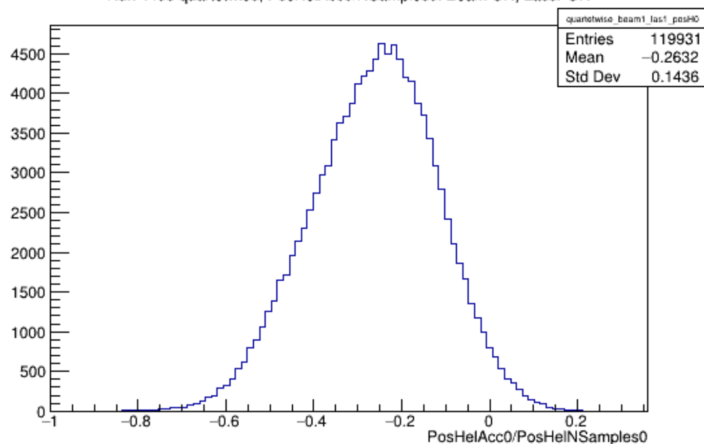
Run 4496 quartetwise, PosHelAcc0/NSamples0: Beam ON, Laser ON
