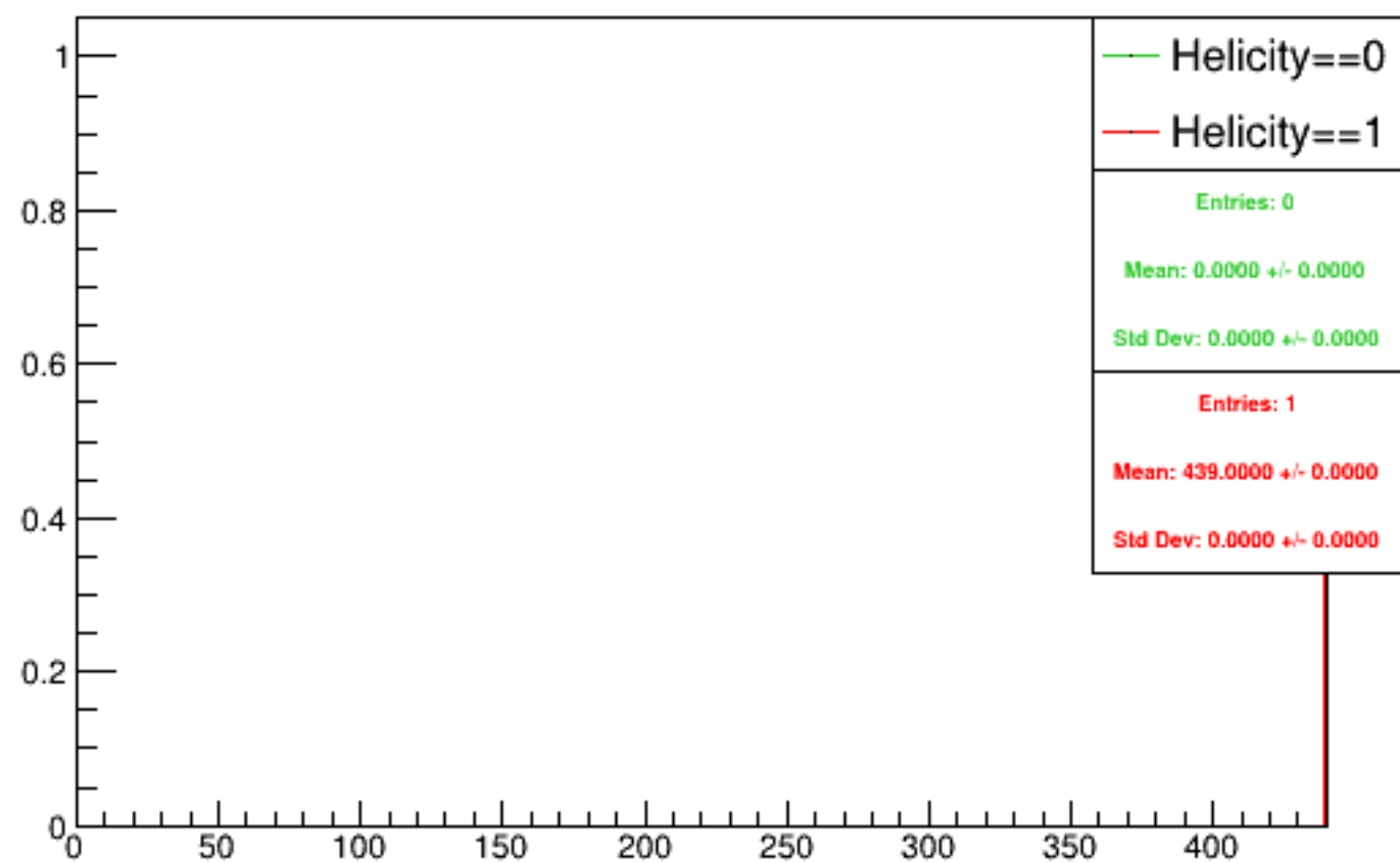
Run 4496 triggerwise, sums: Beam ON, Laser ON
