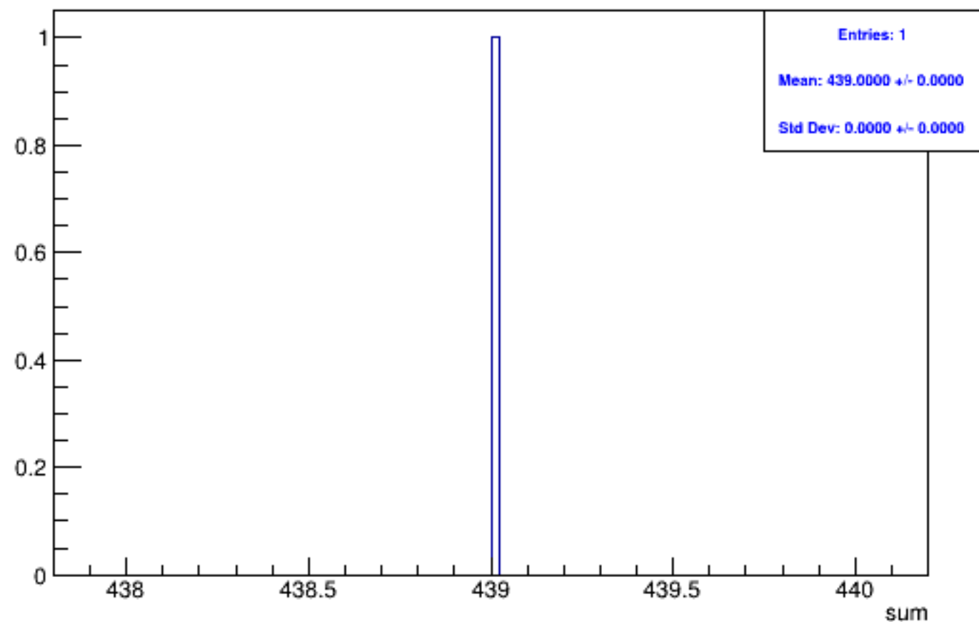
Run 4496 triggerwise, sums: All
