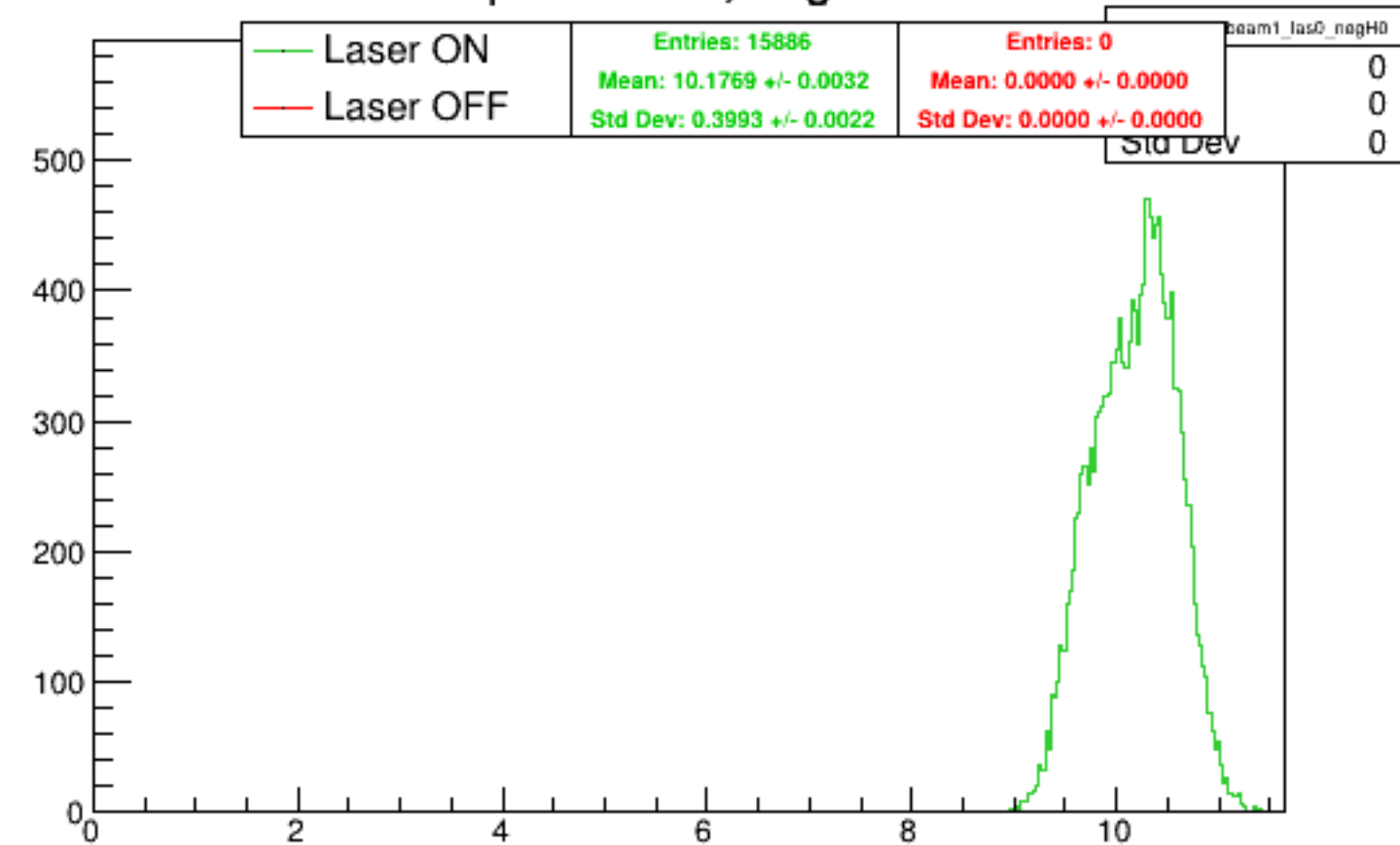
Run 4502 quartetwise, negH0: Beam ON
