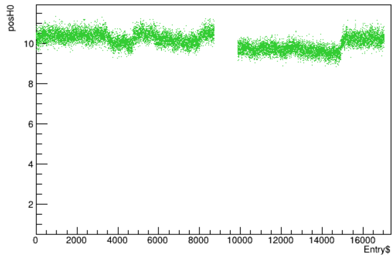
Run 4502 quartetwise, posH0 vs time
