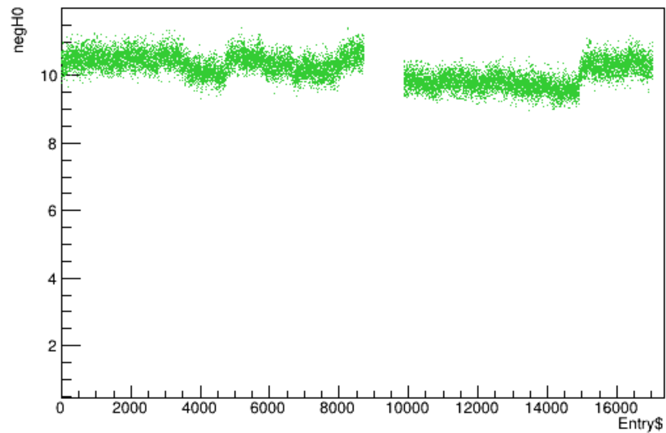
Run 4502 quartetwise, negH0 vs time
