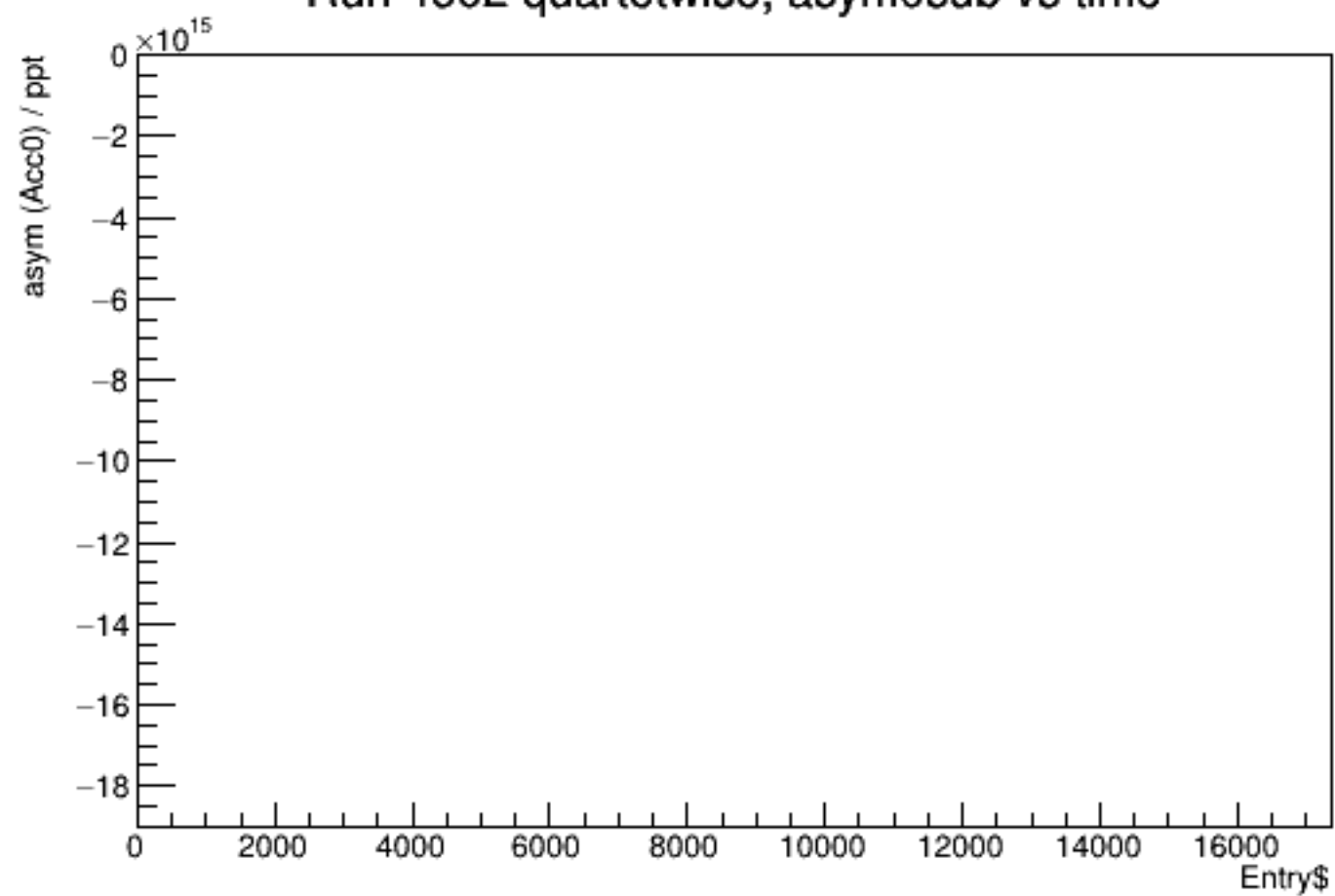
Run 4502 quartetwise, asym0sub vs time
