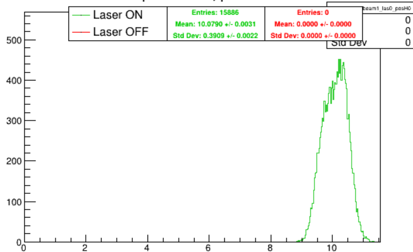
Run 4502 quartetwise, posH0: Beam ON
