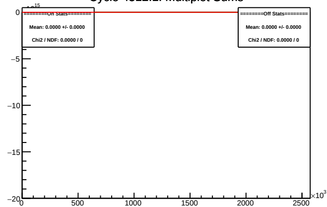
Cycle 4512.1: Multiplet Sums
