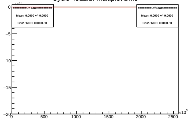
Cycle 4512.1: Multiplet Diffs
