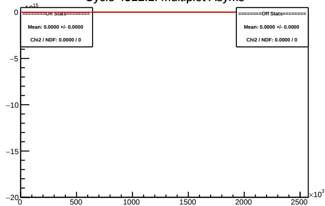
Cycle 4512.1: Multiplet Asyms
