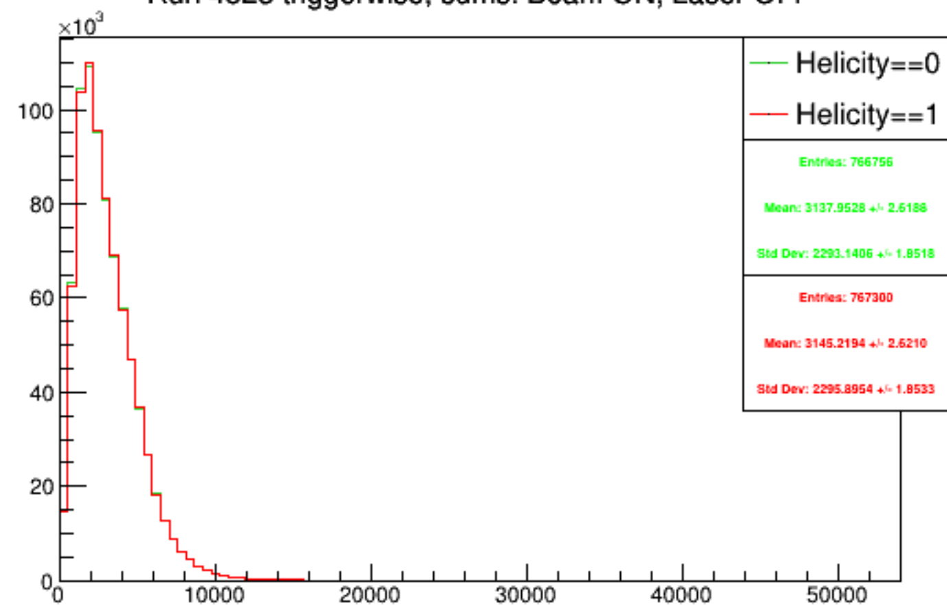
Run 4523 triggerwise, sums: Beam ON, Laser OFF
