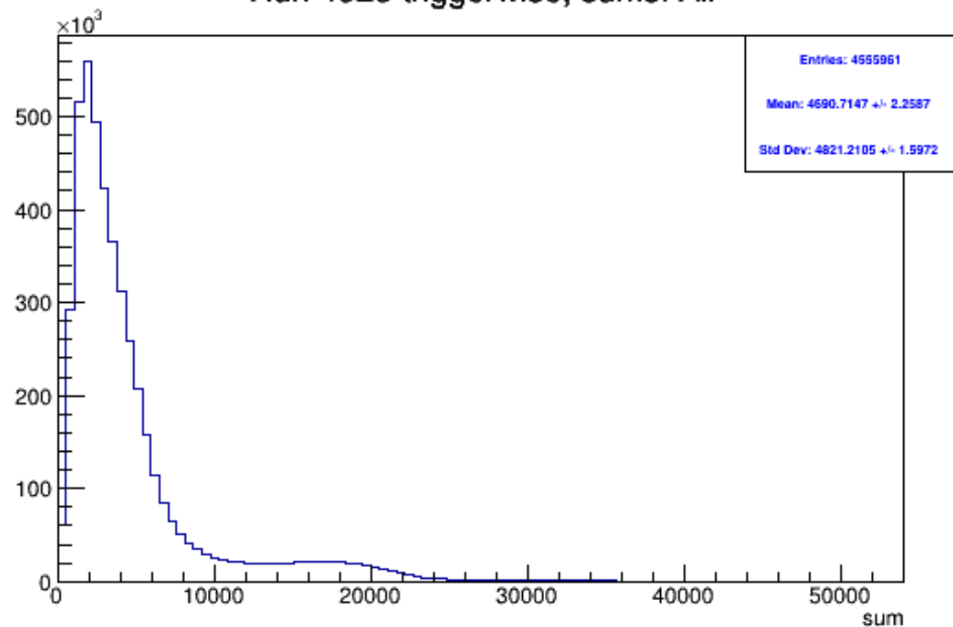
Run 4523 triggerwise, sums: All
