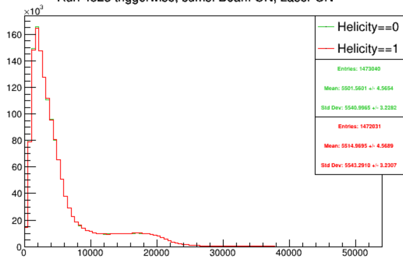
Run 4523 triggerwise, sums: Beam ON, Laser ON
