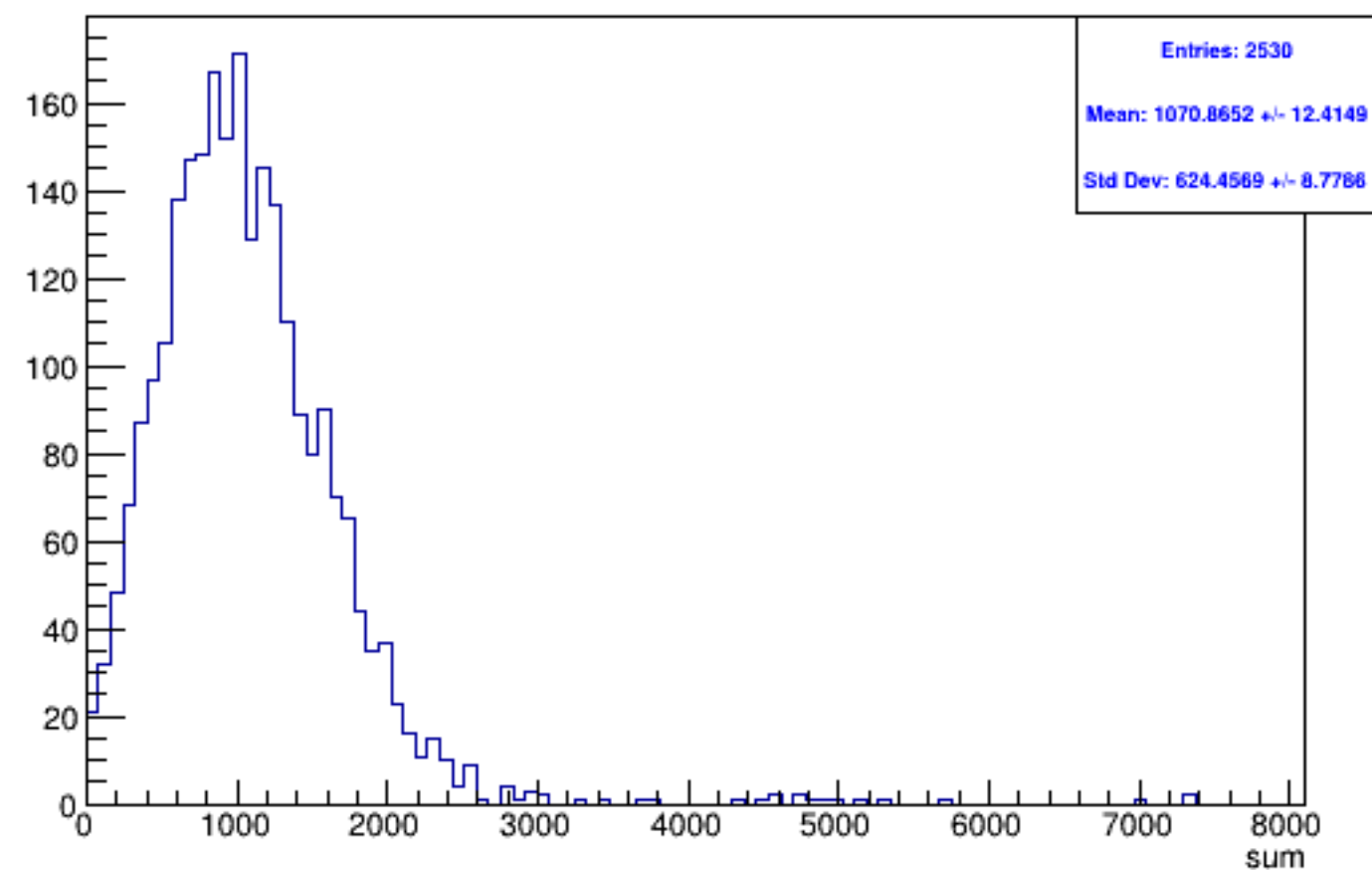
Run 4523 triggerwise, sums: Beam OFF
