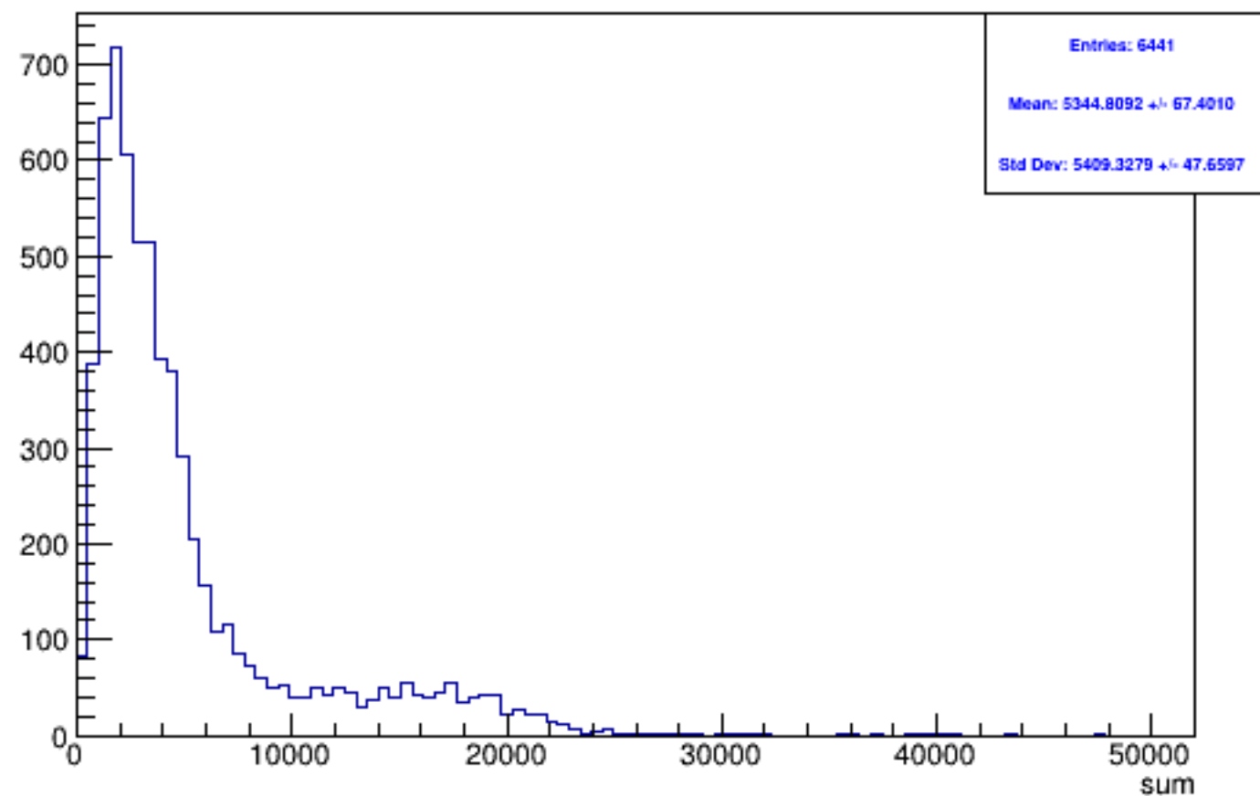
Run 4533 triggerwise, sums: All
