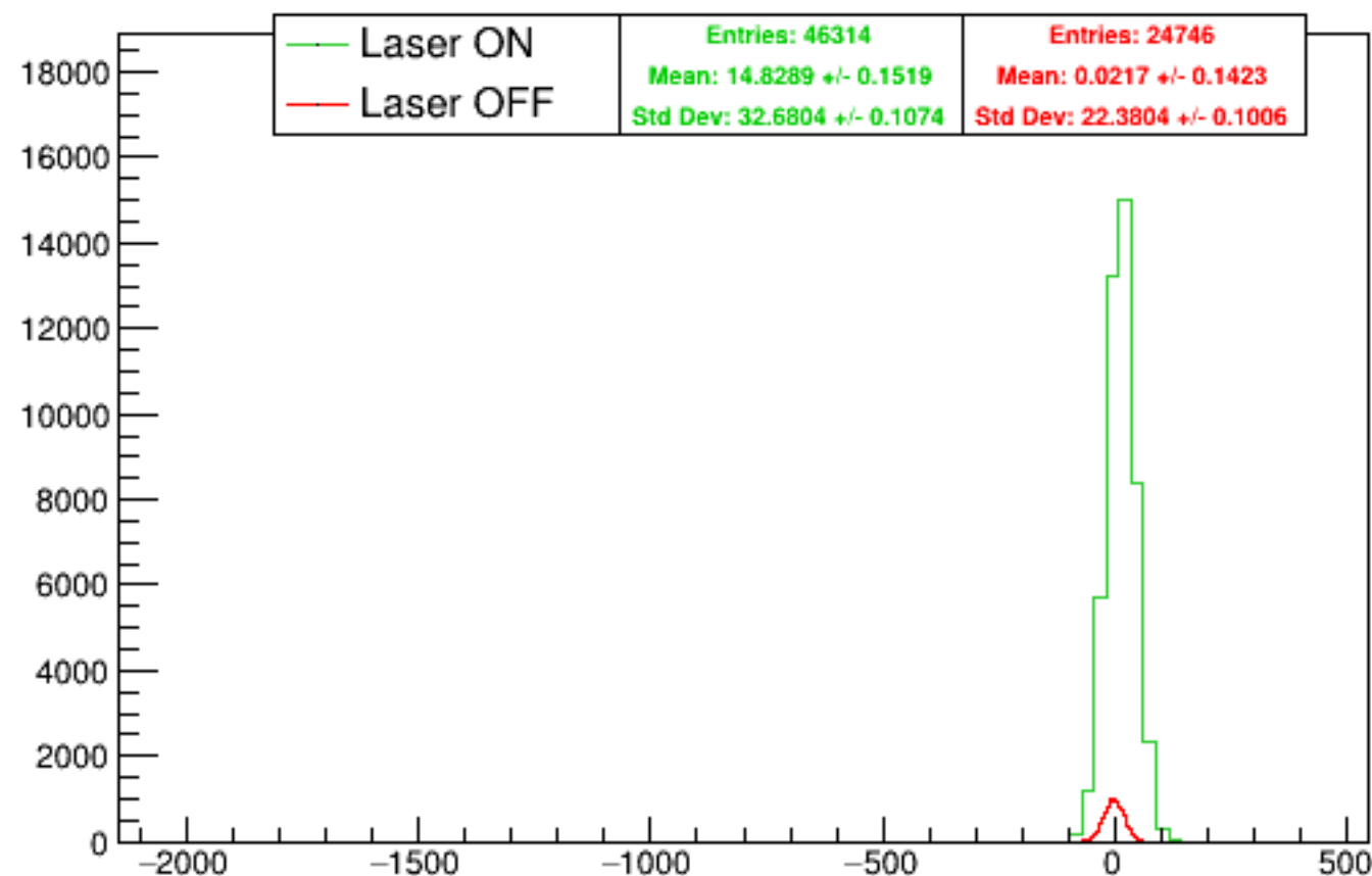
Run 4534 quartetwise, asym0sub: Beam ON
