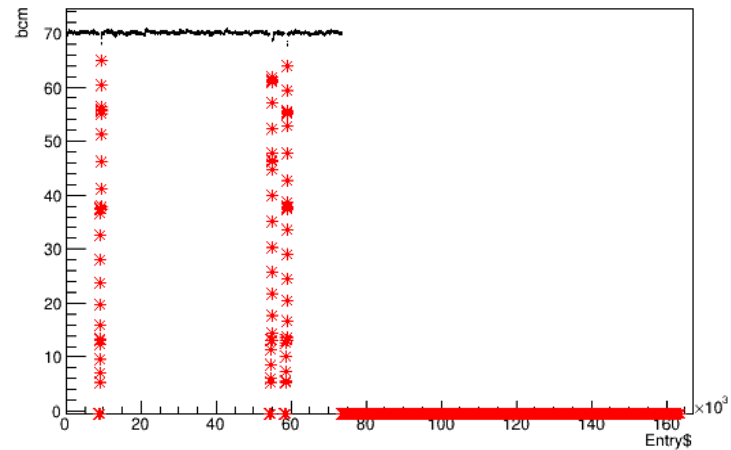
Run 4534 quartetwise, bcm vs time
