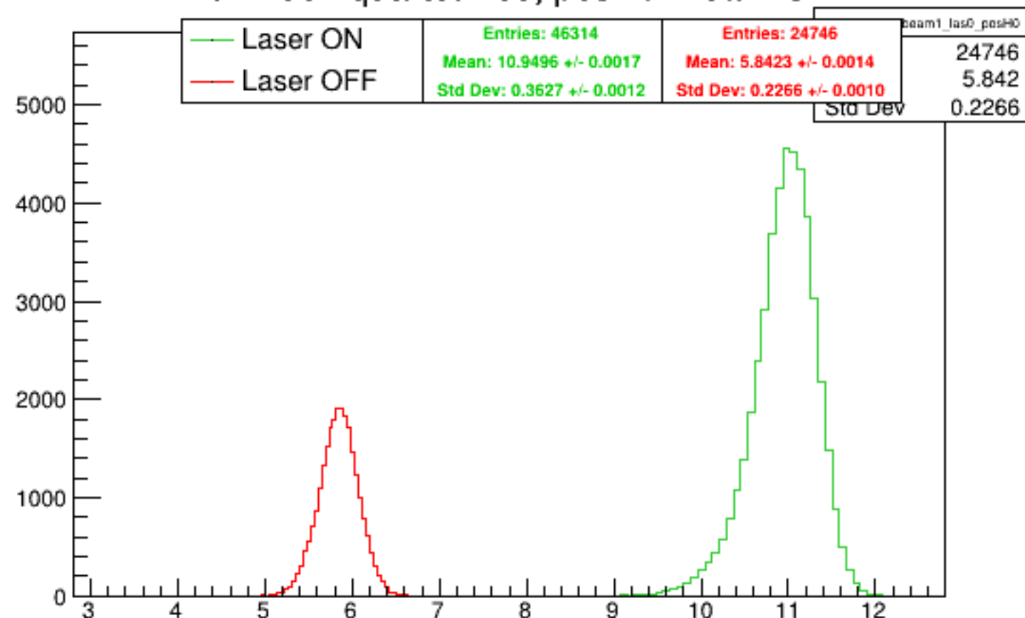
Run 4534 quartetwise, posH0: Beam ON
