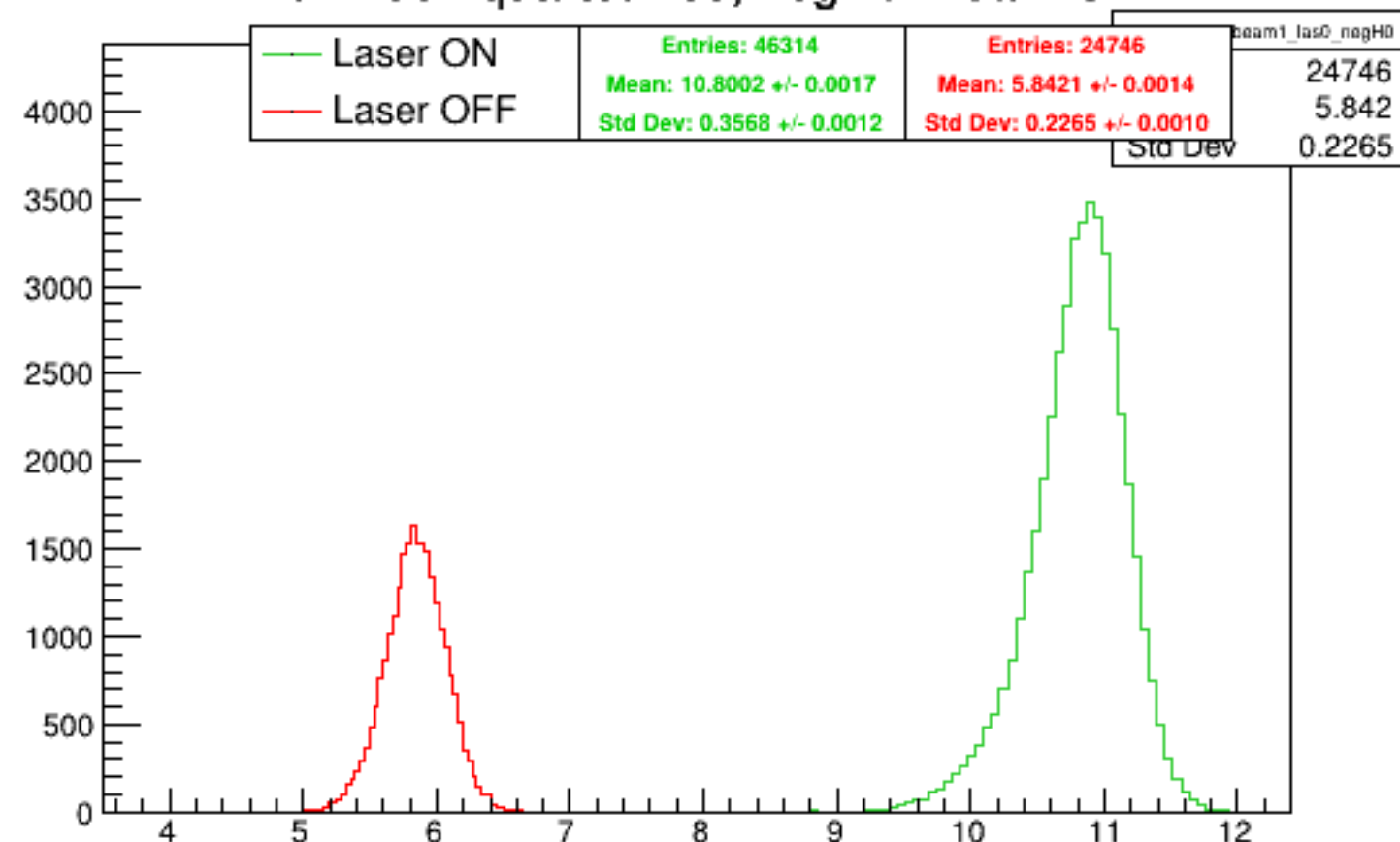
Run 4534 quartetwise, negH0: Beam ON
