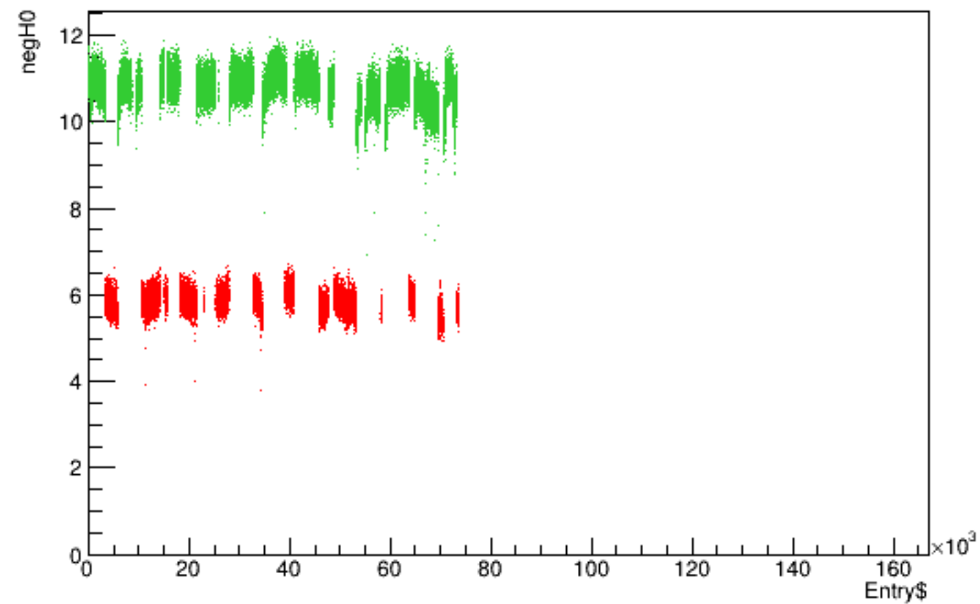
Run 4534 quartetwise, negH0 vs time
