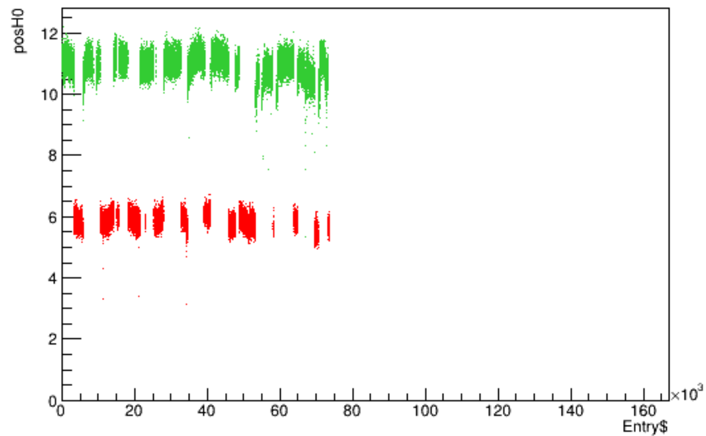
Run 4534 quartetwise, posH0 vs time
