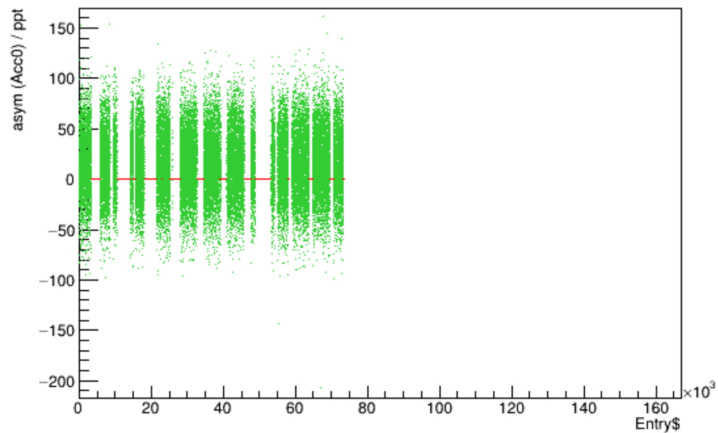
Run 4534 quartetwise, asym0sub vs time
