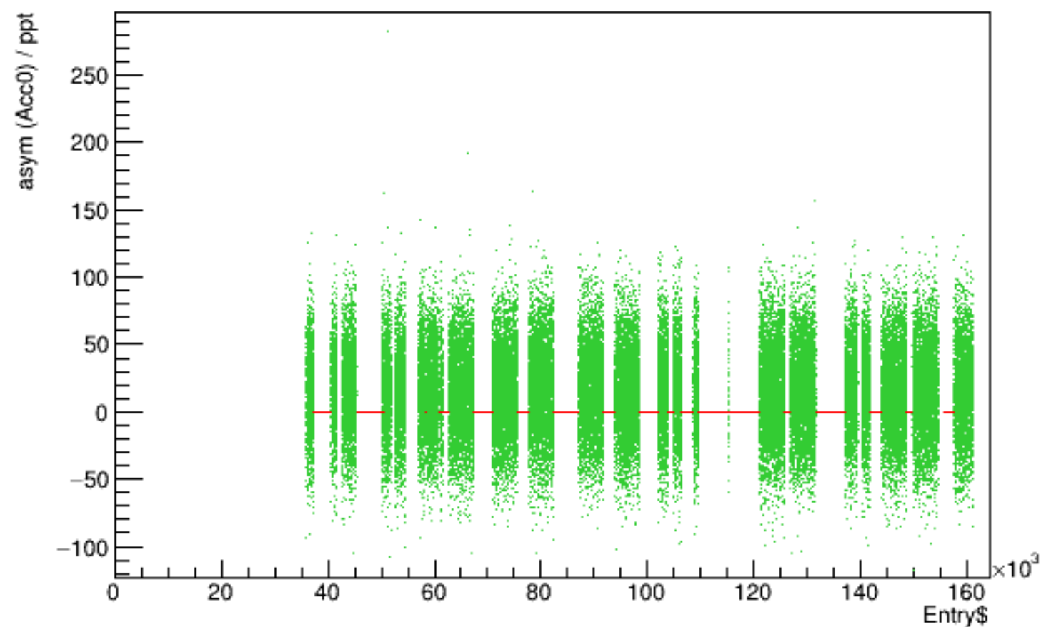
Run 4535 quartetwise, asym0sub vs time
