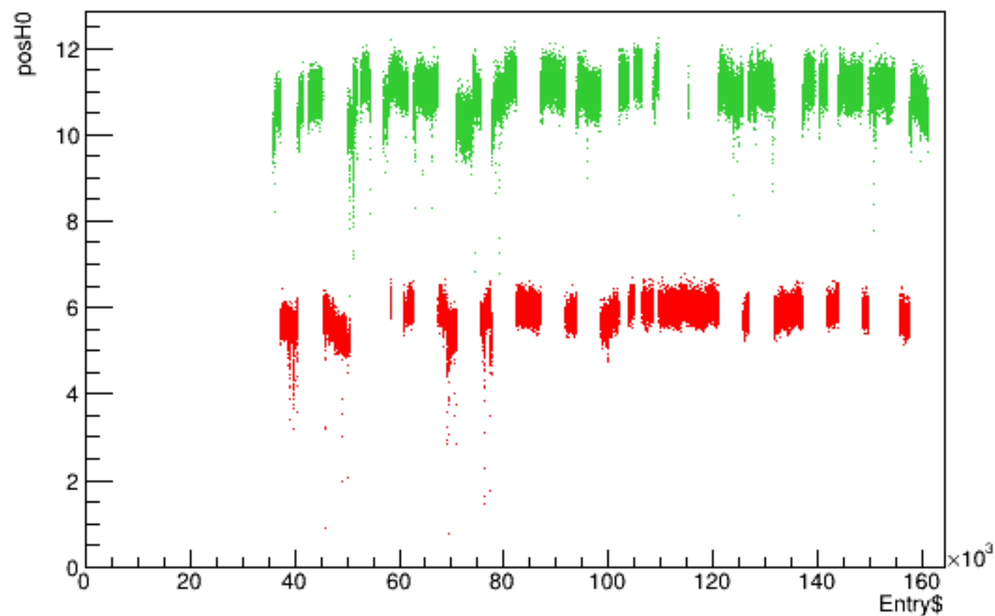
Run 4535 quartetwise, posH0 vs time
