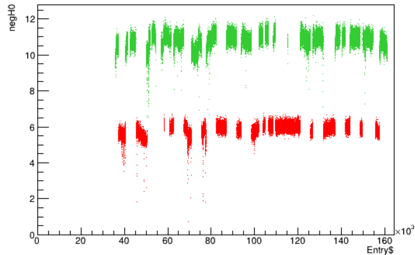
Run 4535 quartetwise, negH0 vs time
