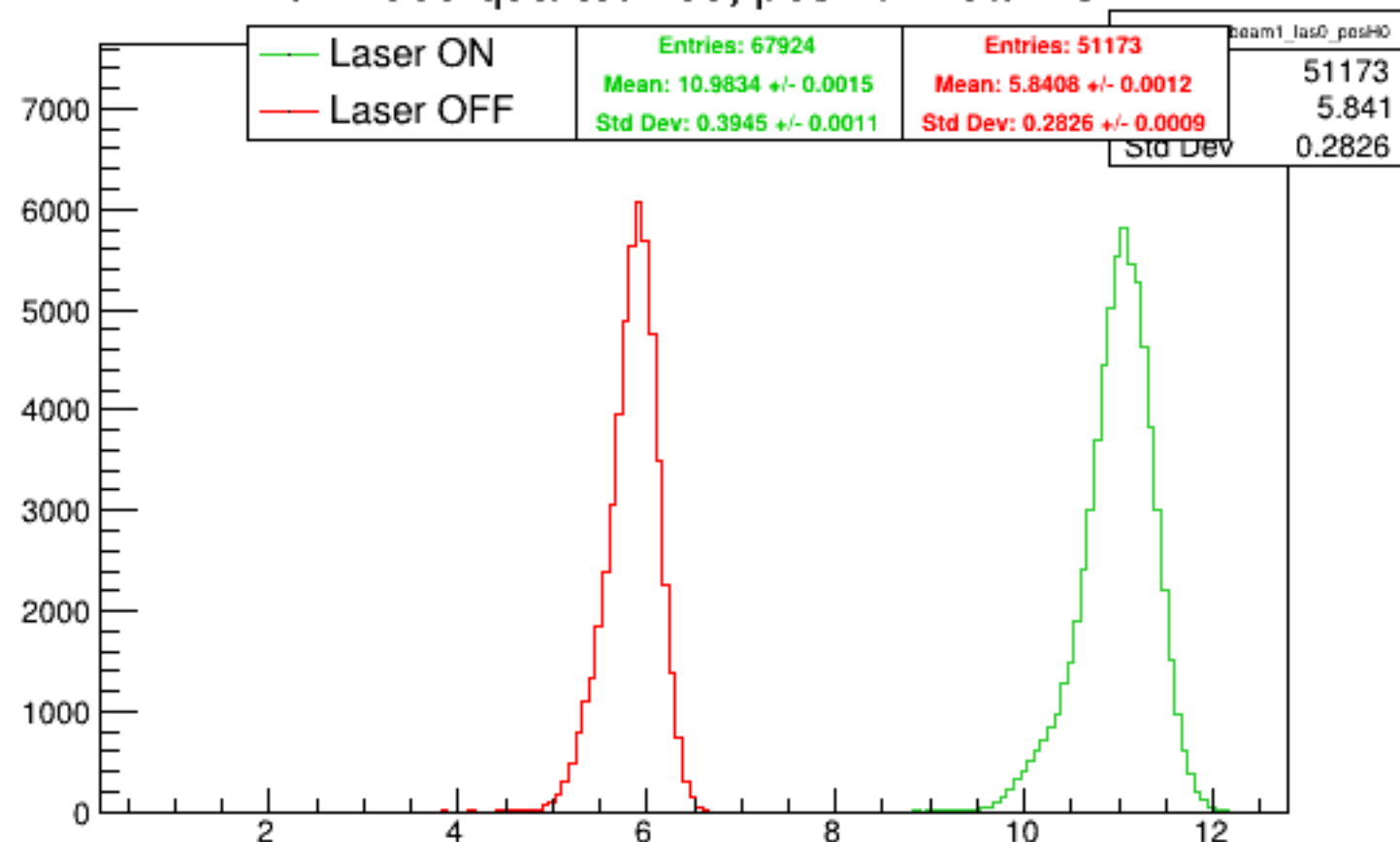
Run 4535 quartetwise, posH0: Beam ON
