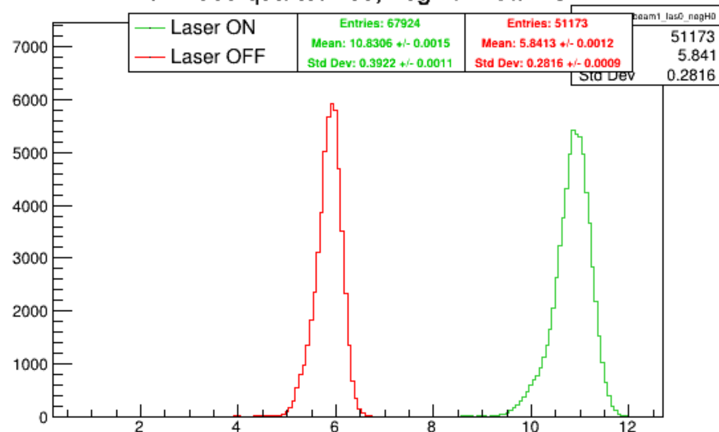
Run 4535 quartetwise, negH0: Beam ON
