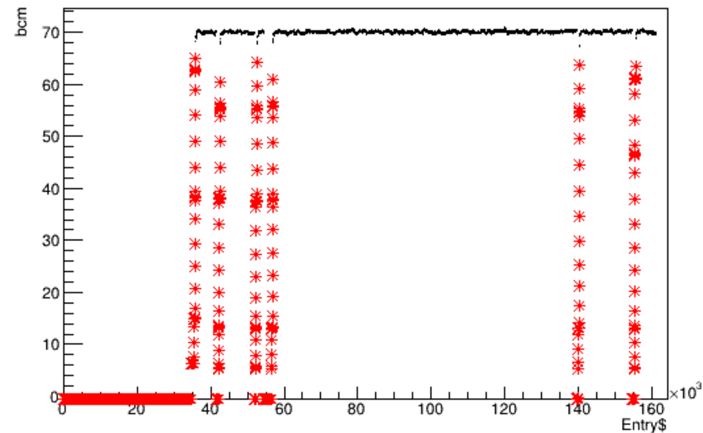
Run 4535 quartetwise, bcm vs time
