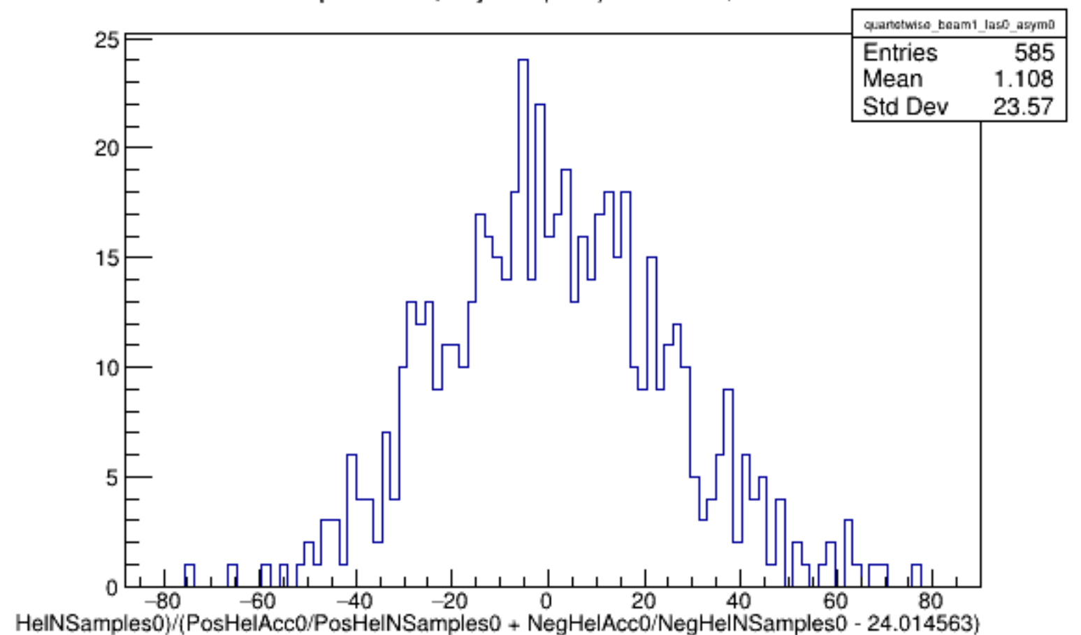
Run 4547 quartetwise, Asyms0 (Raw): Beam ON, Laser OFF
