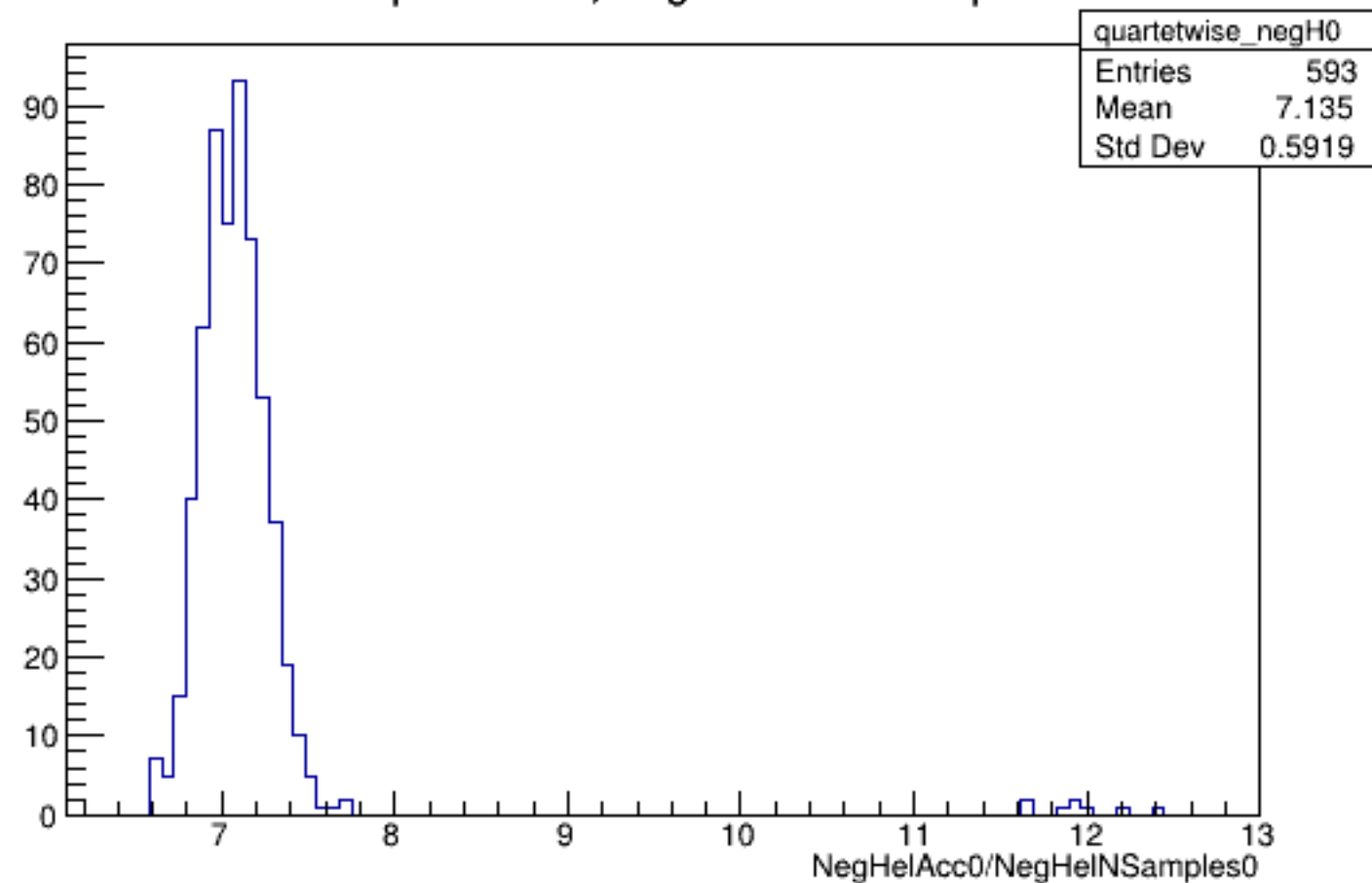
Run 4547 quartetwise, NegHelAcc0/NSamples0: All
