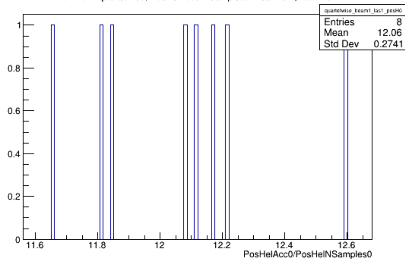
Run 4547 quartetwise, PosHelAcc0/NSamples0: Beam ON, Laser ON
