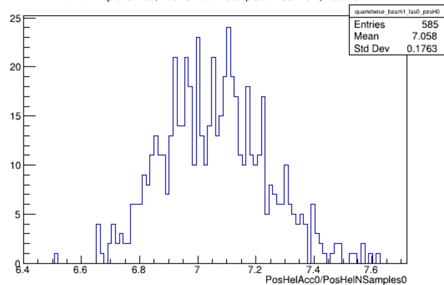
Run 4547 quartetwise, PosHelAcc0/NSamples0: Beam ON, Laser OFF
