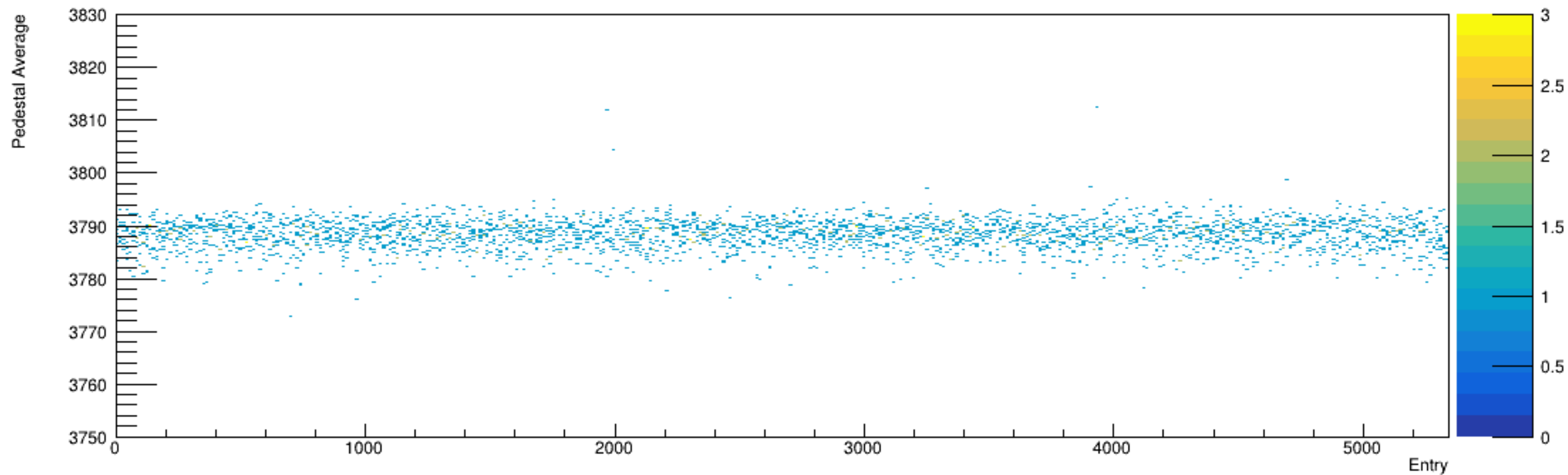
Run 4547, snapshots: Pedestal vs. Time
