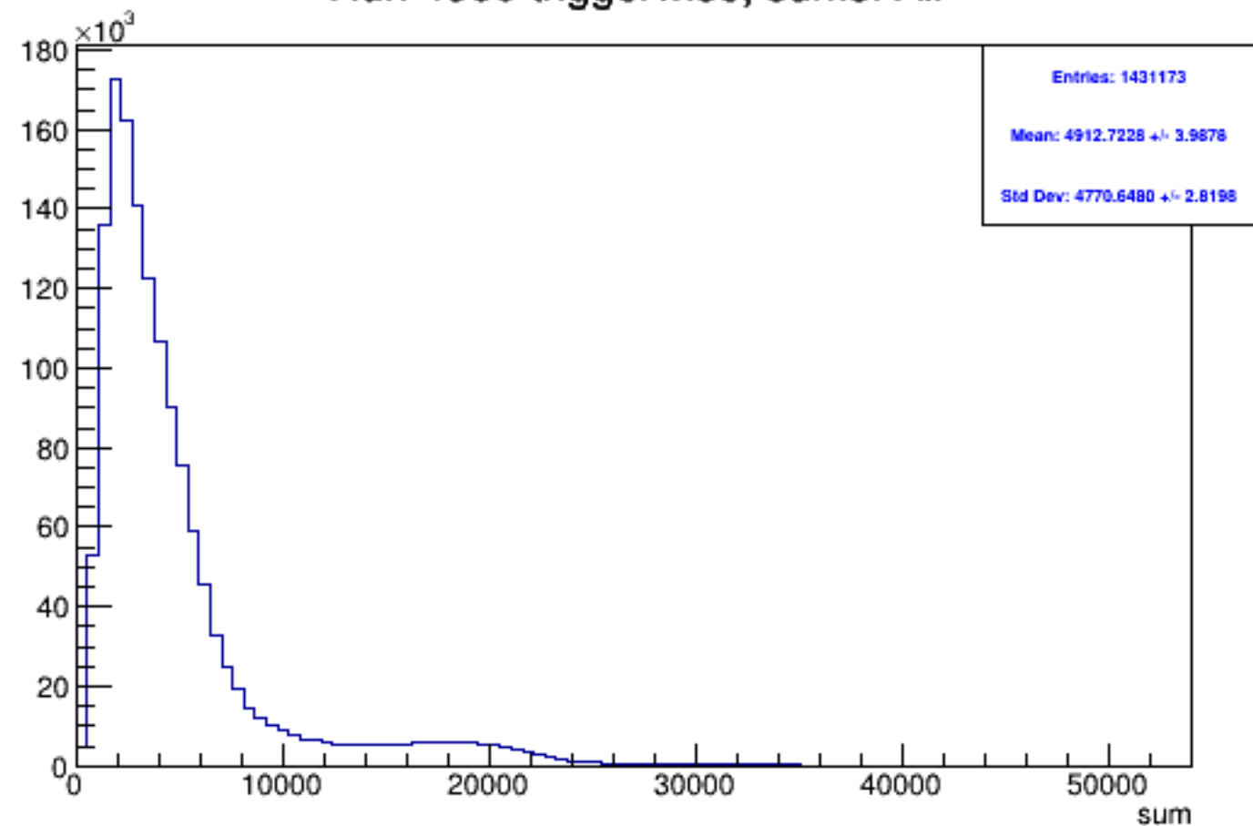
Run 4560 triggerwise, sums: All
