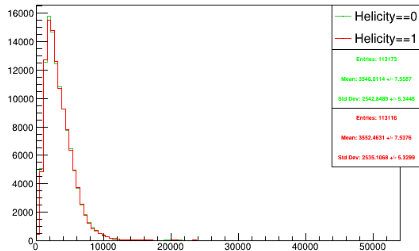
Run 4560 triggerwise, sums: Beam ON, Laser OFF
