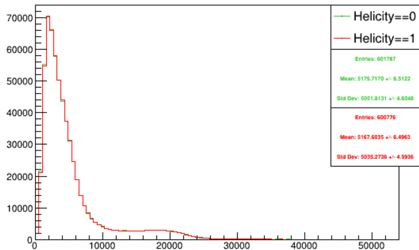
Run 4560 triggerwise, sums: Beam ON, Laser ON
