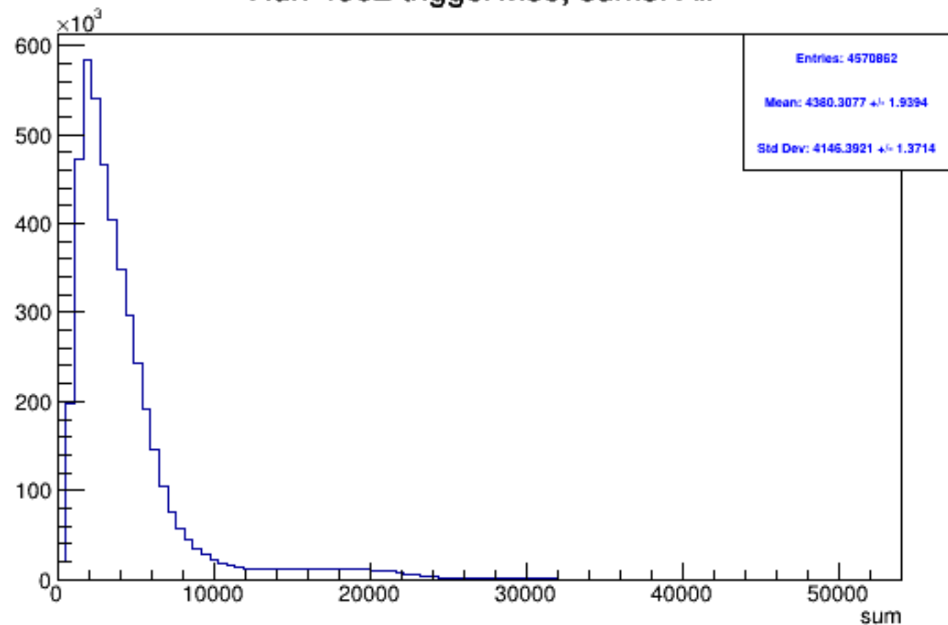
Run 4562 triggerwise, sums: All
