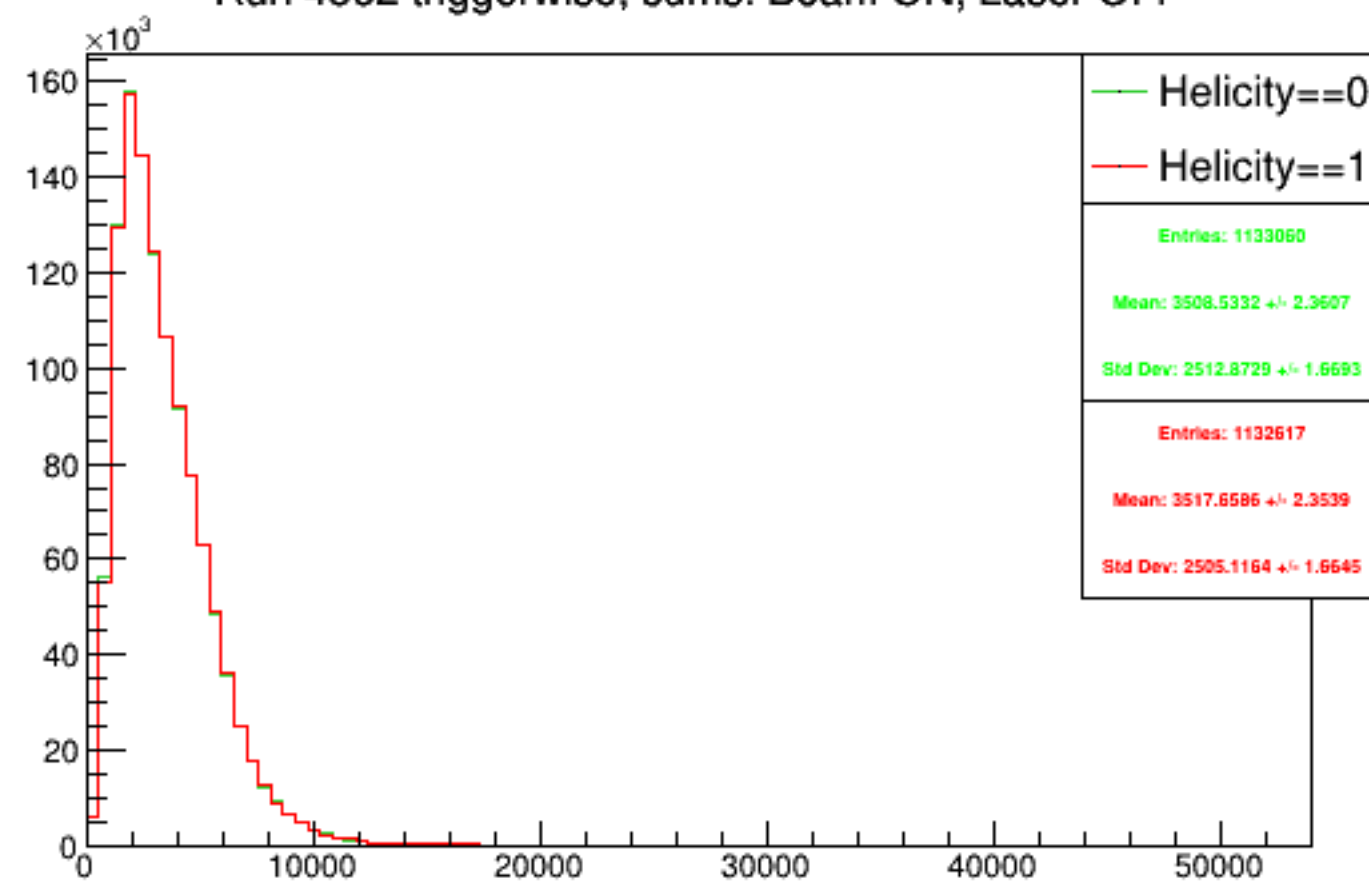
Run 4562 triggerwise, sums: Beam ON, Laser OFF
