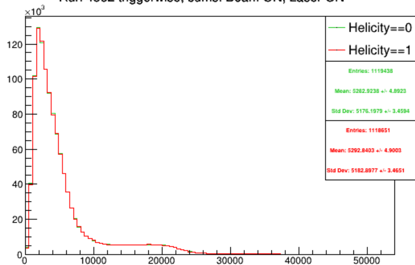
Run 4562 triggerwise, sums: Beam ON, Laser ON
