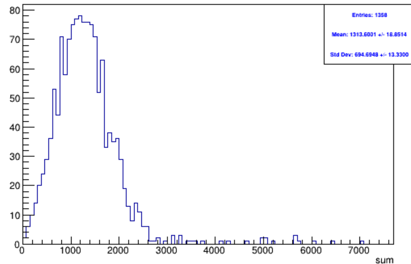
Run 4562 triggerwise, sums: Beam OFF
