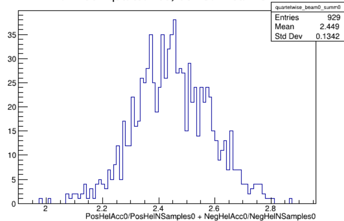
Run 4567 quartetwise, Sums0: Beam OFF
