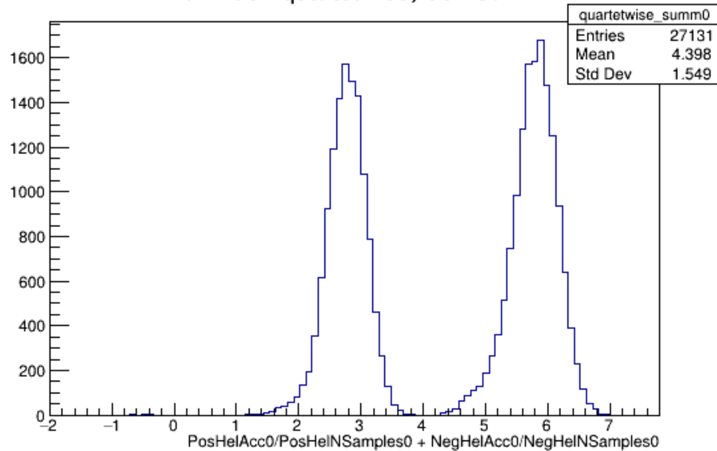
Run 4567 quartetwise, Sums0: All
