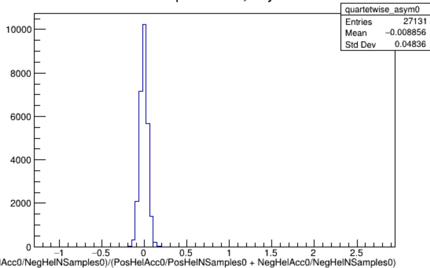
Run 4567 quartetwise, Asyms0: All
