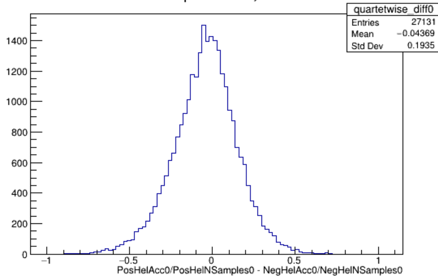
Run 4567 quartetwise, Diffs0: All
