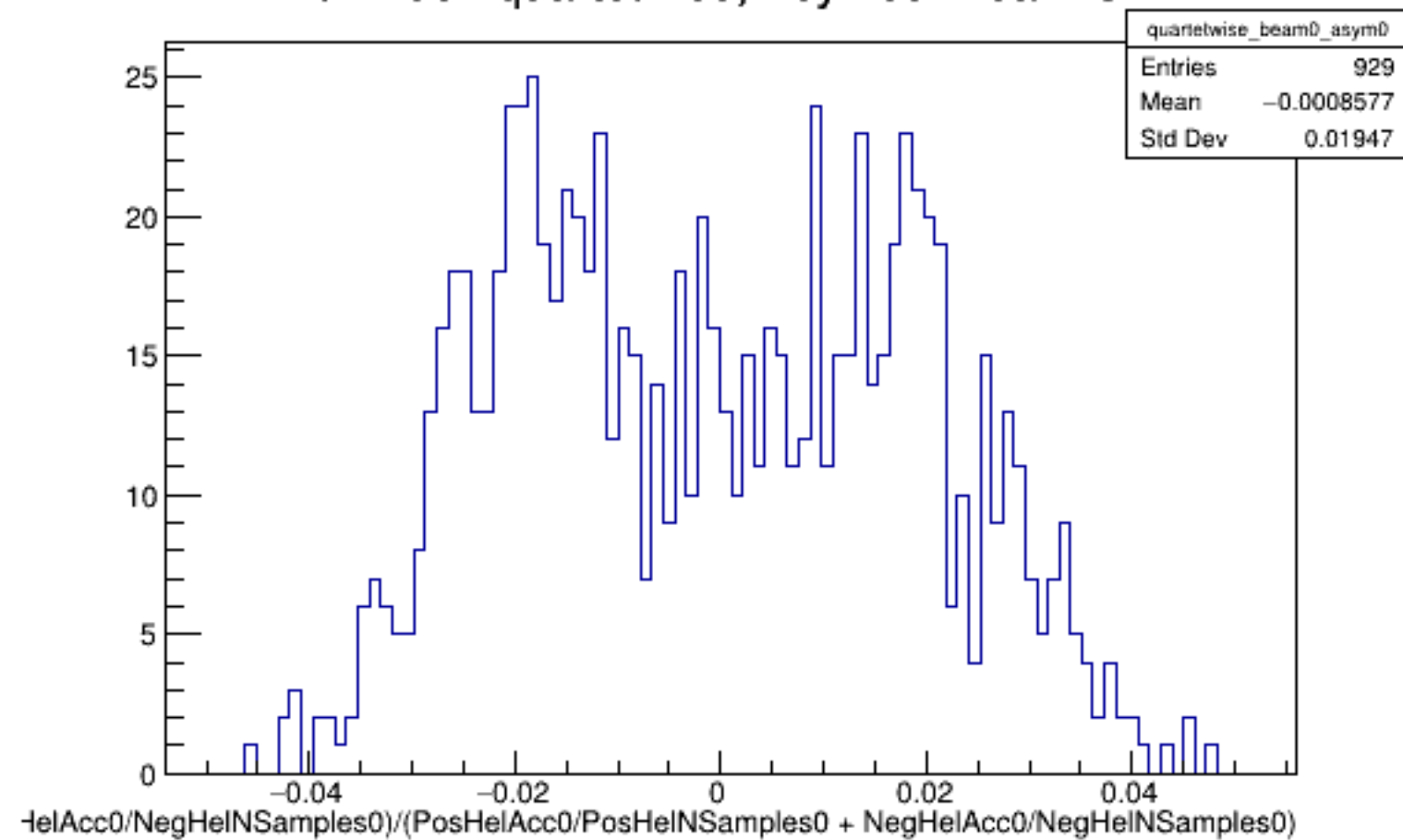
Run 4567 quartetwise, Asyms0: Beam OFF
