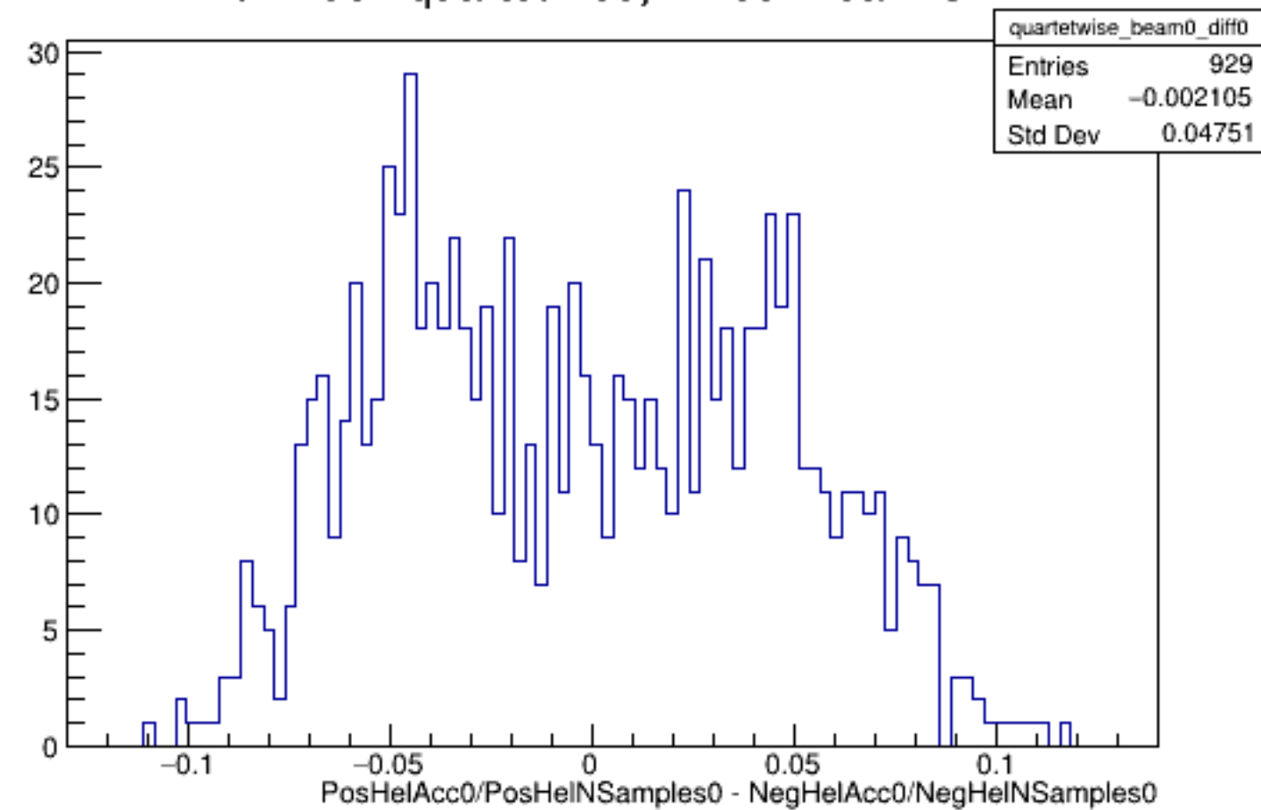
Run 4567 quartetwise, Diffs0: Beam OFF
