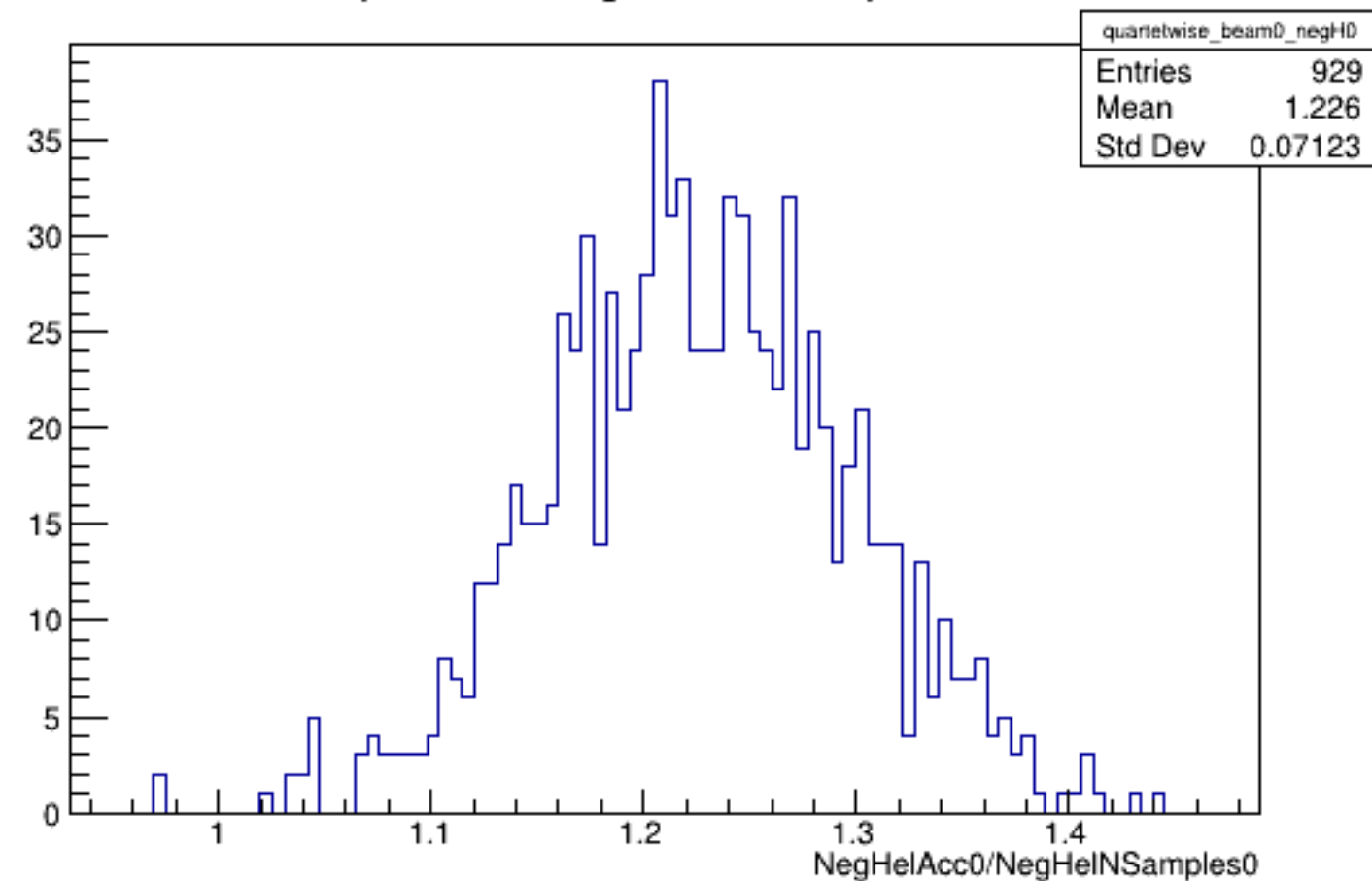
Run 4567 quartetwise, NegHelAcc0/NSamples0: Beam OFF
