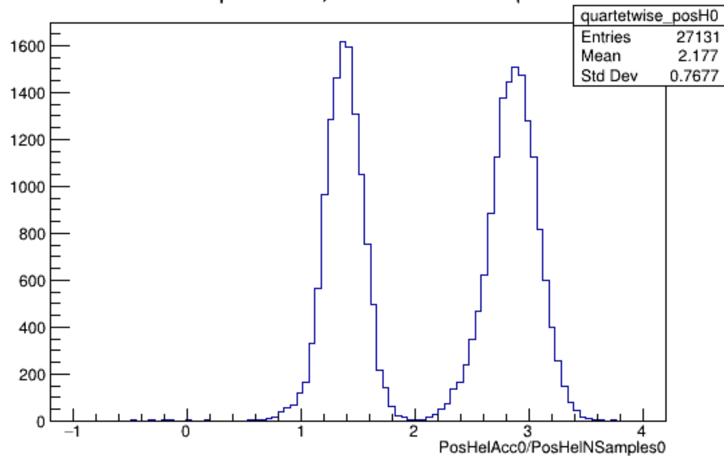
Run 4567 quartetwise, PosHelAcc0/NSamples0: All
