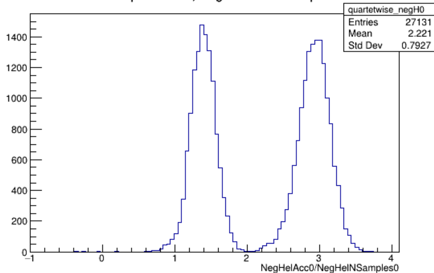
Run 4567 quartetwise, NegHelAcc0/NSamples0: All
