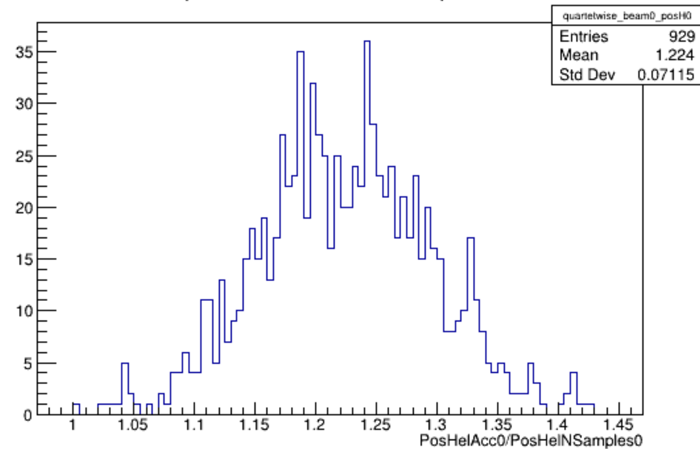
Run 4567 quartetwise, PosHelAcc0/NSamples0: Beam OFF
