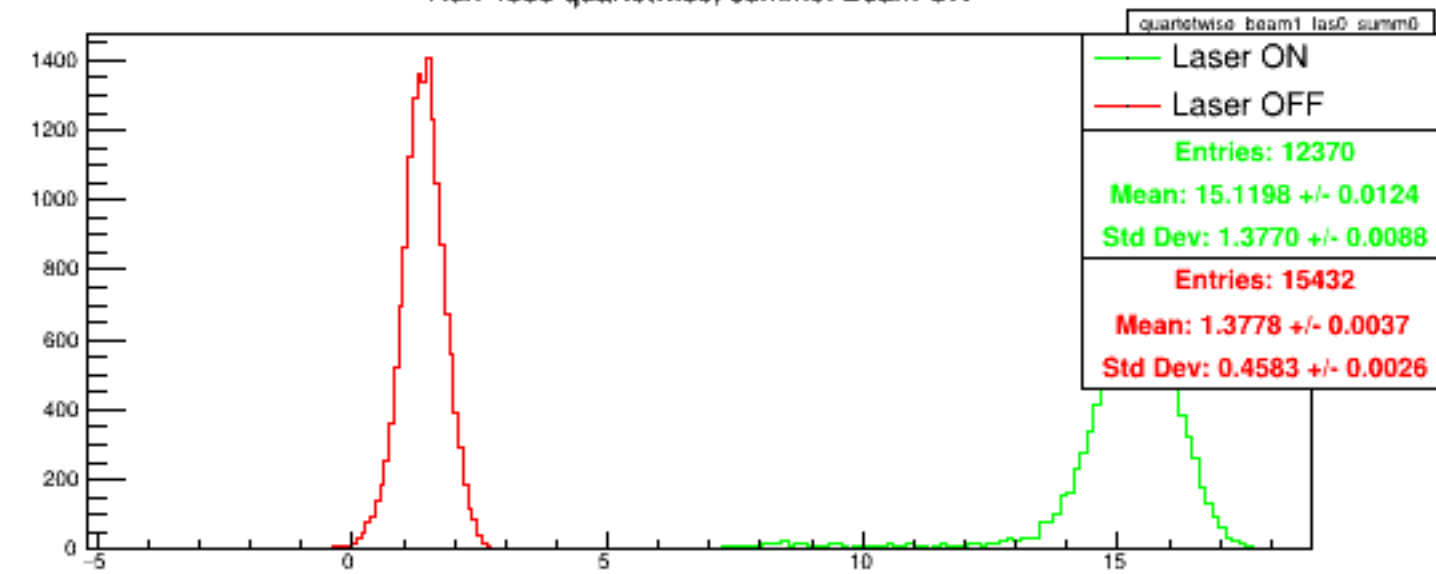
Run 4588 quartetwise, summ0: Beam ON
