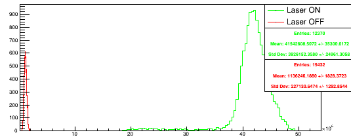
Run 4588 quartetwise, summ4: Beam ON
