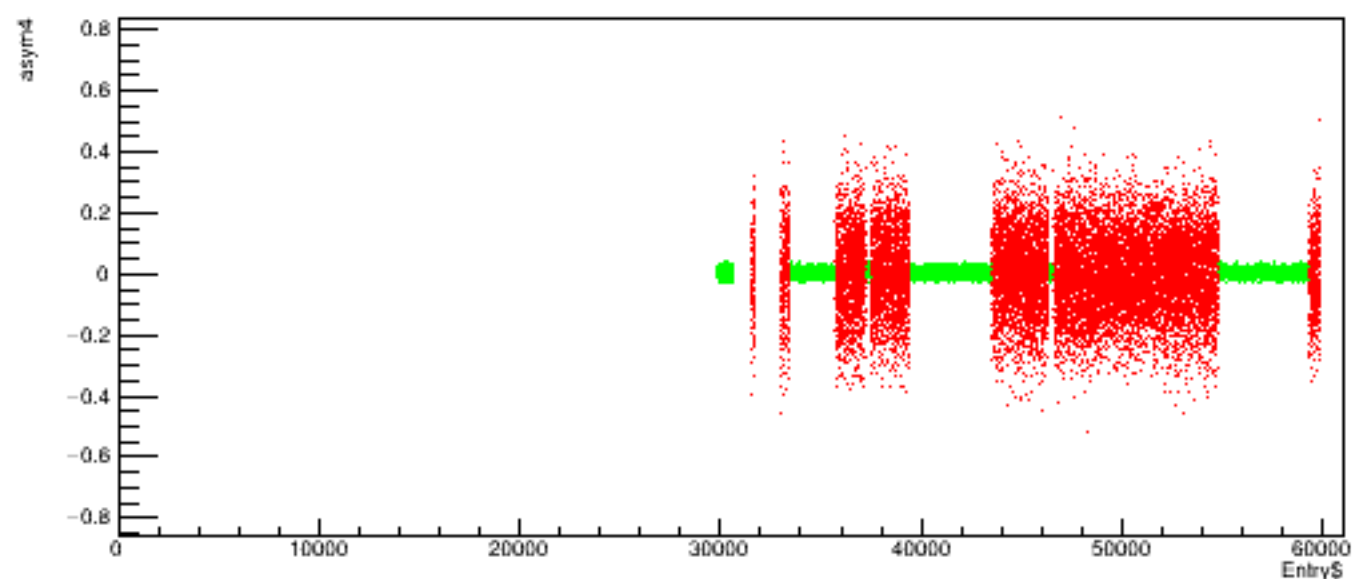
Run 4588 quartetwise, asym4 vs time
