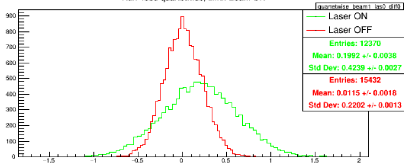
Run 4588 quartetwise, diff0: Beam ON
