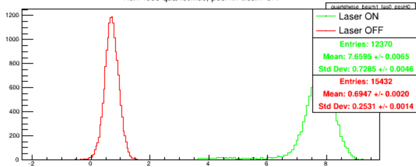
Run 4588 quartetwise, posH0: Beam ON
