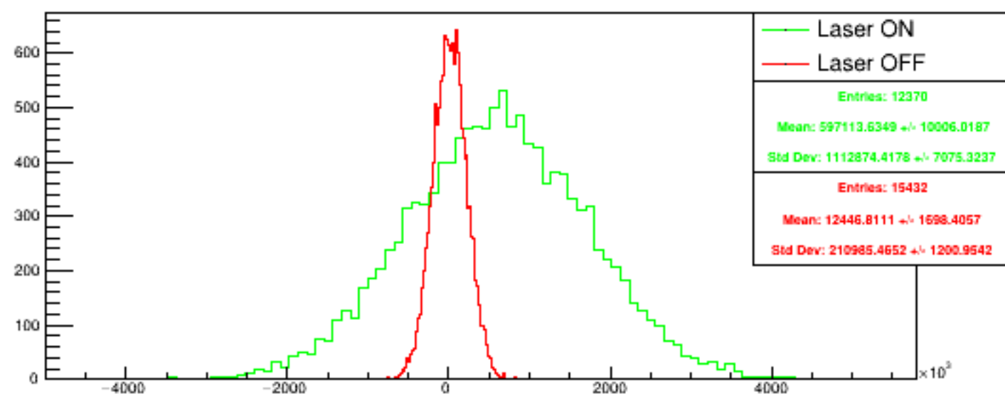
Run 4588 quartetwise, diff4: Beam ON
