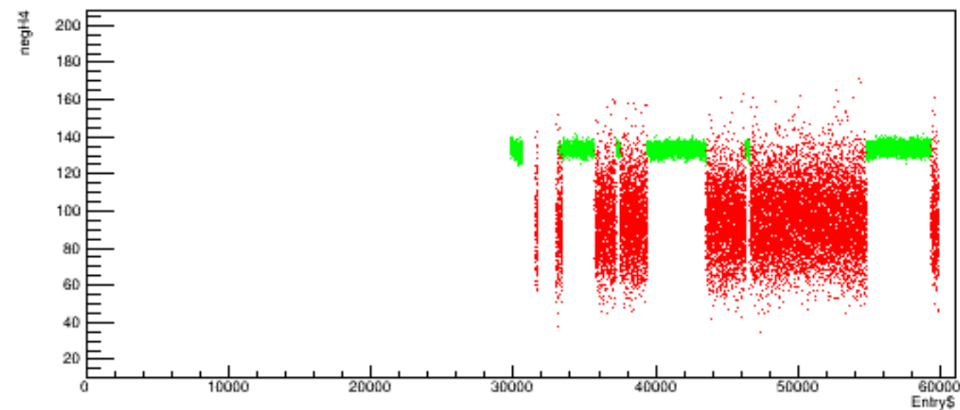
Run 4588 quartetwise, negH4 vs time
