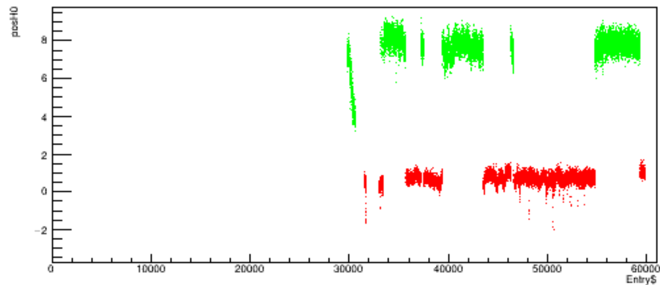
Run 4588 quartetwise, posH0 vs time
