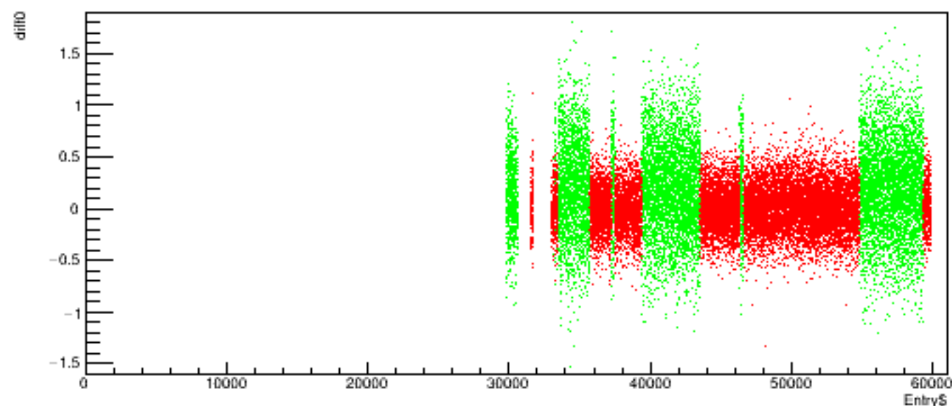
Run 4588 quartetwise, diff0 vs time
