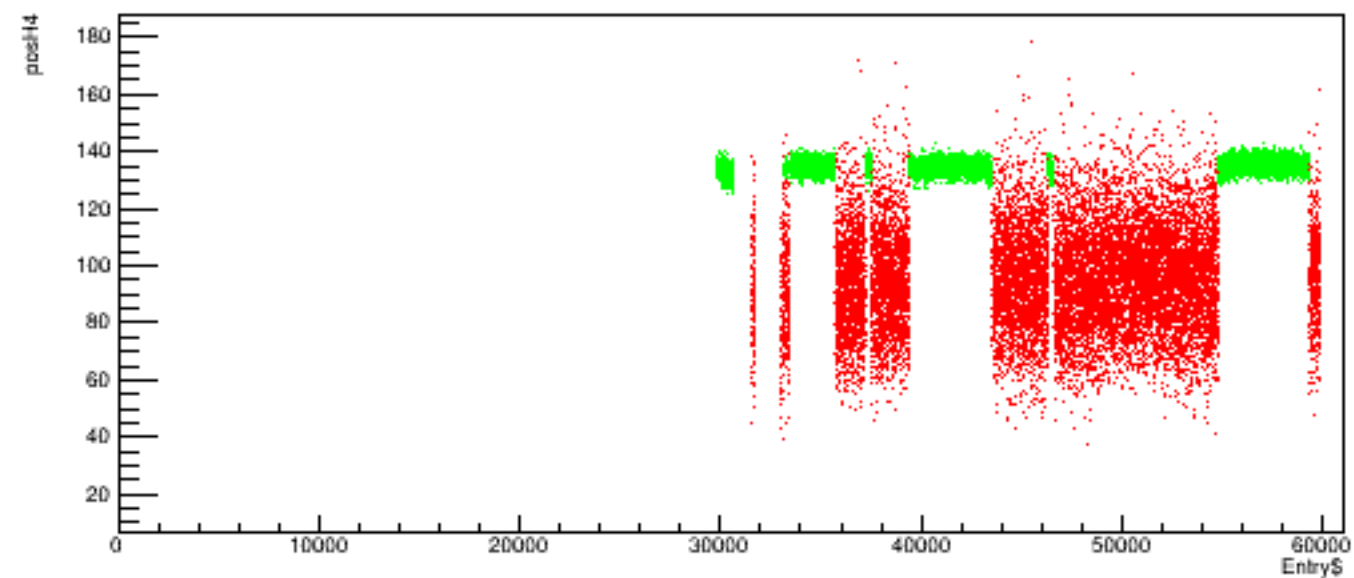
Run 4588 quartetwise, posH4 vs time
