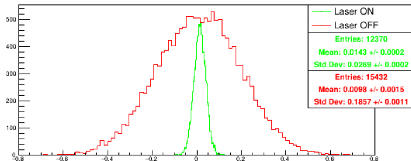
Run 4588 quartetwise, asym4: Beam ON
