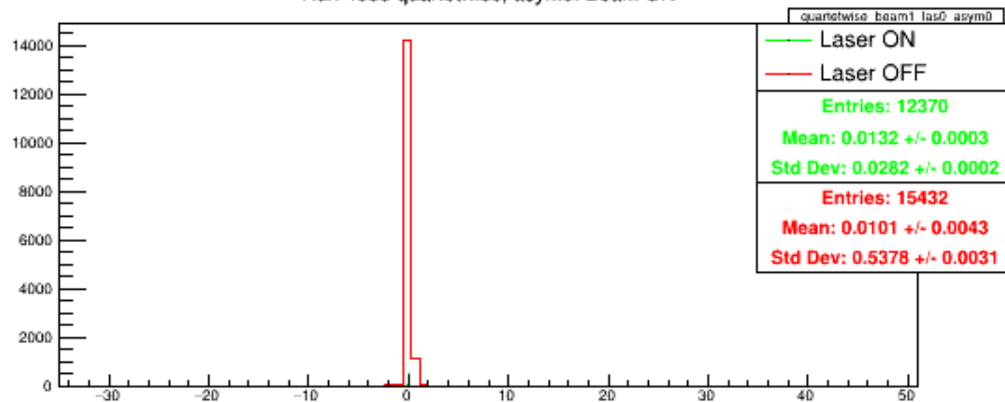
Run 4588 quartetwise, asym0: Beam ON
