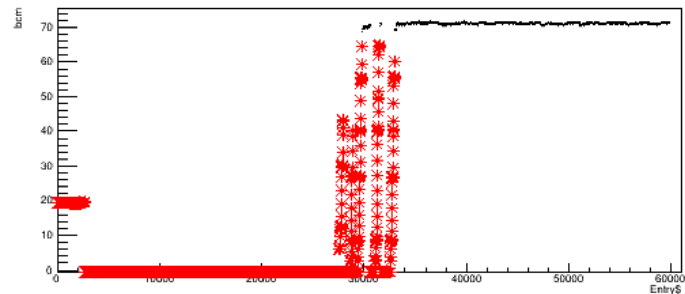
Run 4588 quartetwise, bcm vs time
