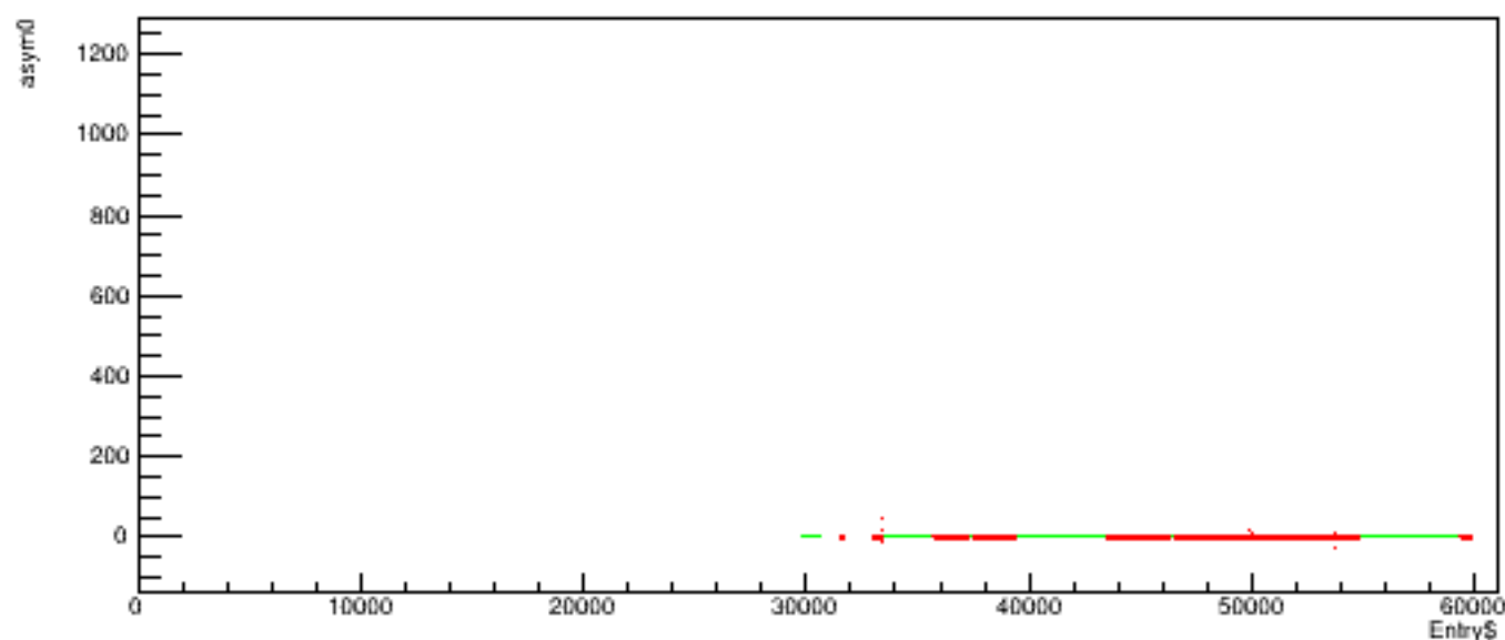
Run 4588 quartetwise, asym0 vs time
