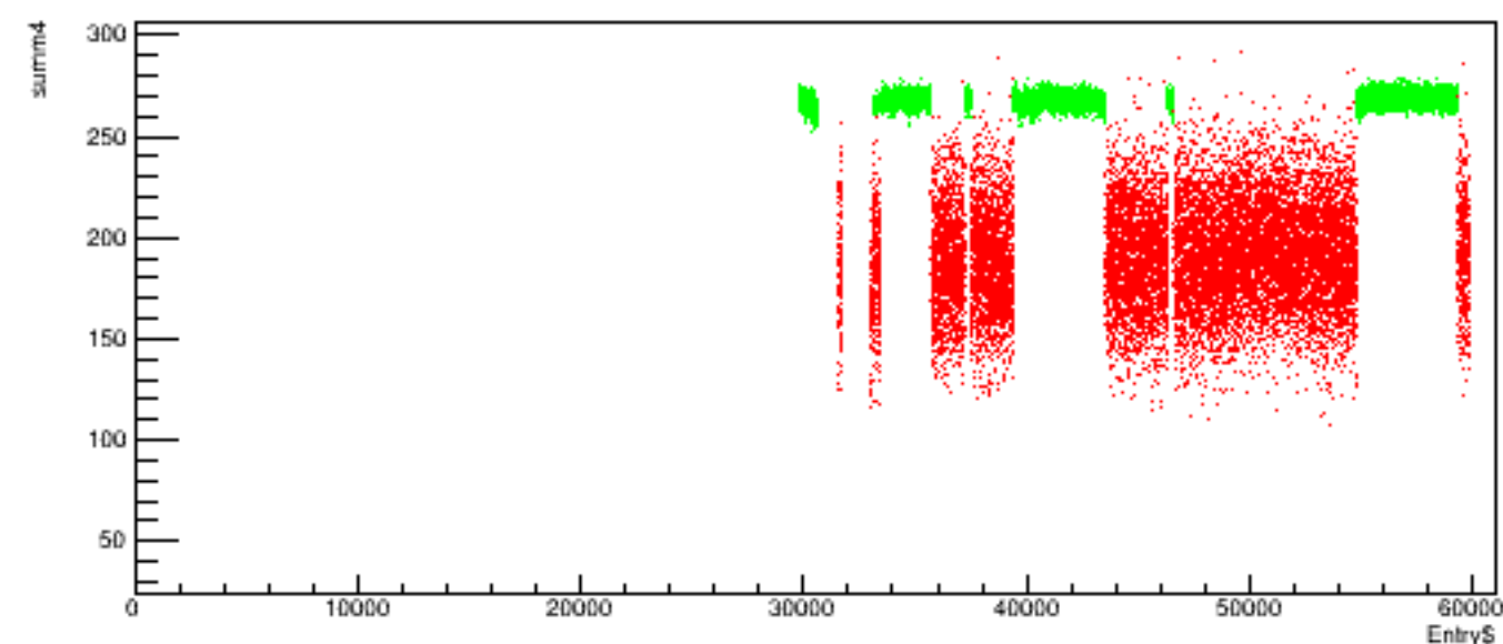
Run 4588 quartetwise, summ4 vs time
