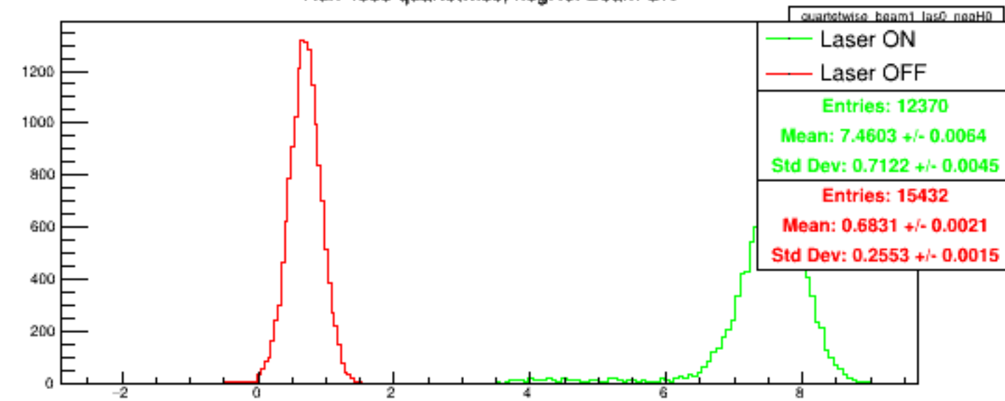
Run 4588 quartetwise, negH0: Beam ON
