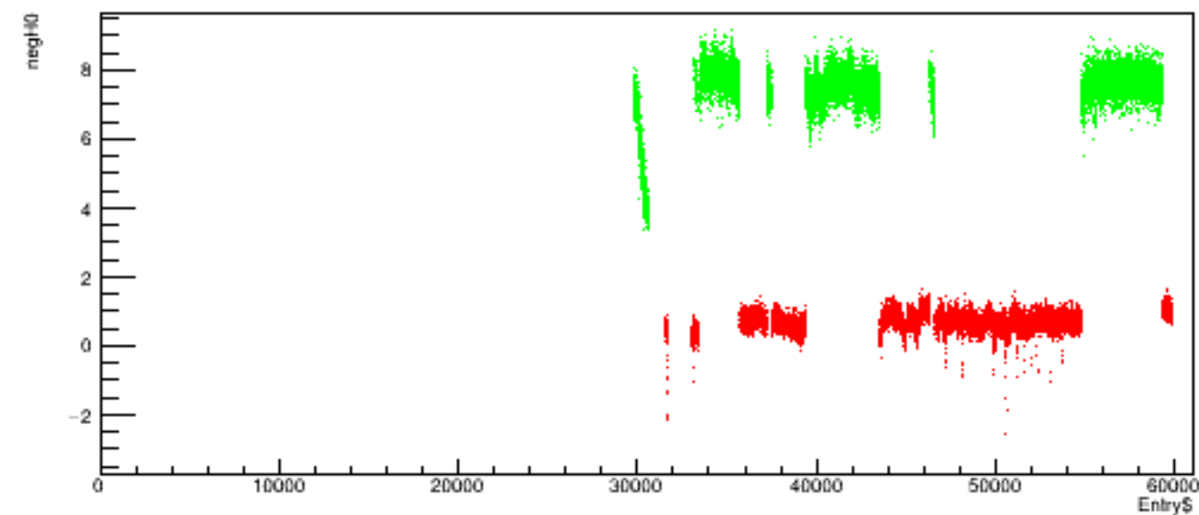
Run 4588 quartetwise, negH0 vs time
