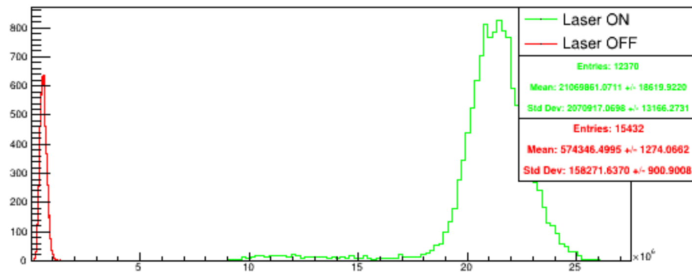
Run 4588 quartetwise, posH4: Beam ON
