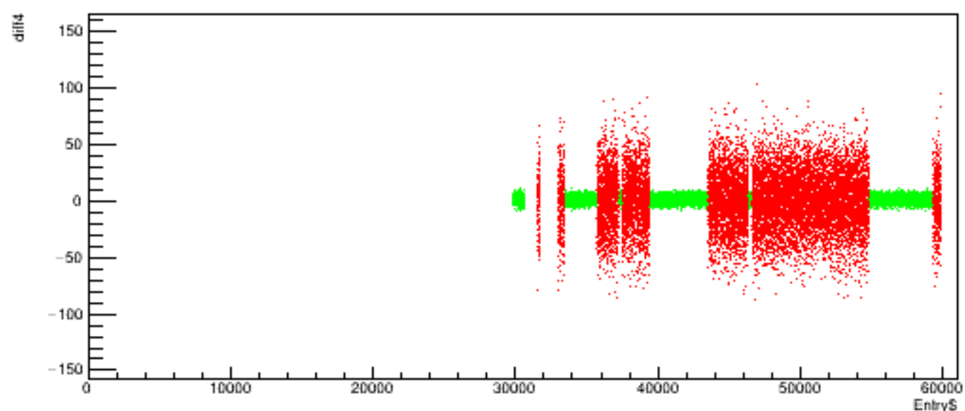
Run 4588 quartetwise, diff4 vs time
