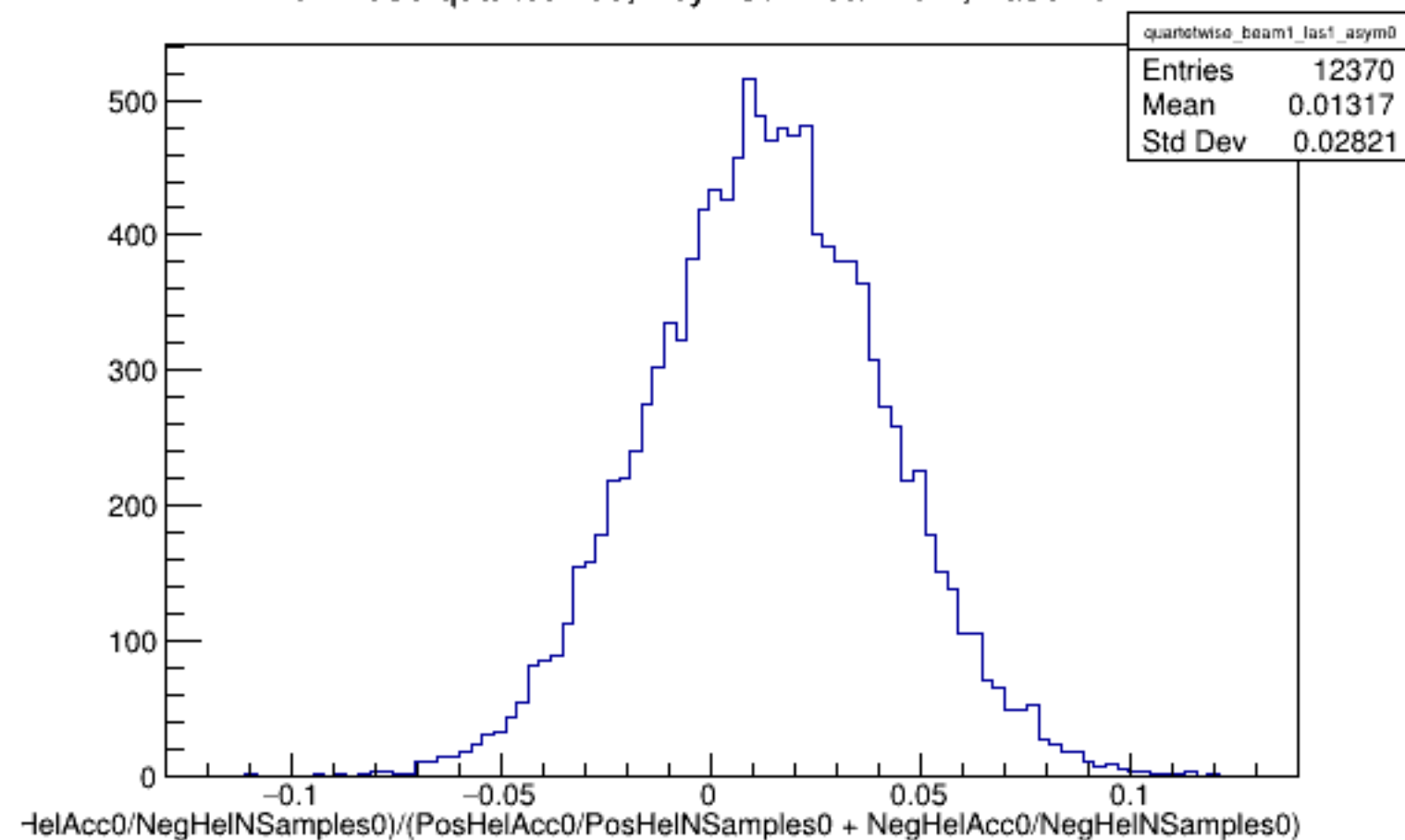
Run 4588 quartetwise, Asyms0: Beam ON, Laser ON
