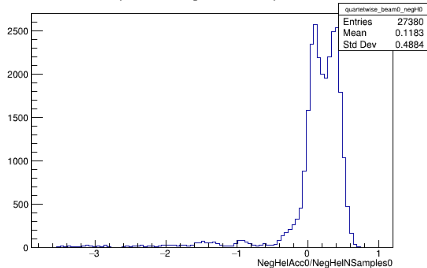
Run 4588 quartetwise, NegHelAcc0/NSamples0: Beam OFF
