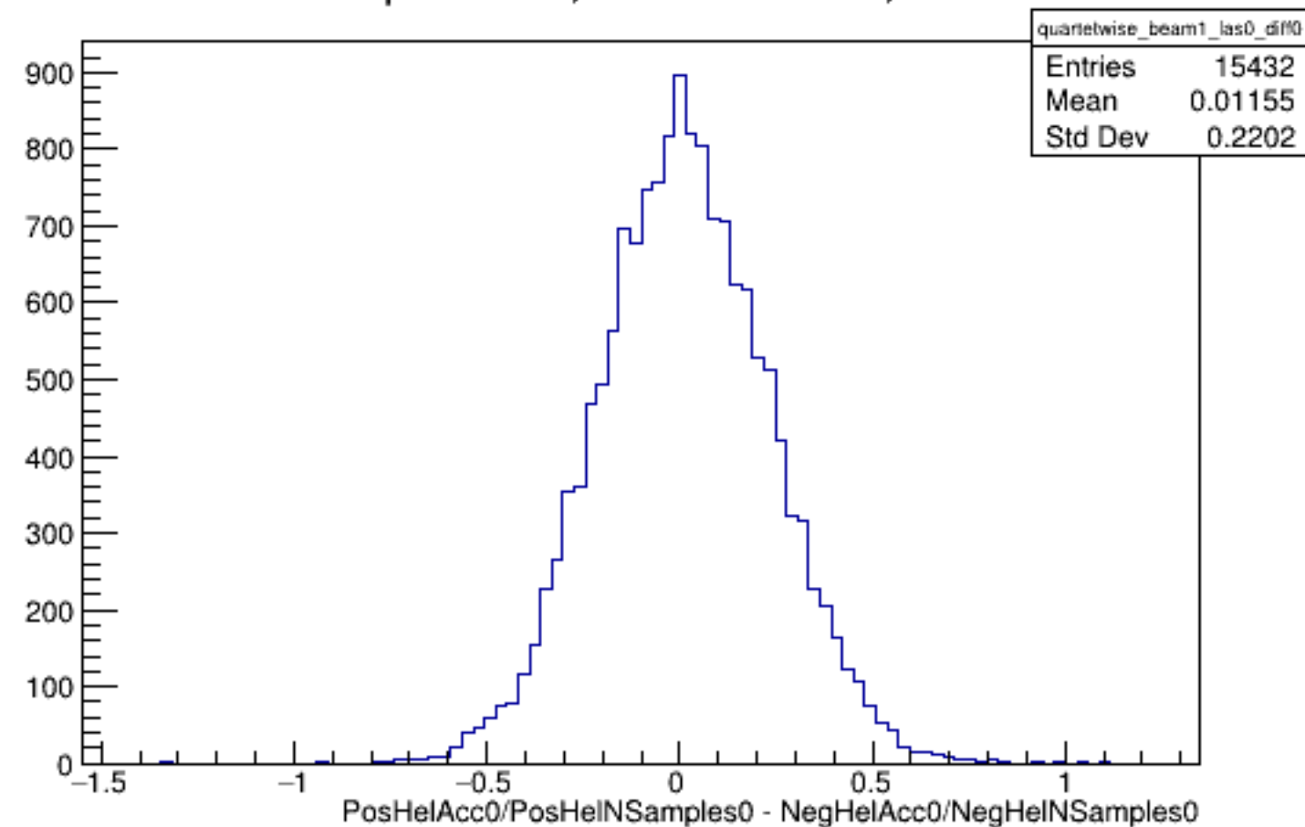
Run 4588 quartetwise, Diffs0: Beam ON, Laser OFF
