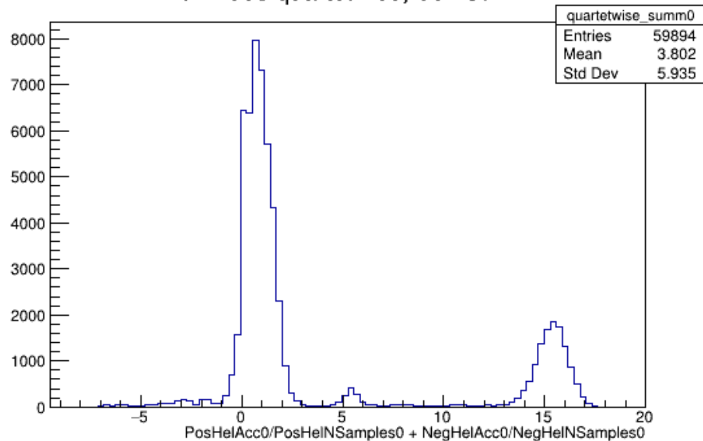
Run 4588 quartetwise, Sums0: All
