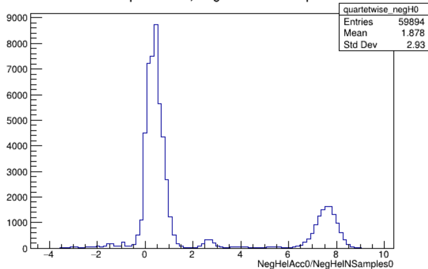
Run 4588 quartetwise, NegHelAcc0/NSamples0: All
