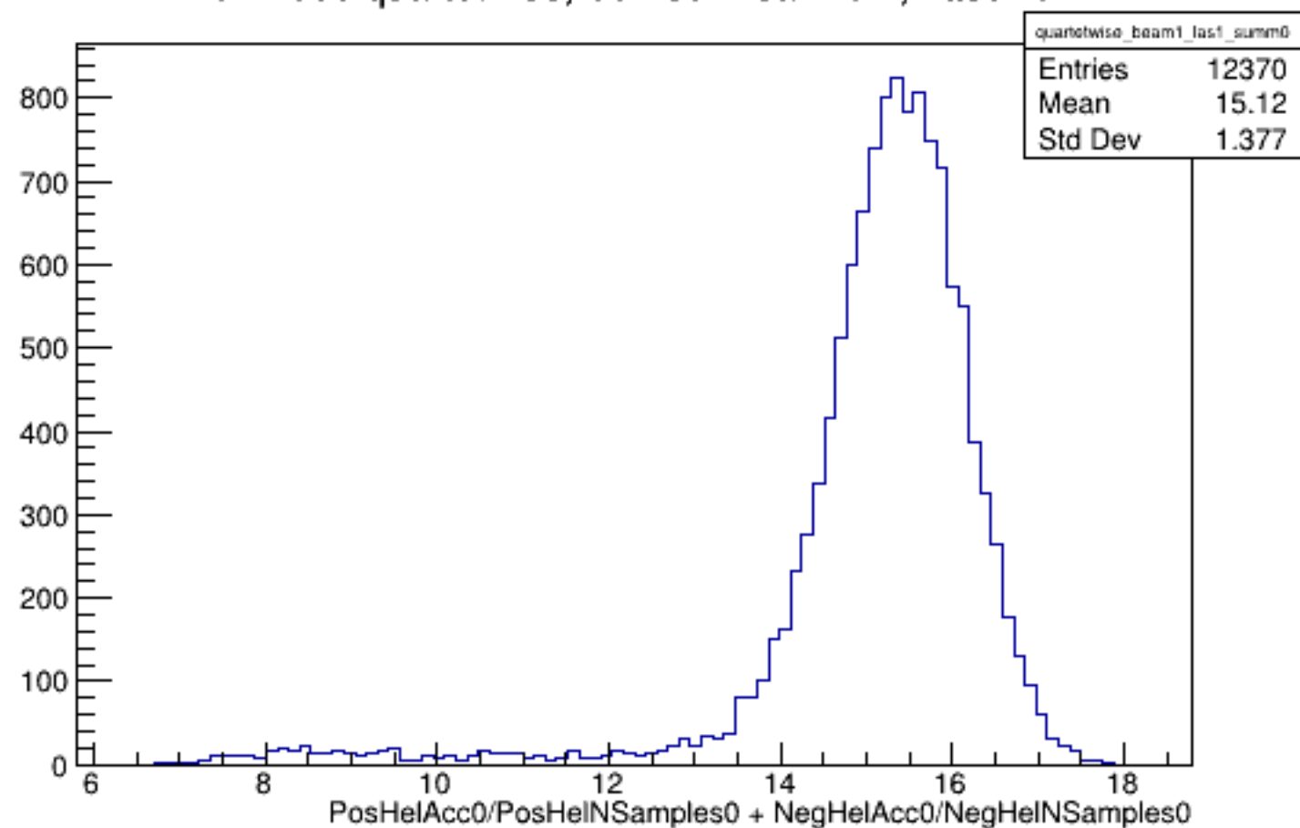
Run 4588 quartetwise, Sums0: Beam ON, Laser ON
