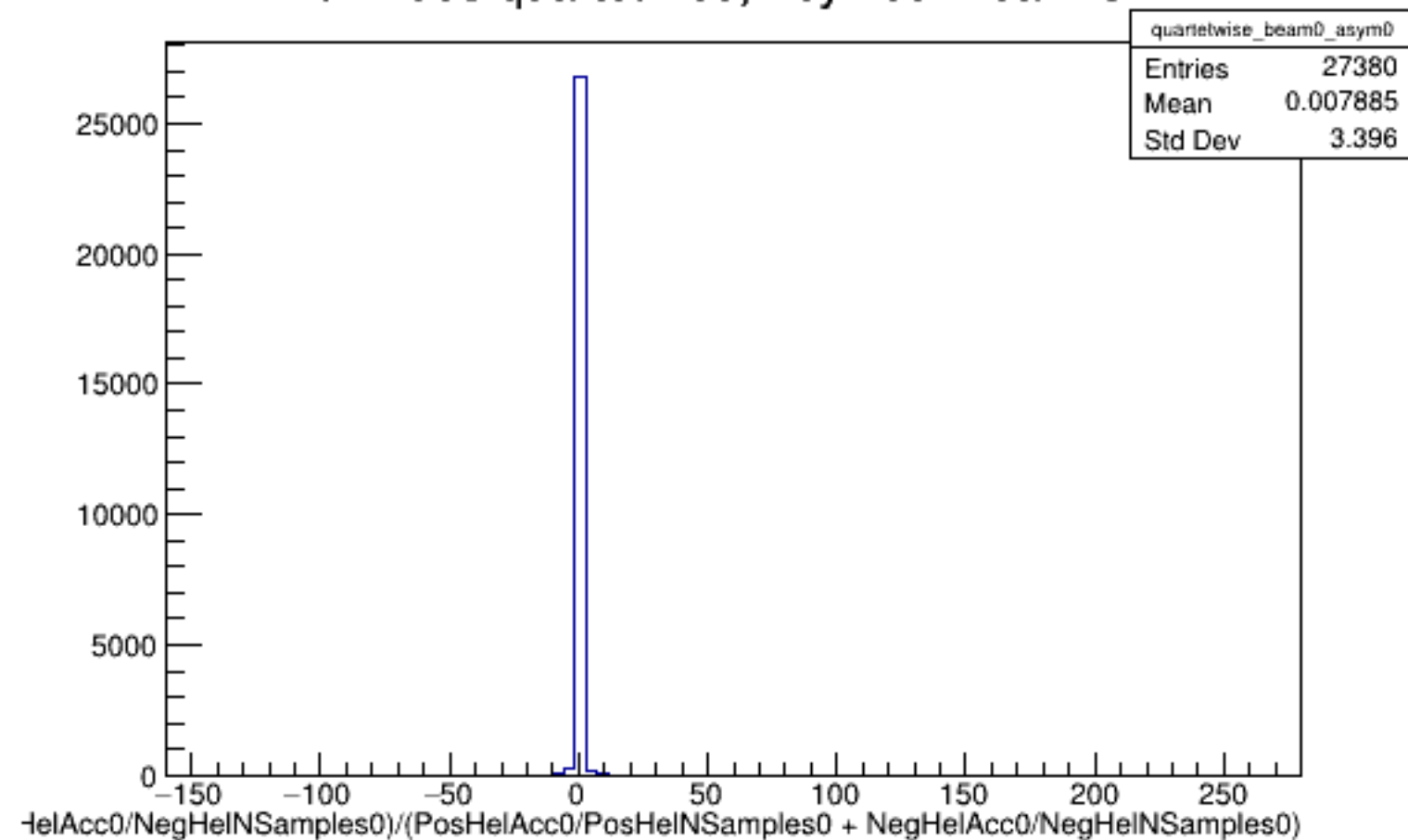
Run 4588 quartetwise, Asyms0: Beam OFF
