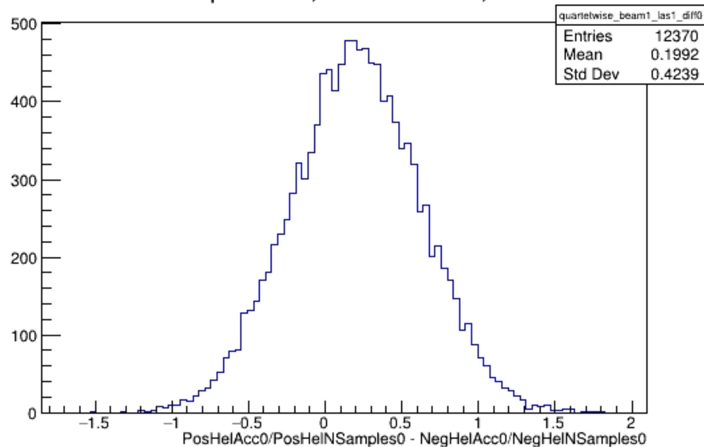
Run 4588 quartetwise, Diffs0: Beam ON, Laser ON
