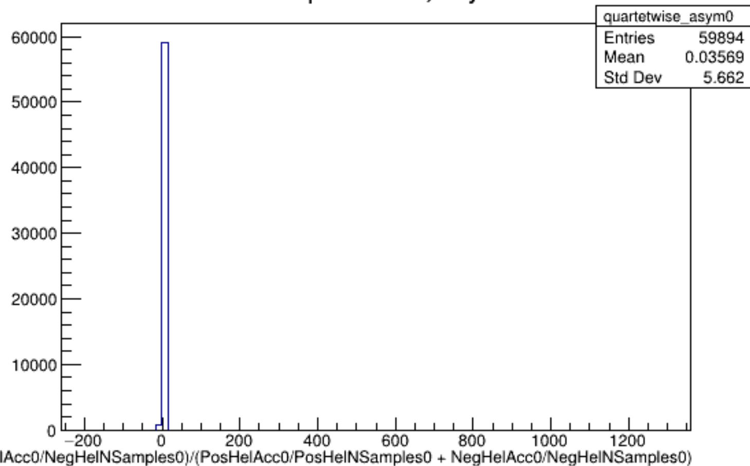
Run 4588 quartetwise, Asyms0: All
