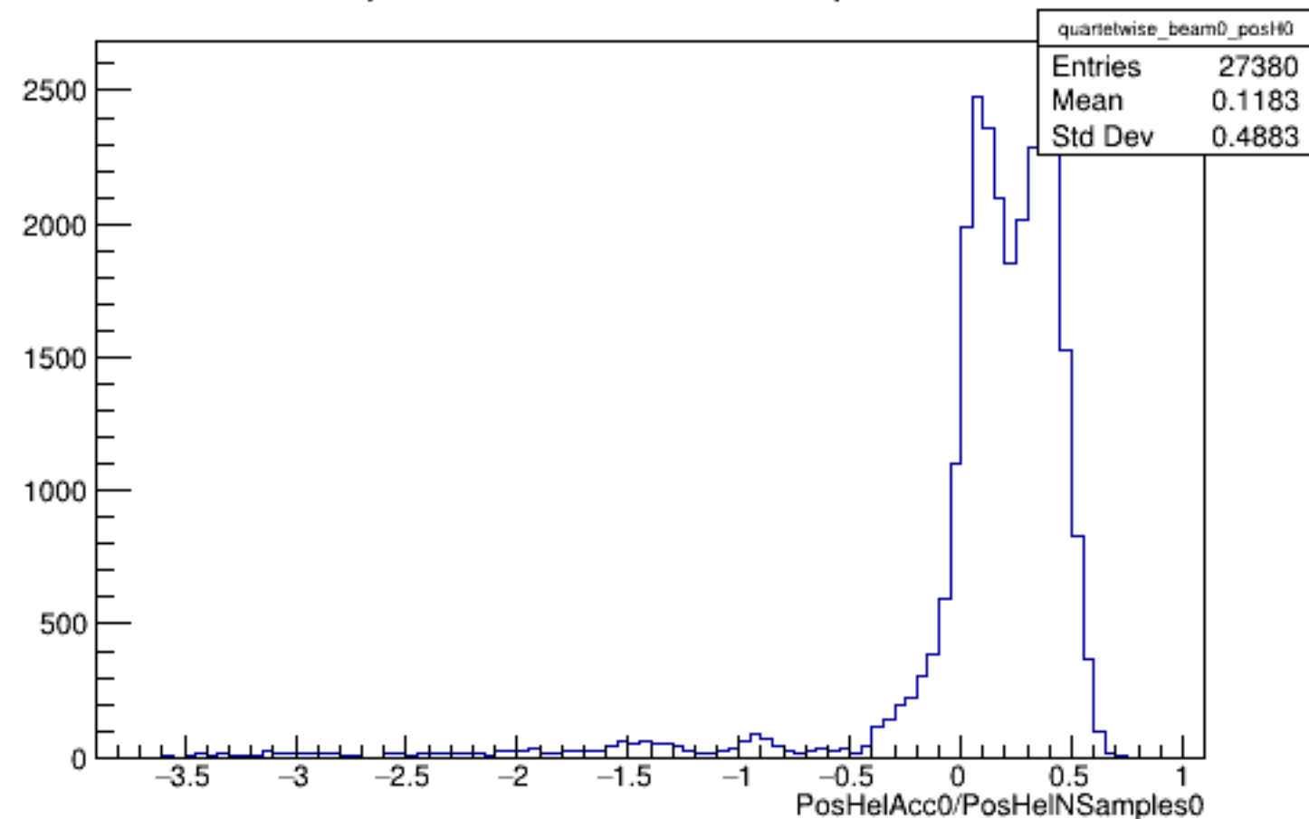
Run 4588 quartetwise, PosHelAcc0/NSamples0: Beam OFF
