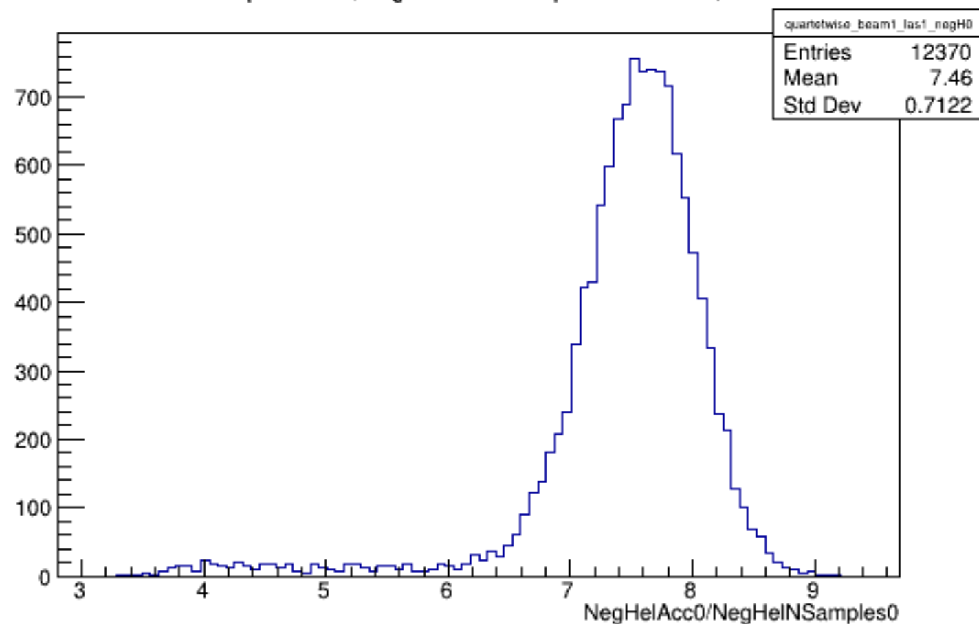
Run 4588 quartetwise, NegHelAcc0/NSamples0: Beam ON, Laser ON
