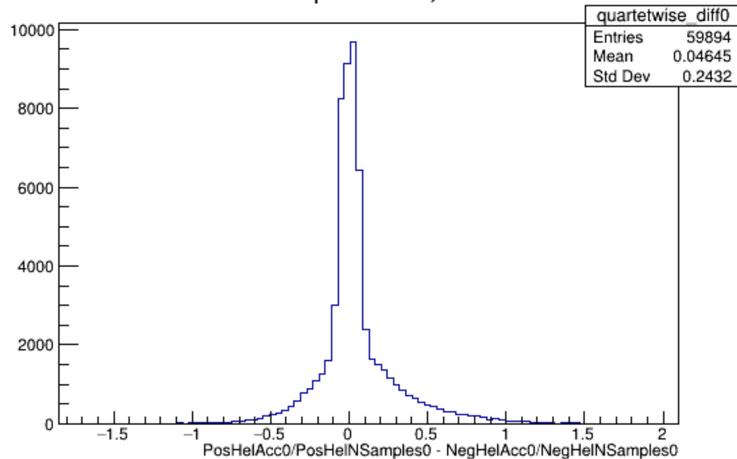
Run 4588 quartetwise, Diffs0: All
