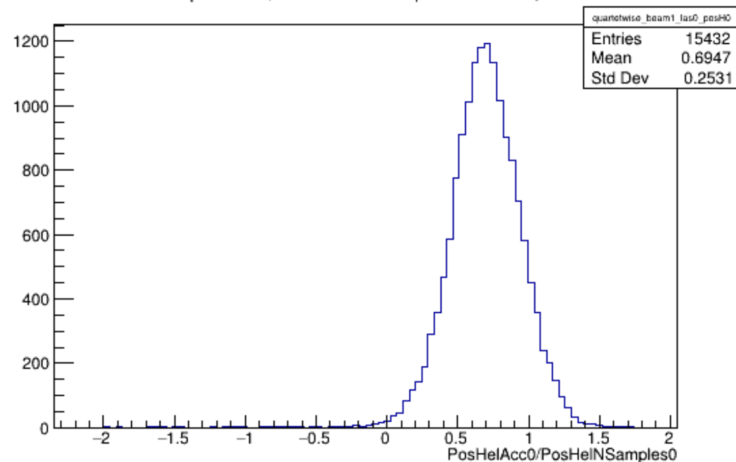
Run 4588 quartetwise, PosHelAcc0/NSamples0: Beam ON, Laser OFF
