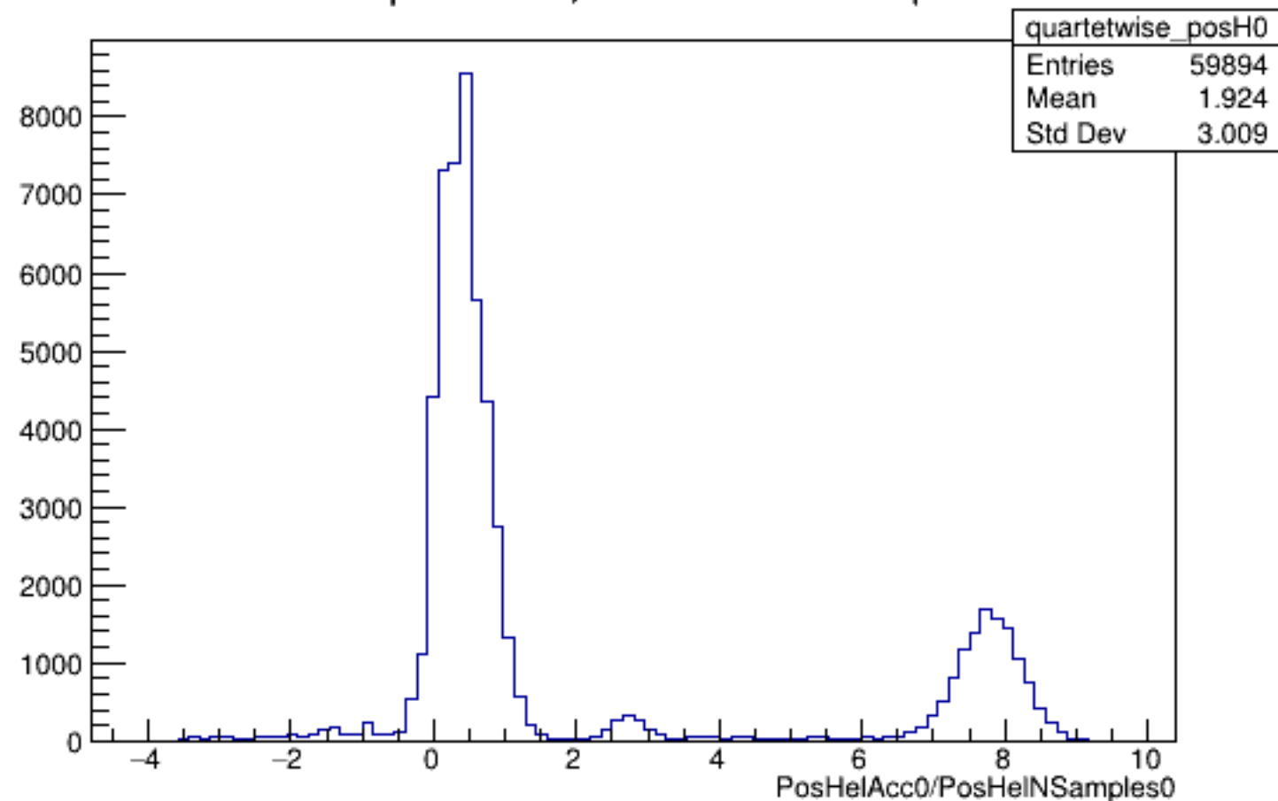
Run 4588 quartetwise, PosHelAcc0/NSamples0: All
