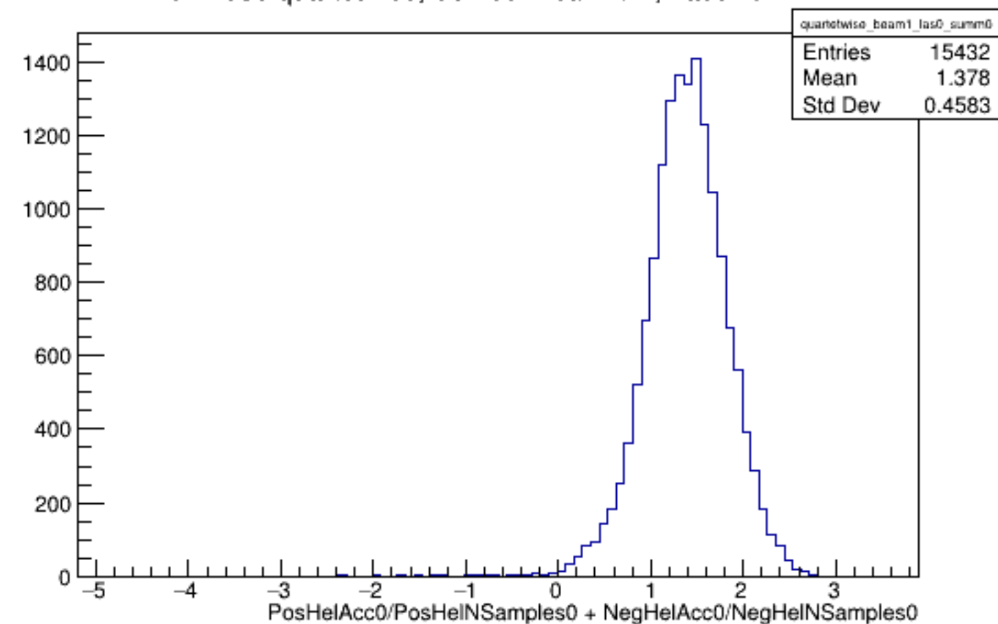
Run 4588 quartetwise, Sums0: Beam ON, Laser OFF
