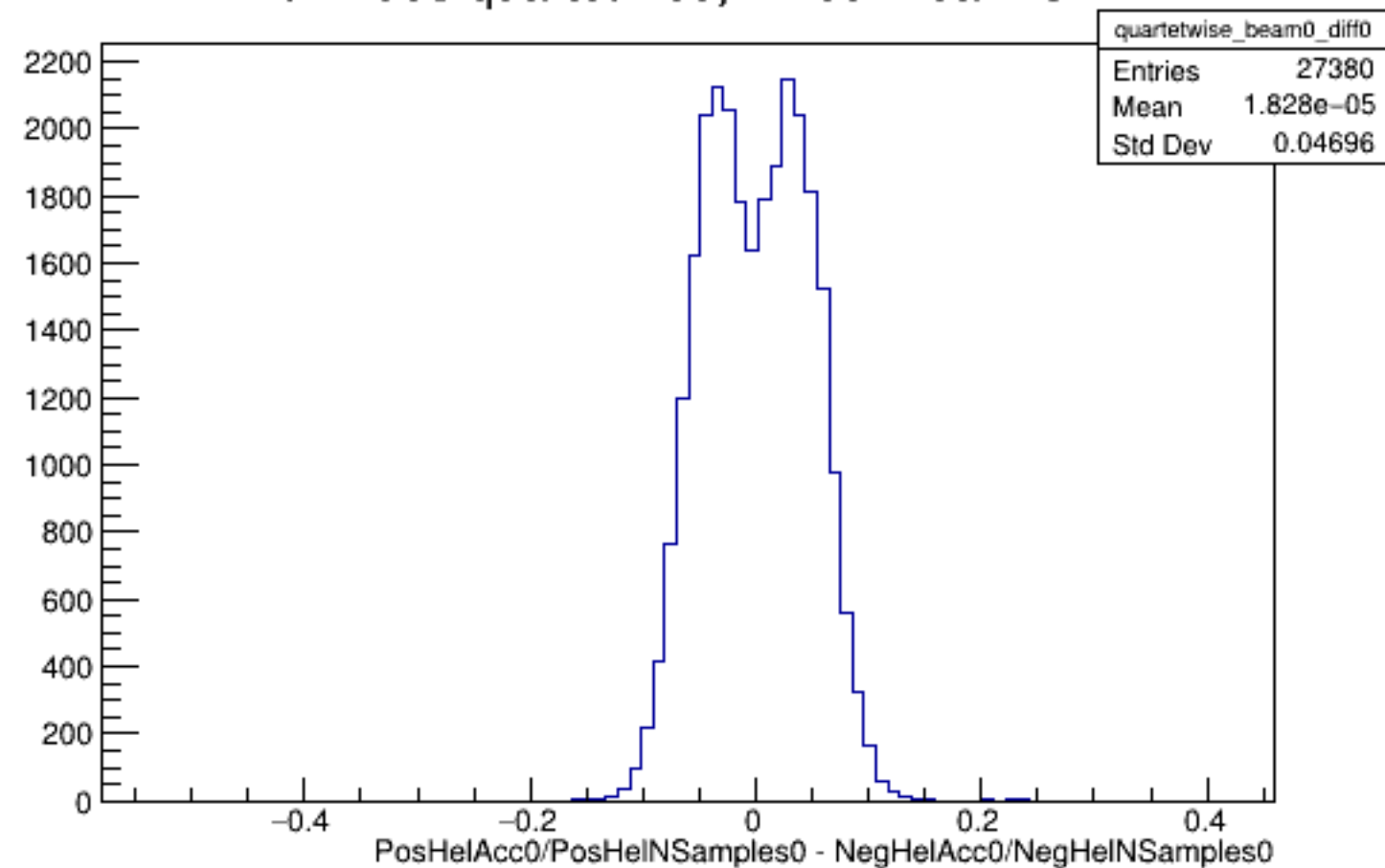
Run 4588 quartetwise, Diffs0: Beam OFF
