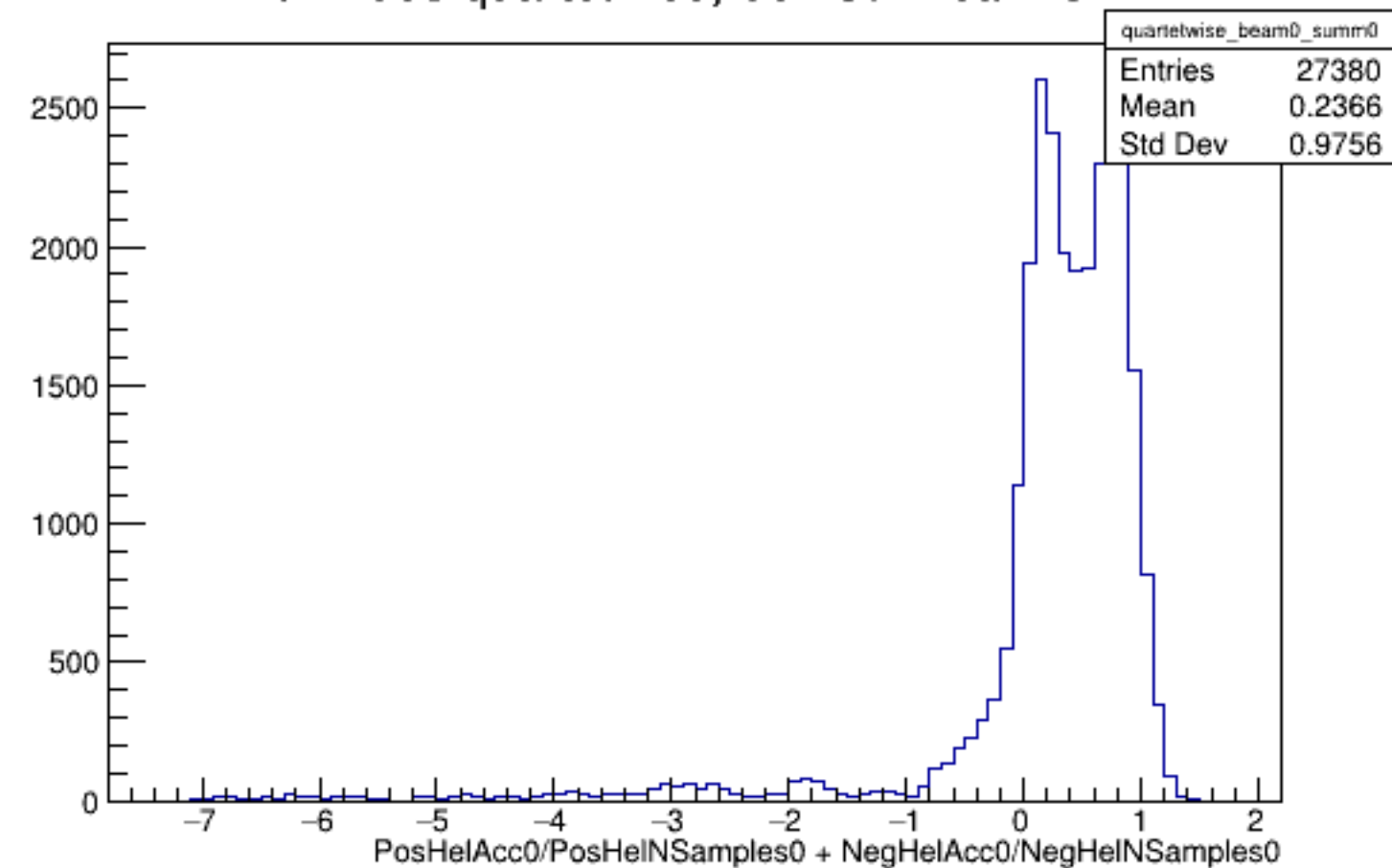
Run 4588 quartetwise, Sums0: Beam OFF
