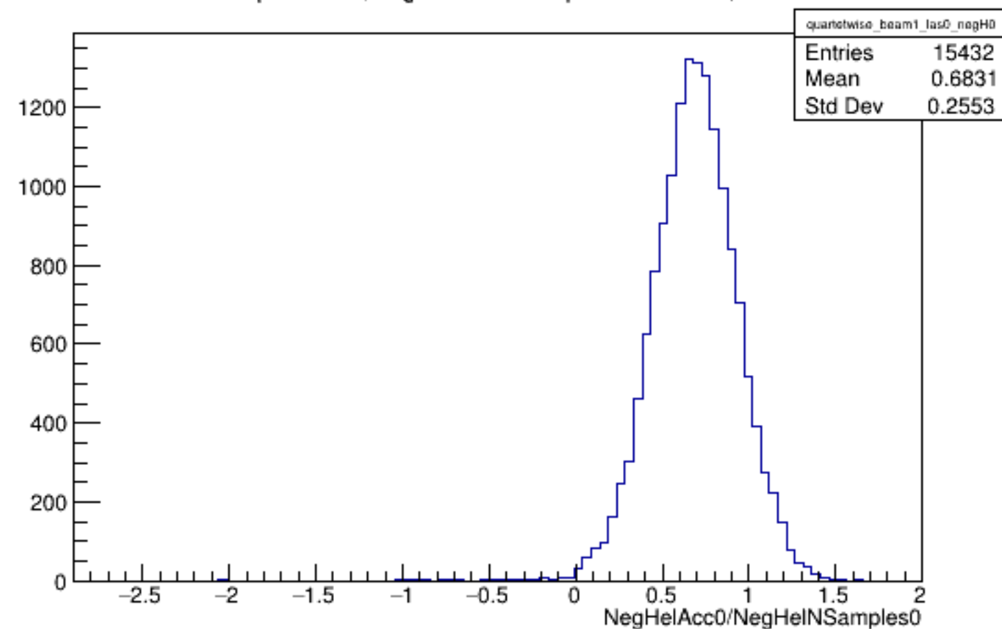
Run 4588 quartetwise, NegHelAcc0/NSamples0: Beam ON, Laser OFF
