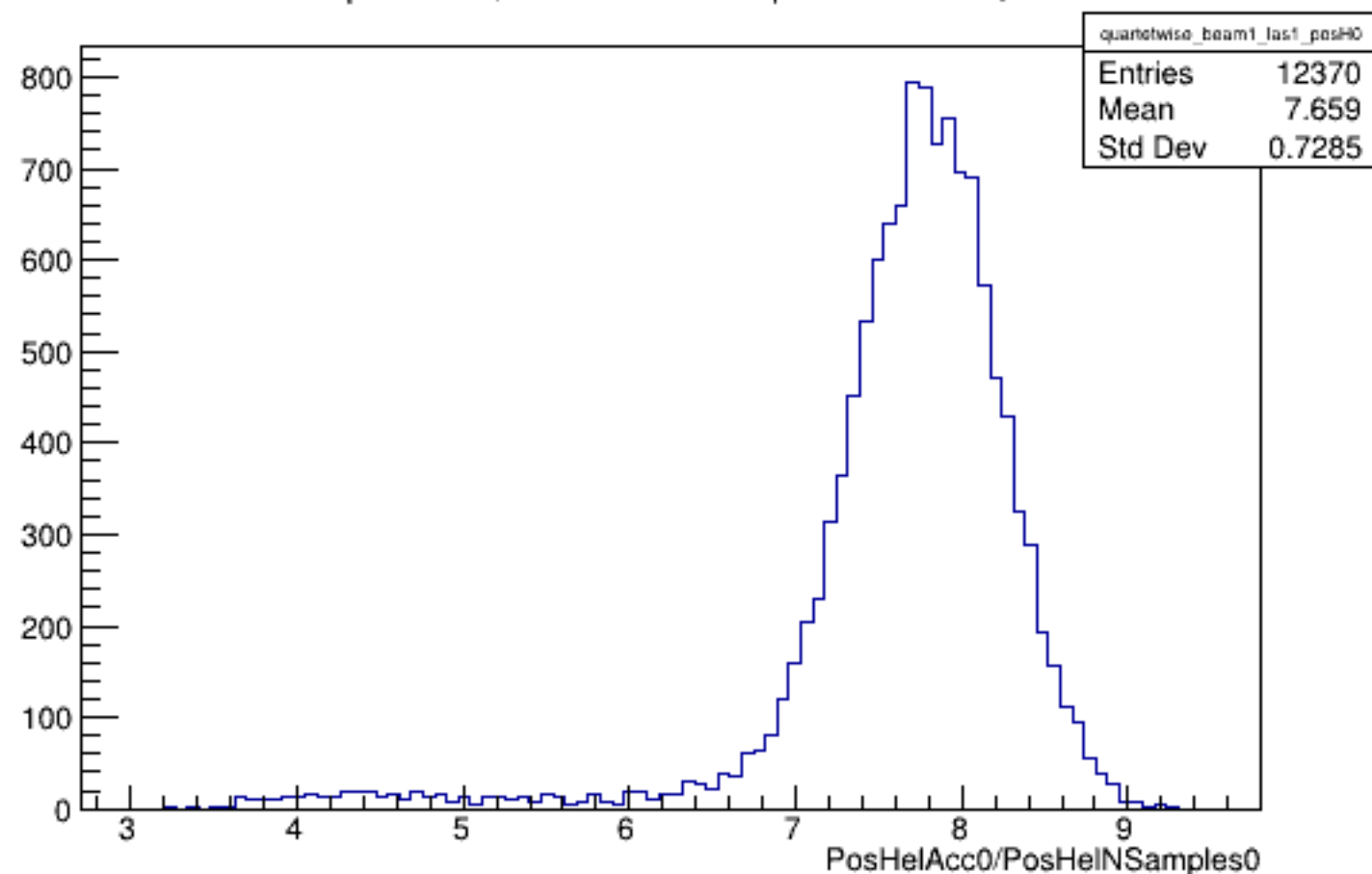
Run 4588 quartetwise, PosHelAcc0/NSamples0: Beam ON, Laser ON
