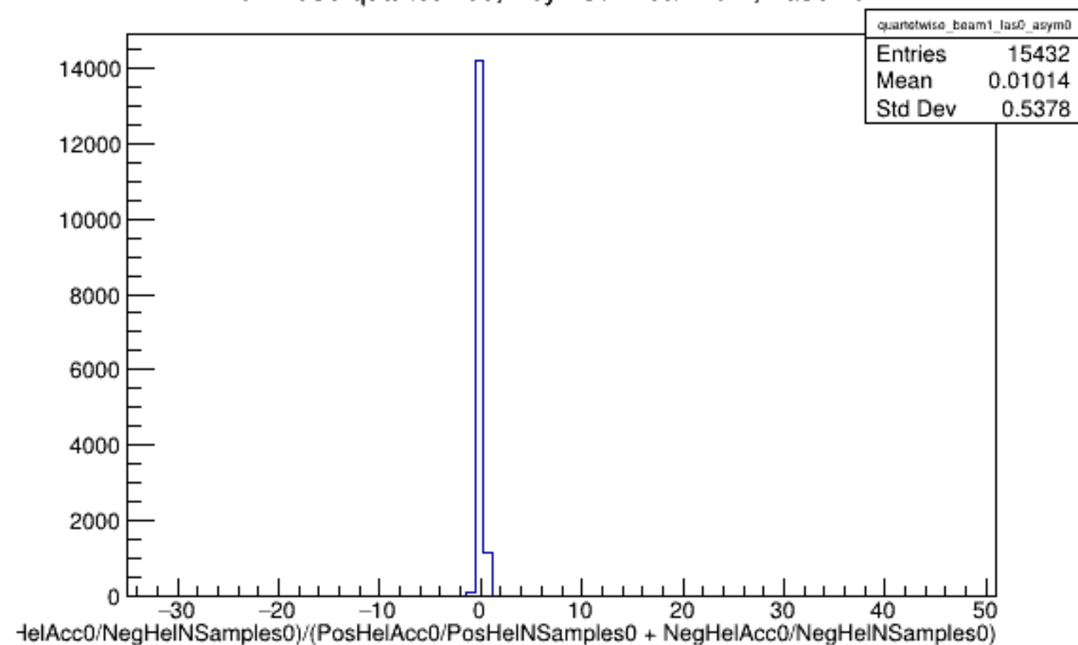
Run 4588 quartetwise, Asyms0: Beam ON, Laser OFF
