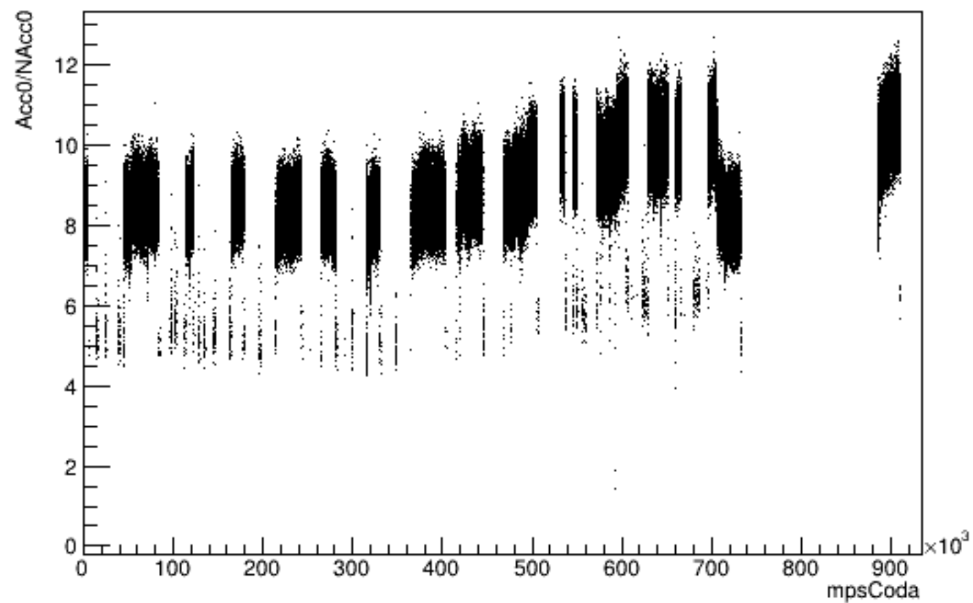
Run 4589 mpwise, Acc0/NAcc0:mpsCoda, beam ON, laser ON
