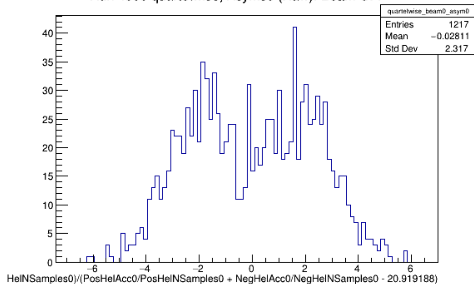
Run 4590 quartetwise, Asyms0 (Raw): Beam OFF
