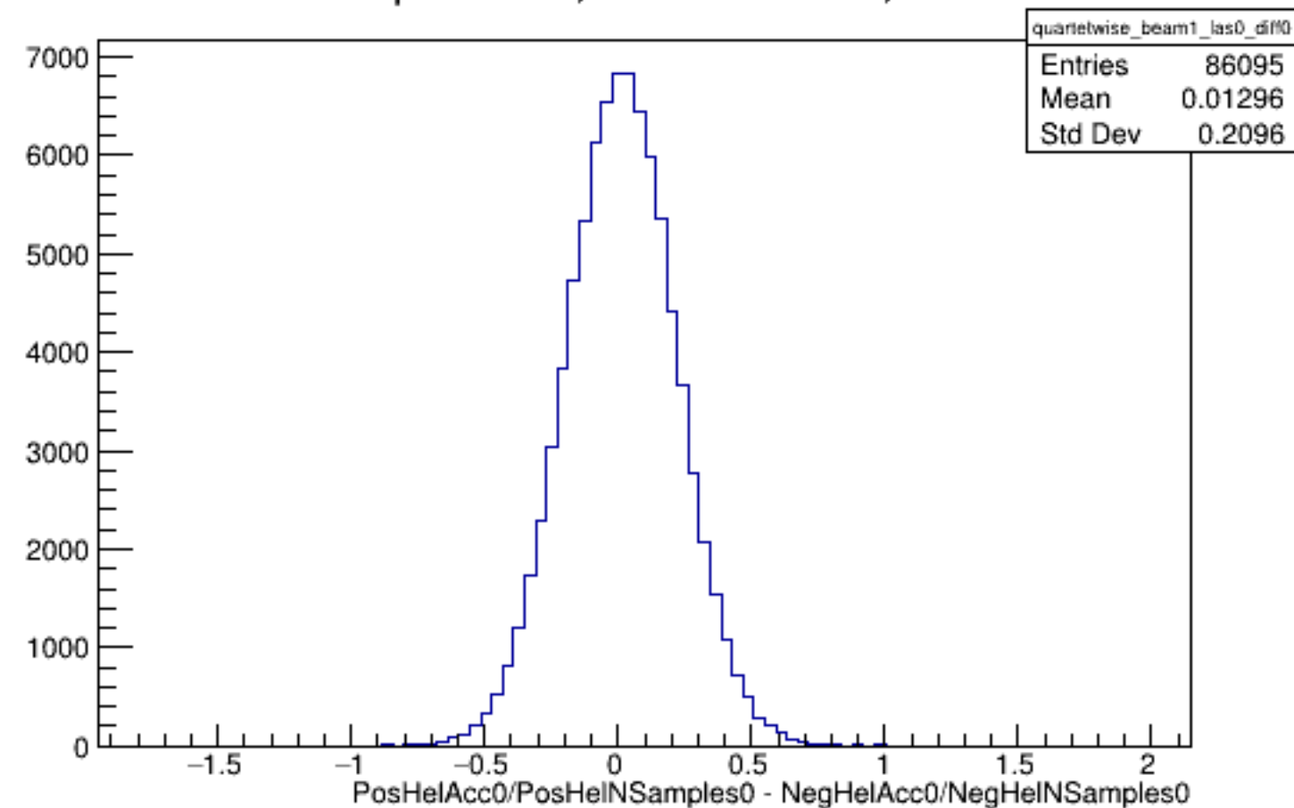
Run 4590 quartetwise, Diffs0: Beam ON, Laser OFF
