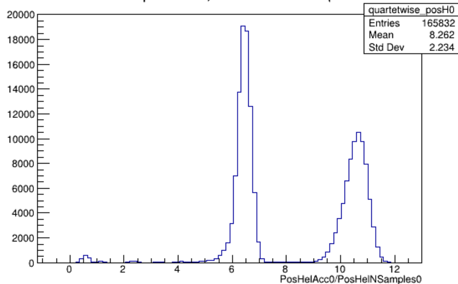
Run 4590 quartetwise, PosHelAcc0/NSamples0: All
