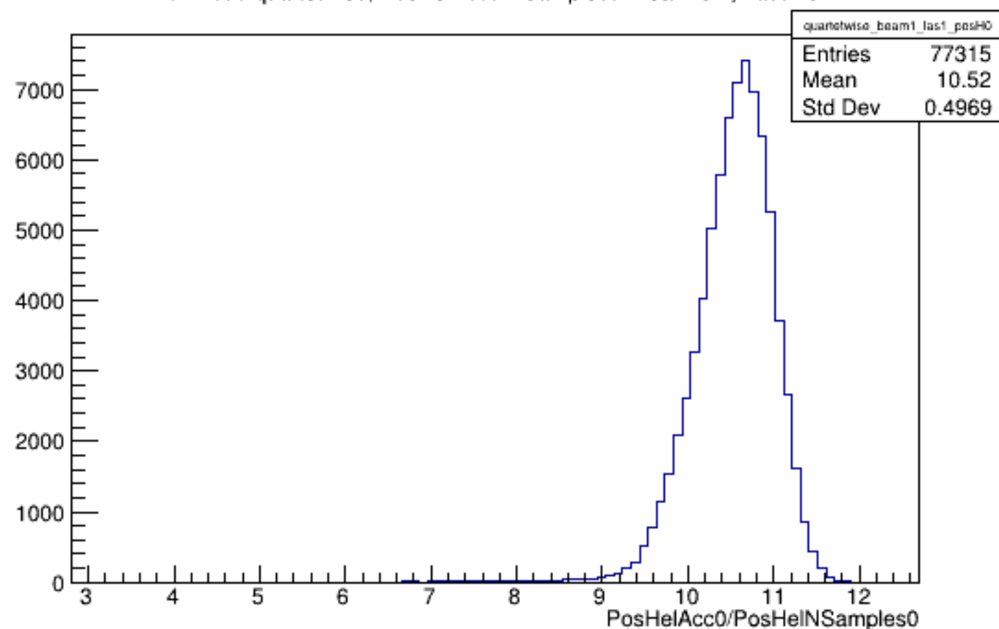
Run 4590 quartetwise, PosHelAcc0/NSamples0: Beam ON, Laser ON
