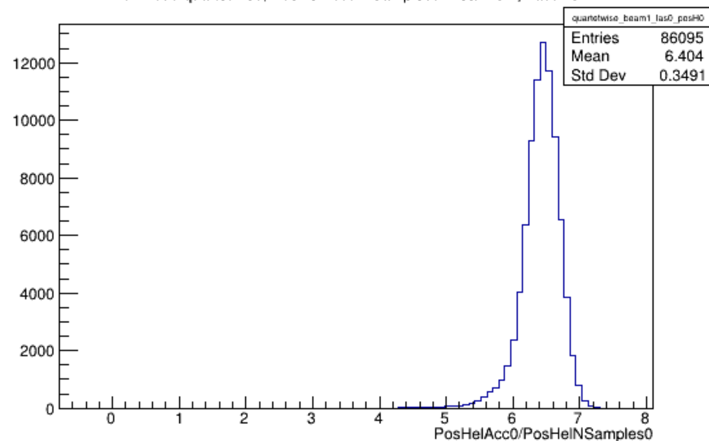
Run 4590 quartetwise, PosHelAcc0/NSamples0: Beam ON, Laser OFF
