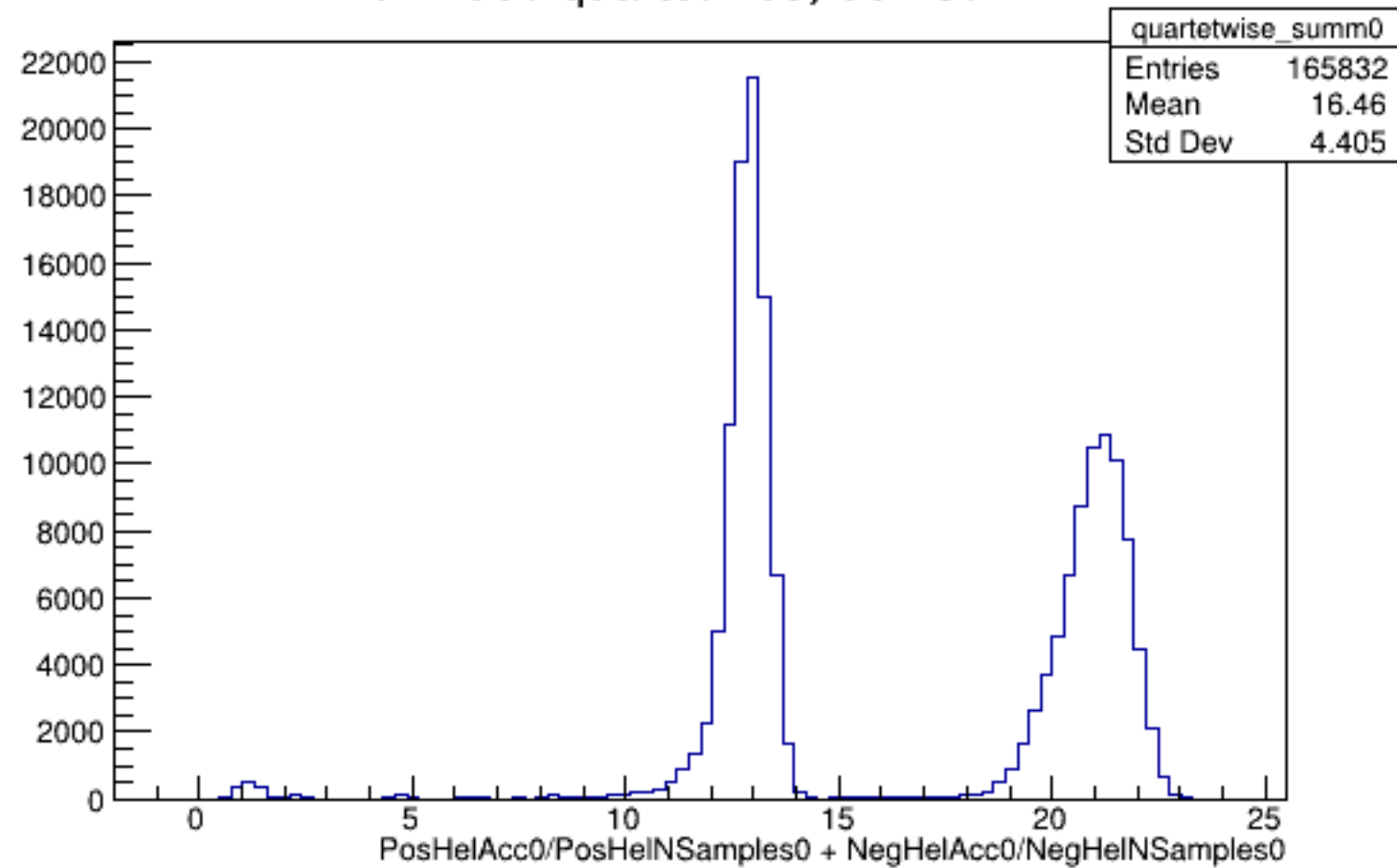
Run 4590 quartetwise, Sums0: All
