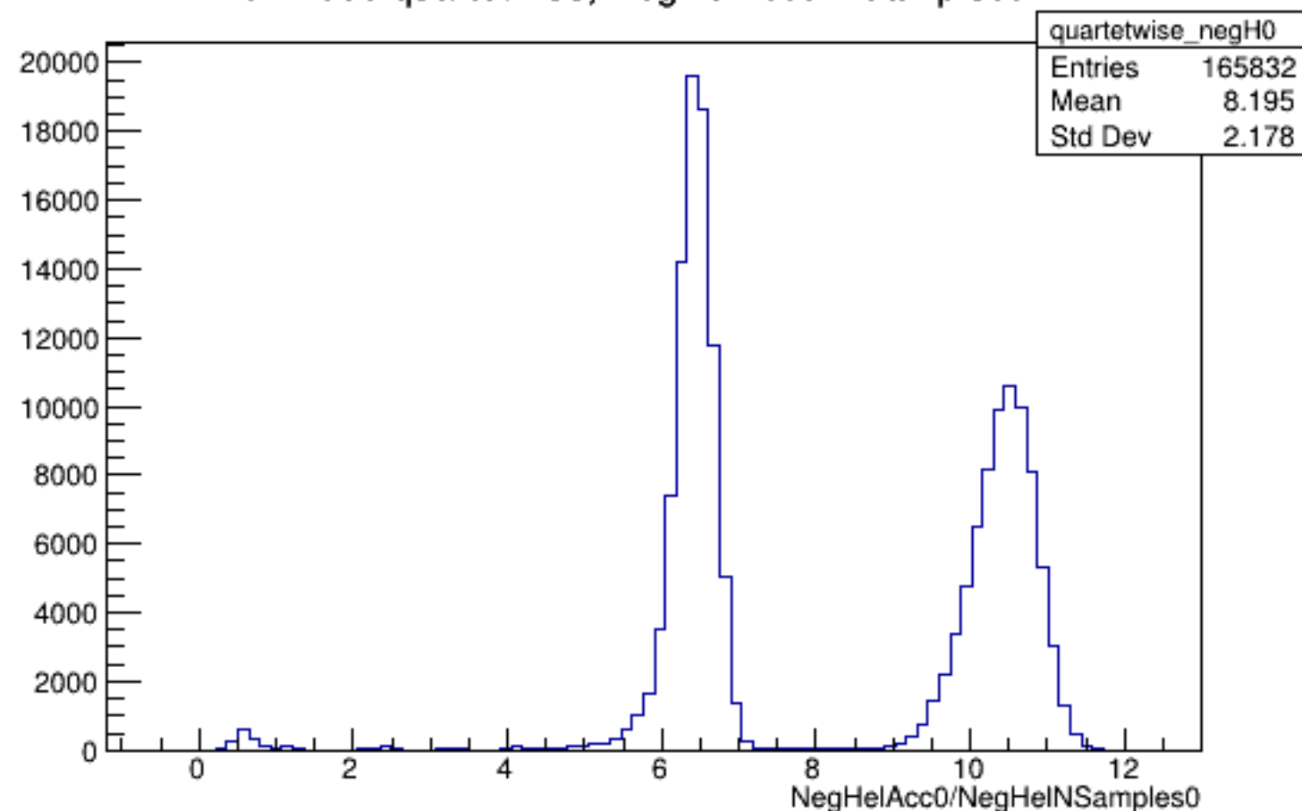
Run 4590 quartetwise, NegHelAcc0/NSamples0: All
