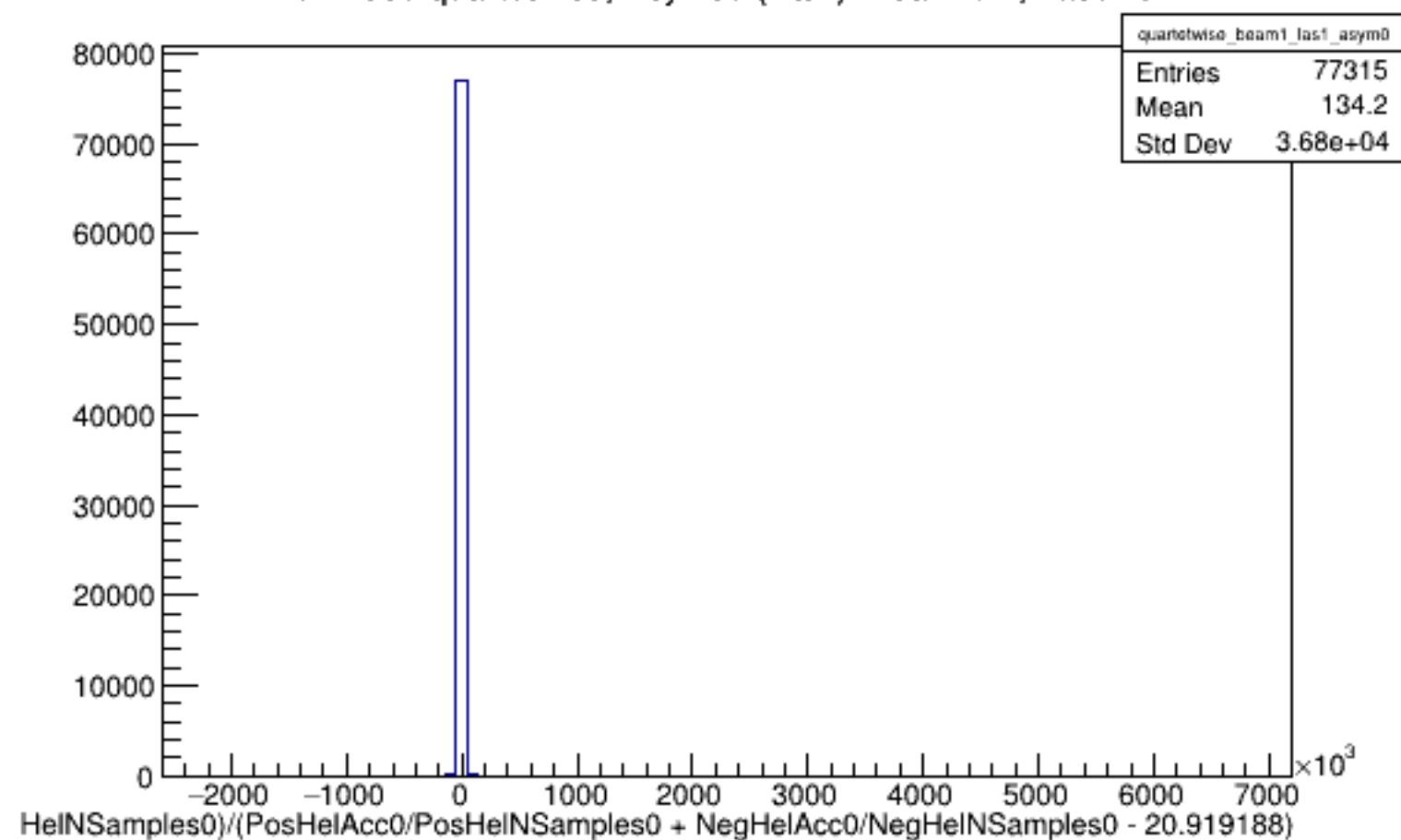
Run 4590 quartetwise, Asyms0 (Raw): Beam ON, Laser ON
