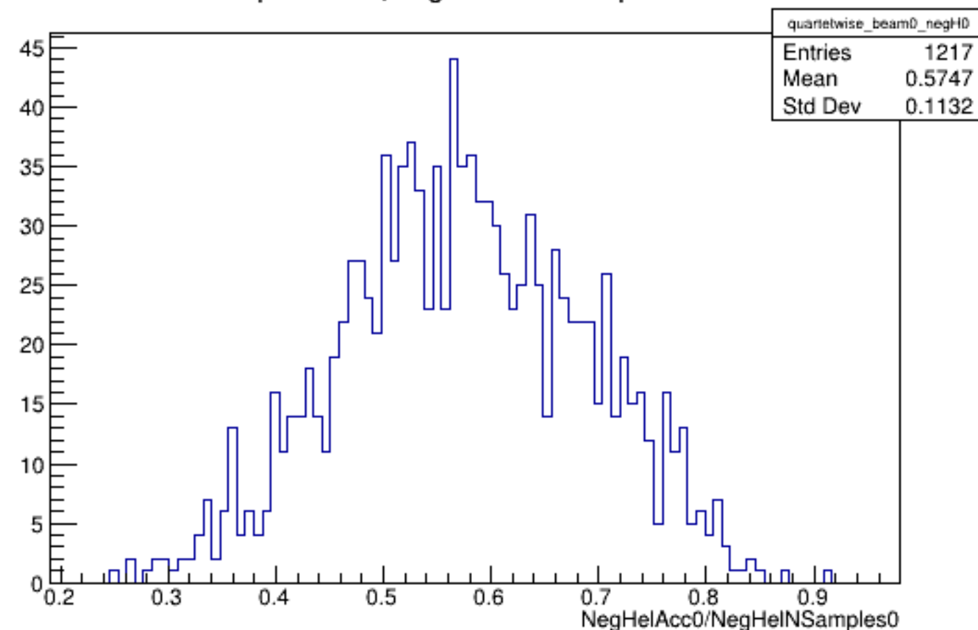
Run 4590 quartetwise, NegHelAcc0/NSamples0: Beam OFF
