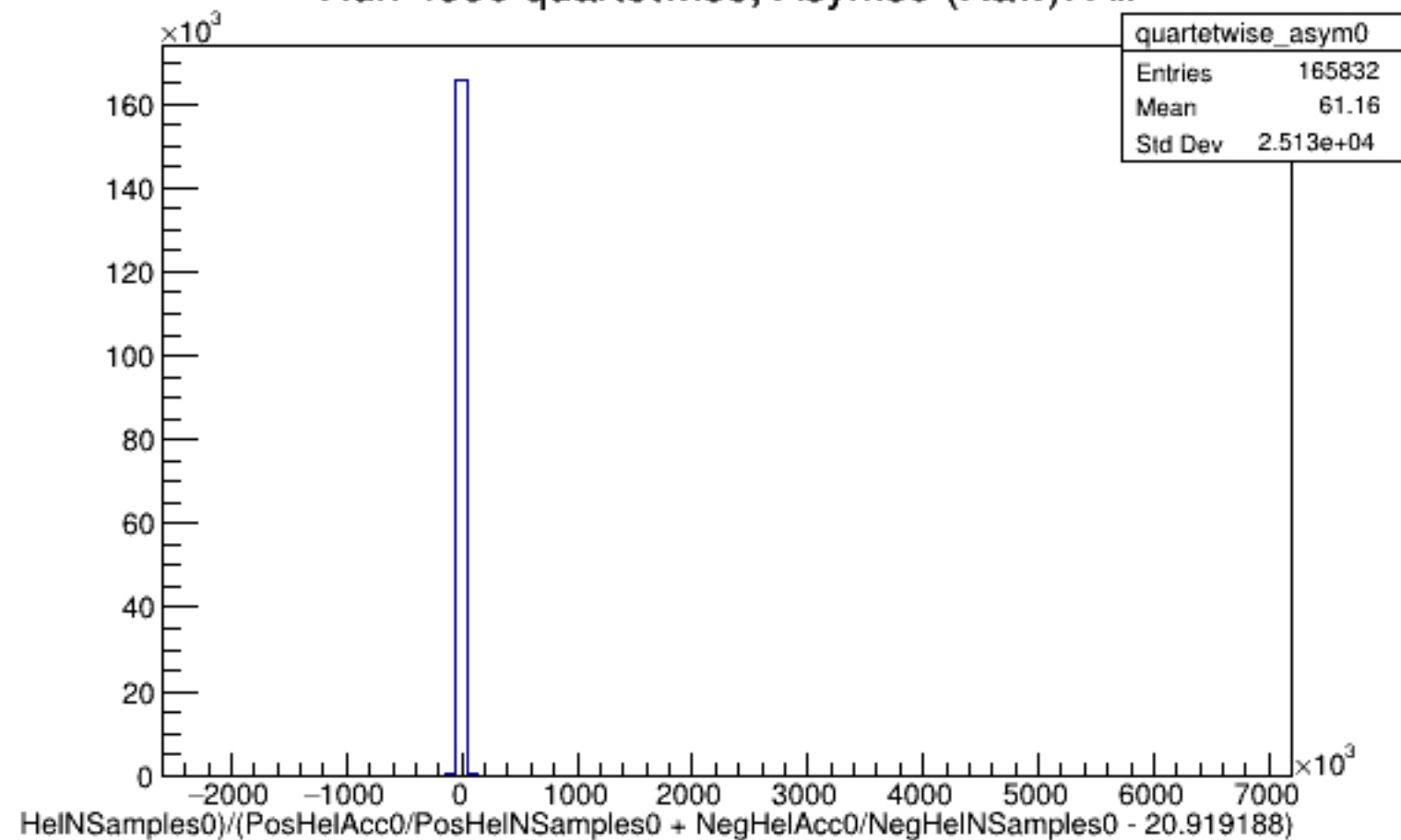
Run 4590 quartetwise, Asyms0 (Raw): All
