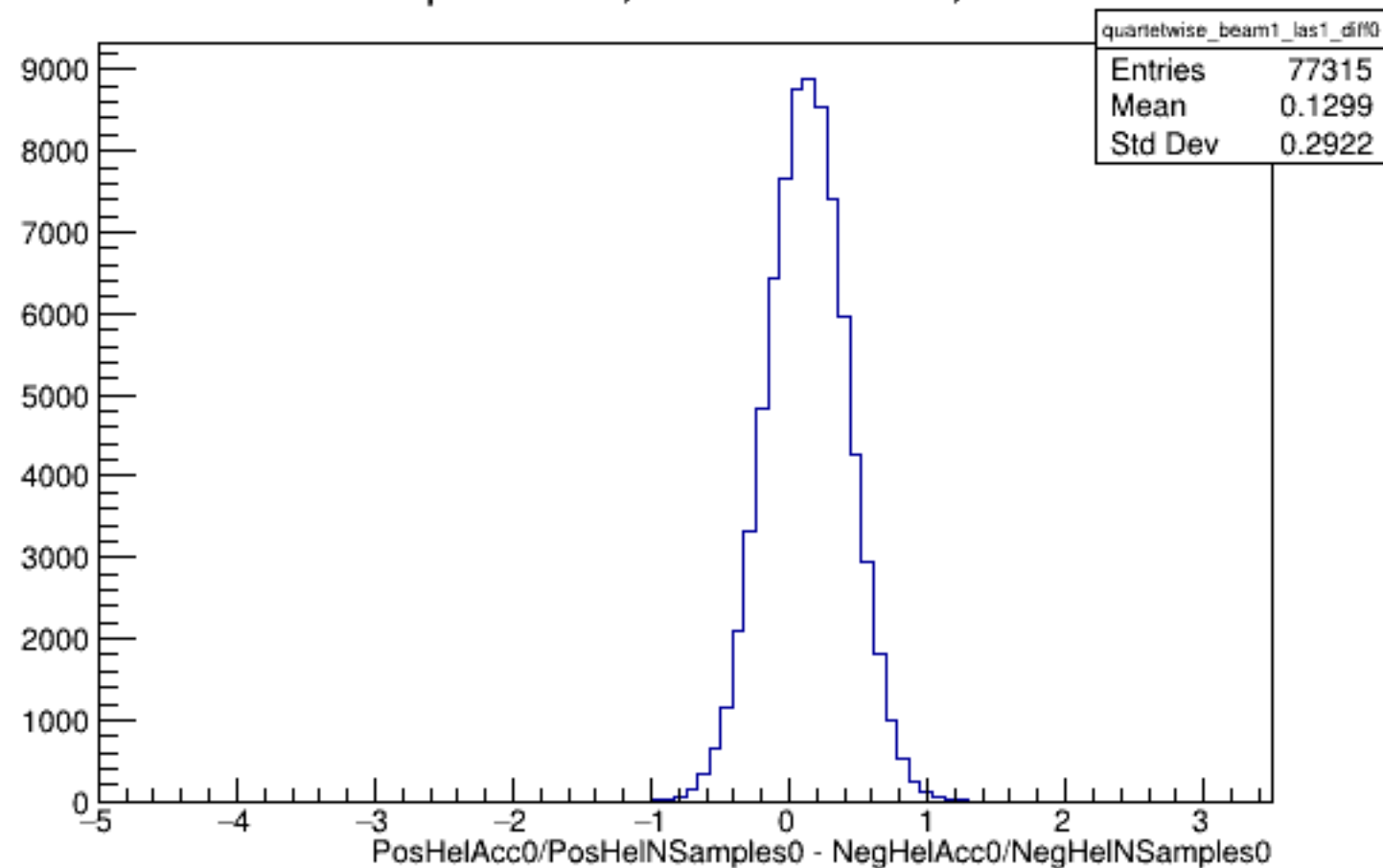
Run 4590 quartetwise, Diffs0: Beam ON, Laser ON
