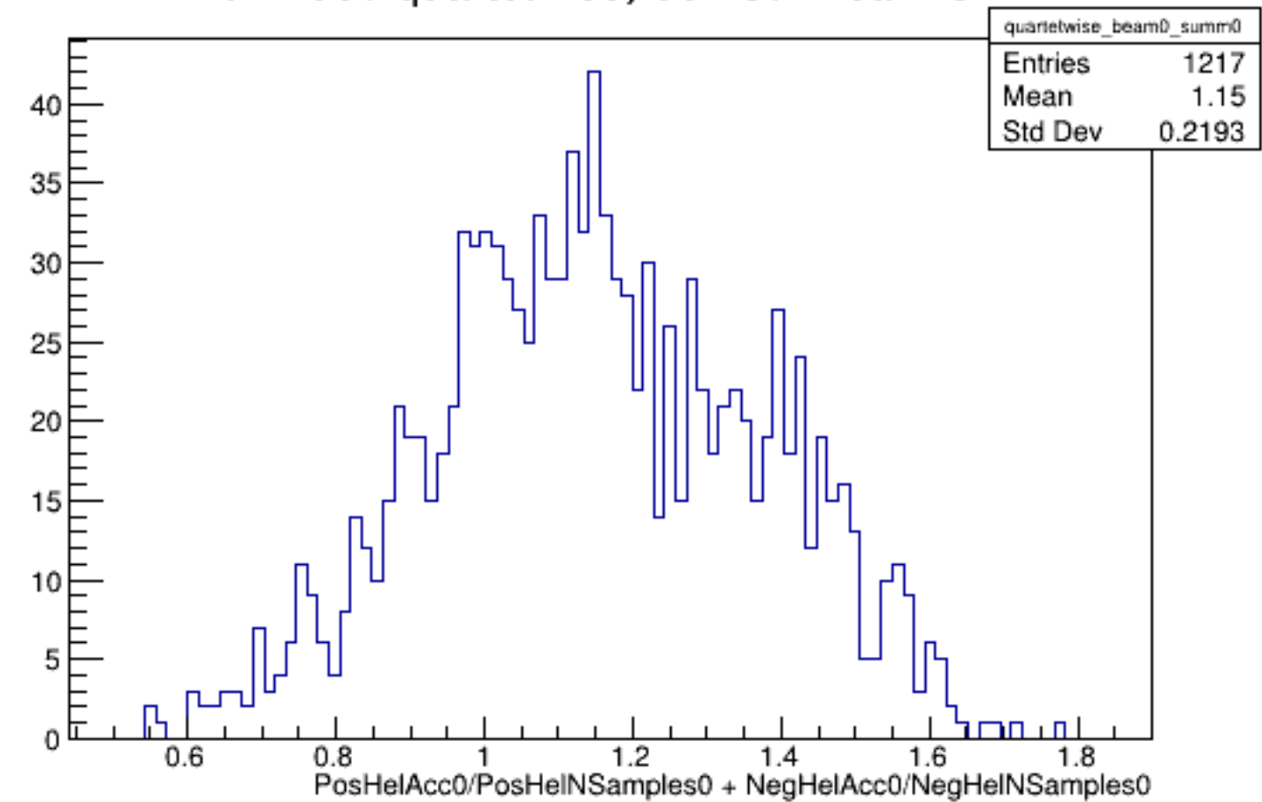
Run 4590 quartetwise, Sums0: Beam OFF
