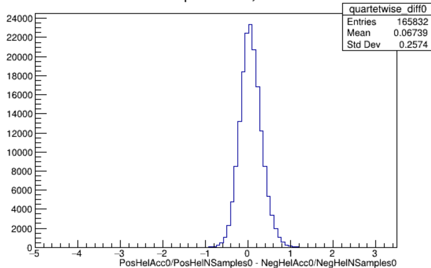
Run 4590 quartetwise, Diffs0: All
