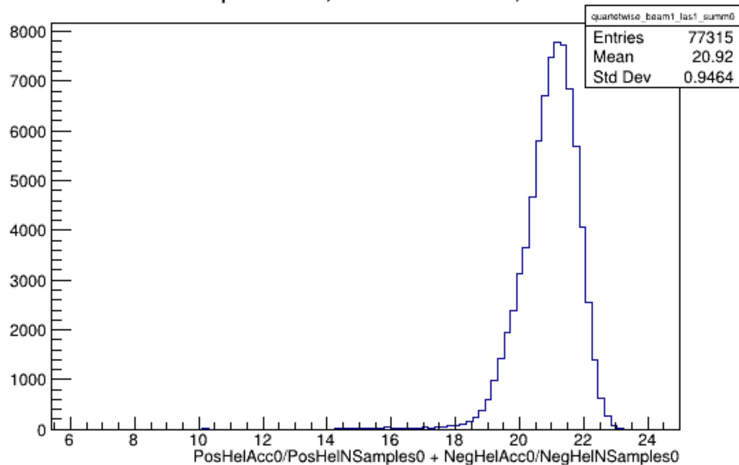
Run 4590 quartetwise, Sums0: Beam ON, Laser ON
