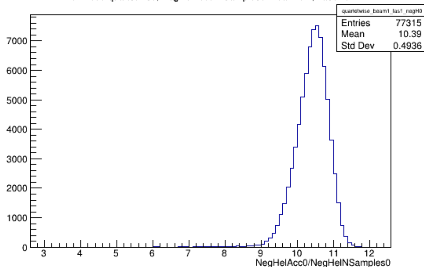
Run 4590 quartetwise, NegHelAcc0/NSamples0: Beam ON, Laser ON
