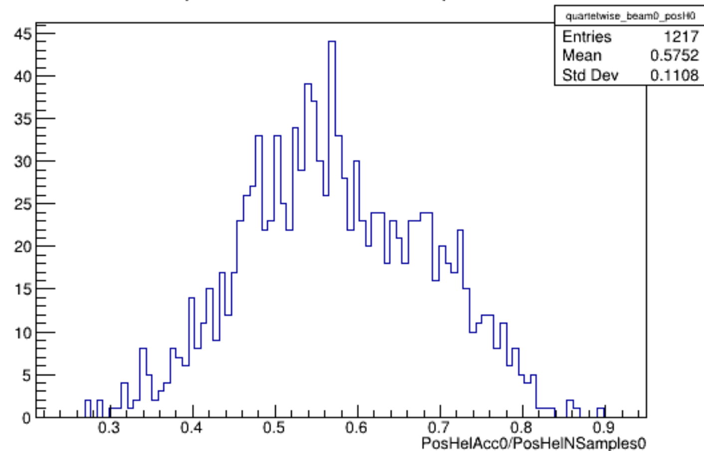
Run 4590 quartetwise, PosHelAcc0/NSamples0: Beam OFF
