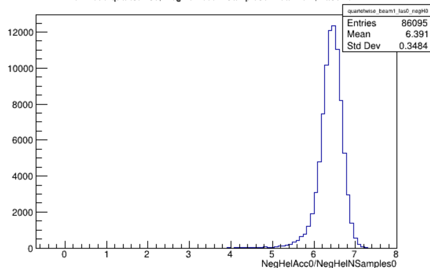
Run 4590 quartetwise, NegHelAcc0/NSamples0: Beam ON, Laser OFF
