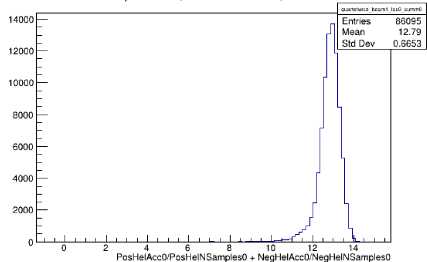
Run 4590 quartetwise, Sums0: Beam ON, Laser OFF
