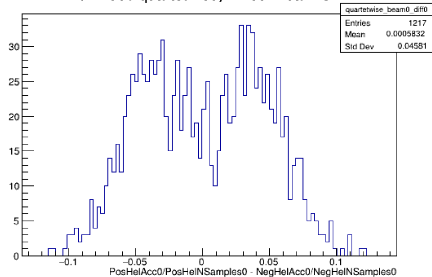
Run 4590 quartetwise, Diffs0: Beam OFF
