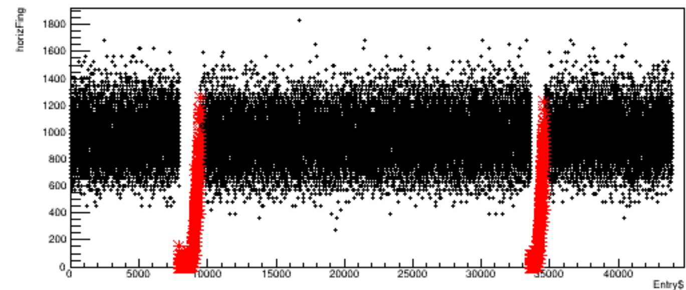
Run 4599, quartetwise: horizFing vs time
