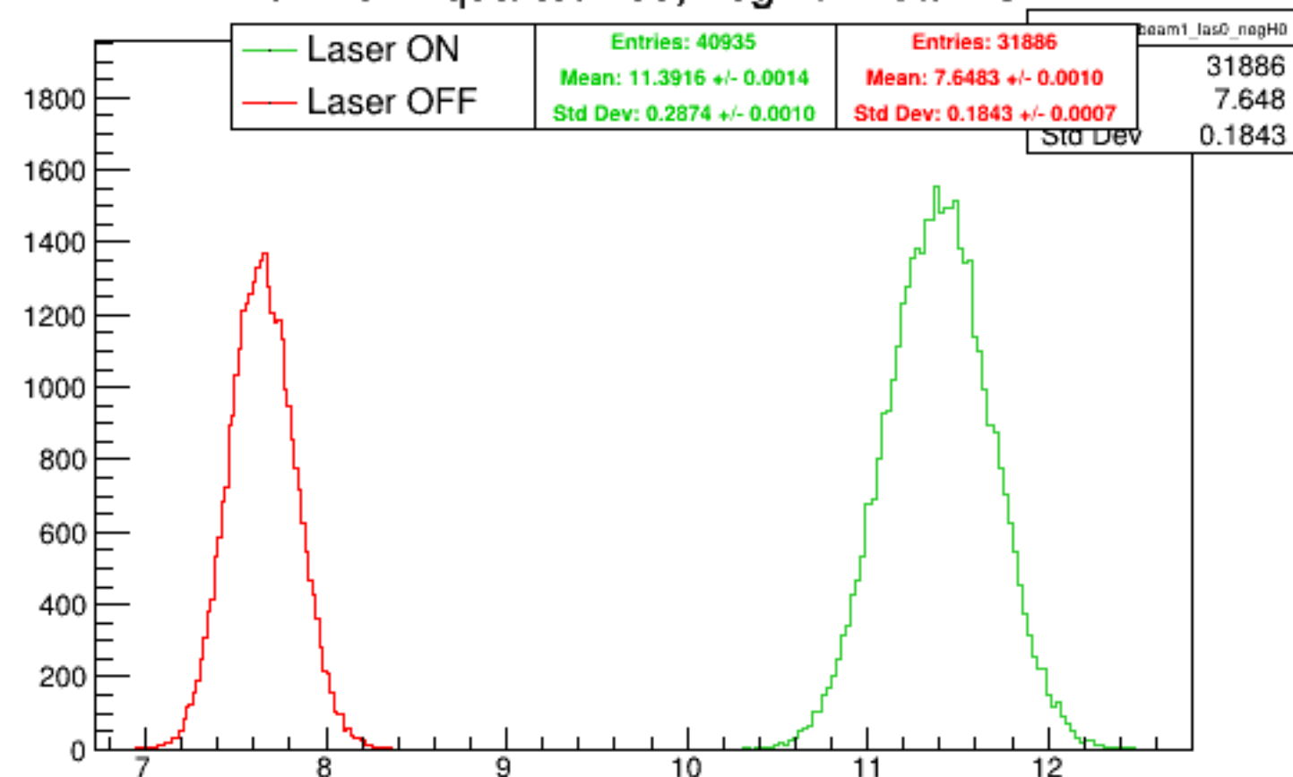
Run 4622 quartetwise, negH0: Beam ON
