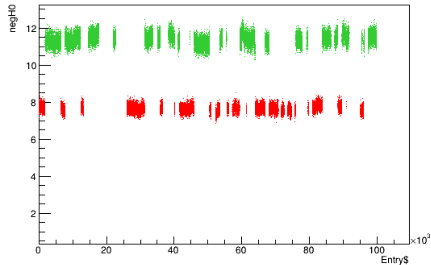
Run 4622 quartetwise, negH0 vs time
