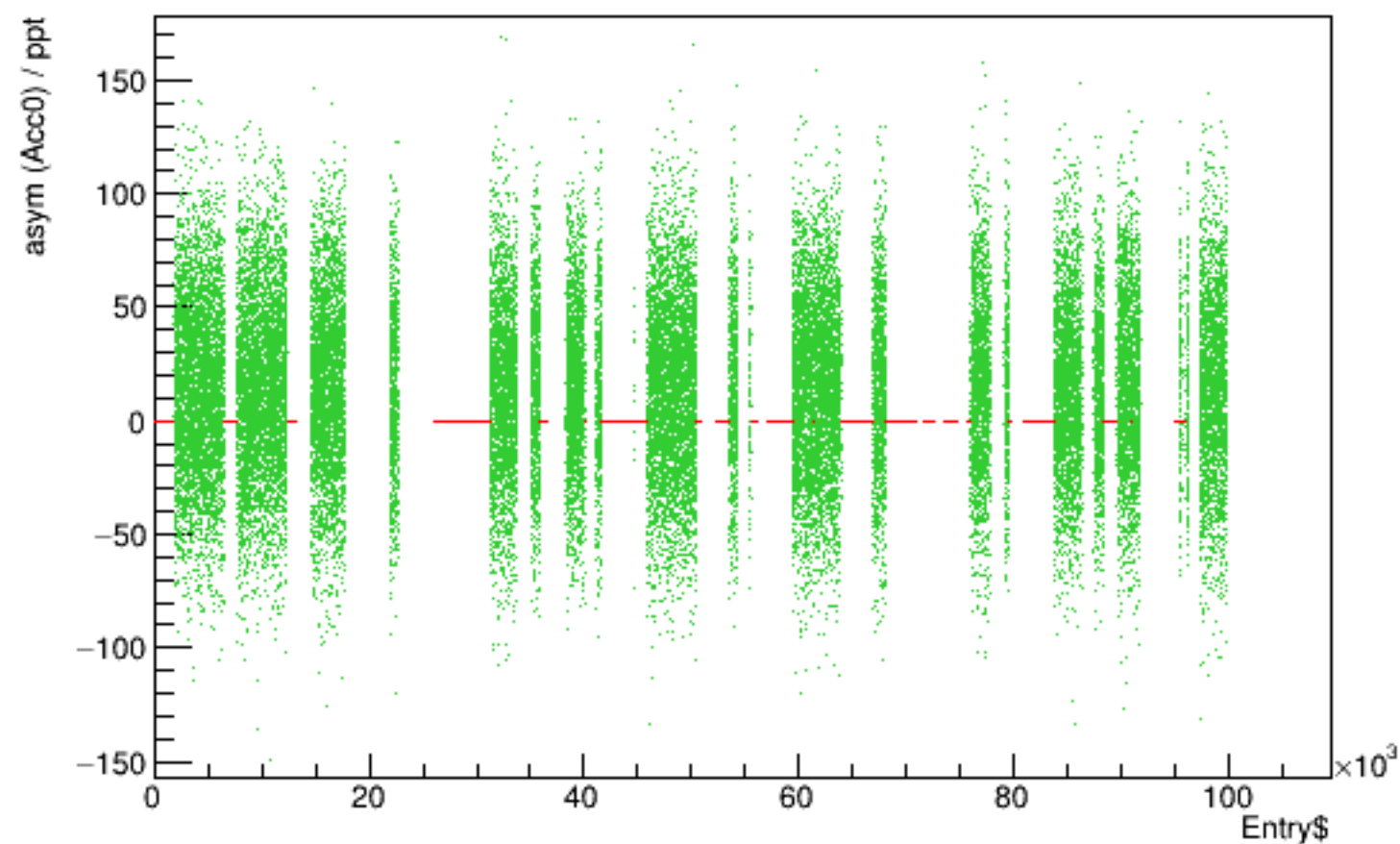
Run 4622 quartetwise, asym0sub vs time
