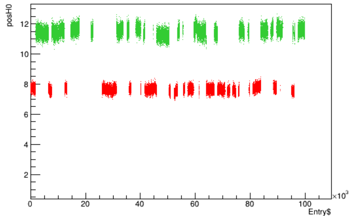
Run 4622 quartetwise, posH0 vs time
