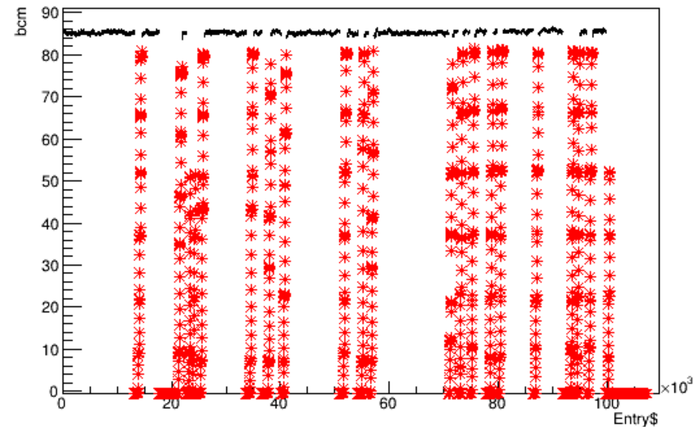
Run 4622 quartetwise, bcm vs time
