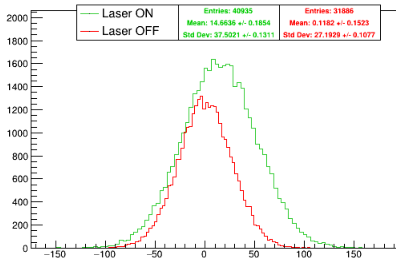
Run 4622 quartetwise, asym0sub: Beam ON
