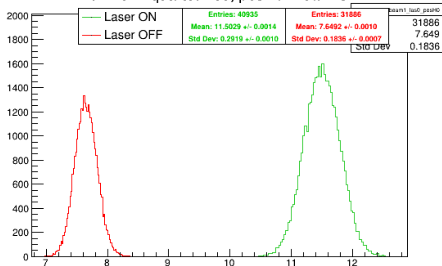
Run 4622 quartetwise, posH0: Beam ON
