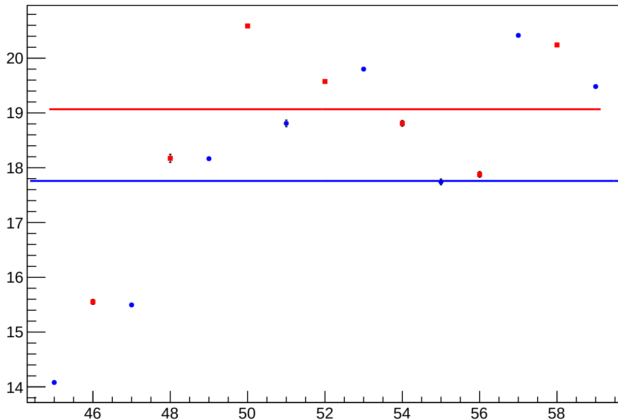
dit_dsr_4eY_slope vs slug
