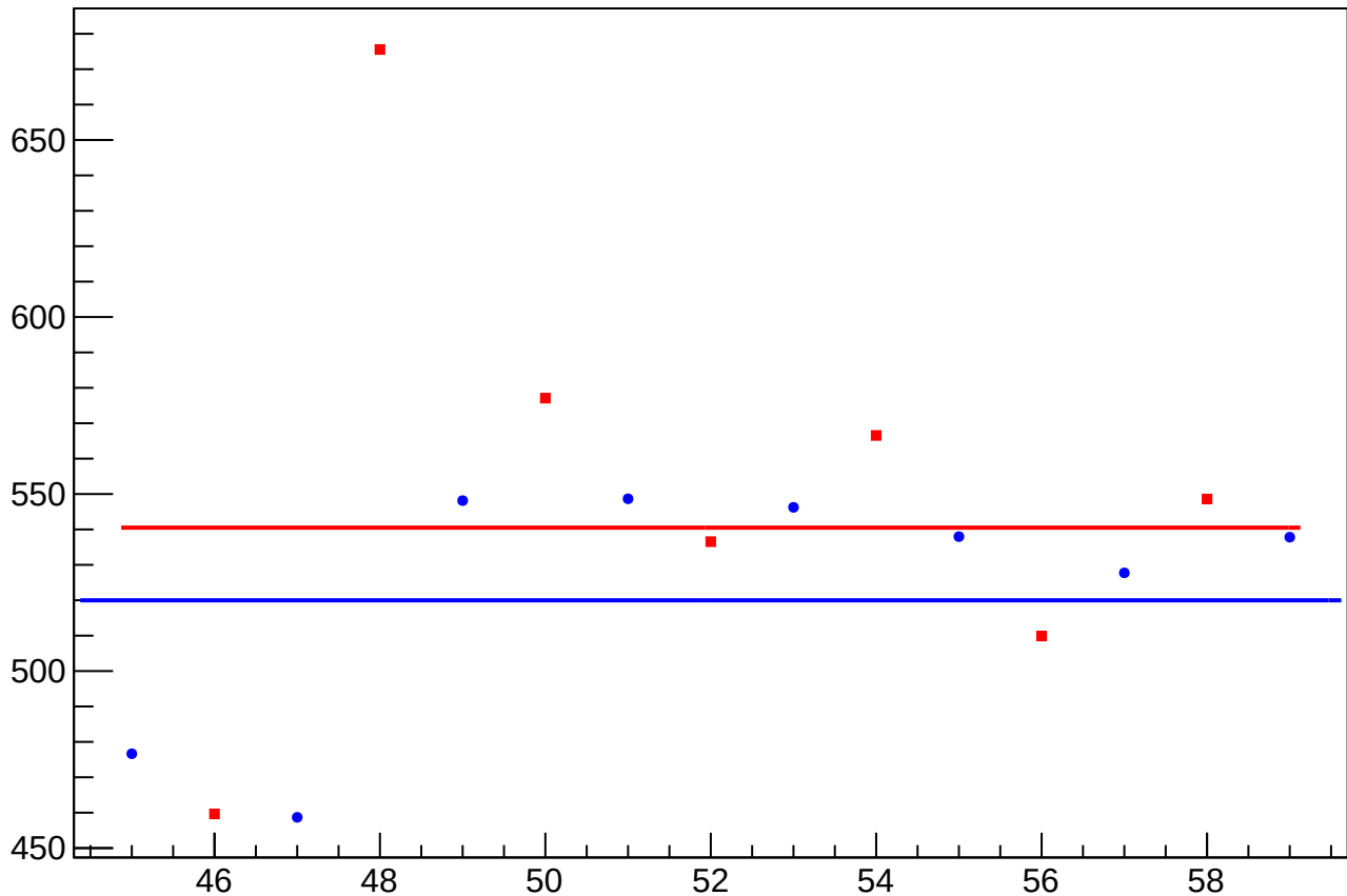
dit_asym_atr1_rms vs slug
