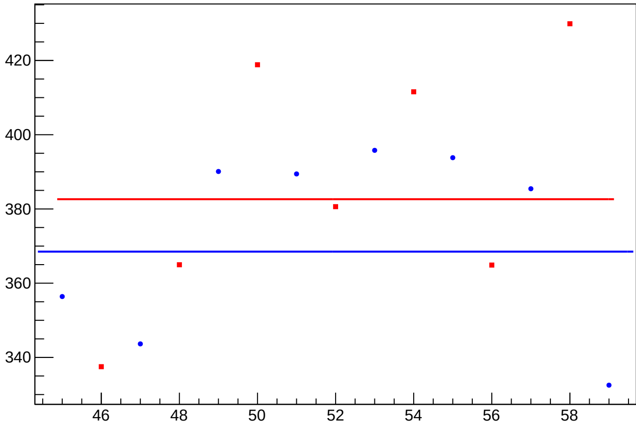
dit_asym_atl2_rms vs slug
