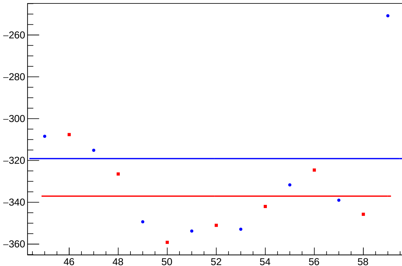
reg_asym_atl2_diff_bpm11X_slope vs slug
