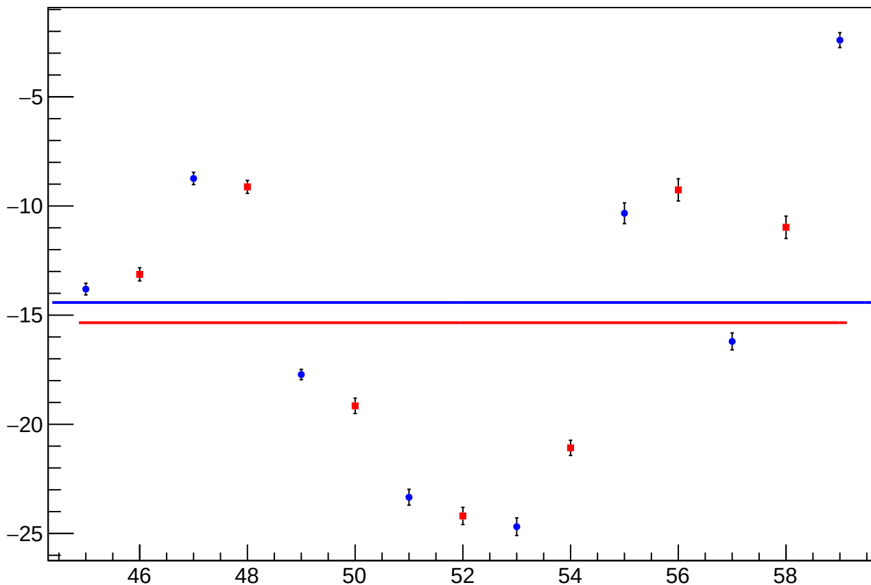
reg_asym_us_avg_diff_bpm4aX_slope vs slug
