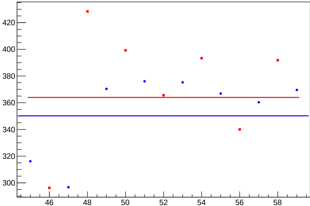
dit_asym_atr_avg_rms vs slug
