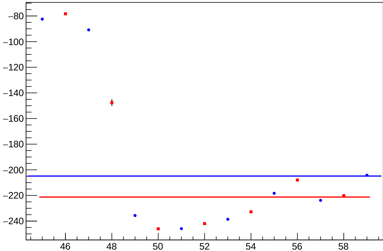
dit_atr1_11X12X_slope vs slug
