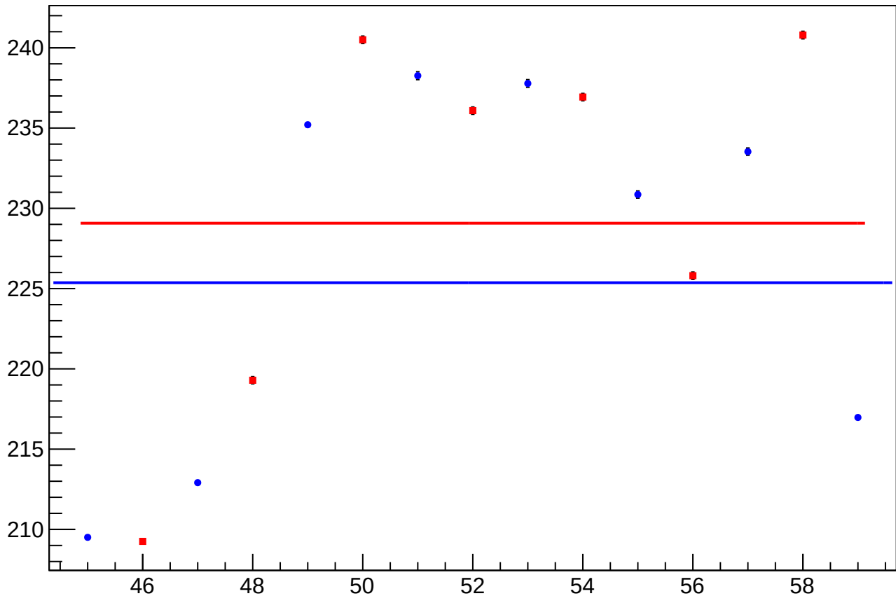
dit_asym_at2_dd_rms vs slug
