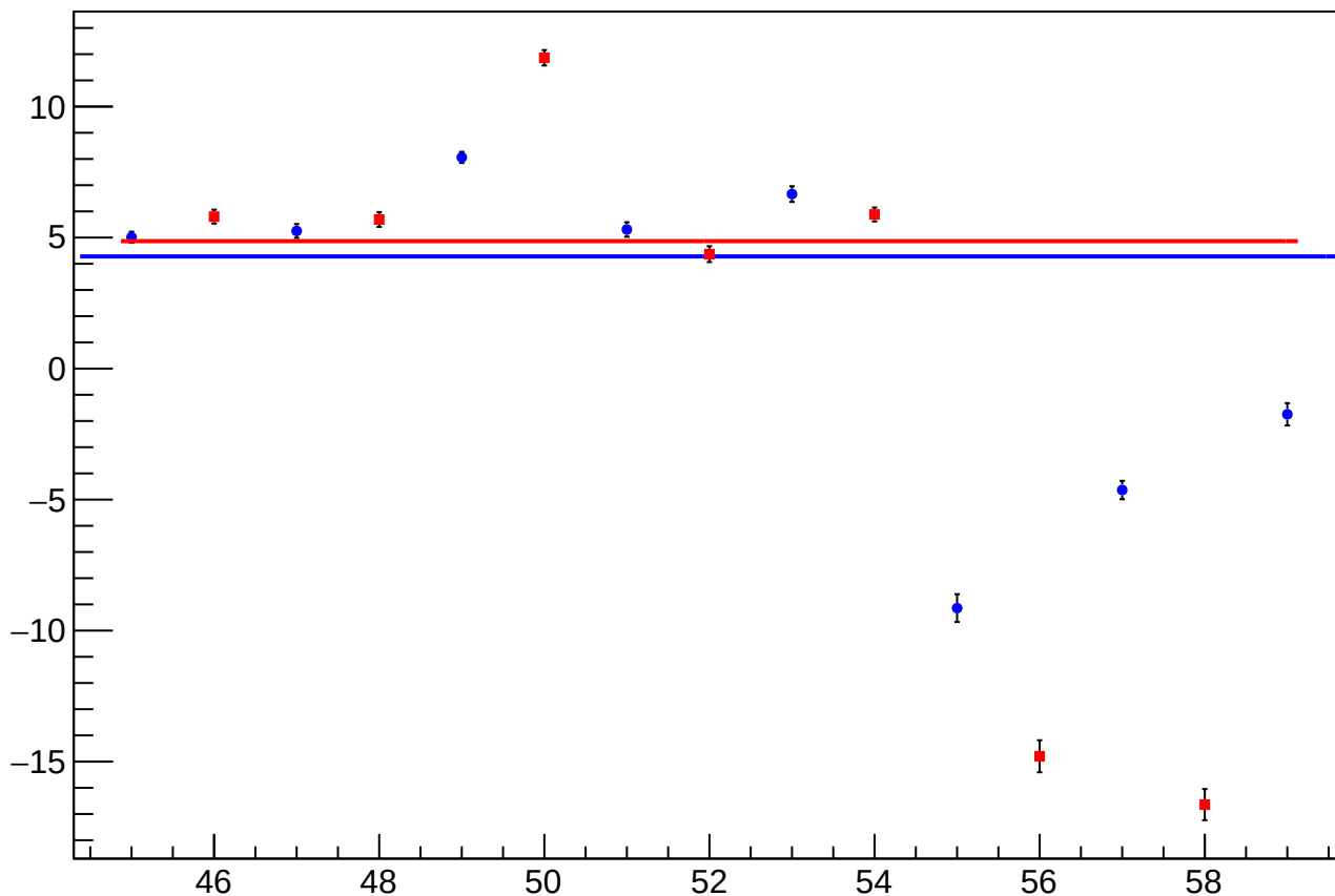
reg_asym_ds_avg_diff_bpm4aY_slope vs slug
