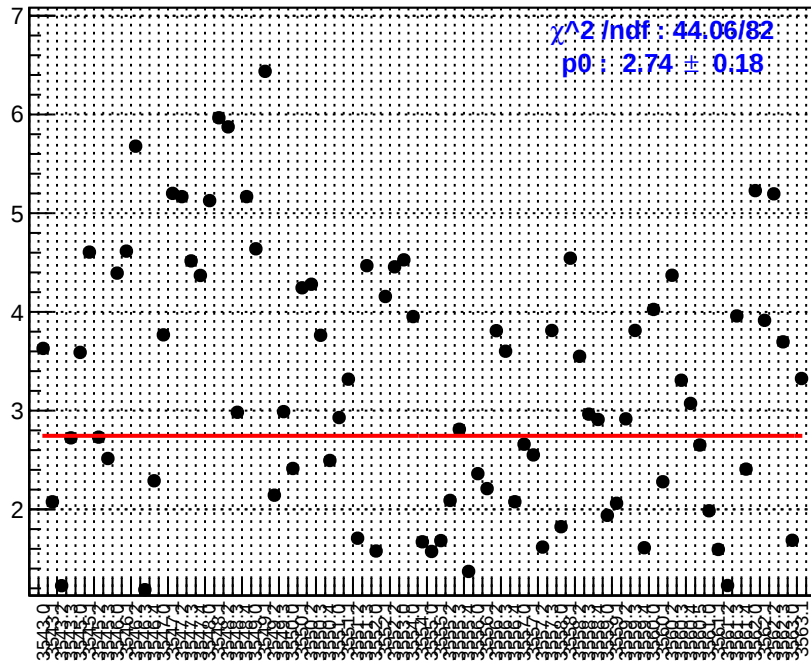
slug10: usr_bpm4eY
