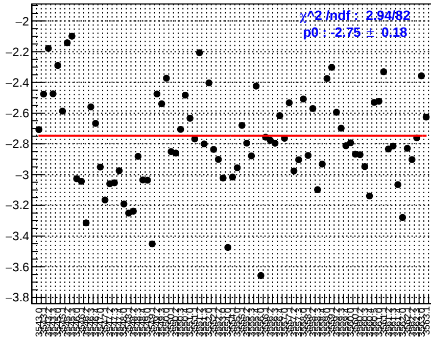
slug10: us_avg_bpm4aY
