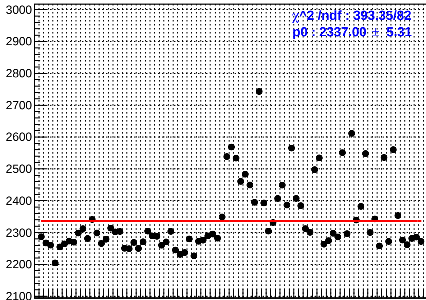
slug10: redi_asym_ds_avg.rms/ppm
