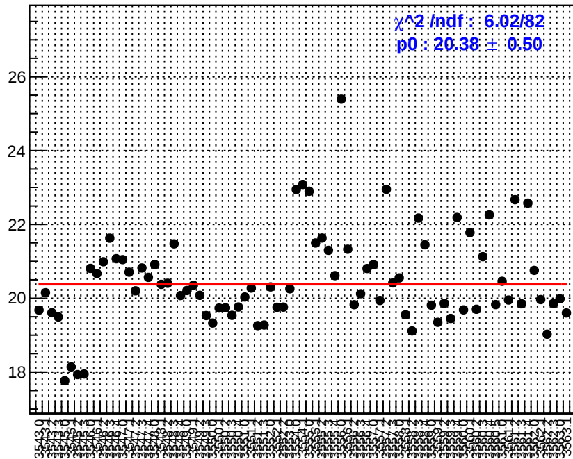
slug10: usl_bpm4eY
