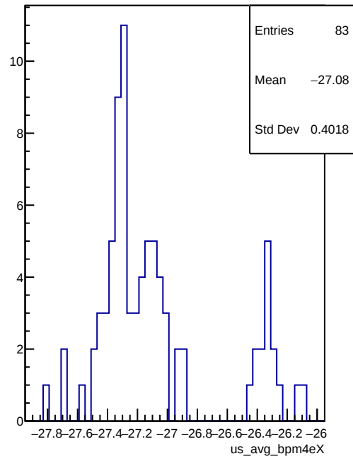
us_avg_bpm4eX
