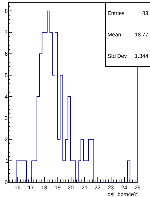
dsl_bpm4eY
