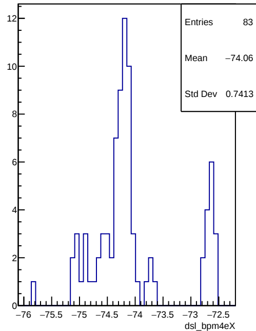
dsl_bpm4eX
