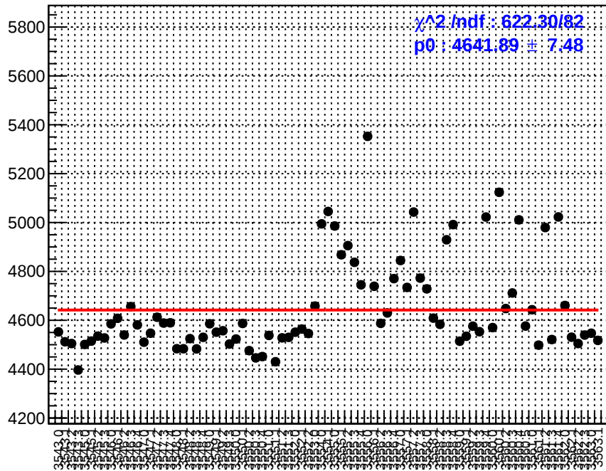
slug10: redi_asym_dsr.rms/ppm
