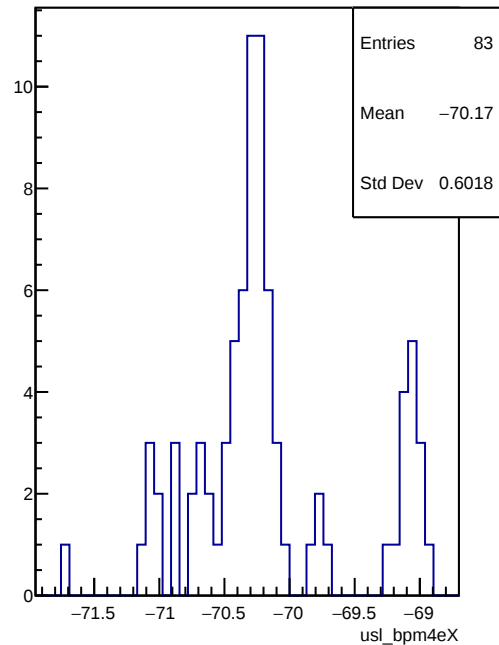
usl_bpm4eX
