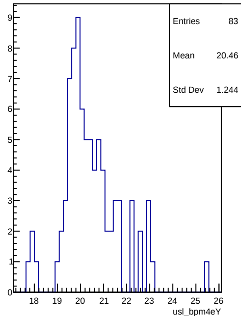
usl_bpm4eY
