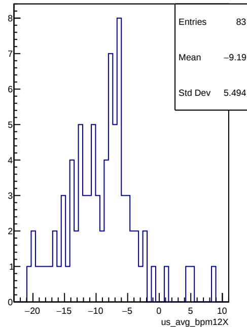
us_avg_bpm12X
