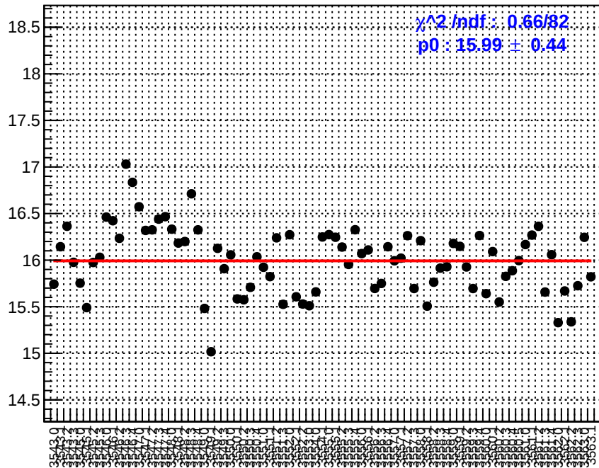
slug10: usr_bpm4eX
