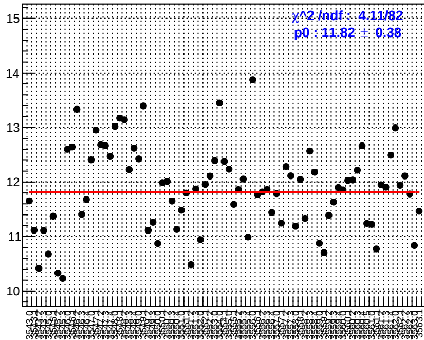
slug10: us_avg_bpm4eY
