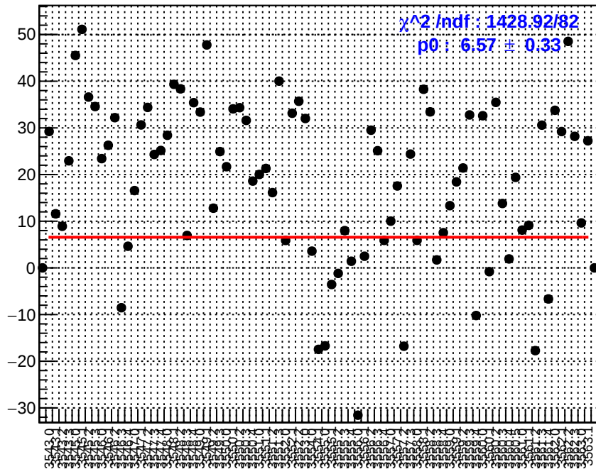
slug10: us_dd_bpm4aX
