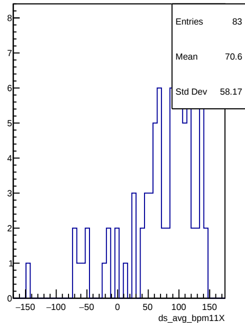
ds_avg_bpm11X
