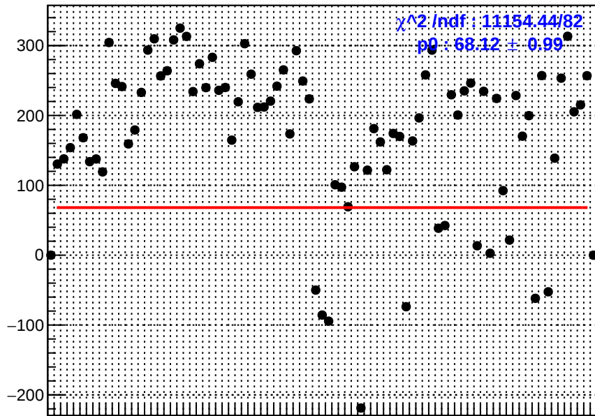
slug10: dsr_bpm11X
