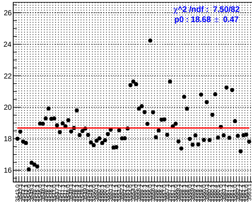
slug10: dsl_bpm4eY
