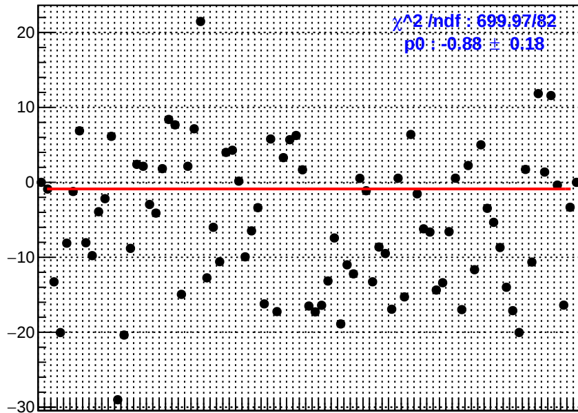
slug10: usr_bpm12X
