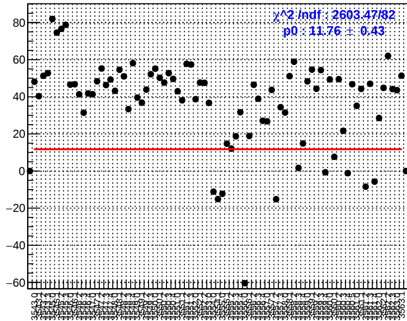
slug10: dsl_bpm4aX
