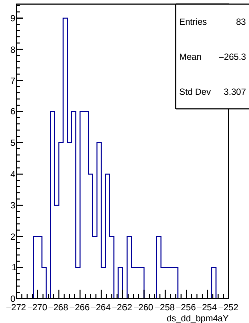
ds_dd_bpm4aY
