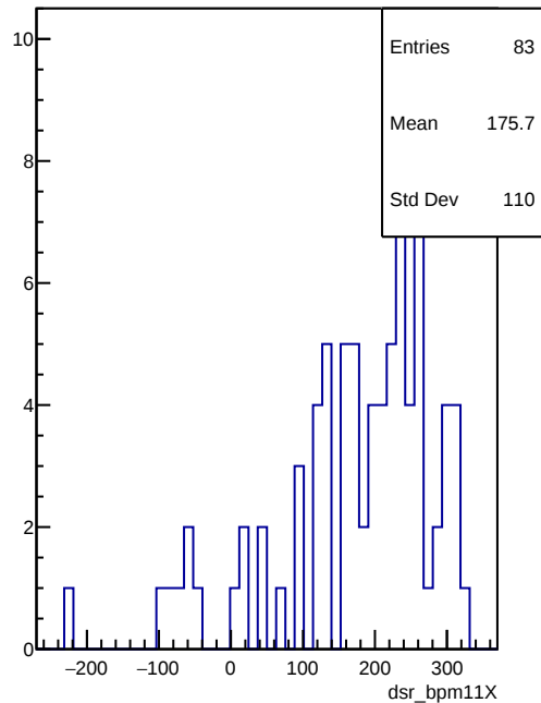
dsr_bpm11X
