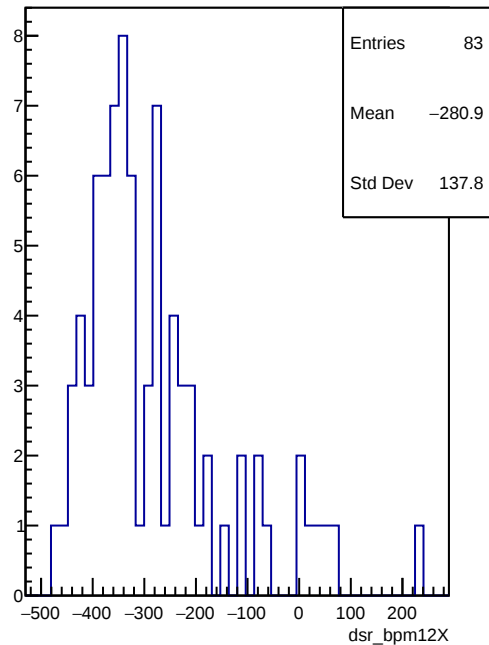
dsr_bpm12X
