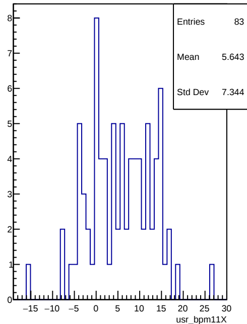
usr_bpm11X
