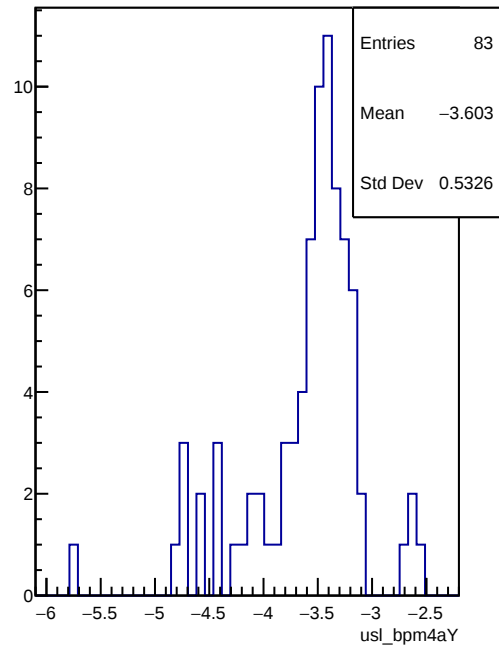
usl_bpm4aY
