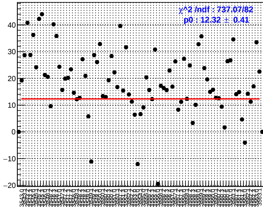
slug10: us_avg_bpm4aX
