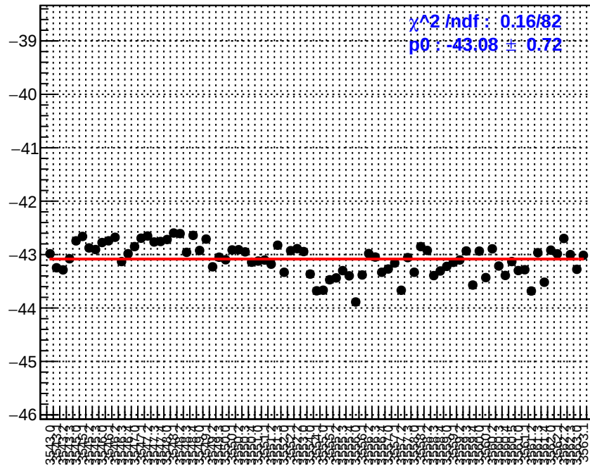
slug10: us_dd_bpm4eX
