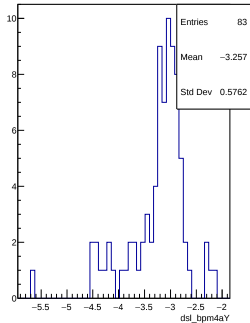
dsl_bpm4aY
