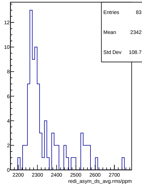
redi_asym_ds_avg.rms/ppm
