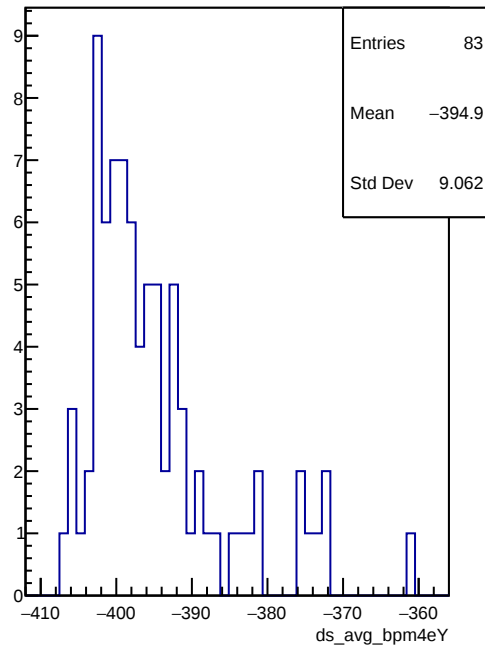
ds_avg_bpm4eY
