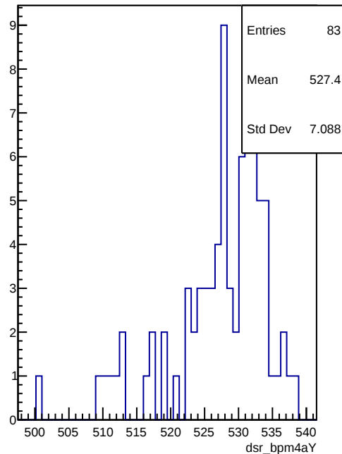
dsr_bpm4aY
