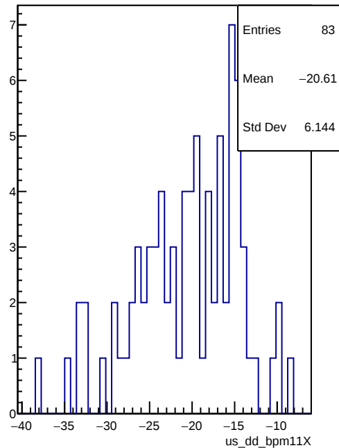
us_dd_bpm11X
