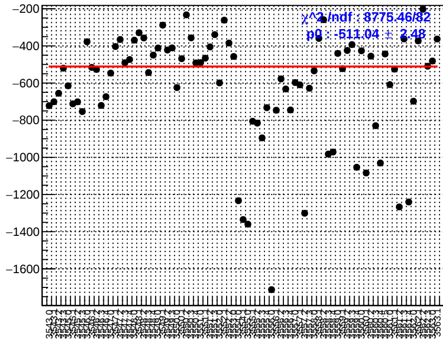
slug10: dsr_bpm4aX
