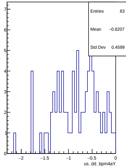
us_dd_bpm4aY
