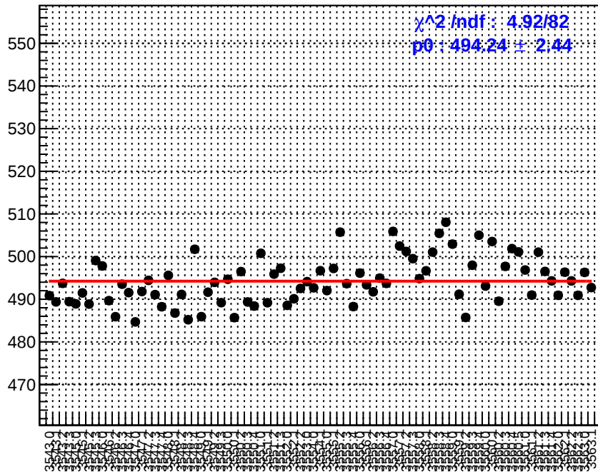
slug10: redi_asym_us_avg.rms/ppm
