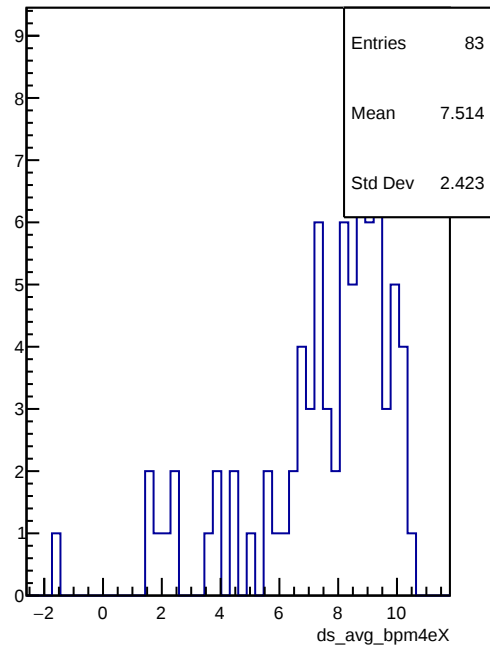
ds_avg_bpm4eX
