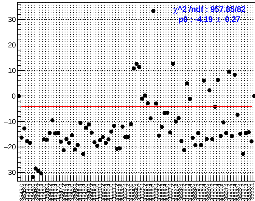
slug10: dsl_bpm12X
