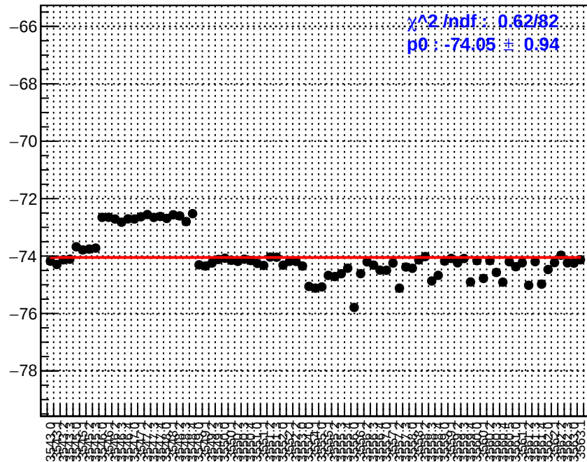
slug10: dsl_bpm4eX
