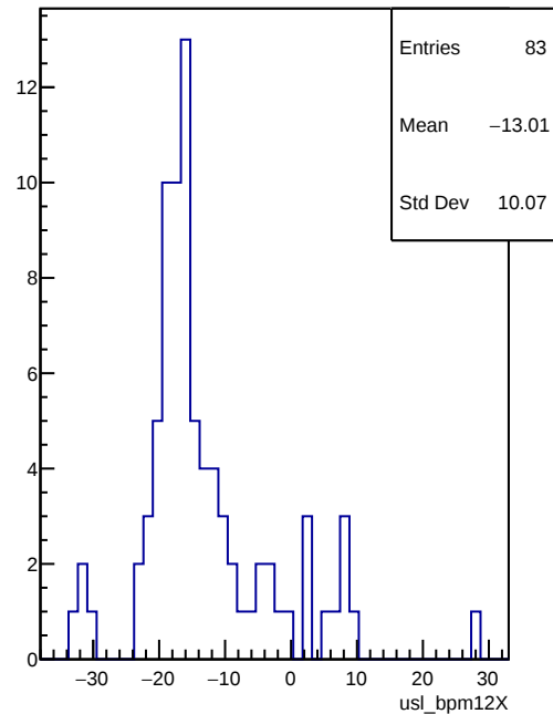
usl_bpm12X
