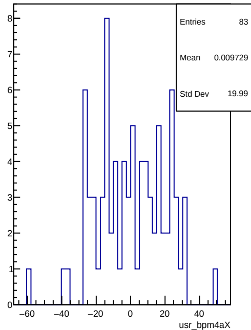
usr_bpm4aX
