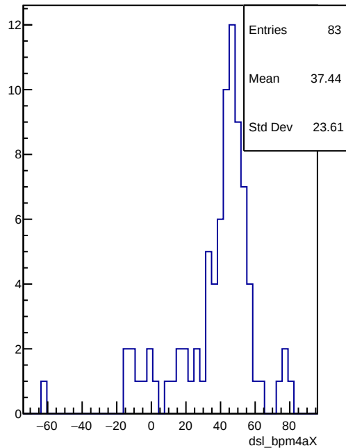
dsl_bpm4aX
