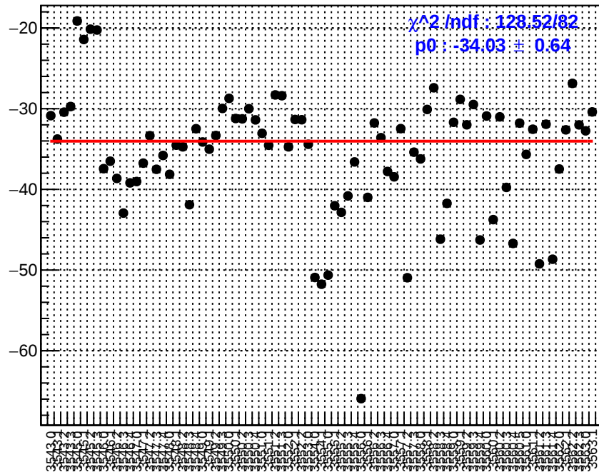
slug10: usl_bpm11X
