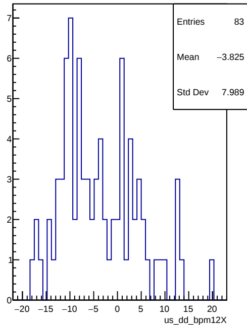
us_dd_bpm12X
