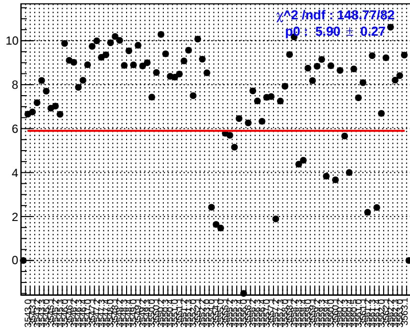
slug10: ds_avg_bpm4eX
