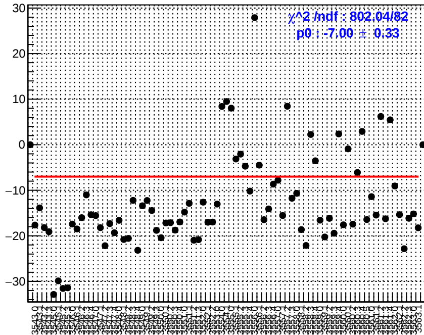
slug10: usl_bpm12X
