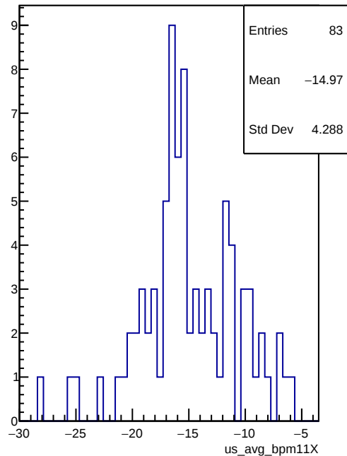
us_avg_bpm11X
