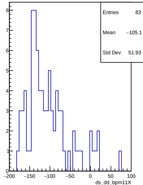
ds_dd_bpm11X
