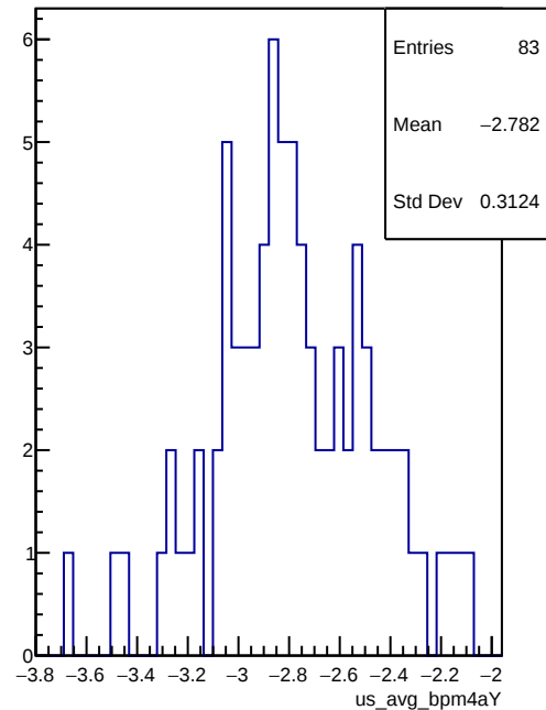
us_avg_bpm4aY
