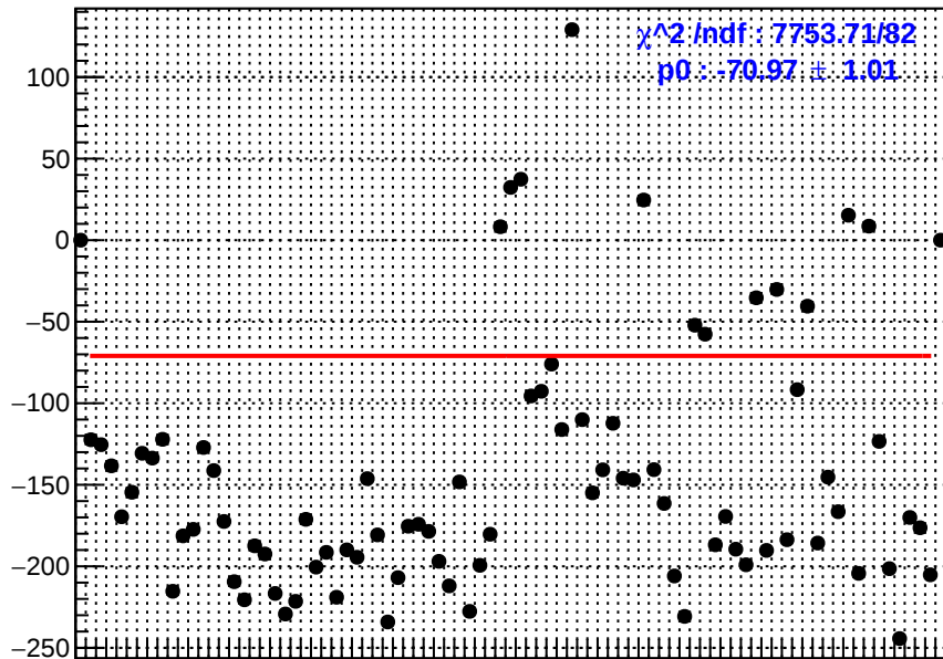
slug10: ds_avg_bpm12X
