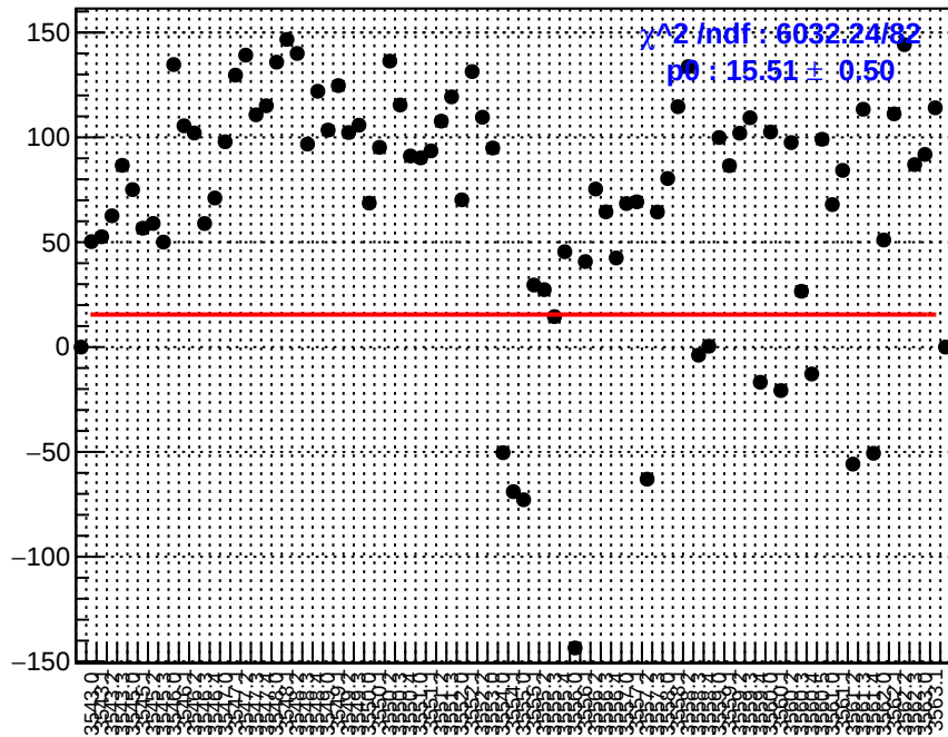
slug10: ds_avg_bpm11X
