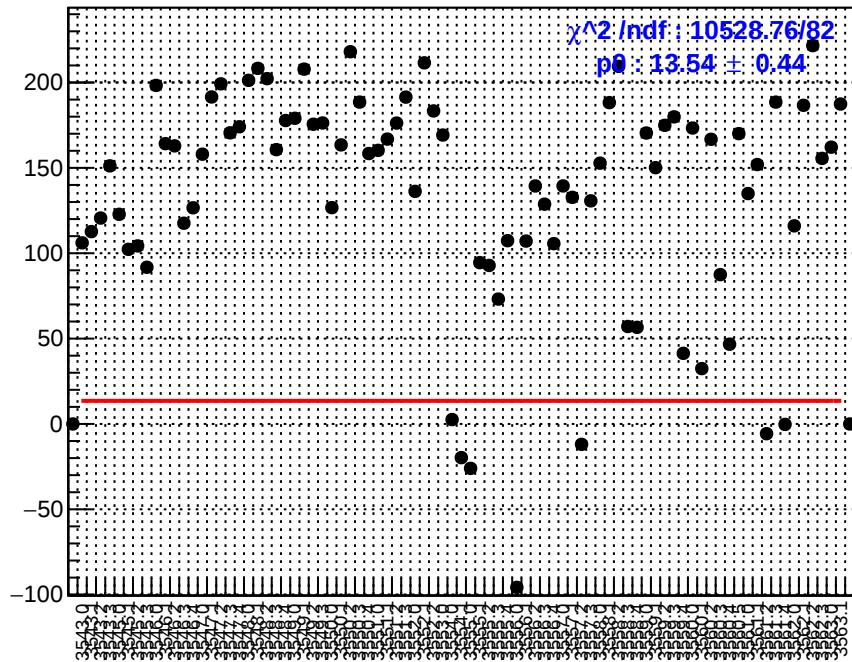
slug10: ds_dd_bpm12X
