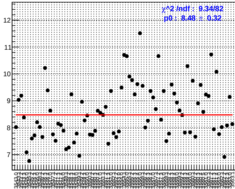
slug10: us_dd_bpm4eY
