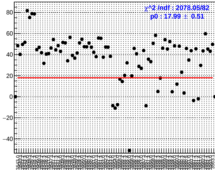
slug10: usl_bpm4aX
