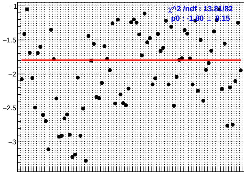
slug10: usr_bpm4aY
