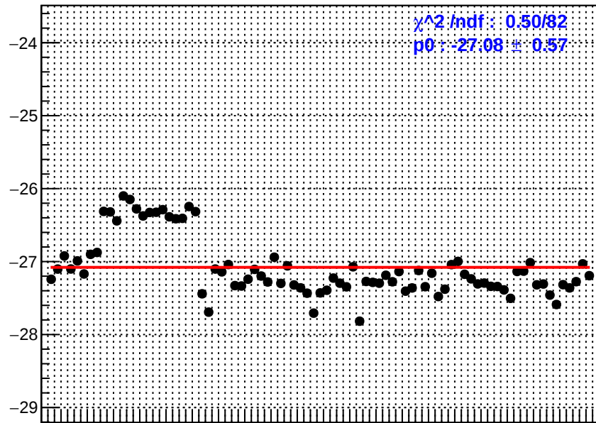
slug10: us_avg_bpm4eX
