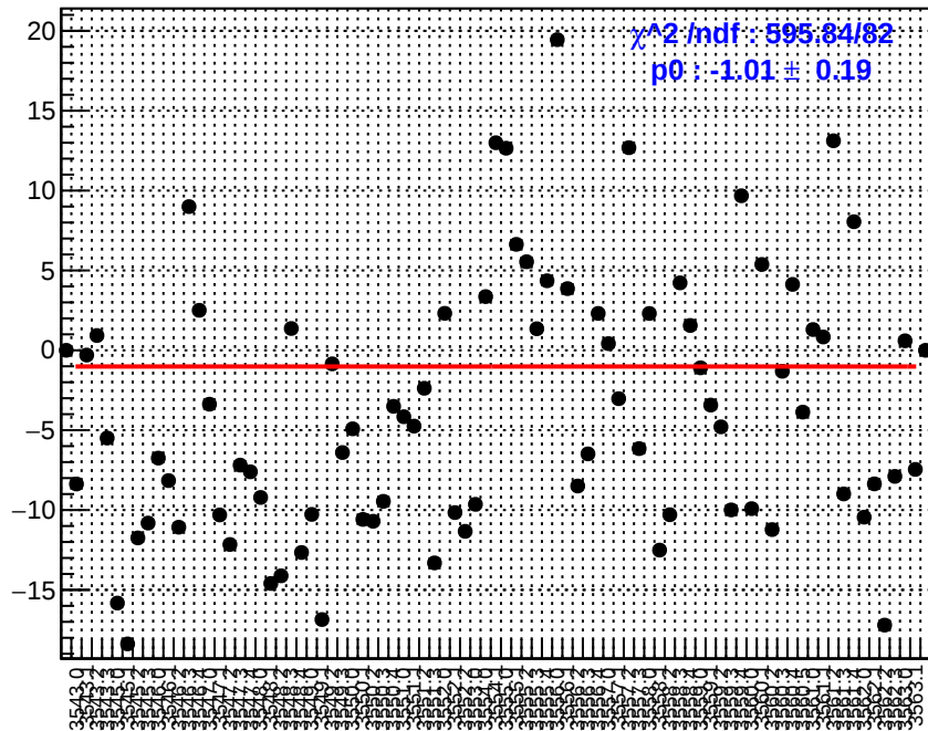
slug10: us_dd_bpm12X
