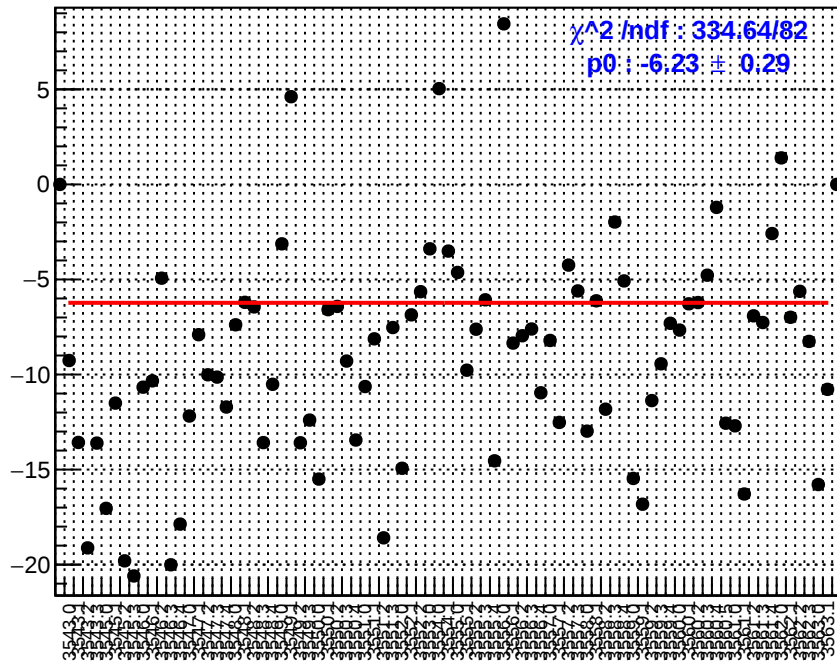
slug10: us_avg_bpm12X
