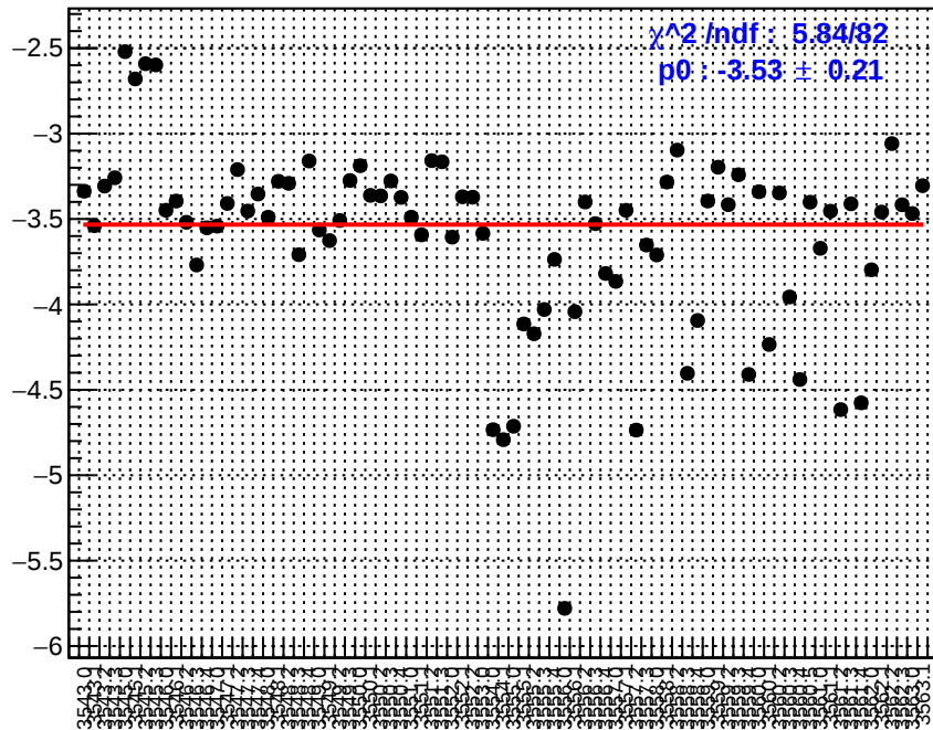
slug10: usl_bpm4aY
