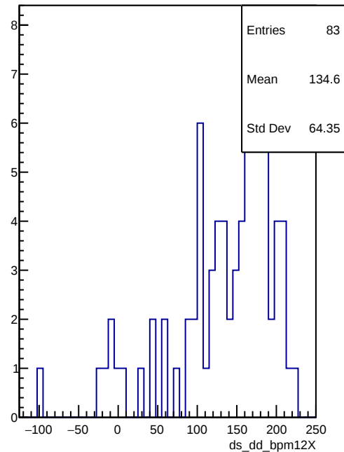
ds_dd_bpm12X
