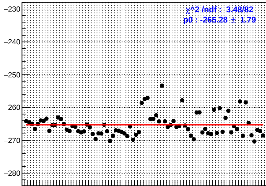
slug10: ds_dd_bpm4aY
