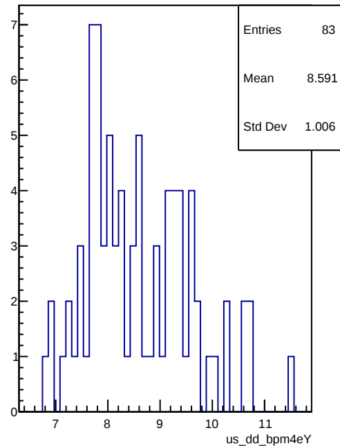
us_dd_bpm4eY
