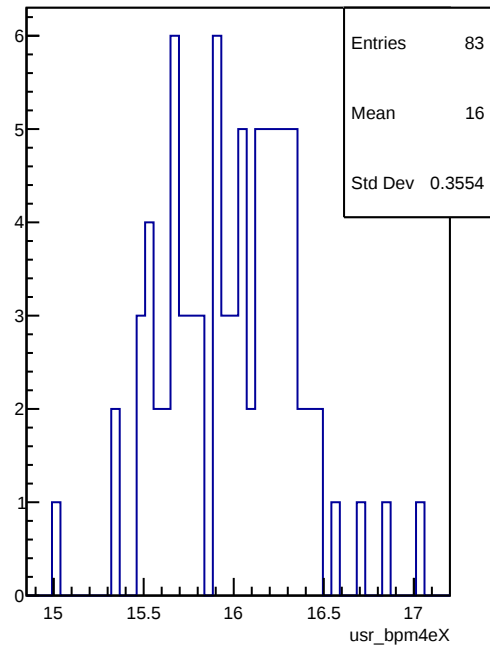
usr_bpm4eX
