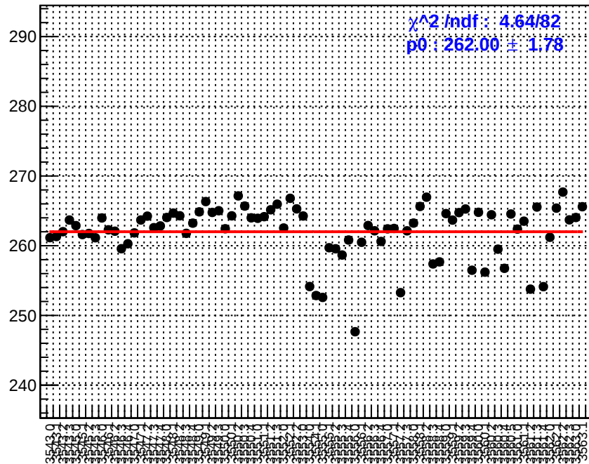
slug10: ds_avg_bpm4aY
