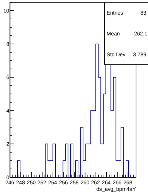
ds_avg_bpm4aY
