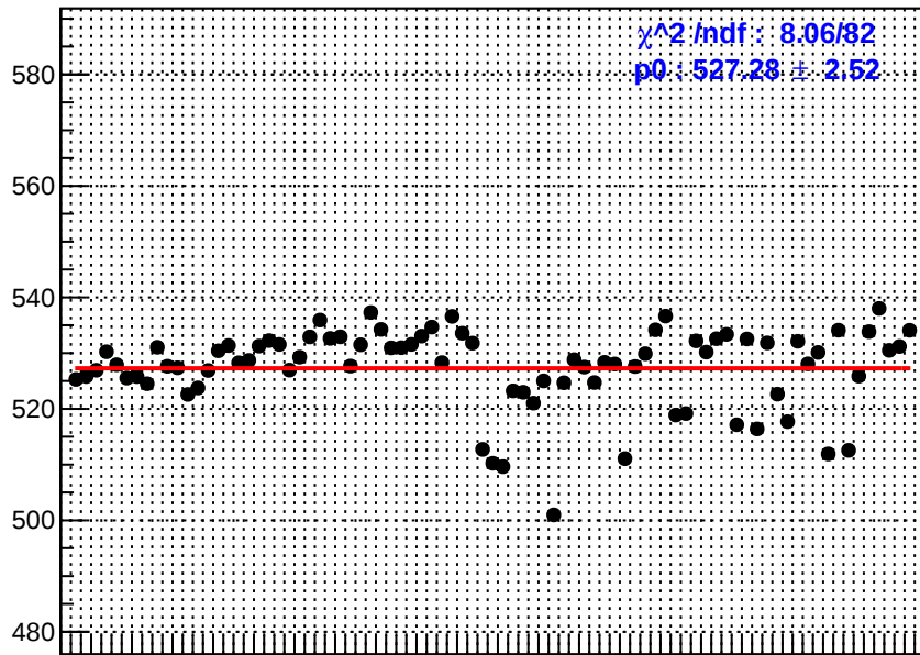
slug10: dsr_bpm4aY
