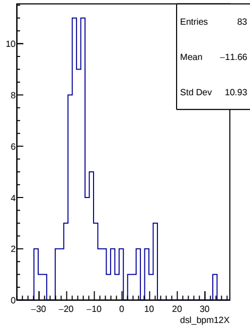
dsl_bpm12X
