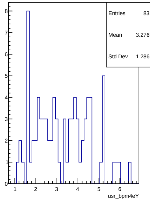
usr_bpm4eY
