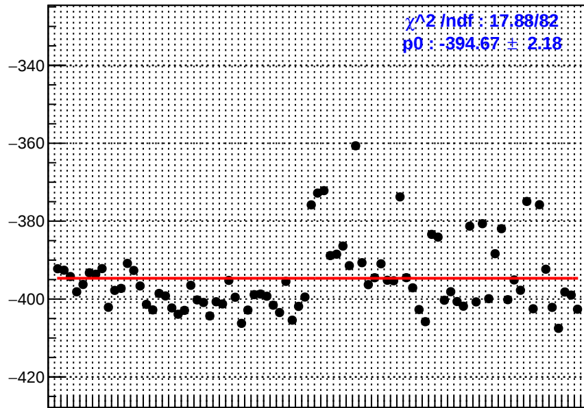
slug10: ds_avg_bpm4eY
