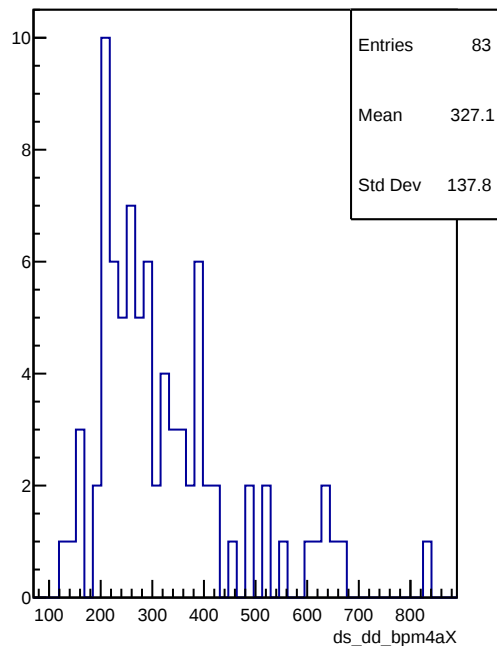
ds_dd_bpm4aX
