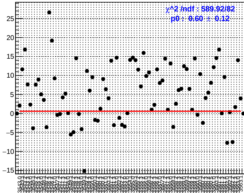
slug10: usr_bpm11X
