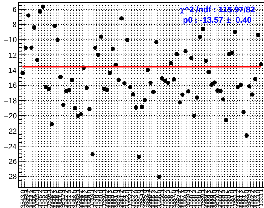
slug10: us_avg_bpm11X
