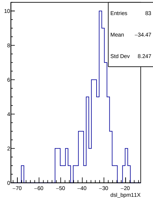
dsl_bpm11X
