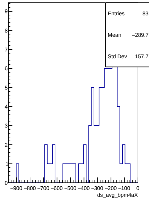
ds_avg_bpm4aX
