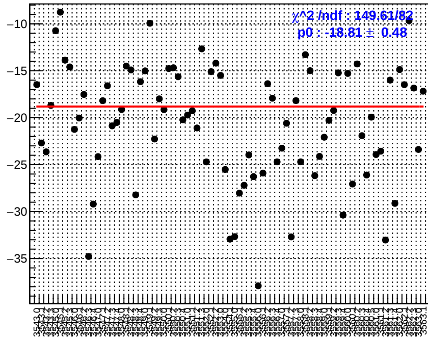
slug10: us_dd_bpm11X
