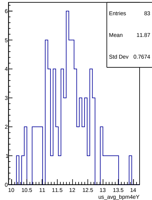
us_avg_bpm4eY
