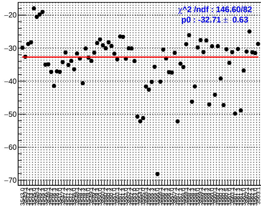
slug10: dsl_bpm11X
