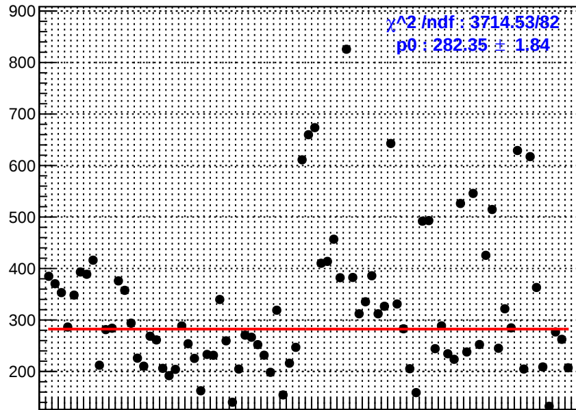
slug10: ds_dd_bpm4aX
