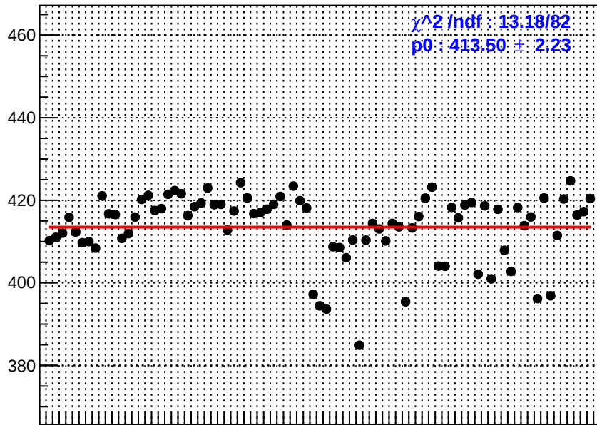
slug10: ds_dd_bpm4eY
