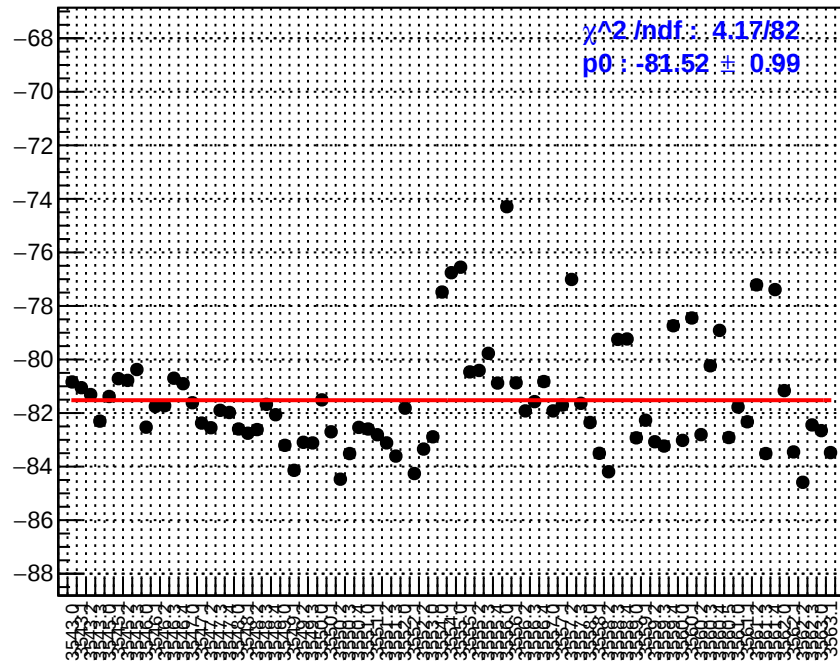
slug10: ds_dd_bpm4eX
