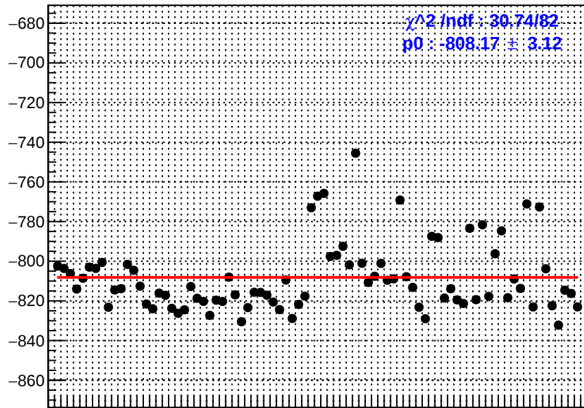
slug10: dsr_bpm4eY
