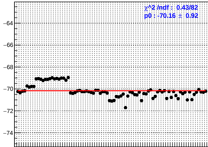
slug10: usl_bpm4eX
