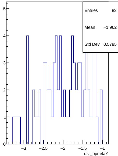
usr_bpm4aY
