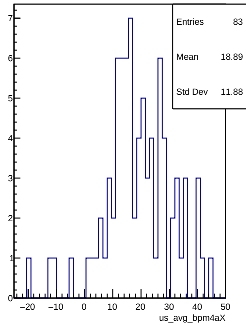
us_avg_bpm4aX
