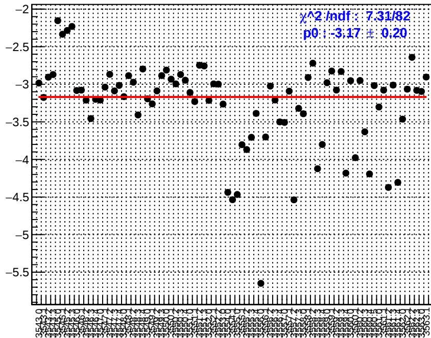
slug10: dsl_bpm4aY
