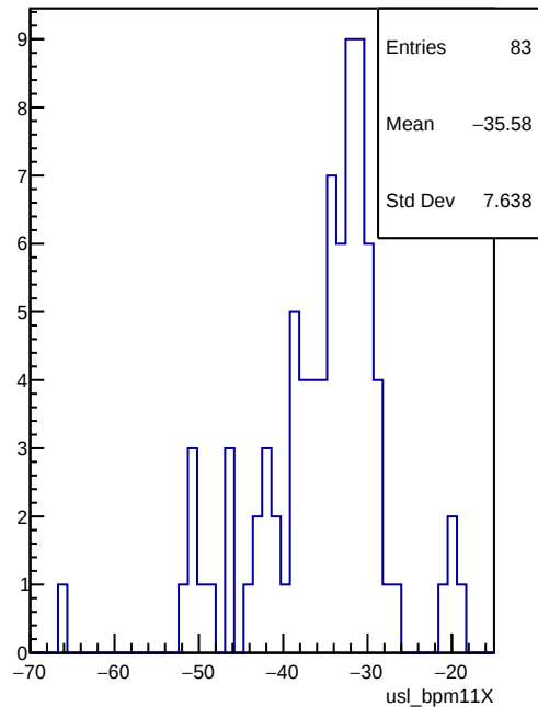
usl_bpm11X
