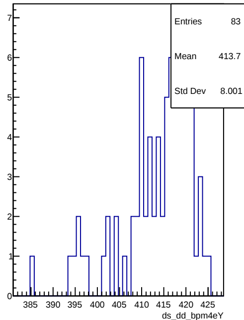
ds_dd_bpm4eY
