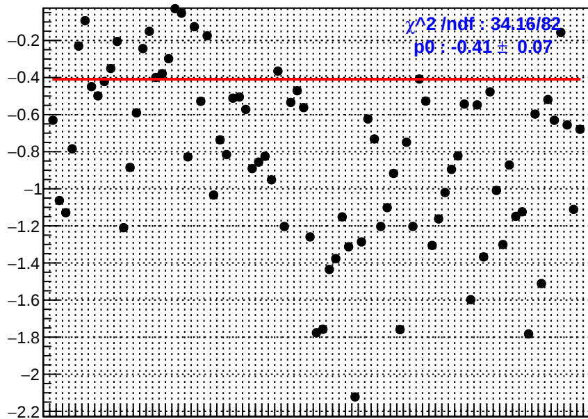
slug10: us_dd_bpm4aY
