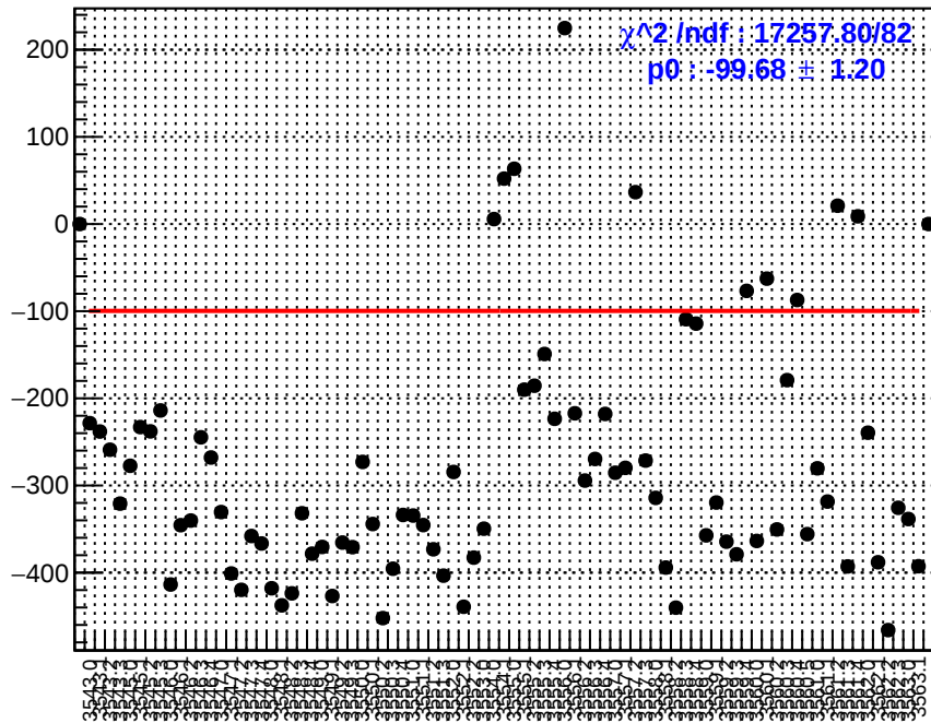
slug10: dsr_bpm12X
