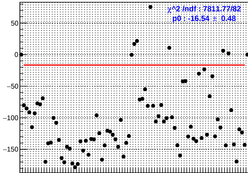
slug10: ds_dd_bpm11X
