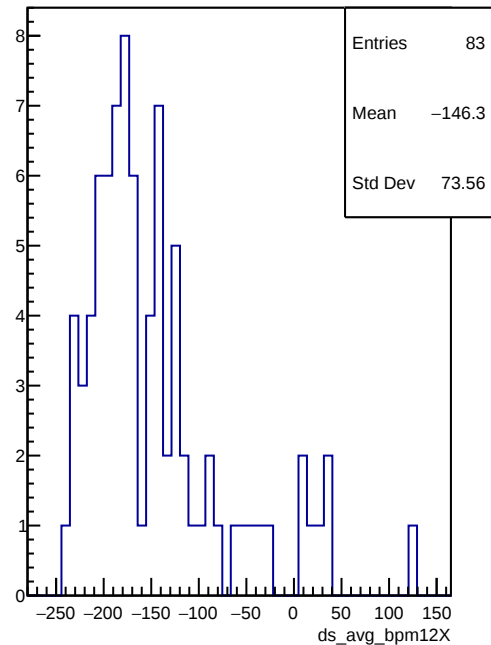
ds_avg_bpm12X
