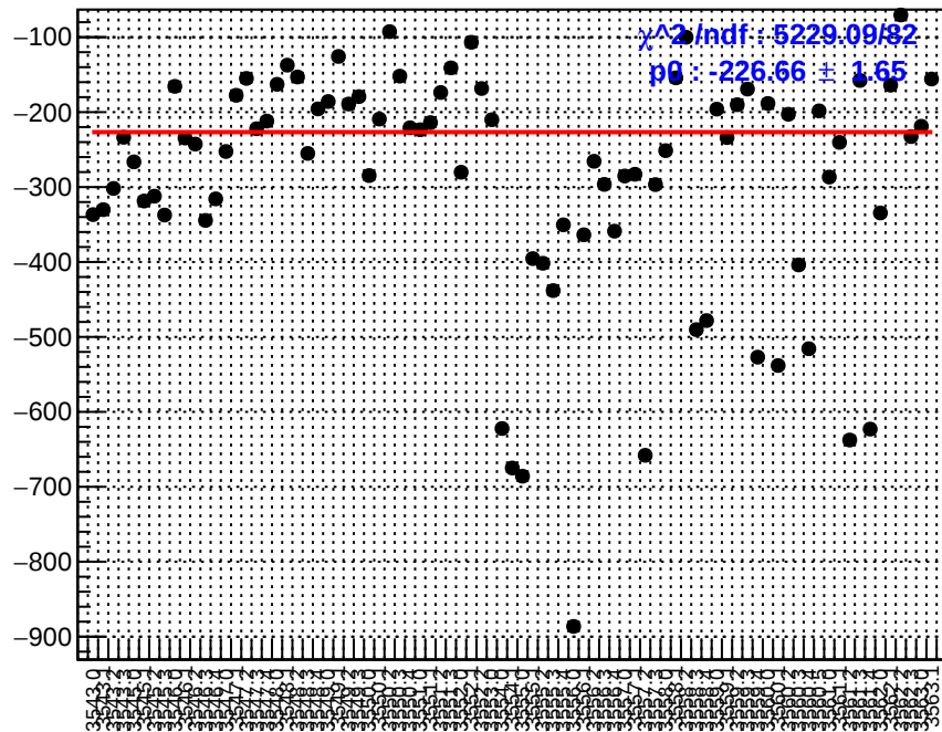
slug10: ds_avg_bpm4aX
