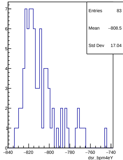
dsr_bpm4eY
