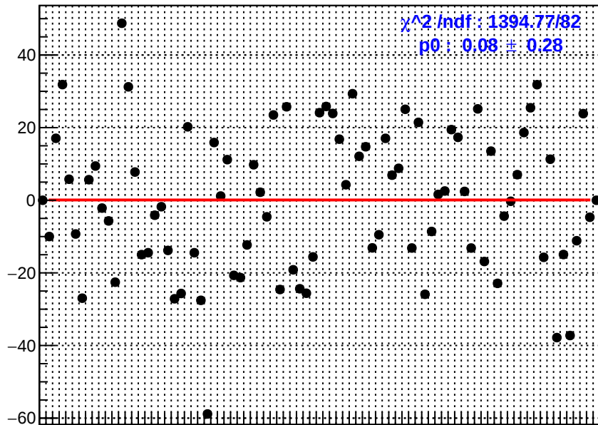
slug10: usr_bpm4aX
