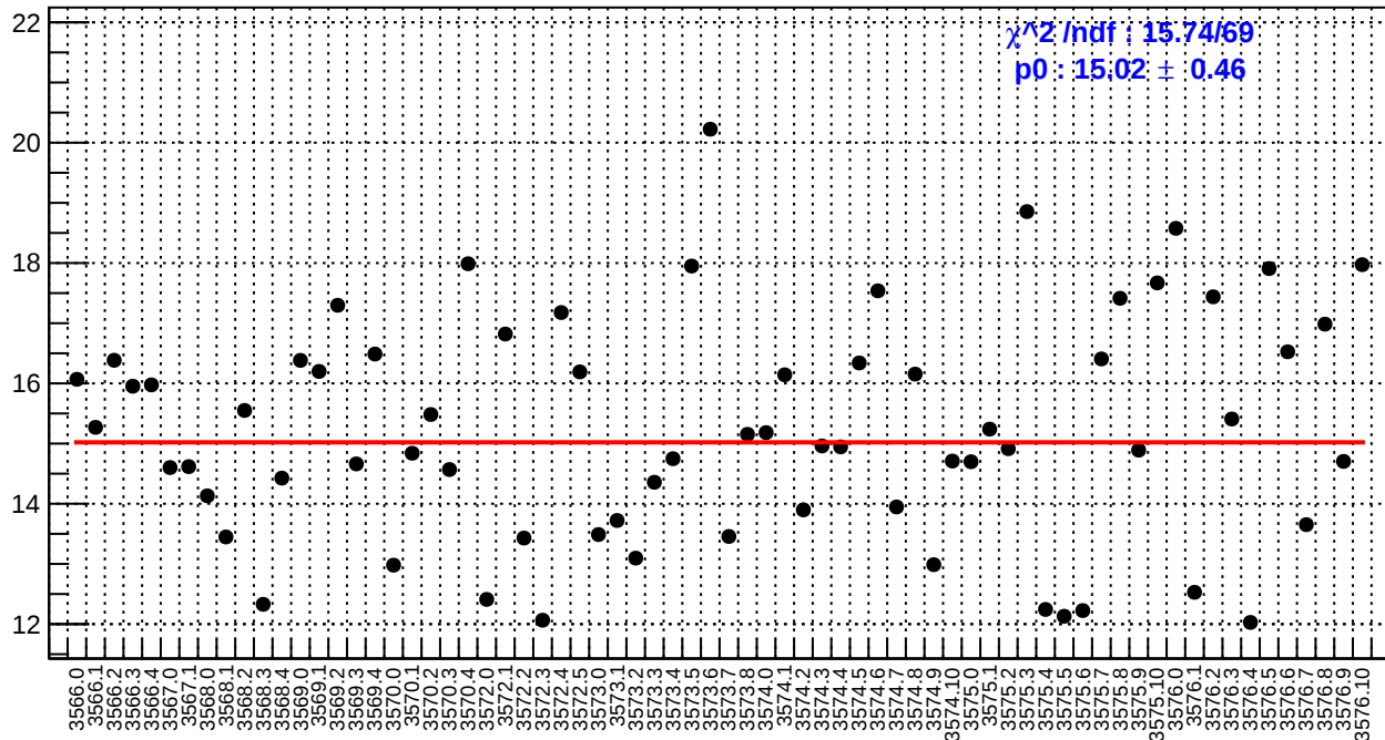
slug11-Left: usr_bpm4eX/(ppb/nm)
