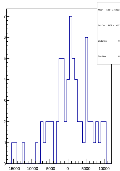
slug11-Left: 1D Corr asym_dsl.mean/ppb-reg_asym_dsl.mean/ppb
