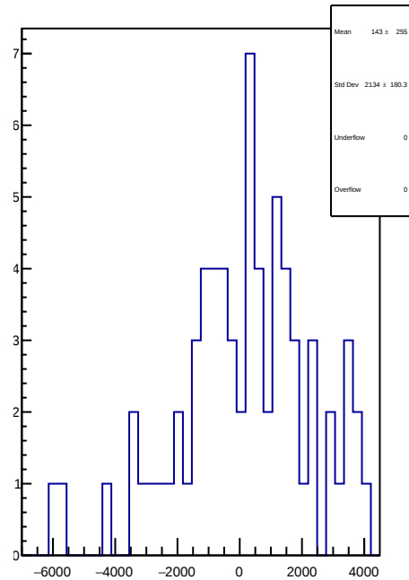
slug11-Left: 1D Corr asym_us_avg.mean/ppb-reg_asym_us_avg.mean/ppb
