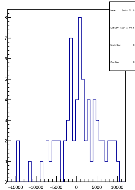
slug11-Left: 1D Corr asym_left_avg.mean/ppb-reg_asym_left_avg.mean/ppb
