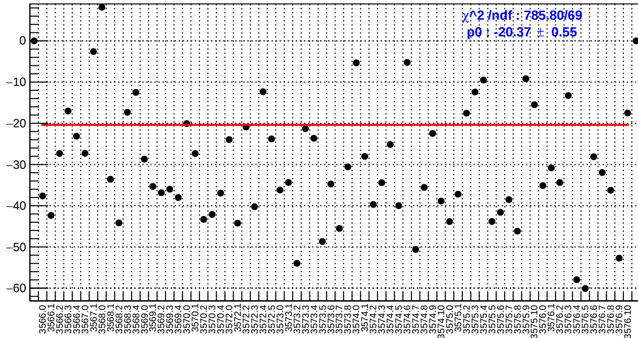
slug11-Left: dsr_bpm4aY/(ppb/nm)
