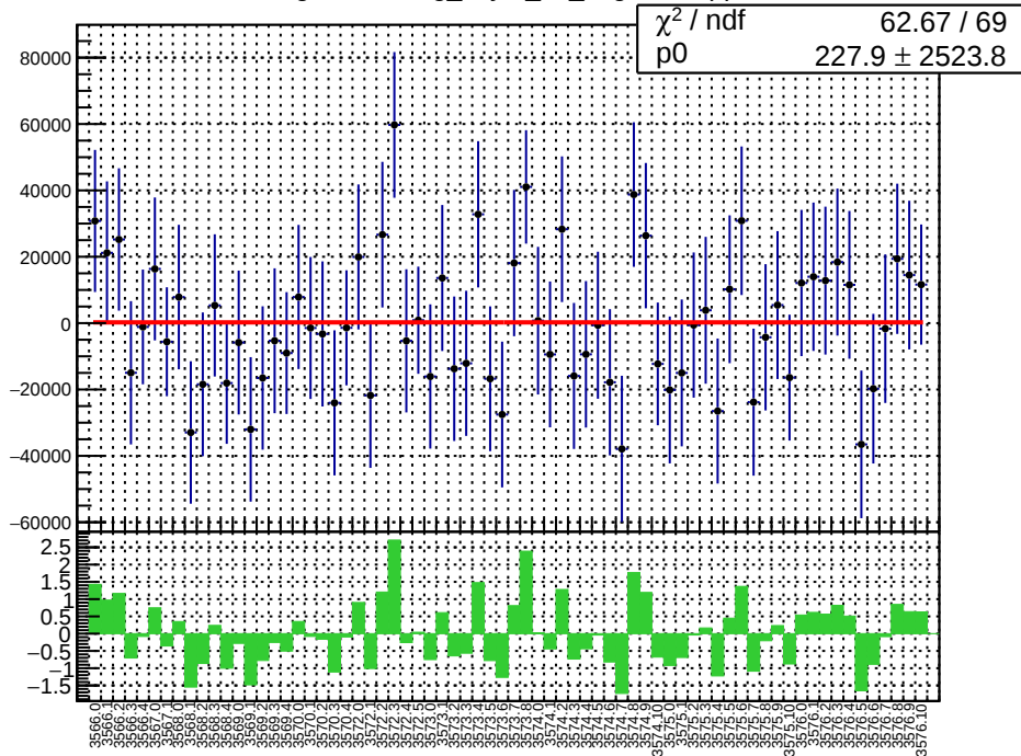
slug11-Left: reg_asym_ds_avg.mean/ppb
