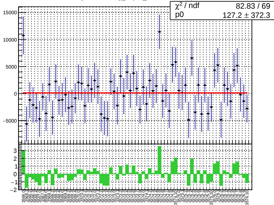
slug11-Left: reg_asym_sam7.mean/ppb
