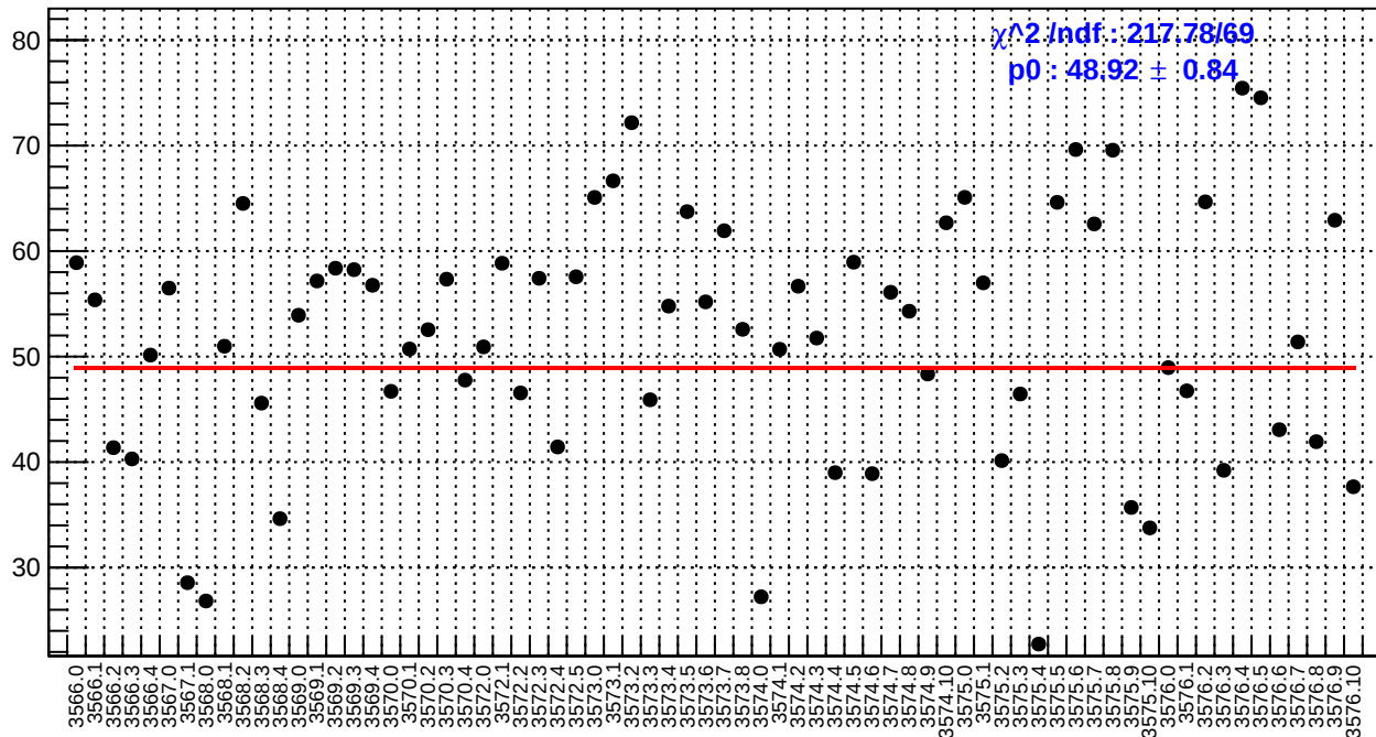
slug11-Left: ds_avg_bpm4eY/(ppb/nm)
