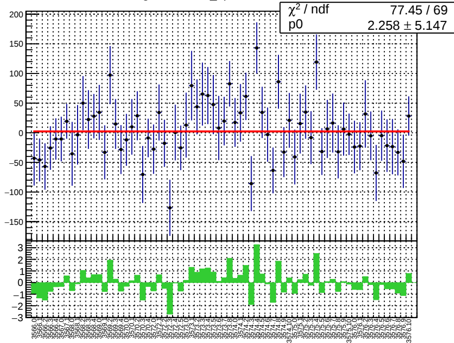
slug11-Left: diff_bpm4eY.mean/nm
