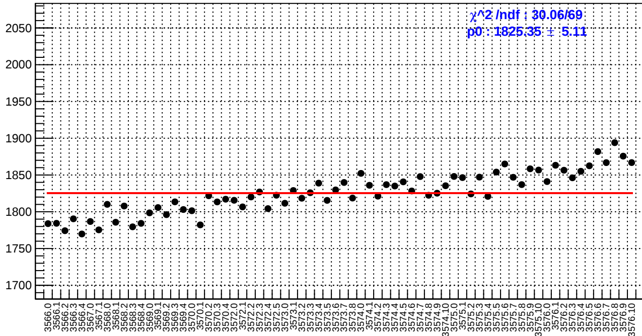
slug11-Left: reg_asym_right_avg.rms/ppm
