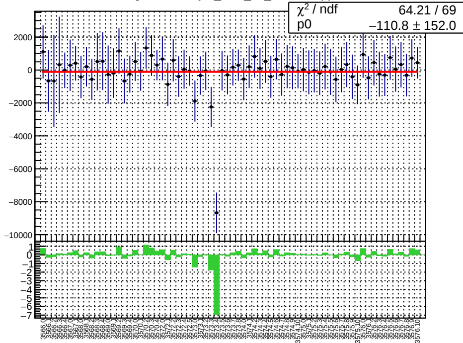
slug11-Left: asym_bcm_an_us.mean/ppb
