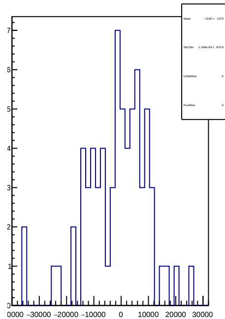
slug11-Left: 1D Corr asym_sam1.mean/ppb-reg_asym_sam1.mean/ppb
