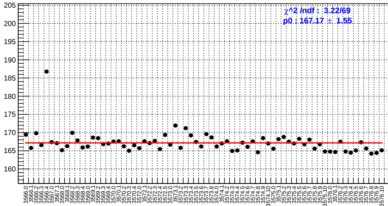
slug11-Left: reg_asym_dsl.rms/ppm
