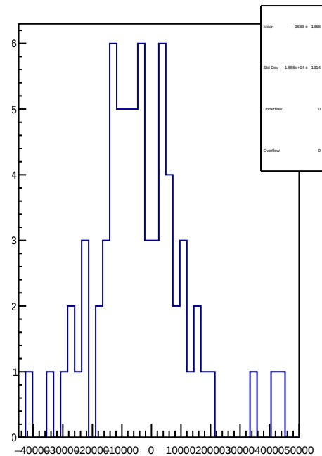
slug11-Right: 1D Corr asym_sam8.mean/ppb-reg_asym_sam8.mean/ppb
