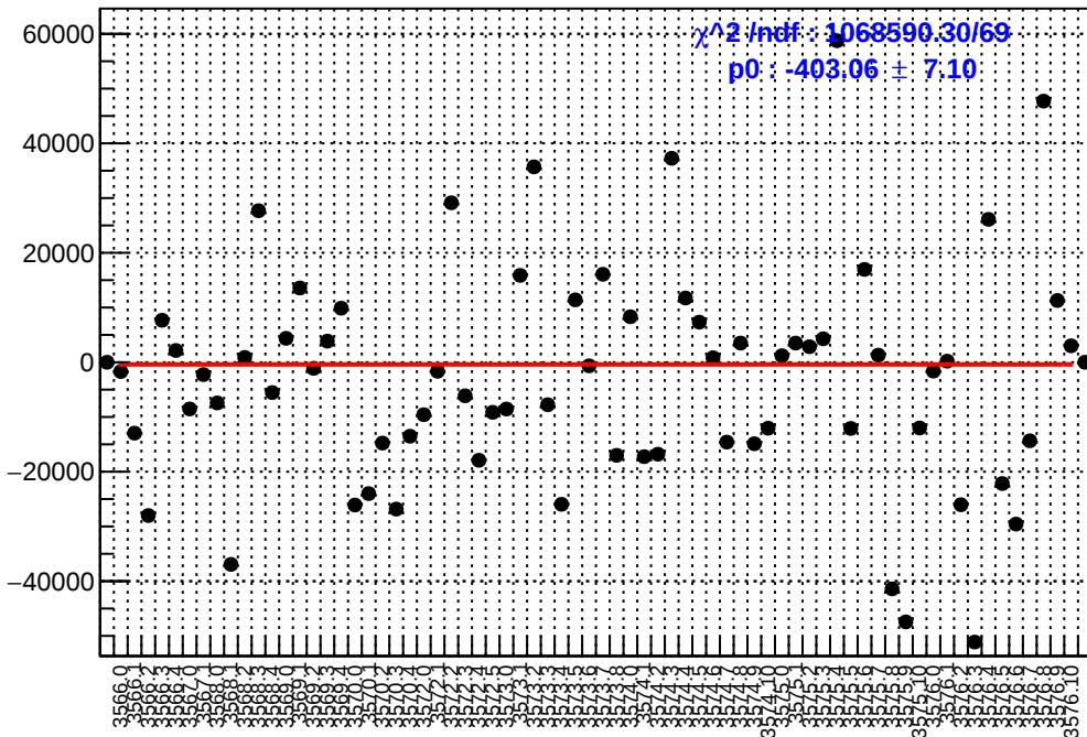
slug11-Left: asym_sam7.mean/ppb-reg_asym_sam7.mean/ppb
