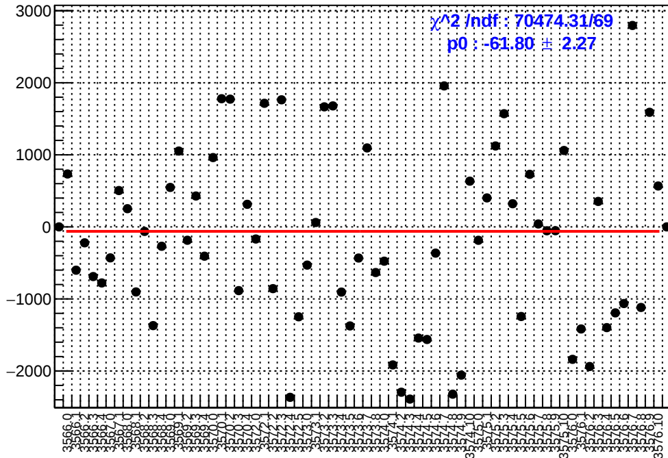
slug11-Left: asym_ds_dd.mean/ppb-reg_asym_ds_dd.mean/ppb
