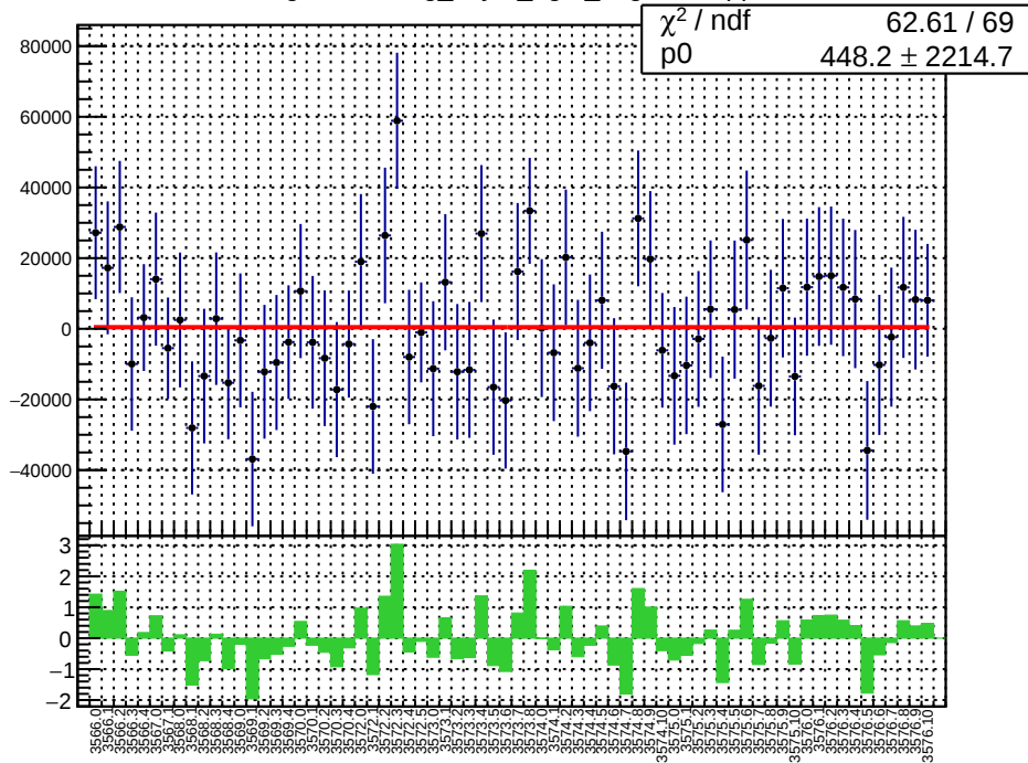
slug11-Left: reg_asym_right_avg.mean/ppb
