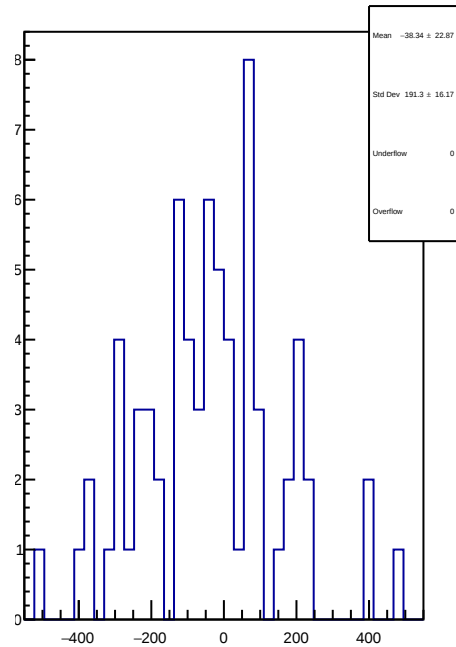
slug11-Left: 1D Corr asym_left_dd.mean/ppb-reg_asym_left_dd.mean/ppb
