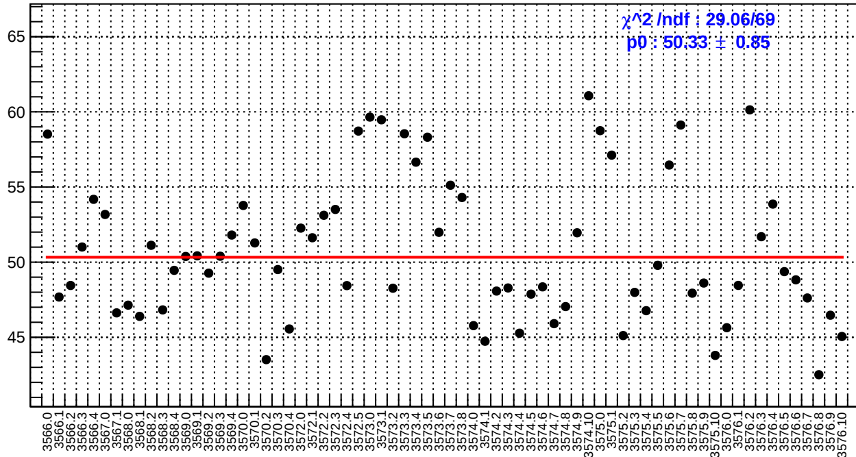
slug11-Left: usl_bpm4eY/(ppb/nm)
