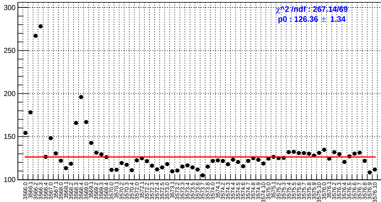
slug11-Left: asym_bcm_an_ds3.rms/ppm
