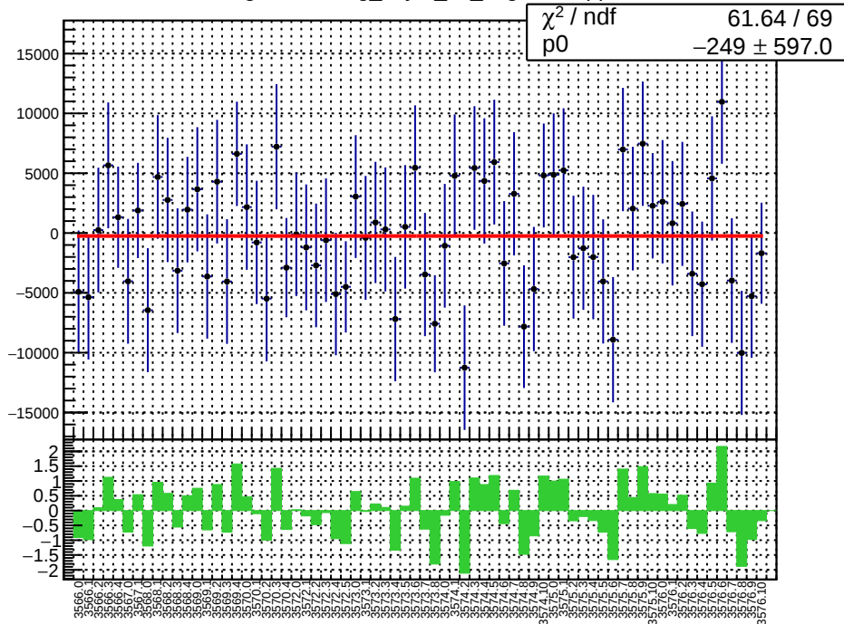
slug11-Left: reg_asym_us_avg.mean/ppb
