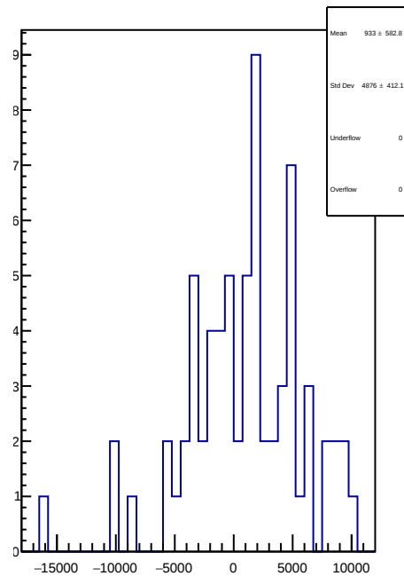
slug11-Left: 1D Corr asym_dsr.mean/ppb-reg_asym_dsr.mean/ppb
