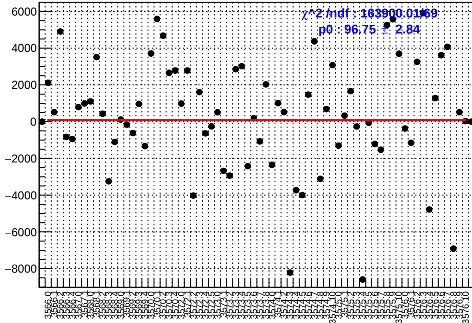
slug11-Left: asym_us_dd.mean/ppb-reg_asym_us_dd.mean/ppb
