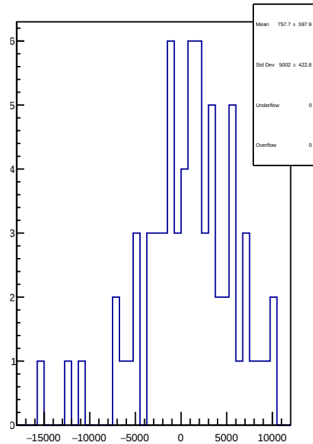
slug11-Left: 1D Corr asym_ds_avg.mean/ppb-reg_asym_ds_avg.mean/ppb
