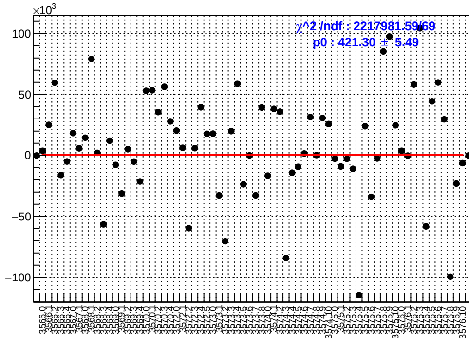
slug11-Left: asym_sam3.mean/ppb-reg_asym_sam3.mean/ppb
