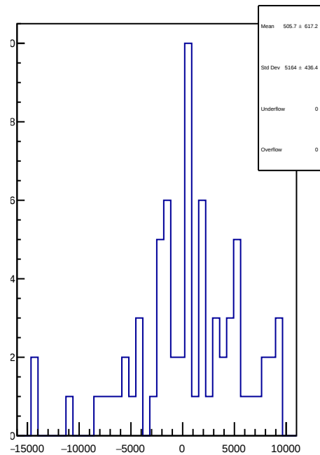
slug11-Left: 1D Corr asym_usl.mean/ppb-reg_asym_usl.mean/ppb
