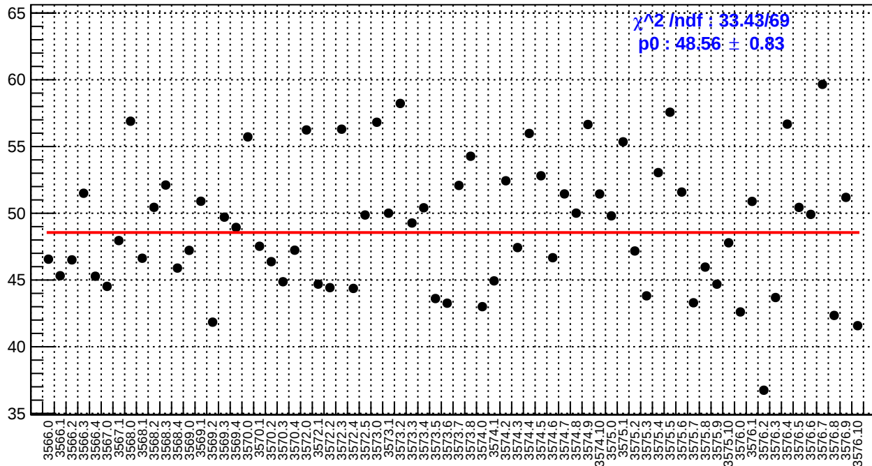
slug11-Left: us_avg_bpm4aX/(ppb/nm)
