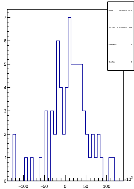
slug11-Left: 1D Corr asym_sam4.mean/ppb-reg_asym_sam4.mean/ppb
