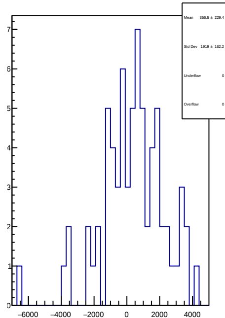
slug11-Left: 1D Corr asym_right_avg.mean/ppb-reg_asym_right_avg.mean/ppb
