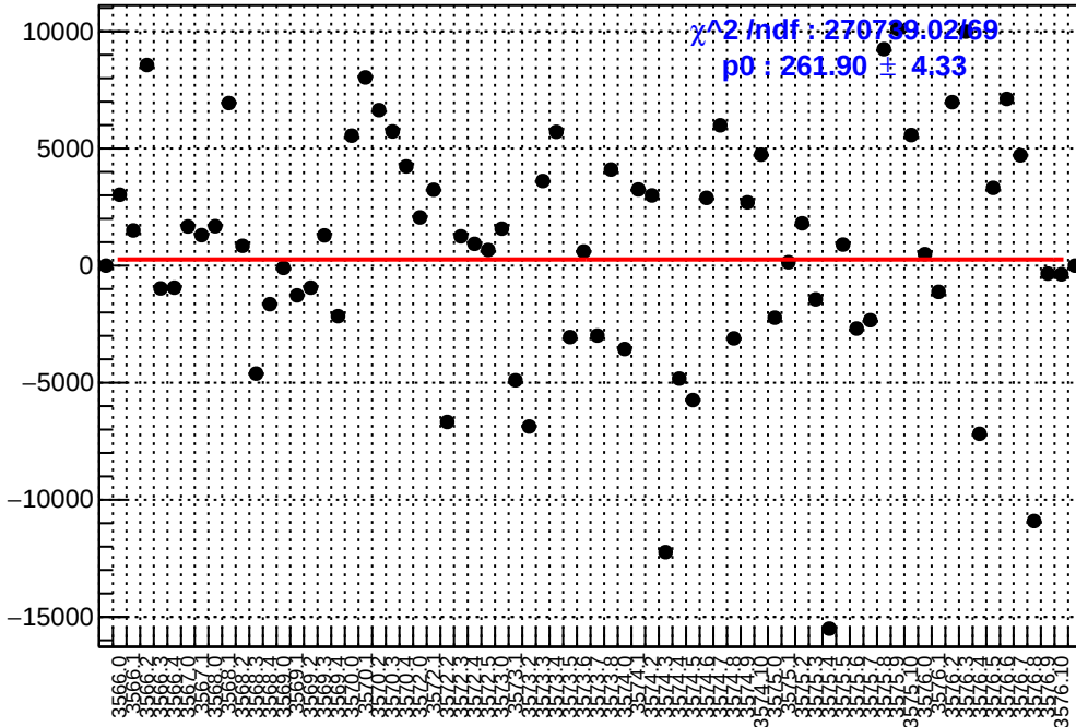
slug11-Left: asym_ds_avg.mean/ppb-reg_asym_ds_avg.mean/ppb
