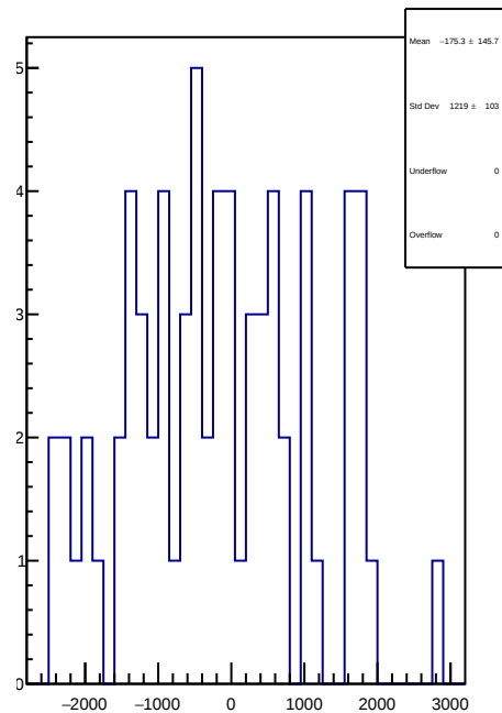
slug11-Left: 1D Corr asym_ds_dd.mean/ppb-reg_asym_ds_dd.mean/ppb
