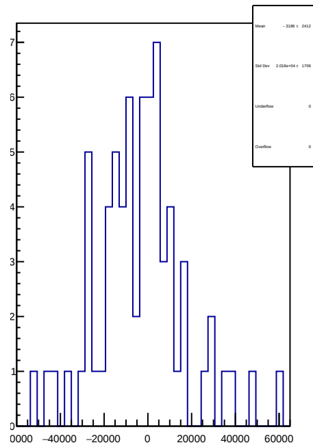
slug11-Left: 1D Corr asym_sam7.mean/ppb-reg_asym_sam7.mean/ppb
