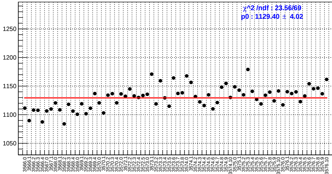
slug11-Left: reg_asym_sam4.rms/ppm
