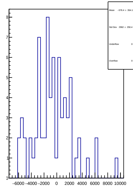
slug11-Left: 1D Corr asym_right_dd.mean/ppb-reg_asym_right_dd.mean/ppb
