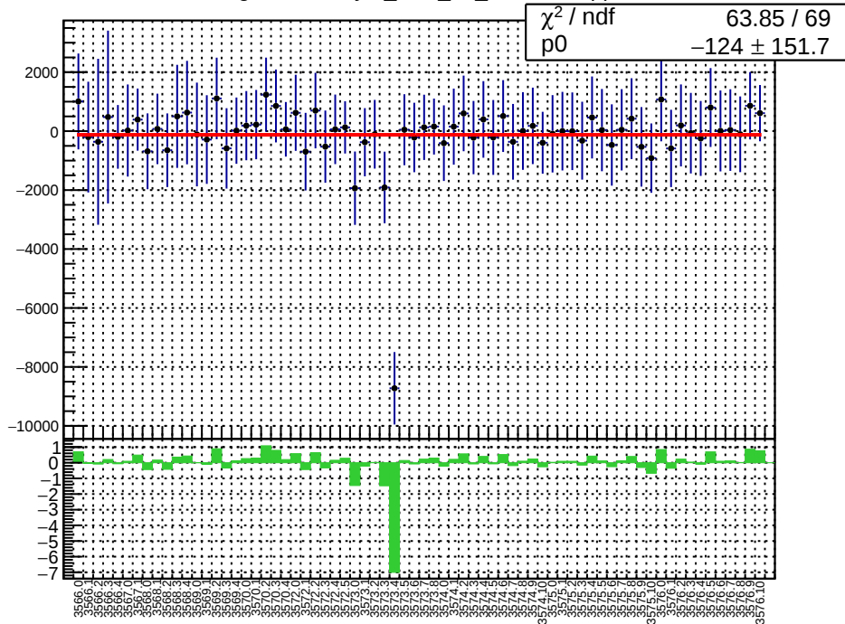
slug11-Left: asym_bcm_an_ds3.mean/ppb
