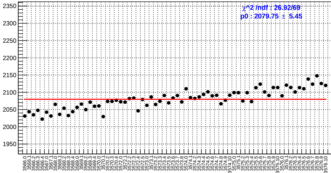
slug11-Left: reg_asym_ds_avg.rms/ppm
