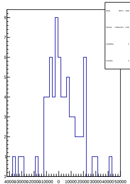
slug11-Left: 1D Corr asym_sam5.mean/ppb-reg_asym_sam5.mean/ppb
