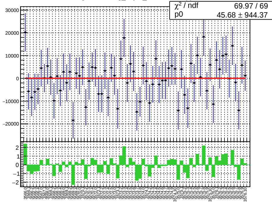
slug11-Left: reg_asym_sam6.mean/ppb
