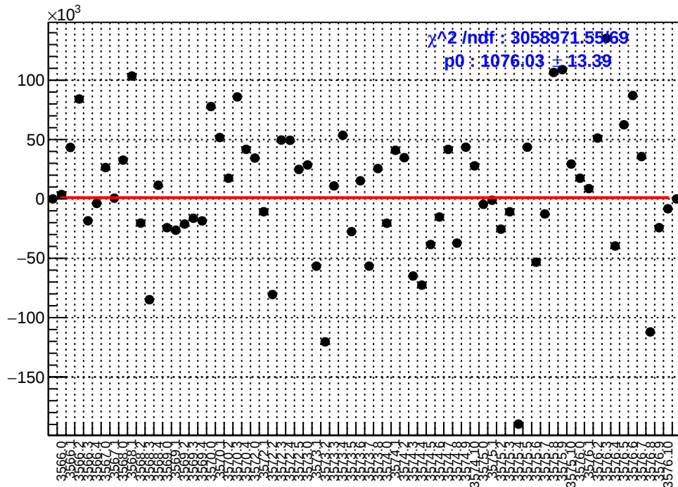
slug11-Left: asym_sam2.mean/ppb-reg_asym_sam2.mean/ppb
