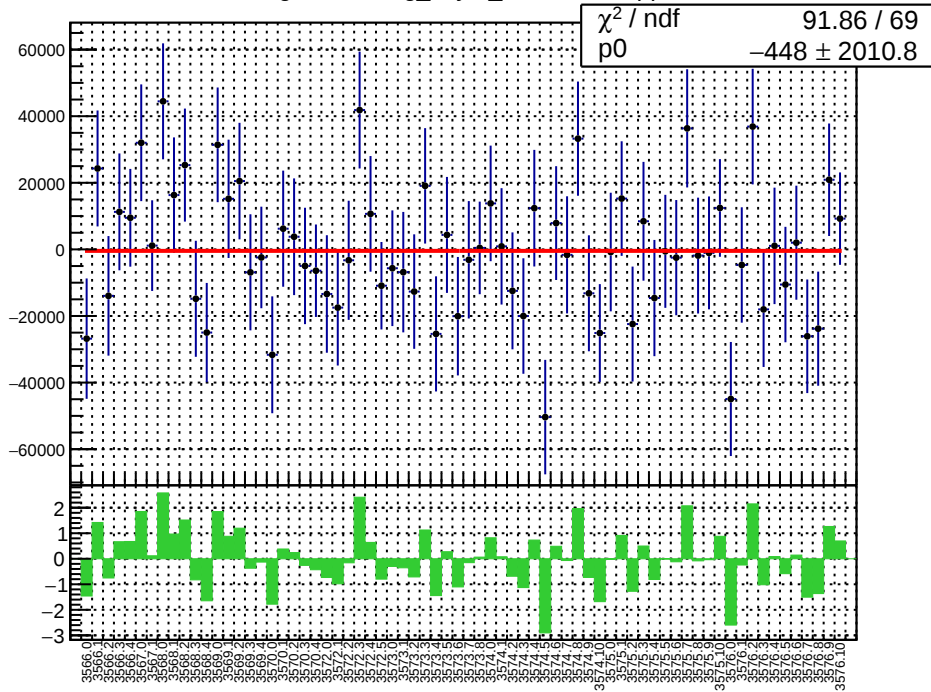
slug11-Left: reg_asym_sam2.mean/ppb
