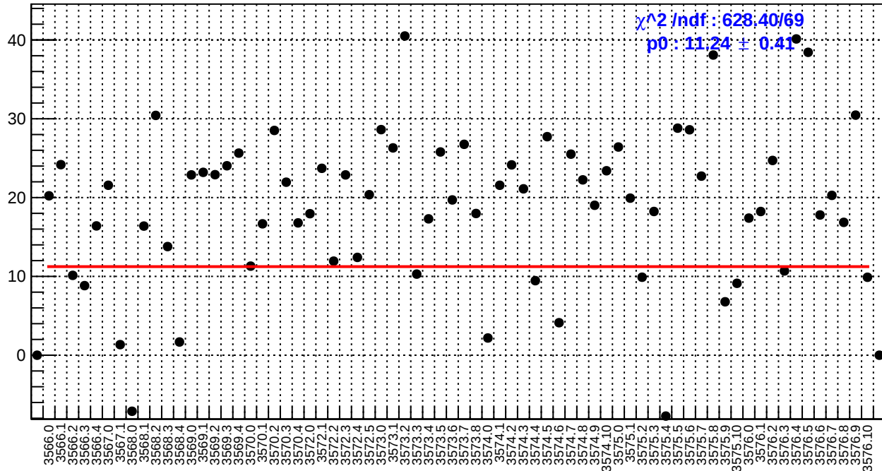
slug11-Left: right_avg_bpm4eY/(ppb/nm)
