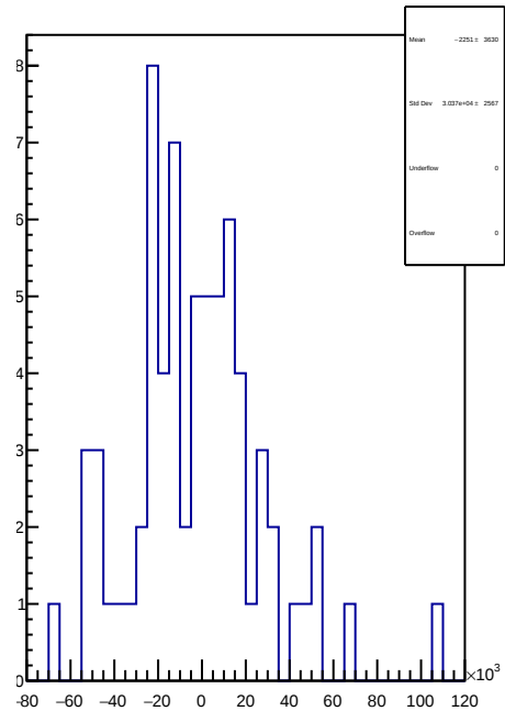
slug11-Left: 1D Corr asym_sam6.mean/ppb-reg_asym_sam6.mean/ppb
