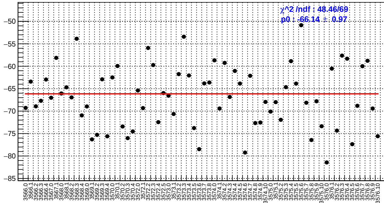
slug11-Left: dsr_bpm4eX/(ppb/nm)
