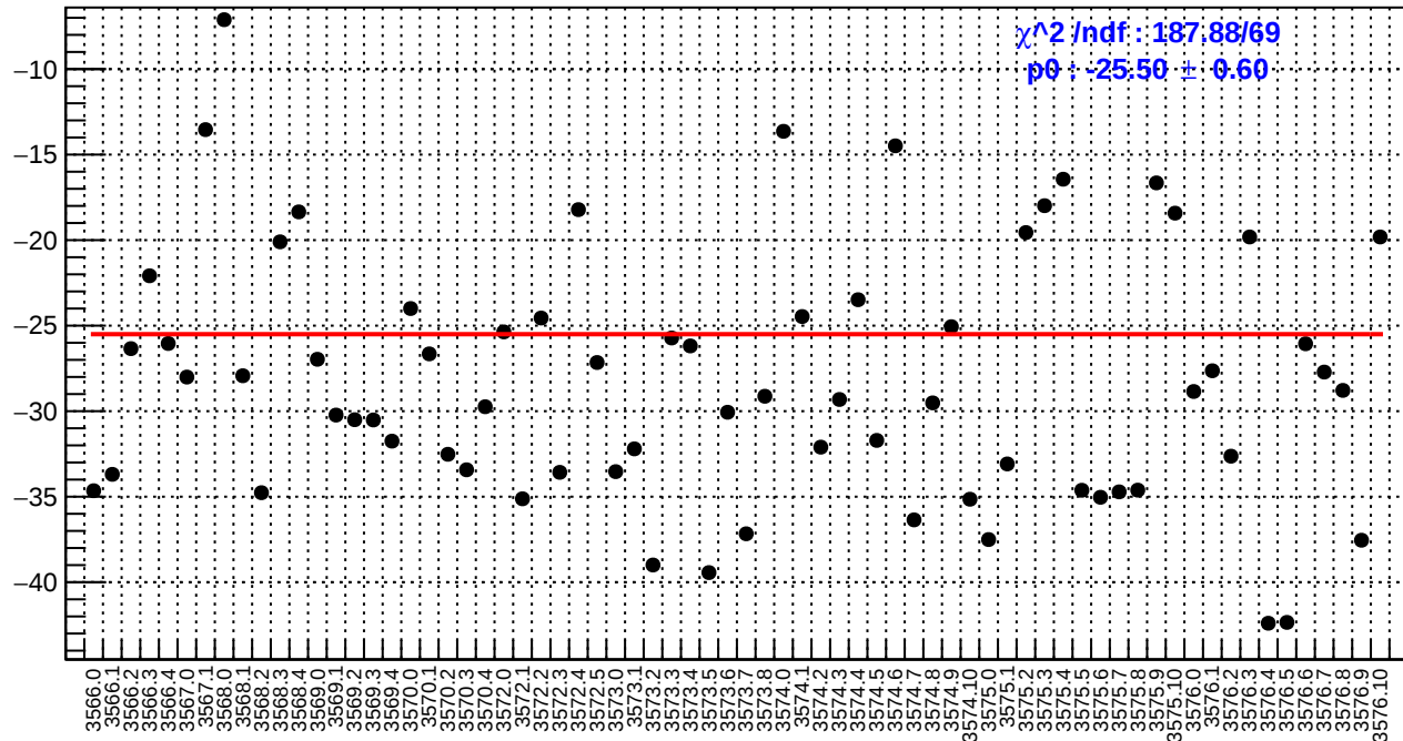
slug11-Left: ds_avg_bpm4aY/(ppb/nm)
