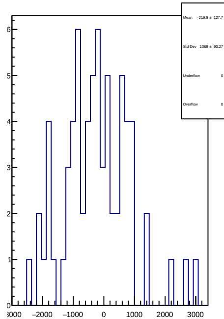
slug11-Left: 1D Corr asym_usr.mean/ppb-reg_asym_usr.mean/ppb
