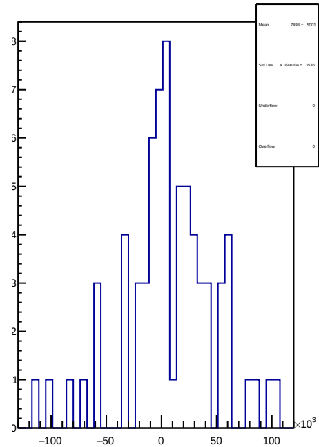
slug11-Left: 1D Corr asym_sam3.mean/ppb-reg_asym_sam3.mean/ppb
