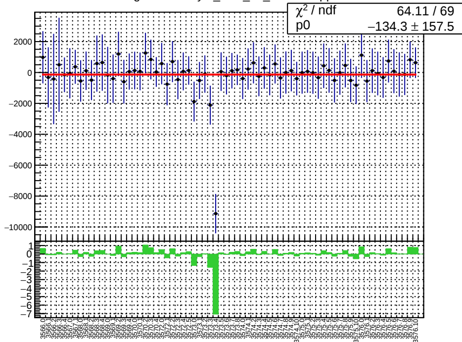
slug11-Left: asym_bcm_an_ds.mean/ppb
