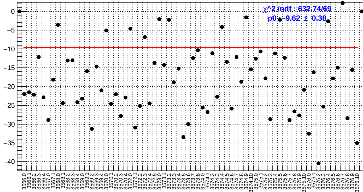
slug11-Left: usr_bpm4aX/(ppb/nm)
