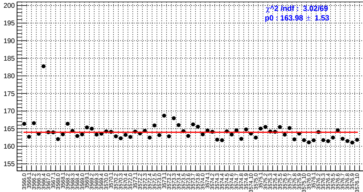
slug11-Left: reg_asym_left_avg.rms/ppm
