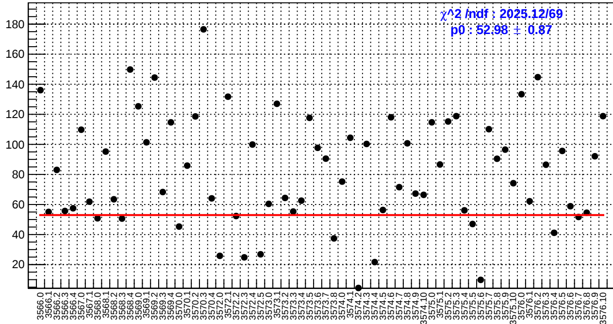
slug11-Left: dsr_bpm4aX/(ppb/nm)
