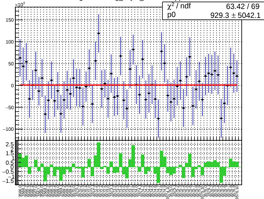
slug11-Left: reg_asym_dsr.mean/ppb
