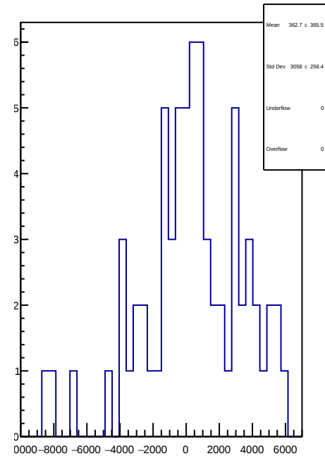
slug11-Left: 1D Cor asym_us_dd.mean/ppb-reg_asym_us_dd.mean/ppb
