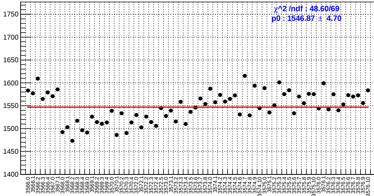
slug11-Left: diff_bpm4aX.rms/nm
