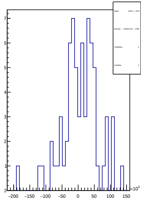
slug11-Left: 1D Corr asym_sam2.mean/ppb-reg_asym_sam2.mean/ppb
