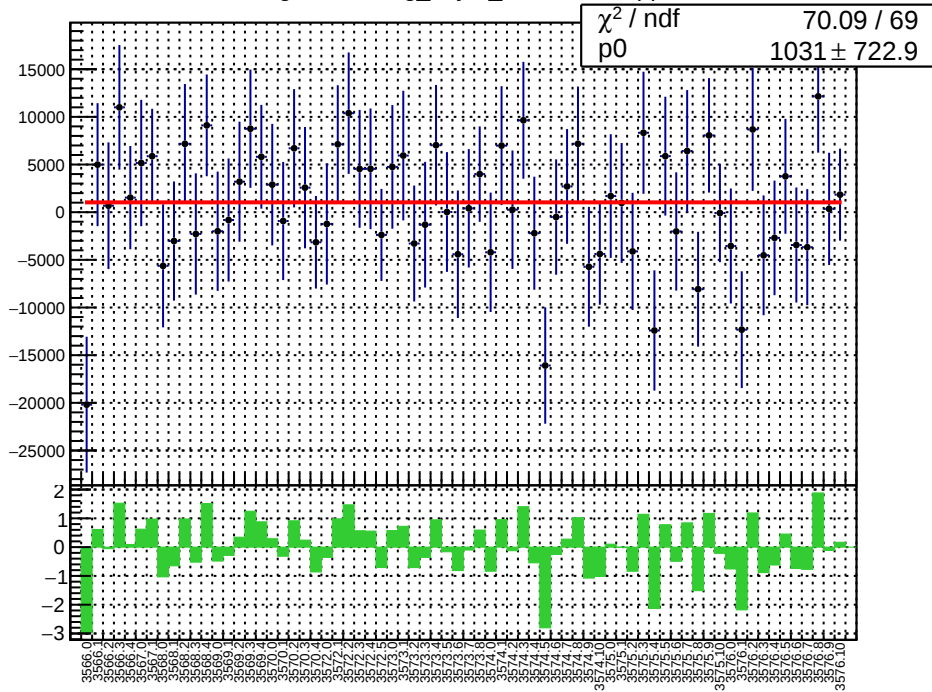
slug11-Left: reg_asym_sam3.mean/ppb
