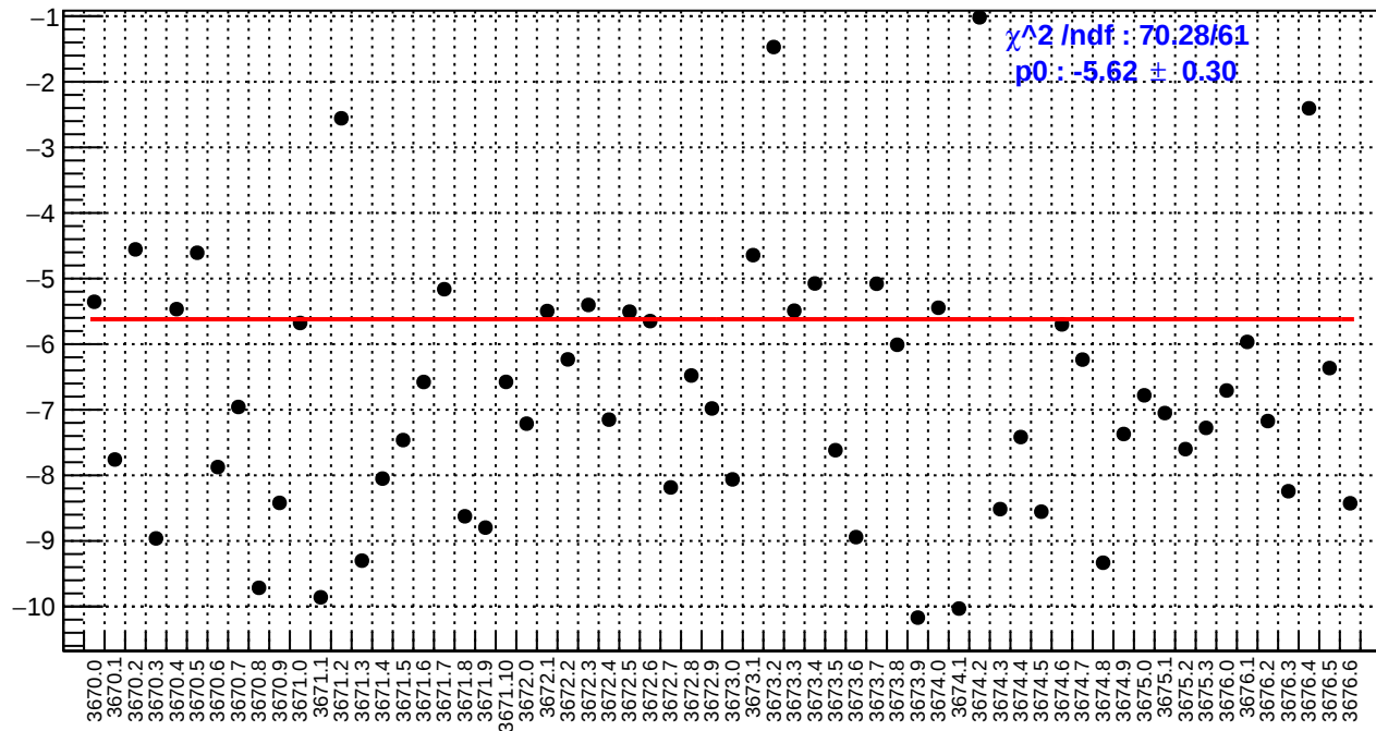
slug15: right_avg_bpm4eY/(ppb/nm)
