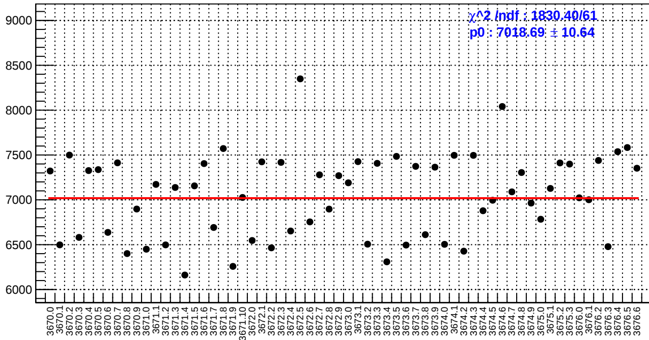
slug15: diff_bpm4aY.rms/nm
