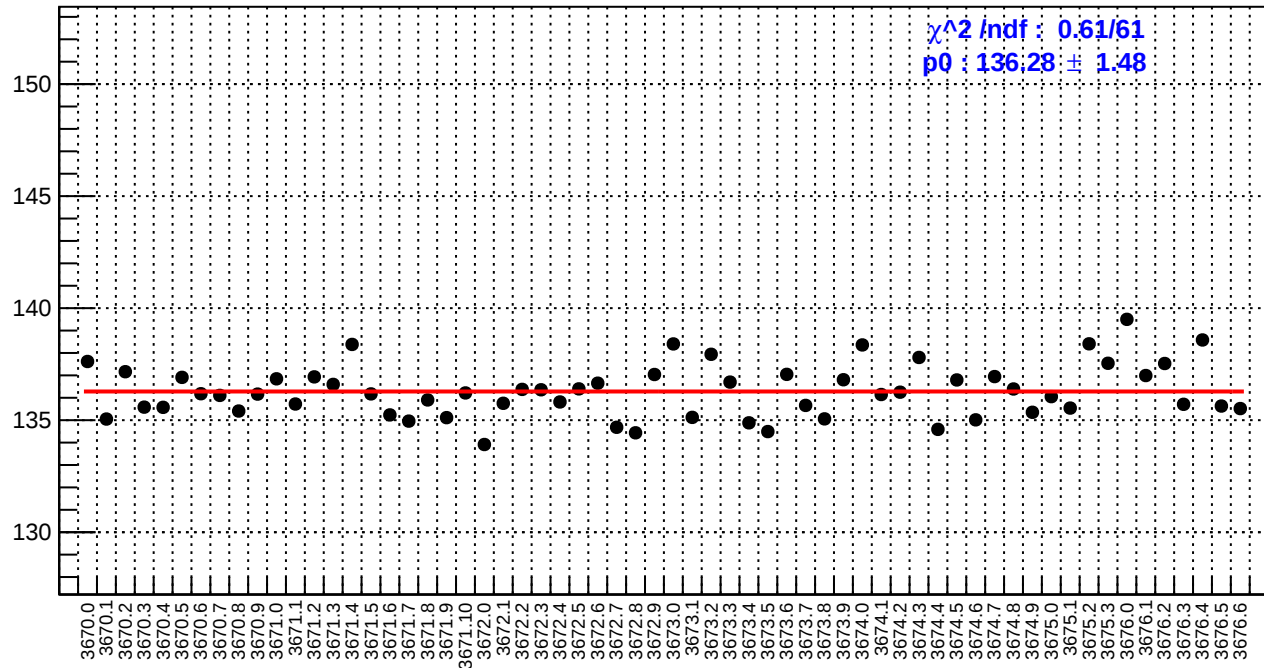
slug15: reg_asym_usr.rms/ppm
