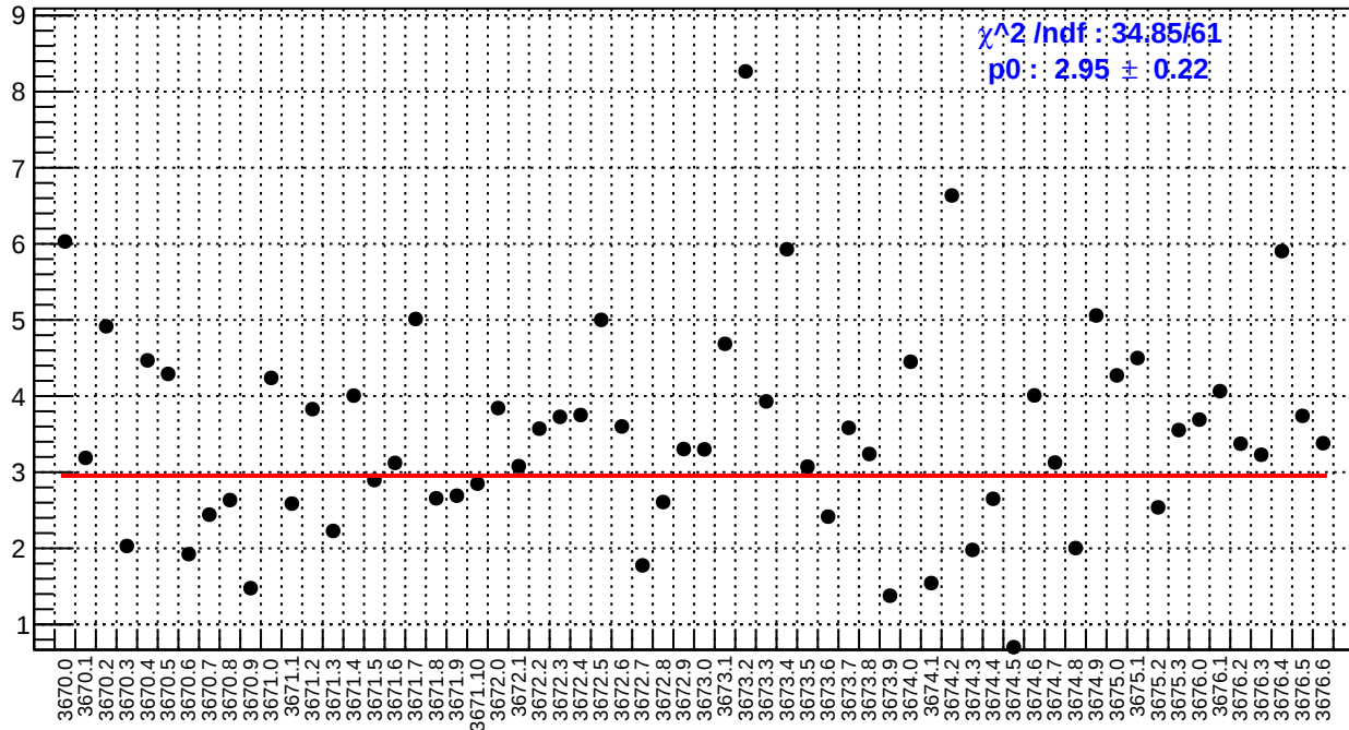
slug15: ds_avg_bpm4eY/(ppb/nm)
