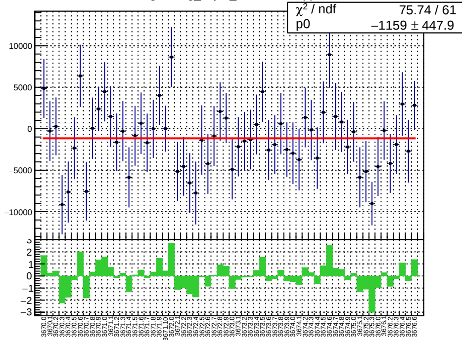
slug15: reg_asym_sam7.mean/ppb
