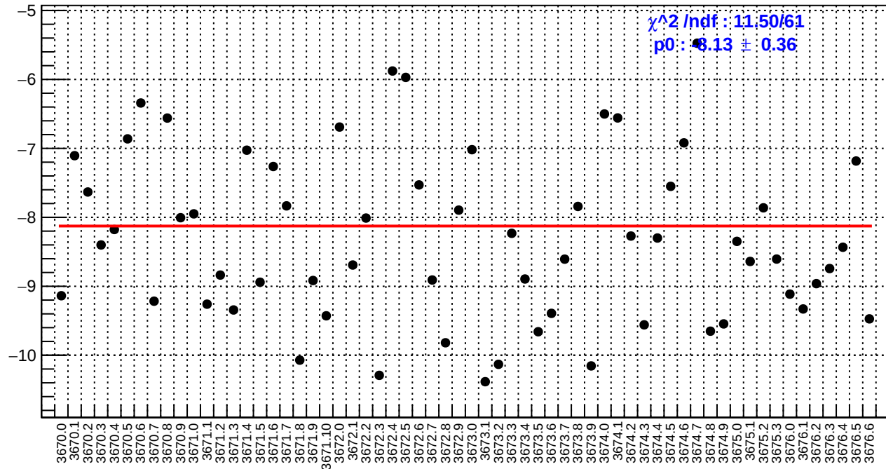
slug15: ds_avg_bpm4aX/(ppb/nm)
