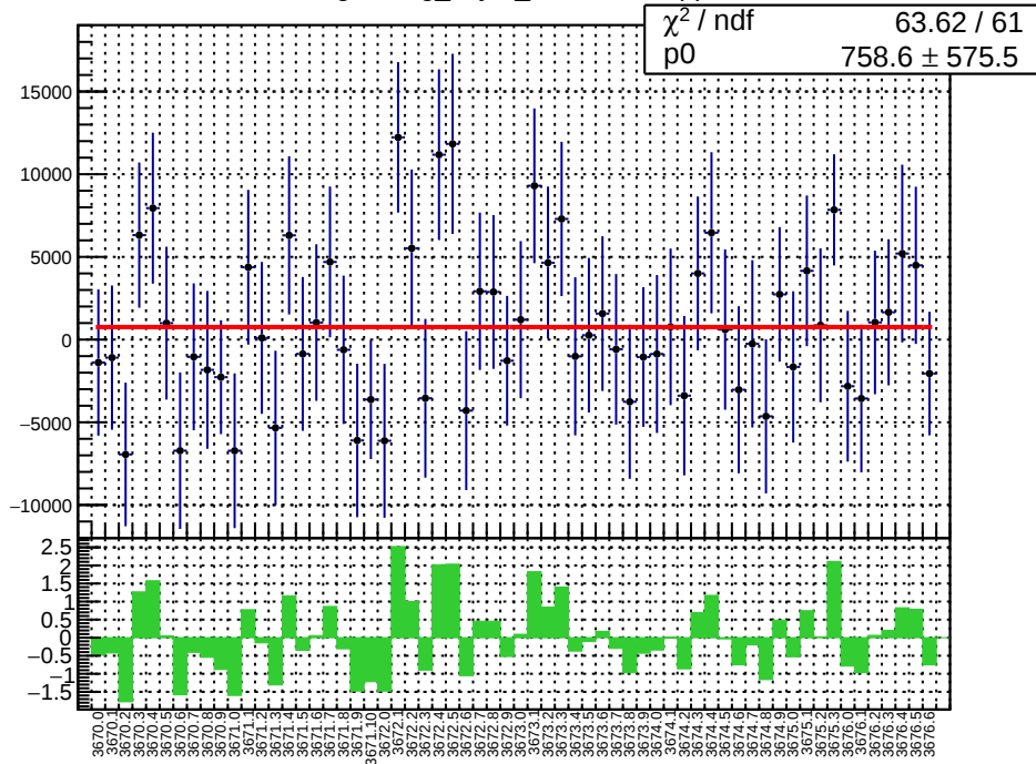
slug15: reg_asym_sam3.mean/ppb
