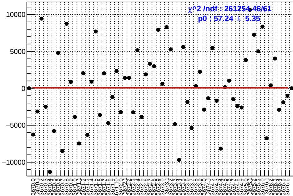
slug15: asym_us_dd.mean/ppb-reg_asym_us_dd.mean/ppb
