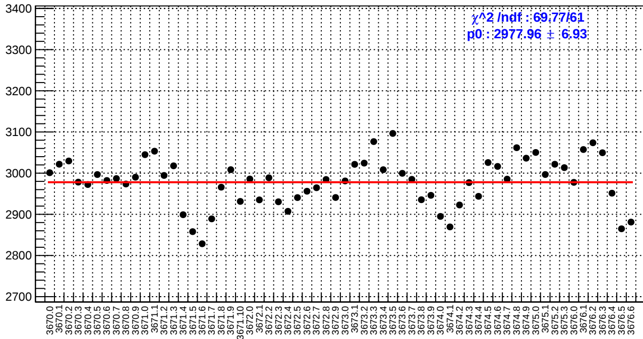
slug15: asym_bcm_an_us.rms/ppm
