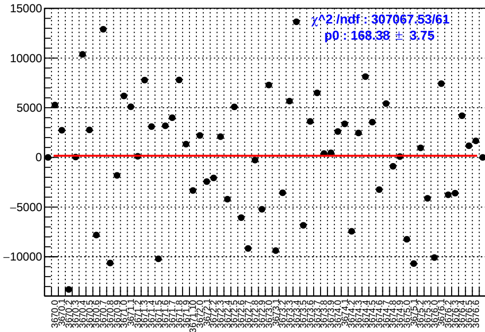
slug15: asym_usr.mean/ppb-reg_asym_usr.mean/ppb
