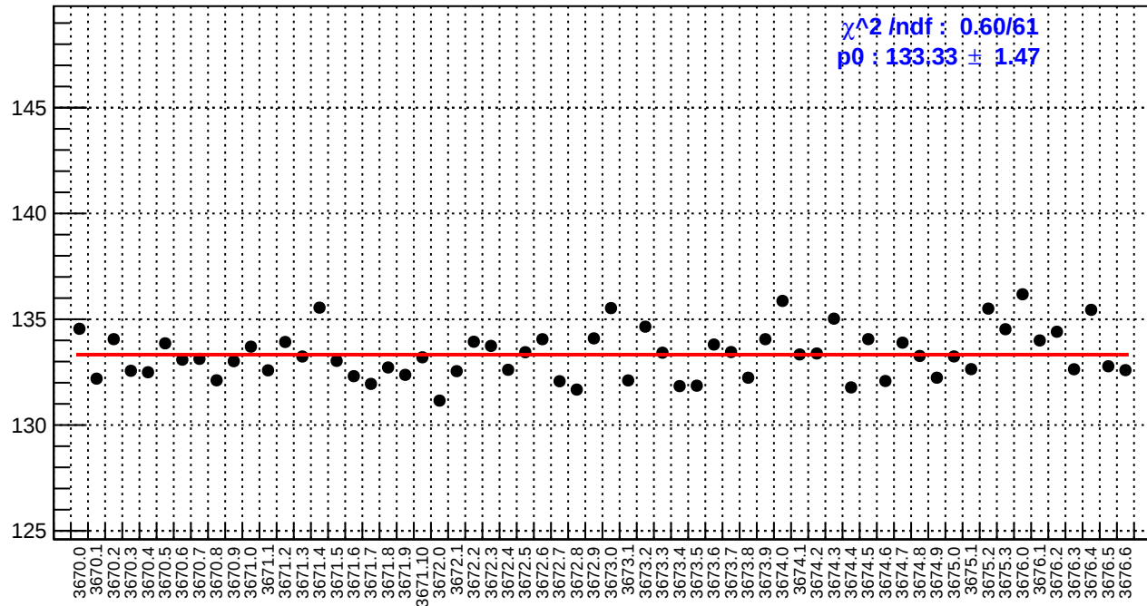
slug15: reg_asym_right_avg.rms/ppm
