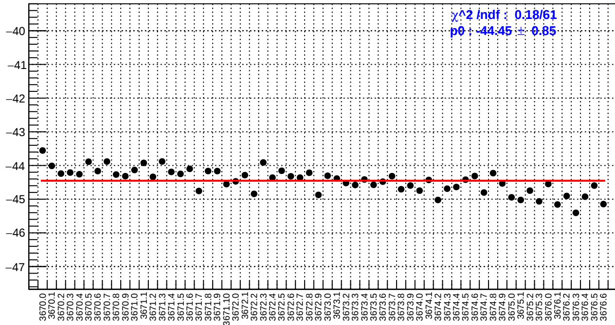
slug15: dsl_bpm12X/(ppb/nm)
