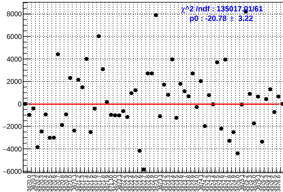
slug15: asym_us_avg.mean/ppb-reg_asym_us_avg.mean/ppb
