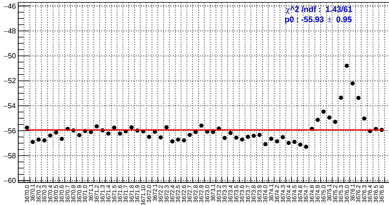
slug15: usl_bpm4eX/(ppb/nm)
