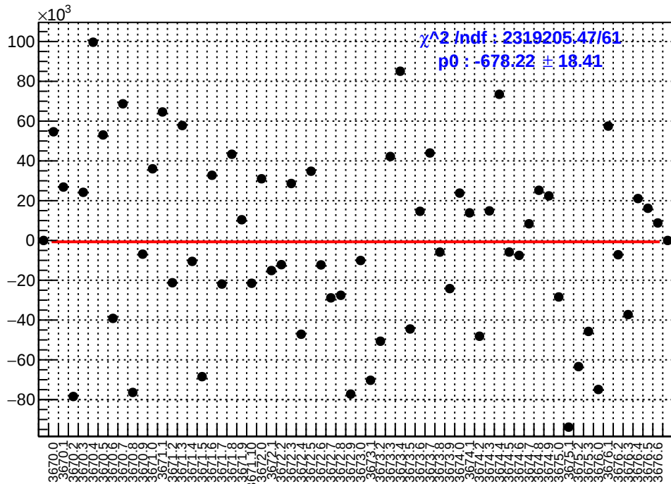
slug15: asym_sam7.mean/ppb-reg_asym_sam7.mean/ppb
