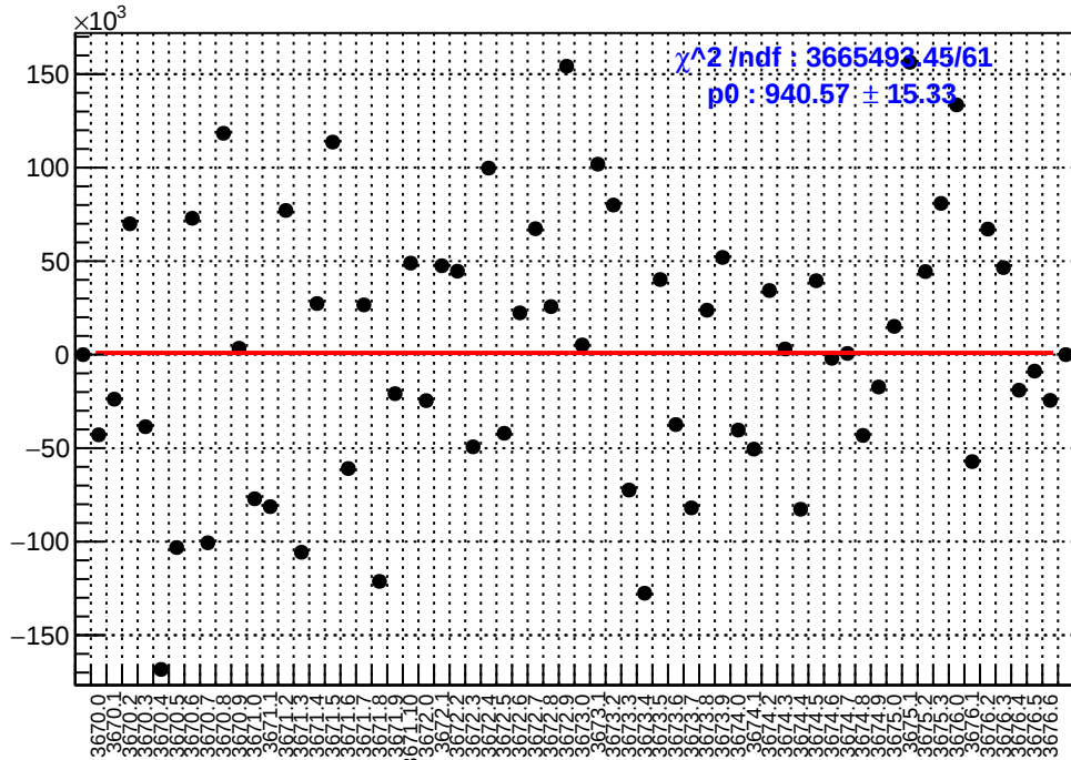
slug15: asym_sam2.mean/ppb-reg_asym_sam2.mean/ppb
