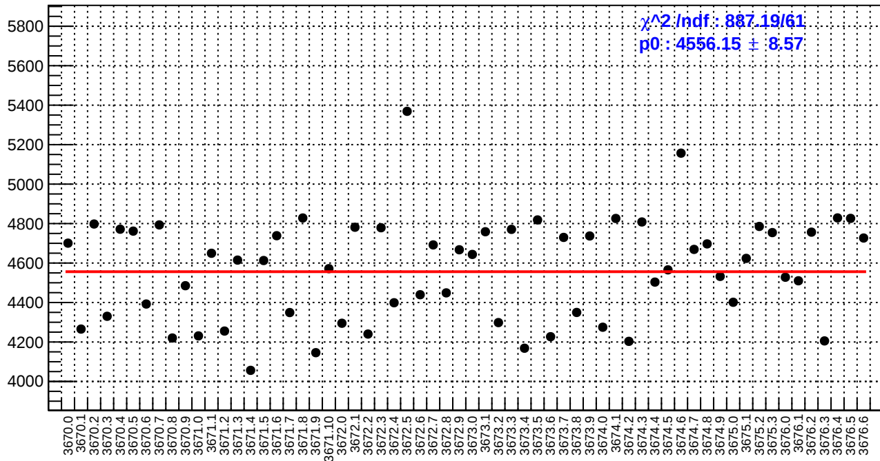
slug15: diff_bpm4eY.rms/nm
