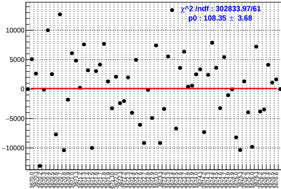
slug15: asym_right_avg.mean/ppb-reg_asym_right_avg.mean/ppb
