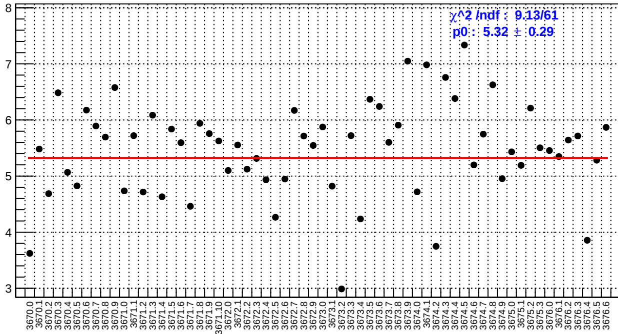
slug15: ds_avg_bpm4aY/(ppb/nm)
