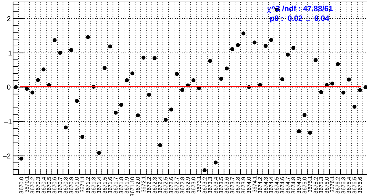
slug15: usl_bpm4aY/(ppb/nm)
