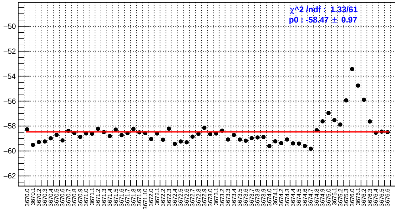
slug15: left_avg_bpm4eX/(ppb/nm)
