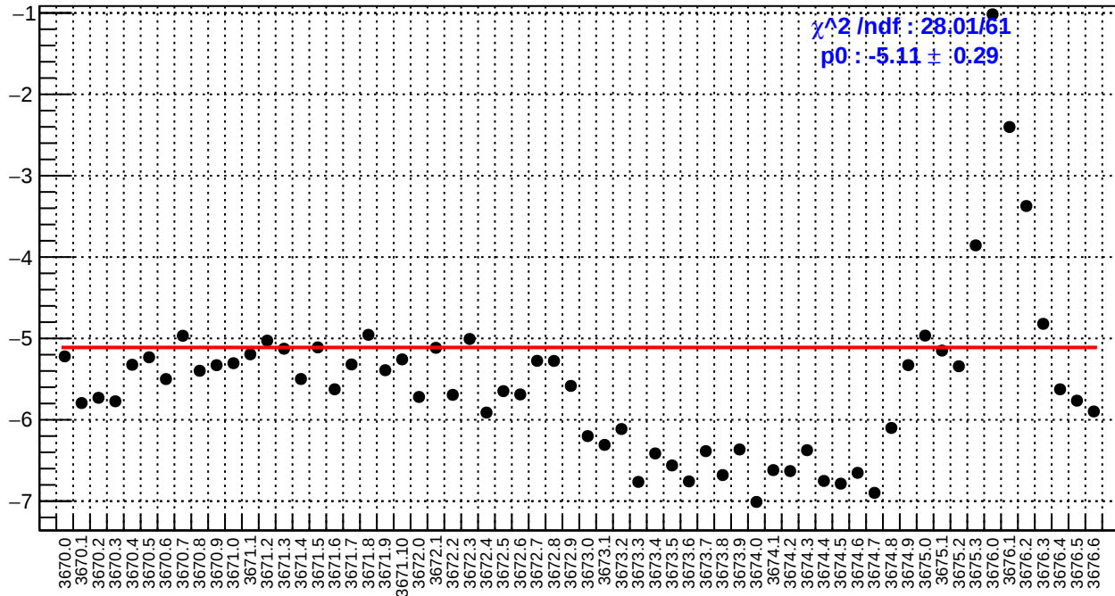
slug15: us_avg_bpm4eX/(ppb/nm)
