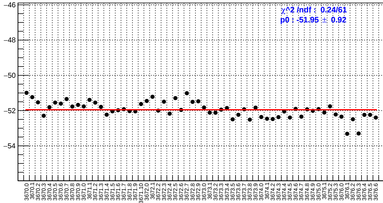
slug15: right_avg_bpm12X/(ppb/nm)
