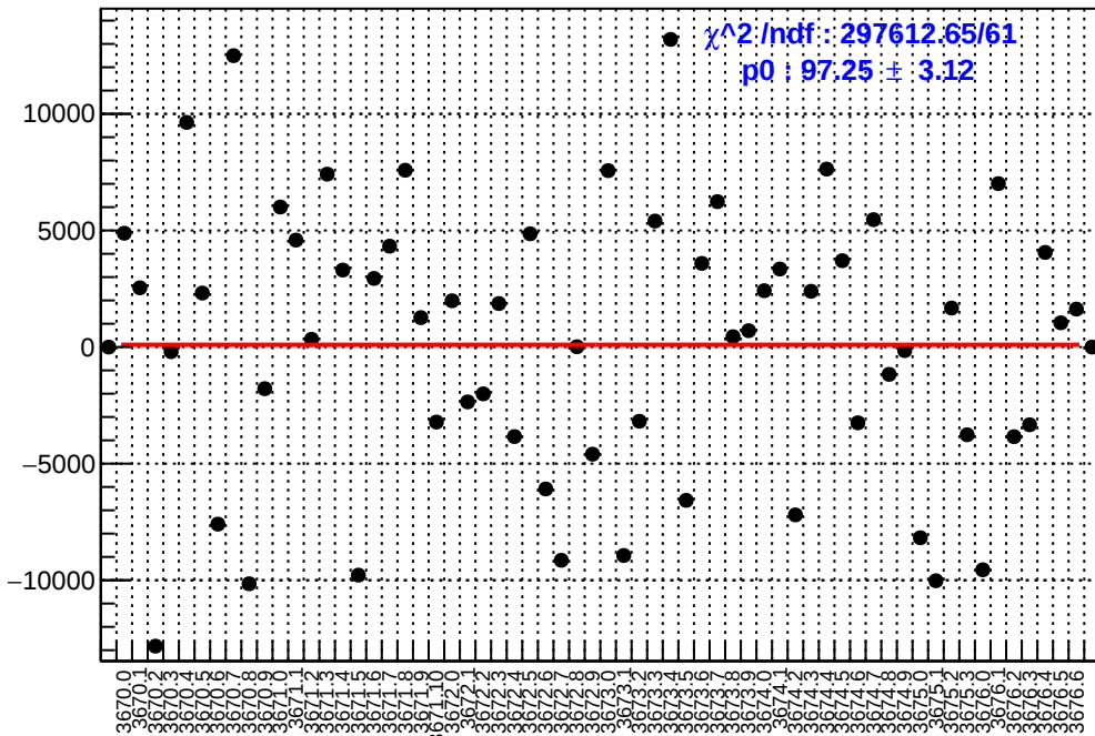
slug15: asym_dsr.mean/ppb-reg_asym_dsr.mean/ppb
