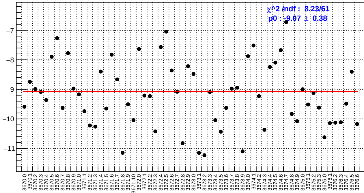
slug15: us_avg_bpm4aX/(ppb/nm)
