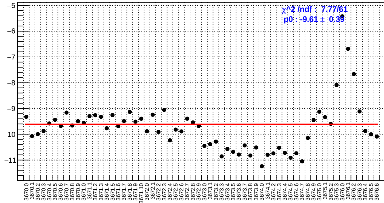
slug15: ds_avg_bpm4eX/(ppb/nm)
