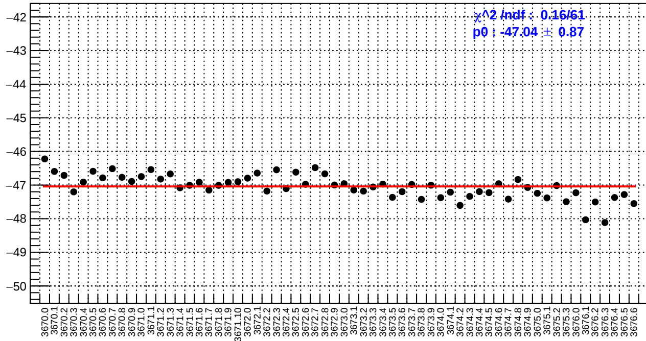
slug15: us_avg_bpm12X/(ppb/nm)
