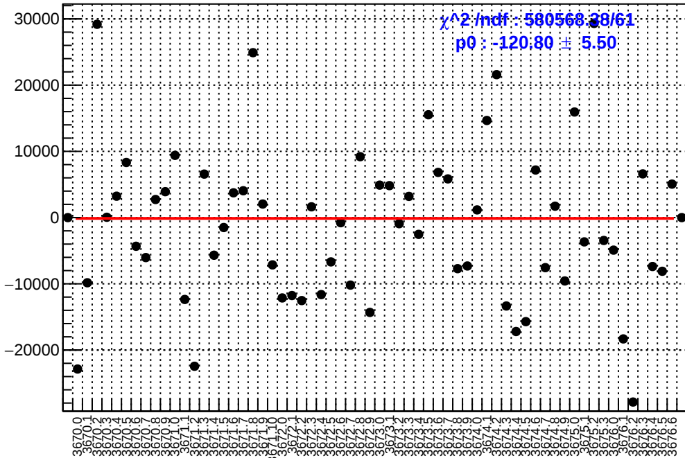
slug15: asym_sam5.mean/ppb-reg_asym_sam5.mean/ppb
