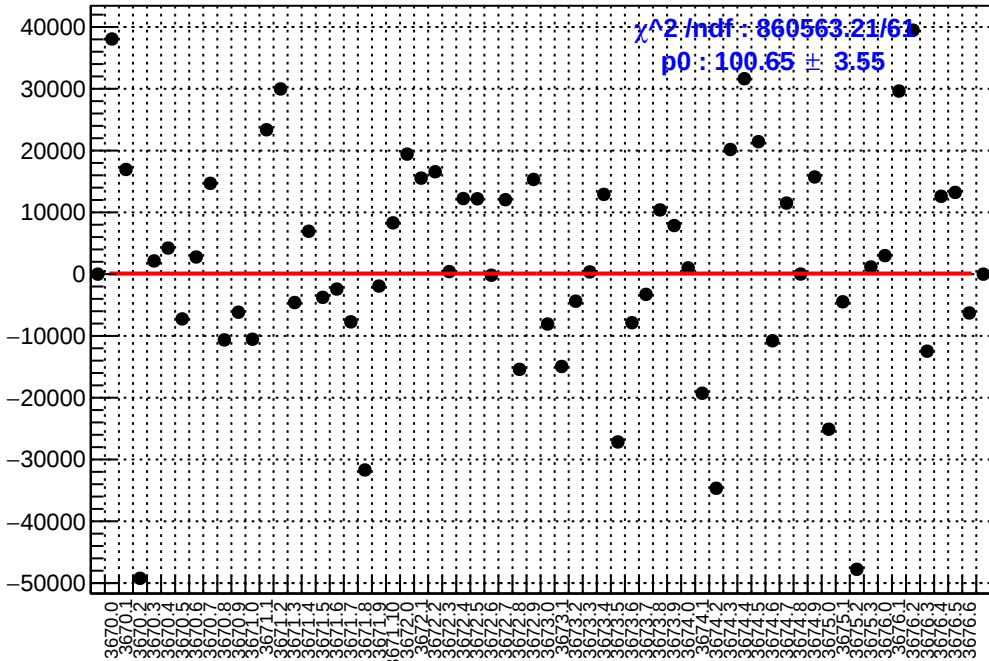
slug15: asym_sam1.mean/ppb-reg_asym_sam1.mean/ppb
