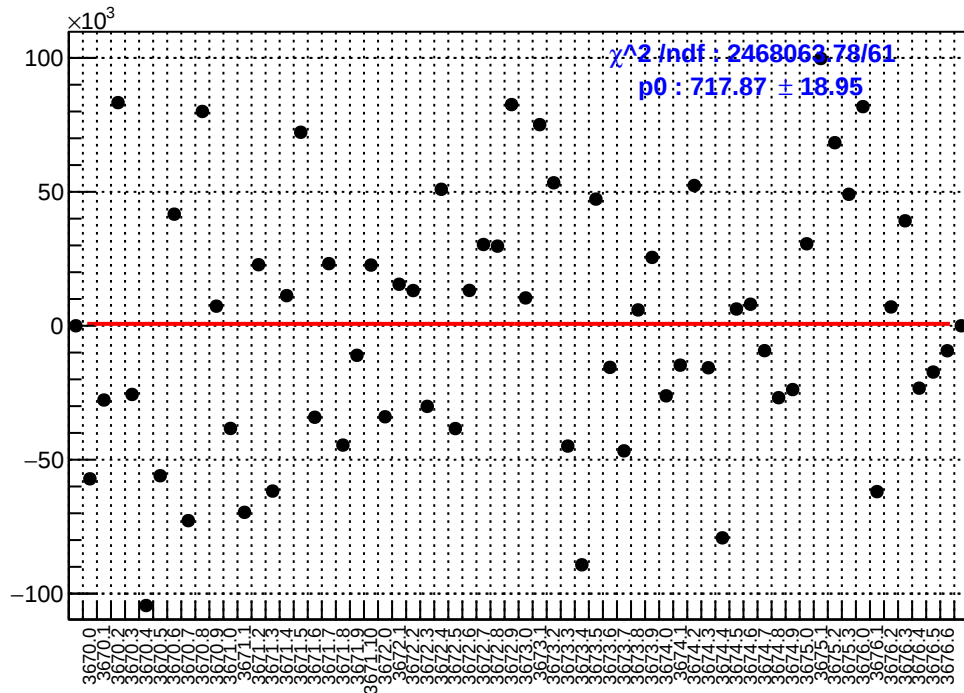
slug15: asym_sam3.mean/ppb-reg_asym_sam3.mean/ppb
