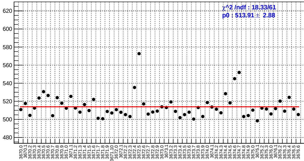
slug15: reg_asym_sam1.rms/ppm
