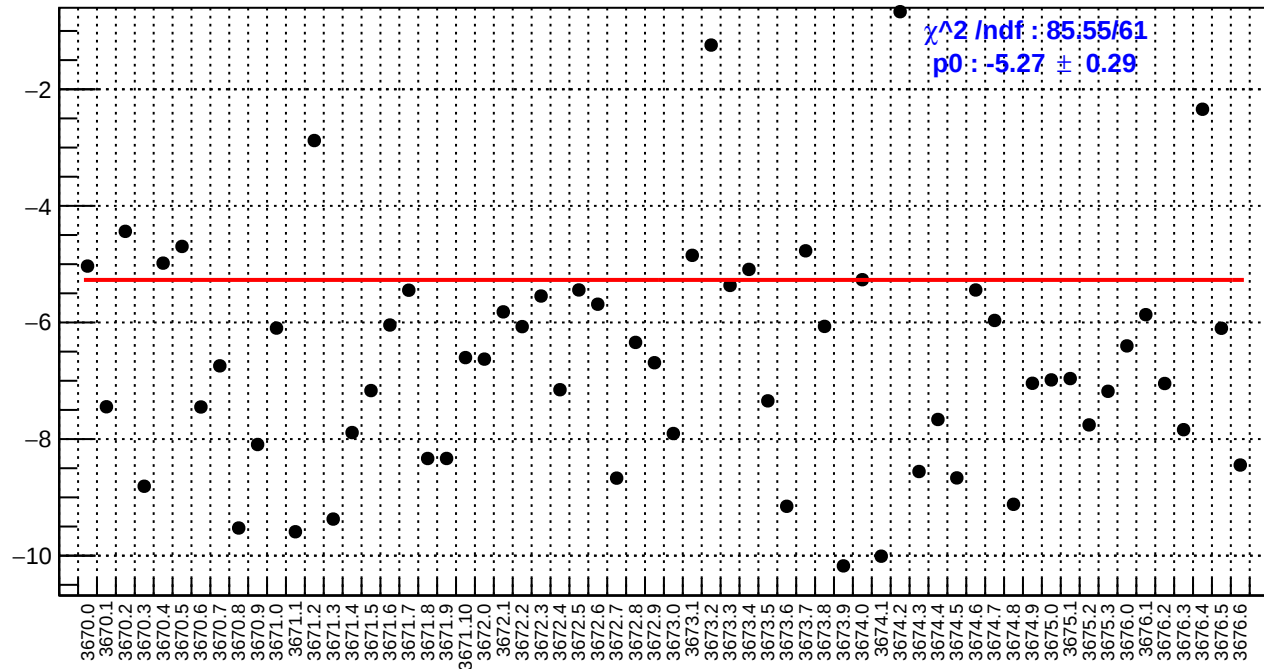
slug15: dsr_bpm4eY/(ppb/nm)
