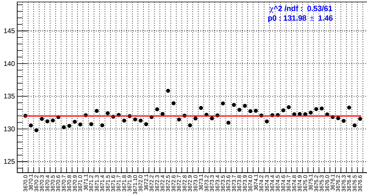
slug15: reg_asym_dsl.rms/ppm
