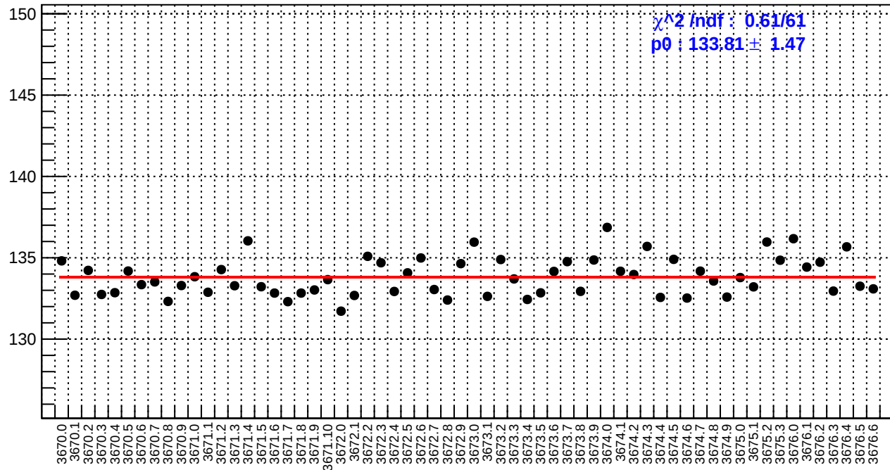
slug15: reg_asym_dsr.rms/ppm
