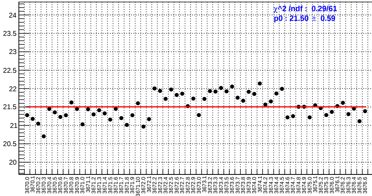
slug15: reg_asym_right_dd.rms/ppm
