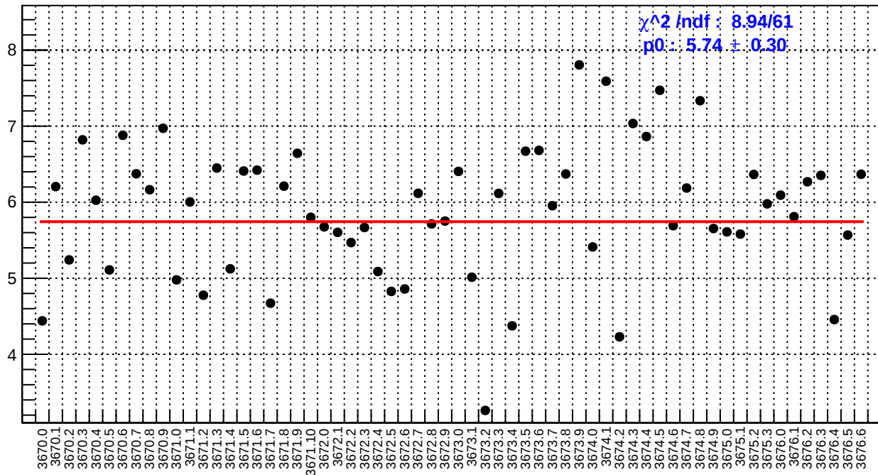
slug15: us_avg_bpm4aY/(ppb/nm)
