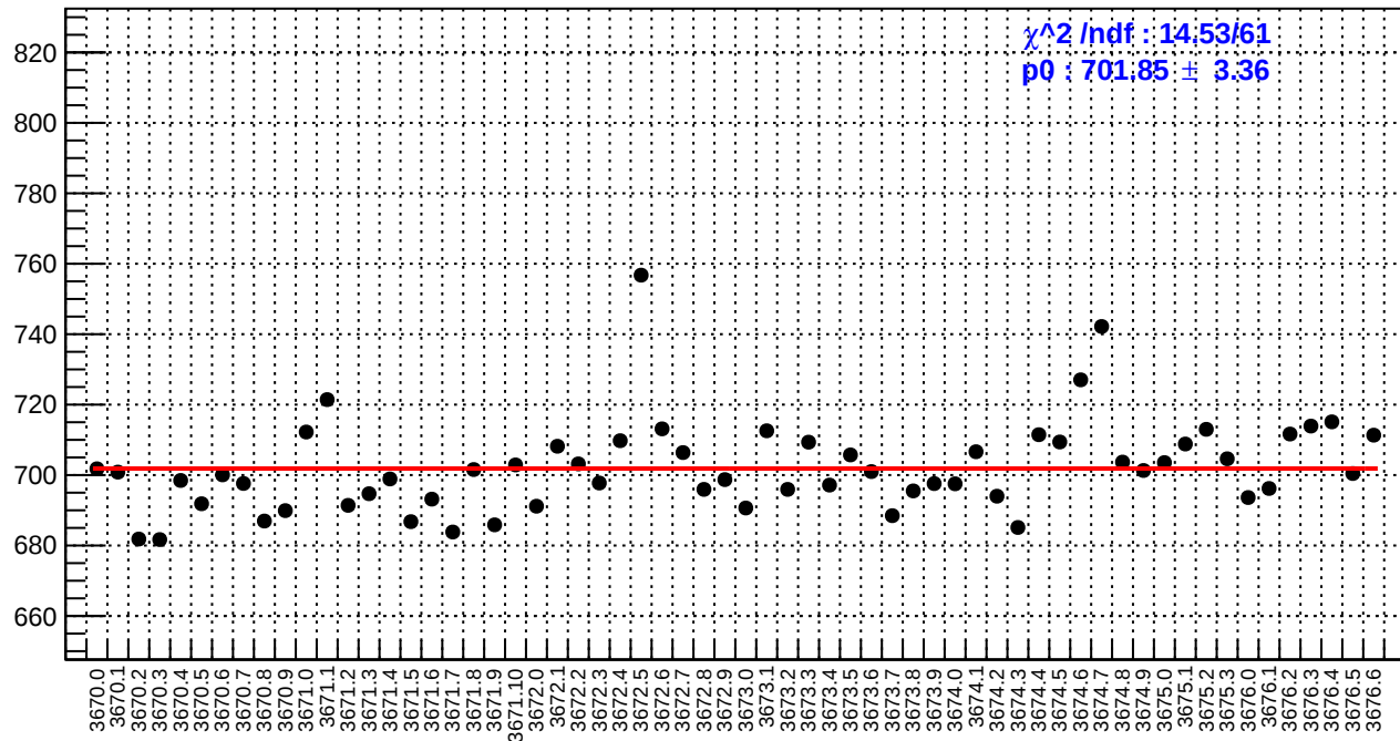
slug15: reg_asym_sam8.rms/ppm
