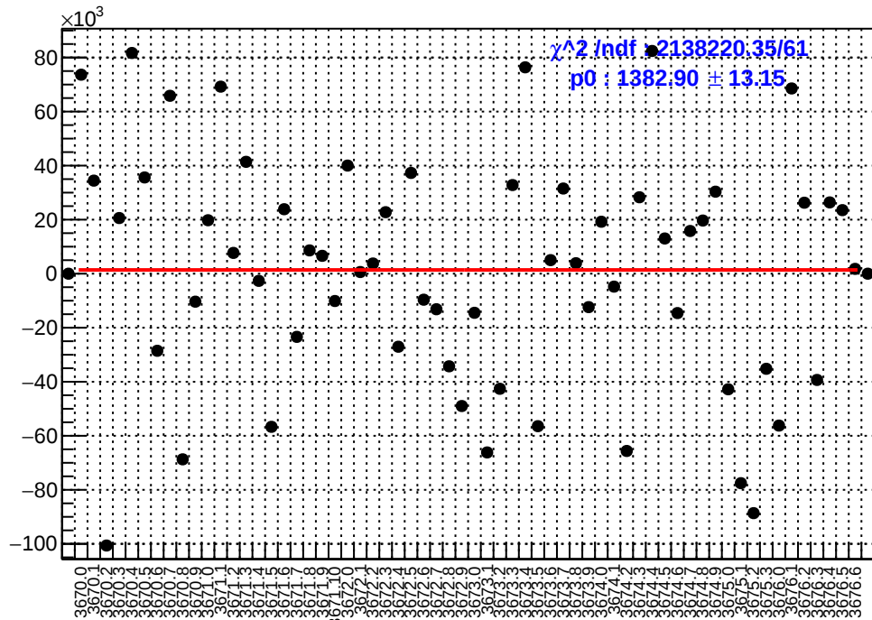
slug15: asym_sam8.mean/ppb-reg_asym_sam8.mean/ppb
