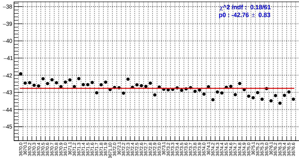
slug15: usl_bpm12X/(ppb/nm)
