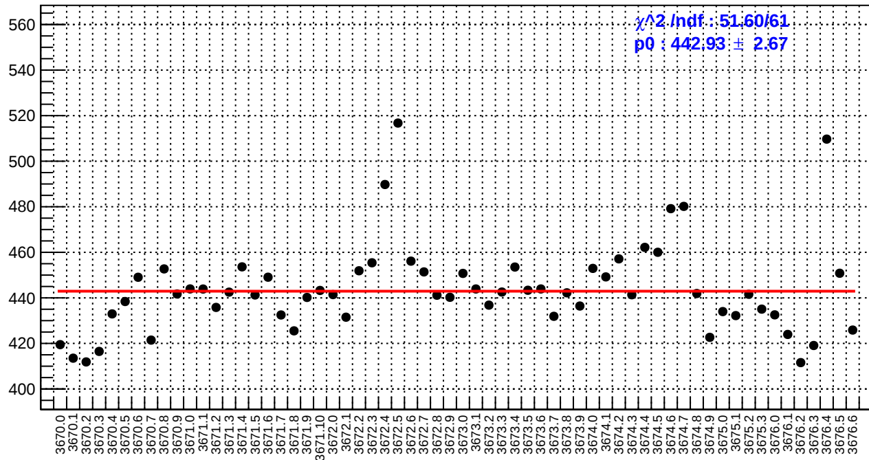
slug15: reg_asym_sam3.rms/ppm
