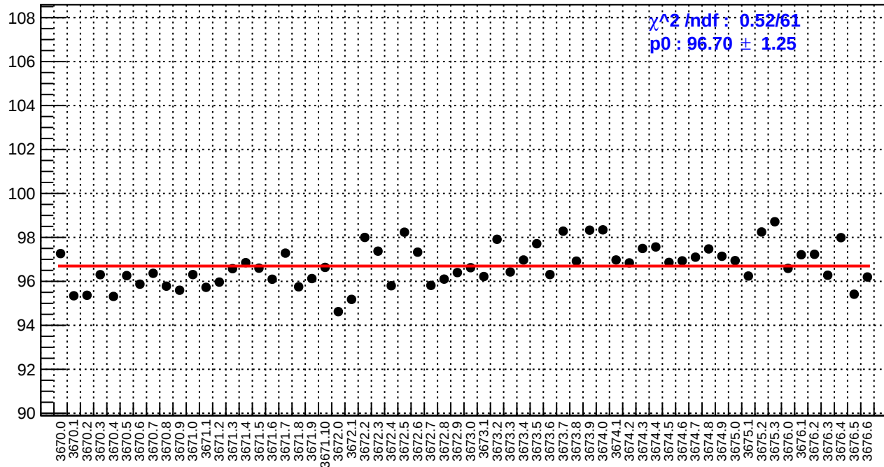
slug15: reg_asym_ds_avg.rms/ppm
