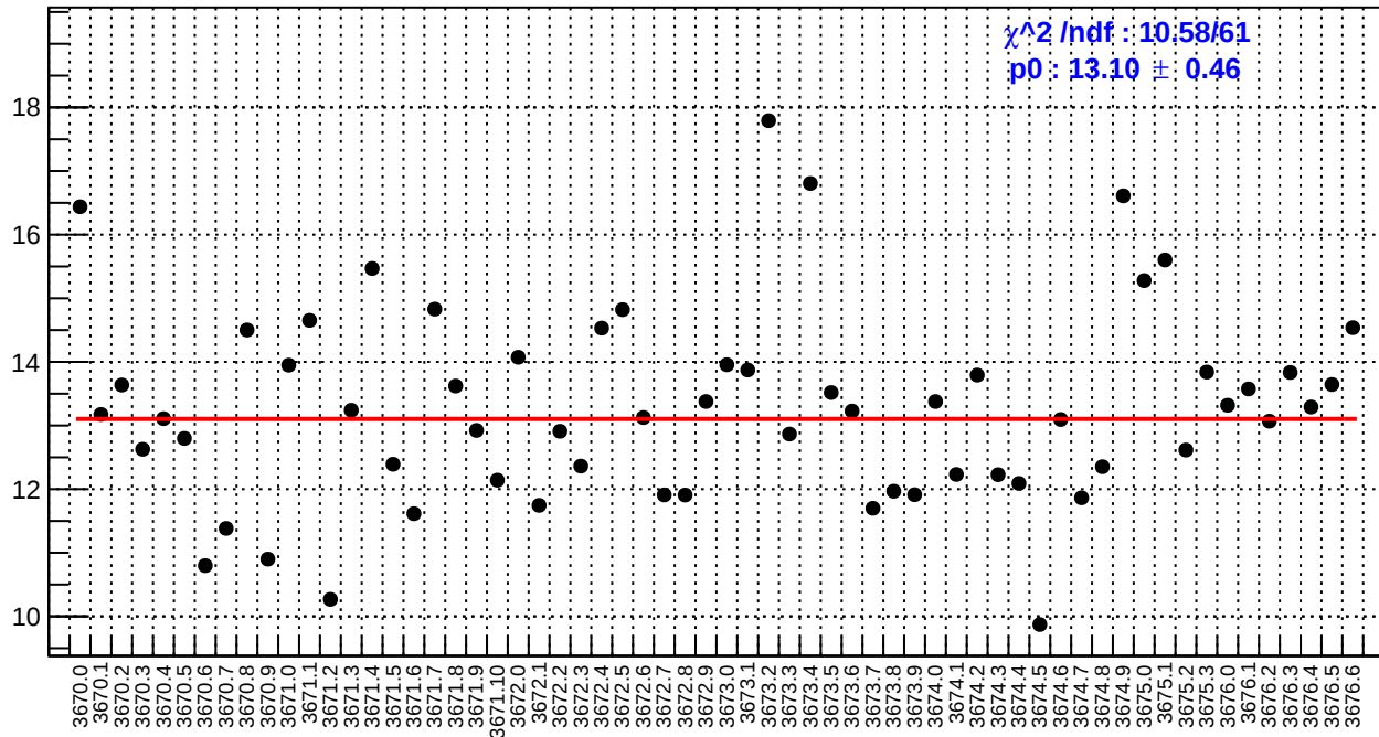
slug15: left_avg_bpm4eY/(ppb/nm)
