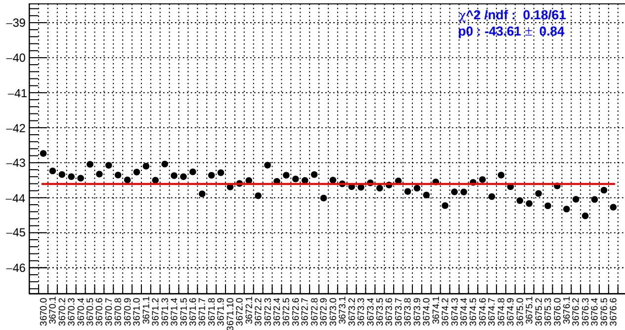
slug15: left_avg_bpm12X/(ppb/nm)
