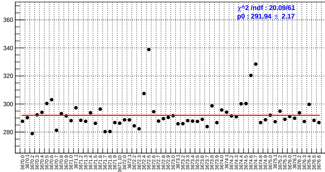
slug15: reg_asym_sam5.rms/ppm
