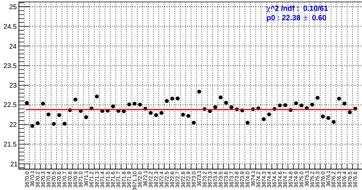
slug15: reg_asym_left_dd.rms/ppm
