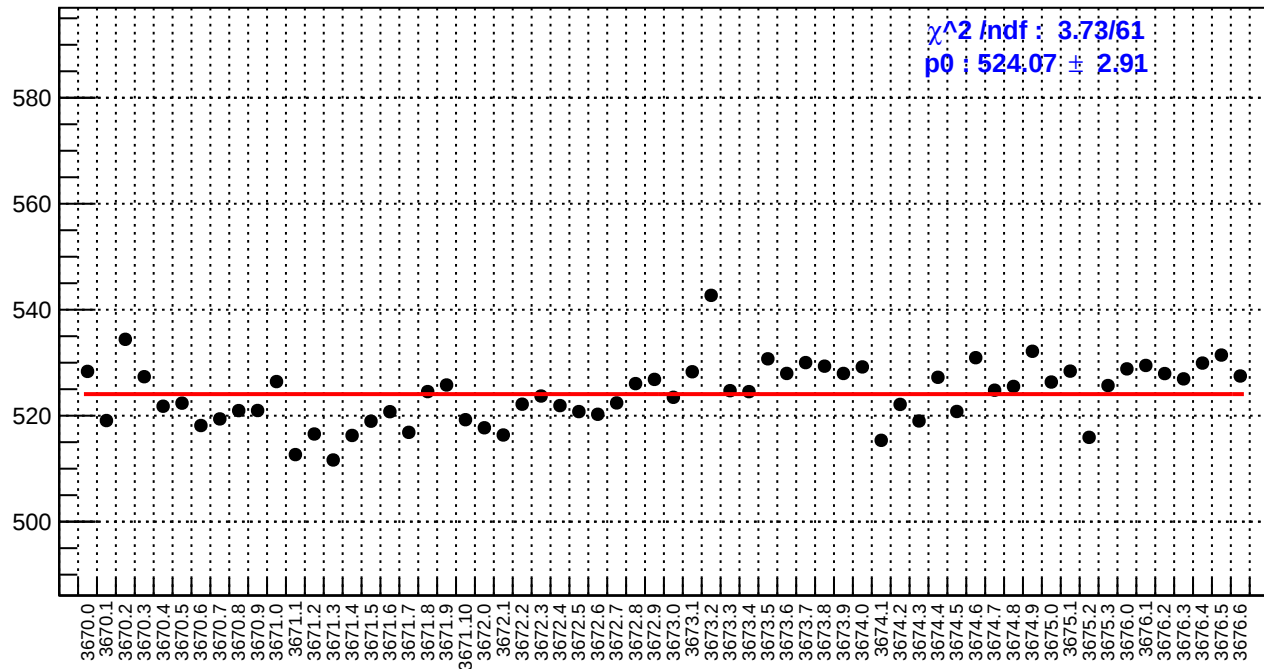
slug15: asym_bcm_an_ds.rms/ppm
