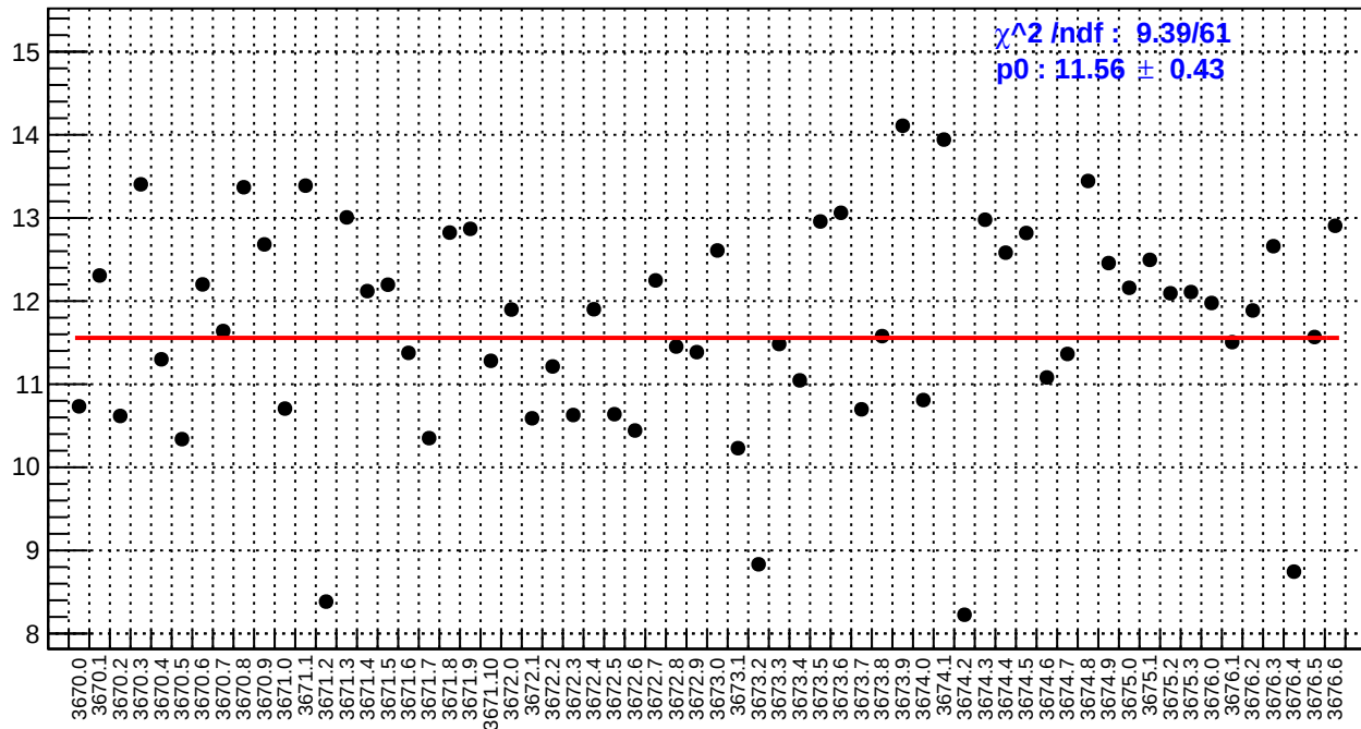
slug15: right_avg_bpm4aY/(ppb/nm)
