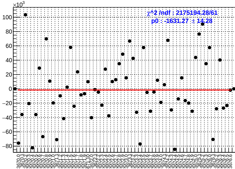
slug15: asym_sam4.mean/ppb-reg_asym_sam4.mean/ppb
