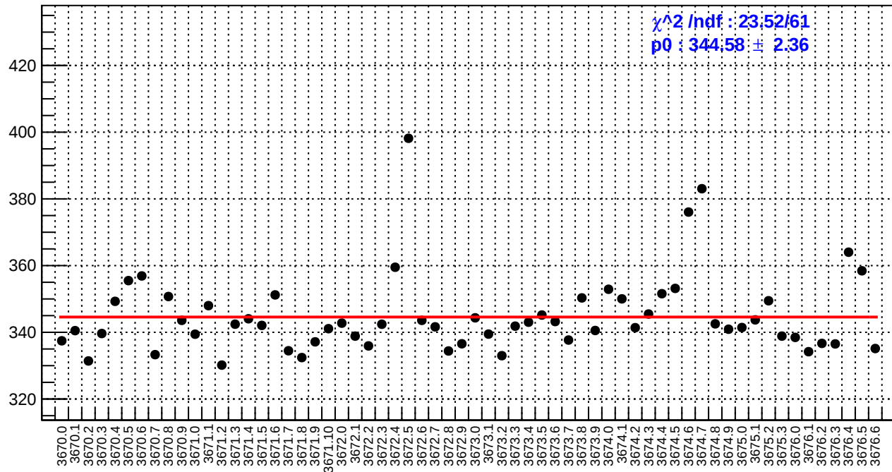
slug15: reg_asym_sam7.rms/ppm
