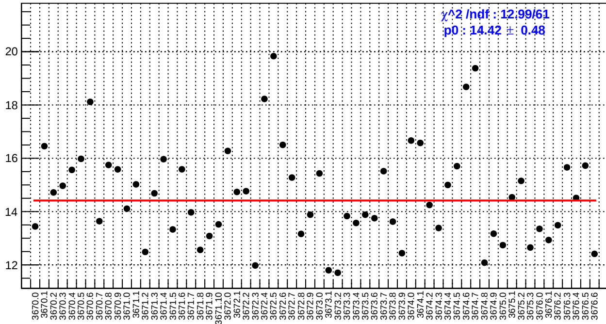
slug15: left_avg_bpm4aX/(ppb/nm)
