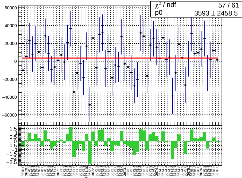
slug15: reg_asym_sam2.mean/ppb
