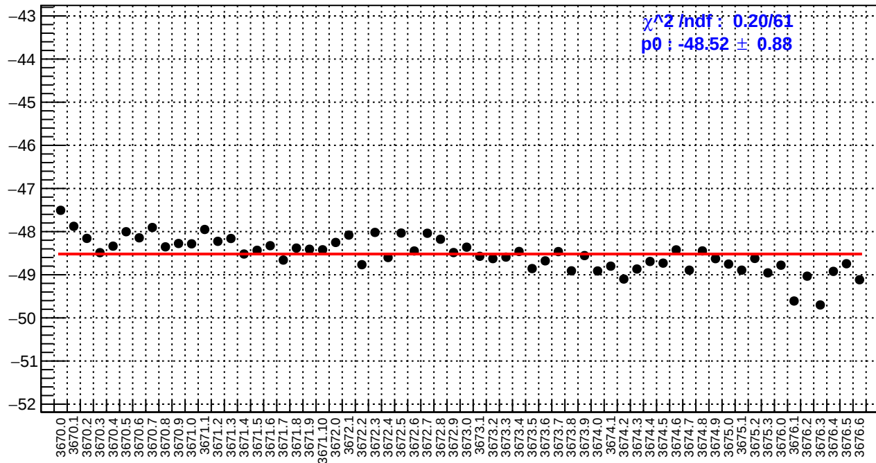
slug15: ds_avg_bpm12X/(ppb/nm)
