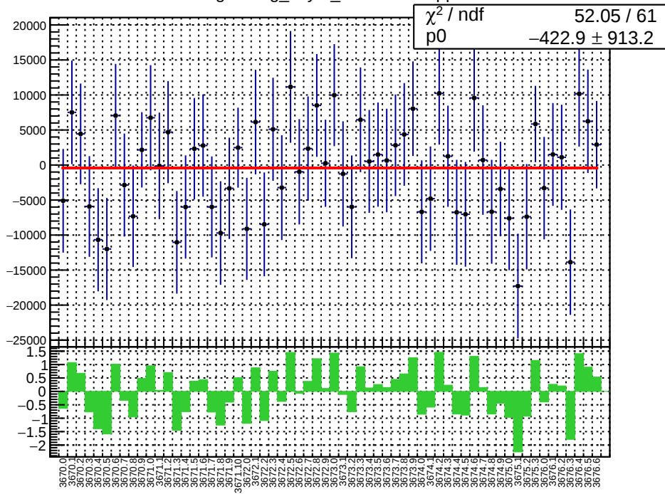
slug15: reg_asym_sam8.mean/ppb
