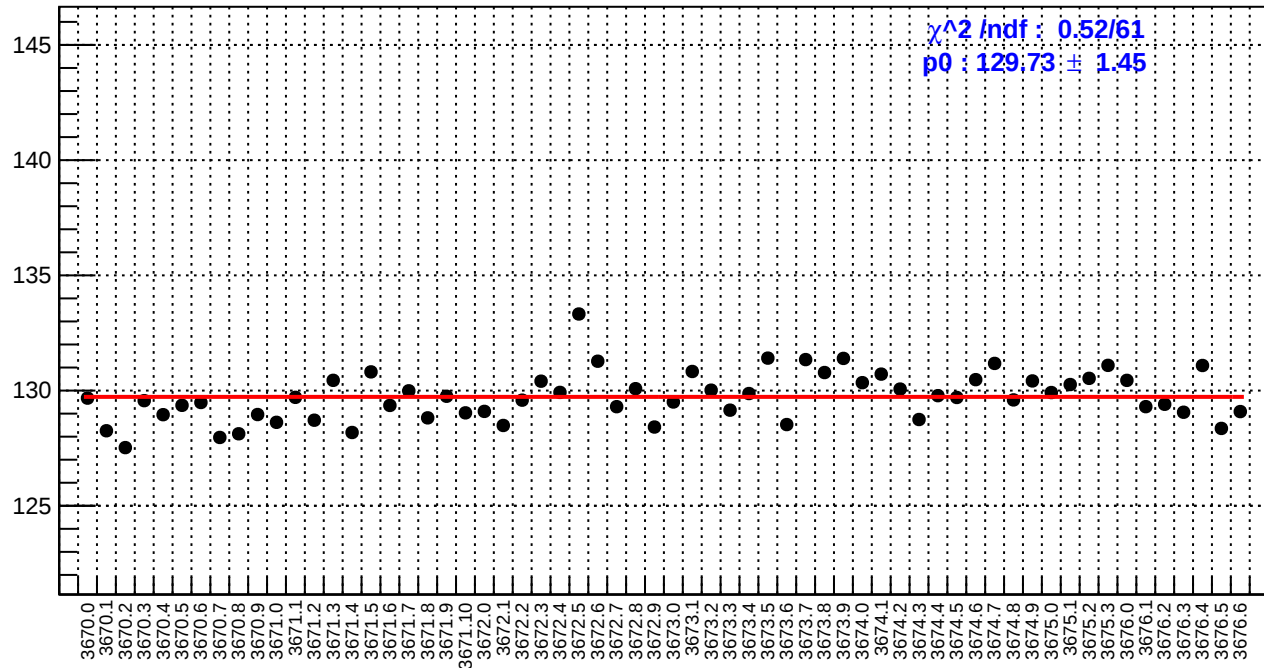
slug15: reg_asym_left_avg.rms/ppm
