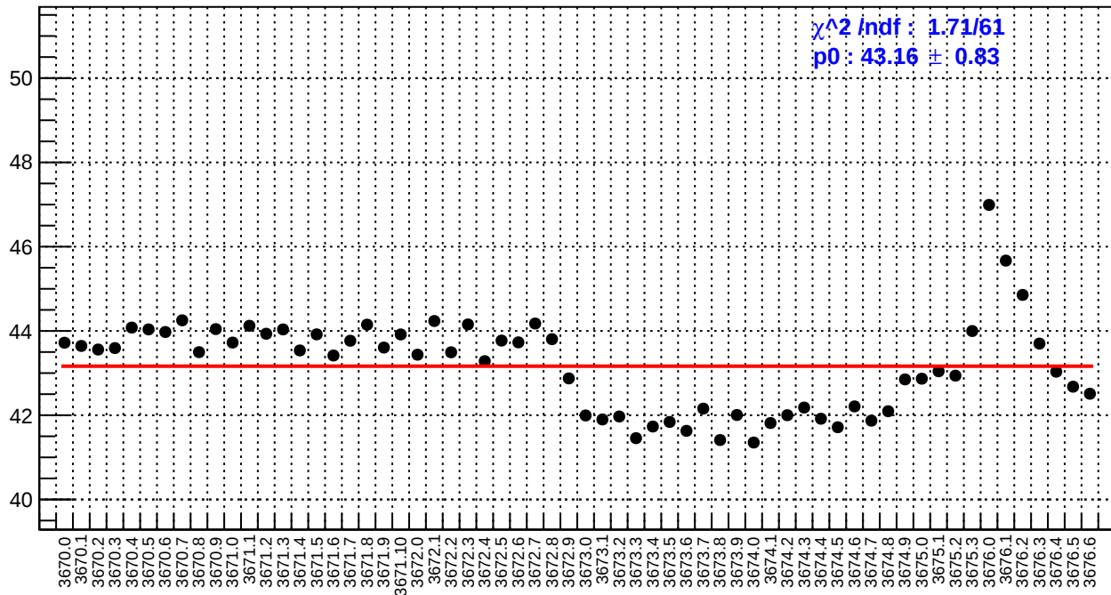
slug15: right_avg_bpm4eX/(ppb/nm)
