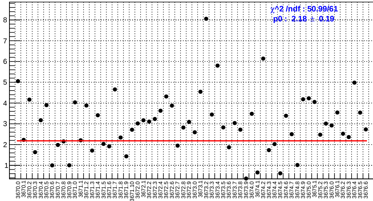
slug15: us_avg_bpm4eY/(ppb/nm)
