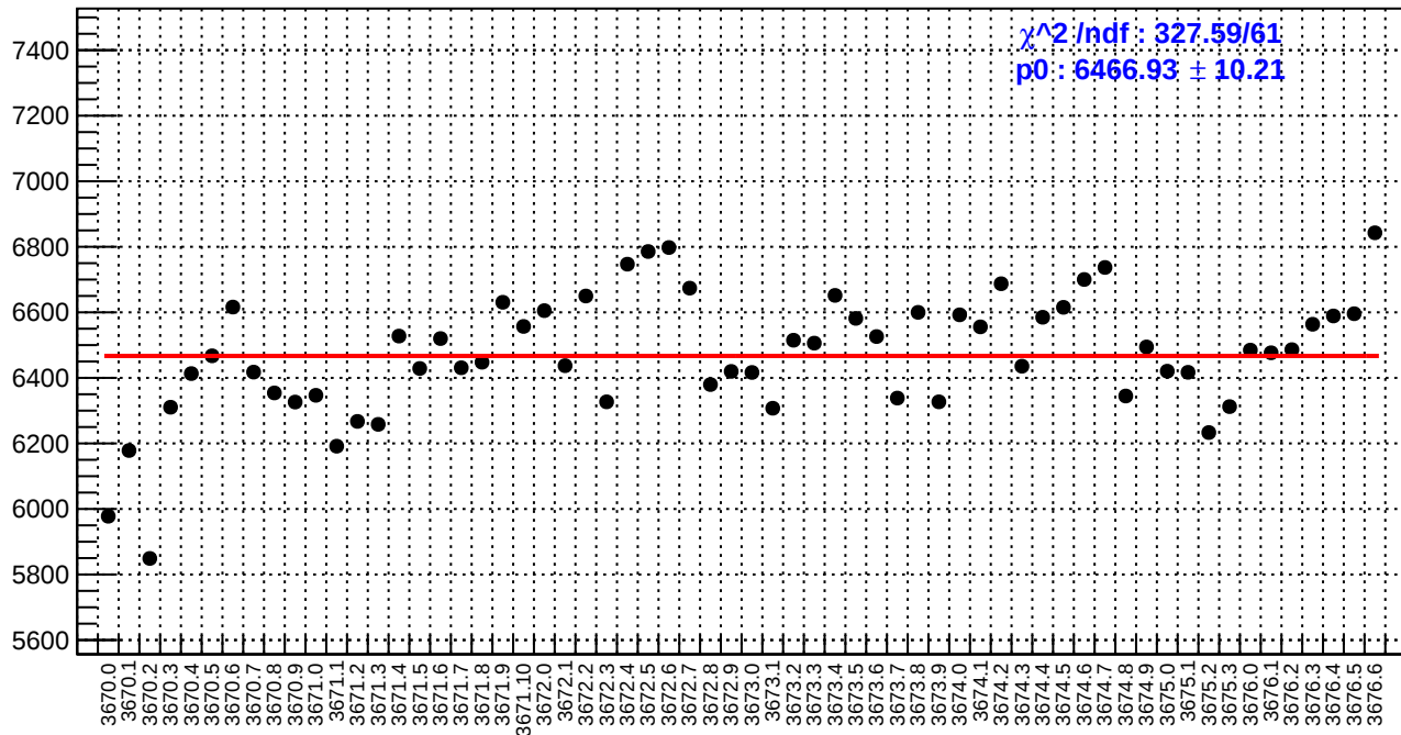
slug15: diff_bpm11X.rms/nm
