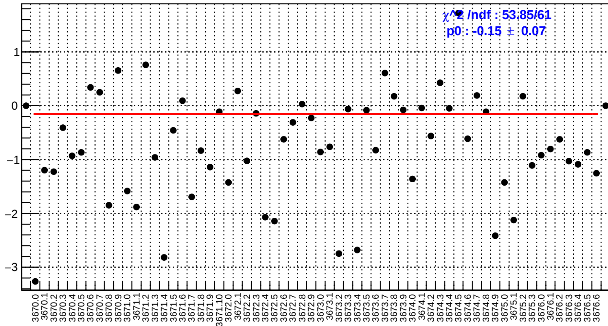
slug15: dsl_bpm4aY/(ppb/nm)
