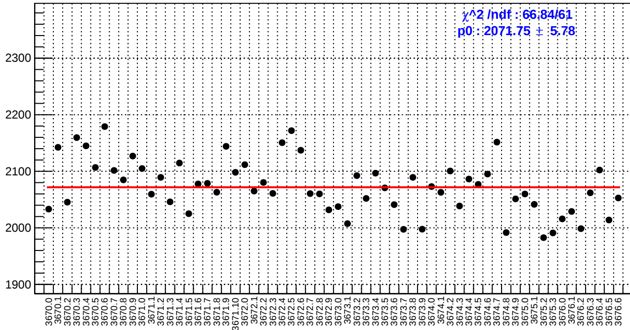
slug15: diff_bpm4aX.rms/nm
