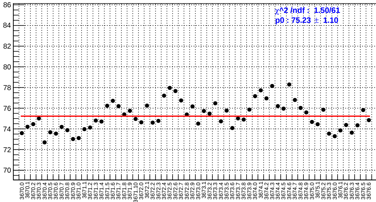
slug15: asym_bcm_an_ds3.rms/ppm
