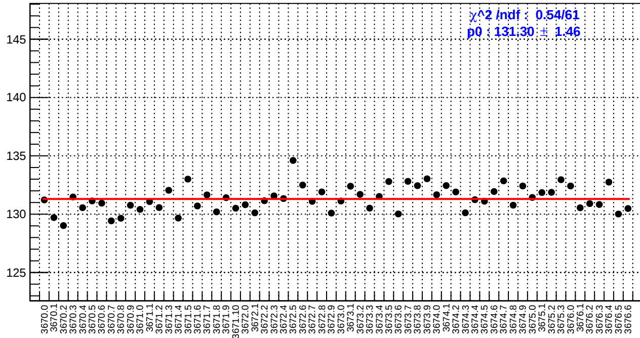
slug15: reg_asym_usl.rms/ppm
