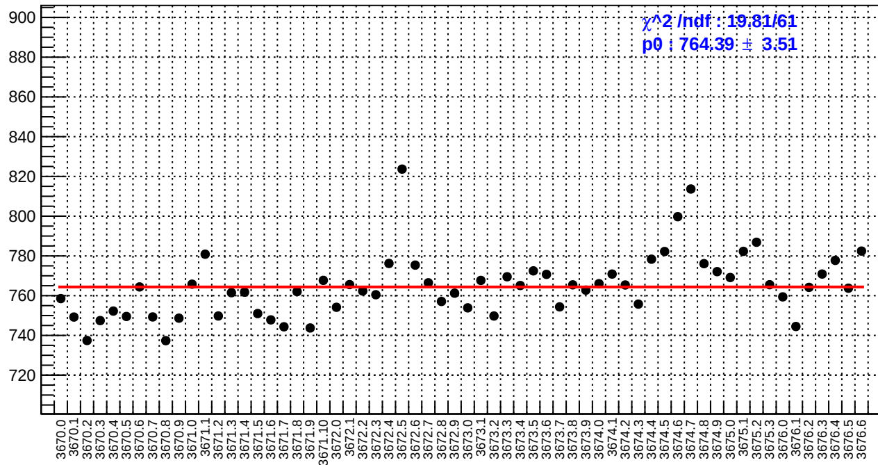
slug15: reg_asym_sam4.rms/ppm
