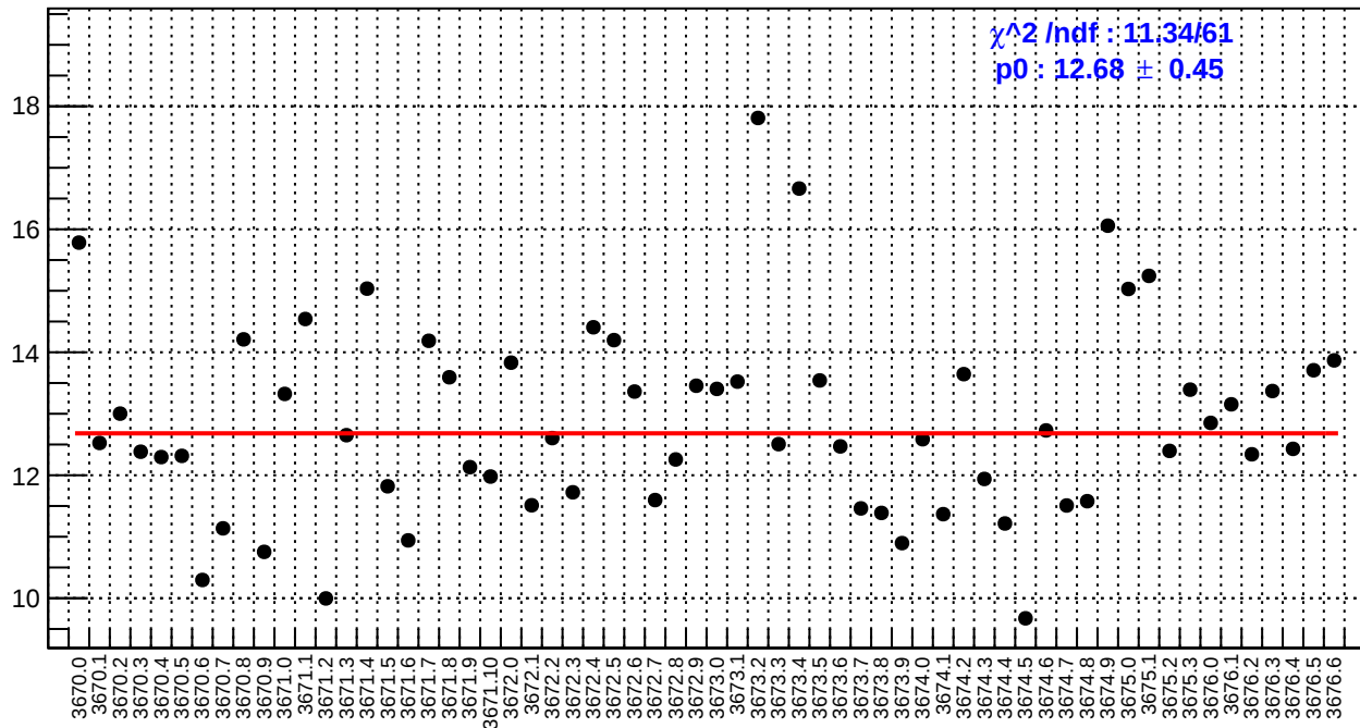
slug15: usl_bpm4eY/(ppb/nm)
