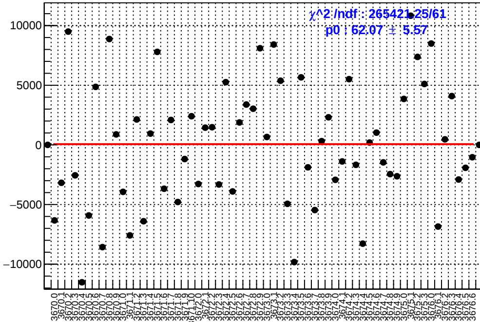
slug15: asym_ds_dd.mean/ppb-reg_asym_ds_dd.mean/ppb
