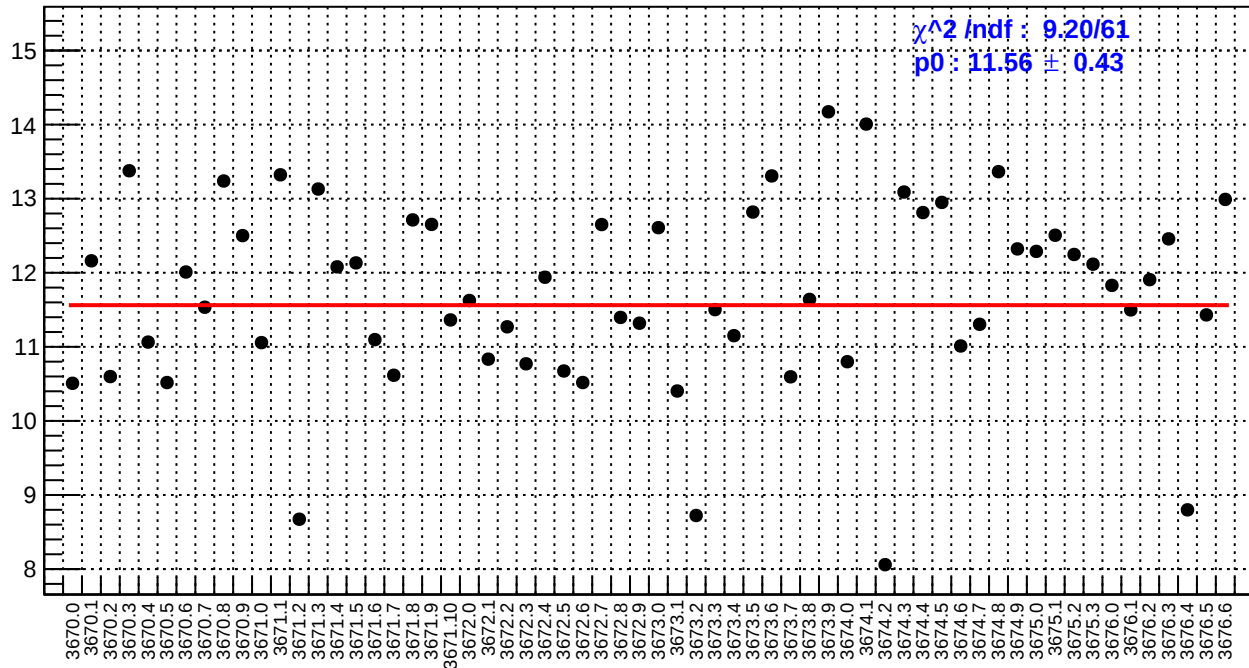
slug15: dsr_bpm4aY/(ppb/nm)
