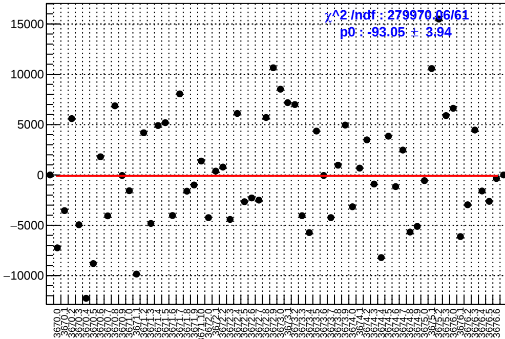
slug15: asym_usl.mean/ppb-reg_asym_usl.mean/ppb
