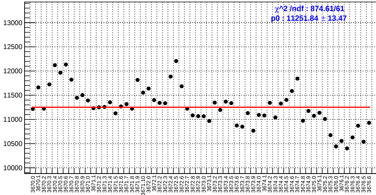
slug15: diff_bpm4eX.rms/nm
