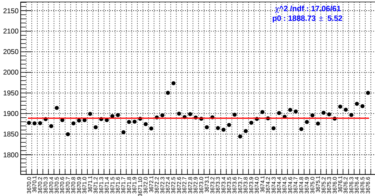
slug15: reg_asym_sam2.rms/ppm
