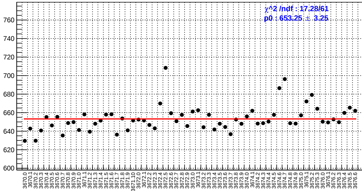
slug15: reg_asym_sam6.rms/ppm
