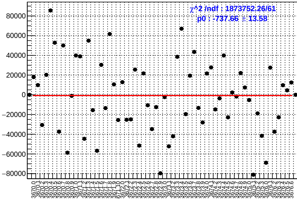
slug15: asym_sam6.mean/ppb-reg_asym_sam6.mean/ppb
