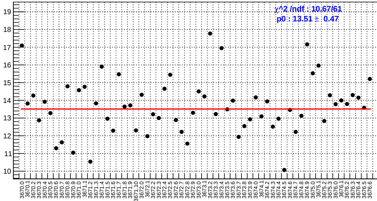
slug15: dsl_bpm4eY/(ppb/nm)
