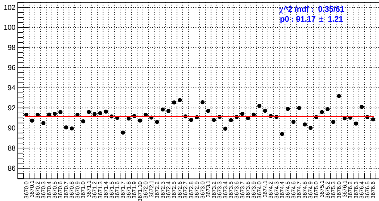
slug15: reg_asym_ds_dd.rms/ppm
