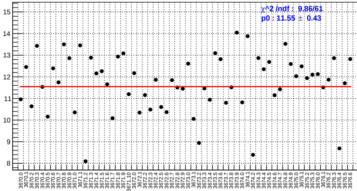
slug15: usr_bpm4aY/(ppb/nm)
