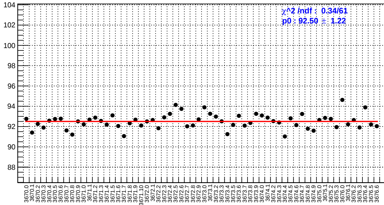
slug15: reg_asym_us_dd.rms/ppm
