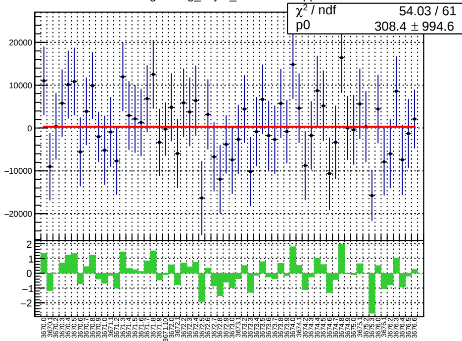
slug15: reg_asym_sam4.mean/ppb
