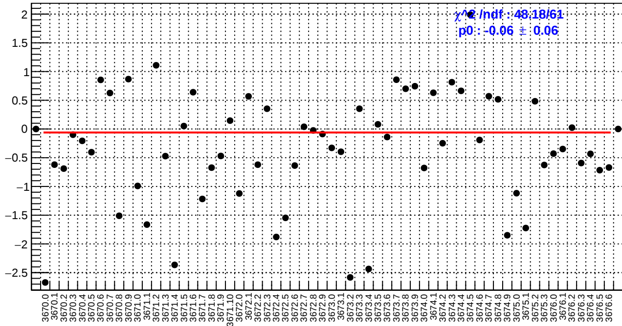
slug15: left_avg_bpm4aY/(ppb/nm)
