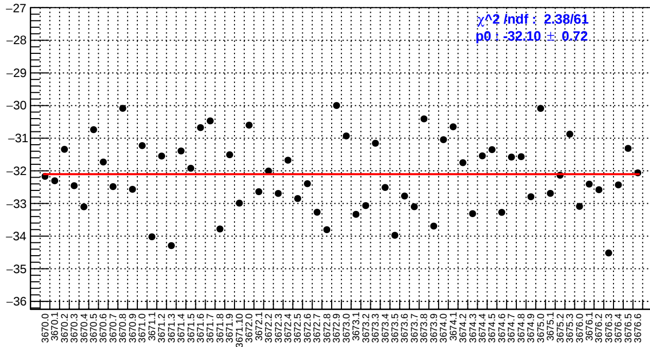
slug15: right_avg_bpm4aX/(ppb/nm)
