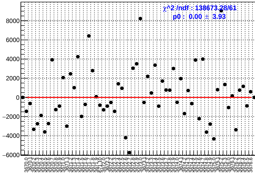
slug15: asym_ds_avg.mean/ppb-reg_asym_ds_avg.mean/ppb
