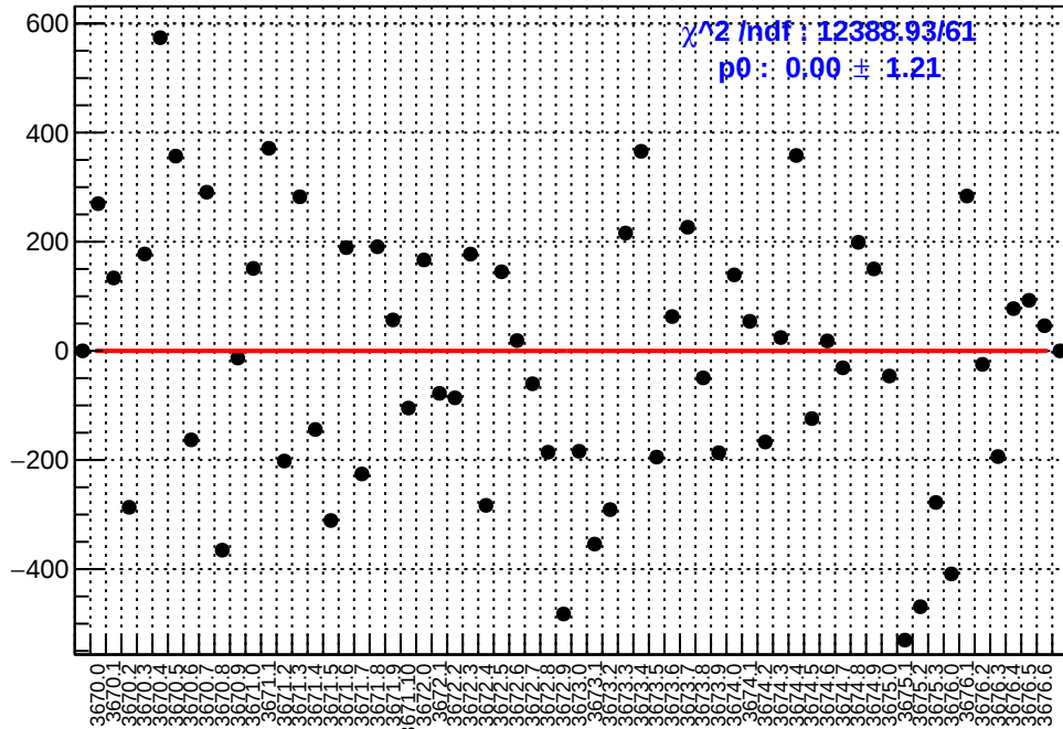
slug15: asym_left_dd.mean/ppb-reg_asym_left_dd.mean/ppb
