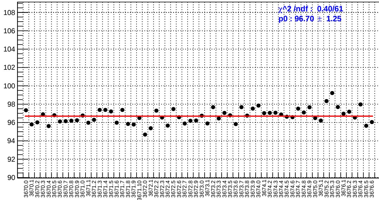
slug15: reg_asym_us_avg.rms/ppm
