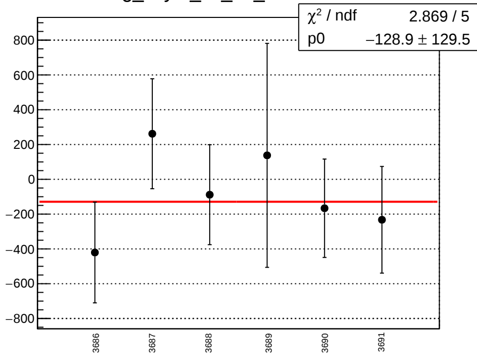
reg_asym_ds_dd_mean vs run
