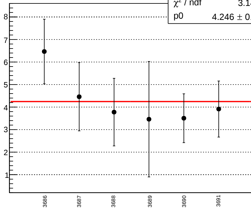
cor_asym_sam5_diff_bpm4aX_slope vs run
