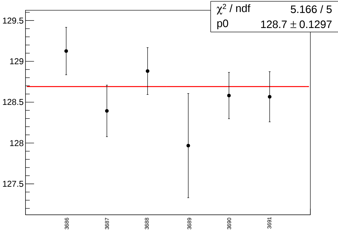
reg_asym_left_avg_rms vs run
