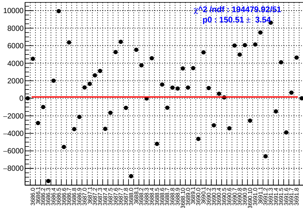
slug17: asym_ds_dd.mean/ppb-reg_asym_ds_dd.mean/ppb
