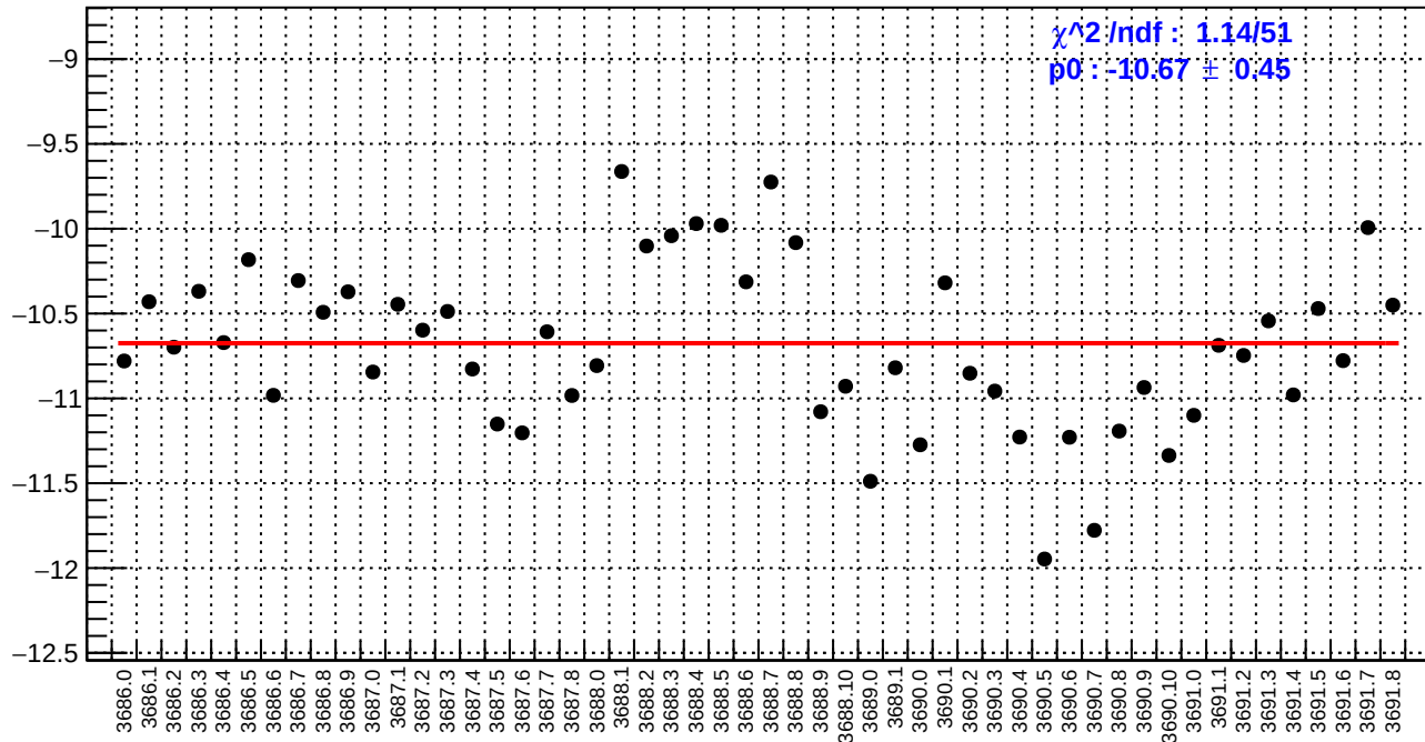
slug17: ds_avg_bpm4eX/(ppb/nm)
