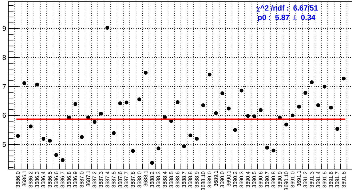
slug17: us_avg_bpm4aY/(ppb/nm)
