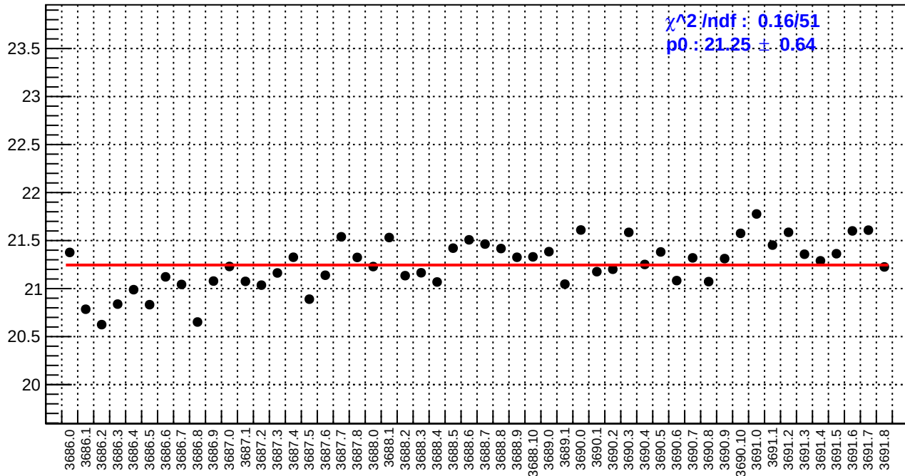
slug17: reg_asym_right_dd.rms/ppm
