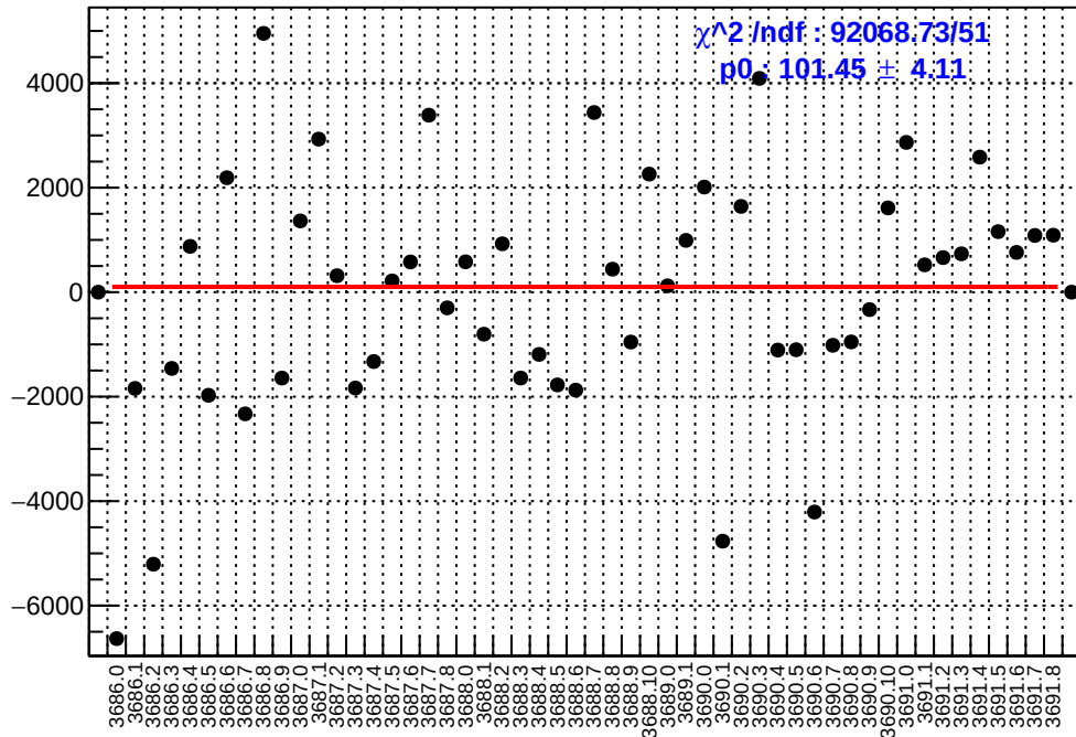
slug17: asym_us_avg.mean/ppb-reg_asym_us_avg.mean/ppb
