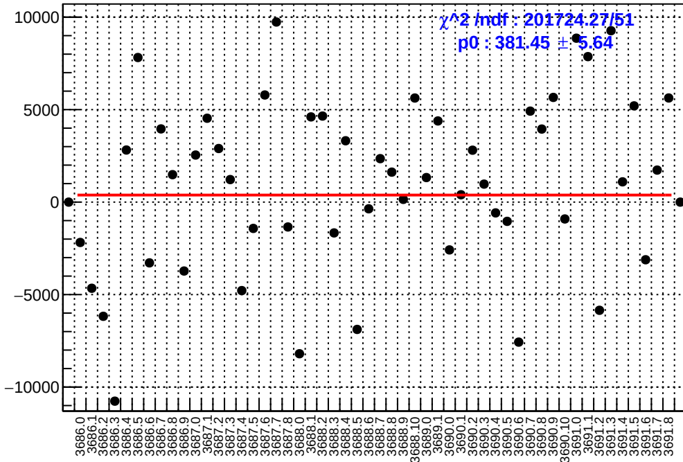
slug17: asym_usl.mean/ppb-reg_asym_usl.mean/ppb
