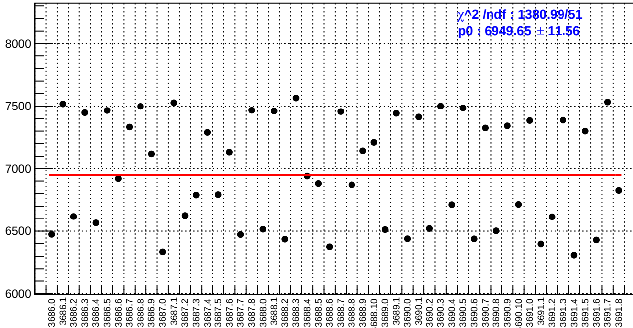
slug17: diff_bpm4aY.rms/nm
