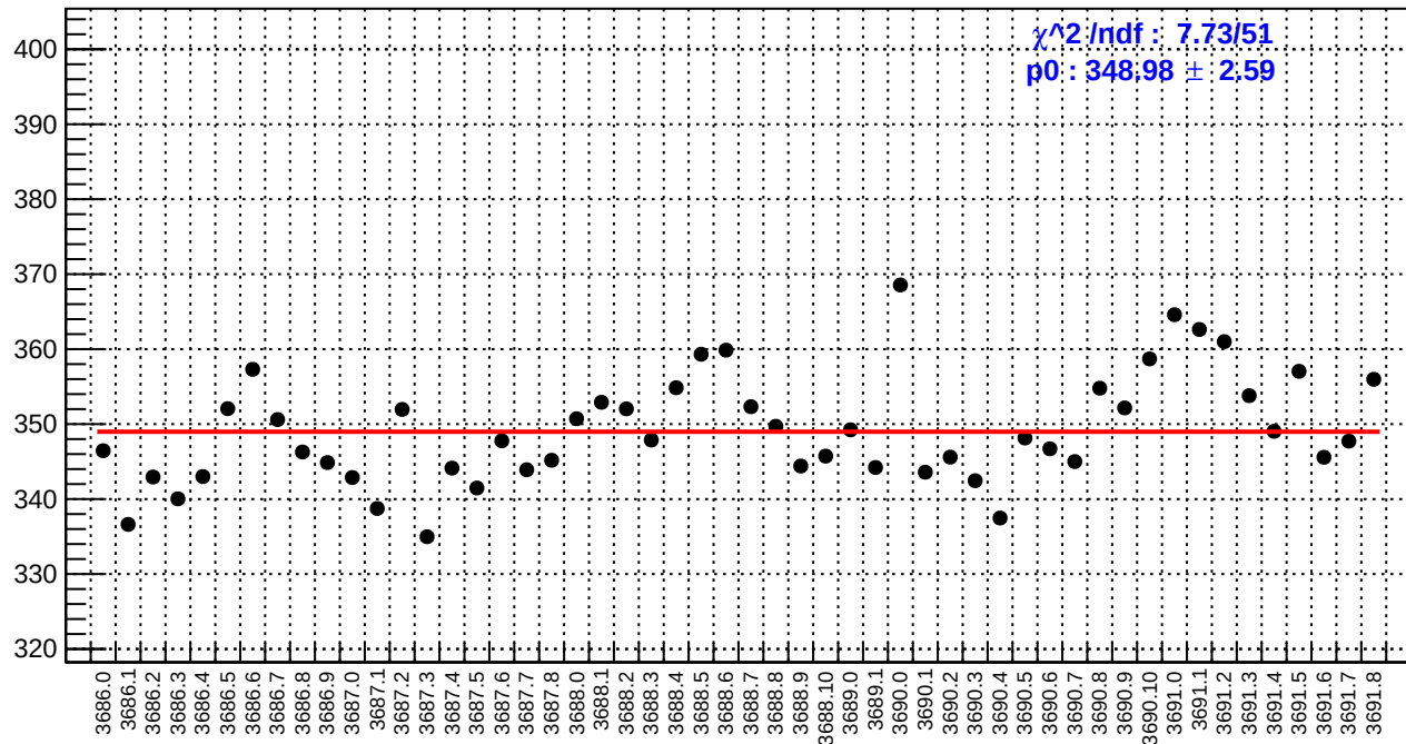
slug17: reg_asym_sam7.rms/ppm
