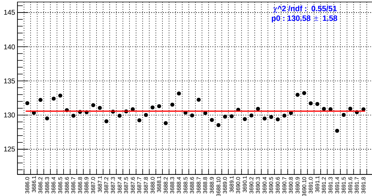
slug17: reg_asym_dsl.rms/ppm
