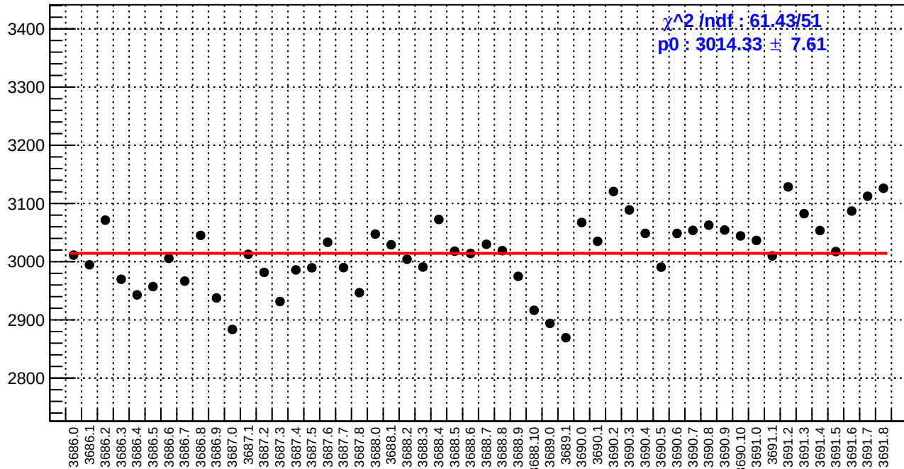
slug17: asym_bcm_an_us.rms/ppm
