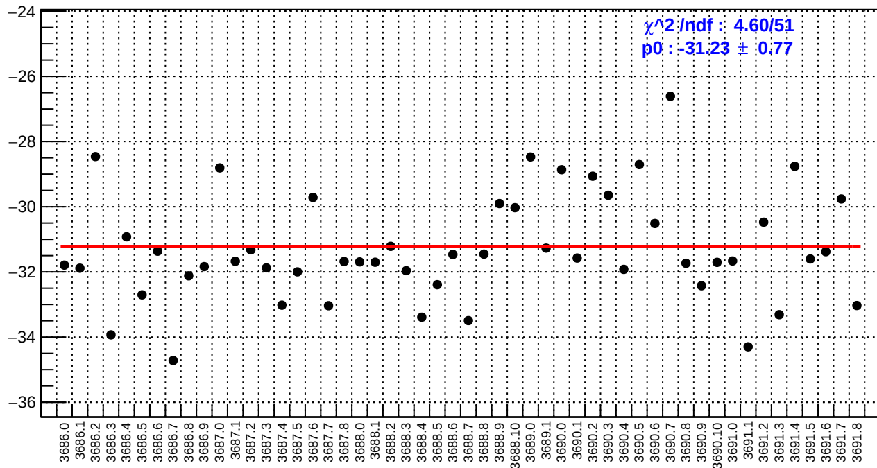
slug17: dsr_bpm4aX/(ppb/nm)
