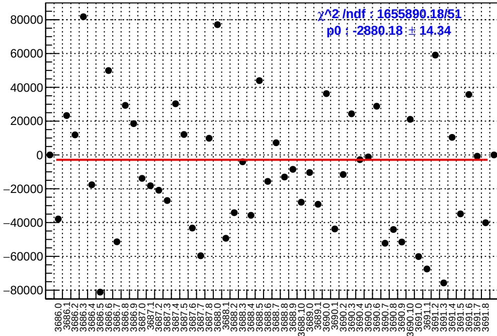
slug17: asym_sam7.mean/ppb-reg_asym_sam7.mean/ppb
