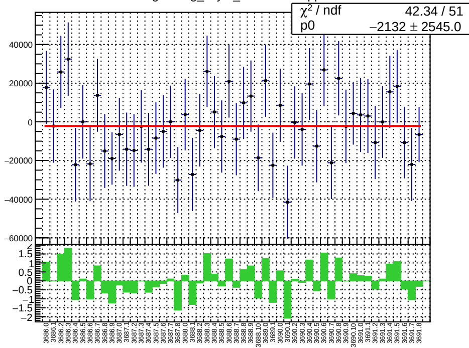
slug17: reg_asym_sam2.mean/ppb
