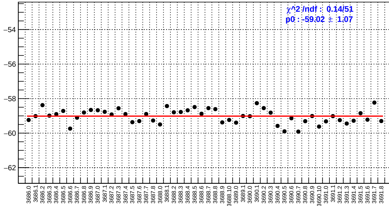
slug17: left_avg_bpm4eX/(ppb/nm)
