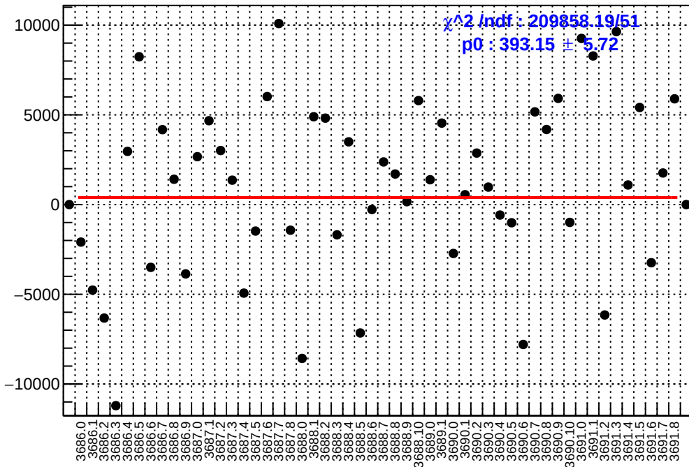
slug17: asym_left_avg.mean/ppb-reg_asym_left_avg.mean/ppb
