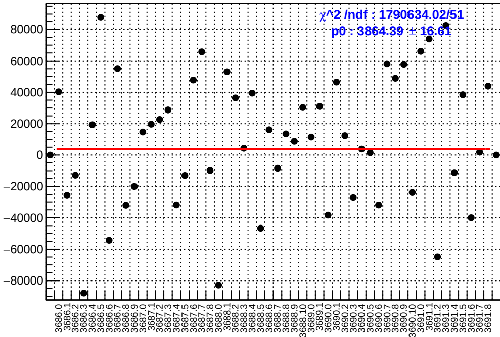
slug17: asym_sam3.mean/ppb-reg_asym_sam3.mean/ppb
