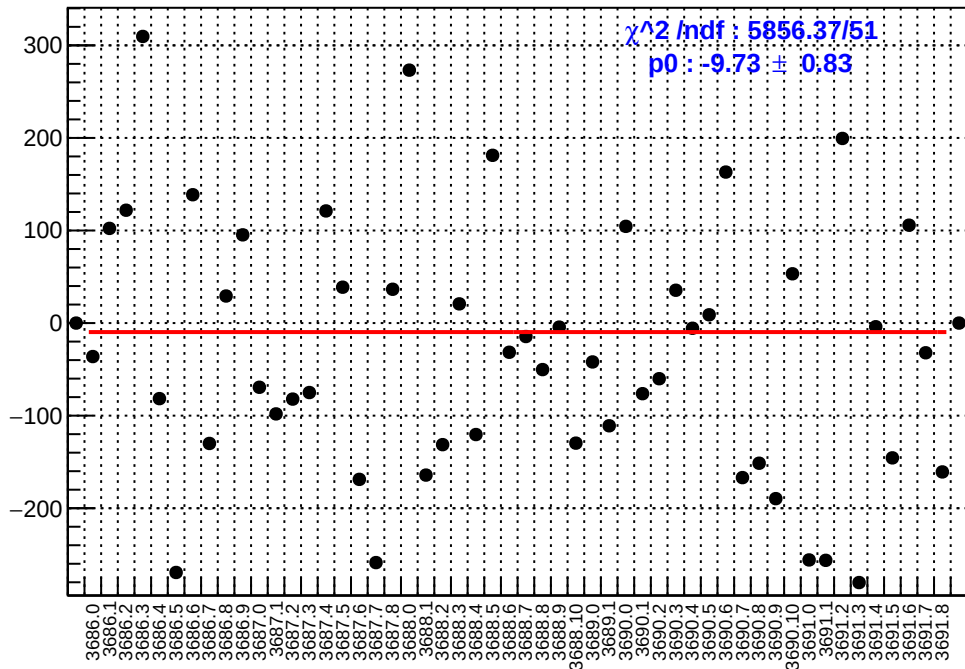
slug17: asym_right_dd.mean/ppb-reg_asym_right_dd.mean/ppb
