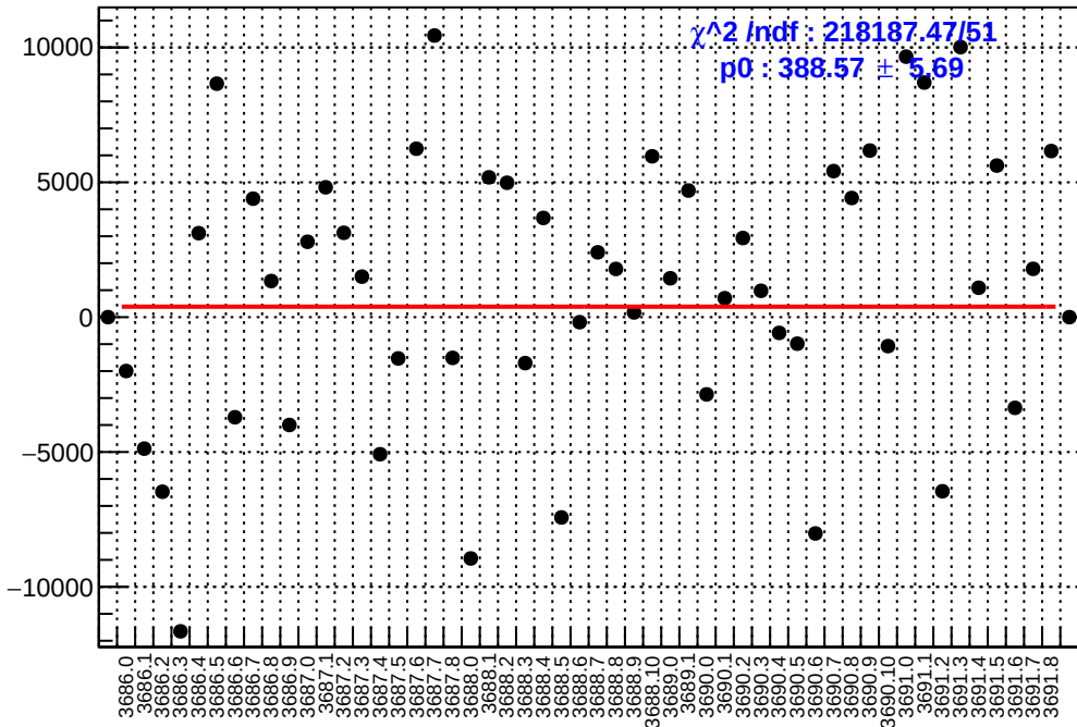
slug17: asym_dsl.mean/ppb-reg_asym_dsl.mean/ppb
