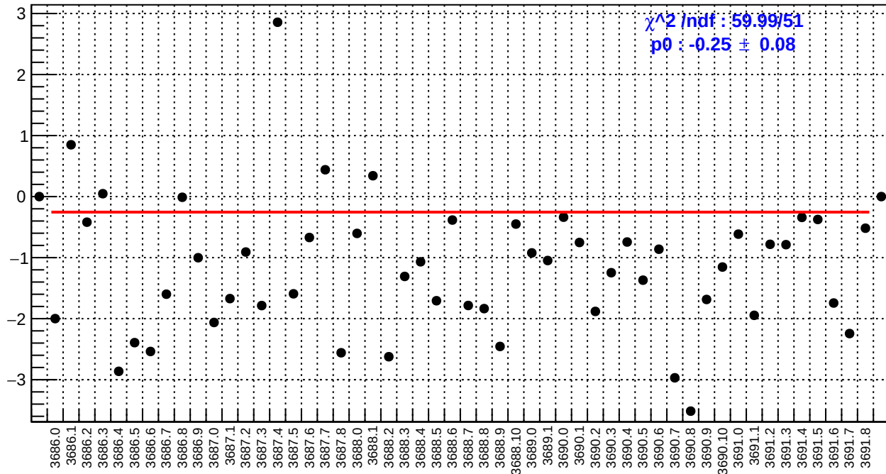
slug17: left_avg_bpm4aY/(ppb/nm)
