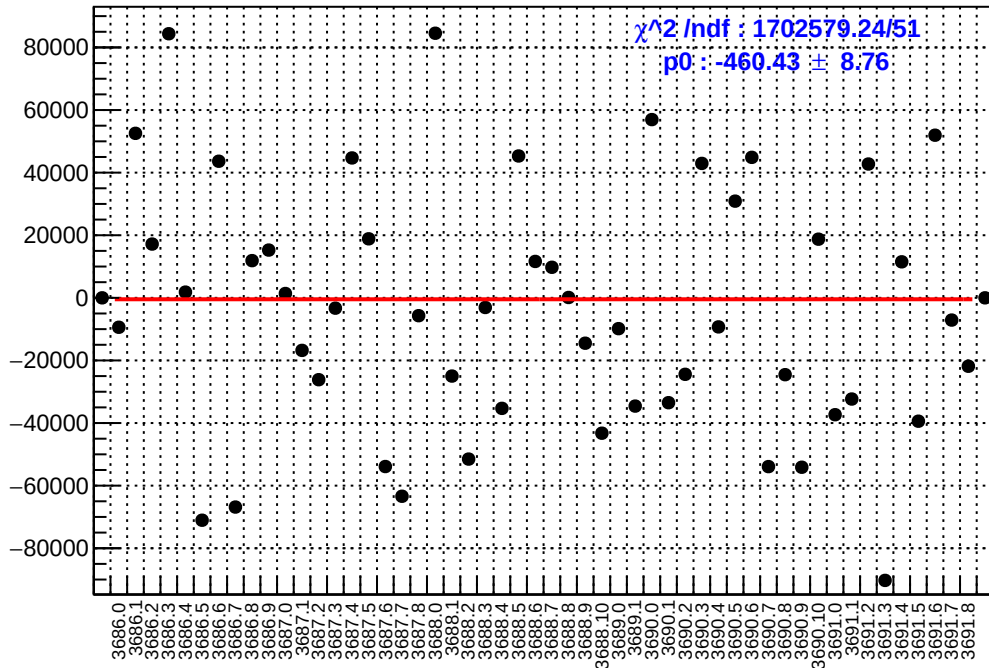
slug17: asym_sam8.mean/ppb-reg_asym_sam8.mean/ppb
