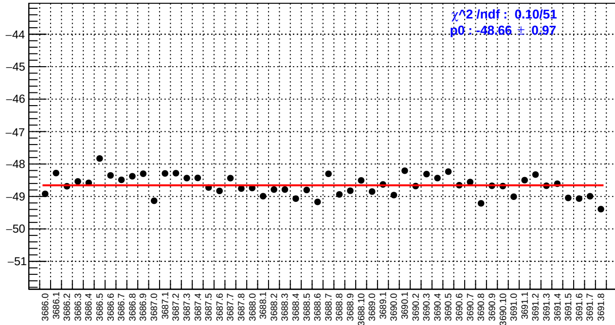
slug17: us_avg_bpm12X/(ppb/nm)
