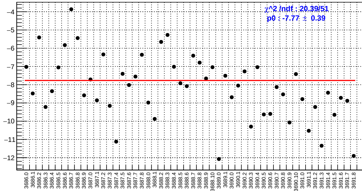
slug17: right_avg_bpm4eY/(ppb/nm)
