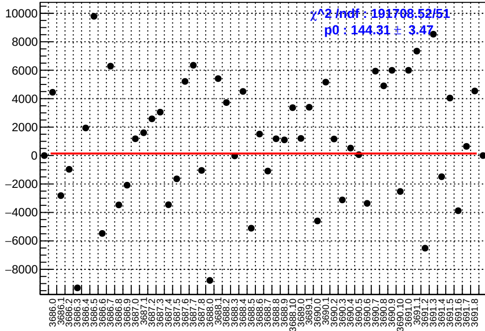
slug17: asym_us_dd.mean/ppb-reg_asym_us_dd.mean/ppb
