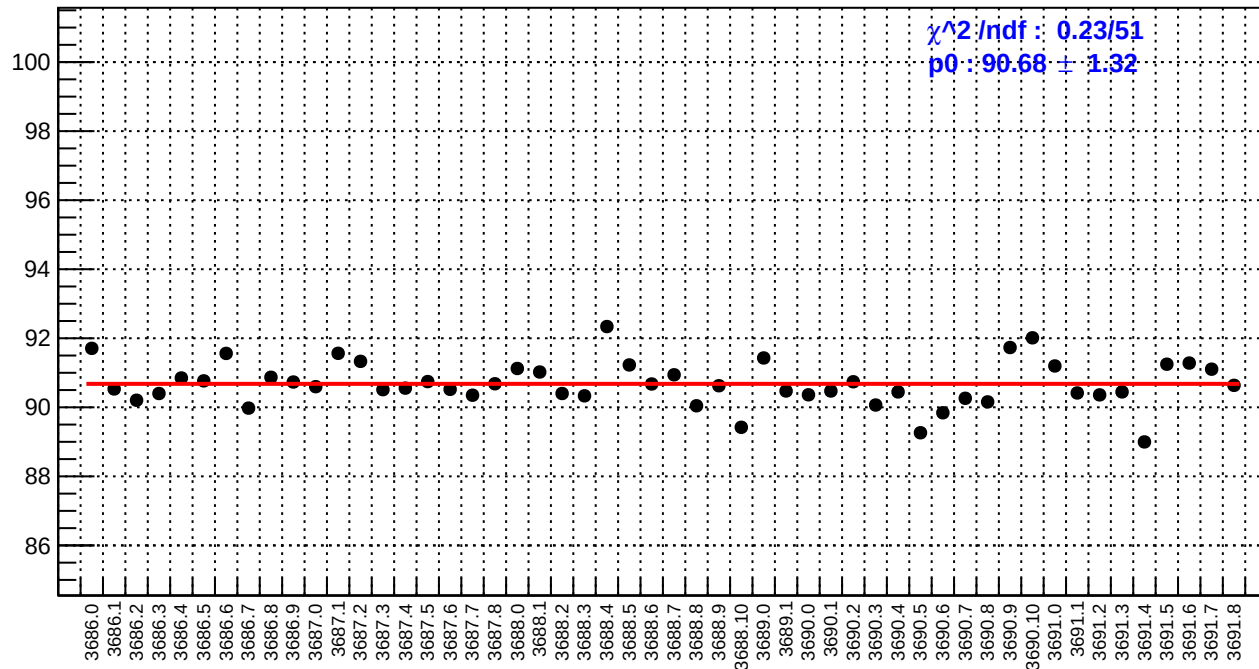
slug17: reg_asym_ds_dd.rms/ppm
