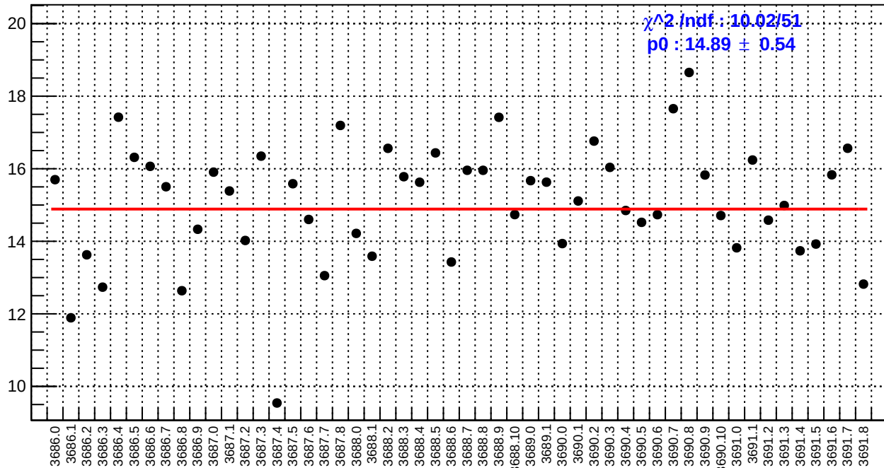
slug17: left_avg_bpm4eY/(ppb/nm)
