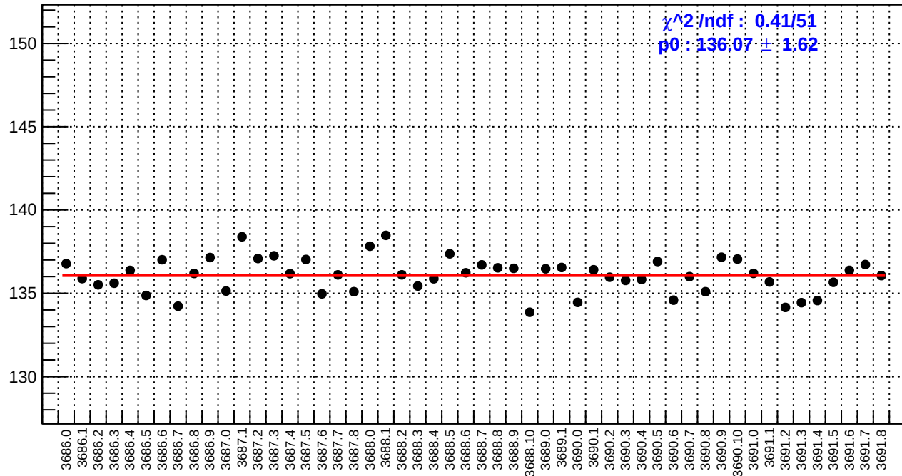
slug17: reg_asym_usr.rms/ppm
