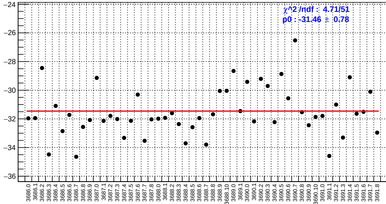
slug17: right_avg_bpm4aX/(ppb/nm)
