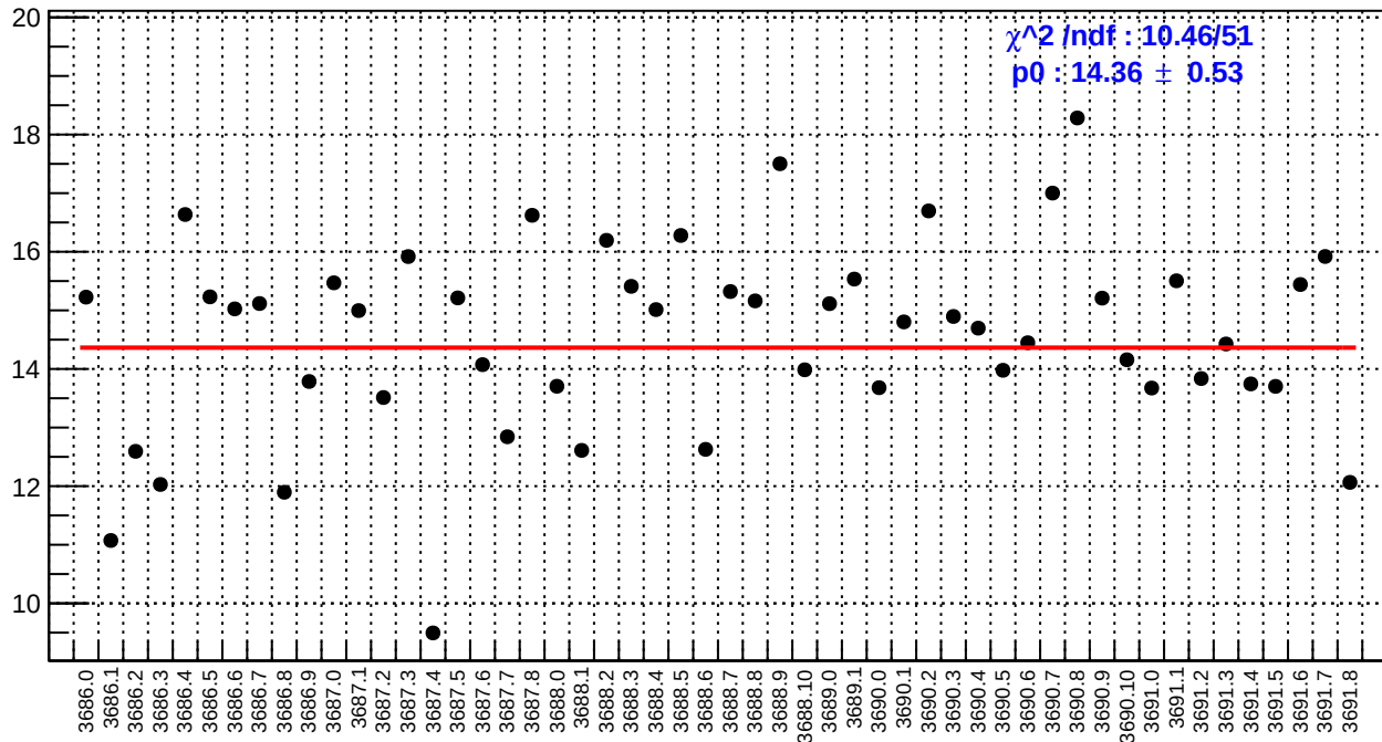
slug17: usl_bpm4eY/(ppb/nm)
