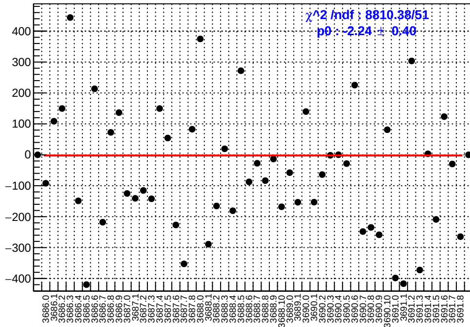
slug17: asym_left_dd.mean/ppb-reg_asym_left_dd.mean/ppb
