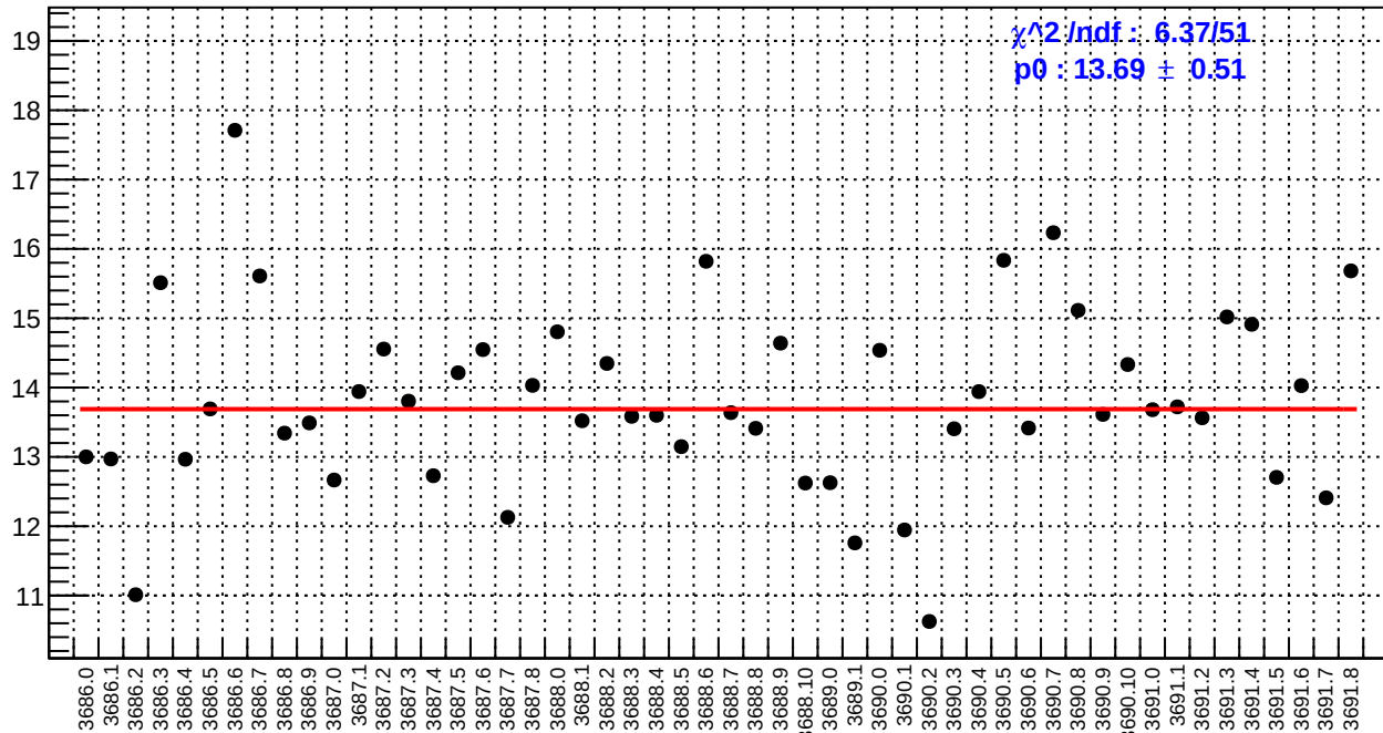
slug17: usl_bpm4aX/(ppb/nm)
