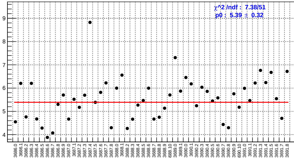
slug17: ds_avg_bpm4aY/(ppb/nm)
