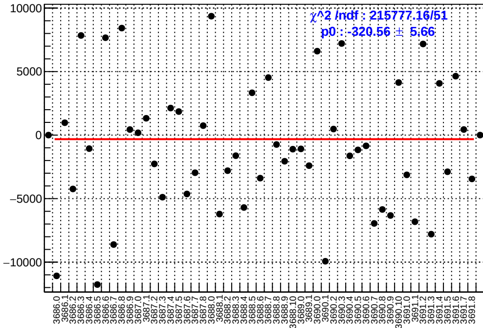
slug17: asym_usr.mean/ppb-reg_asym_usr.mean/ppb
