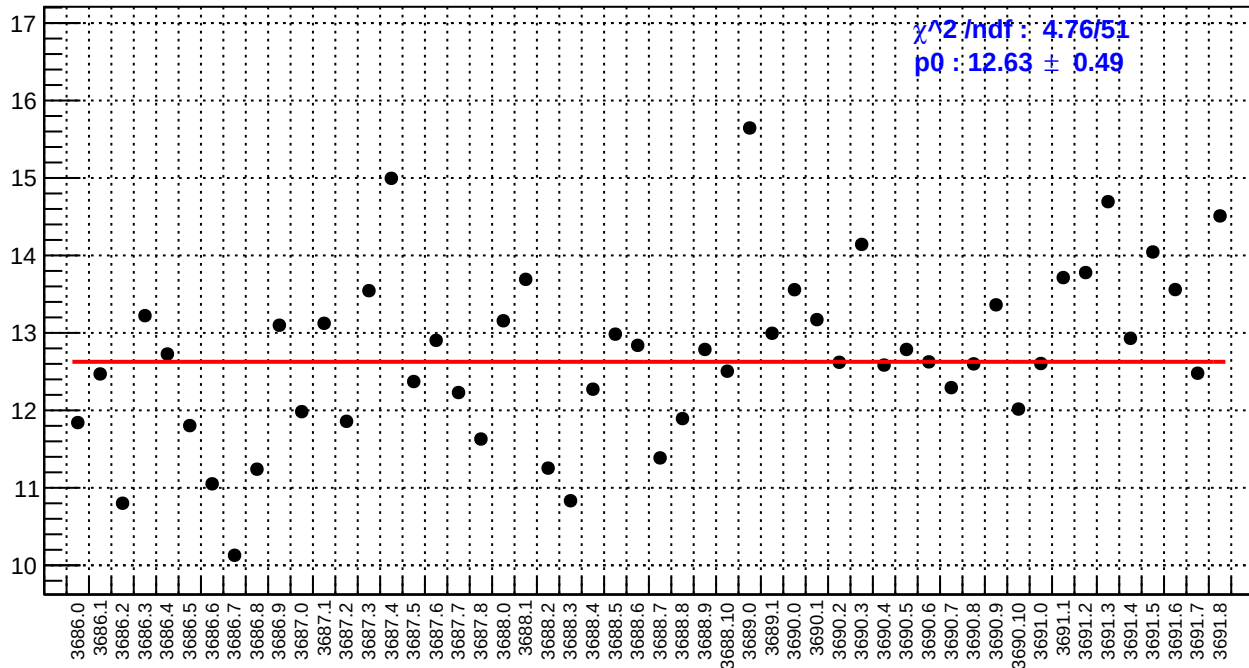
slug17: right_avg_bpm4aY/(ppb/nm)
