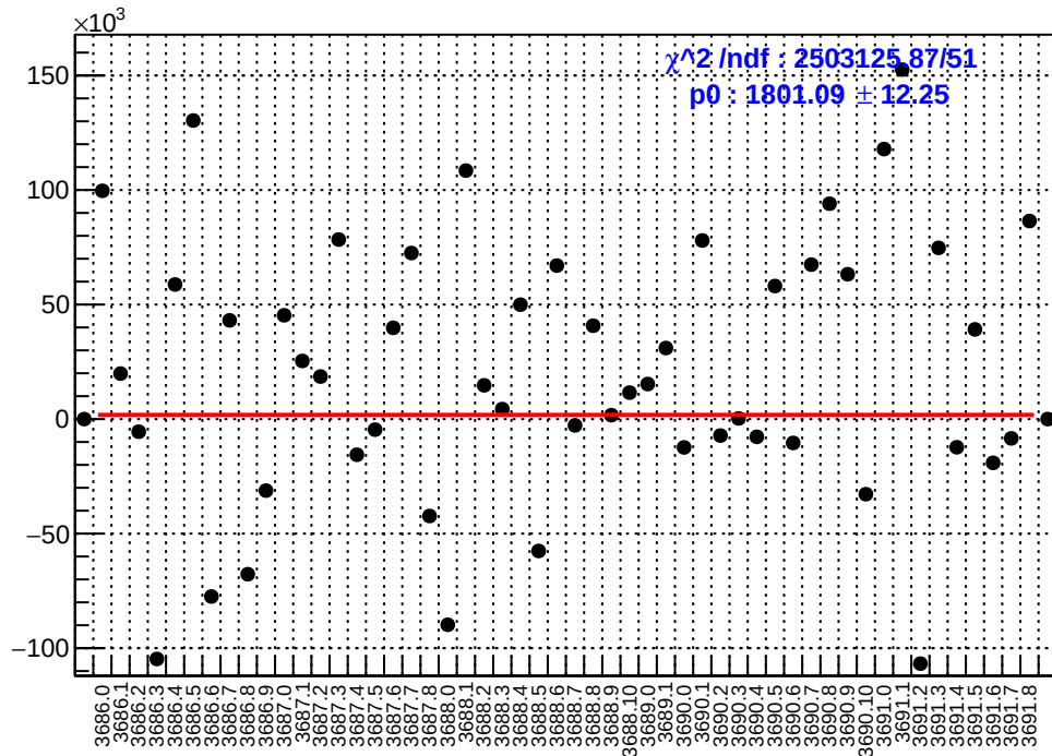
slug17: asym_sam2.mean/ppb-reg_asym_sam2.mean/ppb
