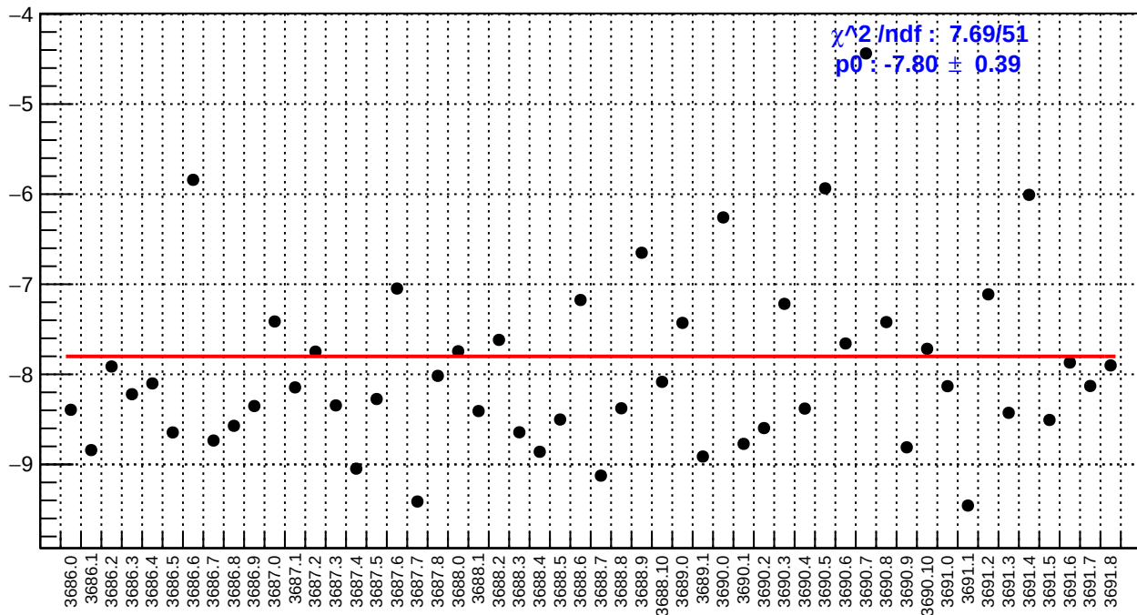
slug17: ds_avg_bpm4aX/(ppb/nm)
