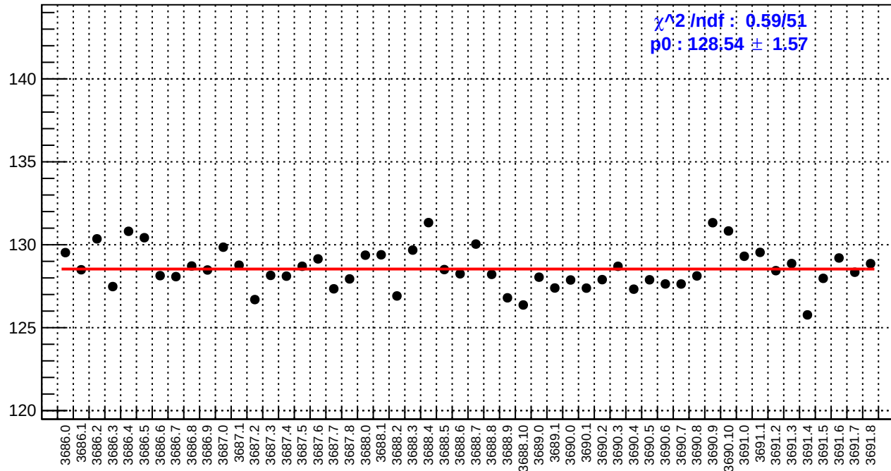
slug17: reg_asym_left_avg.rms/ppm
