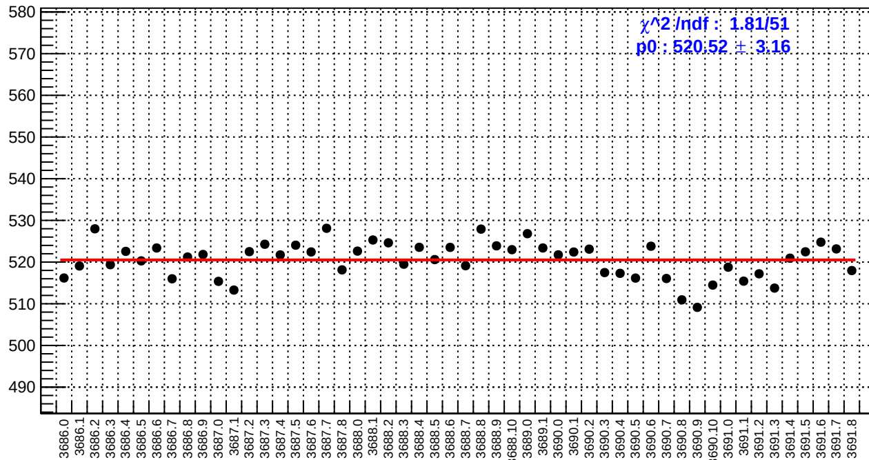
slug17: asym_bcm_an_ds.rms/ppm
