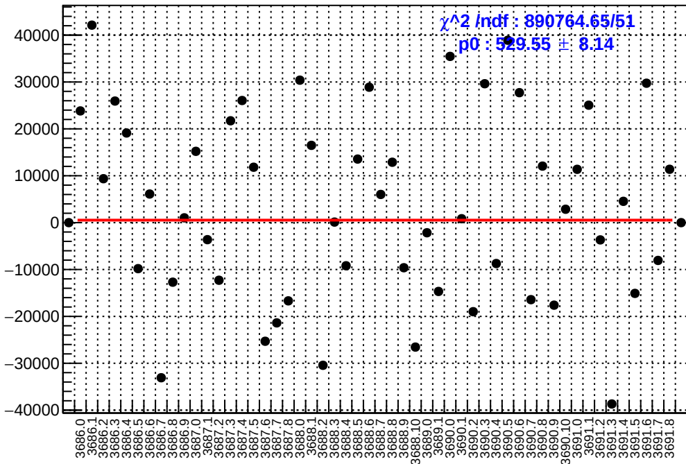
slug17: asym_sam1.mean/ppb-reg_asym_sam1.mean/ppb
