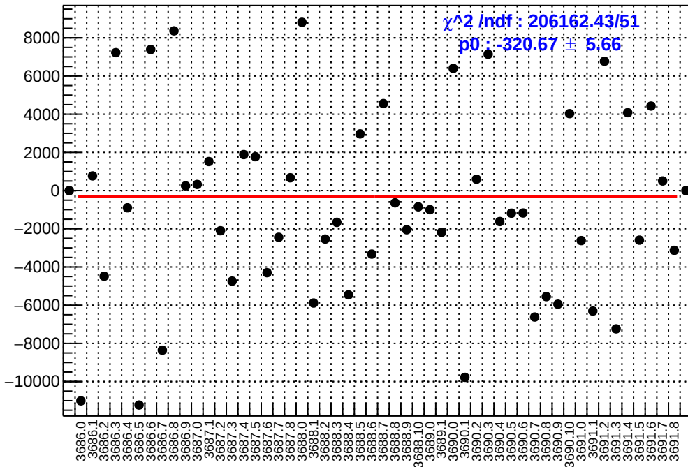
slug17: asym_dsr.mean/ppb-reg_asym_dsr.mean/ppb
