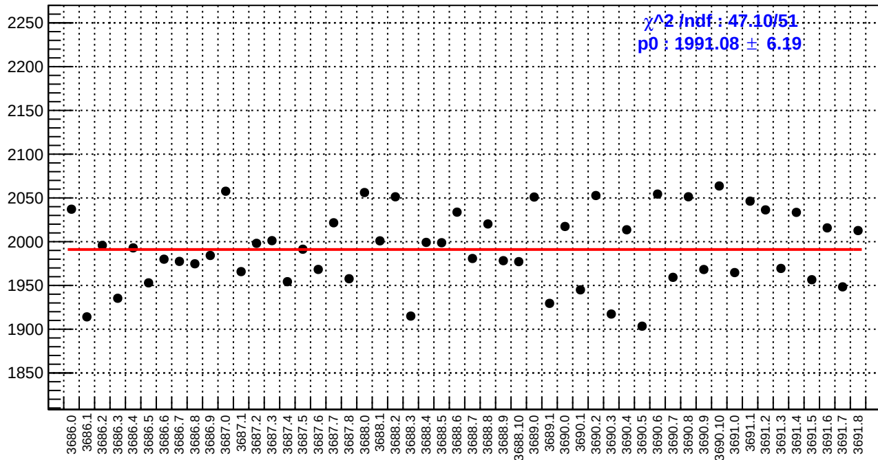
slug17: diff_bpm4aX.rms/nm
