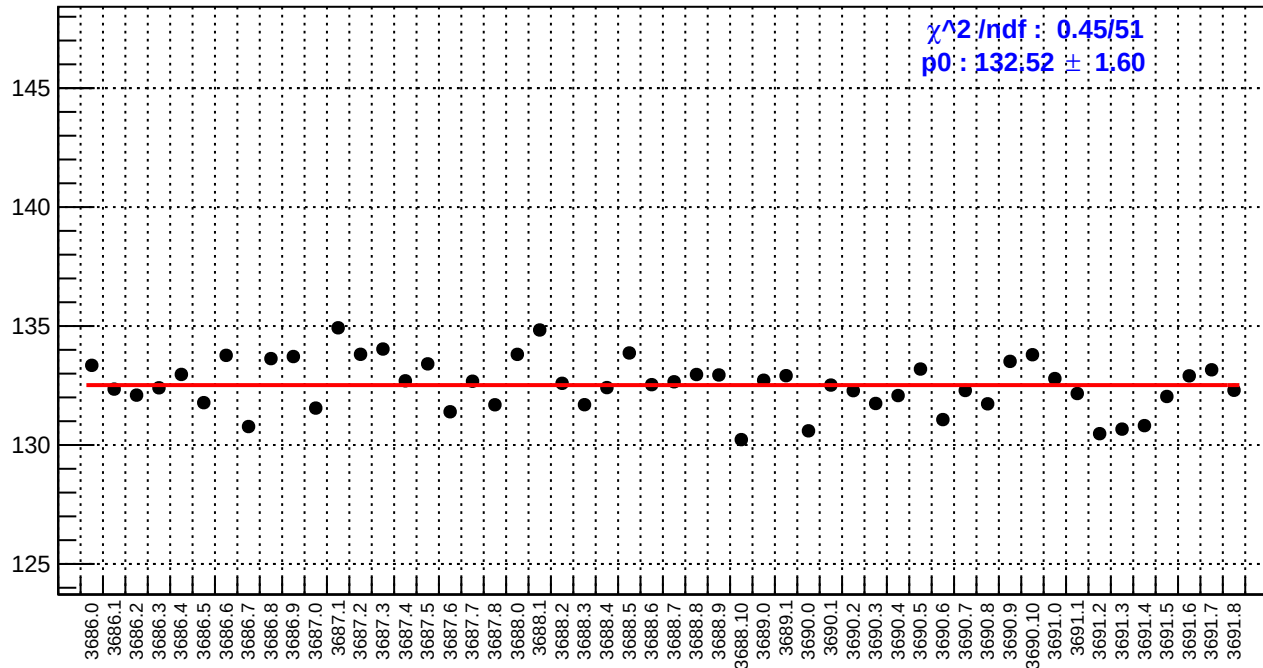
slug17: reg_asym_right_avg.rms/ppm
