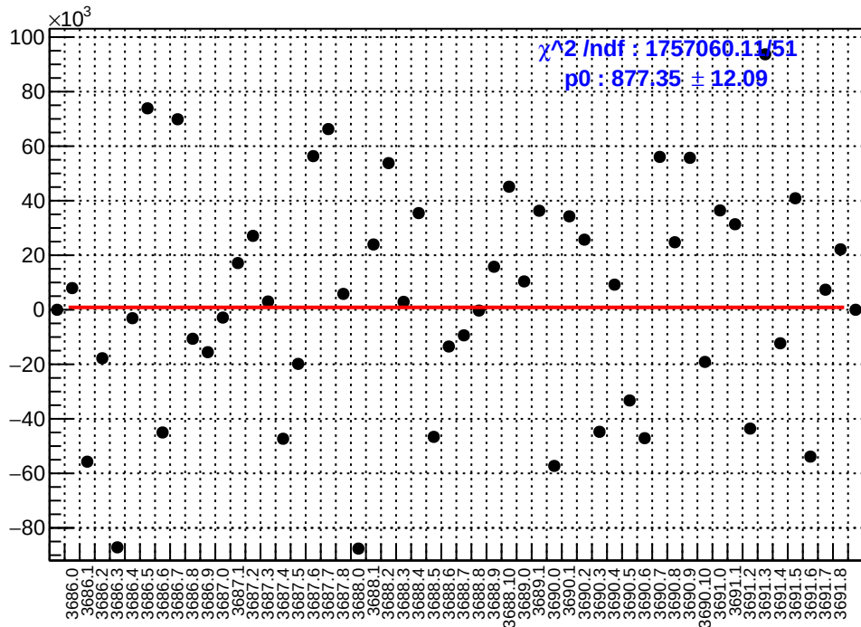
slug17: asym_sam4.mean/ppb-reg_asym_sam4.mean/ppb
