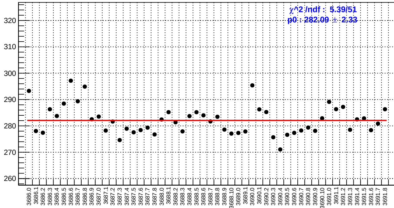
slug17: reg_asym_sam5.rms/ppm
