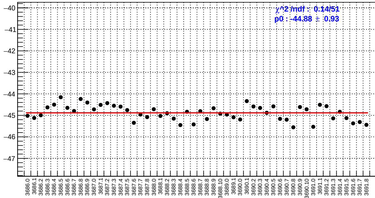
slug17: left_avg_bpm12X/(ppb/nm)
