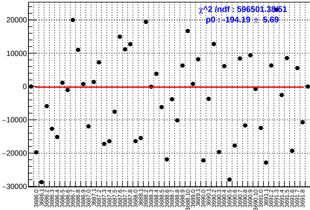
slug17: asym_sam5.mean/ppb-reg_asym_sam5.mean/ppb
