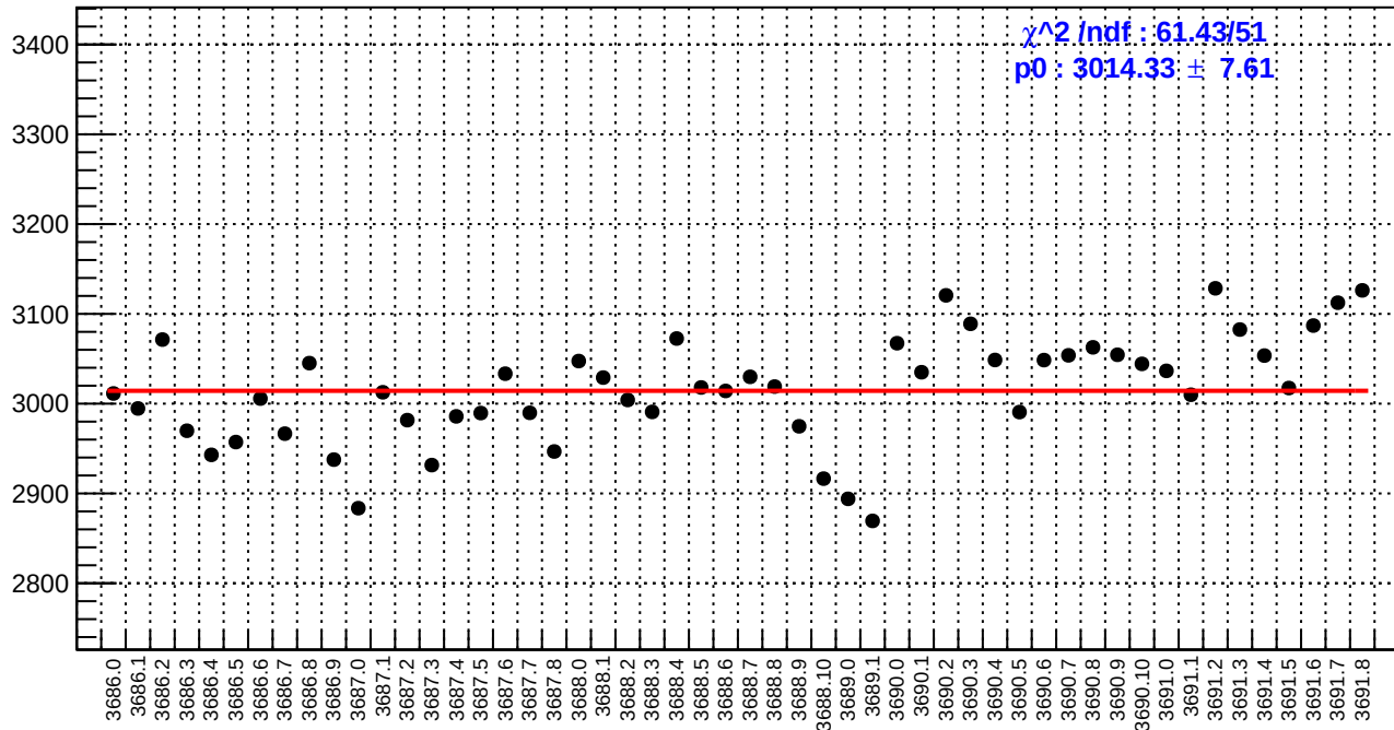
slug17: asym_bcm_an_us.rms/ppm
