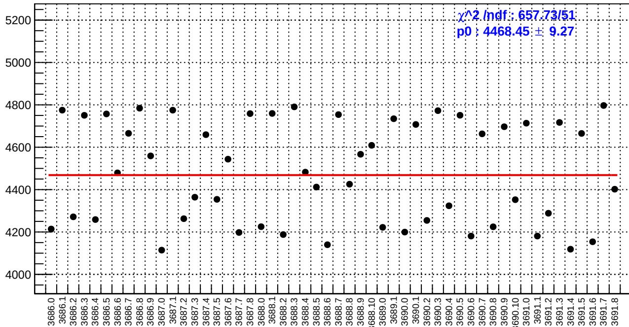
slug17: diff_bpm4eY.rms/nm
