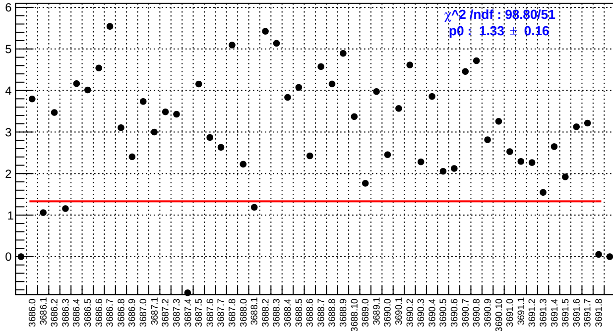
slug17: us_avg_bpm4eY/(ppb/nm)
