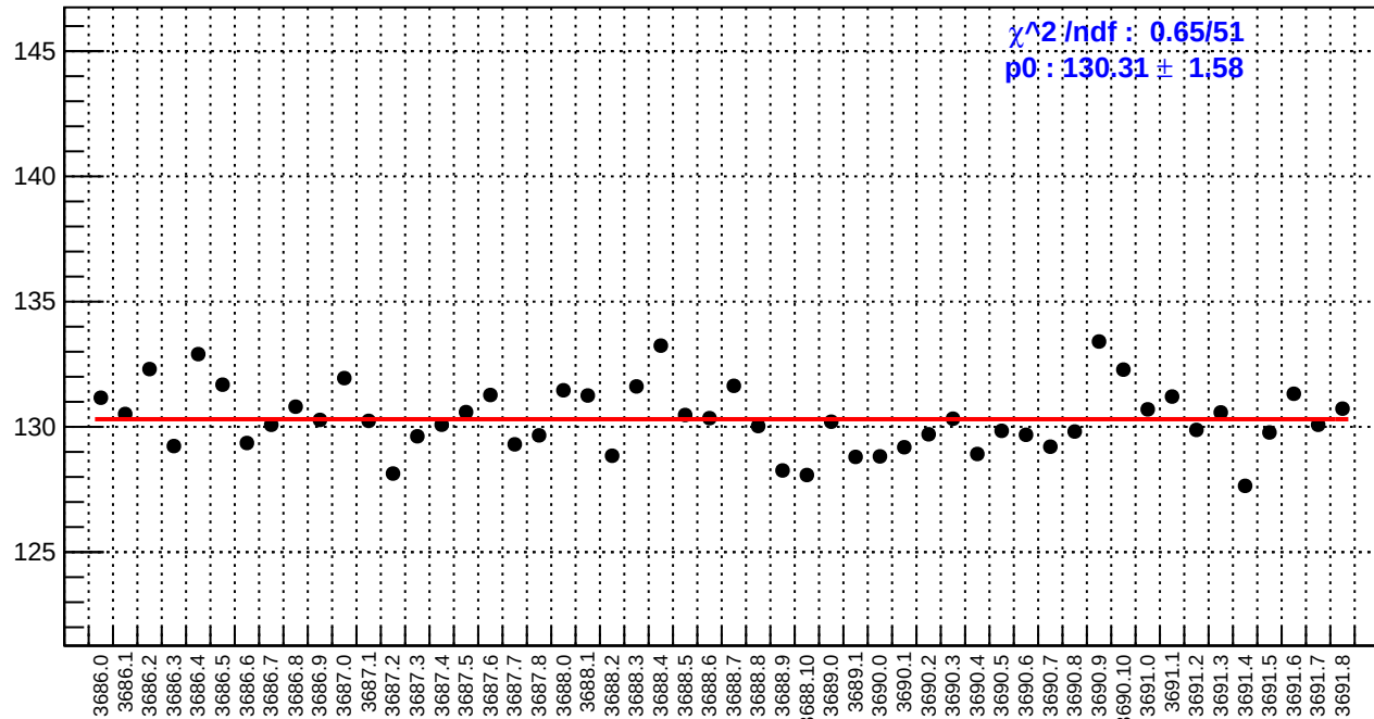
slug17: reg_asym_usl.rms/ppm
