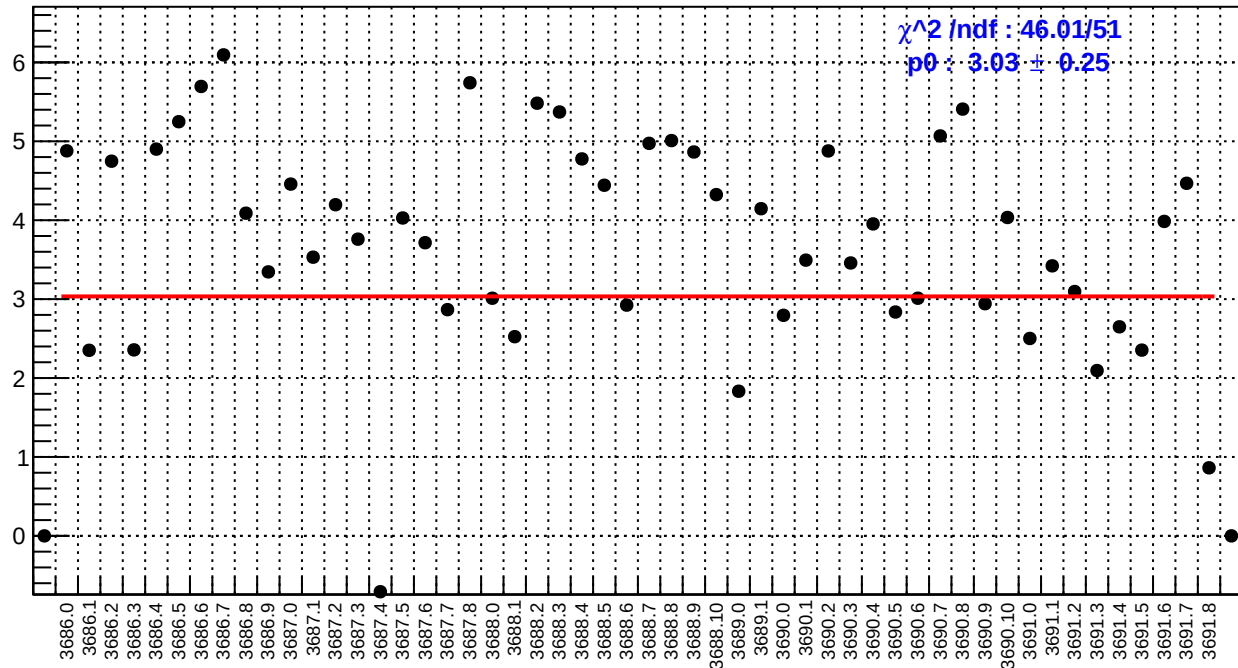
slug17: ds_avg_bpm4eY/(ppb/nm)
