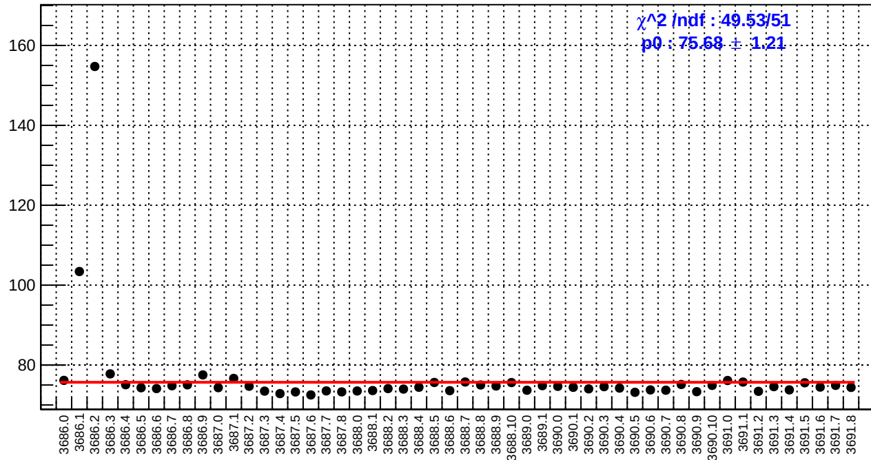
slug17: asym_bcm_an_ds3.rms/ppm
