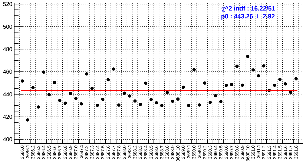
slug17: reg_asym_sam3.rms/ppm
