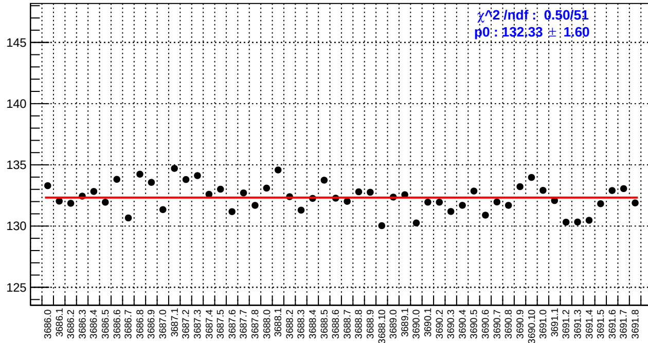
slug17: reg_asym_dsr.rms/ppm
