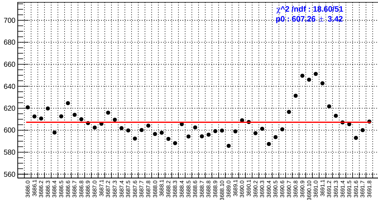
slug17: reg_asym_sam6.rms/ppm
