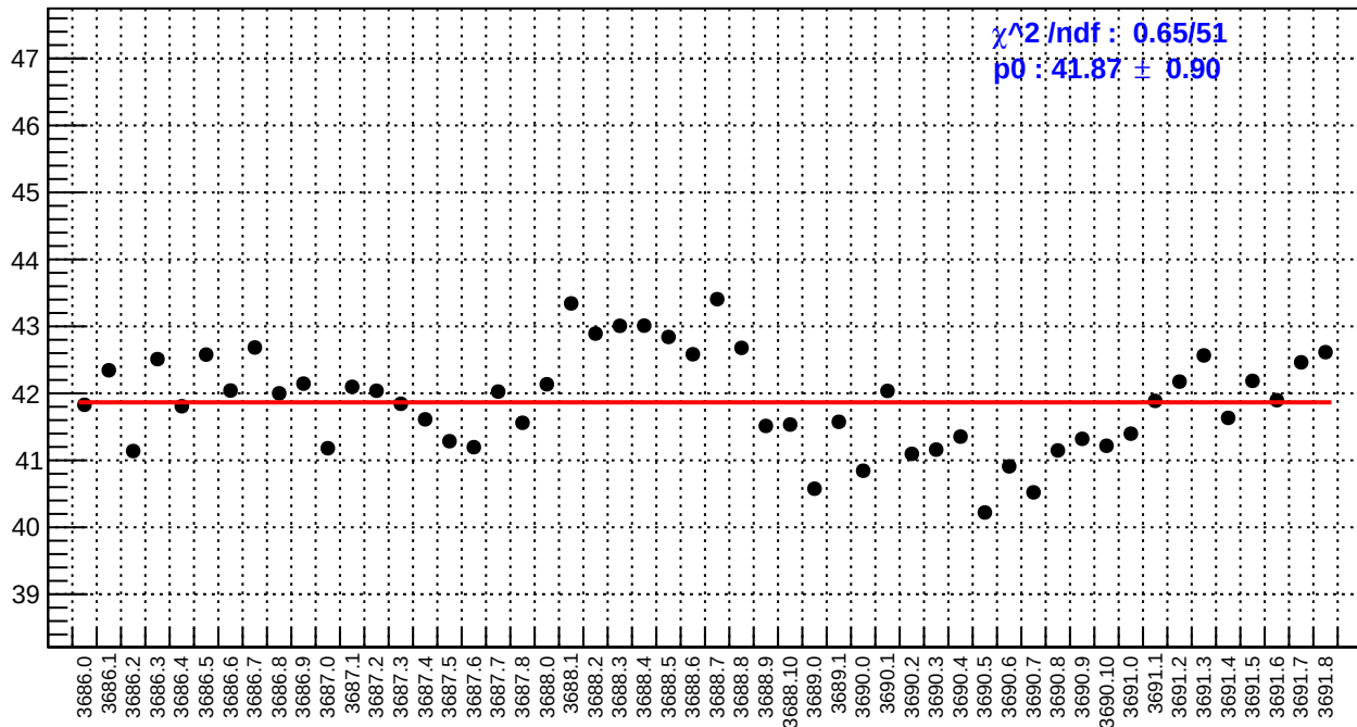
slug17: right_avg_bpm4eX/(ppb/nm)
