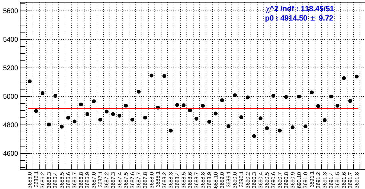
slug17: diff_bpm11X.rms/nm
