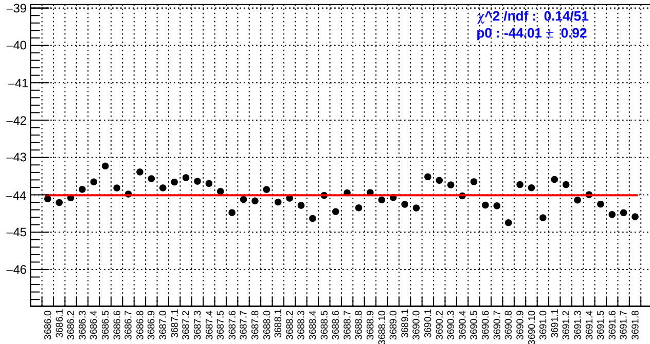
slug17: usl_bpm12X/(ppb/nm)
