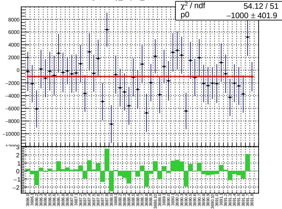
slug17: reg_asym_sam5.mean/ppb
