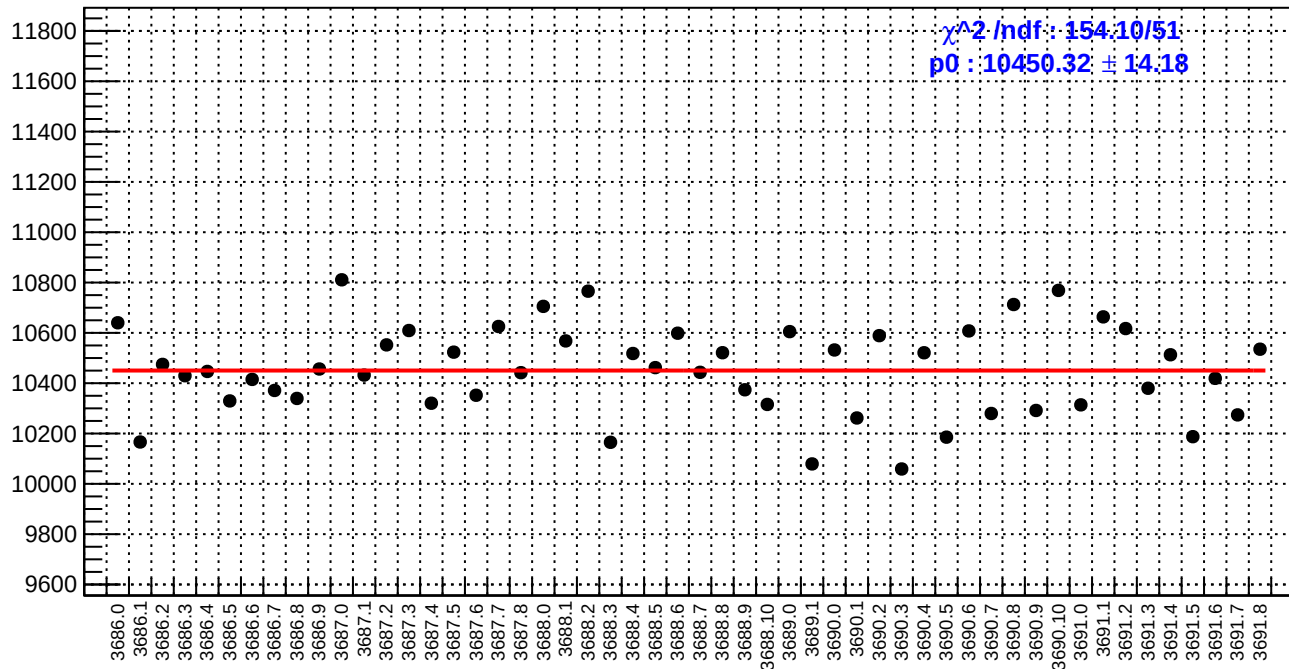
slug17: diff_bpm4eX.rms/nm
