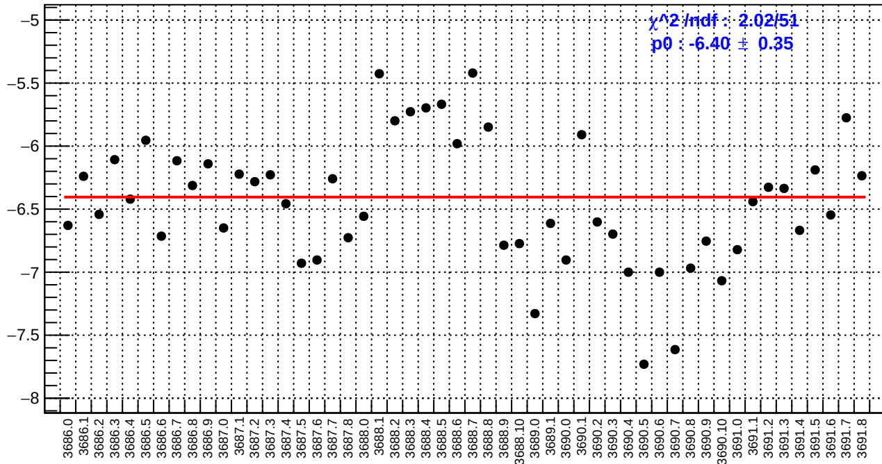
slug17: us_avg_bpm4eX/(ppb/nm)
