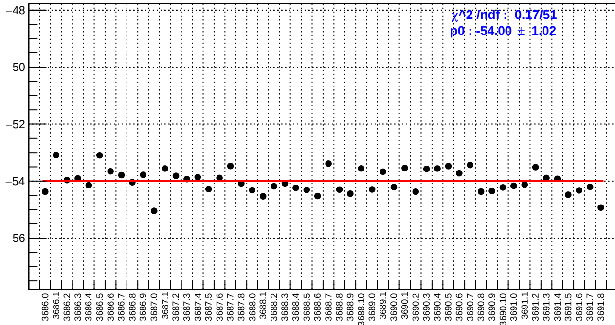
slug17: right_avg_bpm12X/(ppb/nm)
