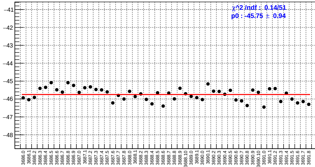
slug17: dsl_bpm12X/(ppb/nm)
