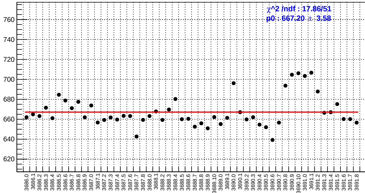
slug17: reg_asym_sam8.rms/ppm
