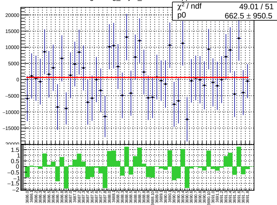
slug17: reg_asym_sam8.mean/ppb
