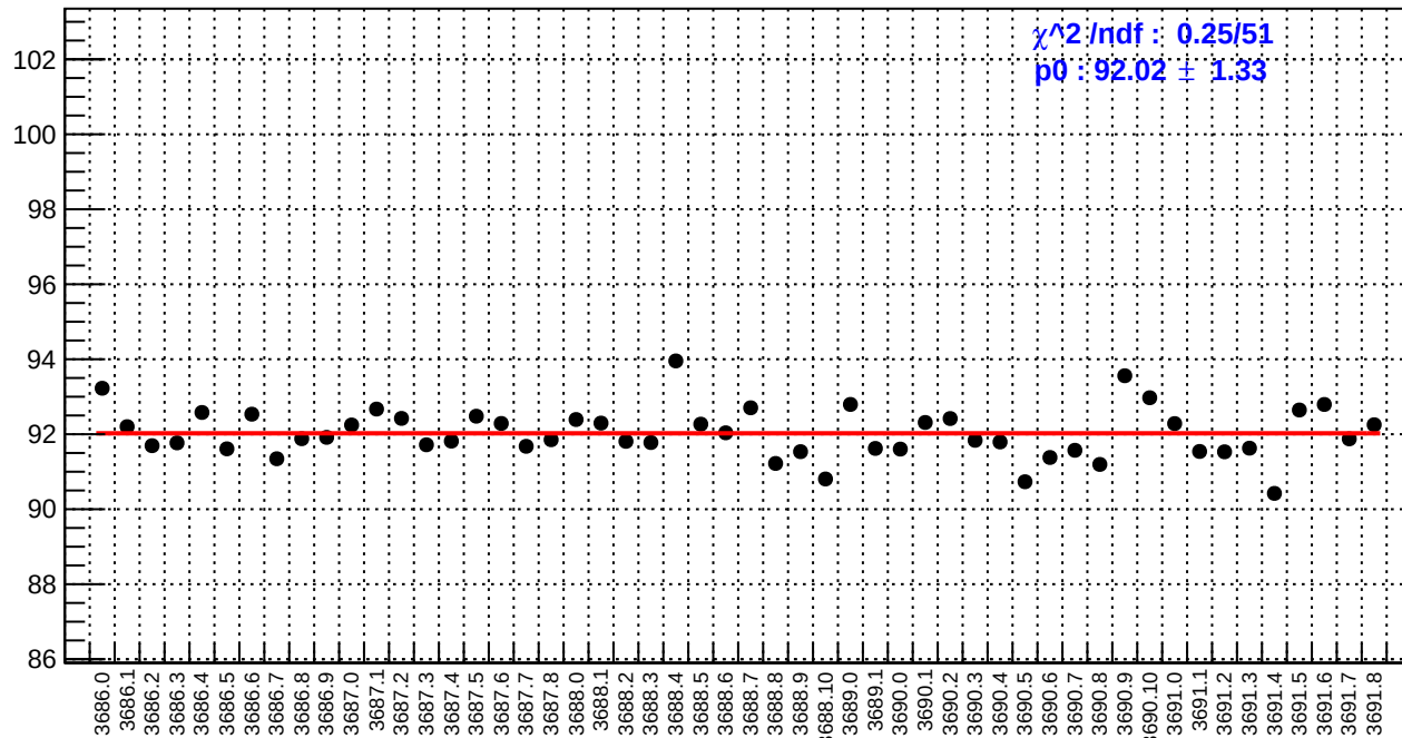
slug17: reg_asym_us_dd.rms/ppm
