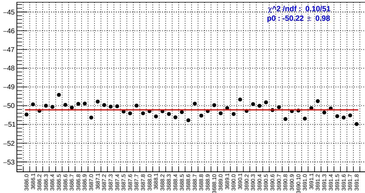
slug17: ds_avg_bpm12X/(ppb/nm)
