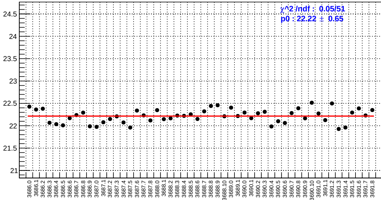
slug17: reg_asym_left_dd.rms/ppm
