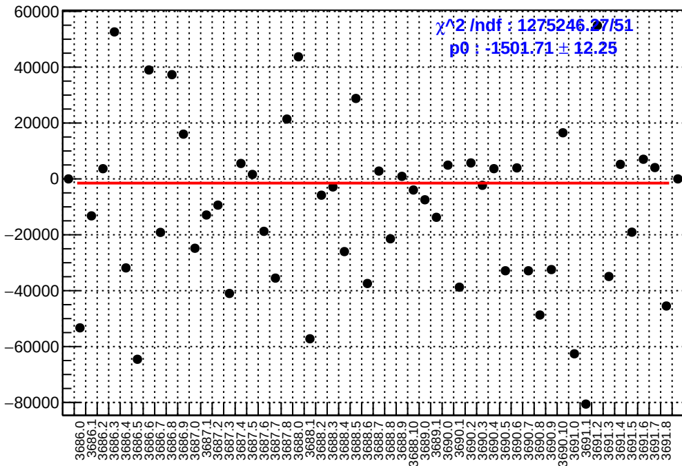
slug17: asym_sam6.mean/ppb-reg_asym_sam6.mean/ppb
