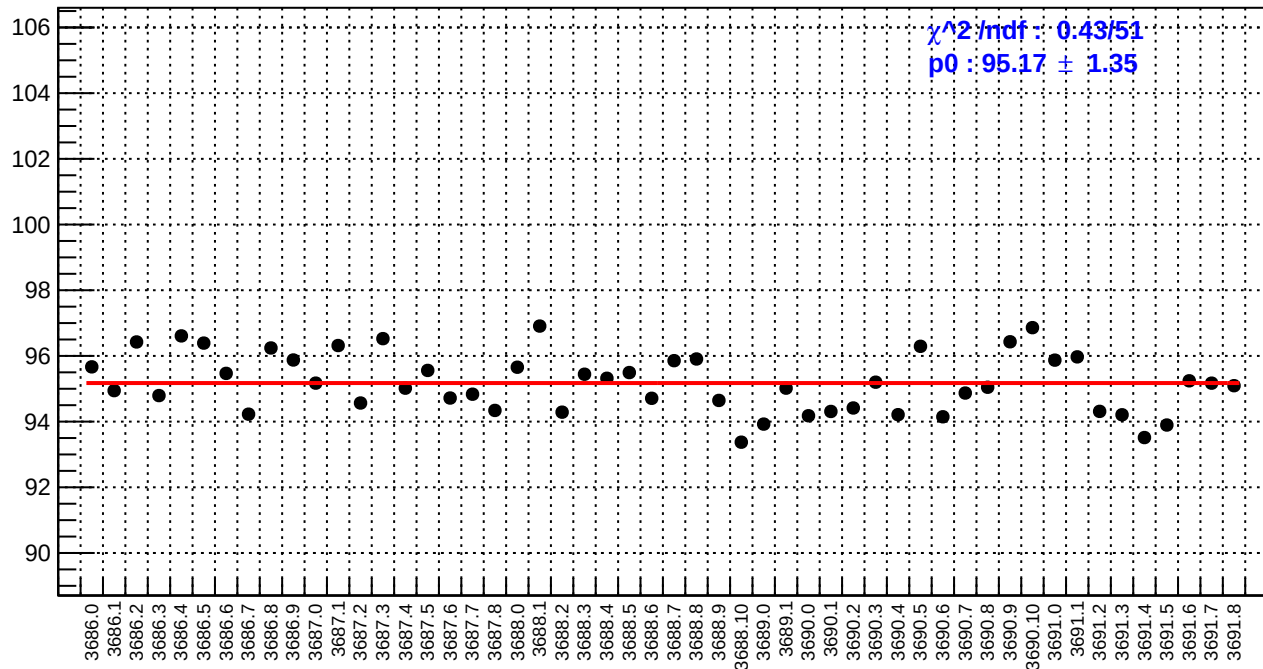
slug17: reg_asym_ds_avg.rms/ppm
