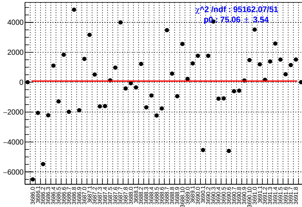
slug17: asym_ds_avg.mean/ppb-reg_asym_ds_avg.mean/ppb
