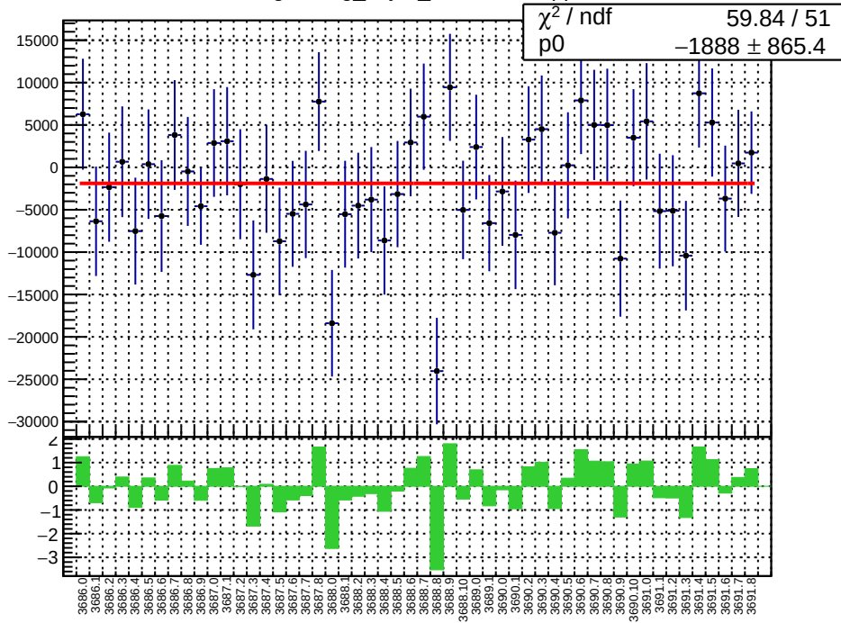
slug17: reg_asym_sam6.mean/ppb
