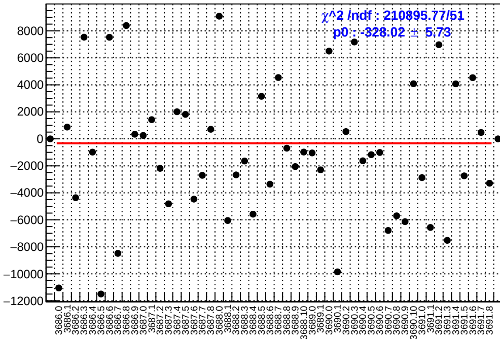
slug17: asym_right_avg.mean/ppb-reg_asym_right_avg.mean/ppb
