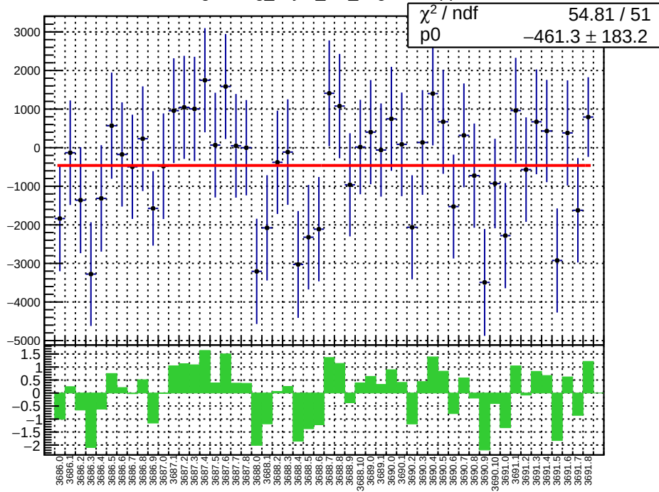
slug17: reg_asym_left_avg.mean/ppb
