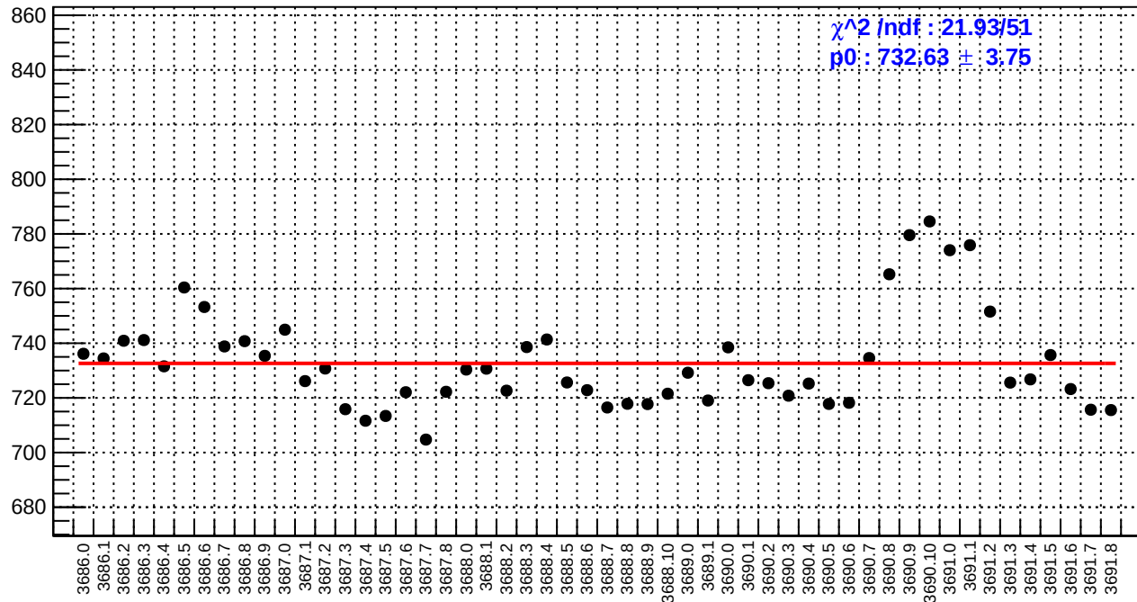
slug17: reg_asym_sam4.rms/ppm
