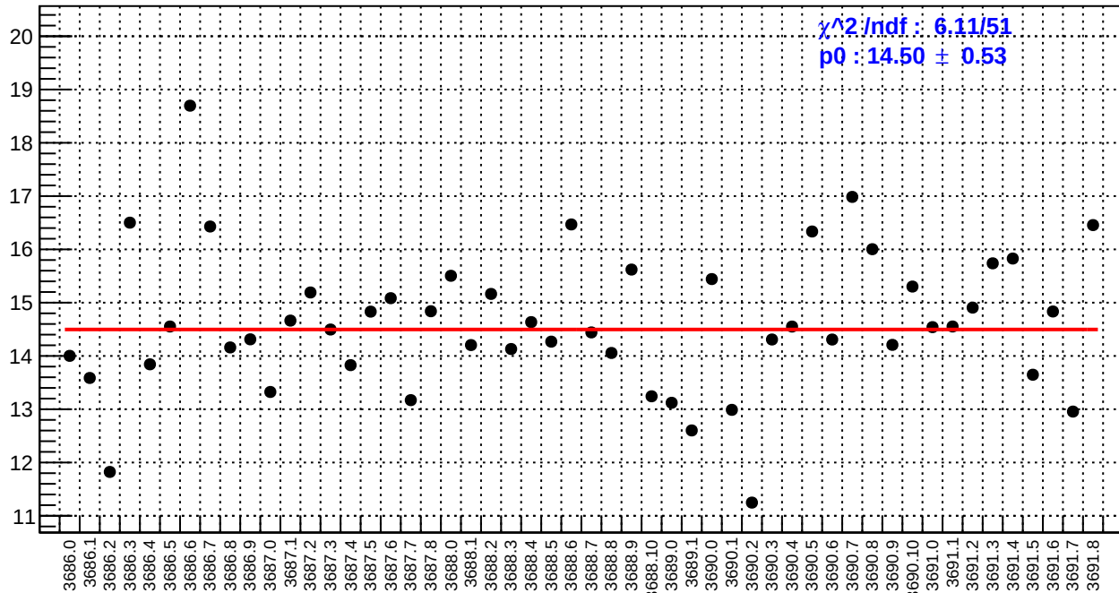
slug17: left_avg_bpm4aX/(ppb/nm)
