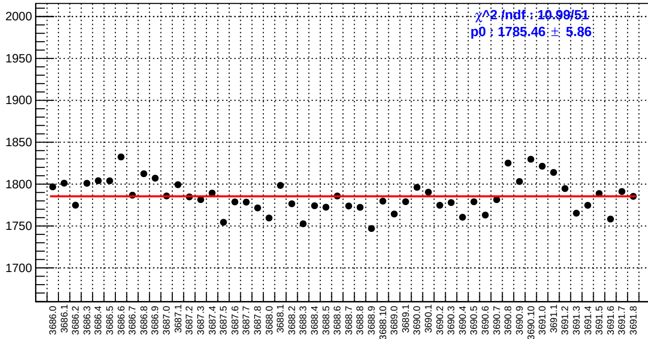
slug17: reg_asym_sam2.rms/ppm
