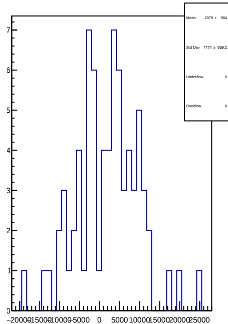
slug18: 1D Corr asym_usl.mean/ppb-reg_asym_usl.mean/ppb
