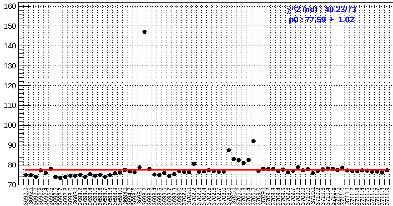
slug18: asym_bcm_an_ds3.rms/ppm
