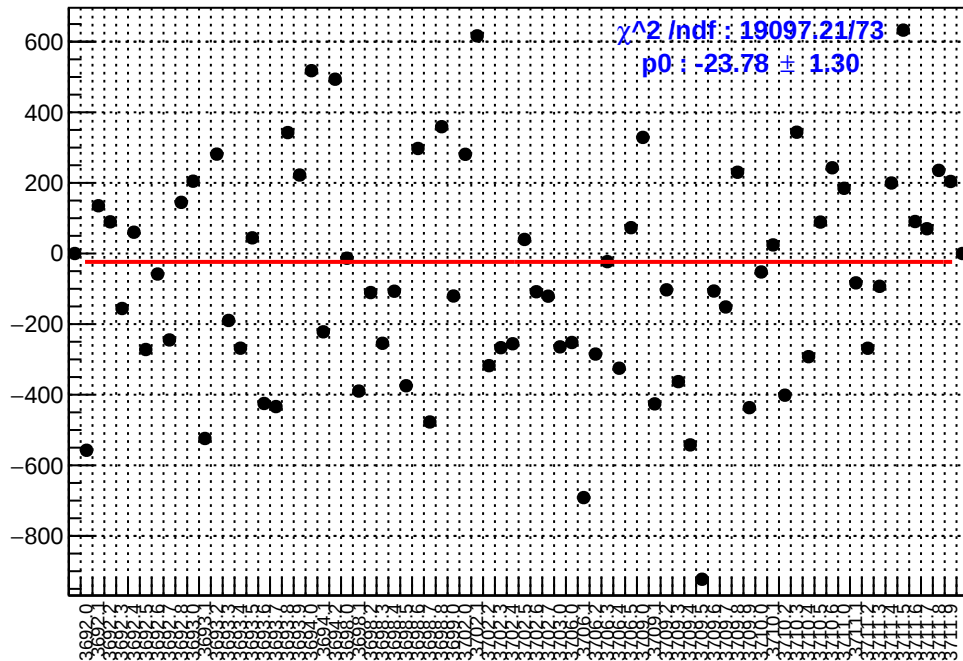
slug18: asym_left_dd.mean/ppb-reg_asym_left_dd.mean/ppb
