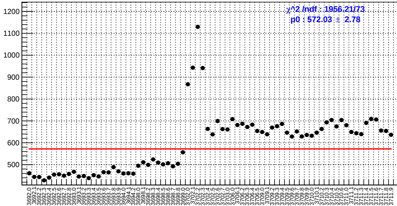
slug18: reg_asym_sam3.rms/ppm
