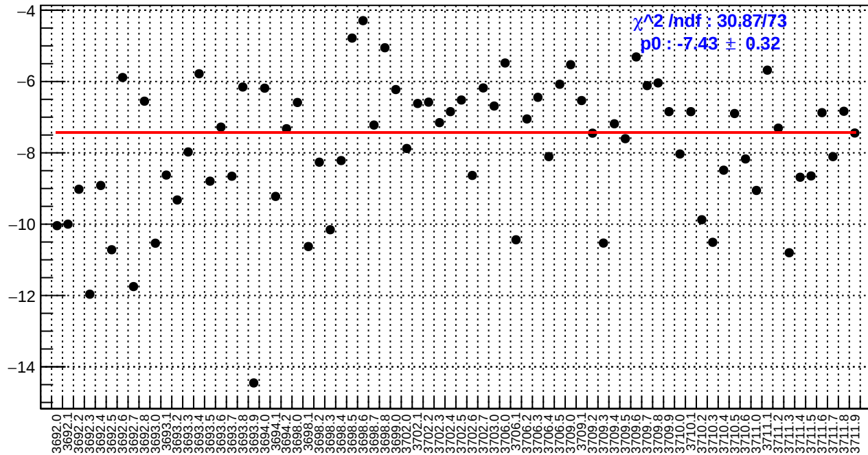
slug18: dsr_bpm4eY/(ppb/nm)
