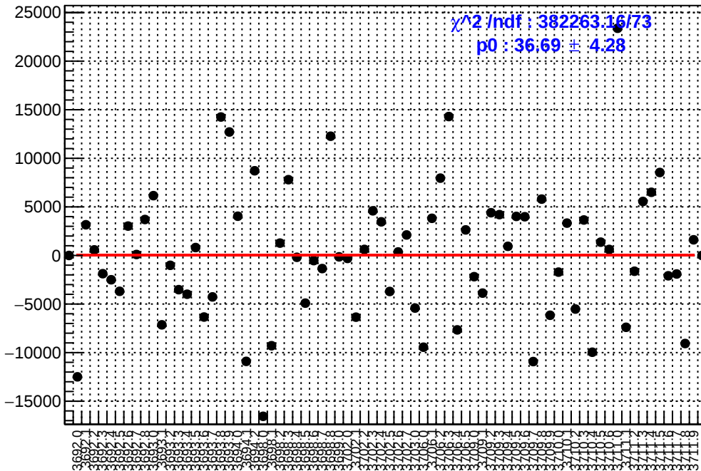
slug18: asym_right_avg.mean/ppb-reg_asym_right_avg.mean/ppb
