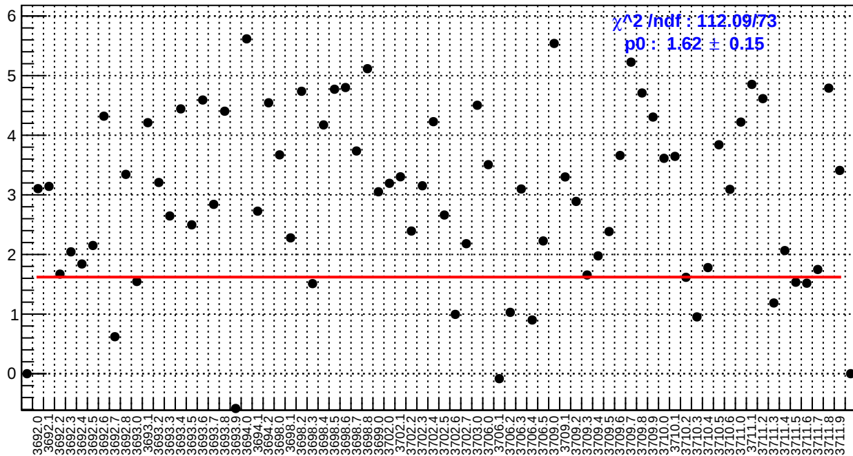
slug18: ds_avg_bpm4eY/(ppb/nm)
