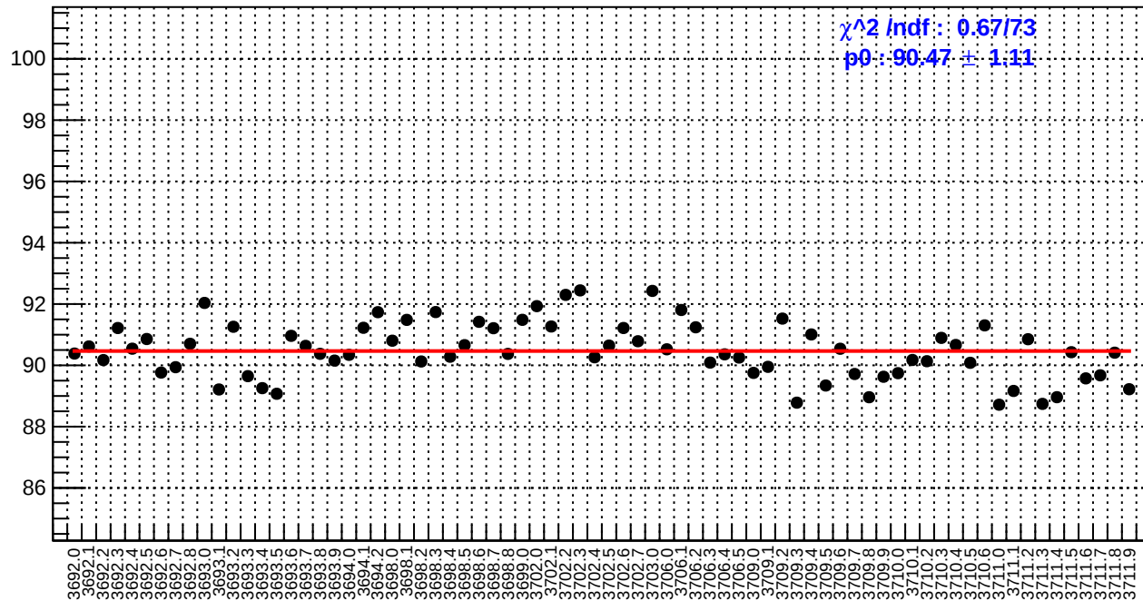
slug18: reg_asym_ds_dd.rms/ppm
