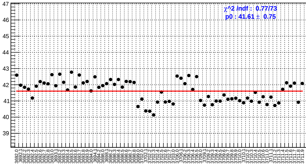
slug18: right_avg_bpm4eX/(ppb/nm)
