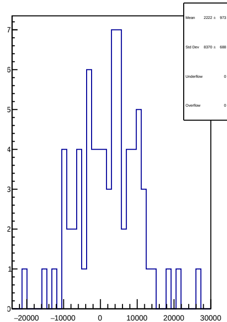
slug18: 1D Corr asym_dsl.mean/ppb-reg_asym_dsl.mean/ppb
