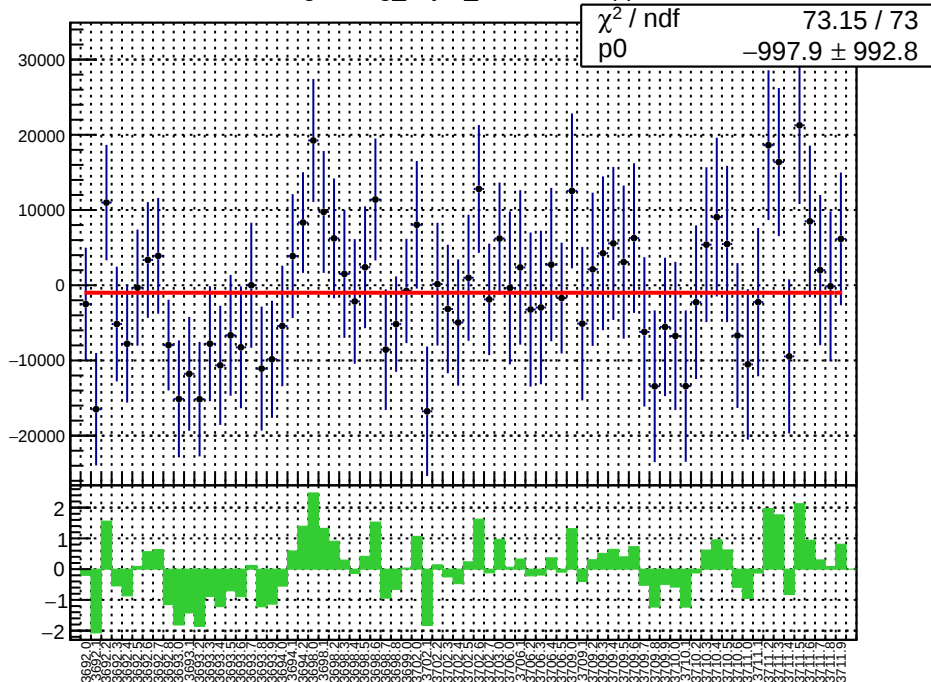
slug18: reg_asym_sam4.mean/ppb
