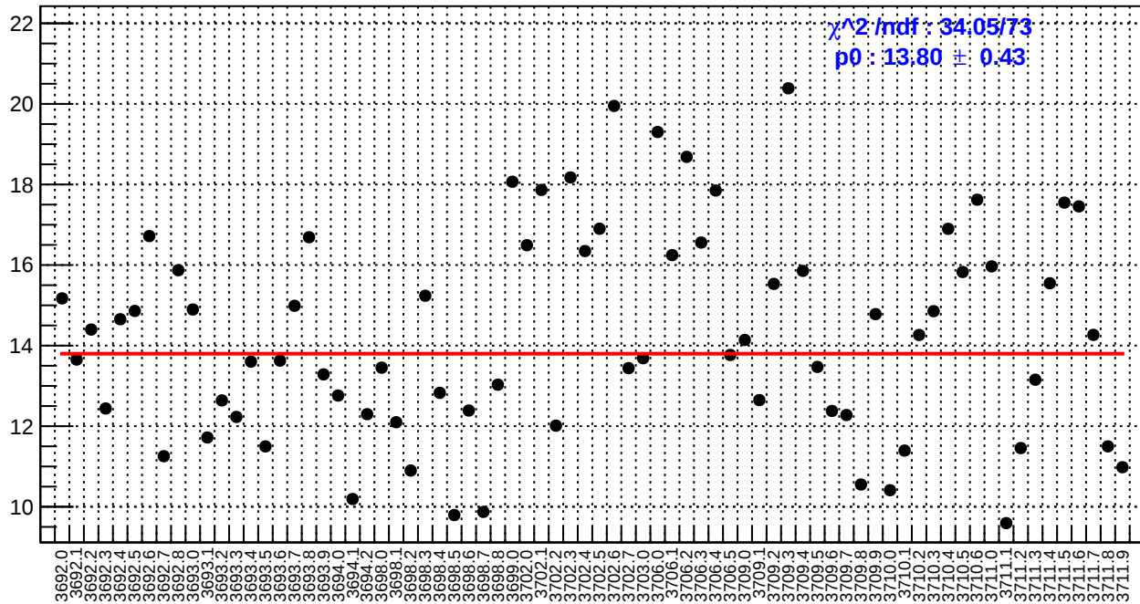
slug18: usl_bpm4aX/(ppb/nm)
