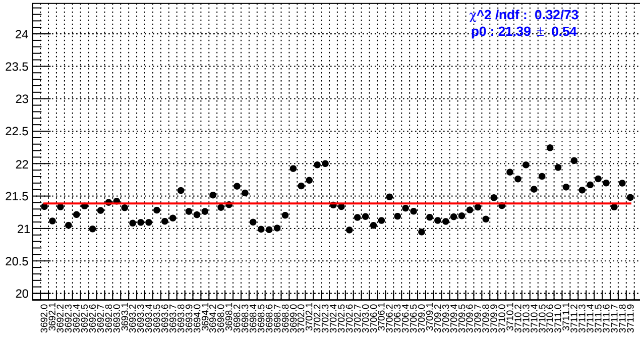
slug18: reg_asym_right_dd.rms/ppm
