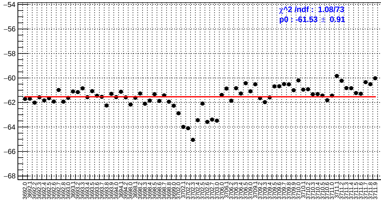
slug18: dsl_bpm4eX/(ppb/nm)
