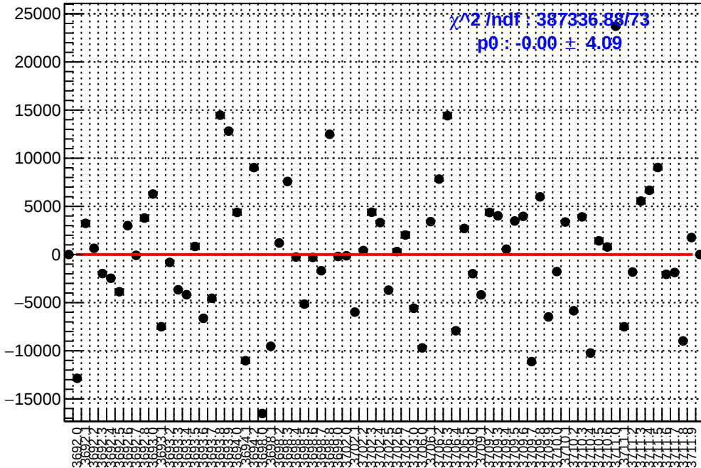
slug18: asym_usr.mean/ppb-reg_asym_usr.mean/ppb
