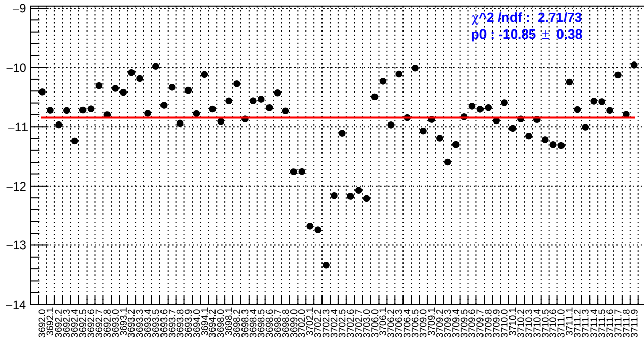
slug18: ds_avg_bpm4eX/(ppb/nm)
