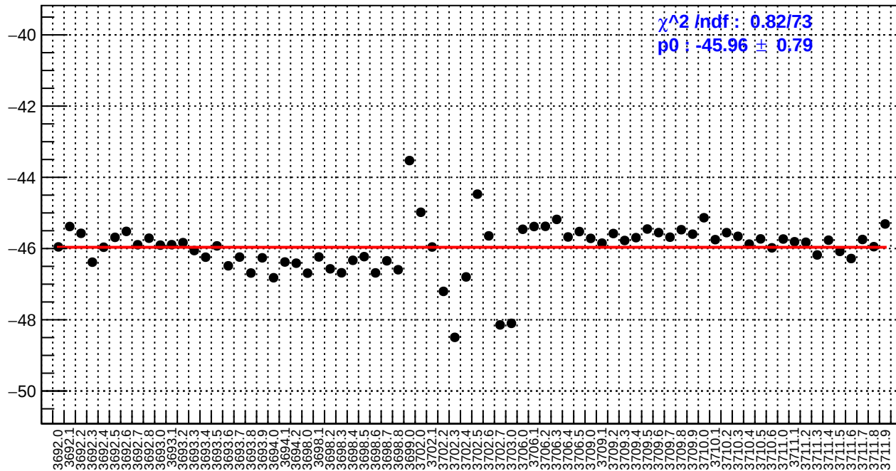
slug18: left_avg_bpm12X/(ppb/nm)
