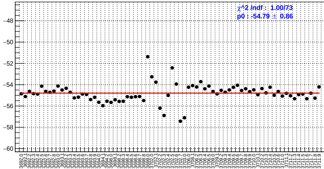
slug18: right_avg_bpm12X/(ppb/nm)
