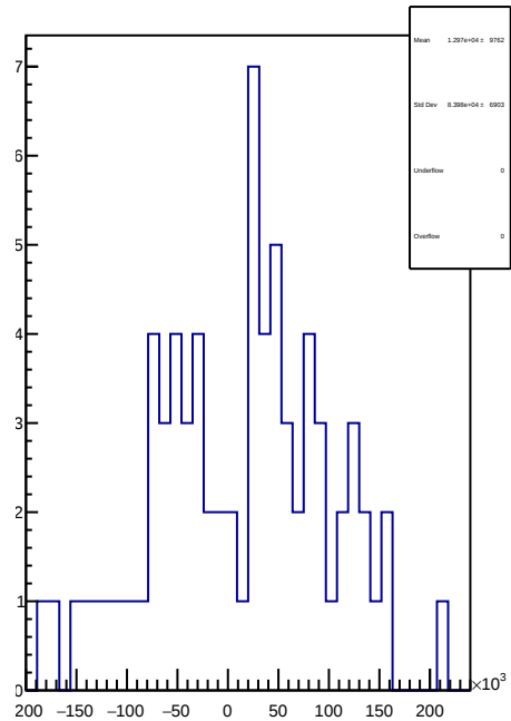
slug18: 1D Corr asym_sam2.mean/ppb-reg_asym_sam2.mean/ppb
