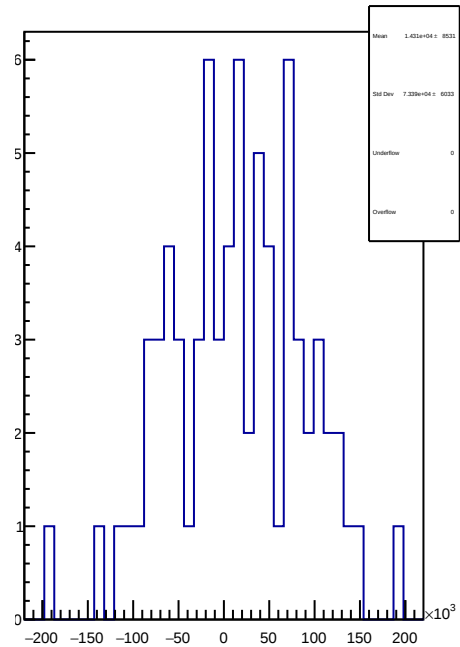
slug18: 1D Corr asym_sam3.mean/ppb-reg_asym_sam3.mean/ppb
