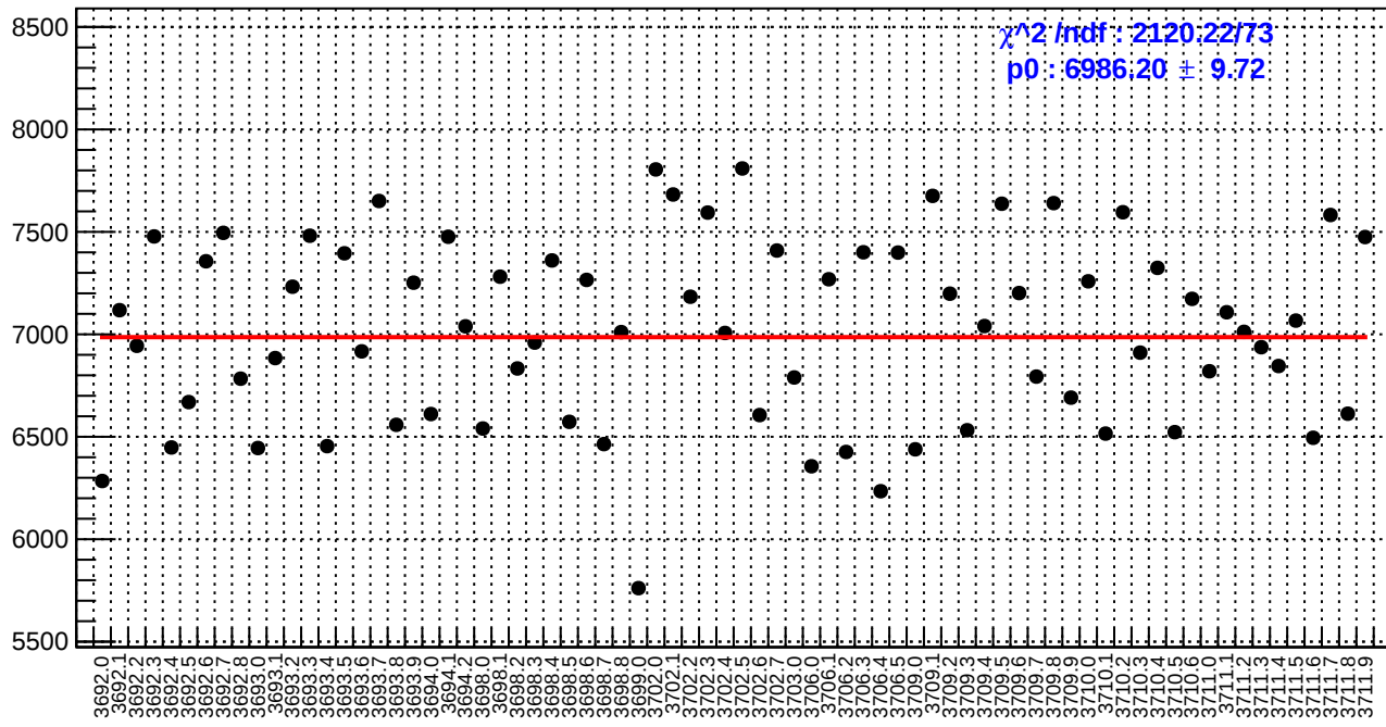
slug18: diff_bpm4aY.rms/nm
