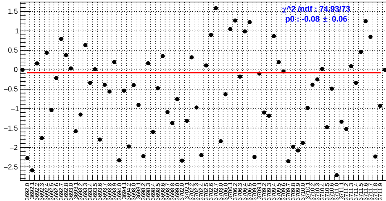
slug18: dsl_bpm4aY/(ppb/nm)
