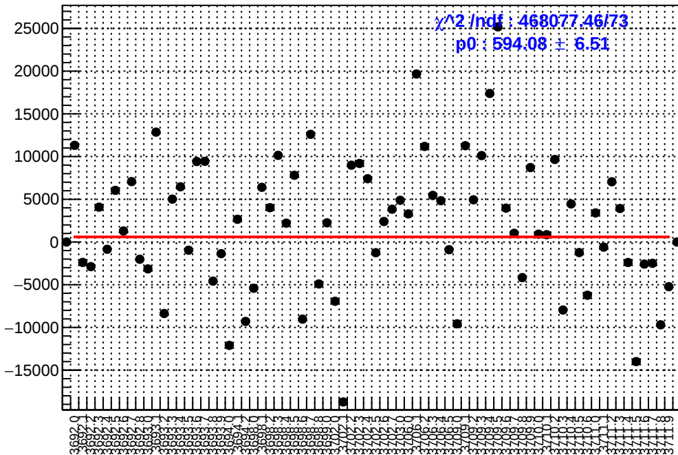
slug18: asym_usl.mean/ppb-reg_asym_usl.mean/ppb
