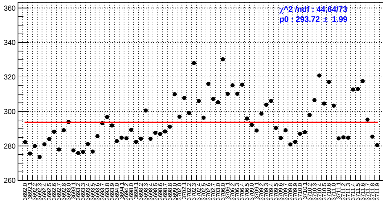
slug18: reg_asym_sam5.rms/ppm
