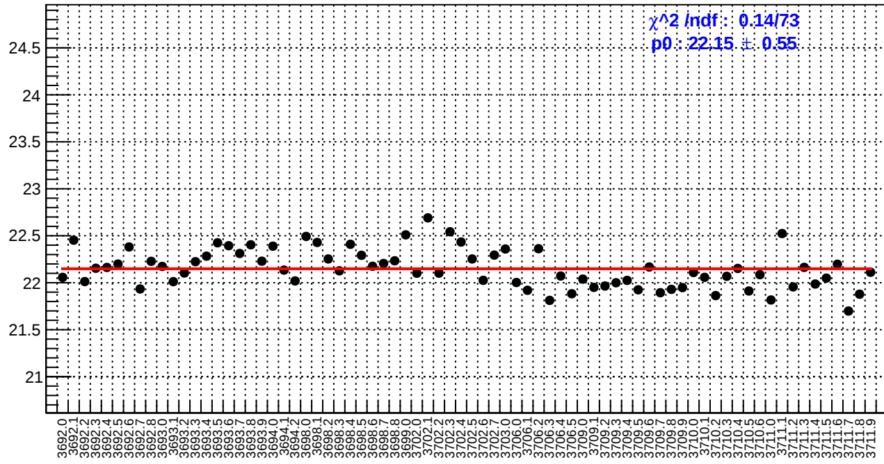
slug18: reg_asym_left_dd.rms/ppm
