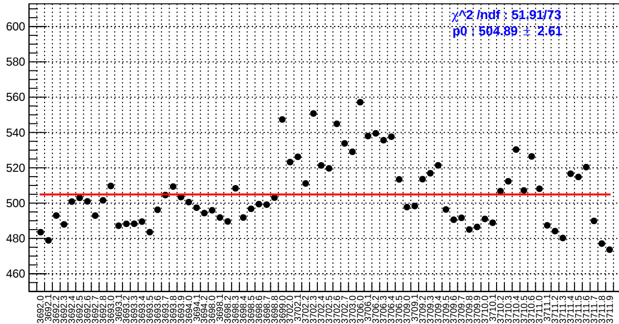
slug18: reg_asym_sam1.rms/ppm
