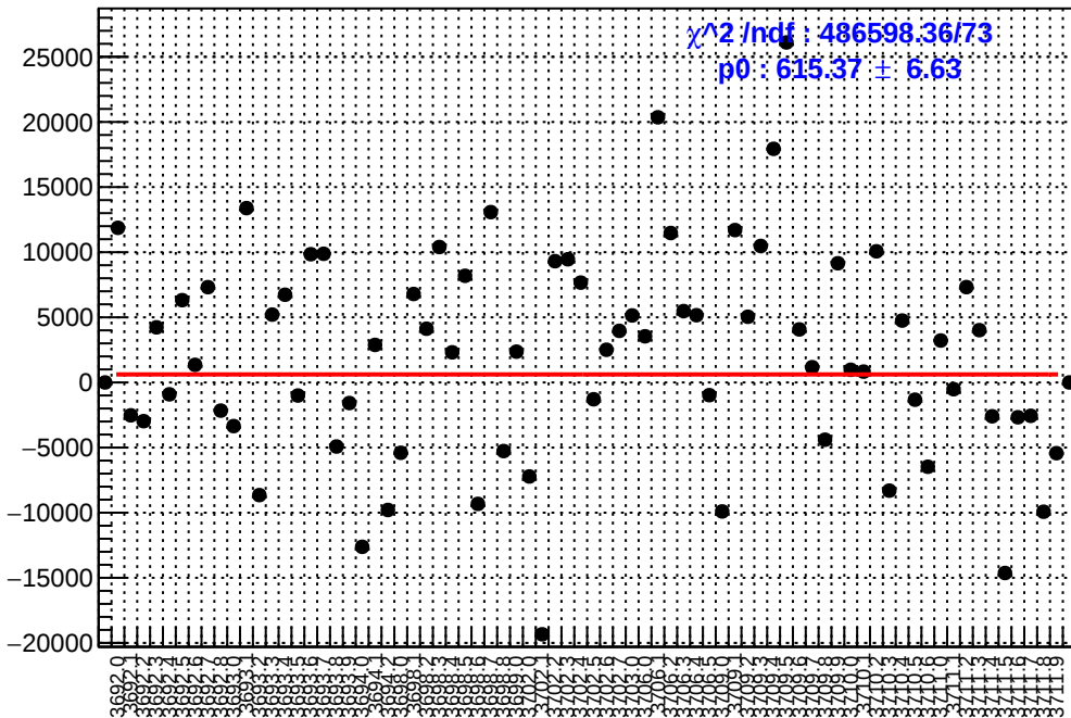
slug18: asym_left_avg.mean/ppb-reg_asym_left_avg.mean/ppb
