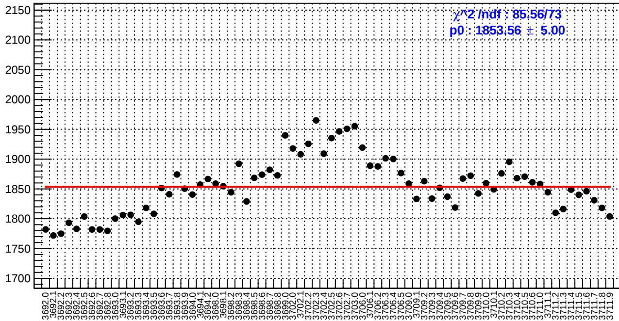
slug18: reg_asym_sam2.rms/ppm
