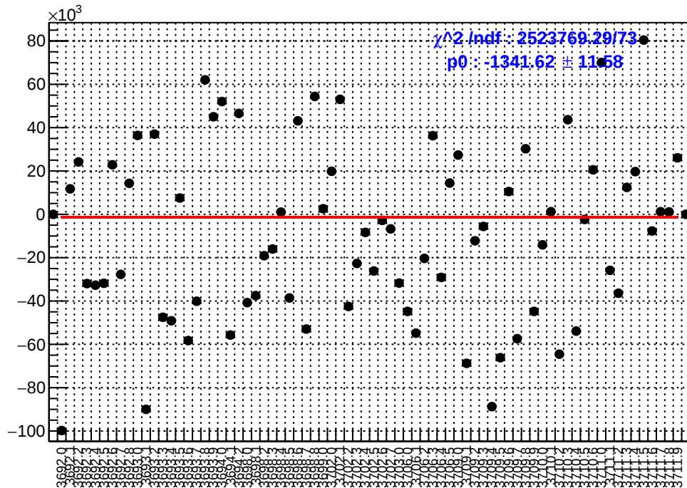
slug18: asym_sam8.mean/ppb-reg_asym_sam8.mean/ppb
