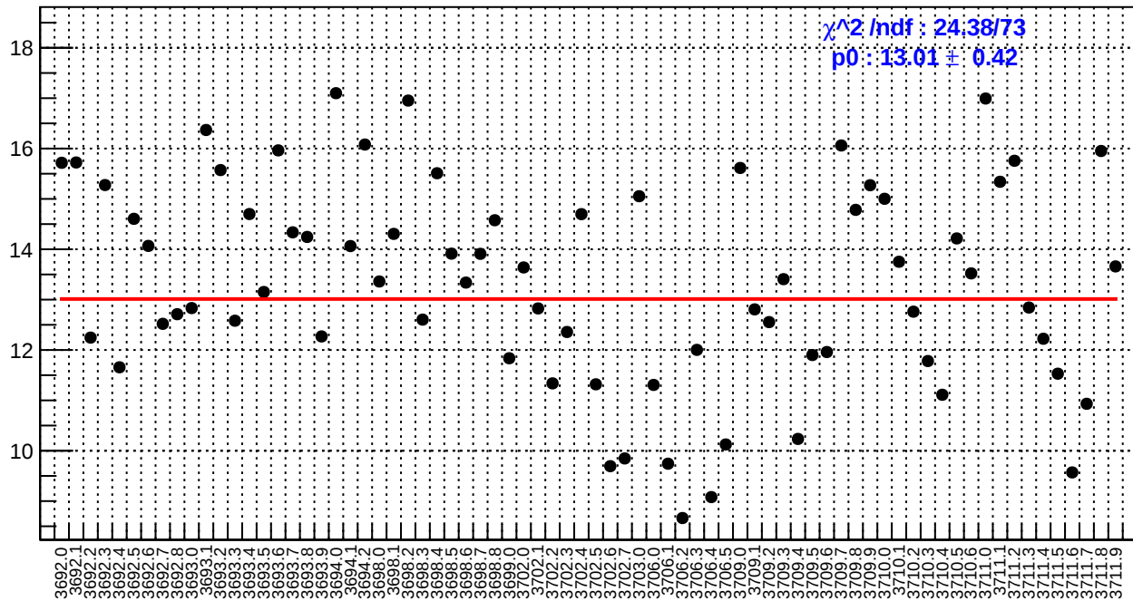
slug18: left_avg_bpm4eY/(ppb/nm)
