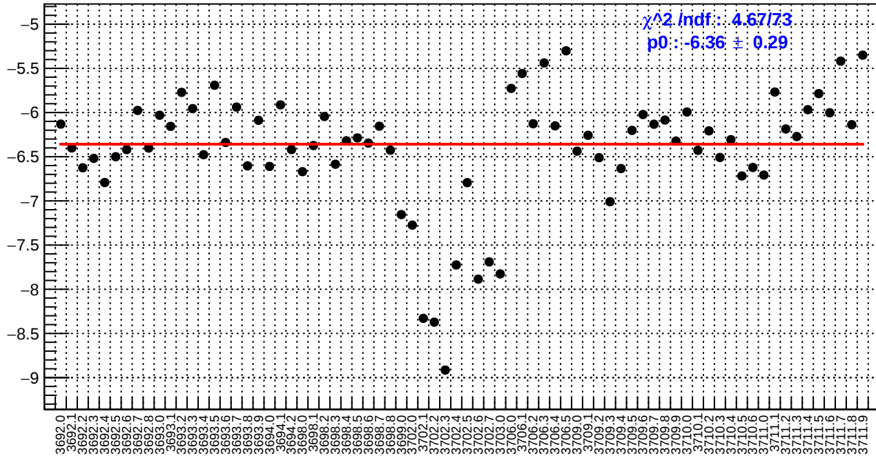
slug18: us_avg_bpm4eX/(ppb/nm)
