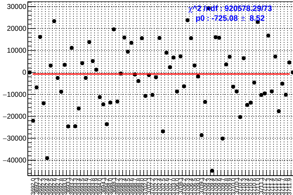
slug18: asym_sam1.mean/ppb-reg_asym_sam1.mean/ppb
