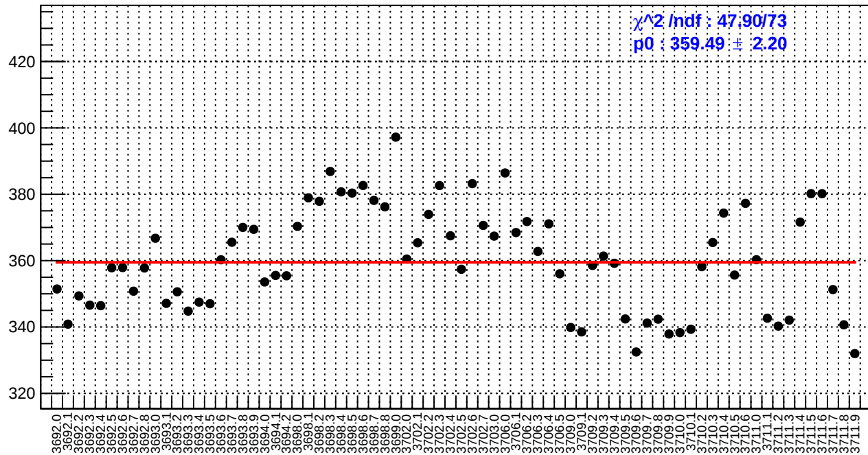
slug18: reg_asym_sam7.rms/ppm
