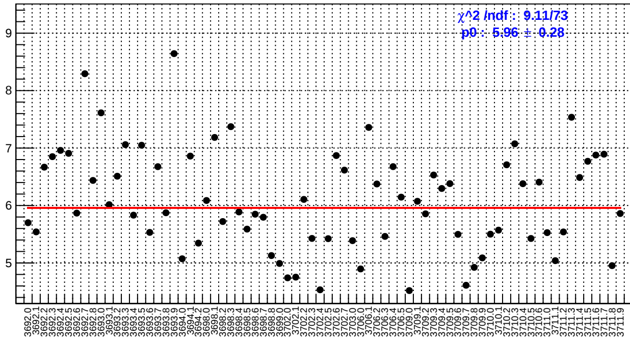
slug18: ds_avg_bpm4aY/(ppb/nm)
