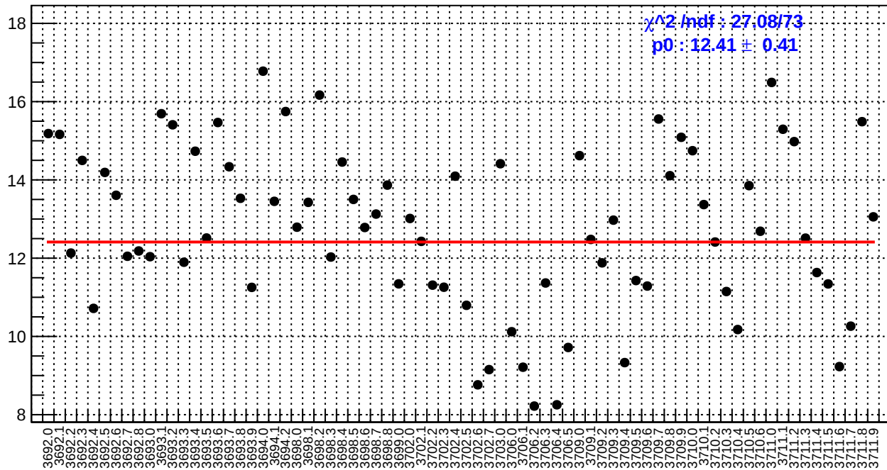
slug18: usl_bpm4eY/(ppb/nm)
