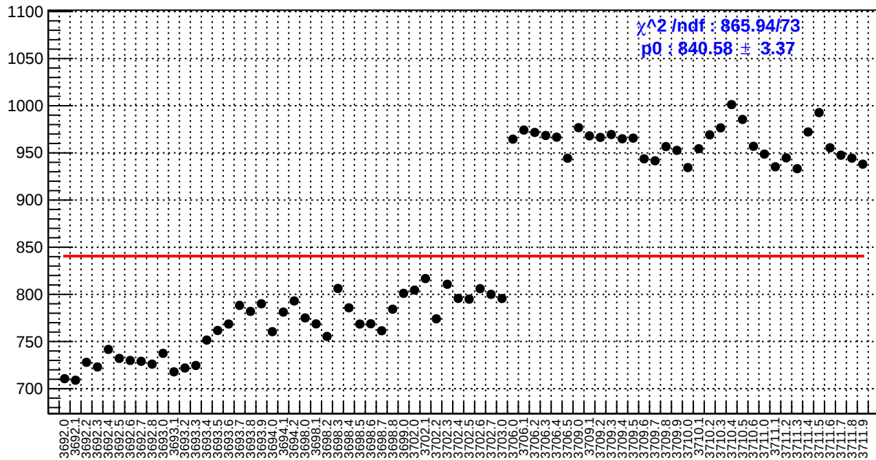
slug18: reg_asym_sam4.rms/ppm
