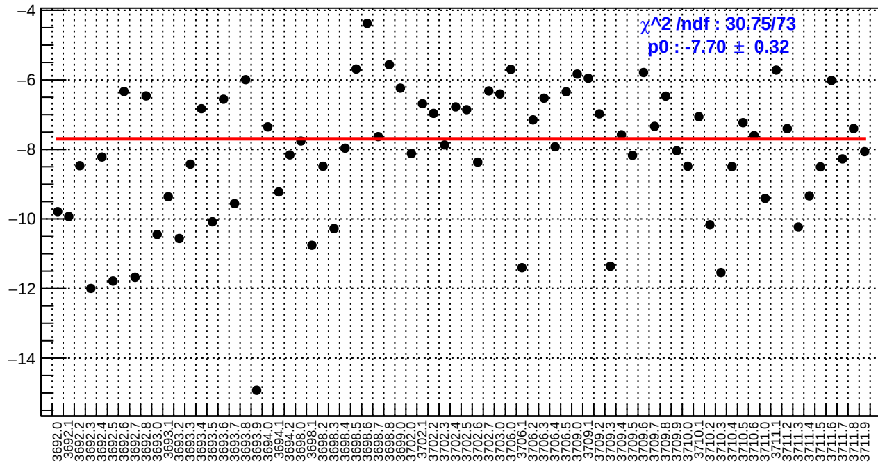
slug18: usr_bpm4eY/(ppb/nm)
