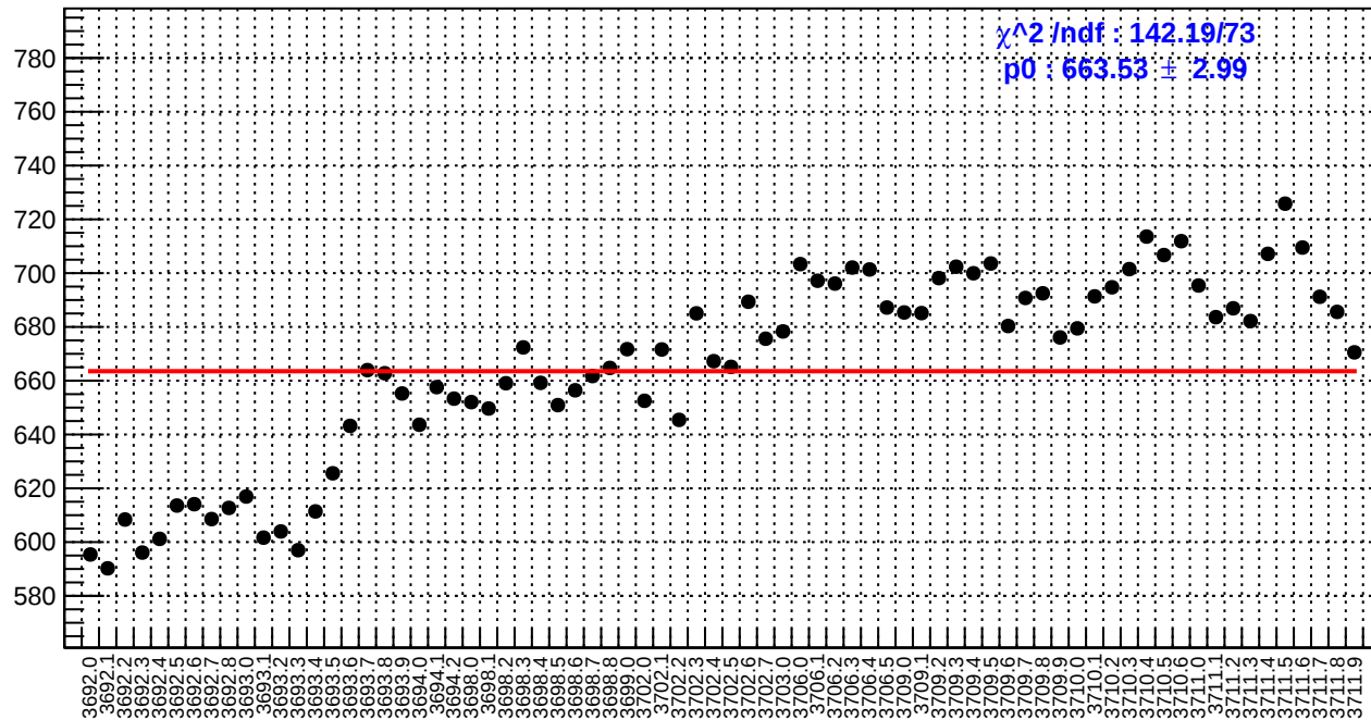
slug18: reg_asym_sam6.rms/ppm
