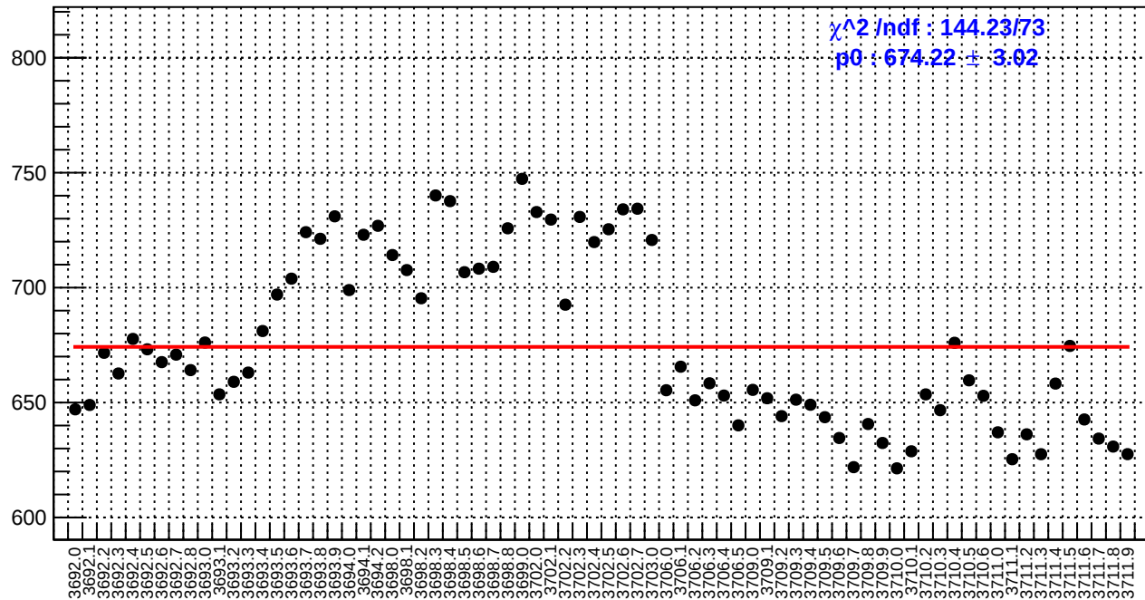
slug18: reg_asym_sam8.rms/ppm
