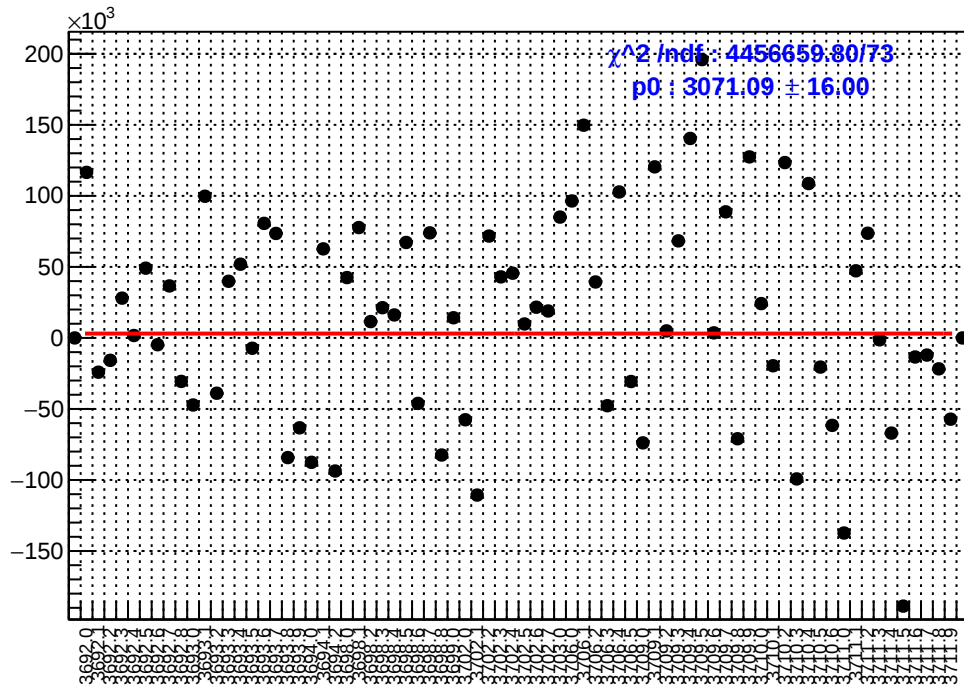
slug18: asym_sam3.mean/ppb-reg_asym_sam3.mean/ppb
