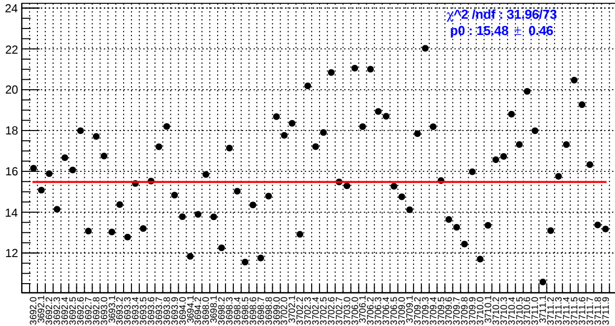
slug18: dsl_bpm4aX/(ppb/nm)
