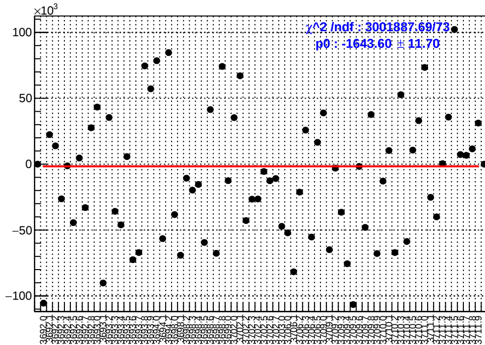
slug18: asym_sam7.mean/ppb-reg_asym_sam7.mean/ppb
