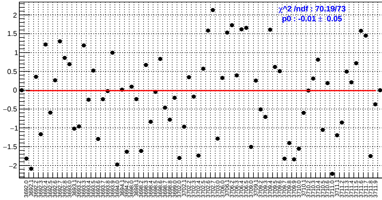
slug18: left_avg_bpm4aY/(ppb/nm)
