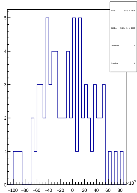
slug18: 1D Corr asym_sam8.mean/ppb-reg_asym_sam8.mean/ppb
