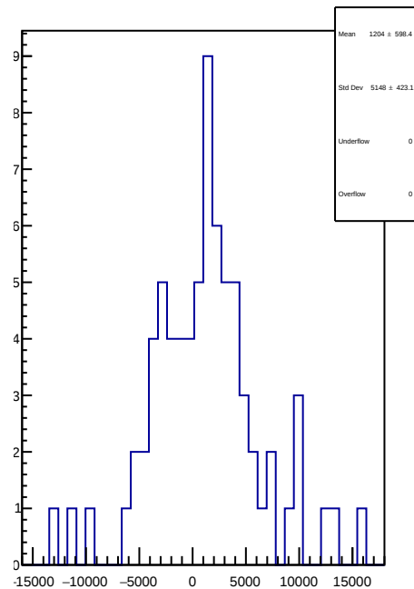
slug18: 1D Corr asym_ds_avg.mean/ppb-reg_asym_ds_avg.mean/ppb
