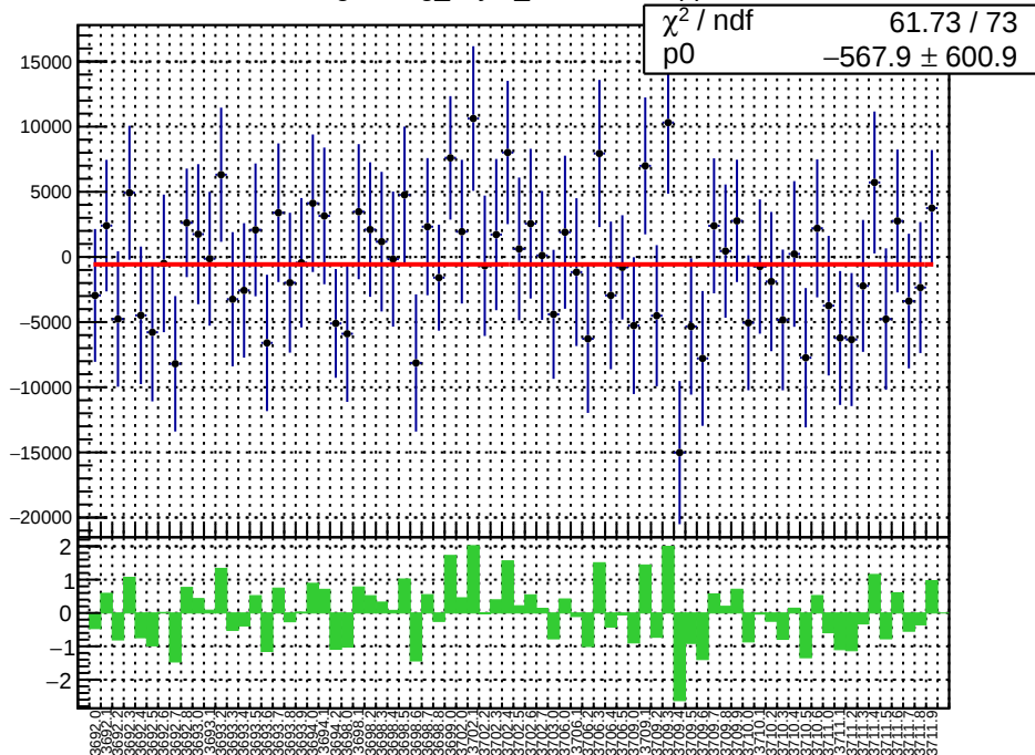
slug18: reg_asym_sam1.mean/ppb
