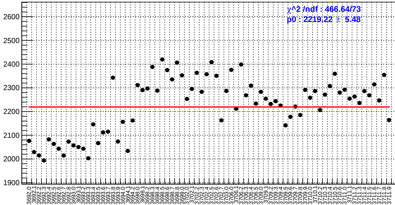
slug18: diff_bpm4aX.rms/nm
