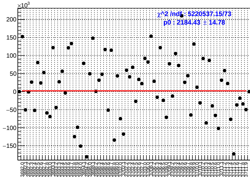
slug18: asym_sam2.mean/ppb-reg_asym_sam2.mean/ppb
