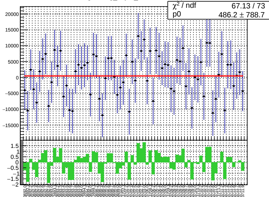
slug18: reg_asym_sam6.mean/ppb
