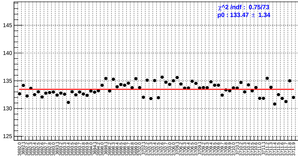
slug18: reg_asym_right_avg.rms/ppm
