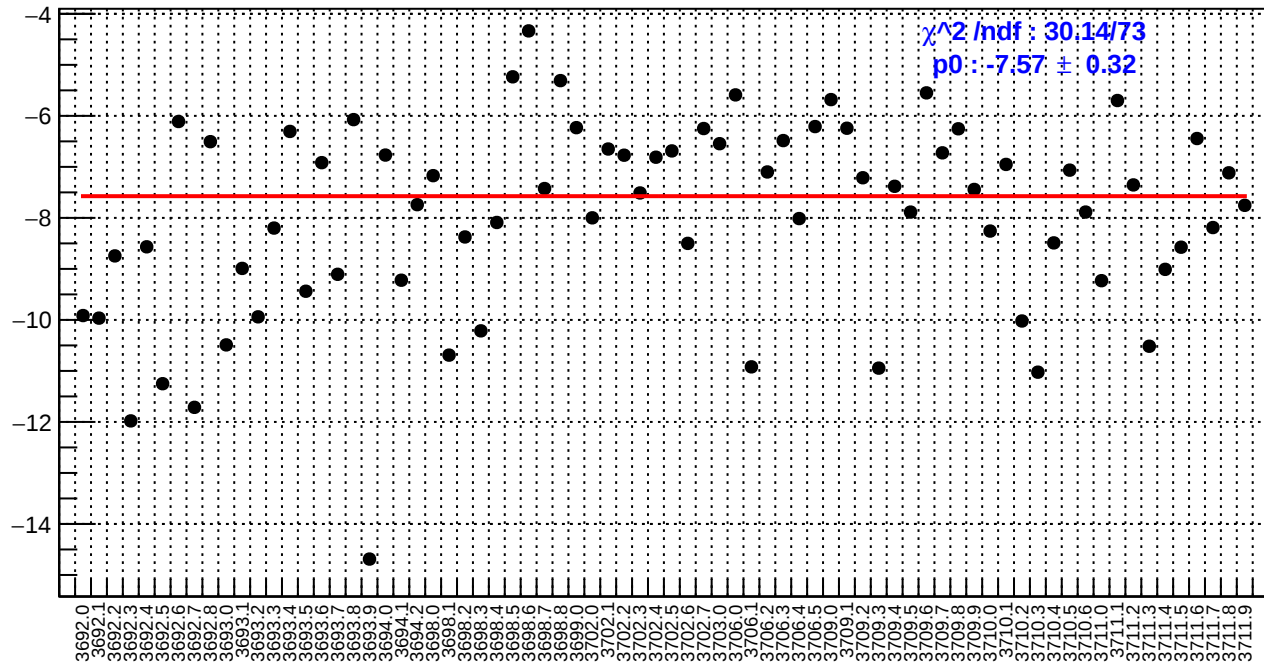
slug18: right_avg_bpm4eY/(ppb/nm)
