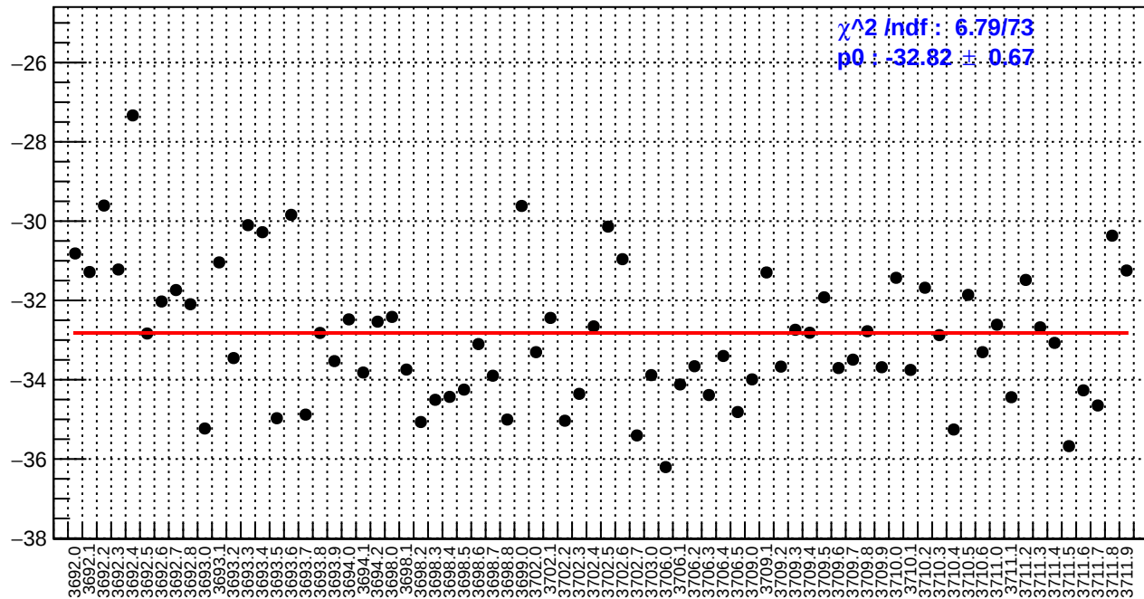
slug18: right_avg_bpm4aX/(ppb/nm)
