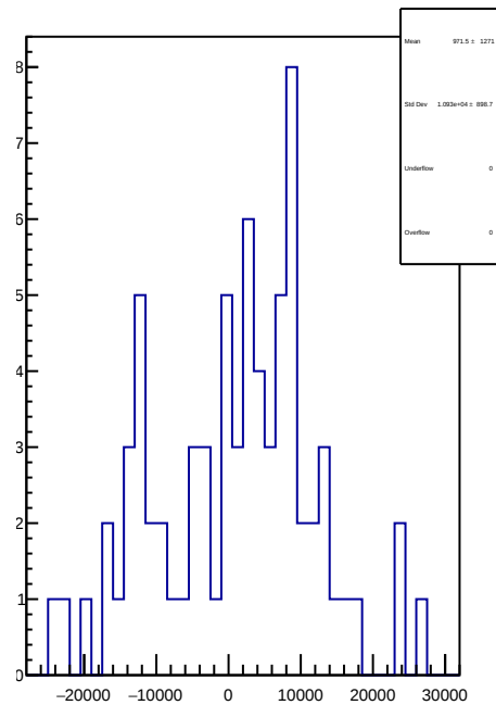
slug18: 1D Corr asym_sam5.mean/ppb-reg_asym_sam5.mean/ppb
