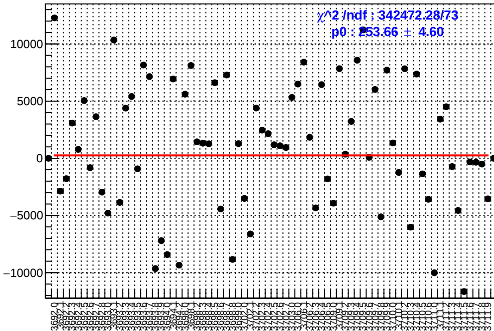
slug18: asym_ds_dd.mean/ppb-reg_asym_ds_dd.mean/ppb
