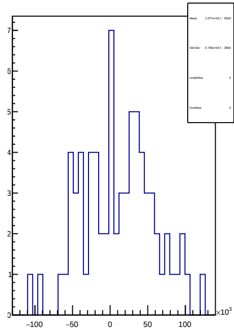
slug18: 1D Corr asym_sam4.mean/ppb-reg_asym_sam4.mean/ppb
