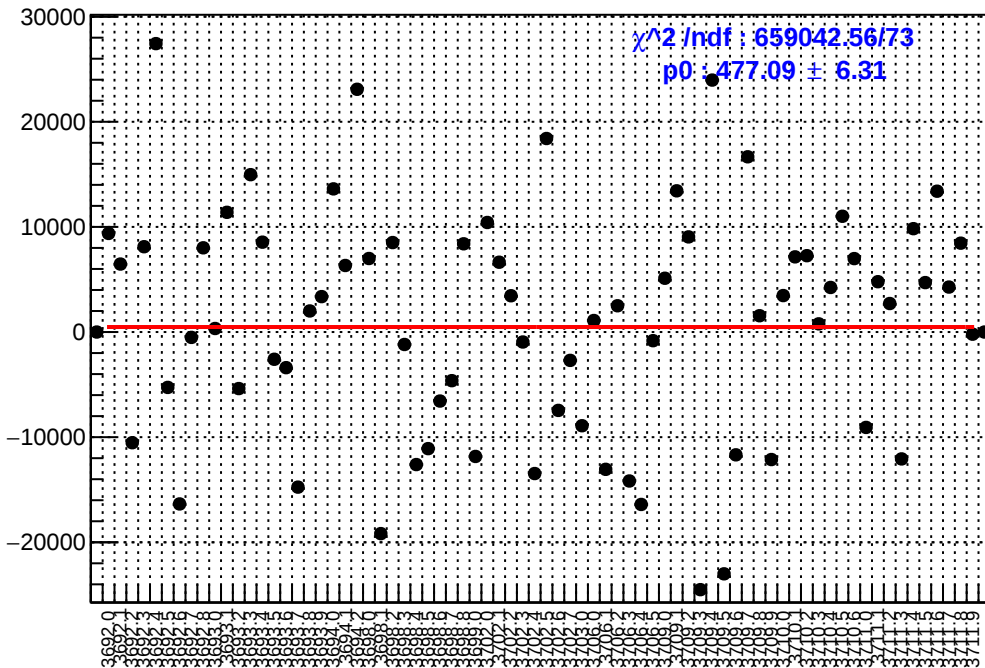
slug18: asym_sam5.mean/ppb-reg_asym_sam5.mean/ppb
