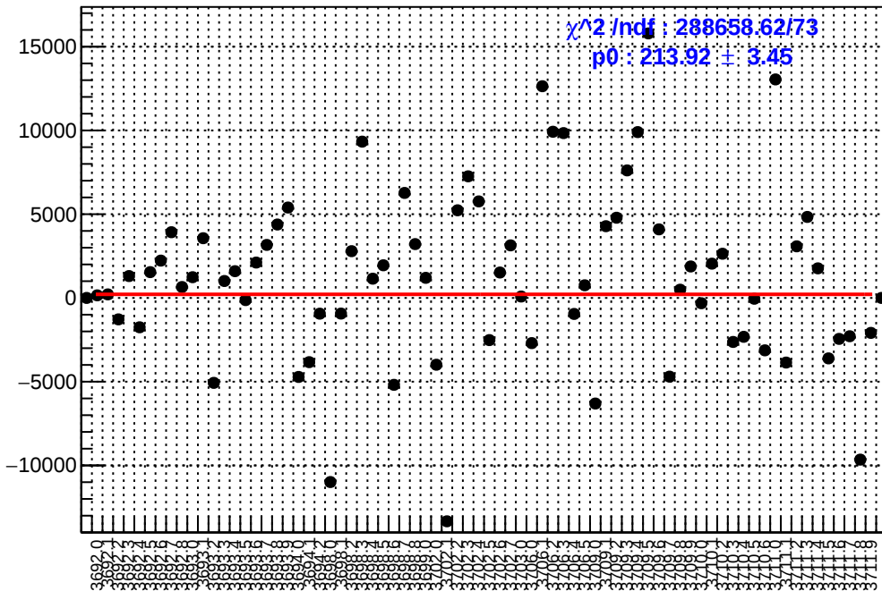
slug18: asym_ds_avg.mean/ppb-reg_asym_ds_avg.mean/ppb
