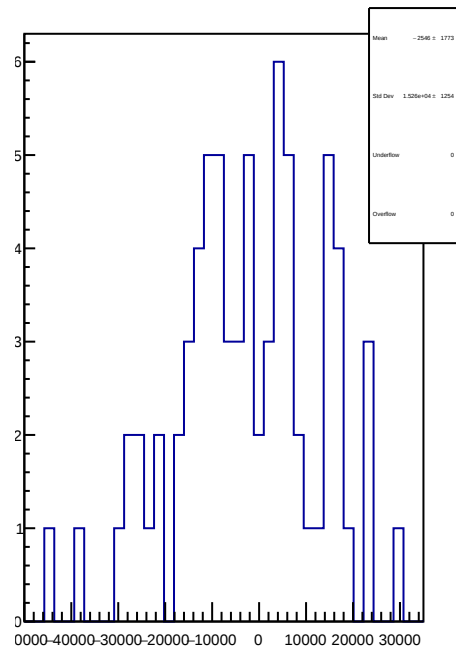
slug18: 1D Corr asym_sam1.mean/ppb-reg_asym_sam1.mean/ppb
