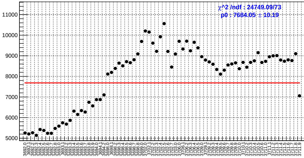
slug18: diff_bpm11X.rms/nm
