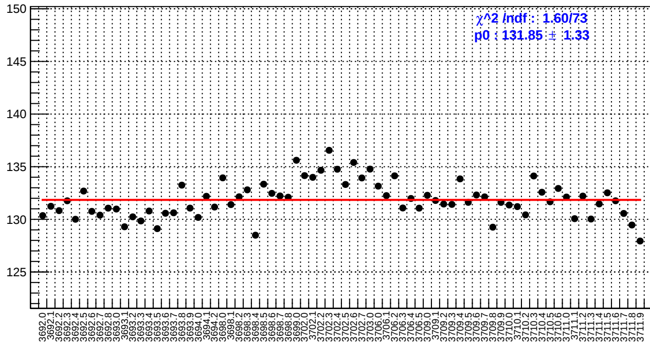
slug18: reg_asym_dsl.rms/ppm
