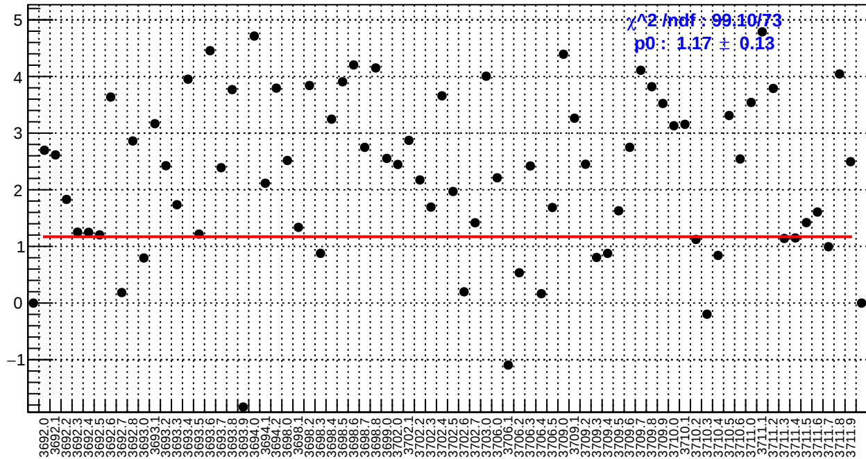
slug18: us_avg_bpm4eY/(ppb/nm)
