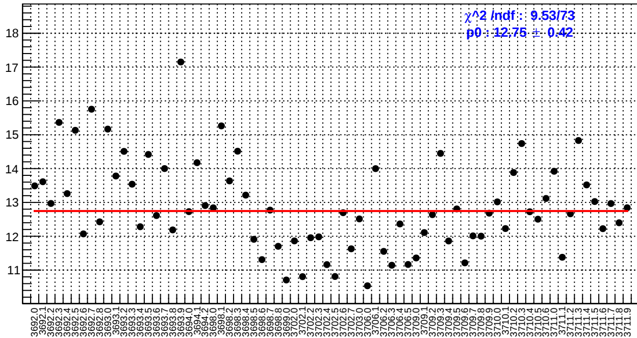
slug18: right_avg_bpm4aY/(ppb/nm)
