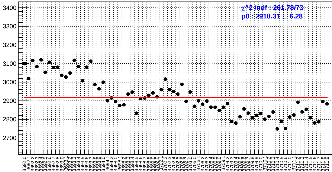
slug18: asym_bcm_an_us.rms/ppm
