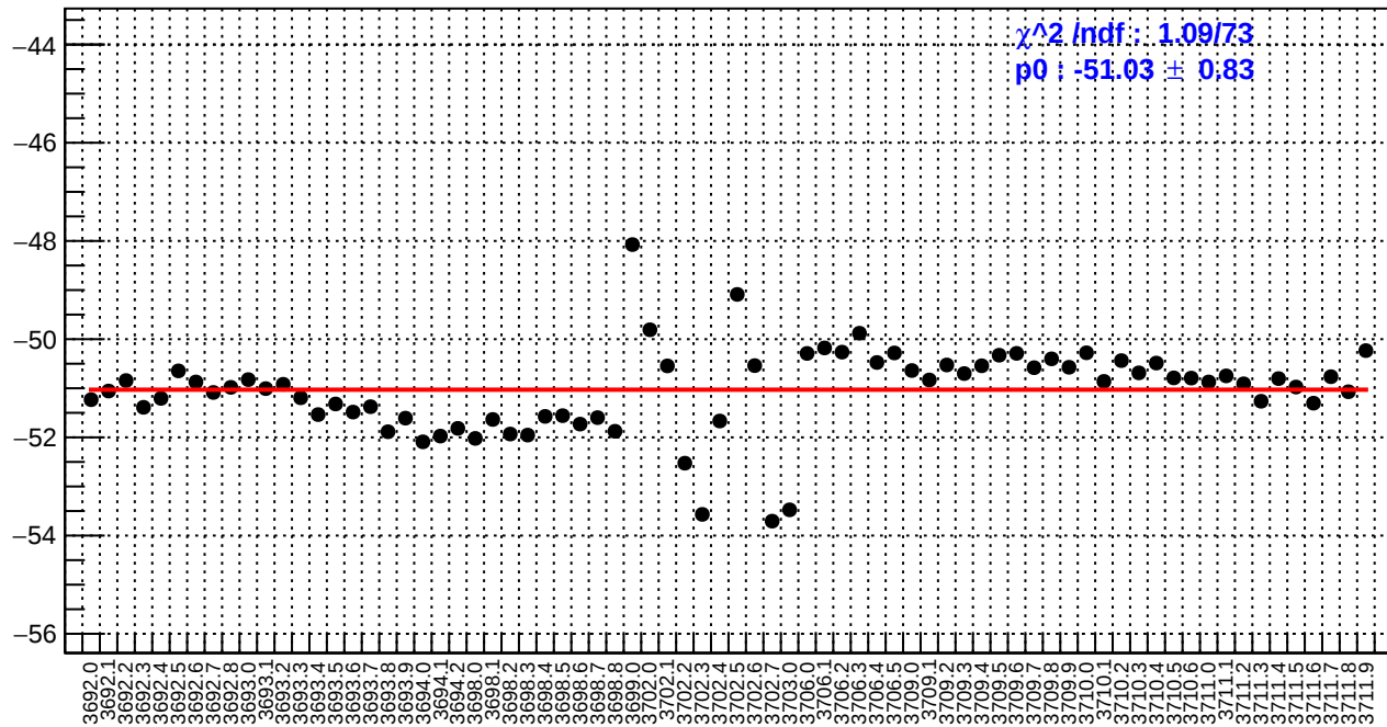
slug18: ds_avg_bpm12X/(ppb/nm)
