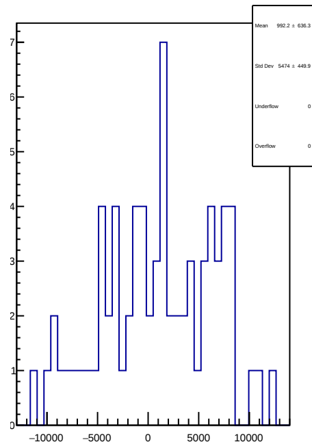
slug18: 1D Corr asym_us_dd.mean/ppb-reg_asym_us_dd.mean/ppb
