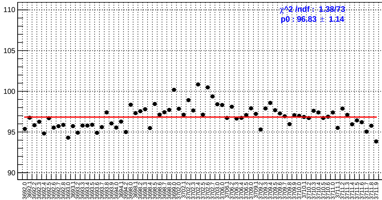
slug18: reg_asym_ds_avg.rms/ppm
