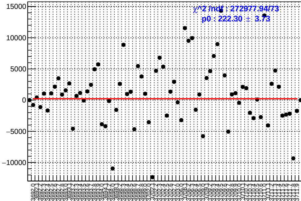
slug18: asym_us_avg.mean/ppb-reg_asym_us_avg.mean/ppb
