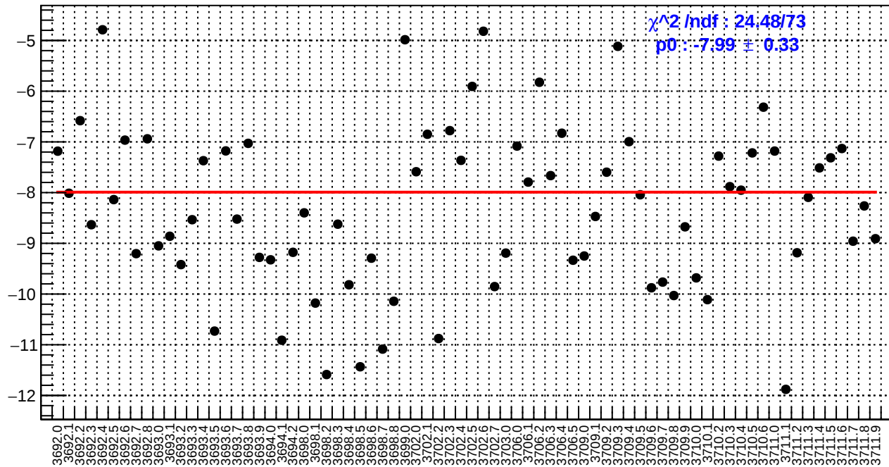
slug18: ds_avg_bpm4aX/(ppb/nm)
