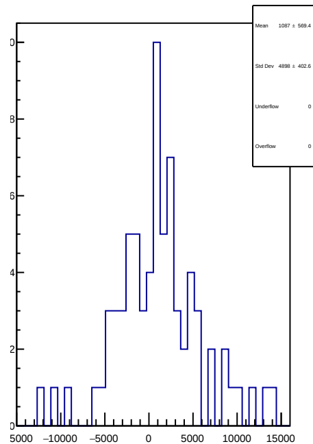
slug18: 1D Corr asym_us_avg.mean/ppb-reg_asym_us_avg.mean/ppb
