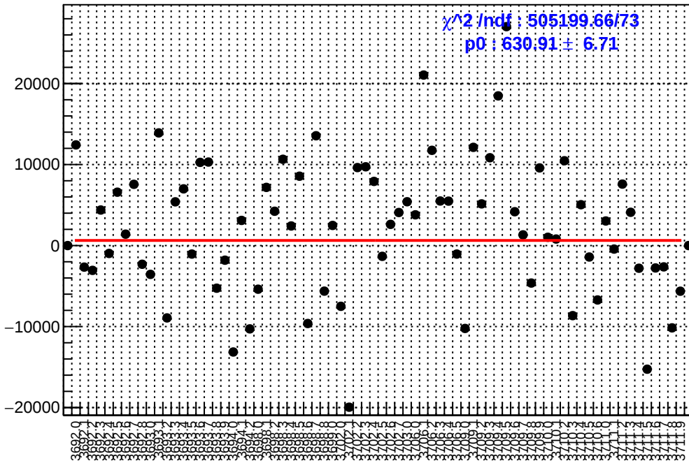
slug18: asym_dsl.mean/ppb-reg_asym_dsl.mean/ppb
