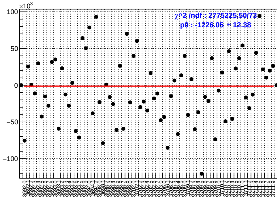
slug18: asym_sam6.mean/ppb-reg_asym_sam6.mean/ppb
