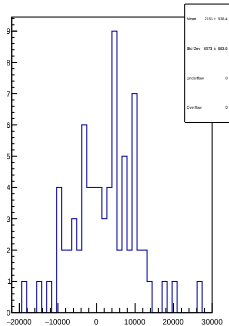
slug18: 1D Corr asym_left_avg.mean/ppb-reg_asym_left_avg.mean/ppb
