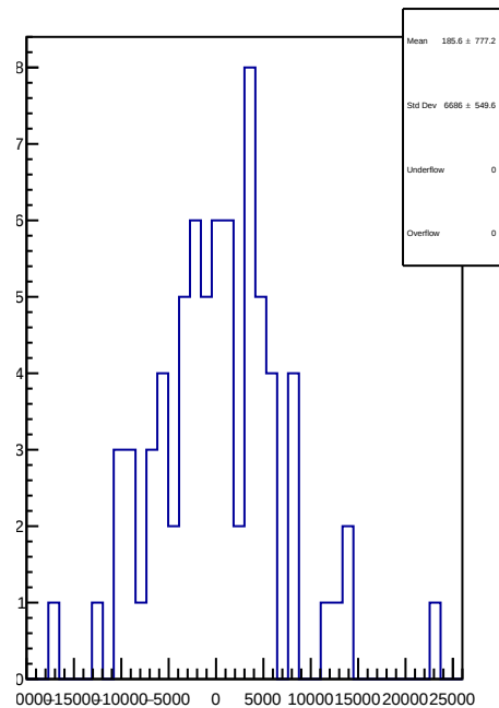
slug18: 1D Corr asym_dsr.mean/ppb-reg_asym_dsr.mean/ppb
