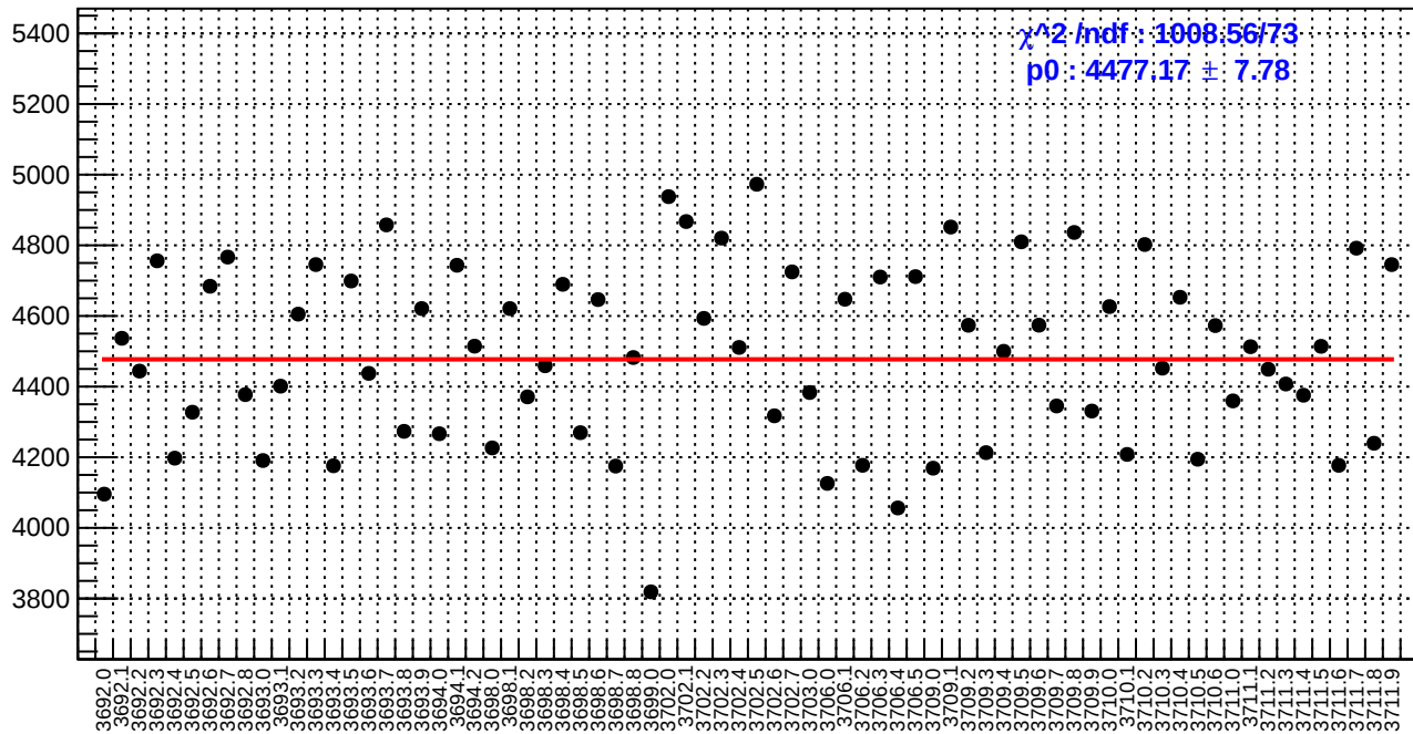
slug18: diff_bpm4eY.rms/nm
