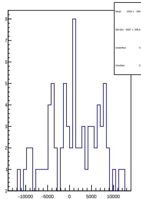
slug18: 1D Corr asym_ds_dd.mean/ppb-reg_asym_ds_dd.mean/ppb
