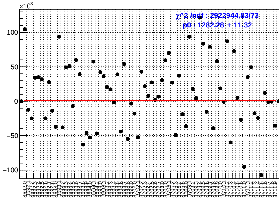
slug18: asym_sam4.mean/ppb-reg_asym_sam4.mean/ppb
