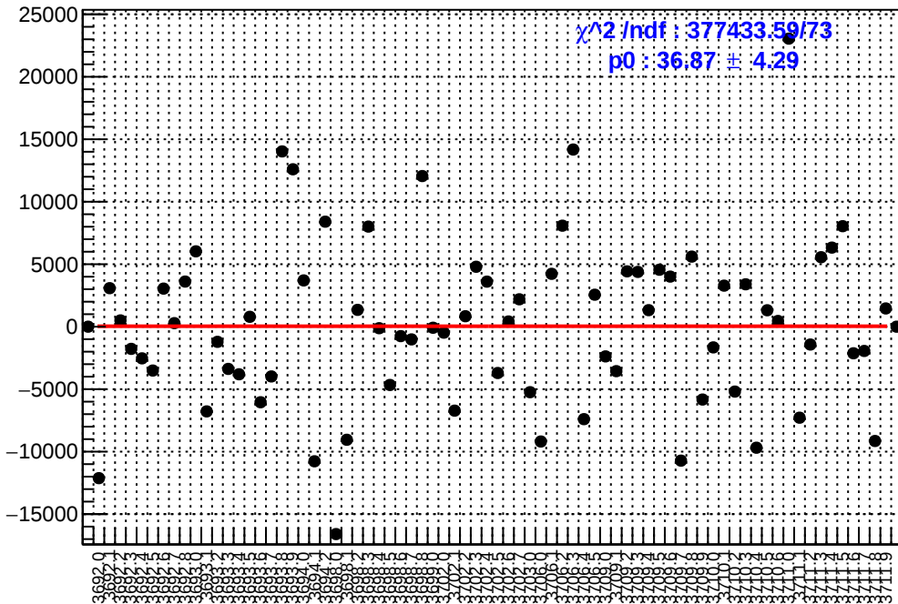
slug18: asym_dsr.mean/ppb-reg_asym_dsr.mean/ppb
