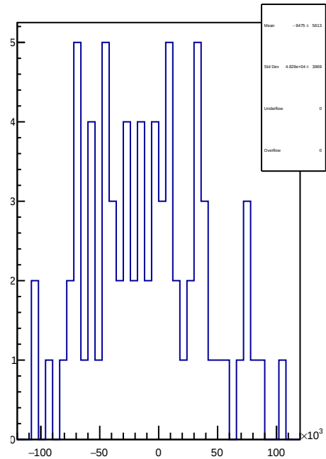
slug18: 1D Corr asym_sam7.mean/ppb-reg_asym_sam7.mean/ppb
