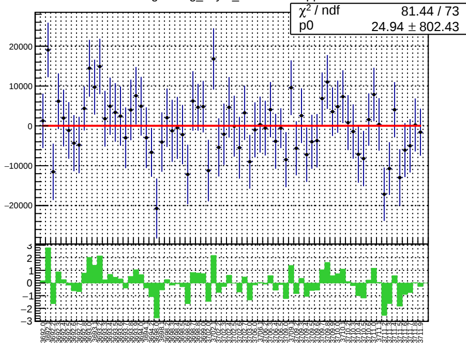
slug18: reg_asym_sam8.mean/ppb
