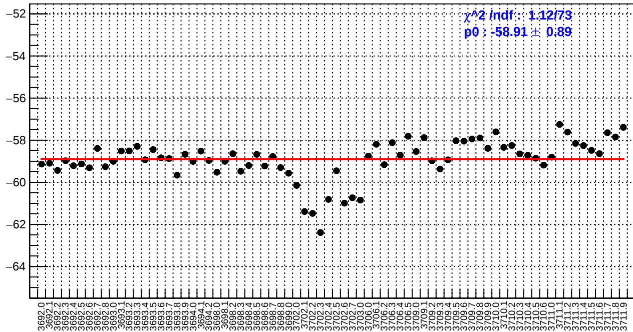
slug18: left_avg_bpm4eX/(ppb/nm)
