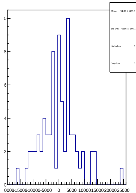
slug18: 1D Corr asym_usr.mean/ppb-reg_asym_usr.mean/ppb
