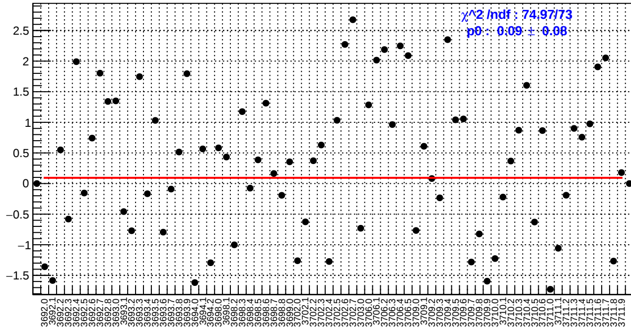
slug18: usl_bpm4aY/(ppb/nm)
