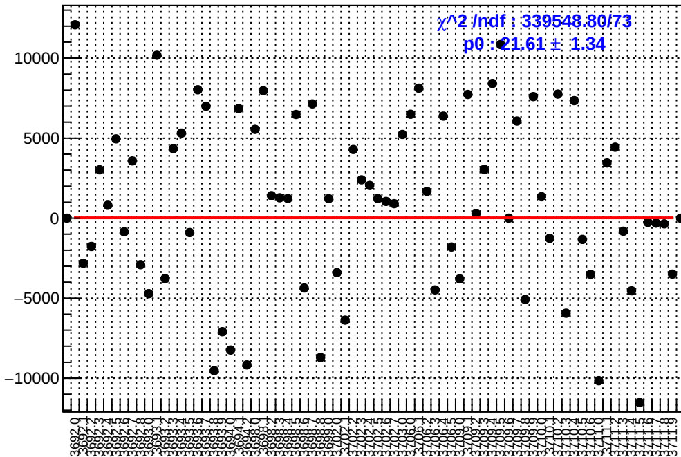
slug18: asym_us_dd.mean/ppb-reg_asym_us_dd.mean/ppb
