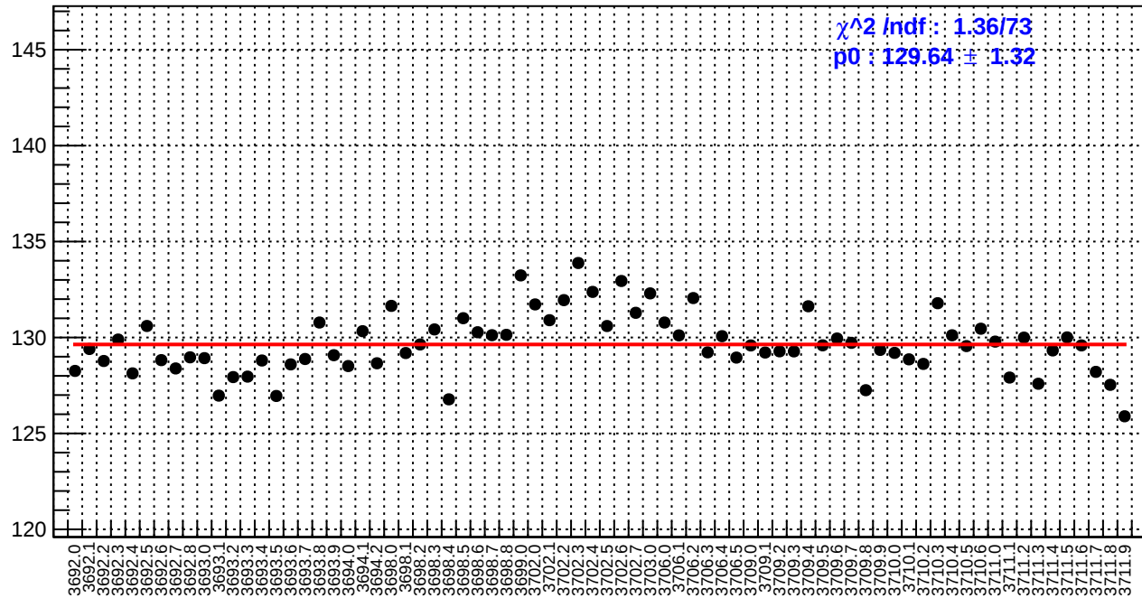
slug18: reg_asym_left_avg.rms/ppm
