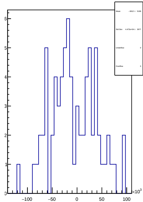
slug18: 1D Corr asym_sam6.mean/ppb-reg_asym_sam6.mean/ppb
