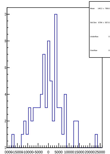
slug18: 1D Corr asym_right_avg.mean/ppb-reg_asym_right_avg.mean/ppb
