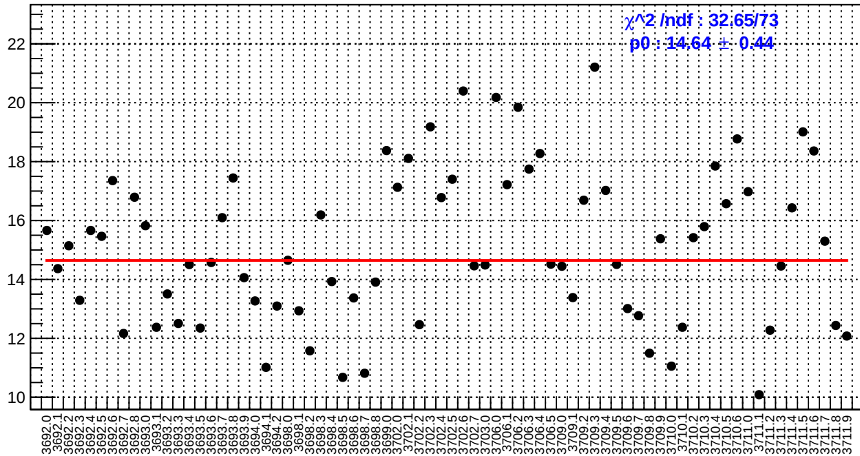
slug18: left_avg_bpm4aX/(ppb/nm)
