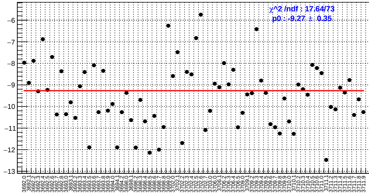
slug18: us_avg_bpm4aX/(ppb/nm)
