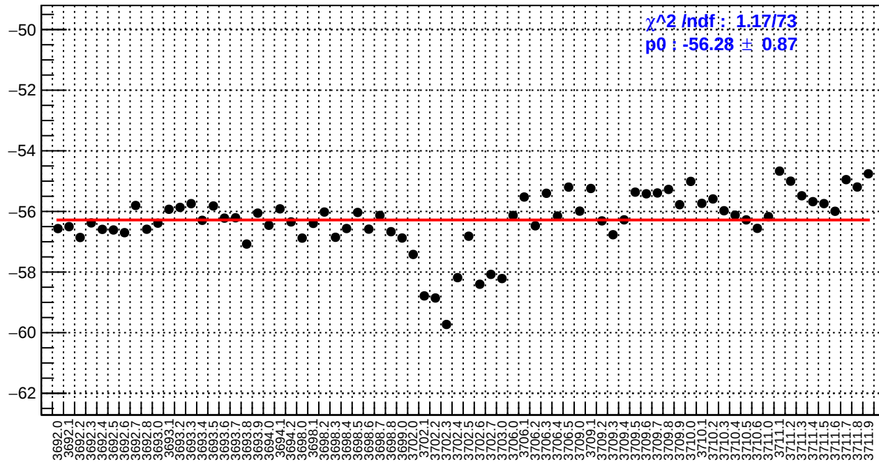
slug18: usl_bpm4eX/(ppb/nm)
