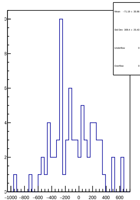
slug18: 1D Corr asym_left_dd.mean/ppb-reg_asym_left_dd.mean/ppb
