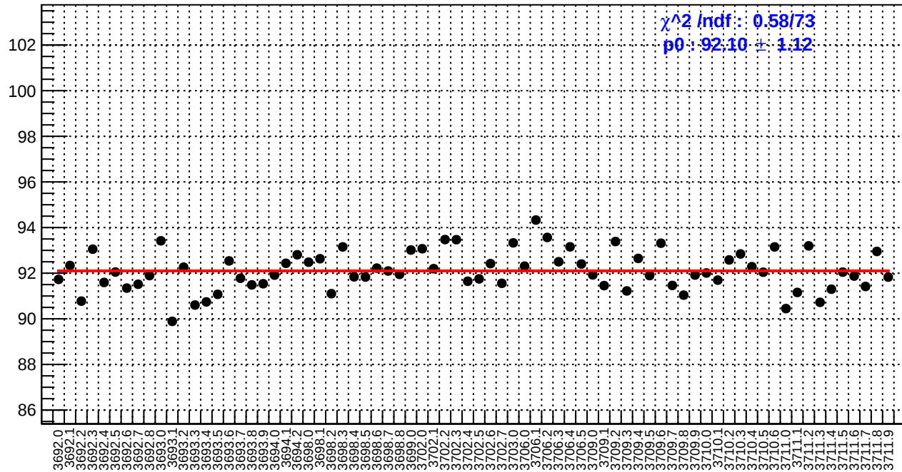
slug18: reg_asym_us_dd.rms/ppm
