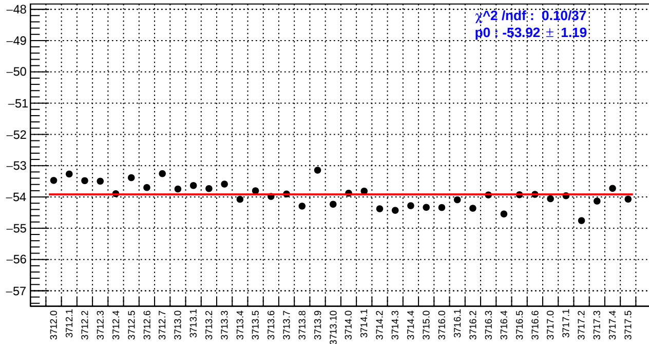
slug19: right_avg_bpm12X/(ppb/nm)
