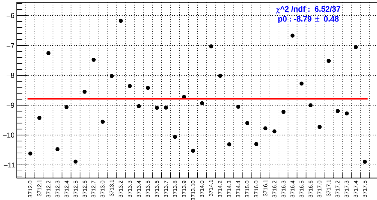
slug19: us_avg_bpm4aX/(ppb/nm)
