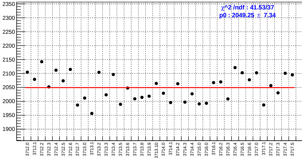
slug19: diff_bpm4aX.rms/nm
