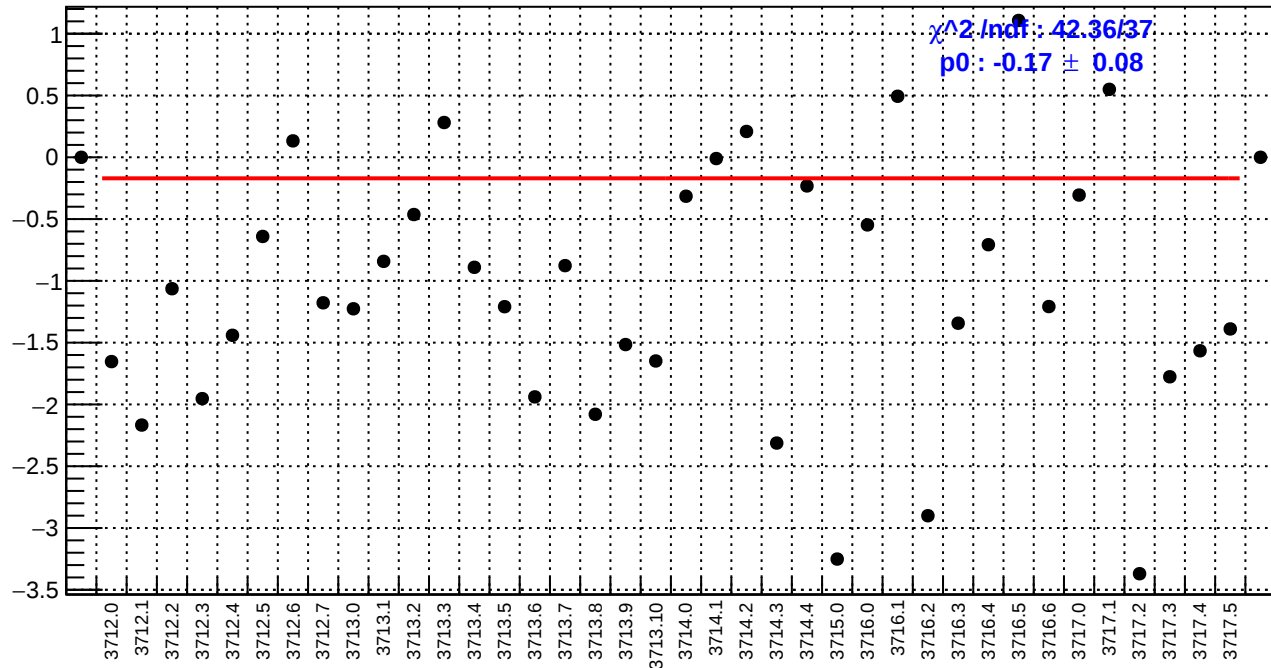
slug19: dsl_bpm4aY/(ppb/nm)
