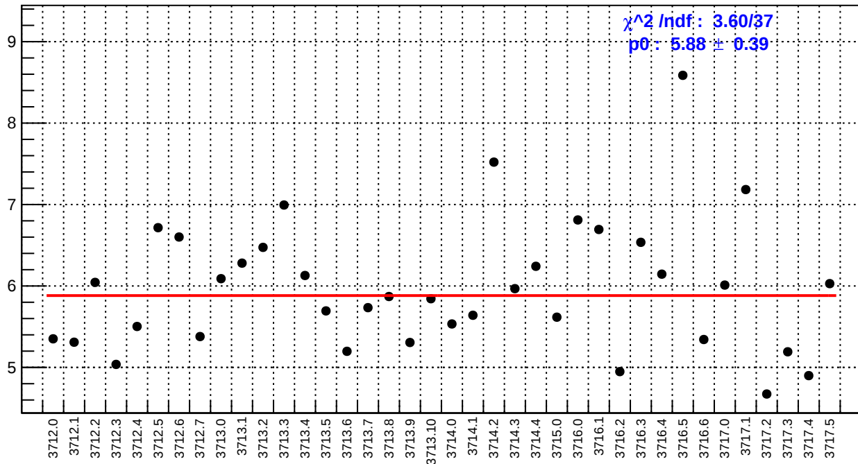
slug19: ds_avg_bpm4aY/(ppb/nm)
