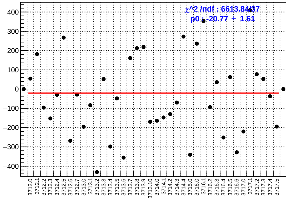
slug19: asym_right_dd.mean/ppb-reg_asym_right_dd.mean/ppb
