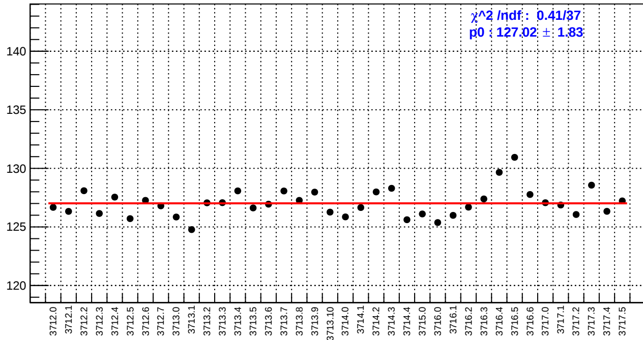
slug19: reg_asym_left_avg.rms/ppm
