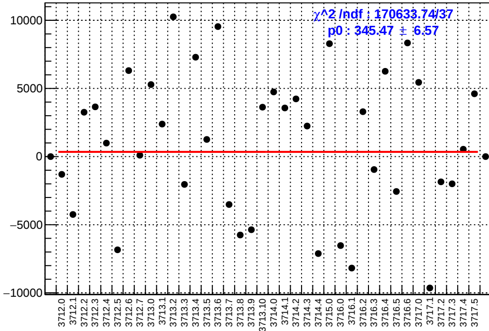
slug19: asym_ds_dd.mean/ppb-reg_asym_ds_dd.mean/ppb
