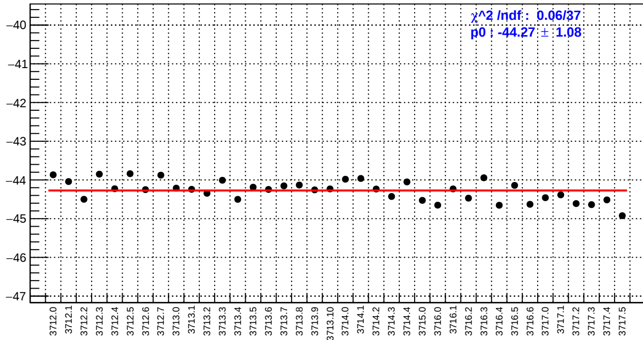
slug19: usl_bpm12X/(ppb/nm)
