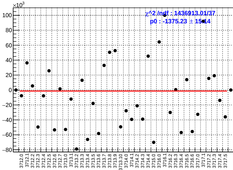
slug19: asym_sam6.mean/ppb-reg_asym_sam6.mean/ppb
