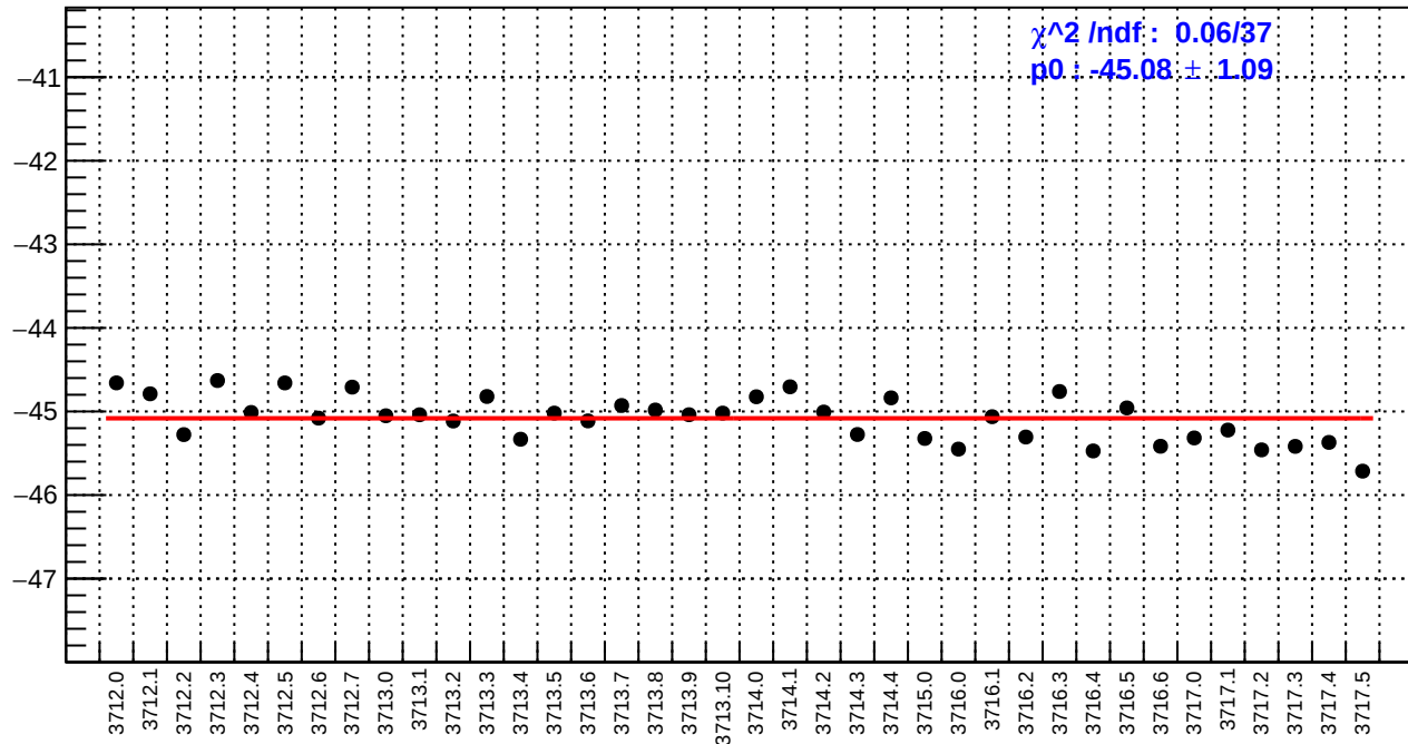
slug19: left_avg_bpm12X/(ppb/nm)
