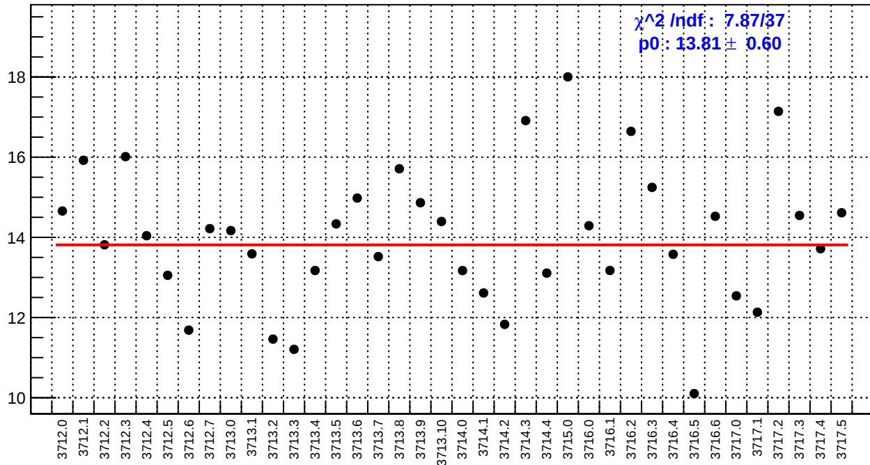
slug19: left_avg_bpm4eY/(ppb/nm)
