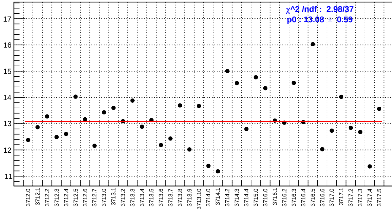
slug19: right_avg_bpm4aY/(ppb/nm)
