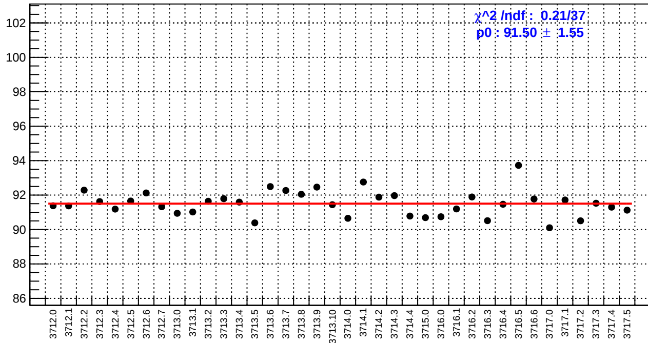
slug19: reg_asym_us_dd.rms/ppm
