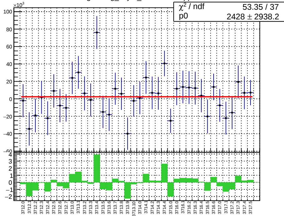
slug19: reg_asym_sam2.mean/ppb
