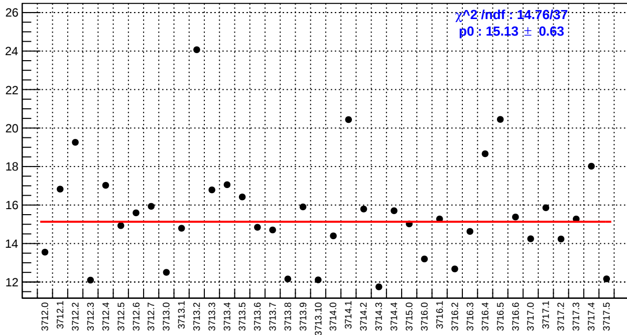
slug19: dsl_bpm4aX/(ppb/nm)
