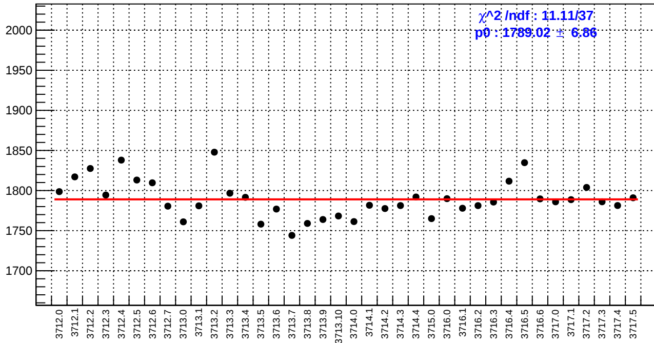
slug19: reg_asym_sam2.rms/ppm
