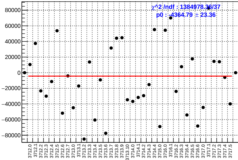
slug19: asym_sam7.mean/ppb-reg_asym_sam7.mean/ppb
