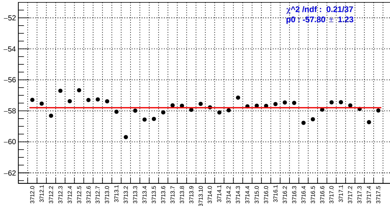
slug19: left_avg_bpm4eX/(ppb/nm)
