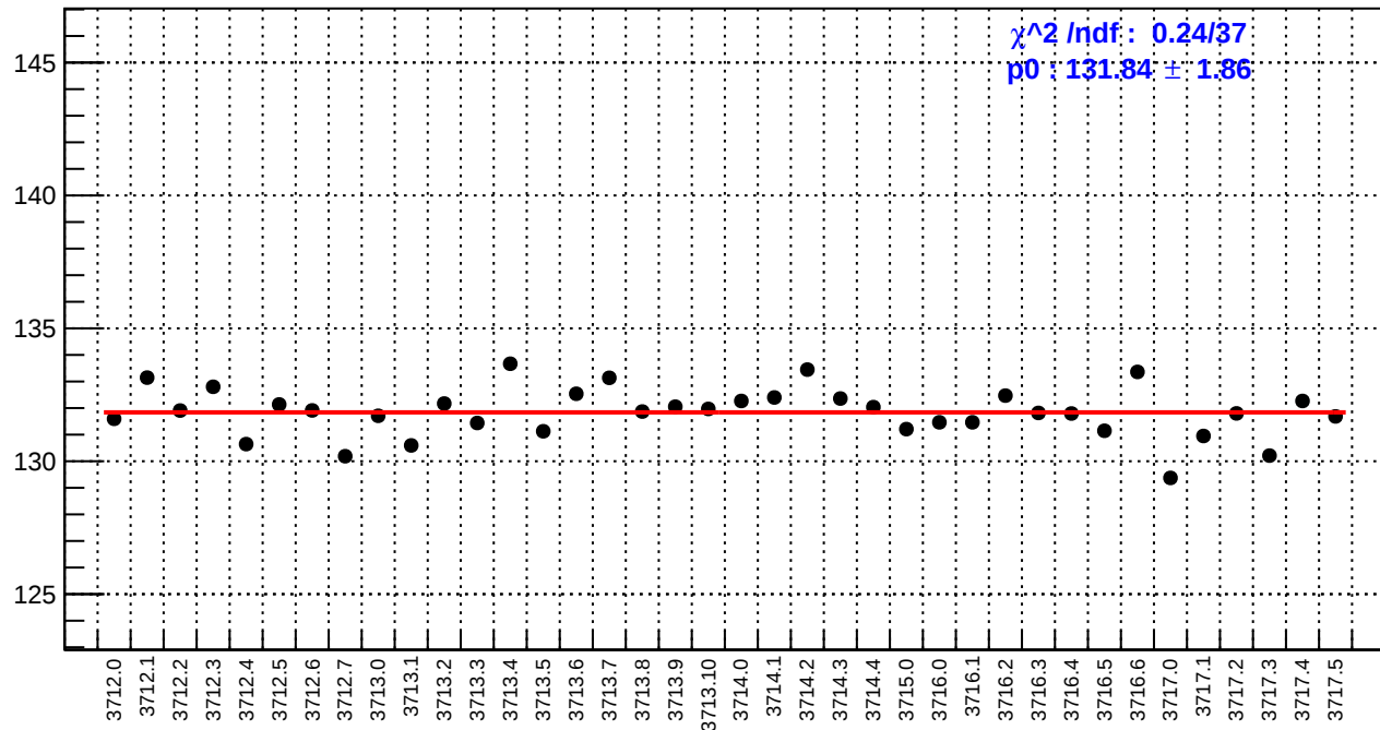
slug19: reg_asym_right_avg.rms/ppm
