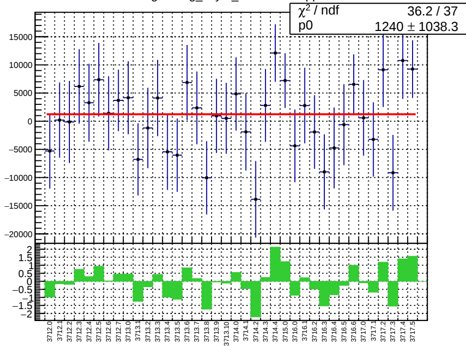
slug19: reg_asym_sam3.mean/ppb
