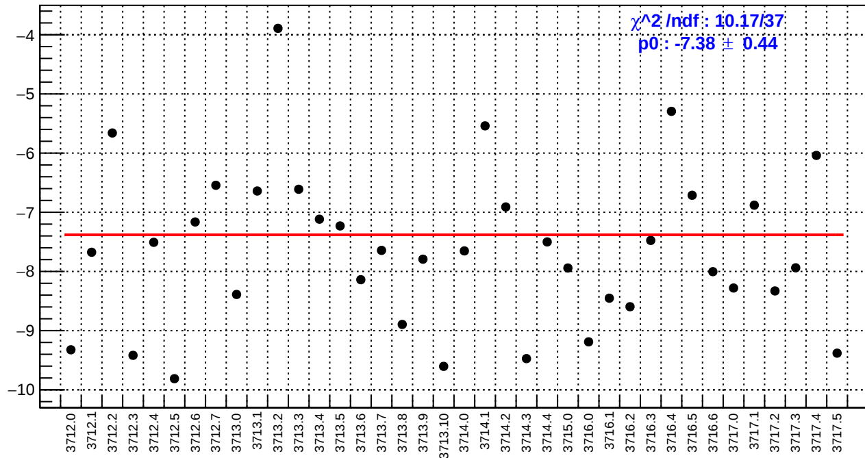
slug19: ds_avg_bpm4aX/(ppb/nm)
