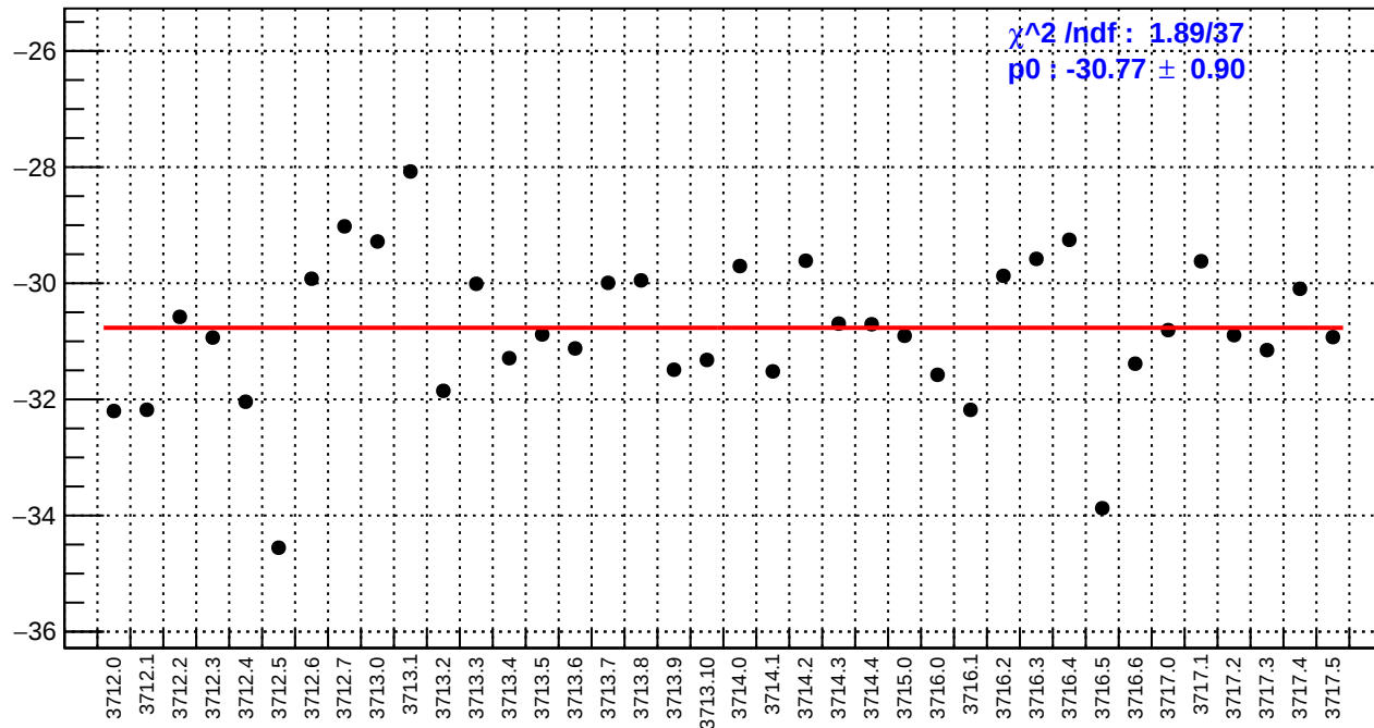
slug19: dsr_bpm4aX/(ppb/nm)
