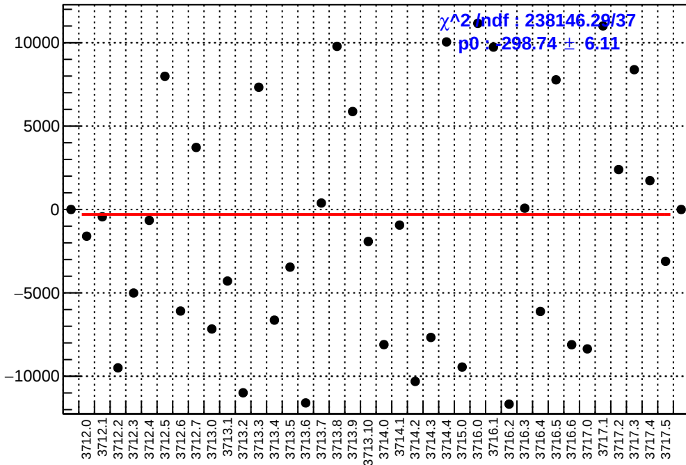
slug19: asym_usr.mean/ppb-reg_asym_usr.mean/ppb
