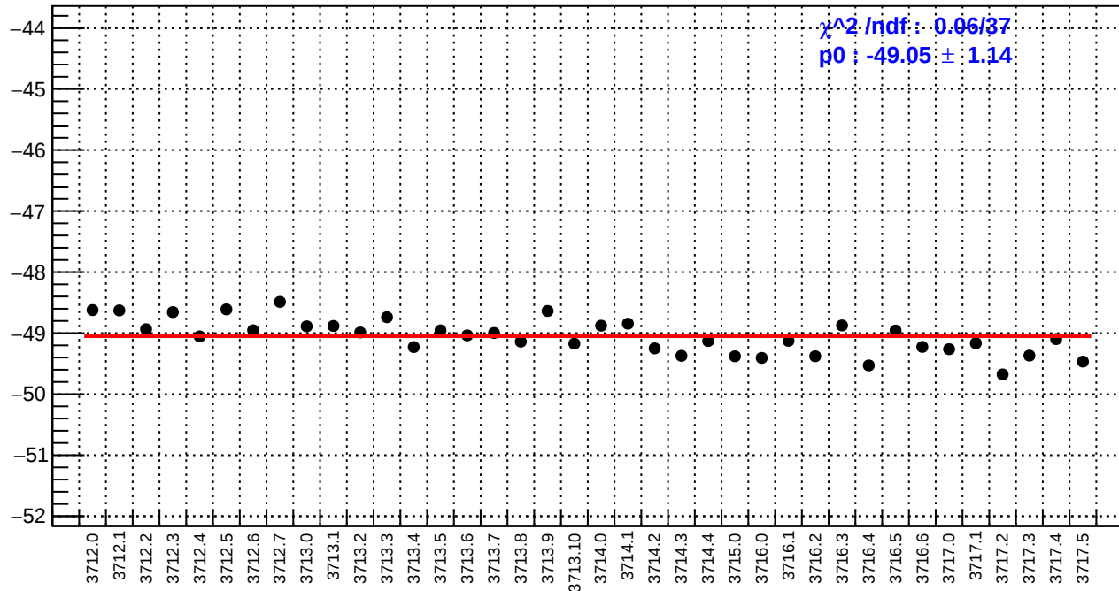
slug19: us_avg_bpm12X/(ppb/nm)
