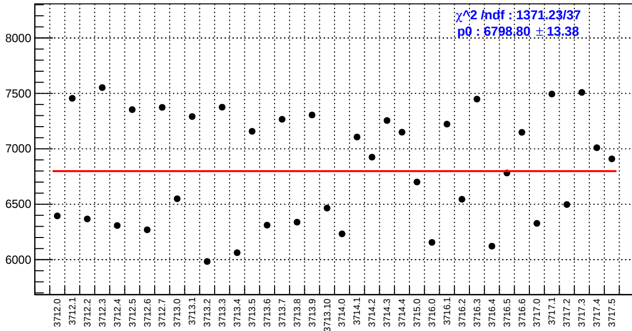
slug19: diff_bpm4aY.rms/nm
