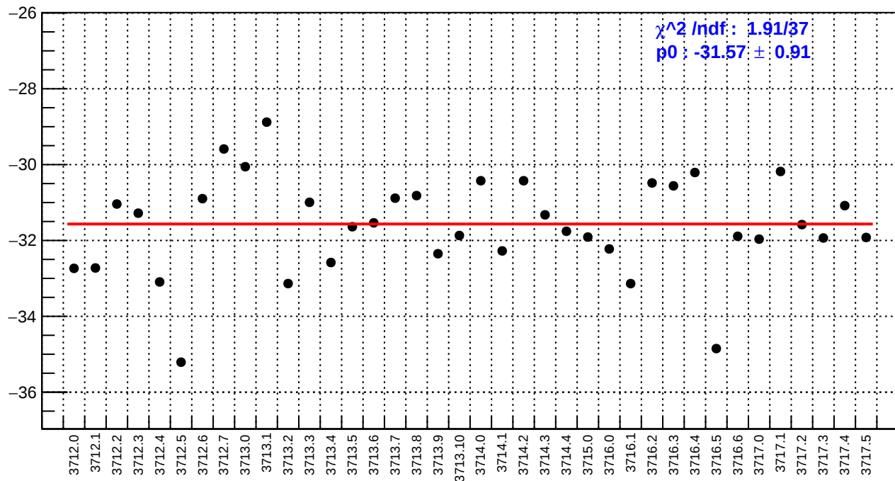
slug19: right_avg_bpm4aX/(ppb/nm)
