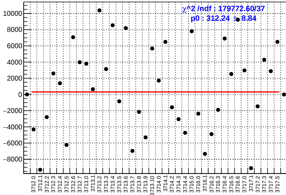
slug19: asym_dsl.mean/ppb-reg_asym_dsl.mean/ppb
