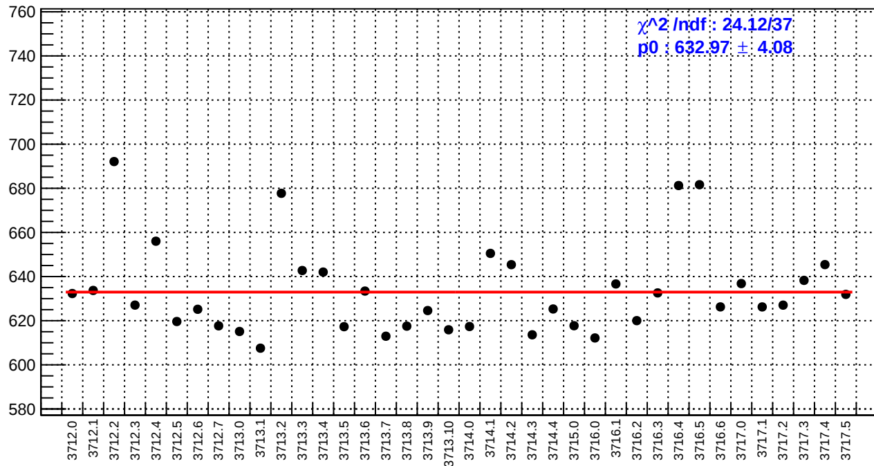
slug19: reg_asym_sam3.rms/ppm
