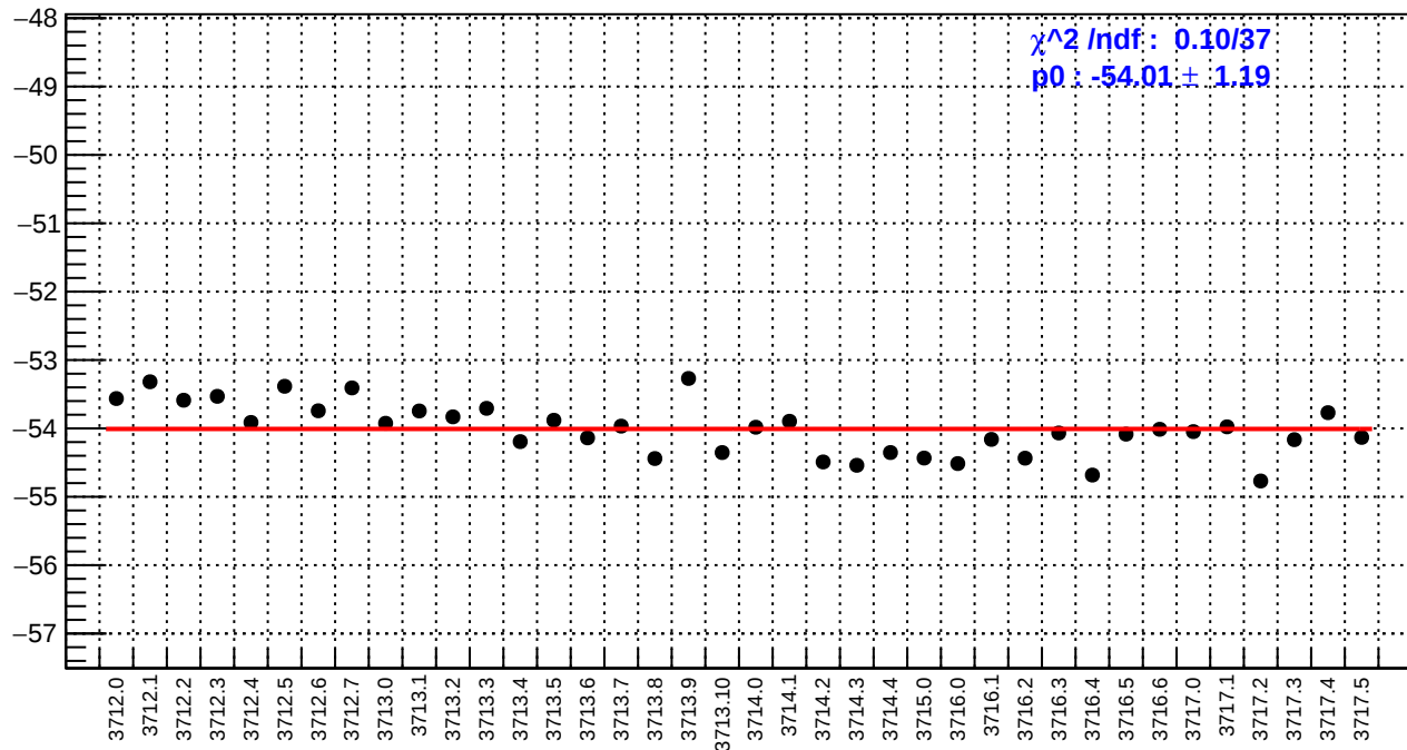
slug19: dsr_bpm12X/(ppb/nm)
