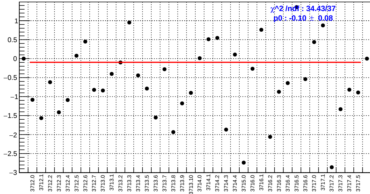
slug19: left_avg_bpm4aY/(ppb/nm)
