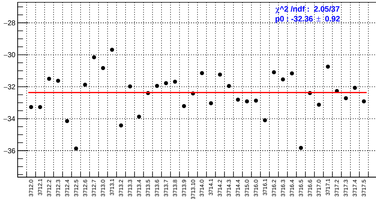
slug19: usr_bpm4aX/(ppb/nm)
