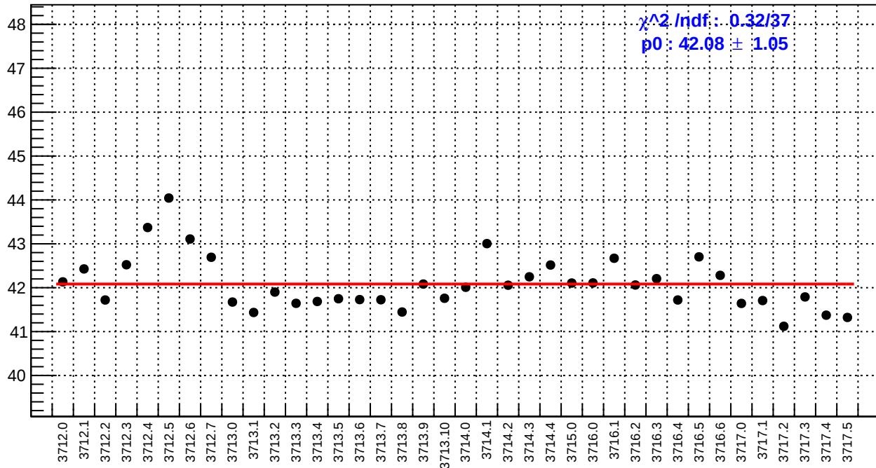
slug19: right_avg_bpm4eX/(ppb/nm)
