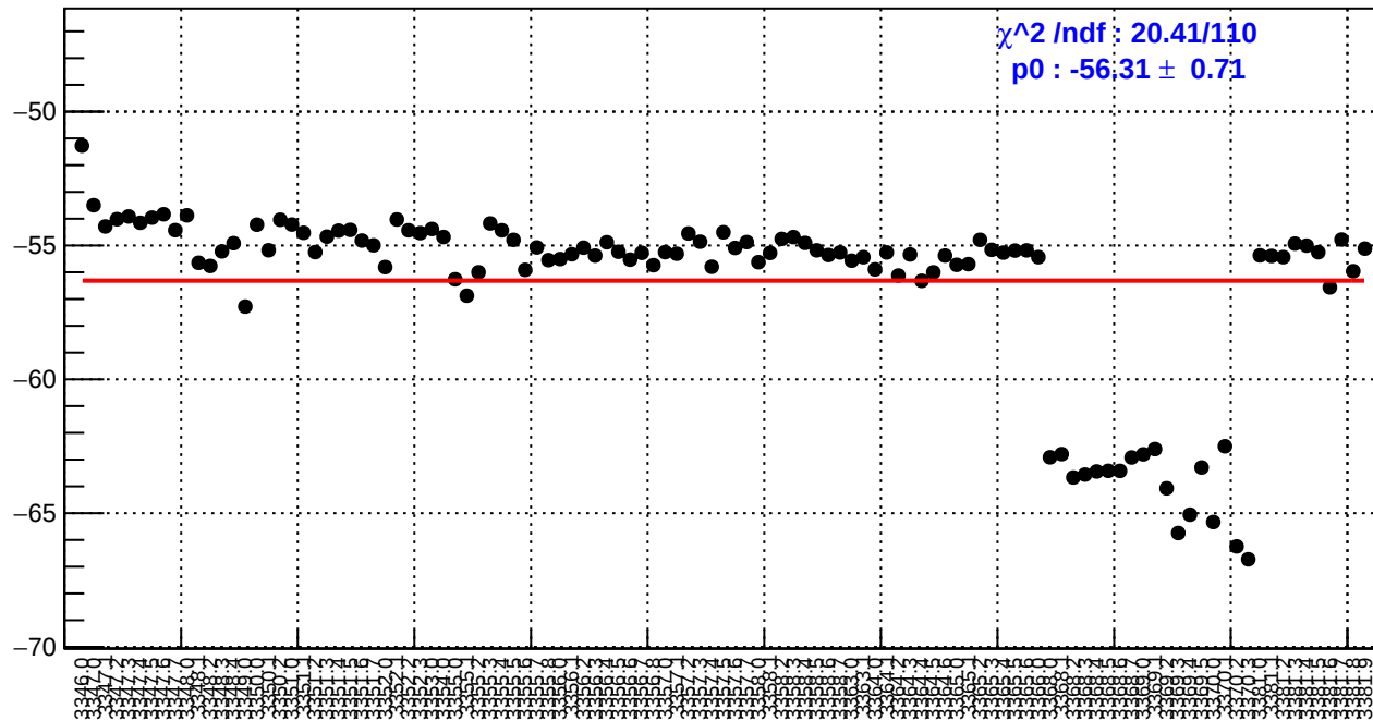
slug2: right_avg_bpm12X/(ppb/nm)
