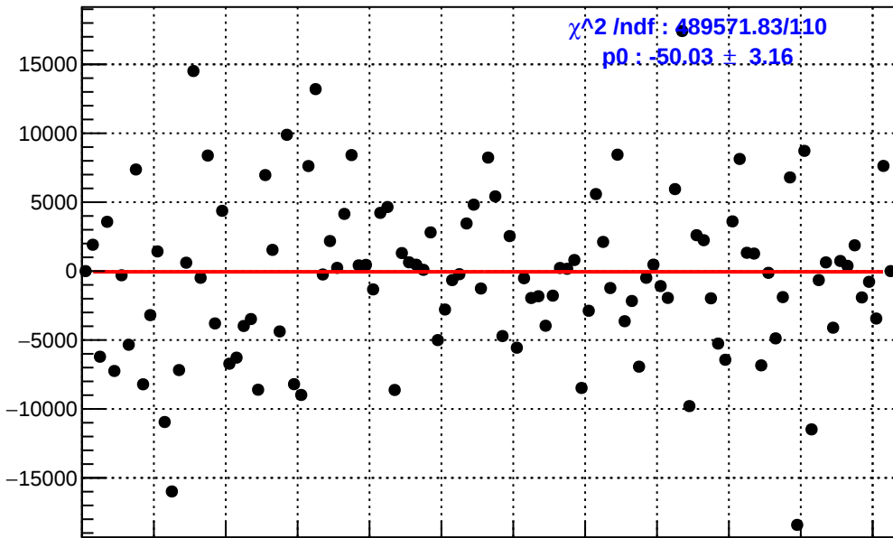
slug2: asym_dsr.mean/ppb-reg_asym_dsr.mean/ppb
