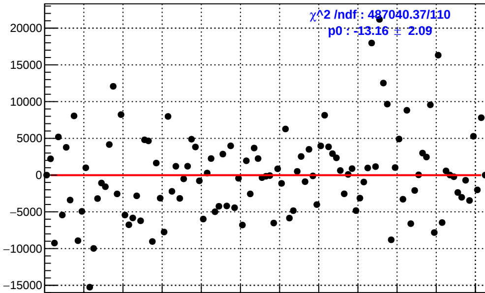
slug2: asym_sam1.mean/ppb-reg_asym_sam1.mean/ppb
