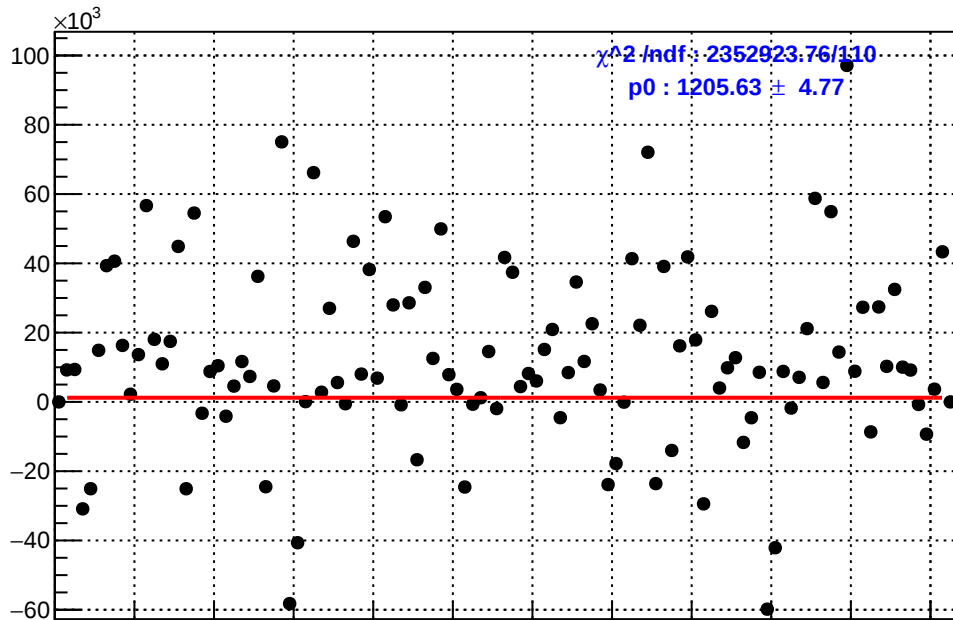
slug2: asym_sam6.mean/ppb-reg_asym_sam6.mean/ppb
