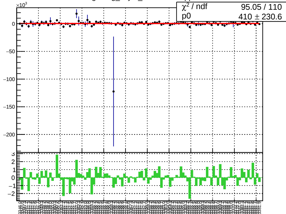
slug2: reg_asym_sam8.mean/ppb
