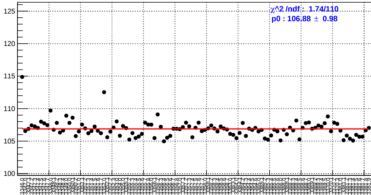
slug2: reg_asym_us_dd.rms/ppm
