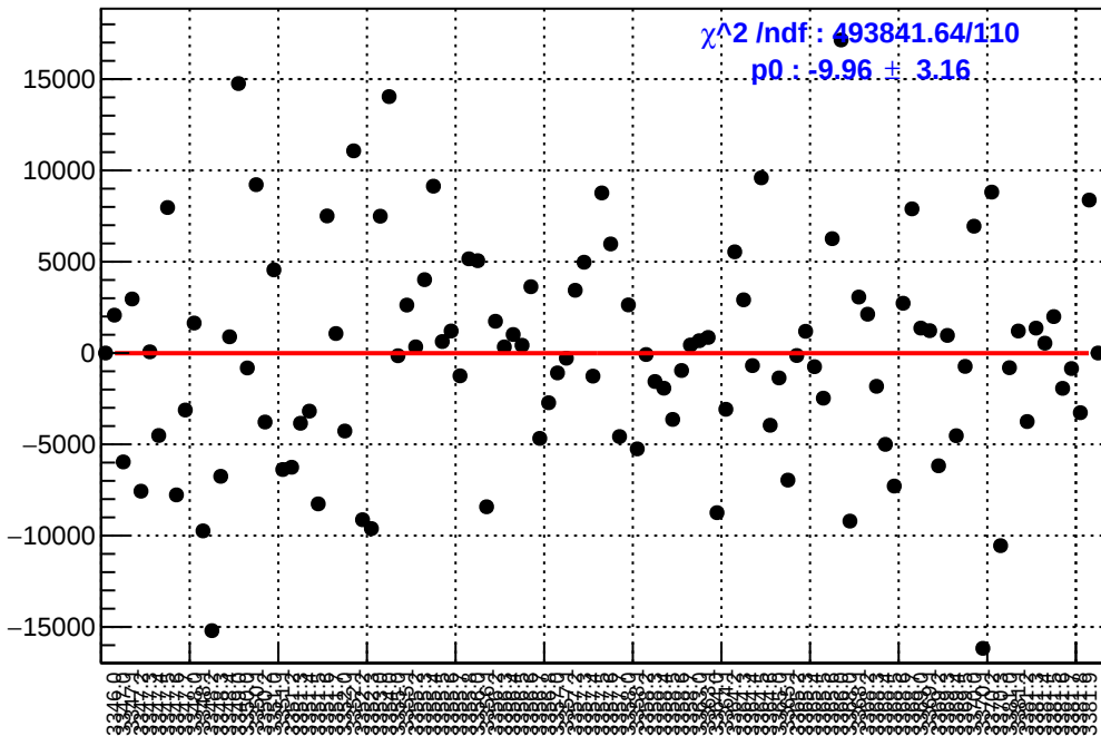
slug2: asym_right_avg.mean/ppb-reg_asym_right_avg.mean/ppb
