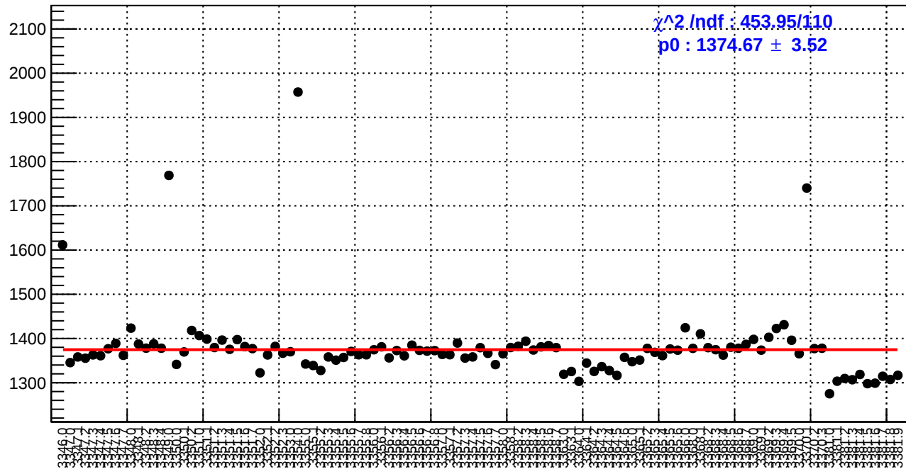
slug2: reg_asym_sam4.rms/ppm
