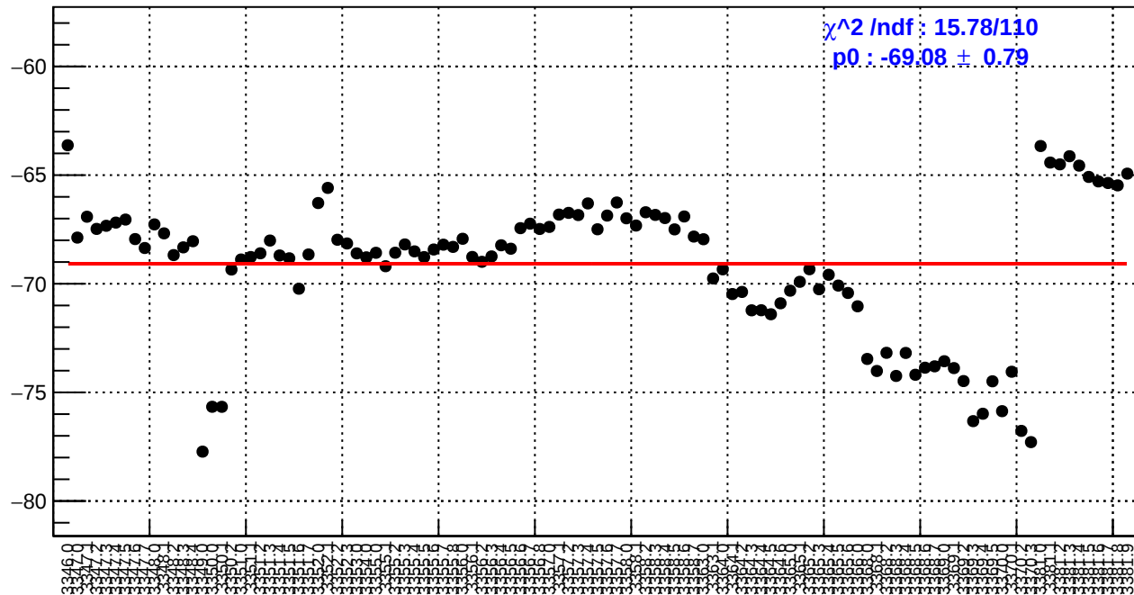
slug2: left_avg_bpm4eX/(ppb/nm)
