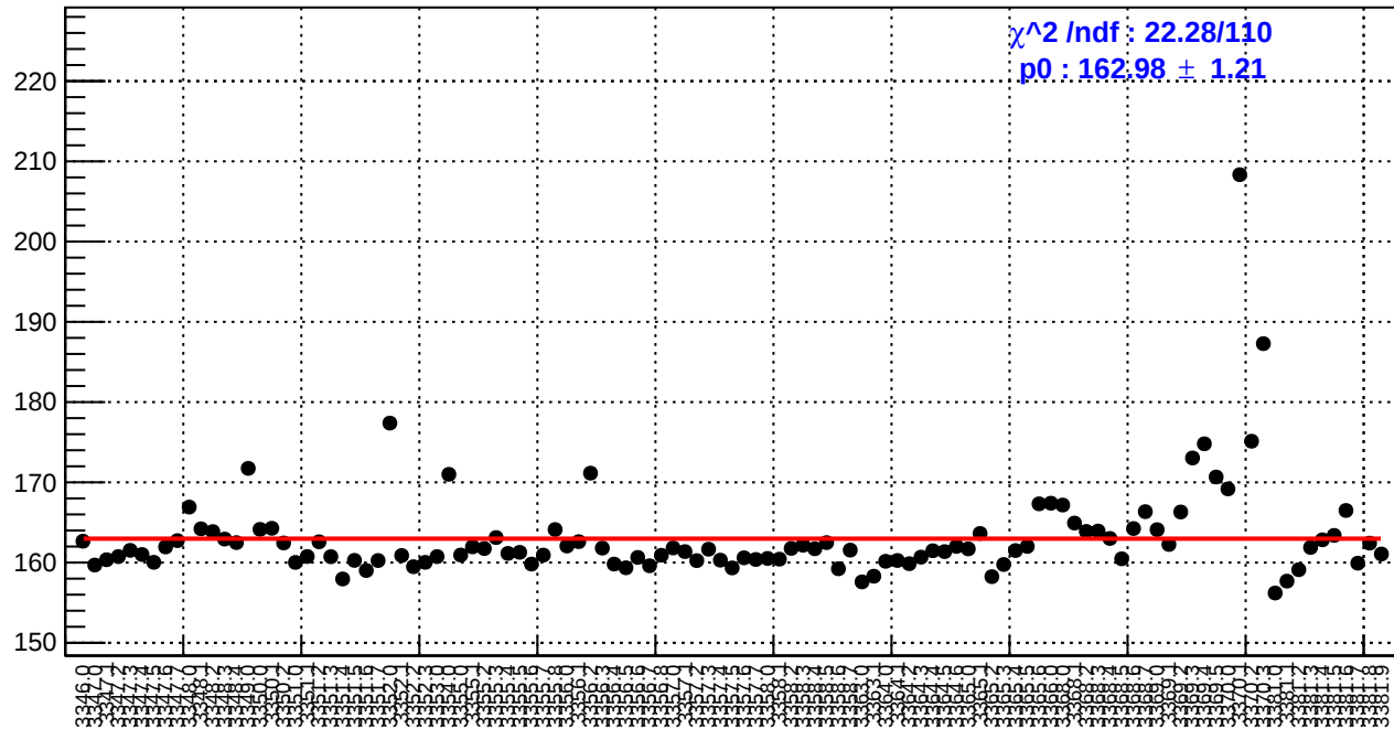
slug2: reg_asym_left_avg.rms/ppm
