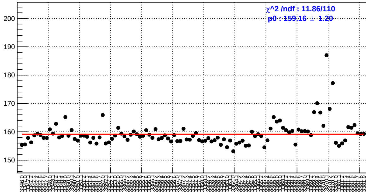
slug2: reg_asym_usr.rms/ppm
