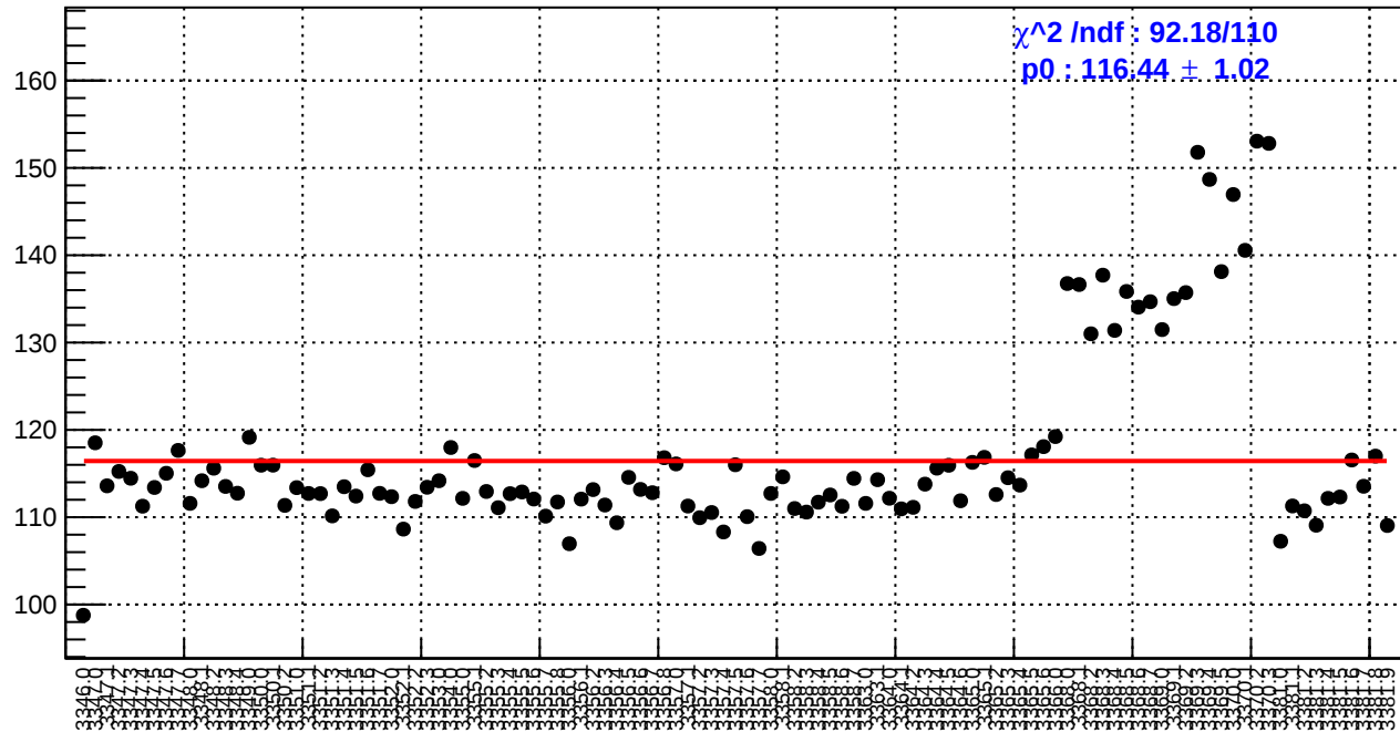
slug2: left_avg_bpm4aX/(ppb/nm)
