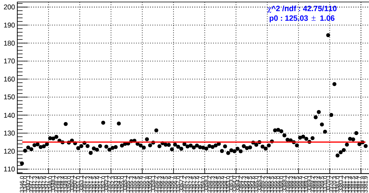
slug2: reg_asym_ds_avg.rms/ppm
