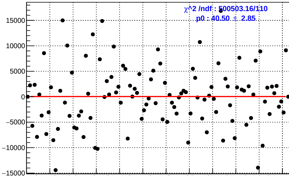
slug2: asym_usr.mean/ppb-reg_asym_usr.mean/ppb
