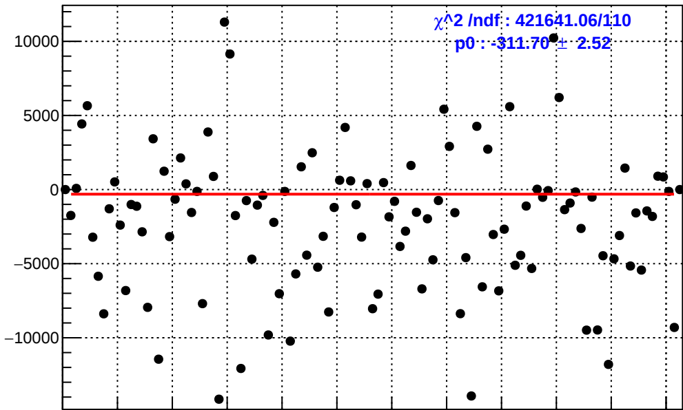
slug2: asym_ds_dd.mean/ppb-reg_asym_ds_dd.mean/ppb
