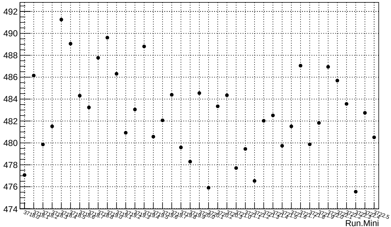
reg_asym_usl.rms/ppm
