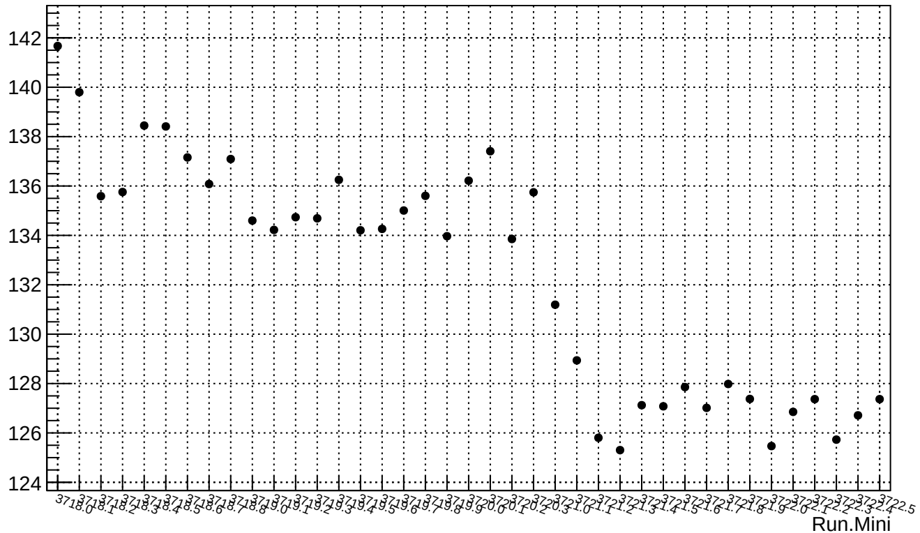
reg_asym_sam_15_avg.rms/ppm
