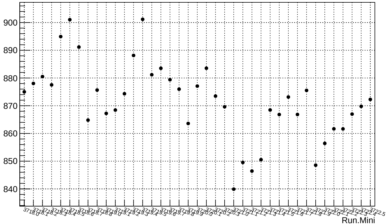
reg_asym_sam_26_dd.rms/ppm
