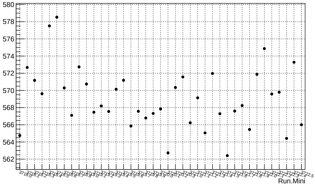
reg_asym_dsl.rms/ppm
