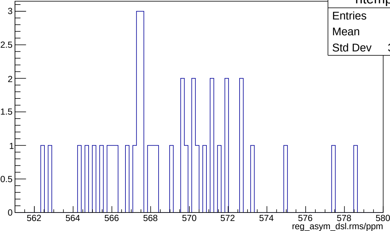
reg_asym_dsl.rms/ppm
