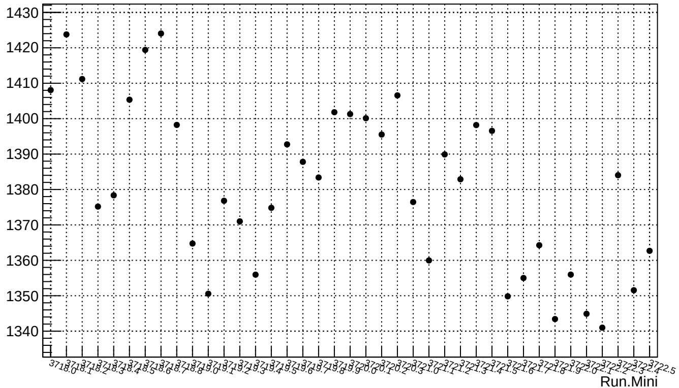
bcm_an_us_ds3_dd.rms/ppm
