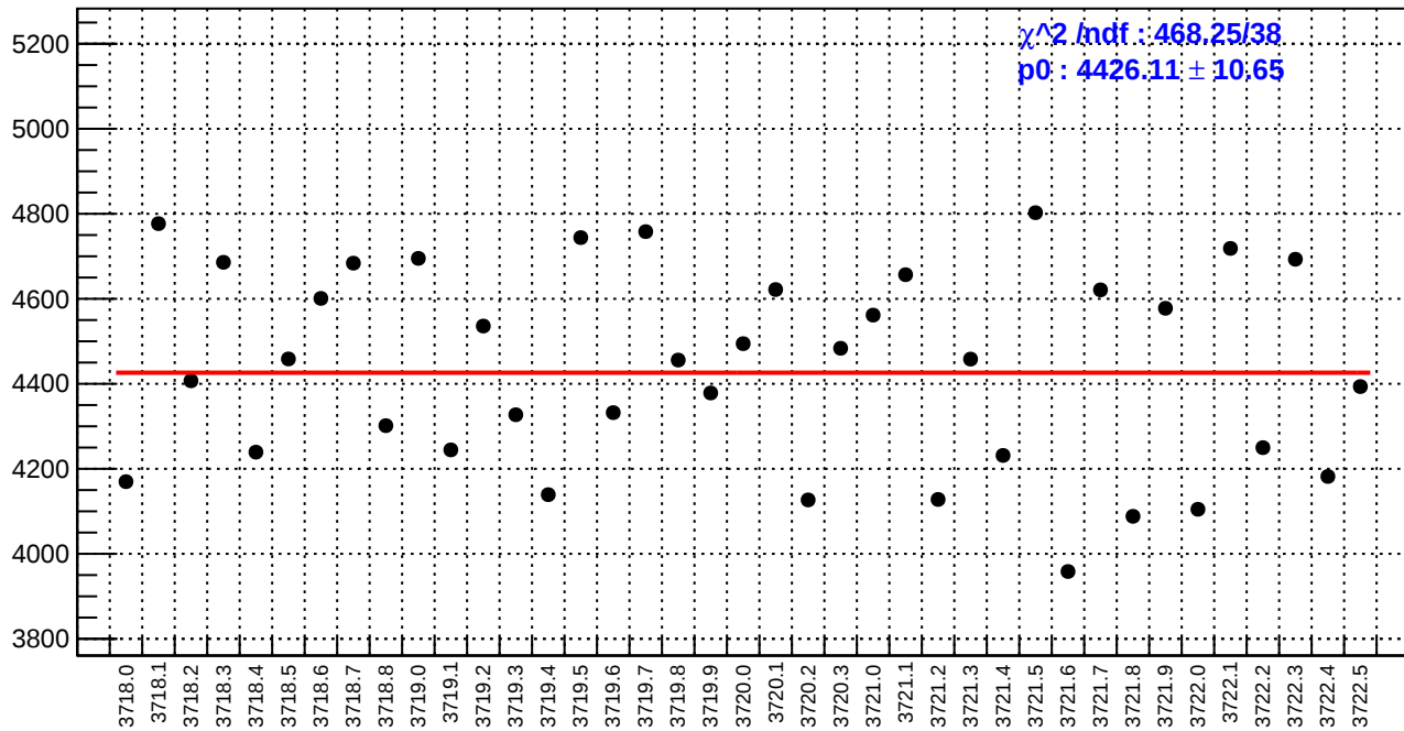
slug20: diff_bpm4eY.rms/nm
