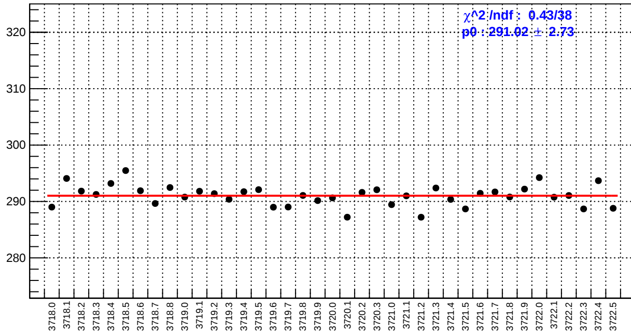
slug20: reg_asym_ds_dd.rms/ppm
