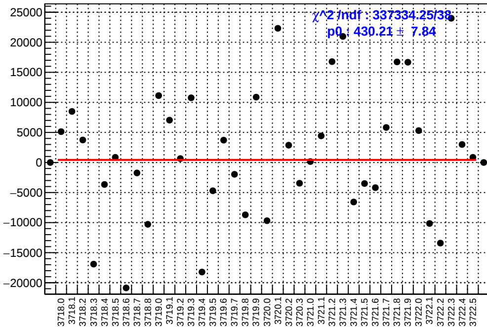
slug20: asym_sam5.mean/ppb-reg_asym_sam5.mean/ppb
