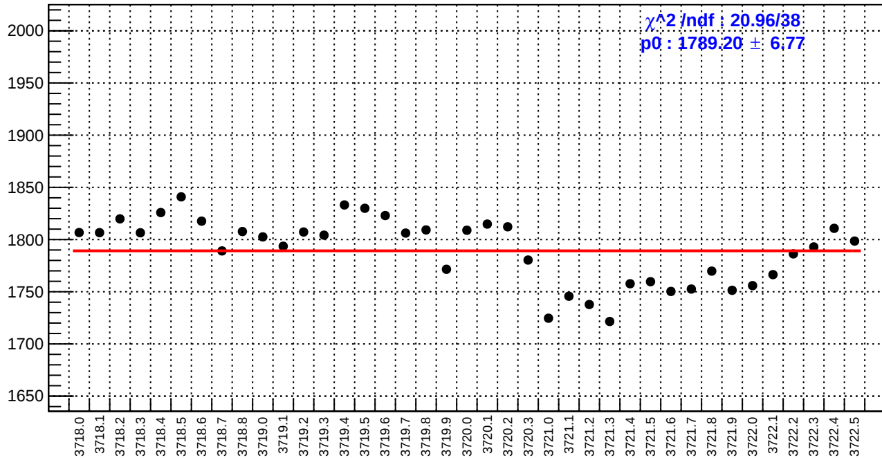
slug20: reg_asym_sam2.rms/ppm
