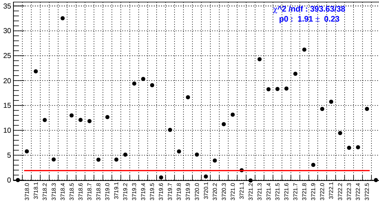
slug20: dsl_bpm4aX/(ppb/nm)
