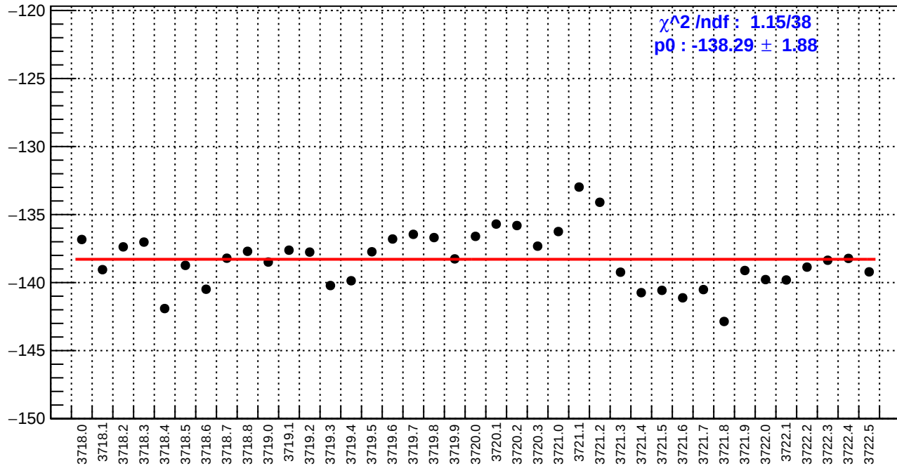
slug20: left_avg_bpm4eX/(ppb/nm)
