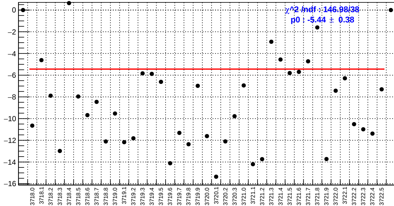
slug20: ds_avg_bpm4aX/(ppb/nm)
