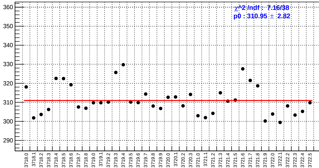
slug20: reg_asym_sam7.rms/ppm
