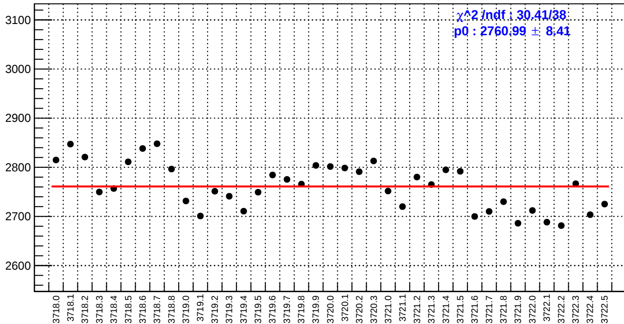
slug20: asym_bcm_an_us.rms/ppm
