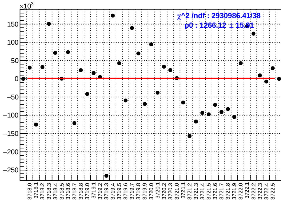
slug20: asym_sam3.mean/ppb-reg_asym_sam3.mean/ppb
