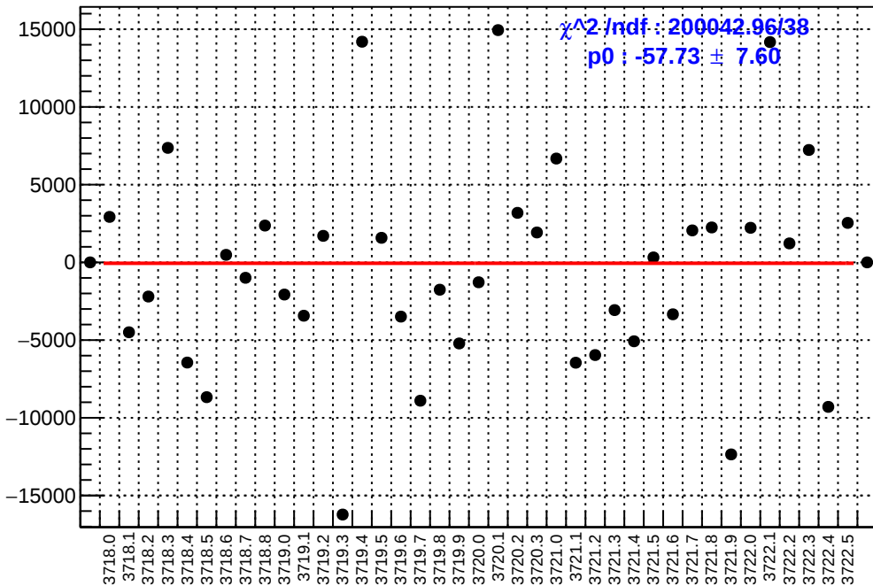
slug20: asym_ds_avg.mean/ppb-reg_asym_ds_avg.mean/ppb
