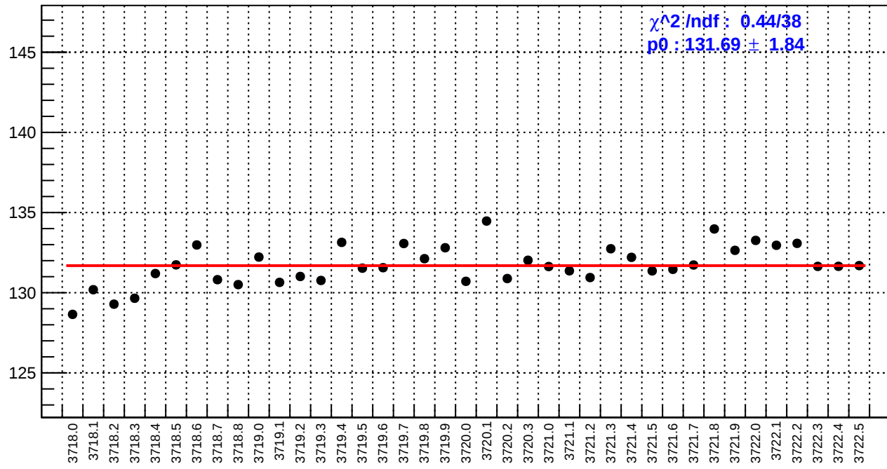
slug20: reg_asym_right_avg.rms/ppm
