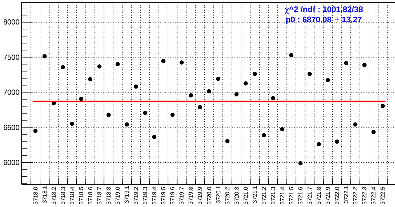
slug20: diff_bpm4aY.rms/nm
