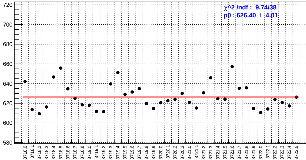
slug20: reg_asym_sam3.rms/ppm
