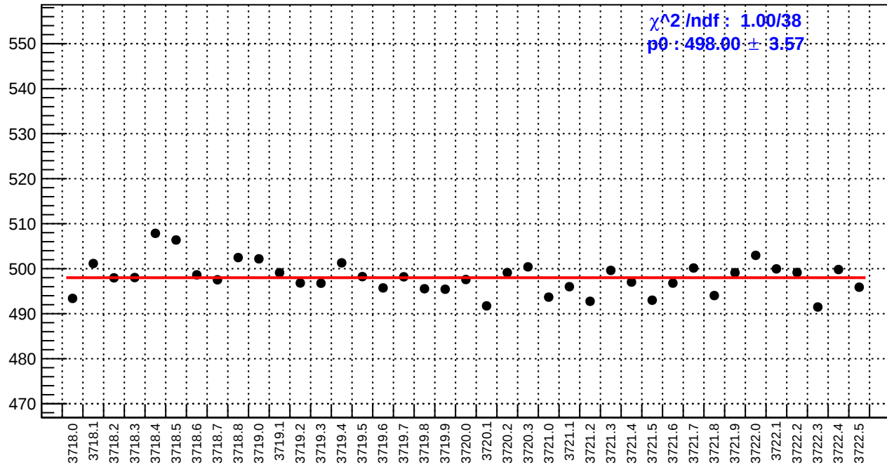
slug20: reg_asym_left_avg.rms/ppm
