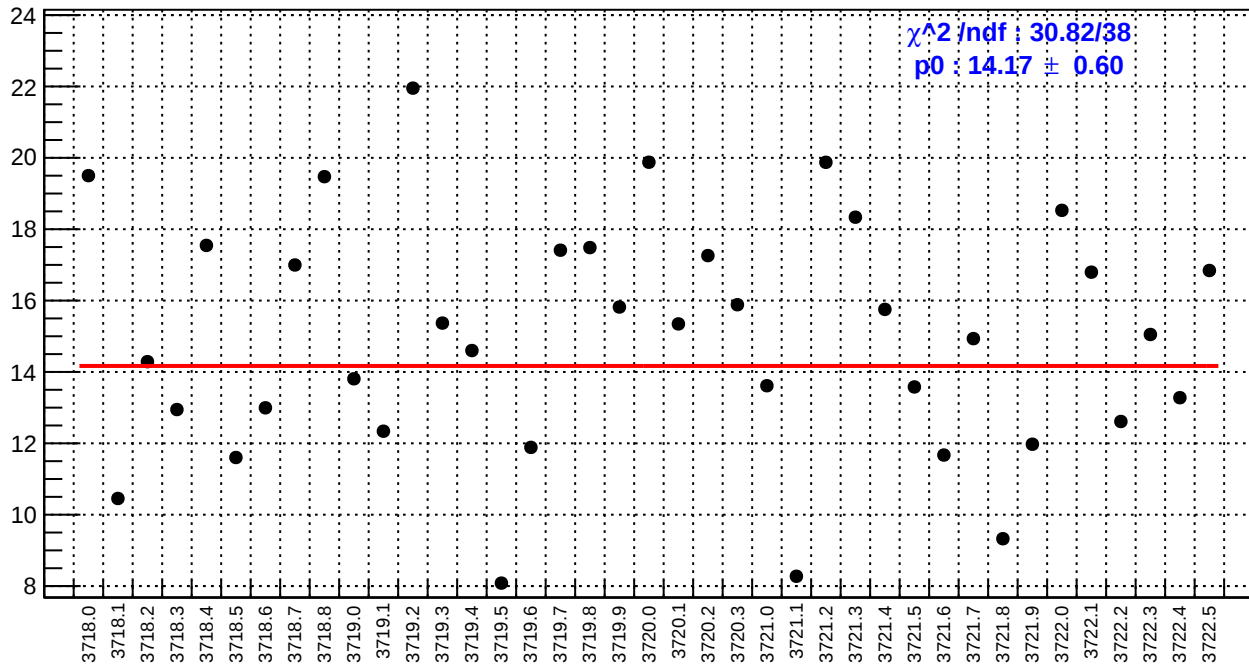
slug20: ds_avg_bpm4eY/(ppb/nm)
