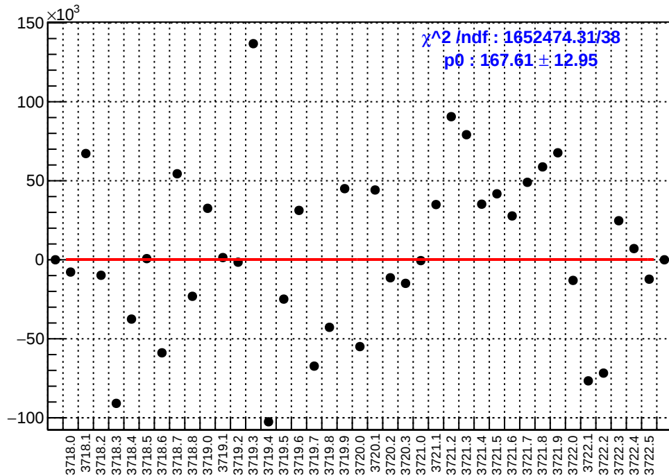
slug20: asym_sam6.mean/ppb-reg_asym_sam6.mean/ppb
