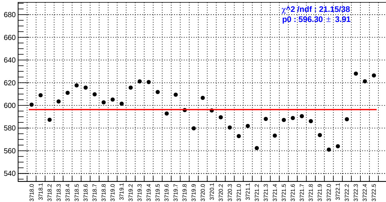
slug20: reg_asym_sam8.rms/ppm
