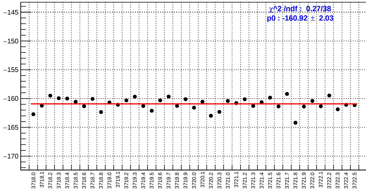
slug20: dsl_bpm12X/(ppb/nm)
