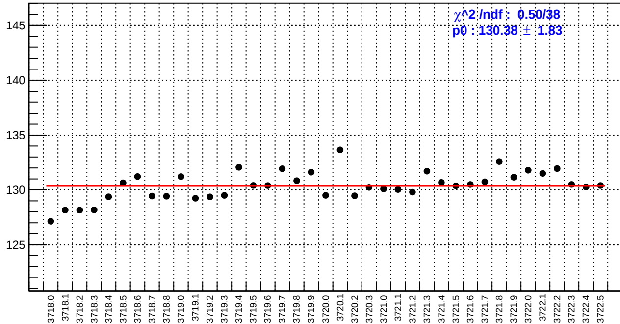
slug20: reg_asym_dsr.rms/ppm
