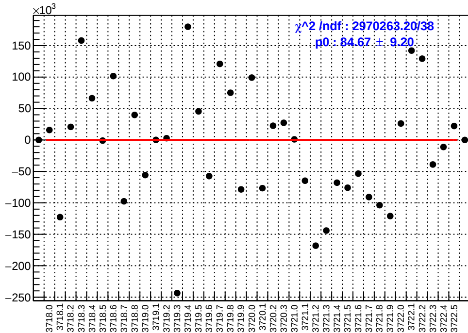
slug20: asym_sam2.mean/ppb-reg_asym_sam2.mean/ppb
