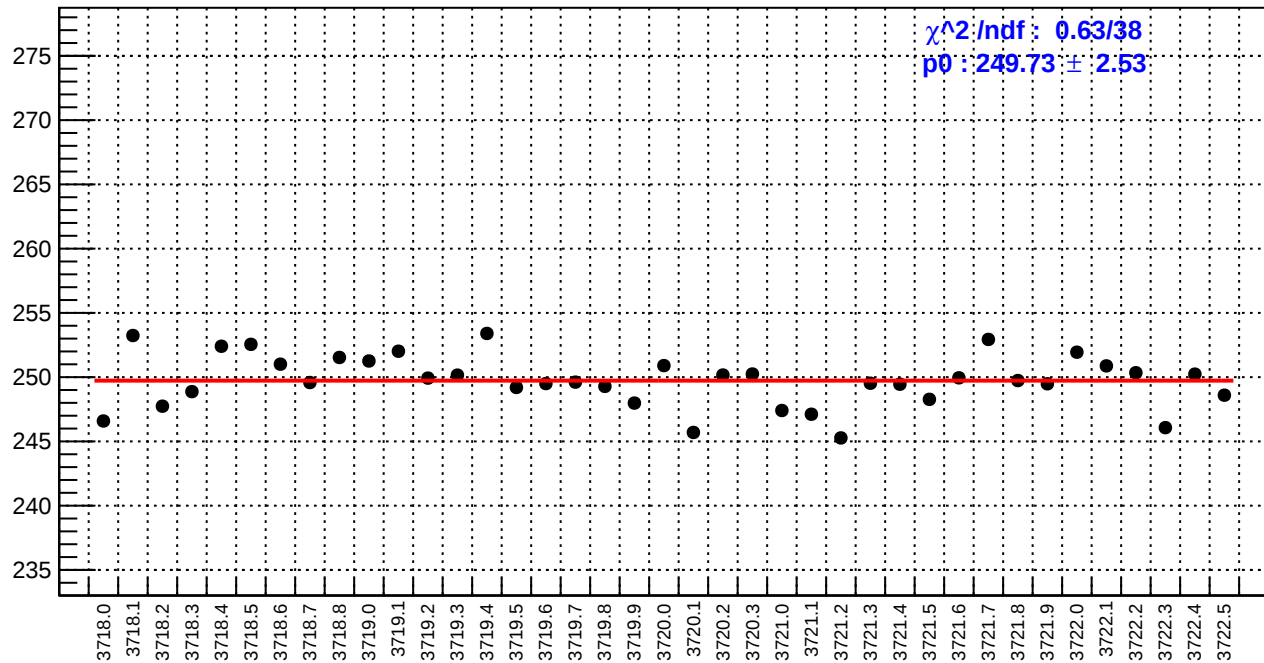
slug20: reg_asym_us_dd.rms/ppm
