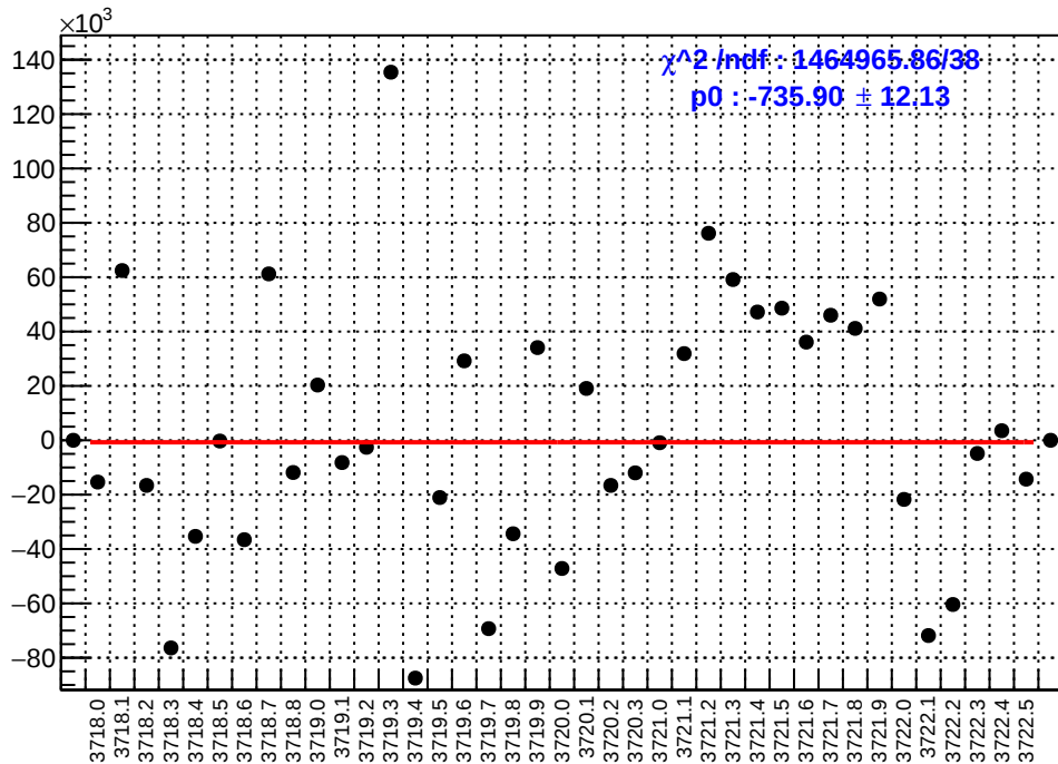
slug20: asym_sam7.mean/ppb-reg_asym_sam7.mean/ppb
