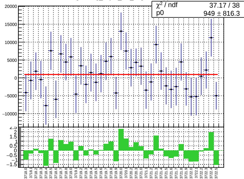
slug20: reg_asym_left_avg.mean/ppb
