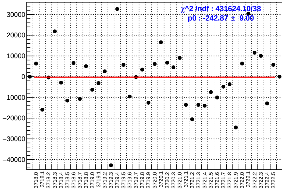
slug20: asym_usl.mean/ppb-reg_asym_usl.mean/ppb
