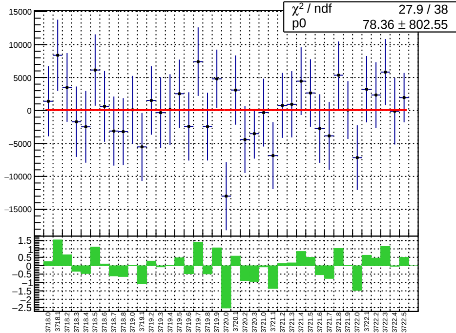
slug20: reg_asym_sam1.mean/ppb
