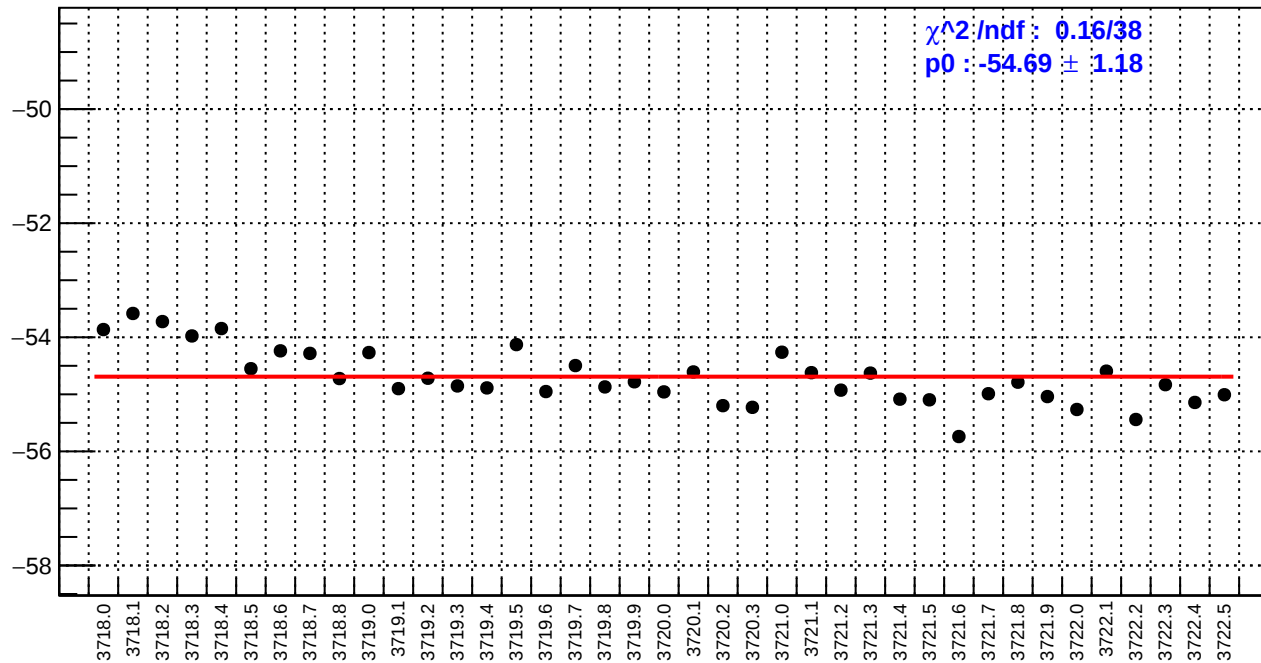
slug20: dsr_bpm12X/(ppb/nm)
