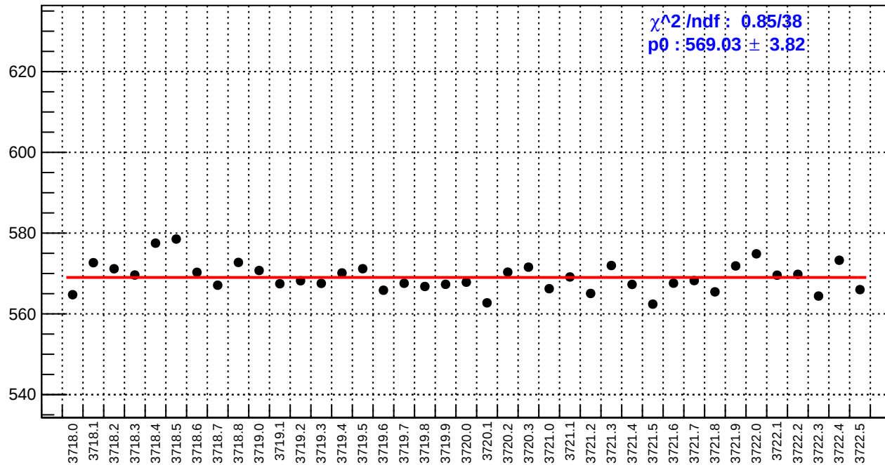
slug20: reg_asym_dsl.rms/ppm
