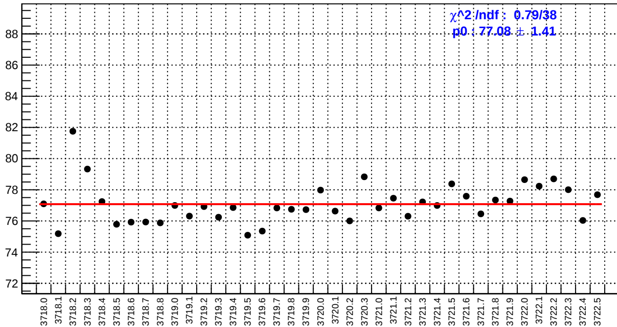
slug20: asym_bcm_an_ds3.rms/ppm
