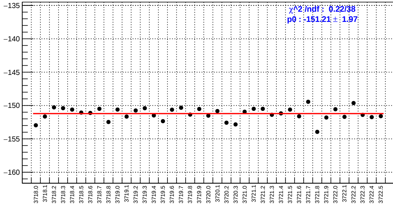
slug20: left_avg_bpm12X/(ppb/nm)
