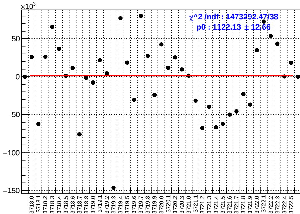
slug20: asym_sam4.mean/ppb-reg_asym_sam4.mean/ppb
