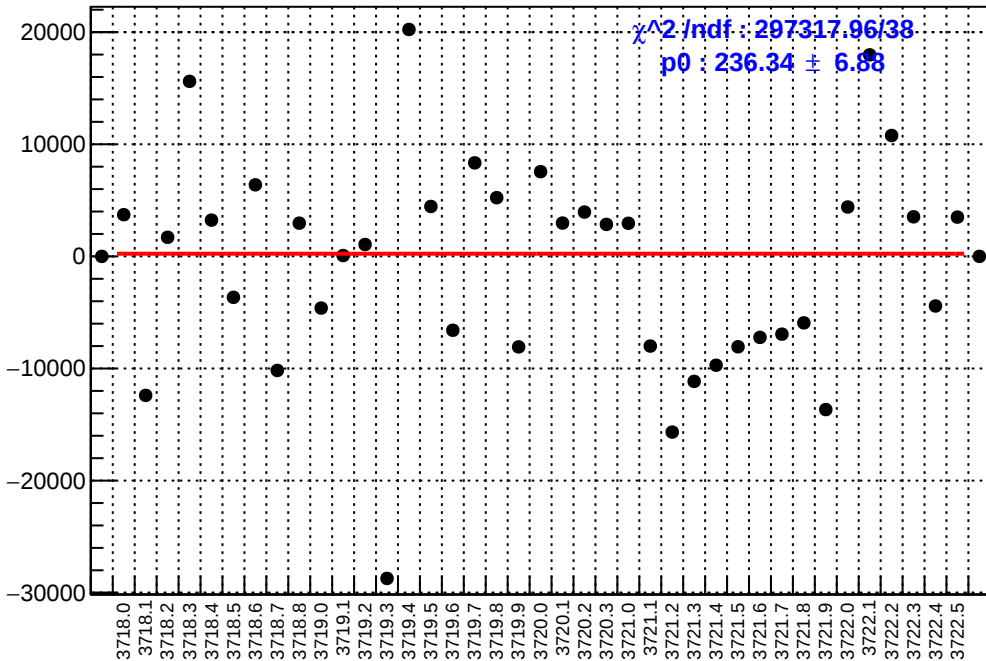
slug20: asym_us_dd.mean/ppb-reg_asym_us_dd.mean/ppb
