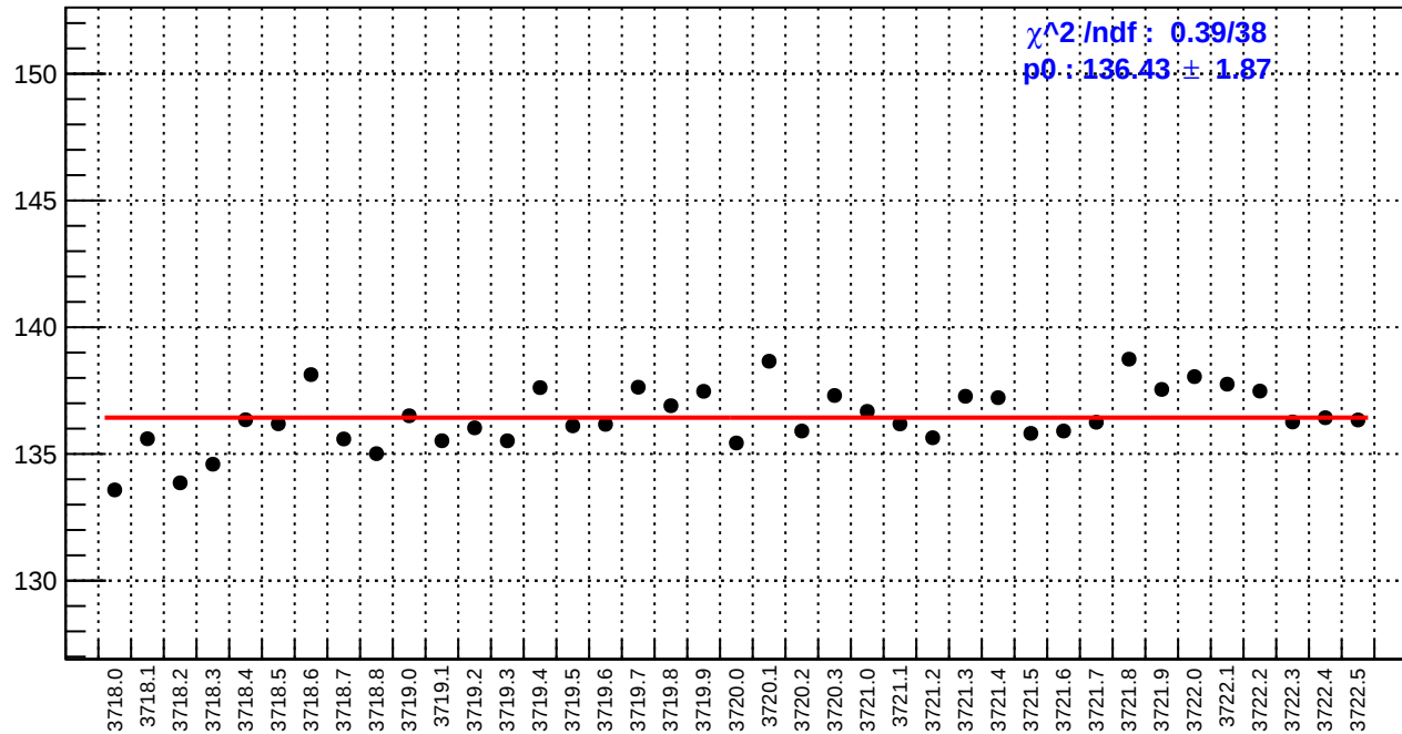
slug20: reg_asym_usr.rms/ppm
