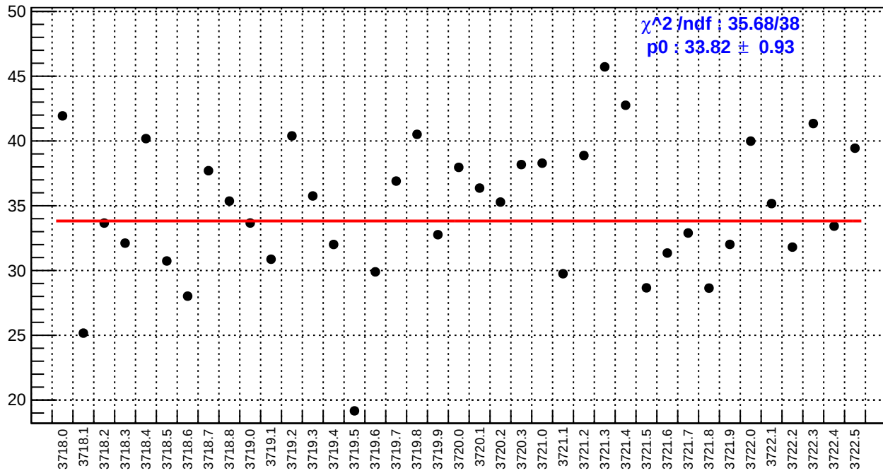
slug20: usl_bpm4eY/(ppb/nm)
