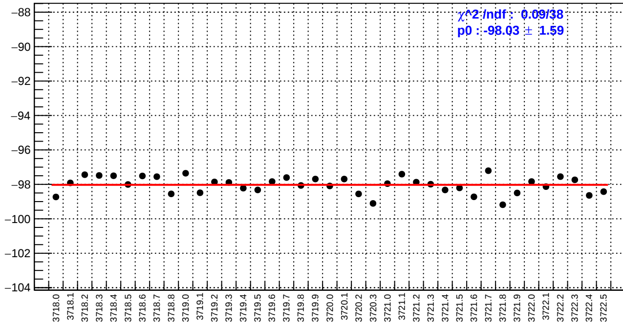
slug20: us_avg_bpm12X/(ppb/nm)
