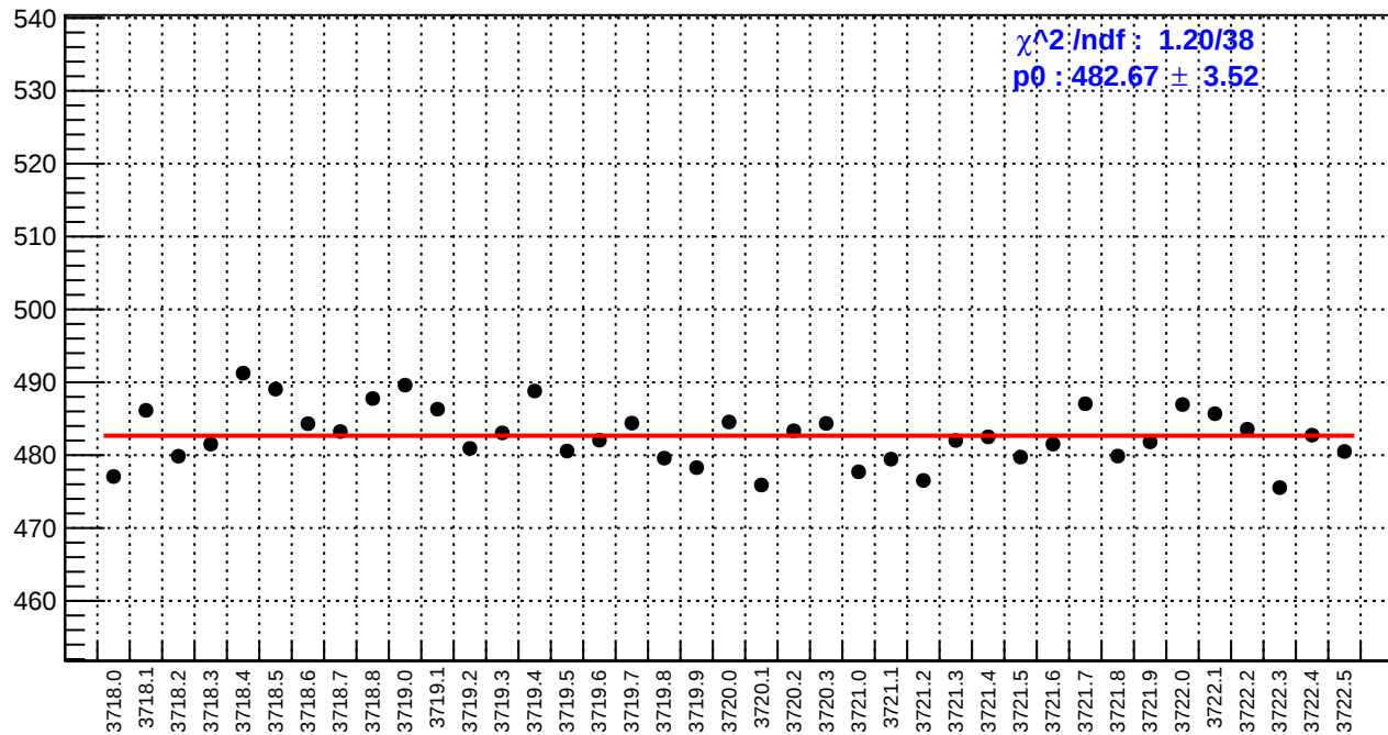
slug20: reg_asym_usl.rms/ppm
