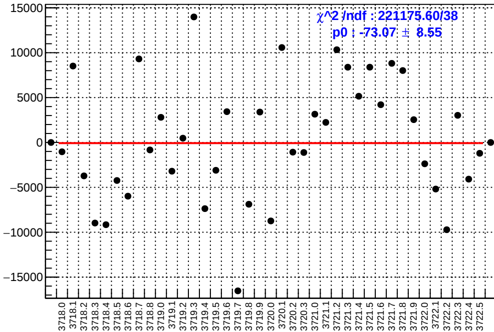
slug20: asym_right_avg.mean/ppb-reg_asym_right_avg.mean/ppb
