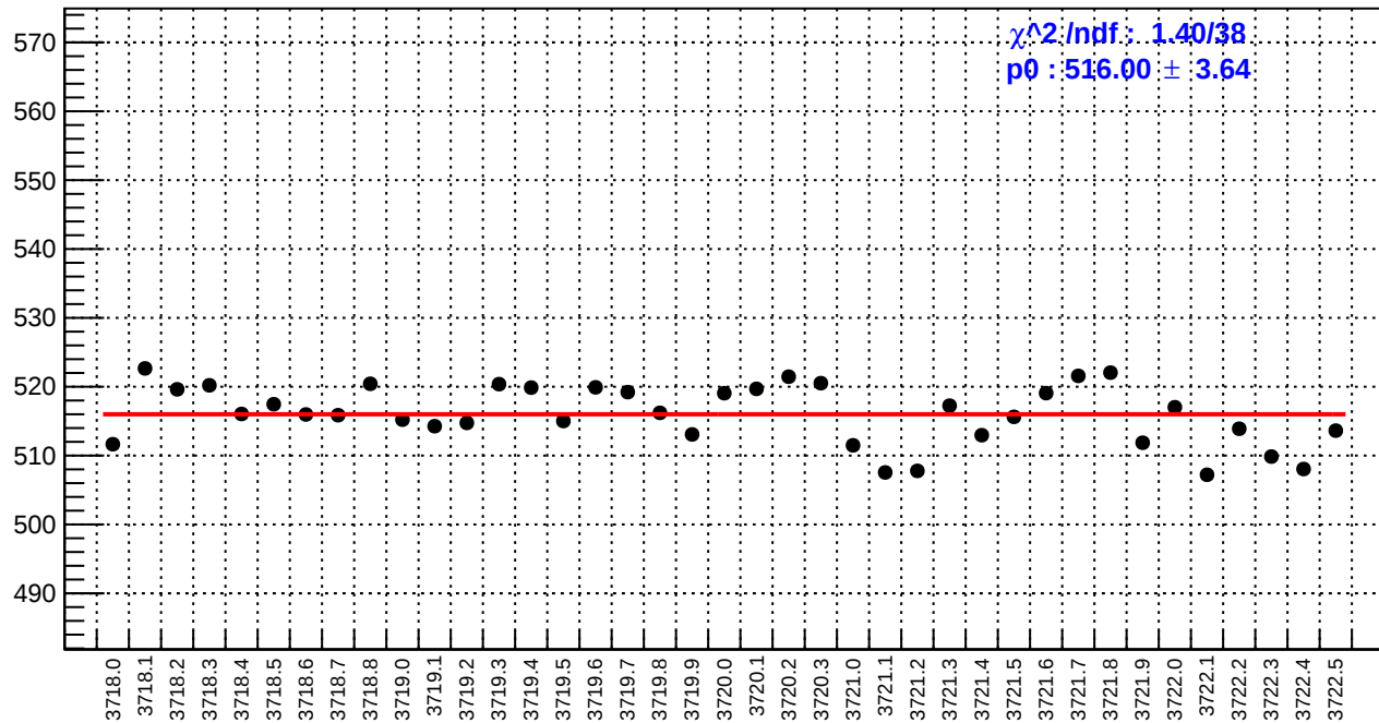
slug20: asym_bcm_an_ds.rms/ppm
