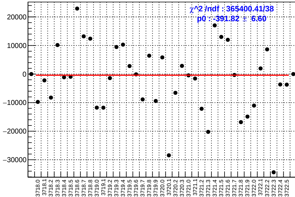
slug20: asym_sam1.mean/ppb-reg_asym_sam1.mean/ppb
