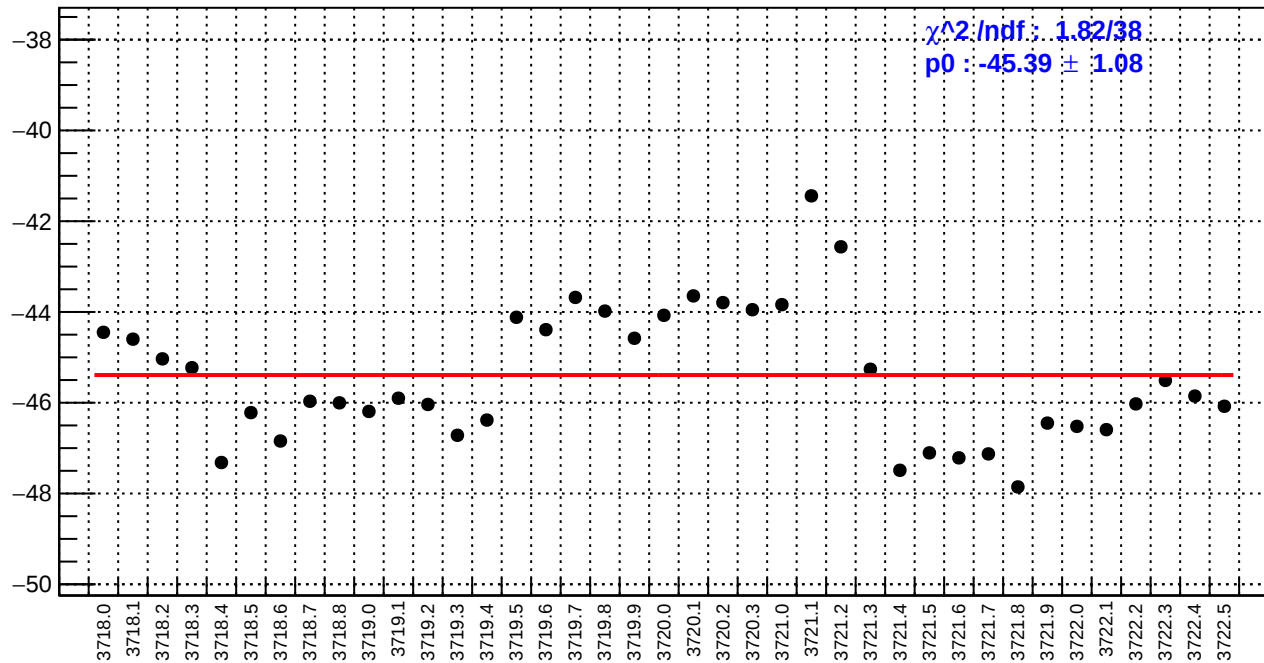
slug20: us_avg_bpm4eX/(ppb/nm)
