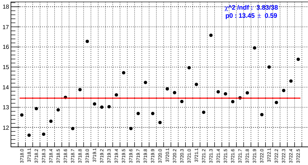
slug20: usr_bpm4aY/(ppb/nm)
