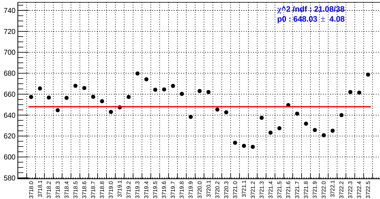
slug20: reg_asym_sam6.rms/ppm
