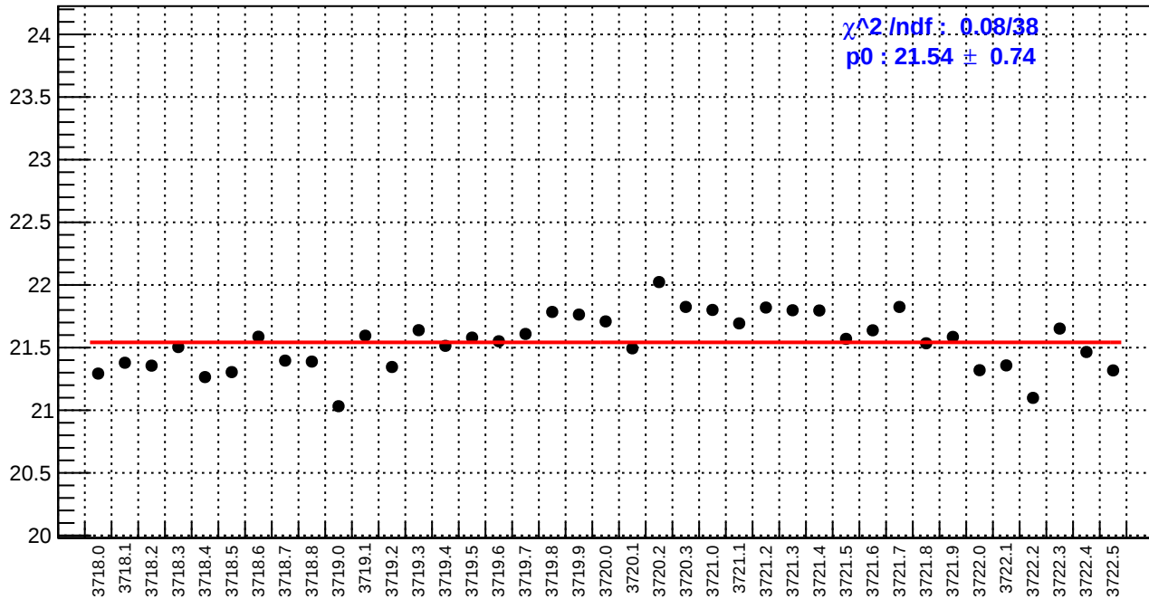
slug20: reg_asym_right_dd.rms/ppm
