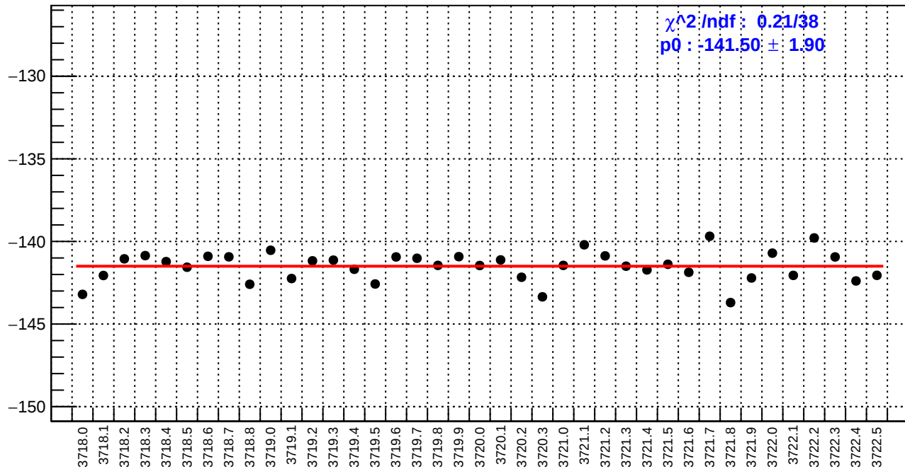
slug20: usl_bpm12X/(ppb/nm)
