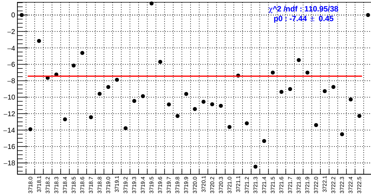
slug20: usl_bpm4aY/(ppb/nm)
