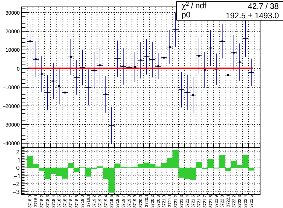
slug20: reg_asym_sam4.mean/ppb
