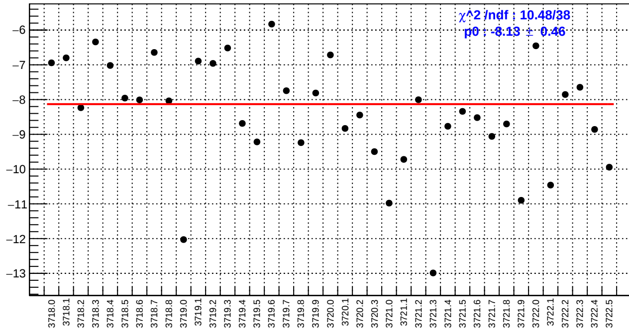
slug20: dsr_bpm4eY/(ppb/nm)
