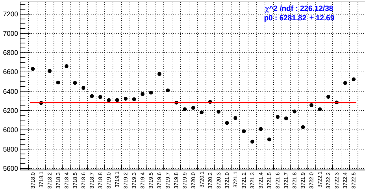
slug20: diff_bpm11X.rms/nm
