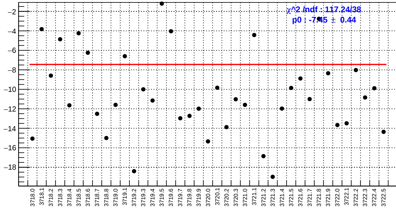
slug20: dsl_bpm4aY/(ppb/nm)
