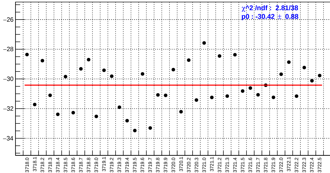
slug20: right_avg_bpm4aX/(ppb/nm)
