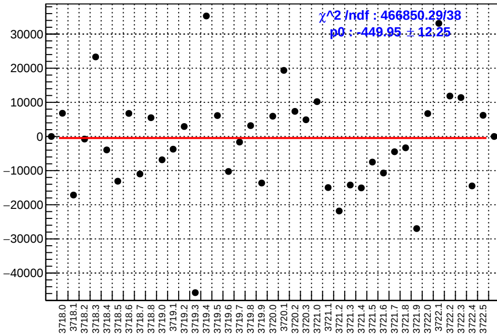
slug20: asym_dsl.mean/ppb-reg_asym_dsl.mean/ppb
