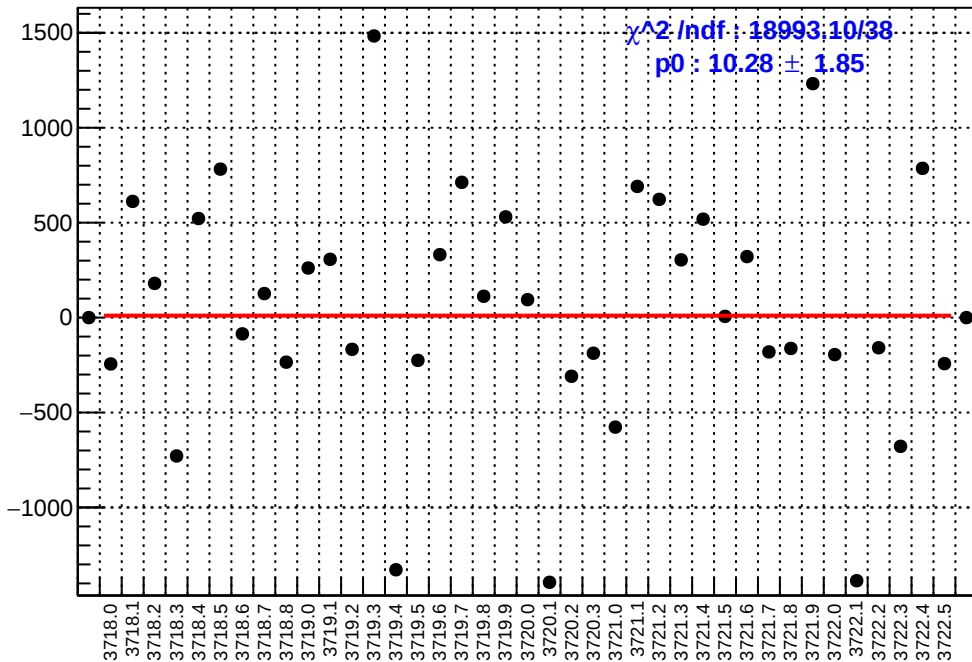
slug20: asym_left_dd.mean/ppb-reg_asym_left_dd.mean/ppb
