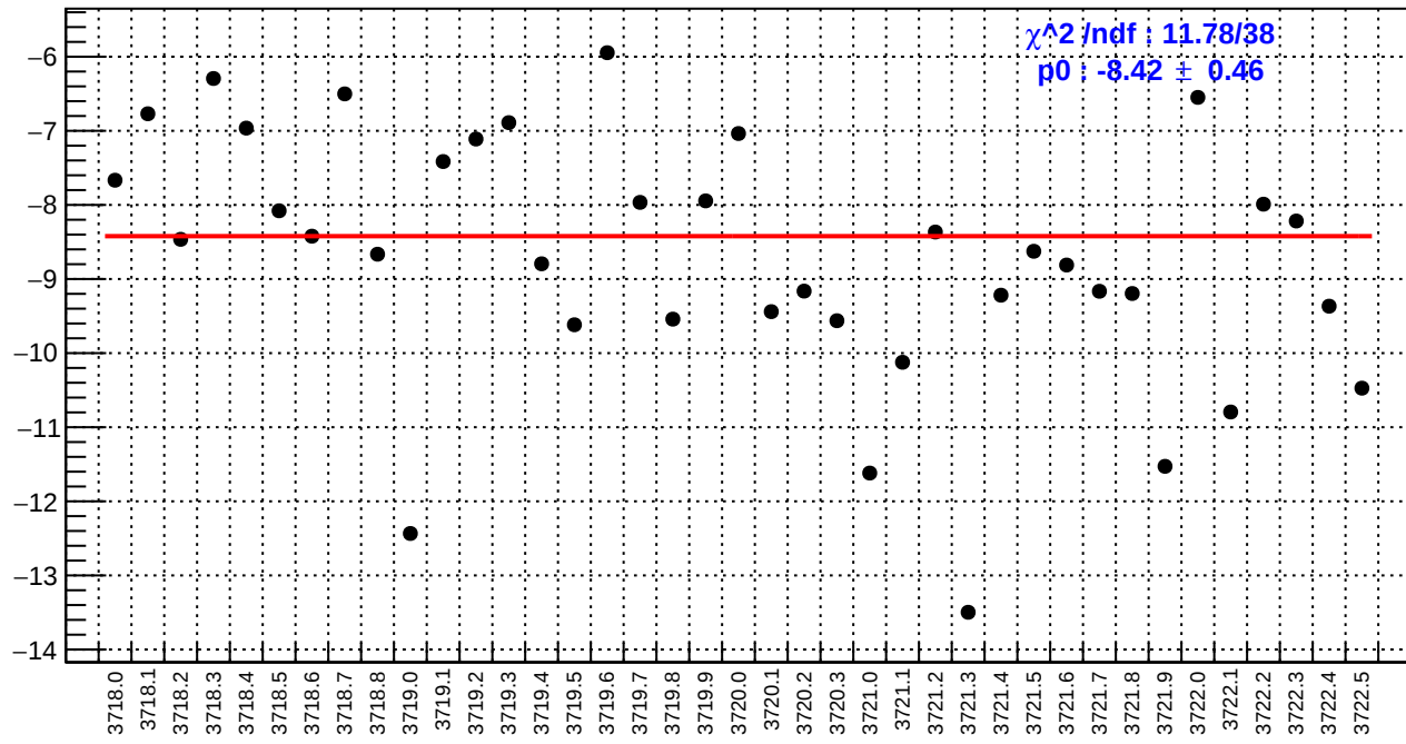
slug20: right_avg_bpm4eY/(ppb/nm)
