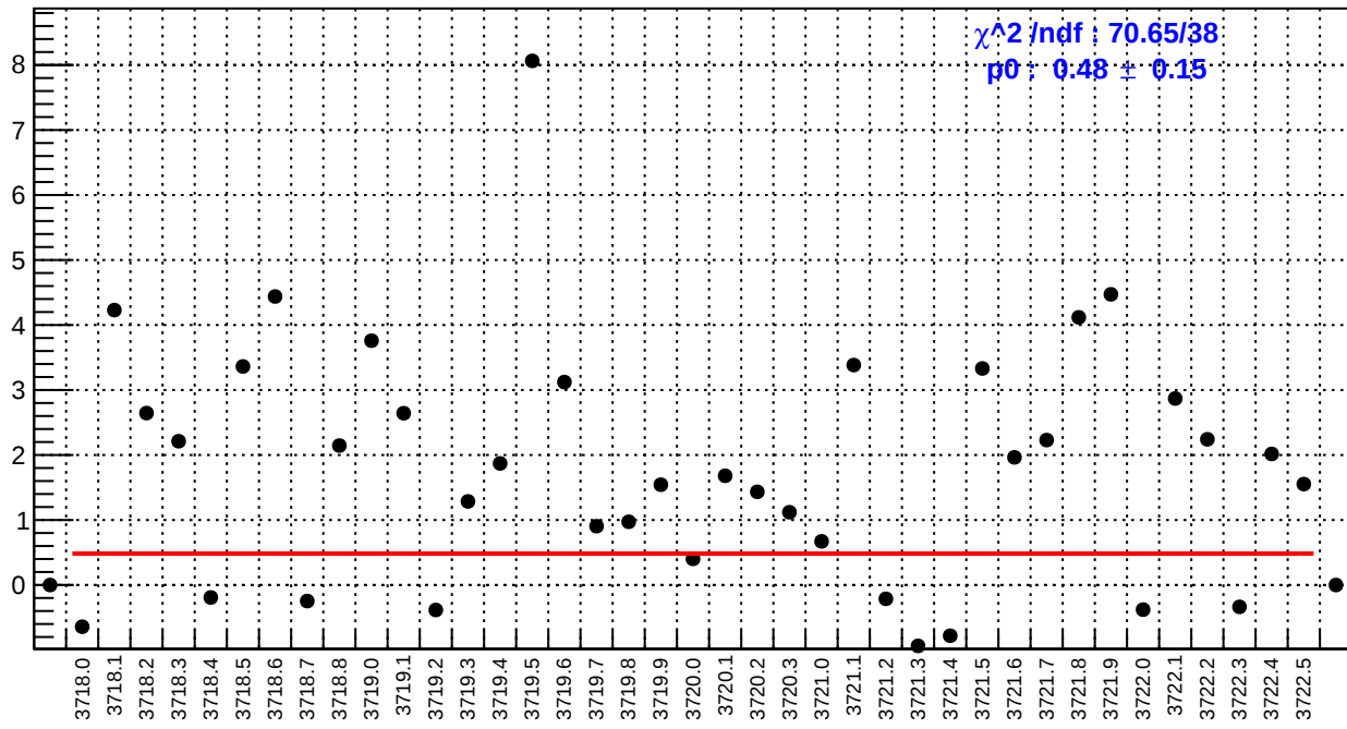
slug20: us_avg_bpm4aY/(ppb/nm)
