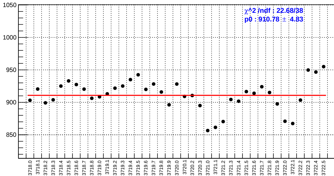
slug20: reg_asym_sam4.rms/ppm
