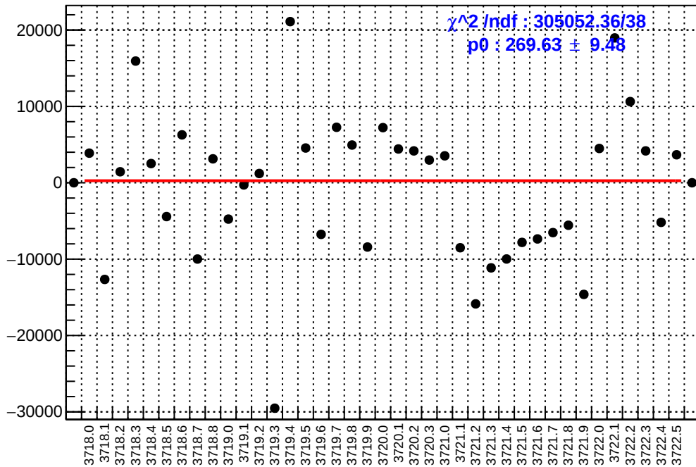
slug20: asym_ds_dd.mean/ppb-reg_asym_ds_dd.mean/ppb
