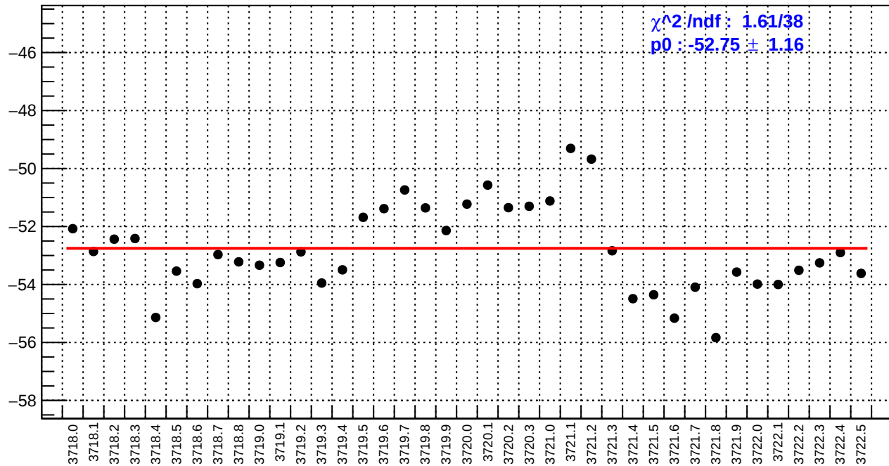
slug20: ds_avg_bpm4eX/(ppb/nm)
