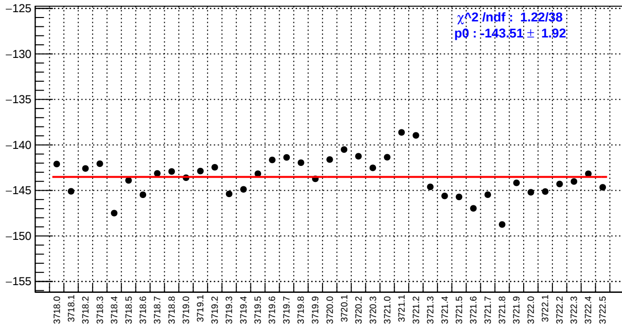
slug20: dsl_bpm4eX/(ppb/nm)
