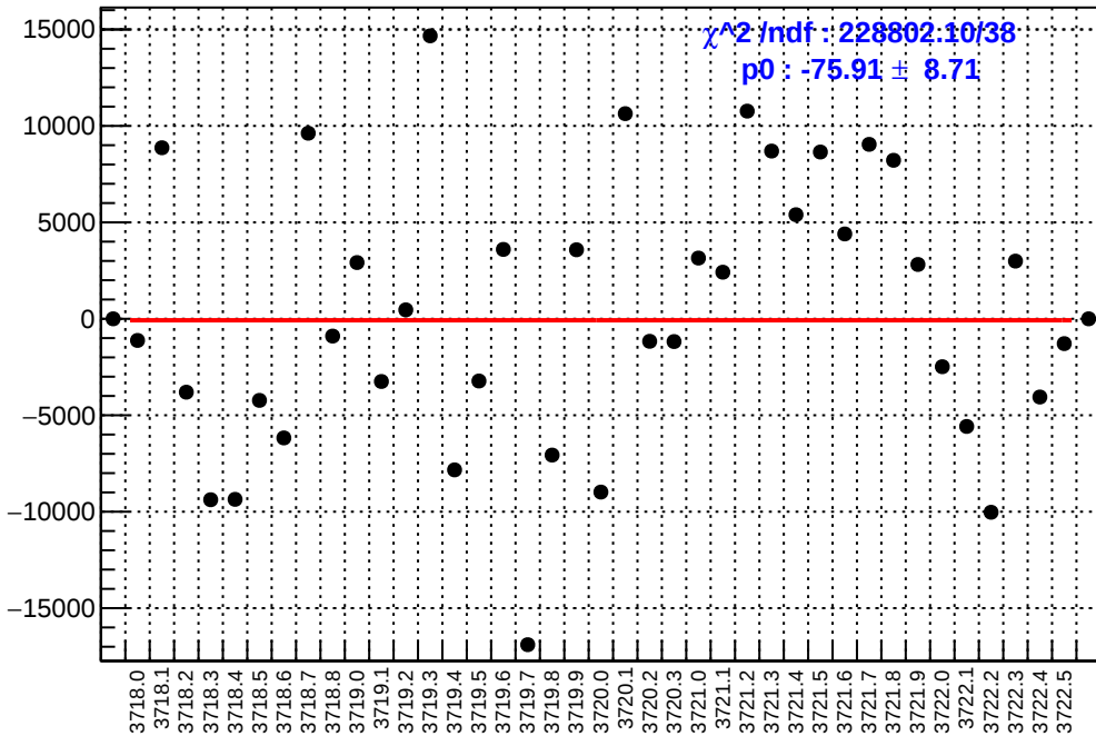
slug20: asym_usr.mean/ppb-reg_asym_usr.mean/ppb
