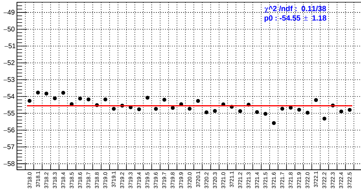
slug20: usr_bpm12X/(ppb/nm)
