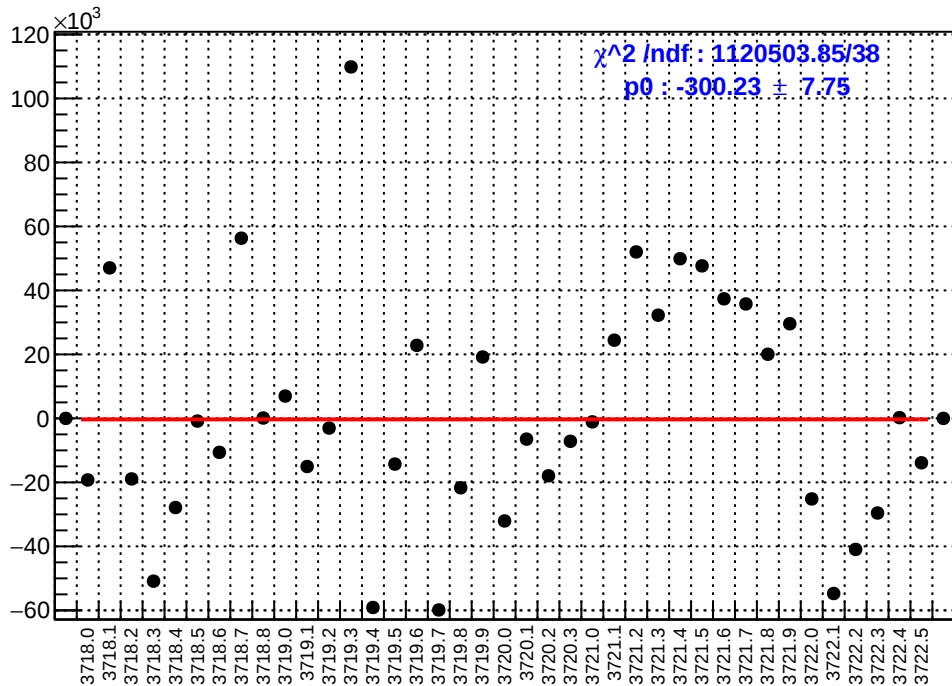
slug20: asym_sam8.mean/ppb-reg_asym_sam8.mean/ppb
