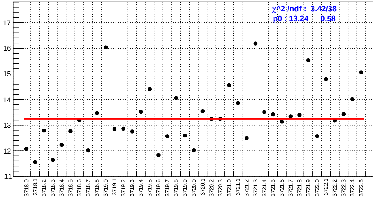
slug20: right_avg_bpm4aY/(ppb/nm)
