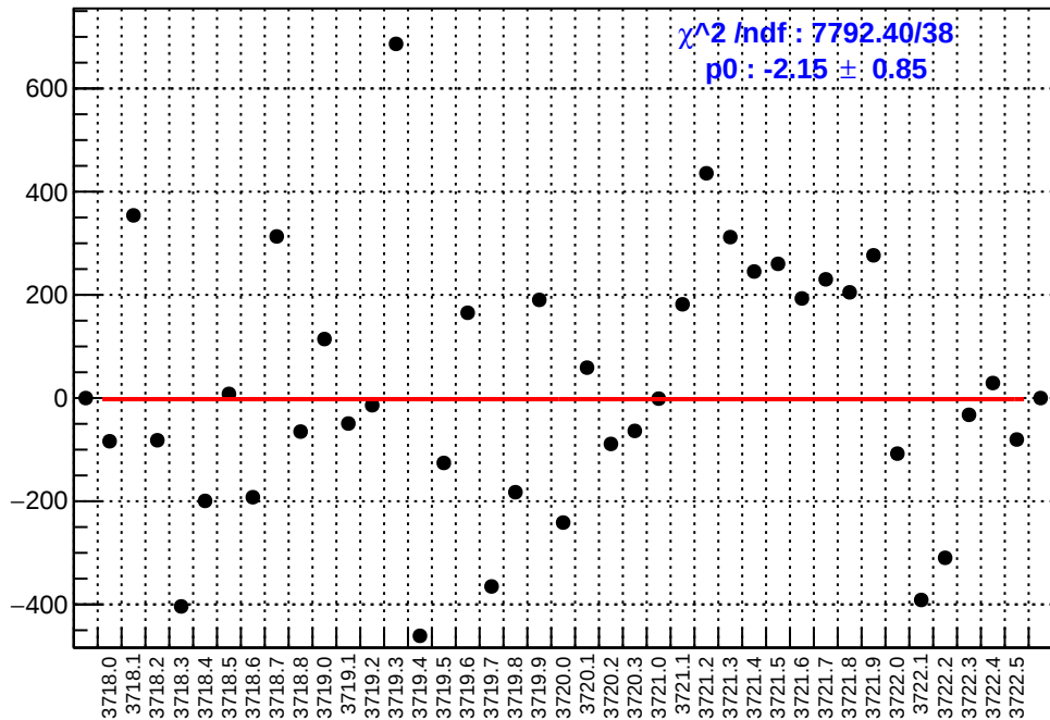
slug20: asym_right_dd.mean/ppb-reg_asym_right_dd.mean/ppb
