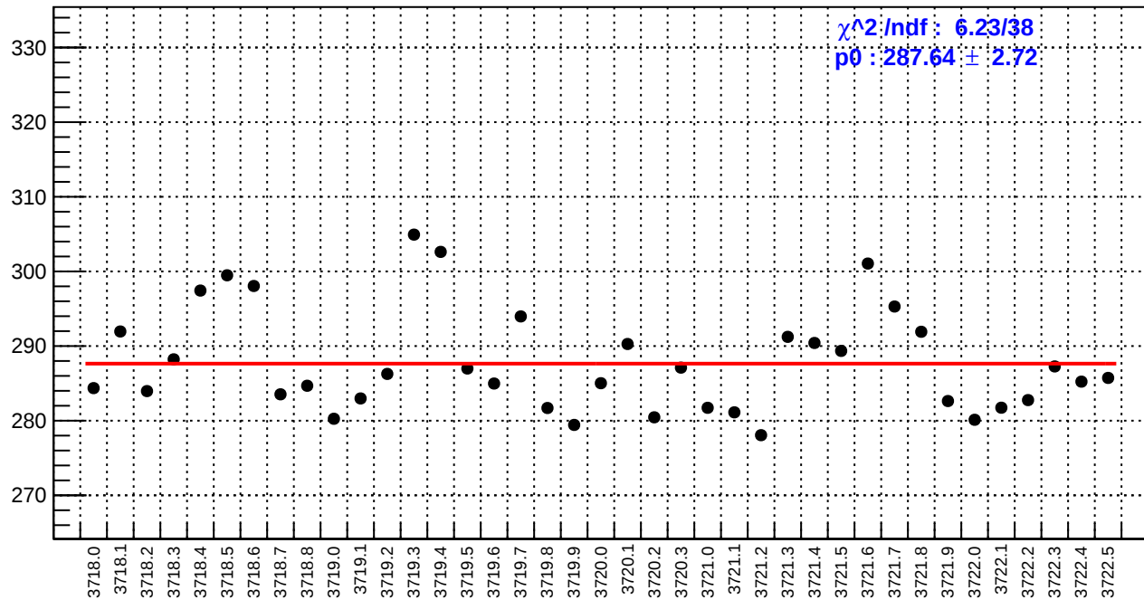
slug20: reg_asym_sam5.rms/ppm
