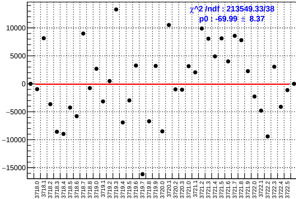
slug20: asym_dsr.mean/ppb-reg_asym_dsr.mean/ppb
