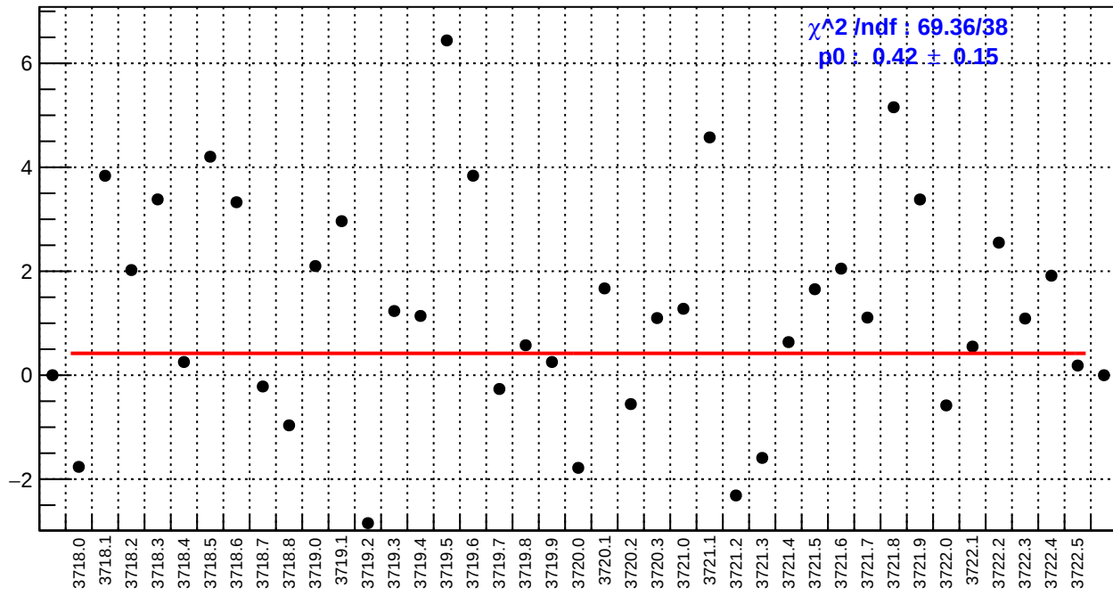
slug20: ds_avg_bpm4aY/(ppb/nm)
