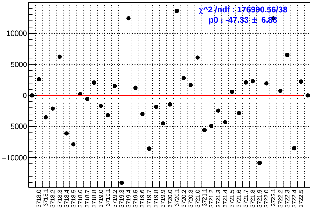
slug20: asym_us_avg.mean/ppb-reg_asym_us_avg.mean/ppb
