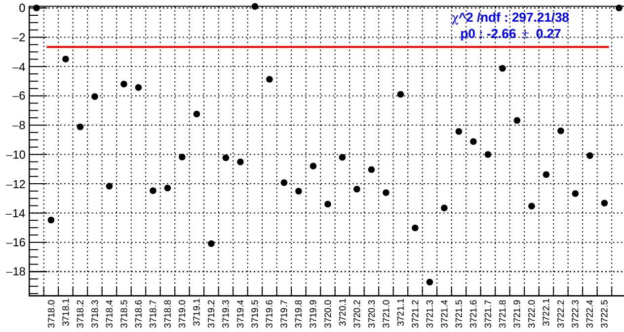
slug20: left_avg_bpm4aY/(ppb/nm)
