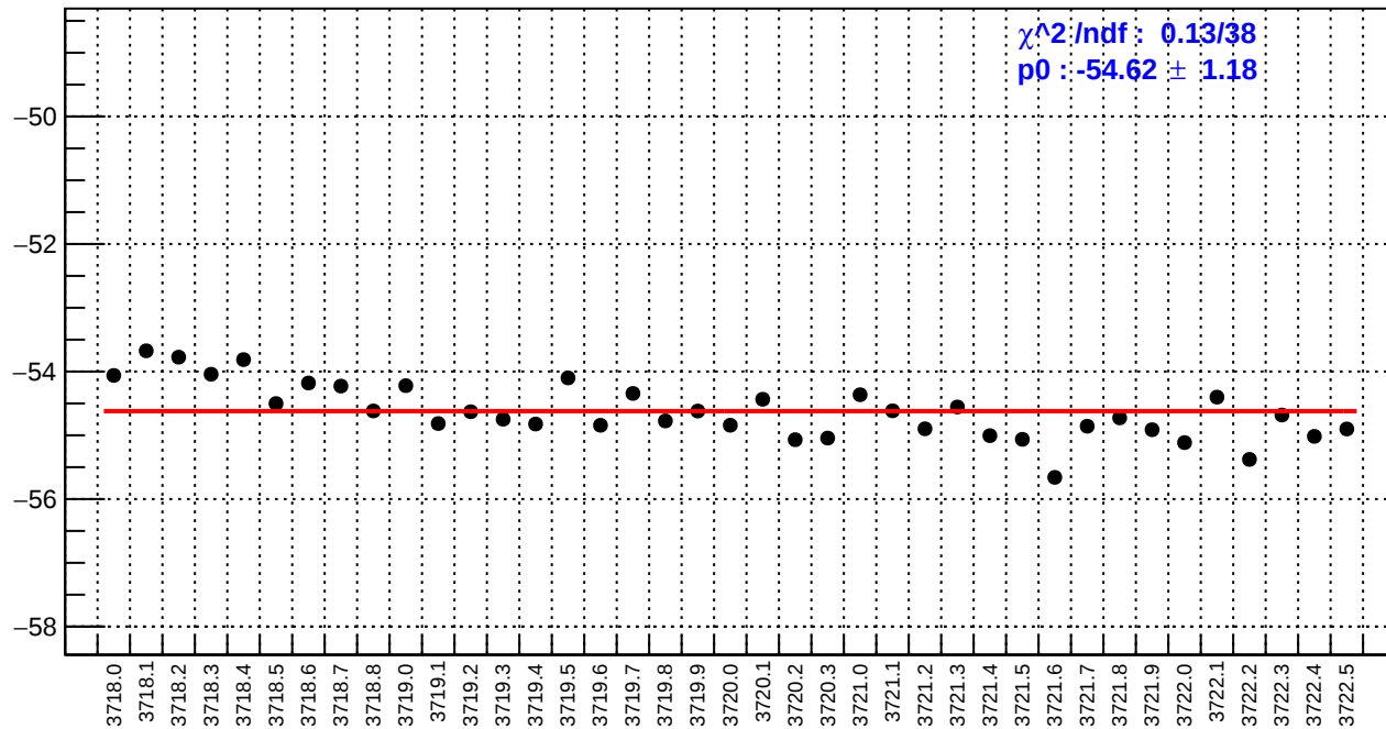
slug20: right_avg_bpm12X/(ppb/nm)
