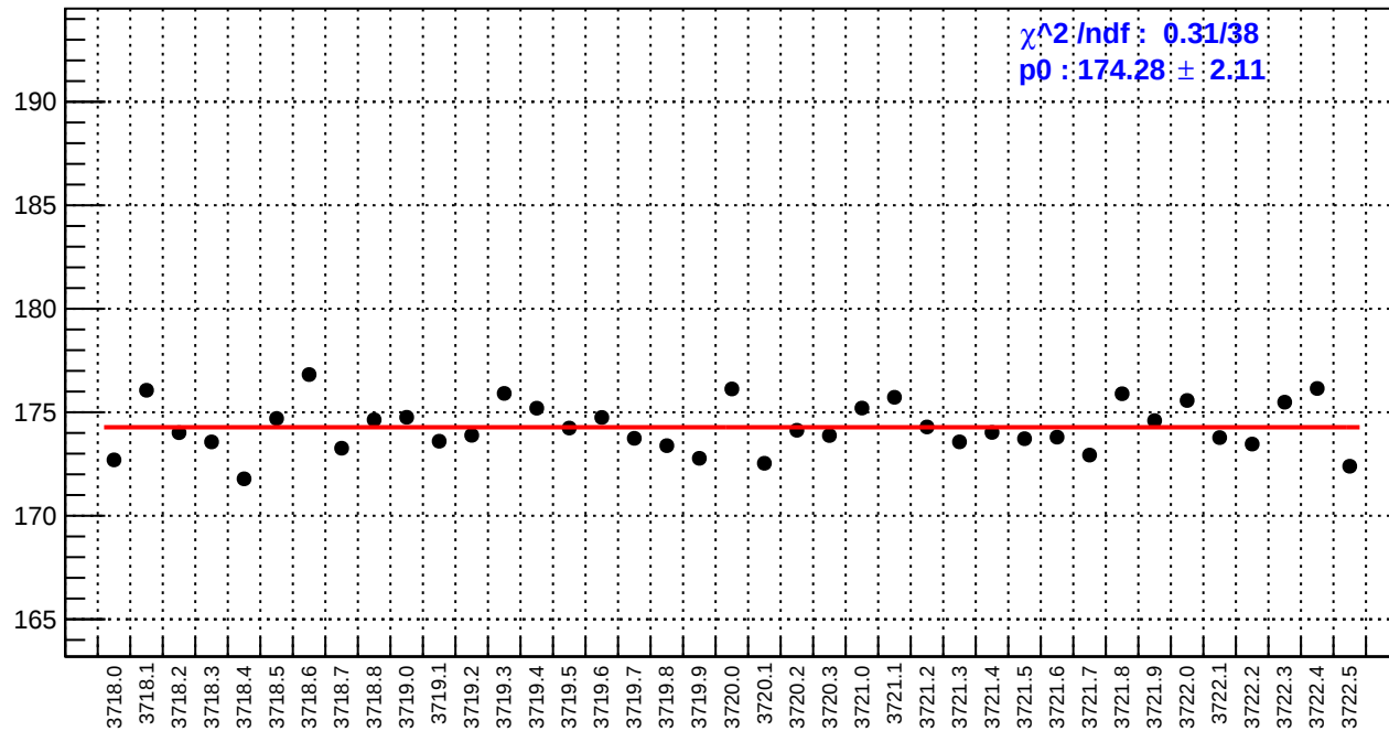
slug20: reg_asym_left_dd.rms/ppm
