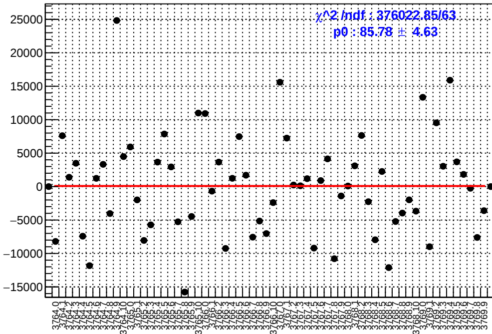
slug22: asym_usl.mean/ppb-reg_asym_usl.mean/ppb
