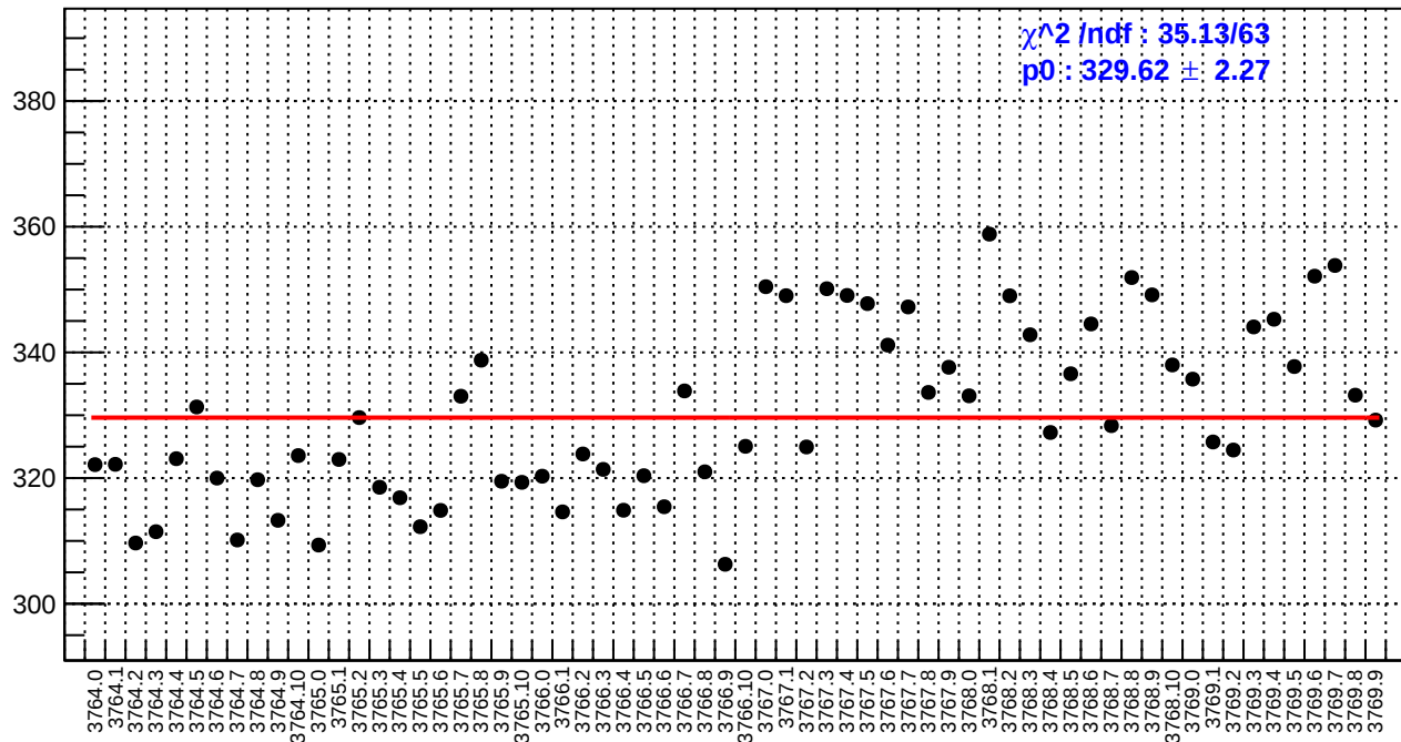
slug22: reg_asym_sam5.rms/ppm
