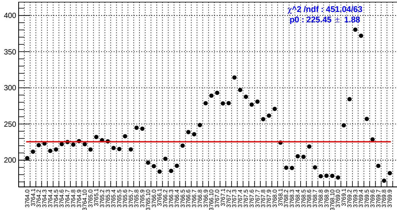
slug22: asym_bcm_an_us.rms/ppm
