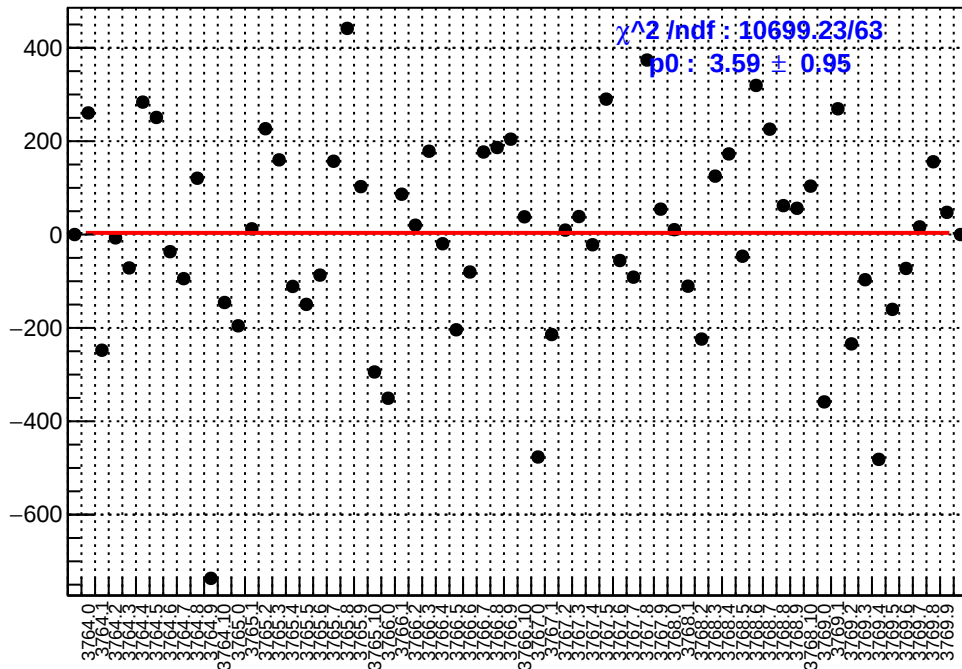
slug22: asym_left_dd.mean/ppb-reg_asym_left_dd.mean/ppb
