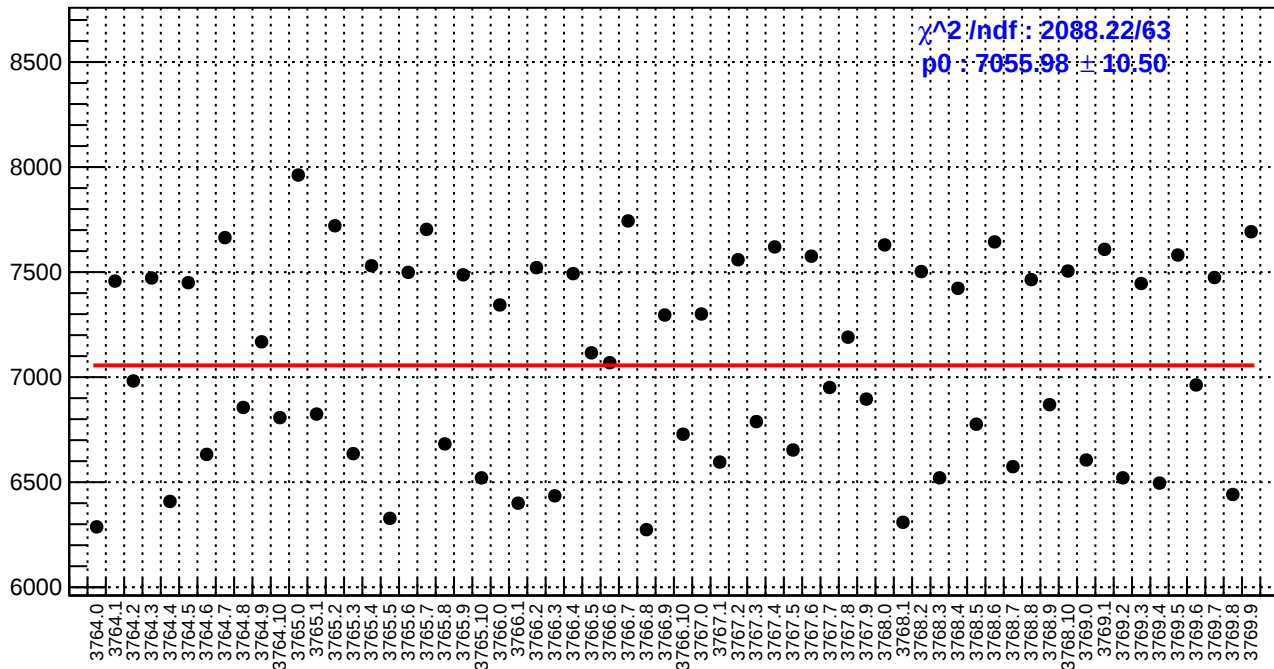
slug22: diff_bpm4aY.rms/nm
