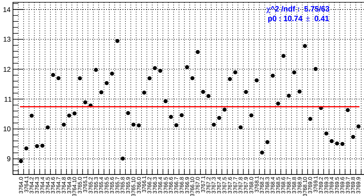
slug22: right_avg_bpm4aY/(ppb/nm)
