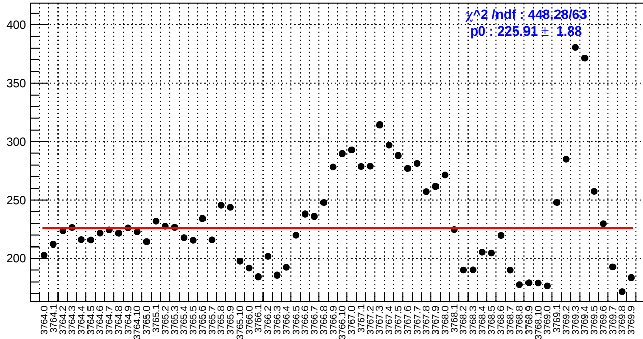
slug22: asym_bcm_an_ds.rms/ppm
