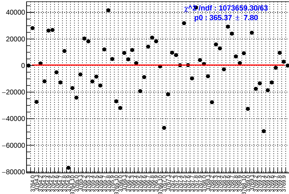
slug22: asym_sam7.mean/ppb-reg_asym_sam7.mean/ppb
