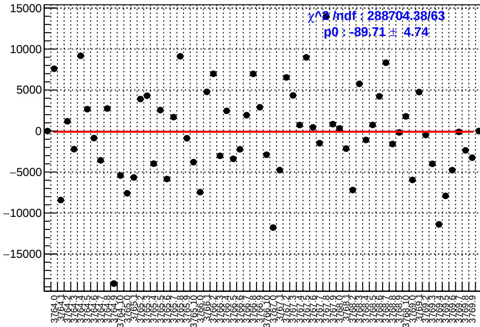
slug22: asym_usr.mean/ppb-reg_asym_usr.mean/ppb
