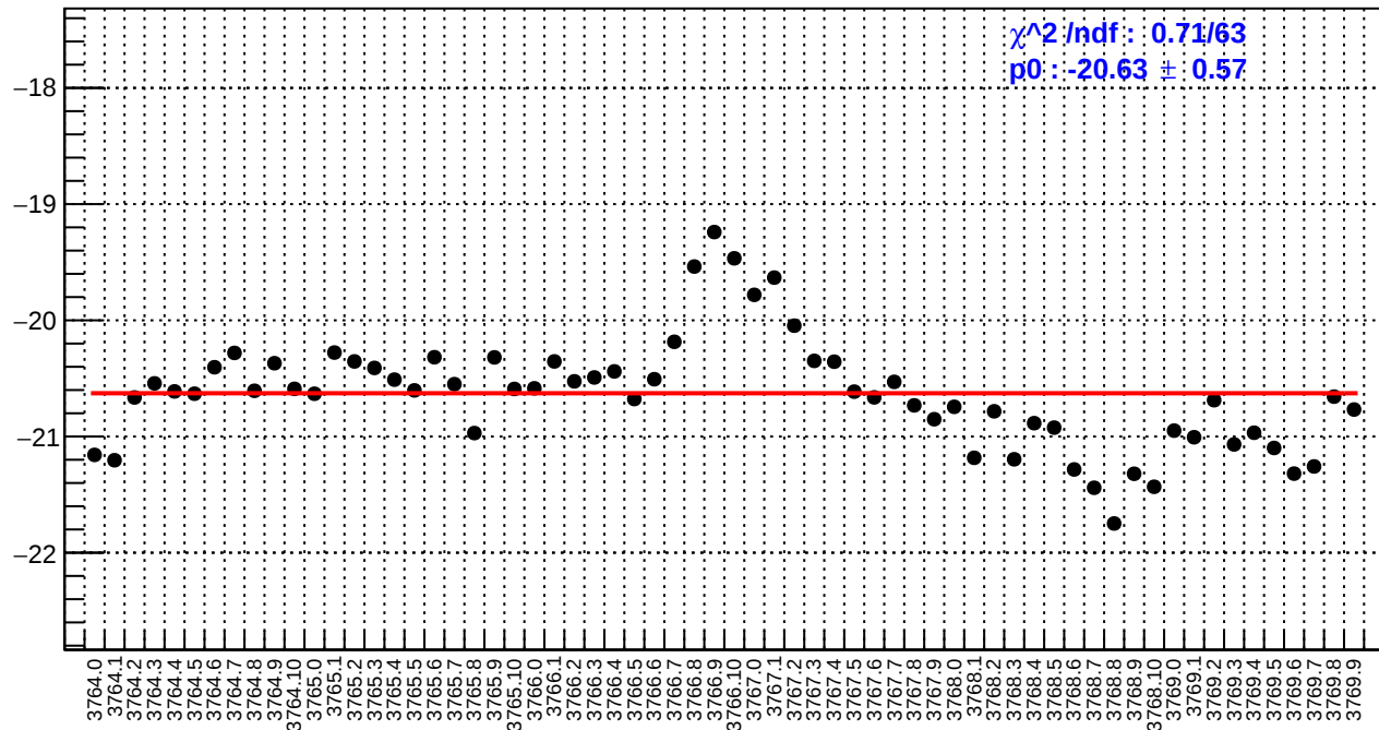
slug22: ds_avg_bpm4eX/(ppb/nm)
