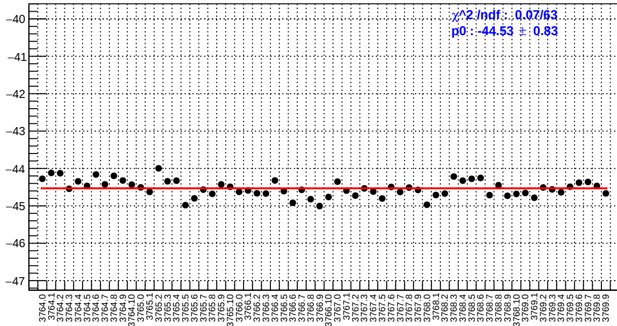
slug22: us_avg_bpm12X/(ppb/nm)
