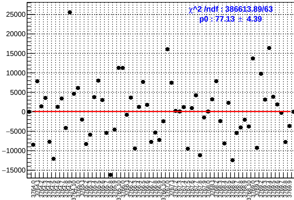
slug22: asym_left_avg.mean/ppb-reg_asym_left_avg.mean/ppb
