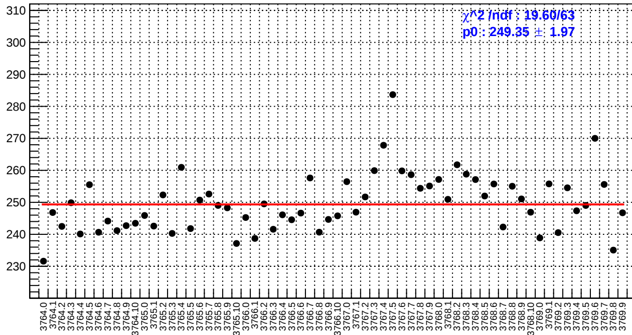
slug22: reg_asym_sam7.rms/ppm
