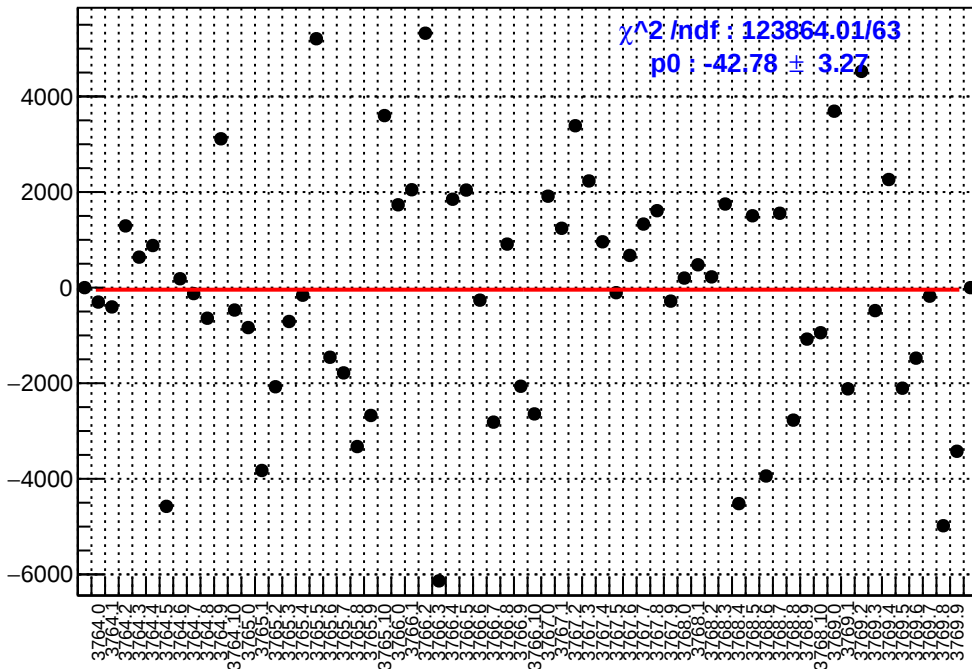
slug22: asym_us_avg.mean/ppb-reg_asym_us_avg.mean/ppb
