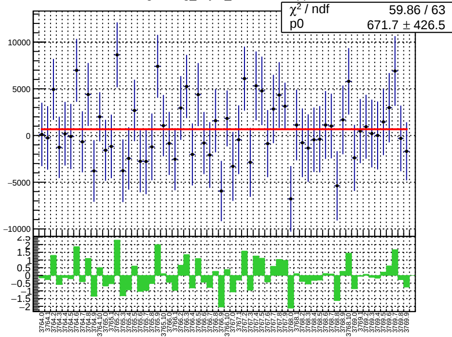
slug22: reg_asym_sam5.mean/ppb
