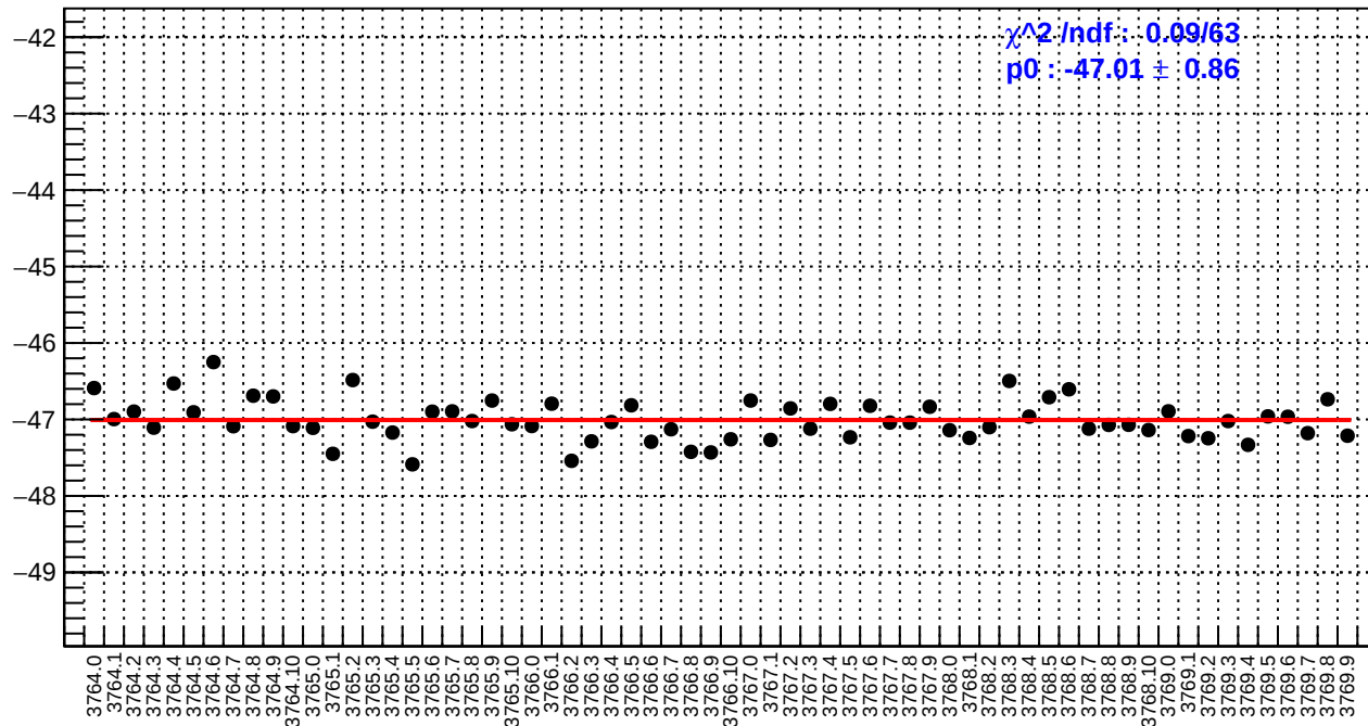
slug22: right_avg_bpm12X/(ppb/nm)
