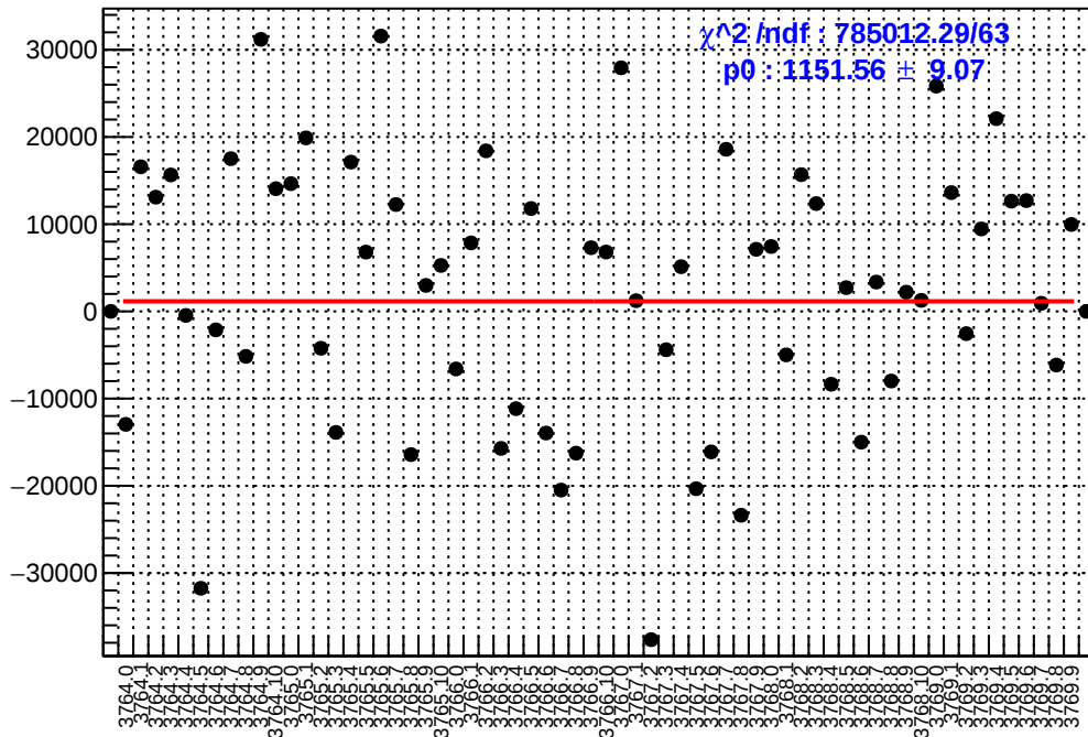
slug22: asym_sam5.mean/ppb-reg_asym_sam5.mean/ppb
