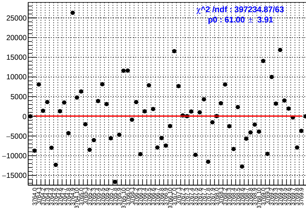
slug22: asym_dsl.mean/ppb-reg_asym_dsl.mean/ppb
