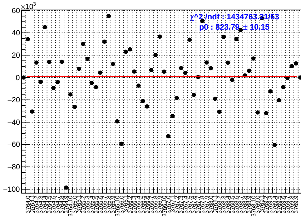
slug22: asym_sam6.mean/ppb-reg_asym_sam6.mean/ppb
