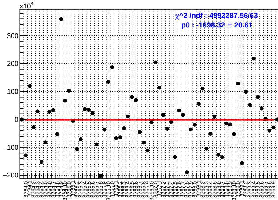
slug22: asym_sam2.mean/ppb-reg_asym_sam2.mean/ppb
