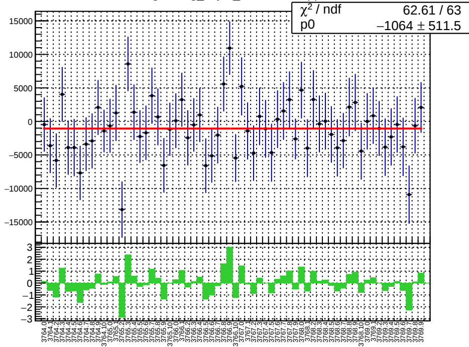
slug22: reg_asym_sam8.mean/ppb
