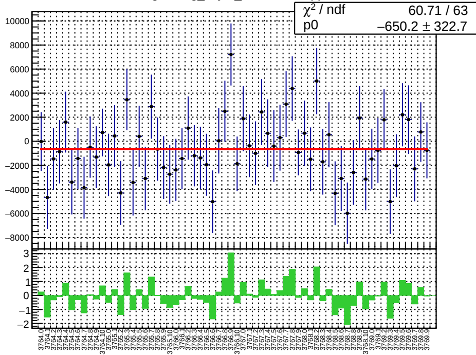
slug22: reg_asym_sam7.mean/ppb
