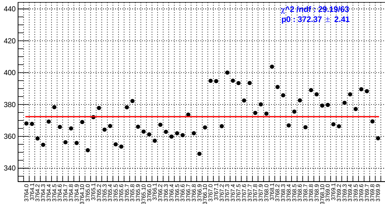
slug22: reg_asym_sam1.rms/ppm
