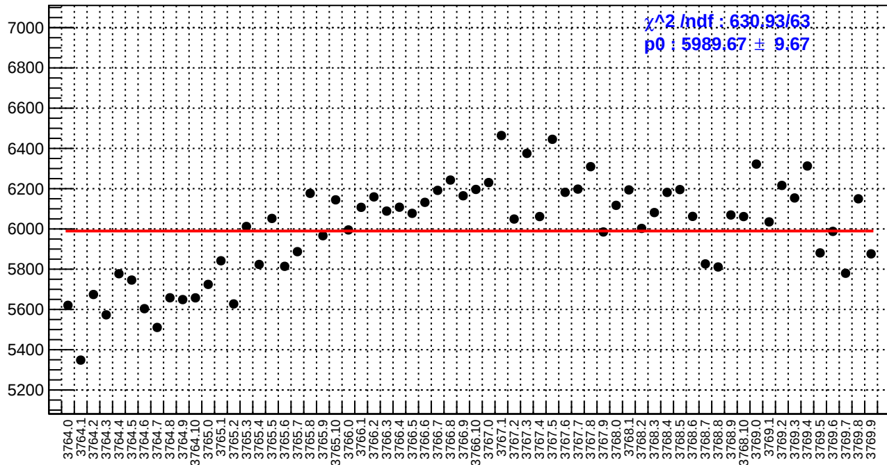
slug22: diff_bpm11X.rms/nm
