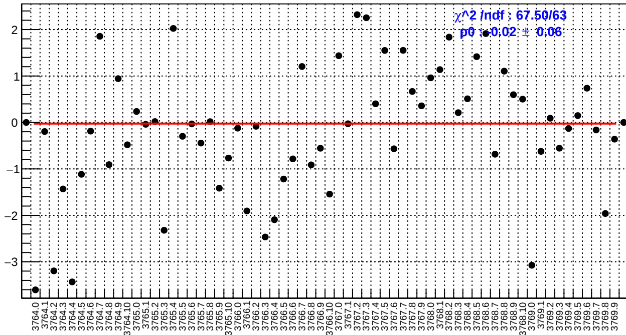
slug22: left_avg_bpm4aY/(ppb/nm)
