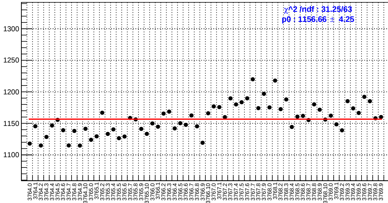
slug22: reg_asym_sam4.rms/ppm
