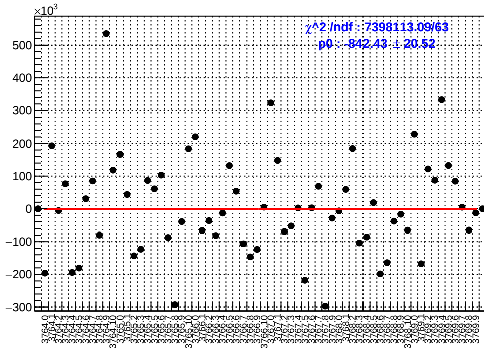
slug22: asym_sam3.mean/ppb-reg_asym_sam3.mean/ppb
