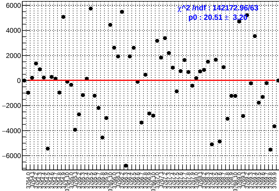
slug22: asym_ds_avg.mean/ppb-reg_asym_ds_avg.mean/ppb
