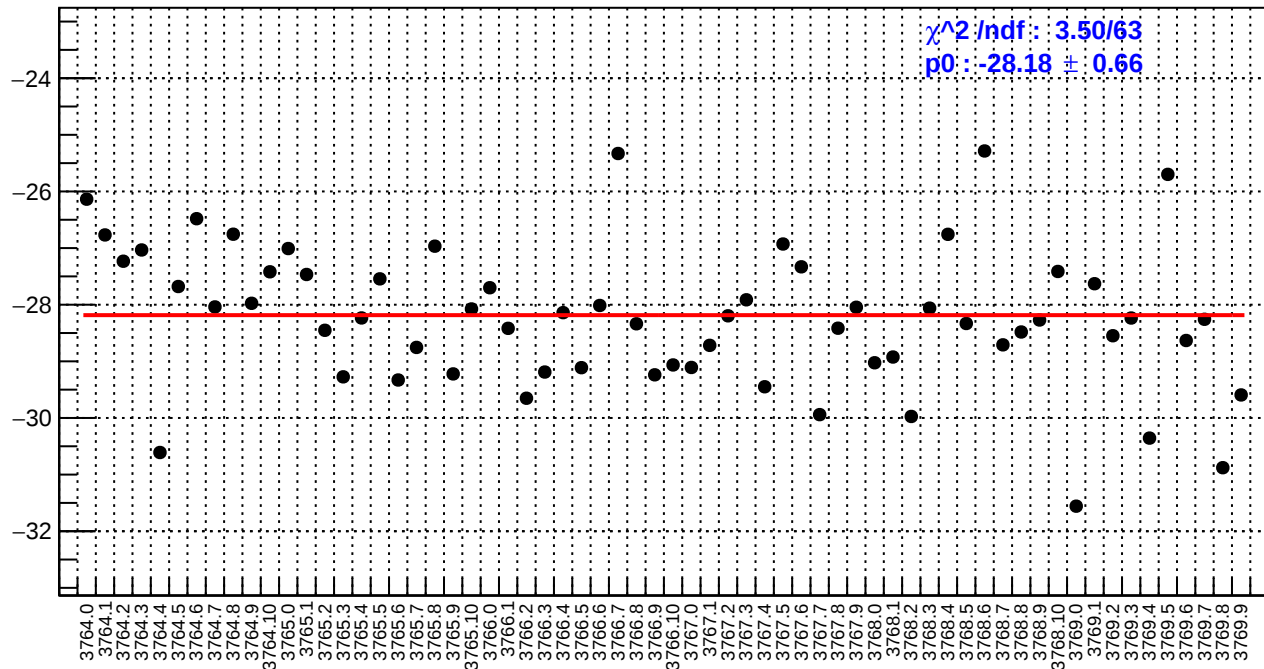
slug22: right_avg_bpm4aX/(ppb/nm)
