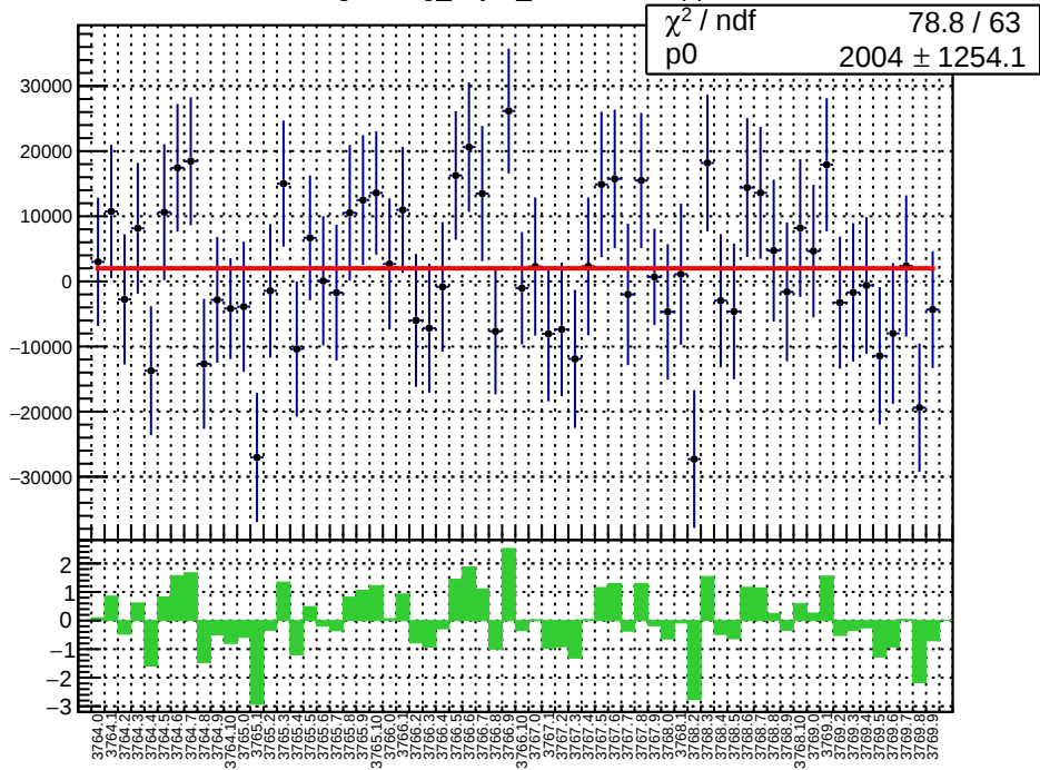
slug22: reg_asym_sam3.mean/ppb
