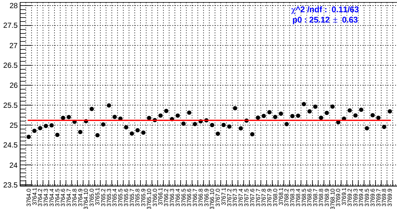
slug22: reg_asym_right_dd.rms/ppm
