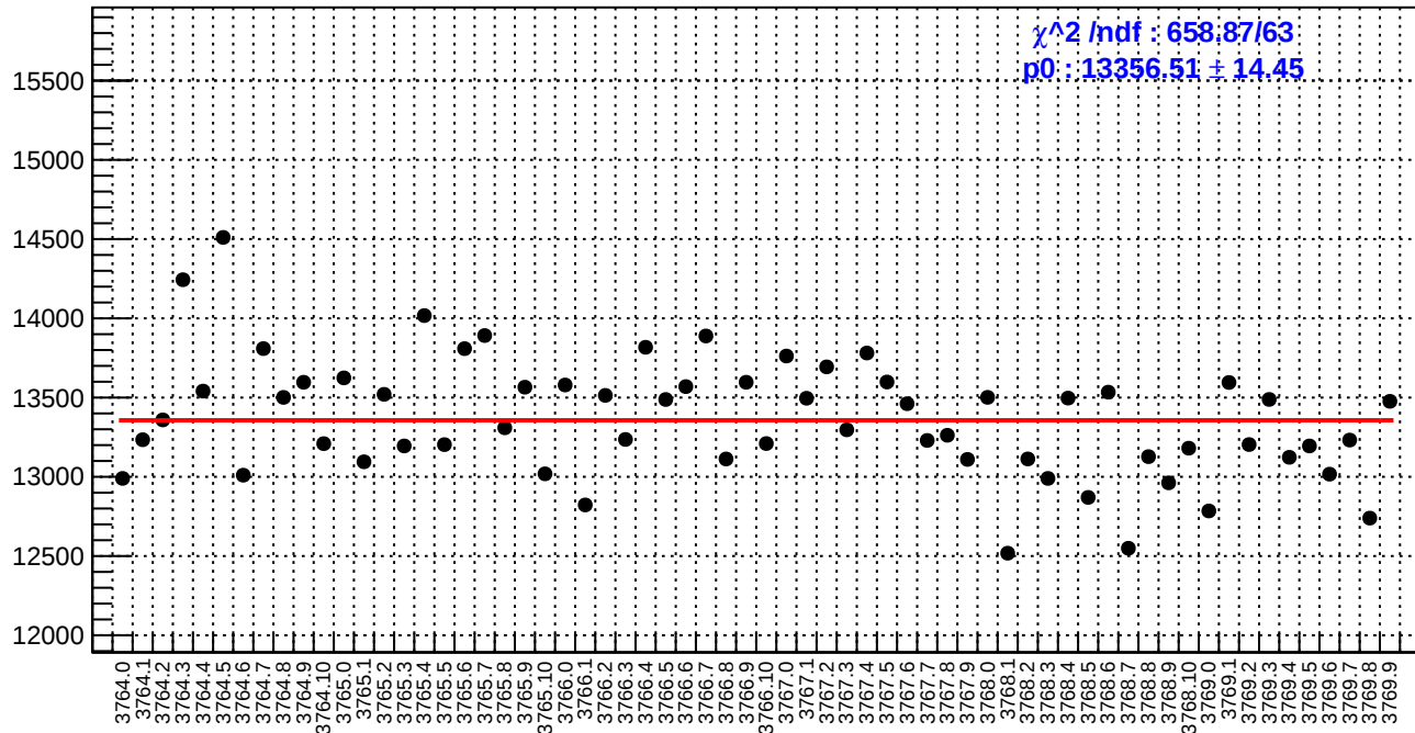
slug22: diff_bpm4eX.rms/nm
