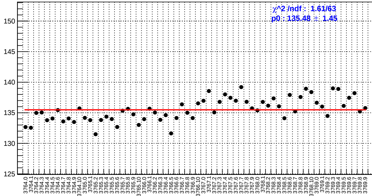
slug22: reg_asym_left_avg.rms/ppm
