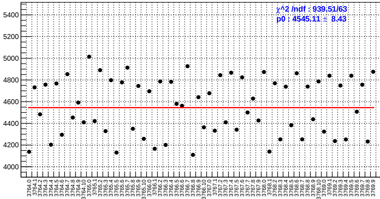
slug22: diff_bpm4eY.rms/nm
