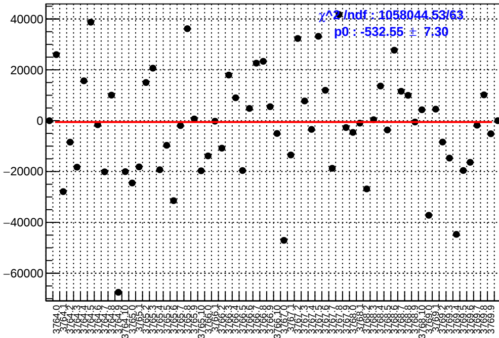
slug22: asym_sam8.mean/ppb-reg_asym_sam8.mean/ppb
