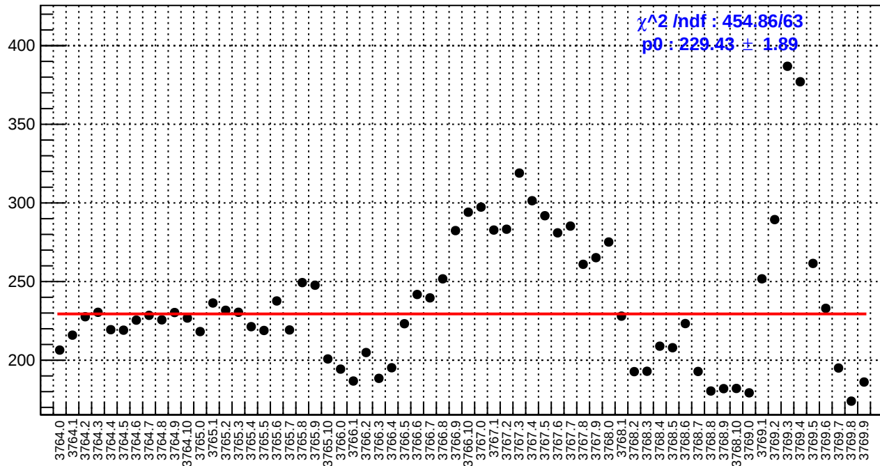
slug22: asym_bcm_an_ds3.rms/ppm
