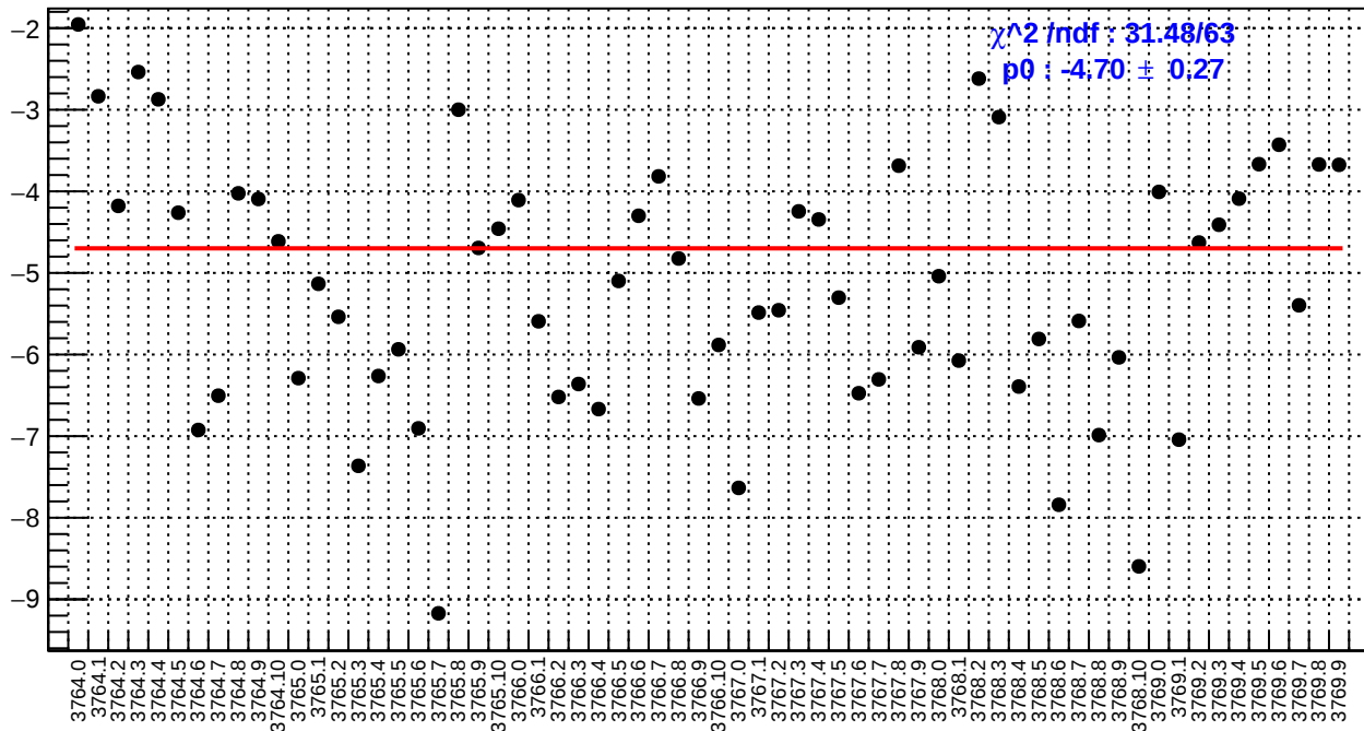
slug22: right_avg_bpm4eY/(ppb/nm)
