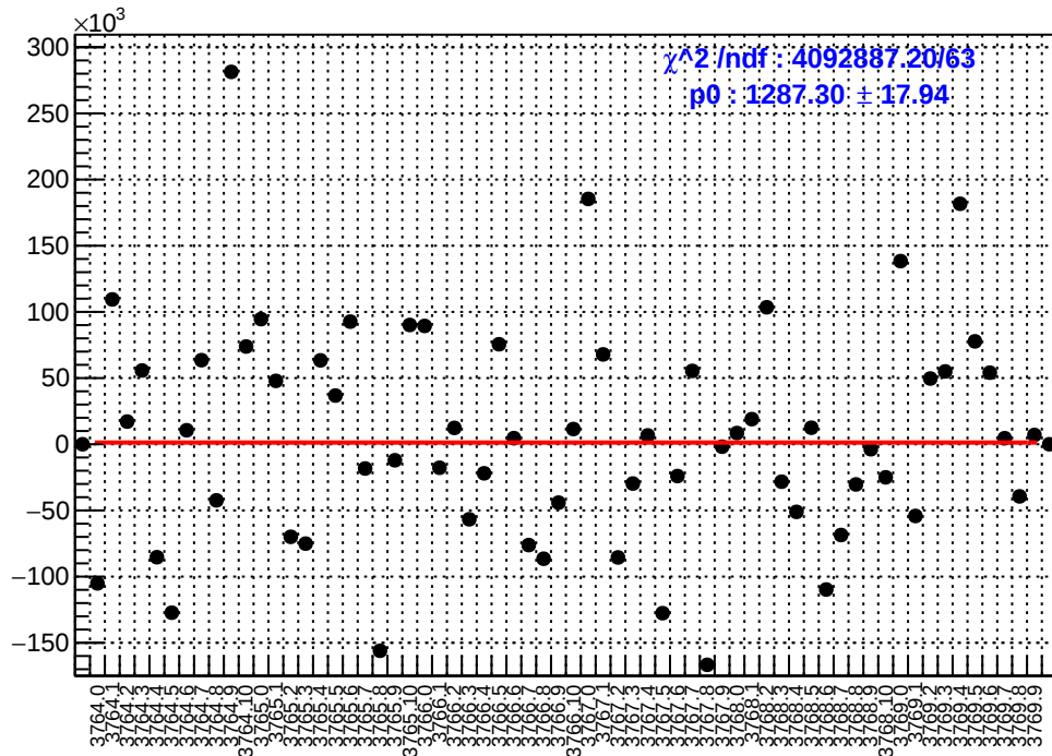
slug22: asym_sam4.mean/ppb-reg_asym_sam4.mean/ppb
