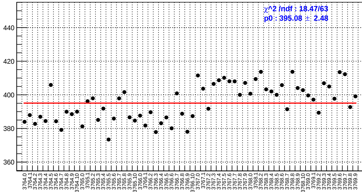
slug22: reg_asym_sam8.rms/ppm
