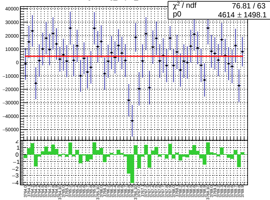
slug22: reg_asym_sam4.mean/ppb
