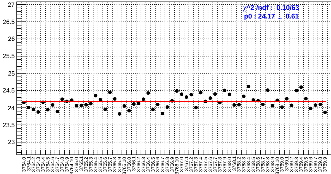
slug22: reg_asym_left_dd.rms/ppm
