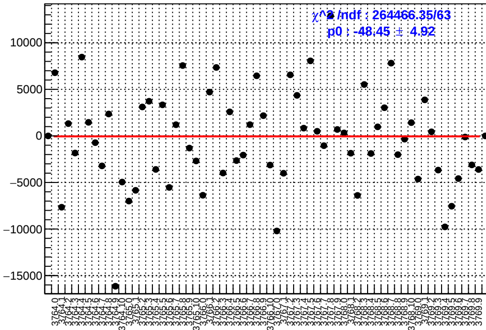
slug22: asym_dsr.mean/ppb-reg_asym_dsr.mean/ppb
