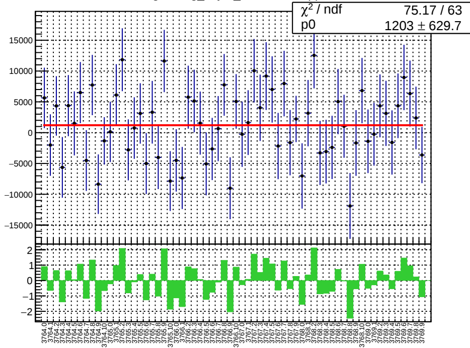
slug22: reg_asym_sam6.mean/ppb
