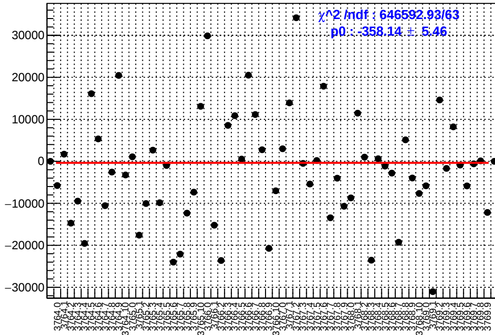
slug22: asym_sam1.mean/ppb-reg_asym_sam1.mean/ppb
