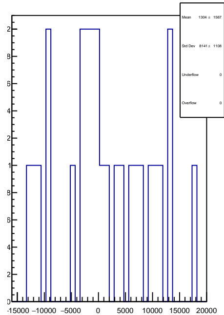
slug25-Left: 1D Corr asym_usl.mean/ppb-reg_asym_usl.mean/ppb
