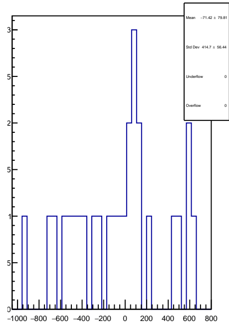
slug25-Left: 1D Corr asym_right_dd.mean/ppb-reg_asym_right_dd.mean/ppb
