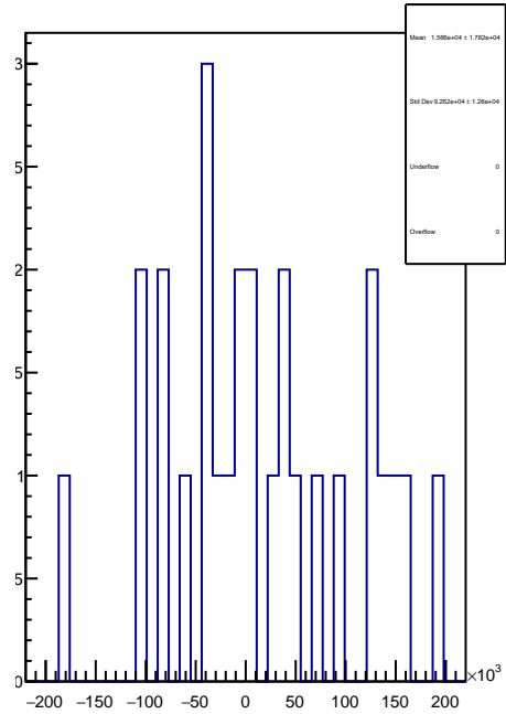
slug25-Left: 1D Corr asym_sam4.mean/ppb-reg_asym_sam4.mean/ppb
