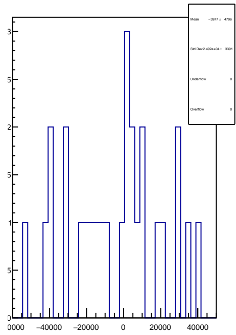
slug25-Left: 1D Corr asym_sam7.mean/ppb-reg_asym_sam7.mean/ppb
