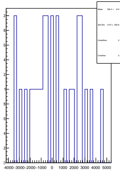
slug25-Left: 1D Corr asym_us_avg.mean/ppb-reg_asym_us_avg.mean/ppb
