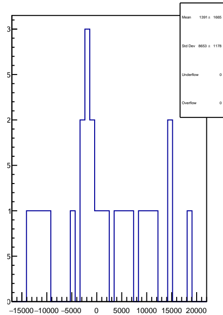
slug25-Left: 1D Corr asym_dsl.mean/ppb-reg_asym_dsl.mean/ppb
