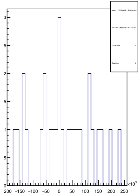
slug25-Left: 1D Corr asym_sam2.mean/ppb-reg_asym_sam2.mean/ppb
