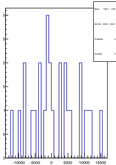
slug25-Left: 1D Corr asym_ds_dd.mean/ppb-reg_asym_ds_dd.mean/ppb
