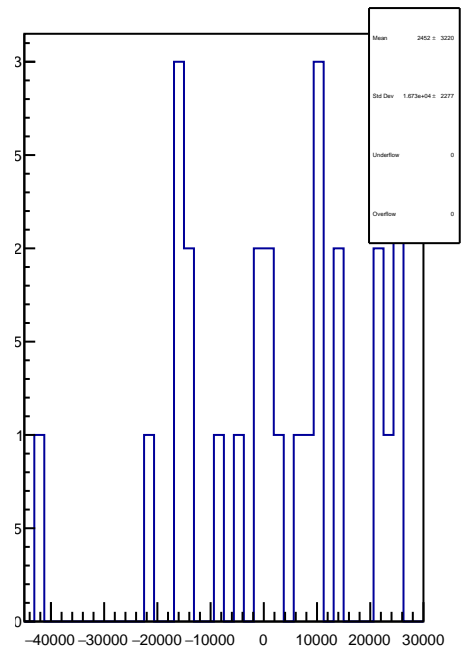
slug25-Left: 1D Corr asym_sam5.mean/ppb-reg_asym_sam5.mean/ppb
