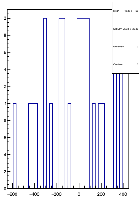
slug25-Left: 1D Corr asym_left_dd.mean/ppb-reg_asym_left_dd.mean/ppb
