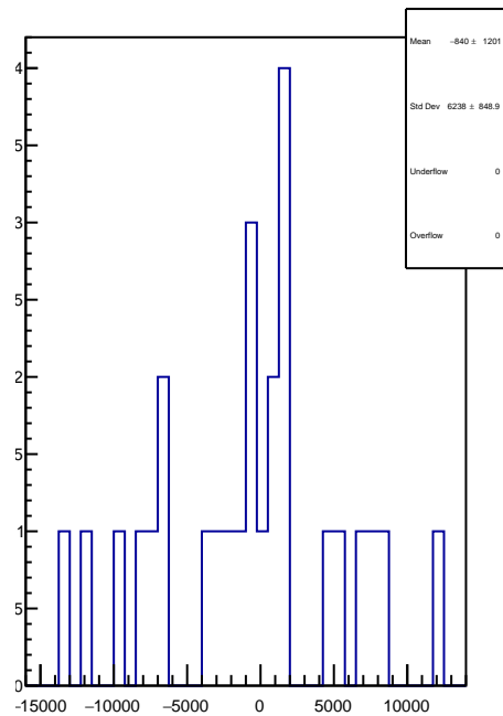
slug25-Left: 1D Corr asym_right_avg.mean/ppb-reg_asym_right_avg.mean/ppb
