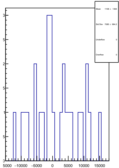
slug25-Left: 1D Corr asym_us_dd.mean/ppb-reg_asym_us_dd.mean/ppb
