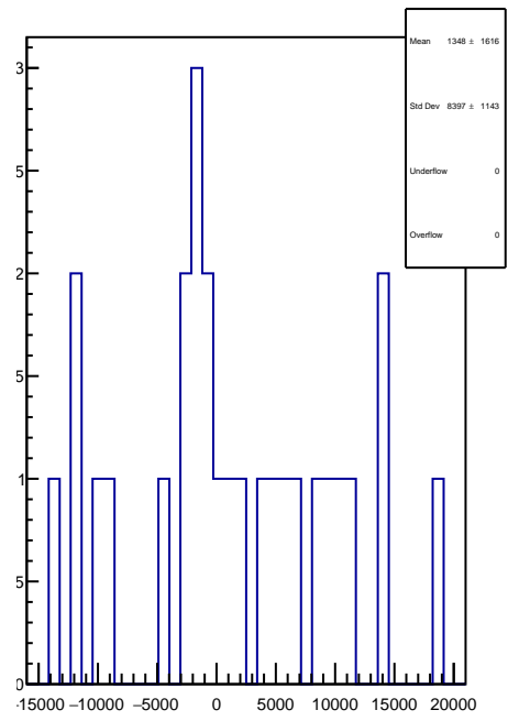
slug25-Left: 1D Corr asym_left_avg.mean/ppb-reg_asym_left_avg.mean/ppb
