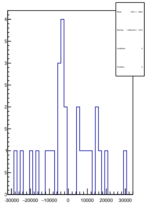
slug25-Left: 1D Corr asym_sam1.mean/ppb-reg_asym_sam1.mean/ppb
