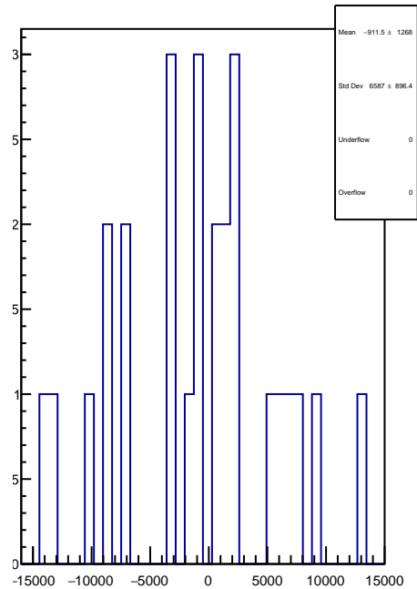
slug25-Left: 1D Corr asym_usr.mean/ppb-reg_asym_usr.mean/ppb
