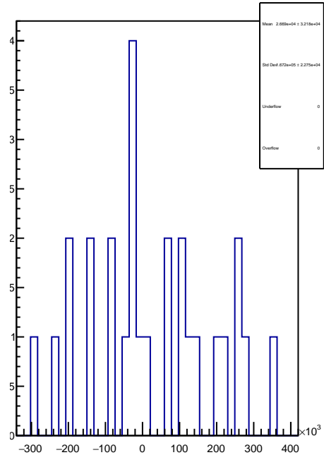
slug25-Left: 1D Corr asym_sam3.mean/ppb-reg_asym_sam3.mean/ppb
