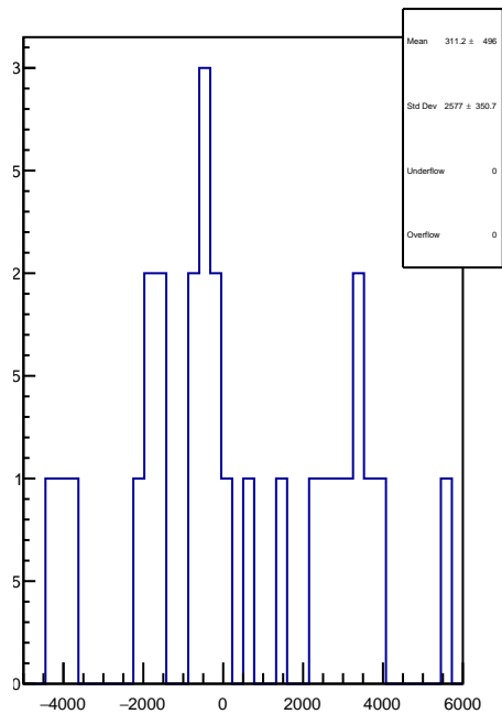
slug25-Left: 1D Corr asym_ds_avg.mean/ppb-reg_asym_ds_avg.mean/ppb
