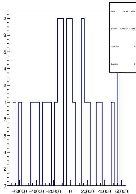
slug25-Left: 1D Corr asym_sam6.mean/ppb-reg_asym_sam6.mean/ppb
