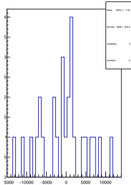
slug25-Left: 1D Corr asym_dsr.mean/ppb-reg_asym_dsr.mean/ppb
