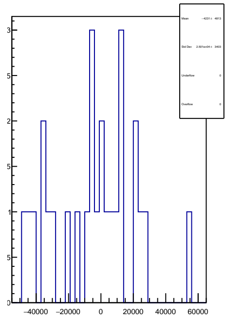
slug25-Left: 1D Corr asym_sam8.mean/ppb-reg_asym_sam8.mean/ppb
