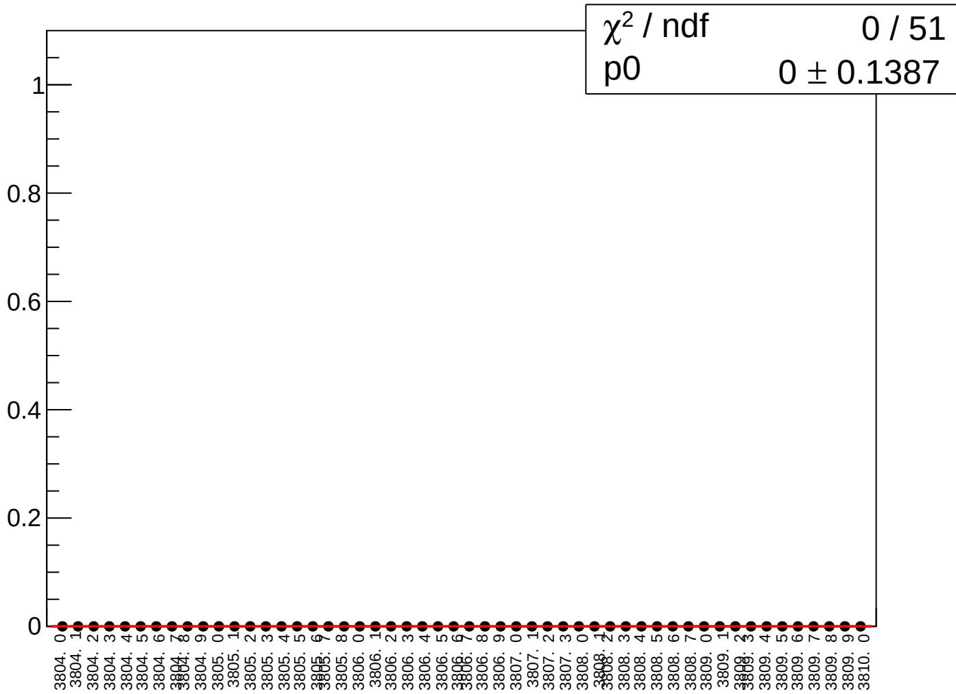
cor_sam_48_avg_rms vs run
