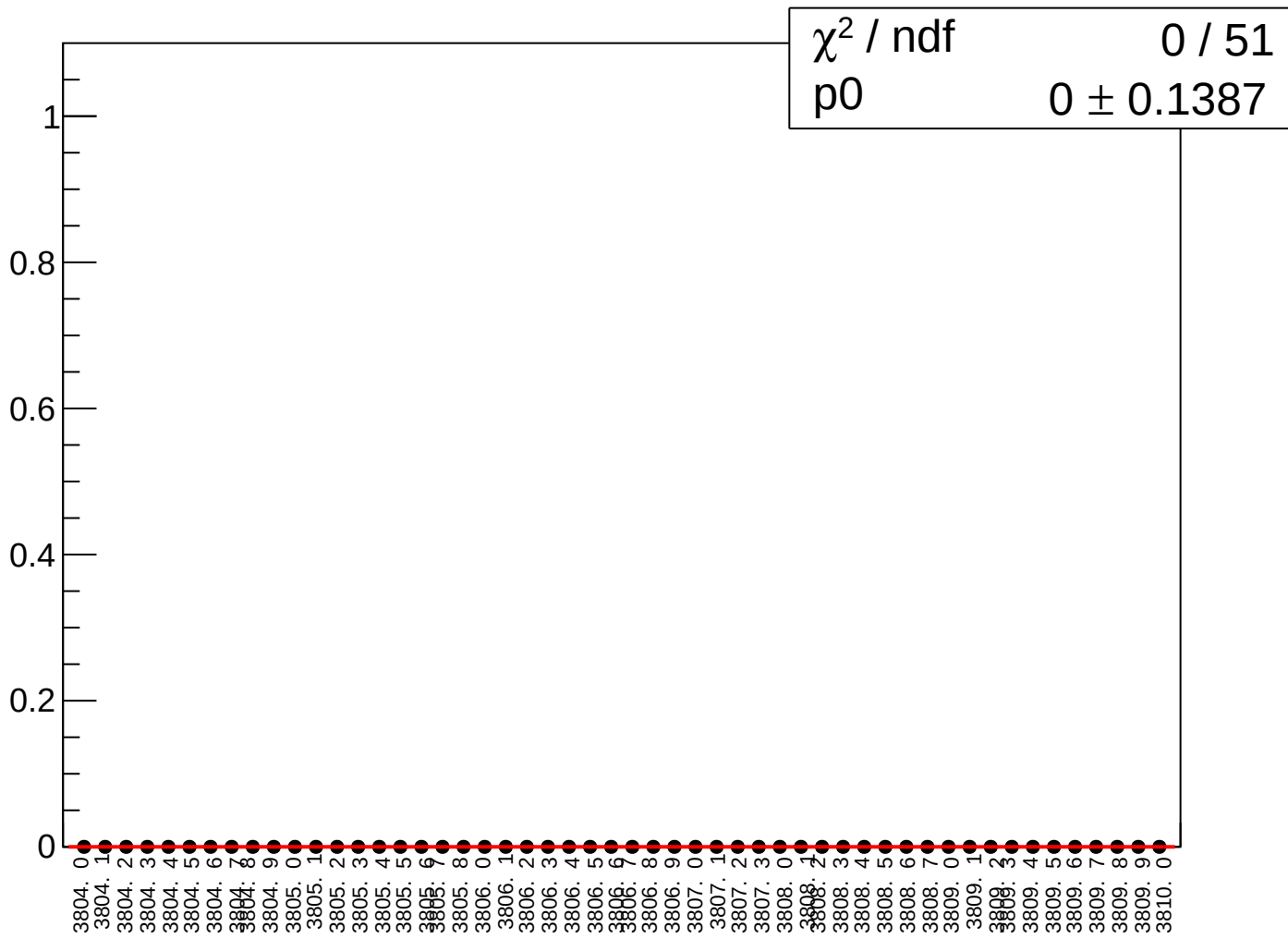
cor_sam_37_dd_rms vs run
