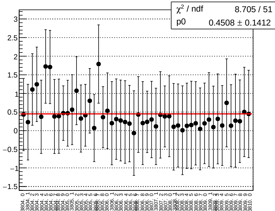
reg_asym_us_dd_diff_bpm11X_slope vs run
