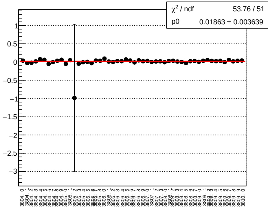
reg bcm an us ds dd diff bpm4eX slope vs run
