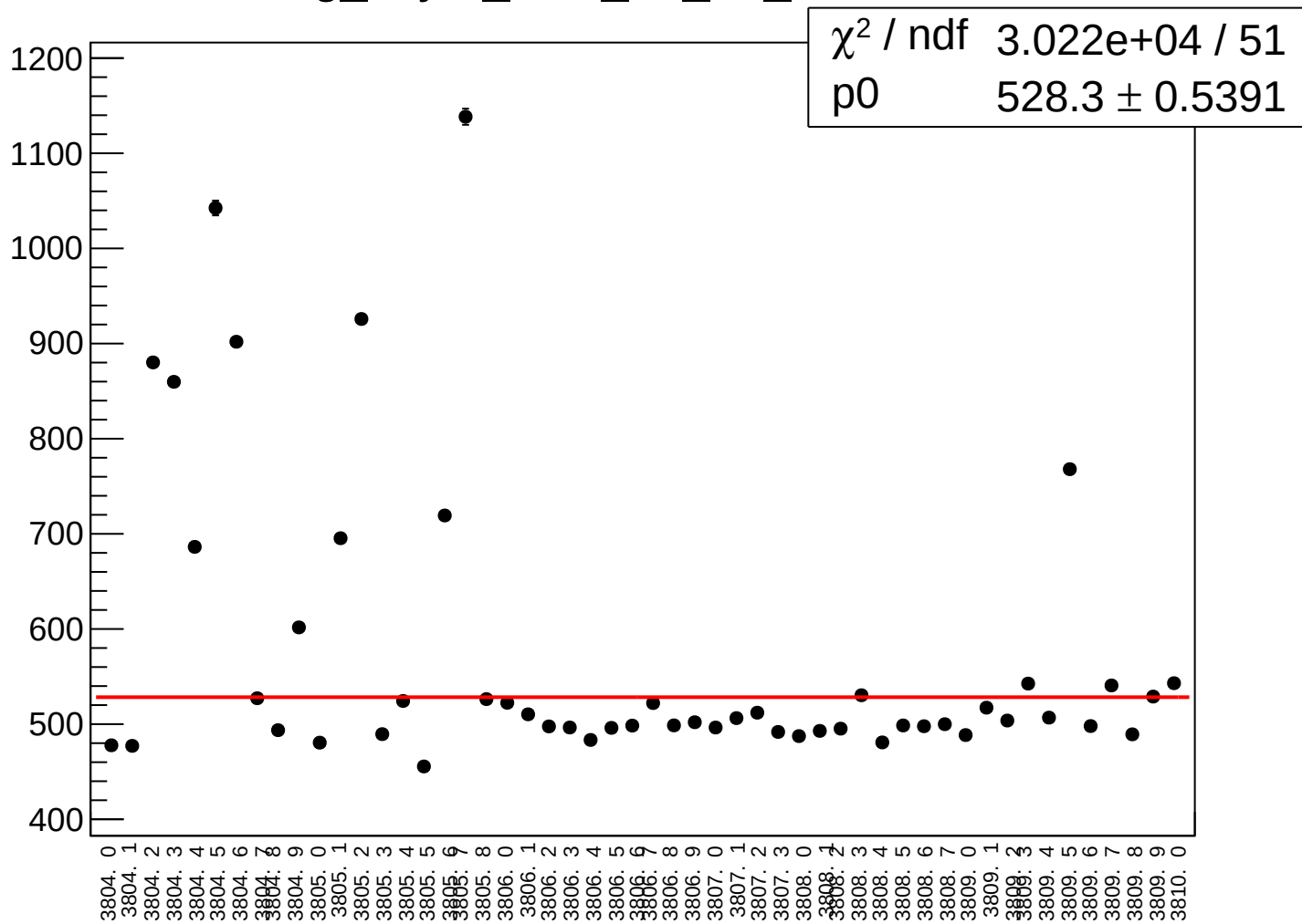
reg_asym_sam_37_dd_rms vs run
