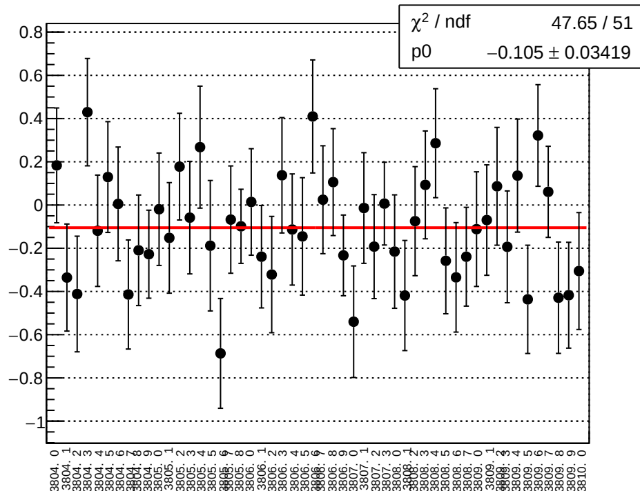
reg_bcm_dg_us_dg_ds_dd_diff_bpm4x_slope vs run
