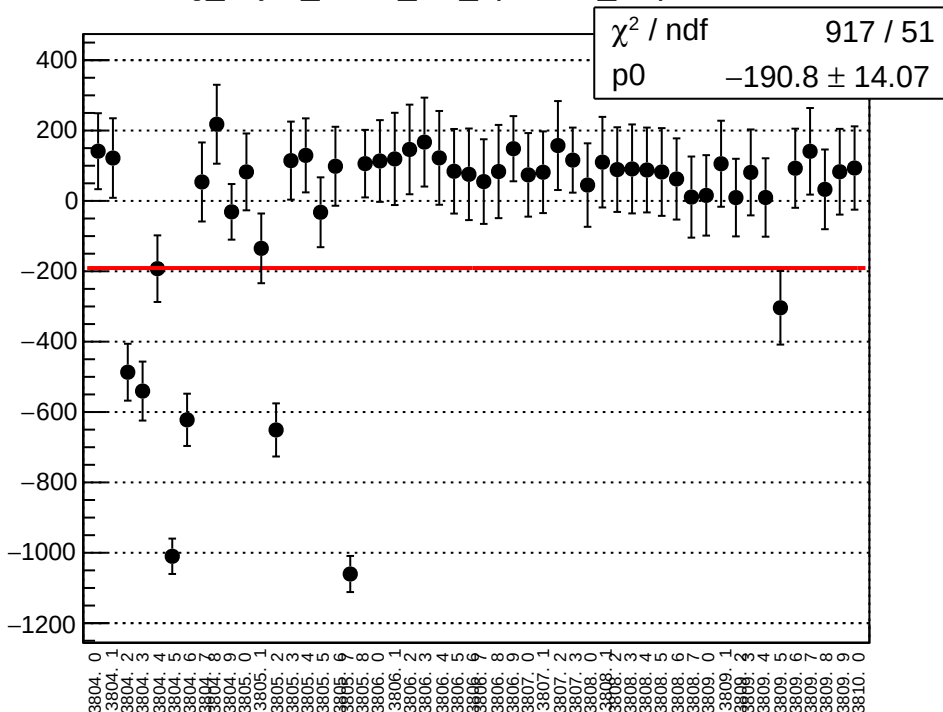
reg_asym_sam2_diff_bpm4eY_slope vs run
