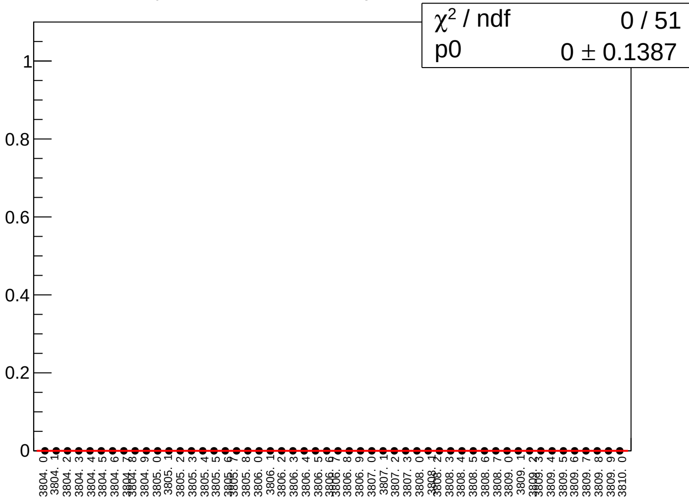
yield_sam_48_avg_rms vs run
