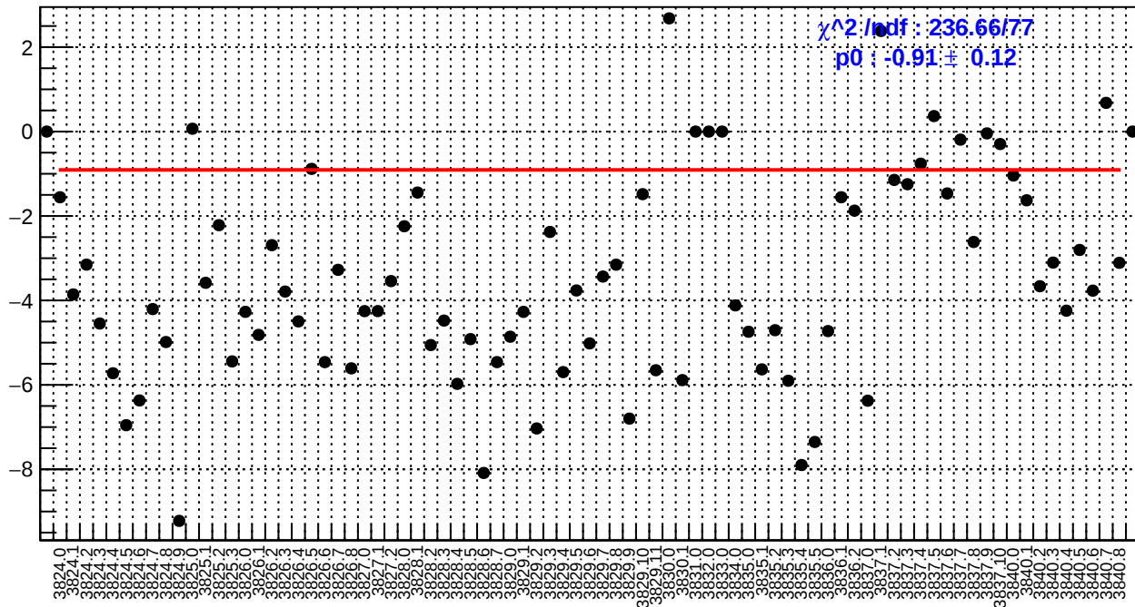
slug28: right_avg_bpm4eY/(ppb/nm)
