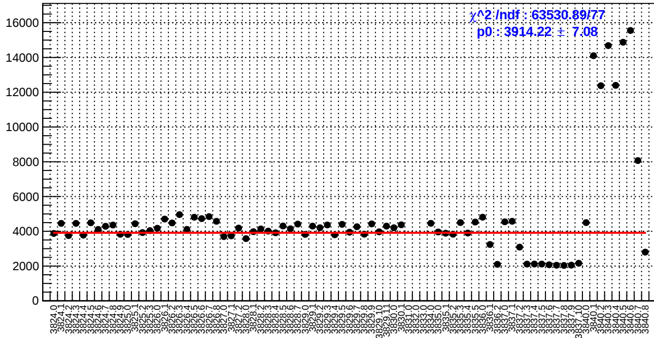
slug28: diff_bpm4eY.rms/nm
