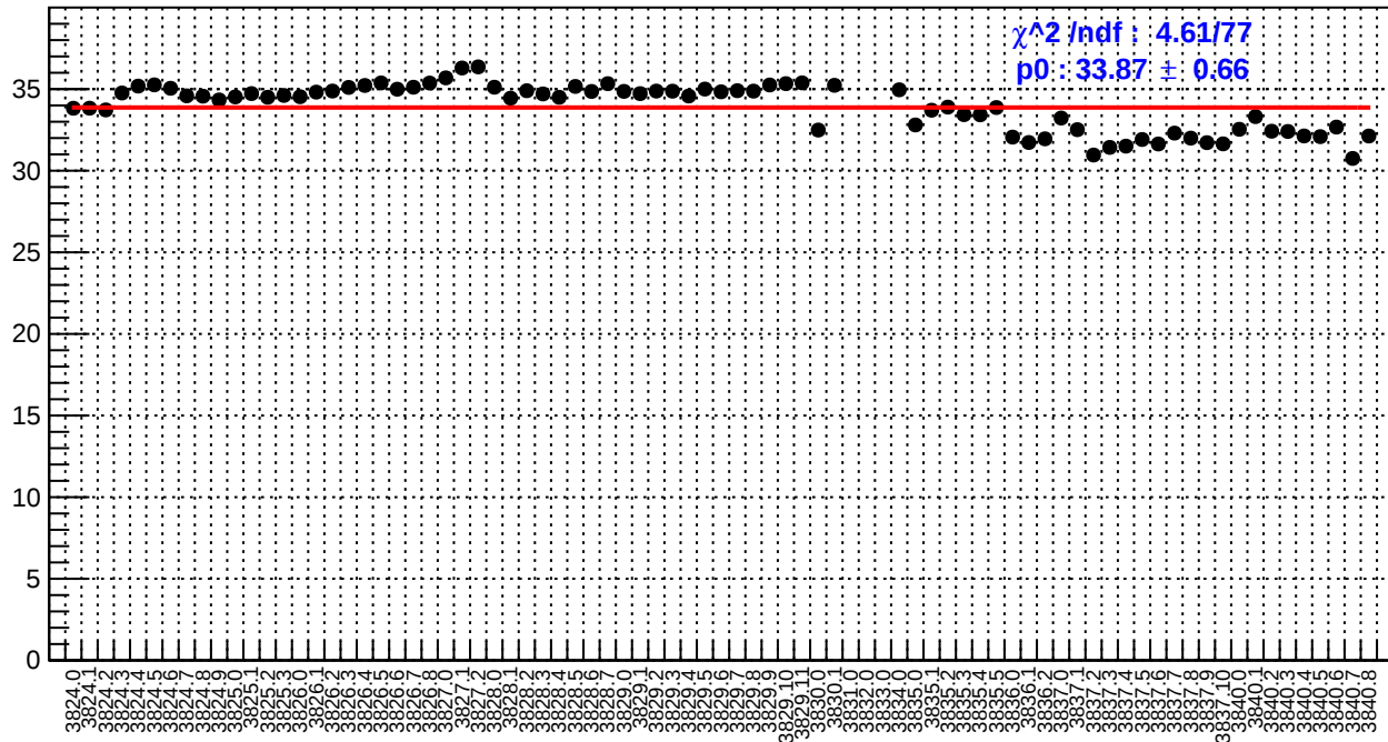
slug28: right_avg_bpm4eX/(ppb/nm)
