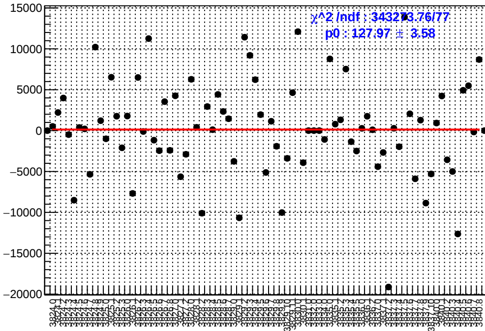
slug28: asym_dsr.mean/ppb-reg_asym_dsr.mean/ppb
