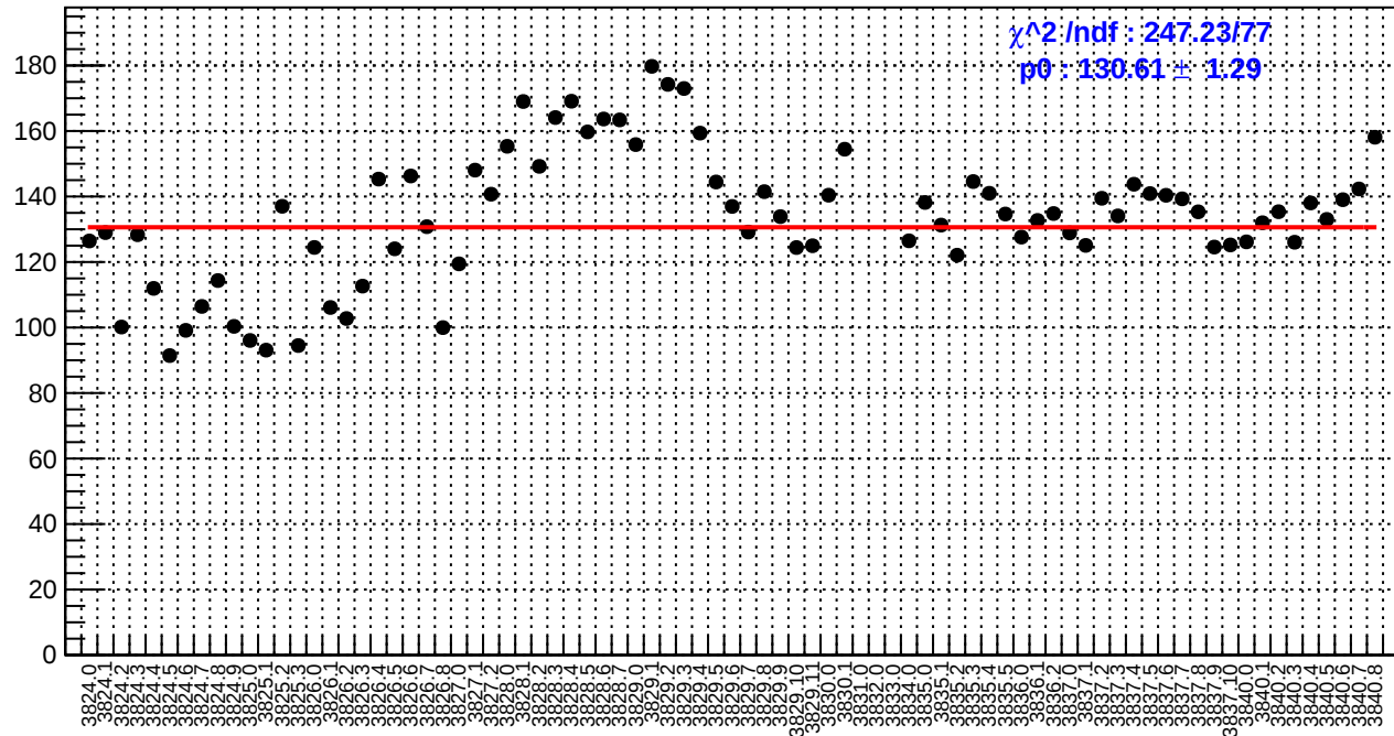
slug28: asym_bcm_an_ds3.rms/ppm
