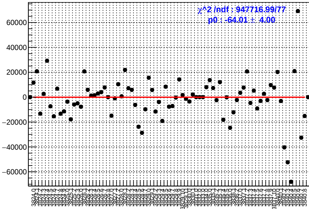
slug28: asym_sam5.mean/ppb-reg_asym_sam5.mean/ppb
