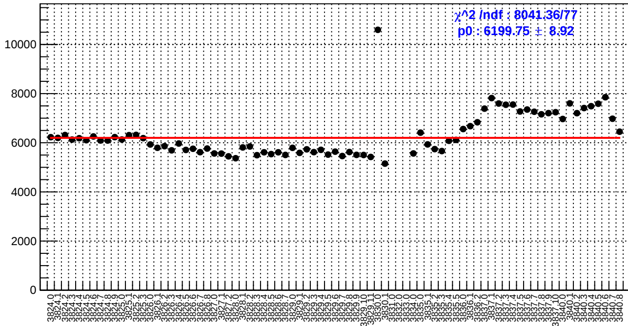
slug28: diff_bpm11X.rms/nm
