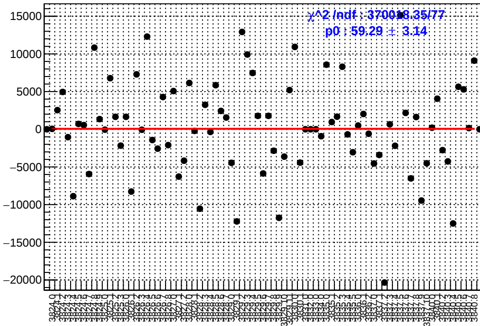
slug28: asym_usr.mean/ppb-reg_asym_usr.mean/ppb
