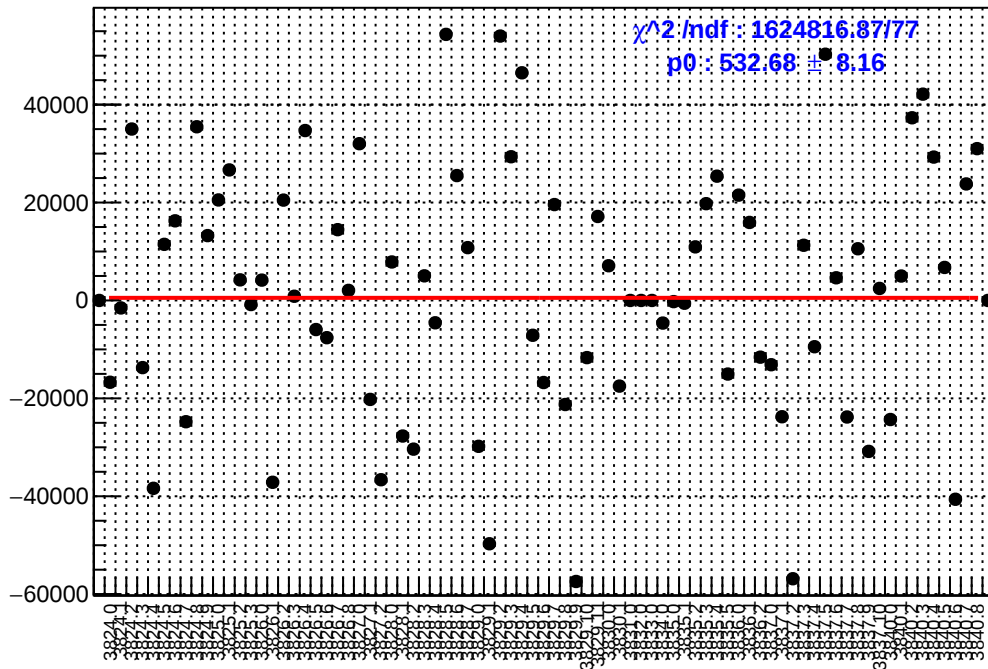
slug28: asym_sam8.mean/ppb-reg_asym_sam8.mean/ppb
