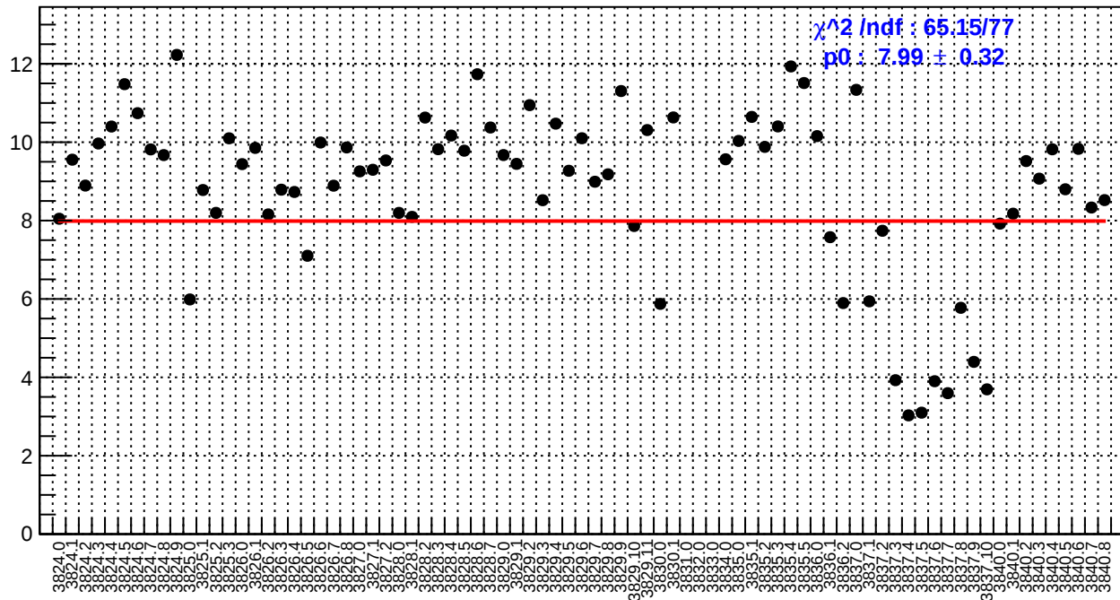
slug28: right_avg_bpm4aY/(ppb/nm)
