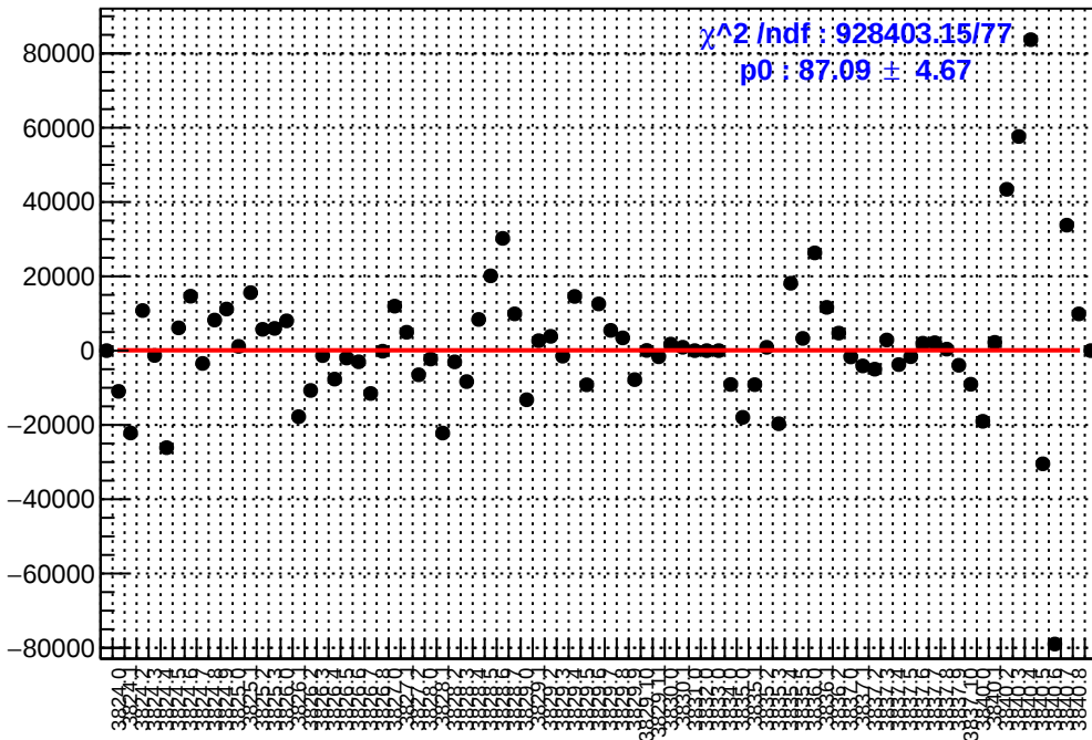
slug28: asym_sam1.mean/ppb-reg_asym_sam1.mean/ppb
