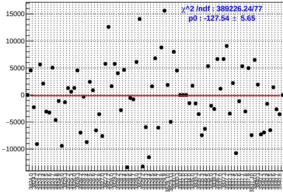
slug28: asym_usl.mean/ppb-reg_asym_usl.mean/ppb
