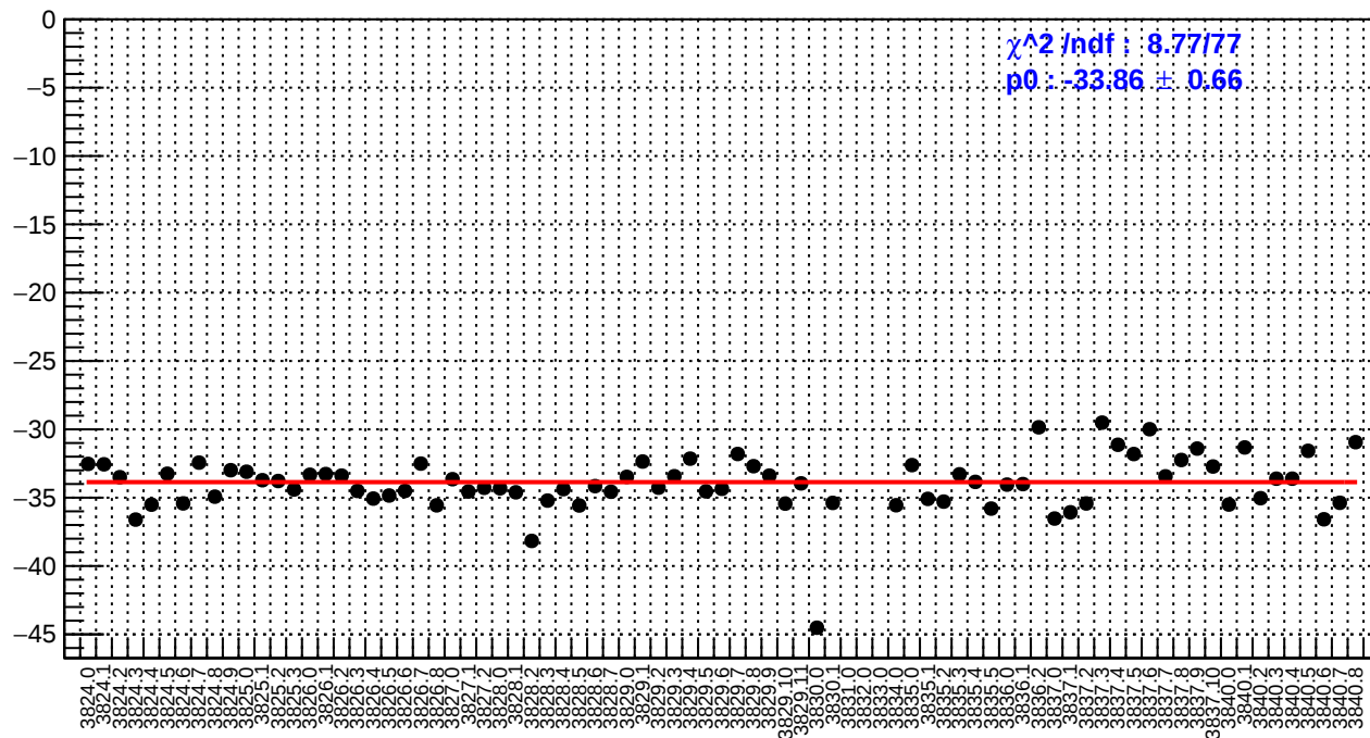
slug28: right_avg_bpm4aX/(ppb/nm)
