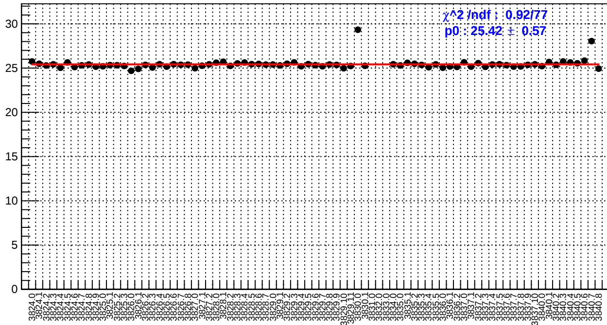
slug28: reg_asym_right_dd.rms/ppm
