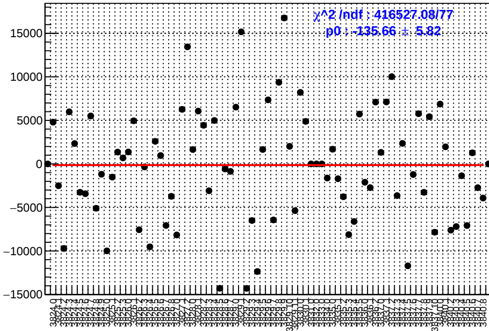
slug28: asym_dsl.mean/ppb-reg_asym_dsl.mean/ppb
