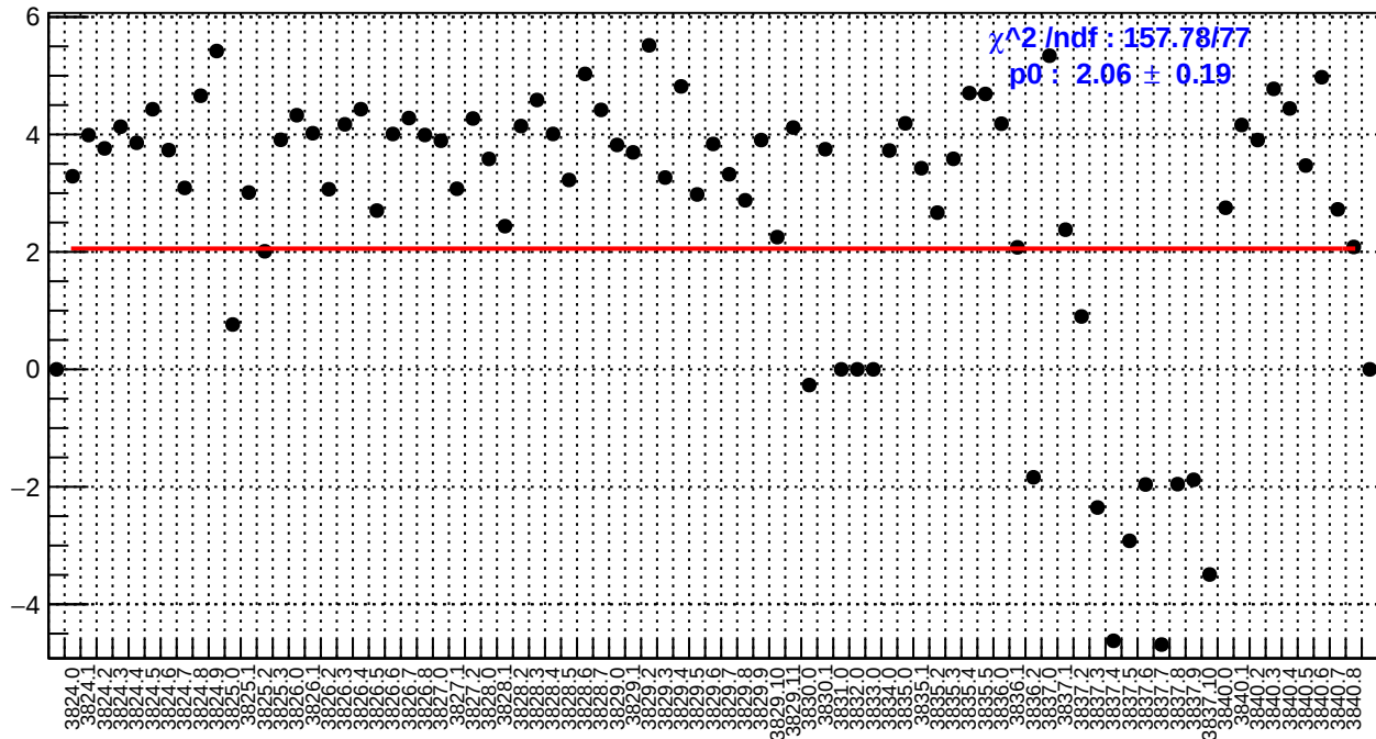
slug28: ds_avg_bpm4aY/(ppb/nm)
