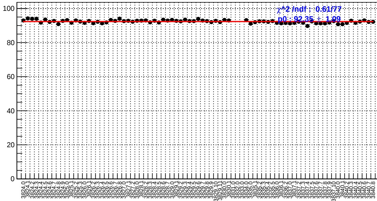
slug28: reg_asym_us_dd.rms/ppm
