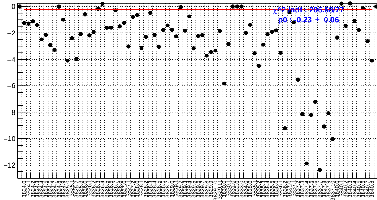
slug28: dsl_bpm4aY/(ppb/nm)
