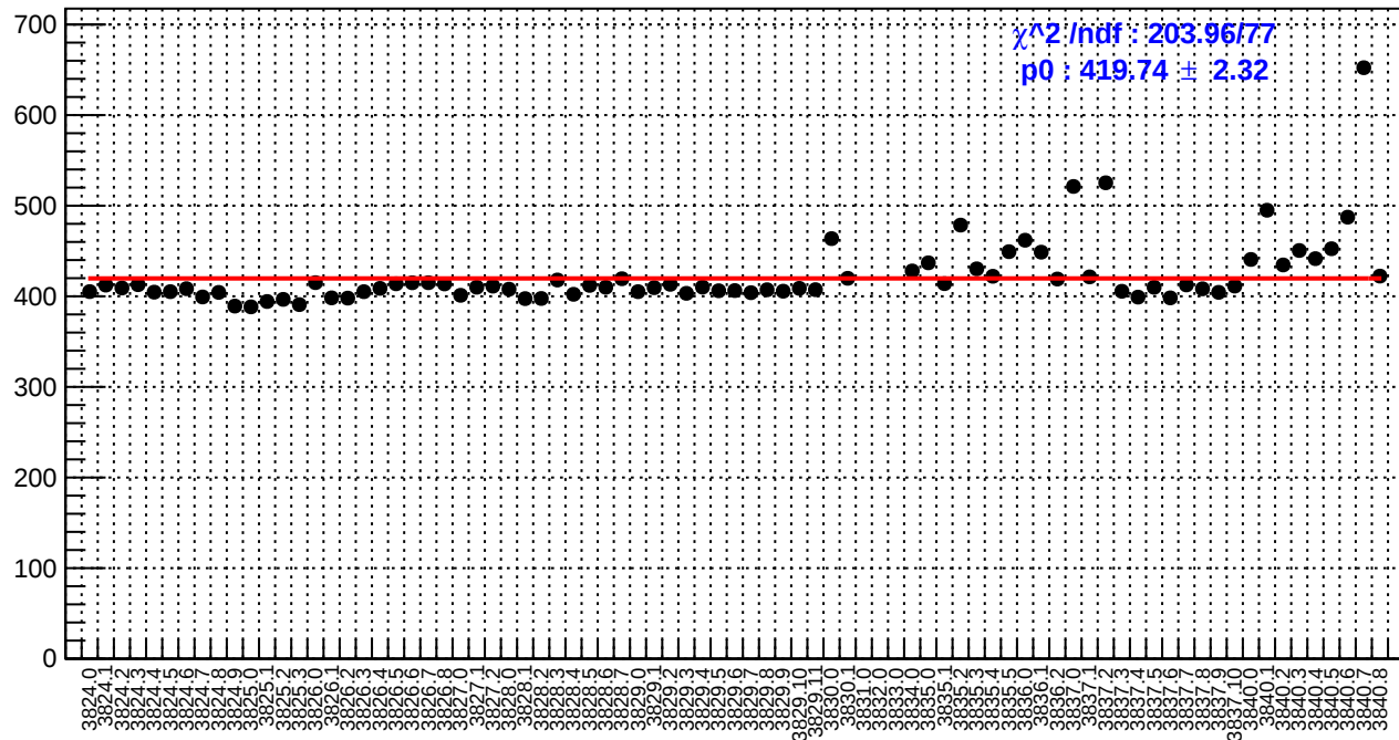
slug28: reg_asym_sam8.rms/ppm
