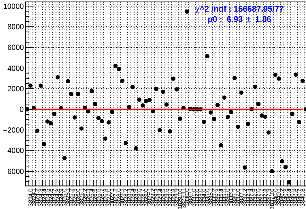
slug28: asym_us_avg.mean/ppb-reg_asym_us_avg.mean/ppb
