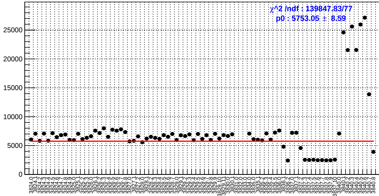
slug28: diff_bpm4aY.rms/nm
