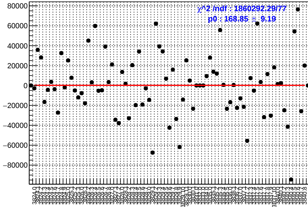
slug28: asym_sam6.mean/ppb-reg_asym_sam6.mean/ppb
