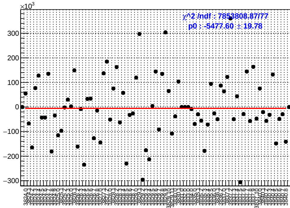
slug28: asym_sam3.mean/ppb-reg_asym_sam3.mean/ppb
