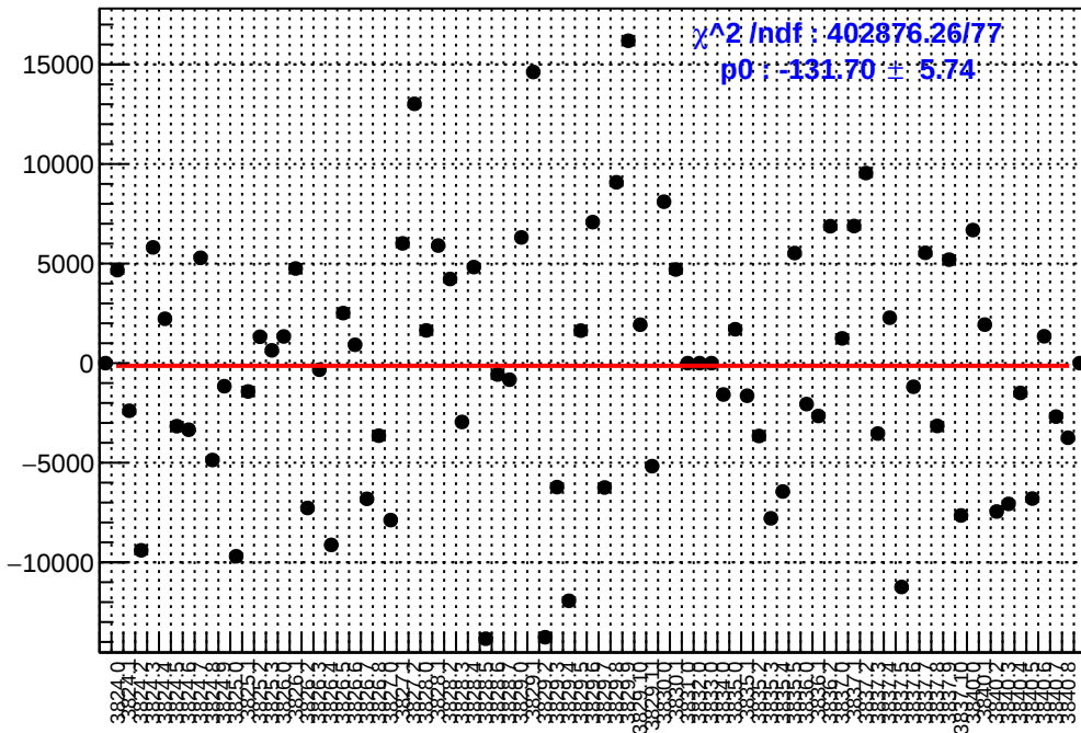
slug28: asym_left_avg.mean/ppb-reg_asym_left_avg.mean/ppb
