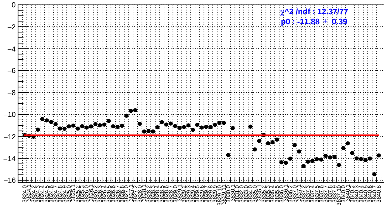
slug28: us_avg_bpm4eX/(ppb/nm)
