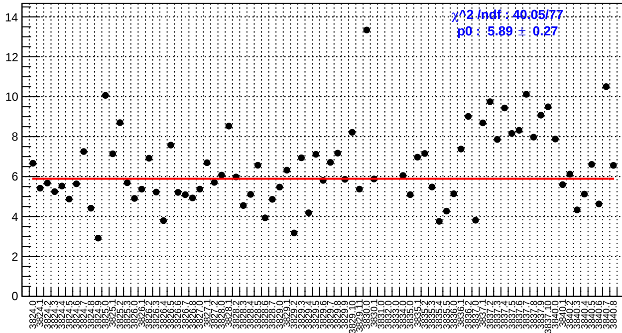
slug28: ds_avg_bpm4eY/(ppb/nm)
