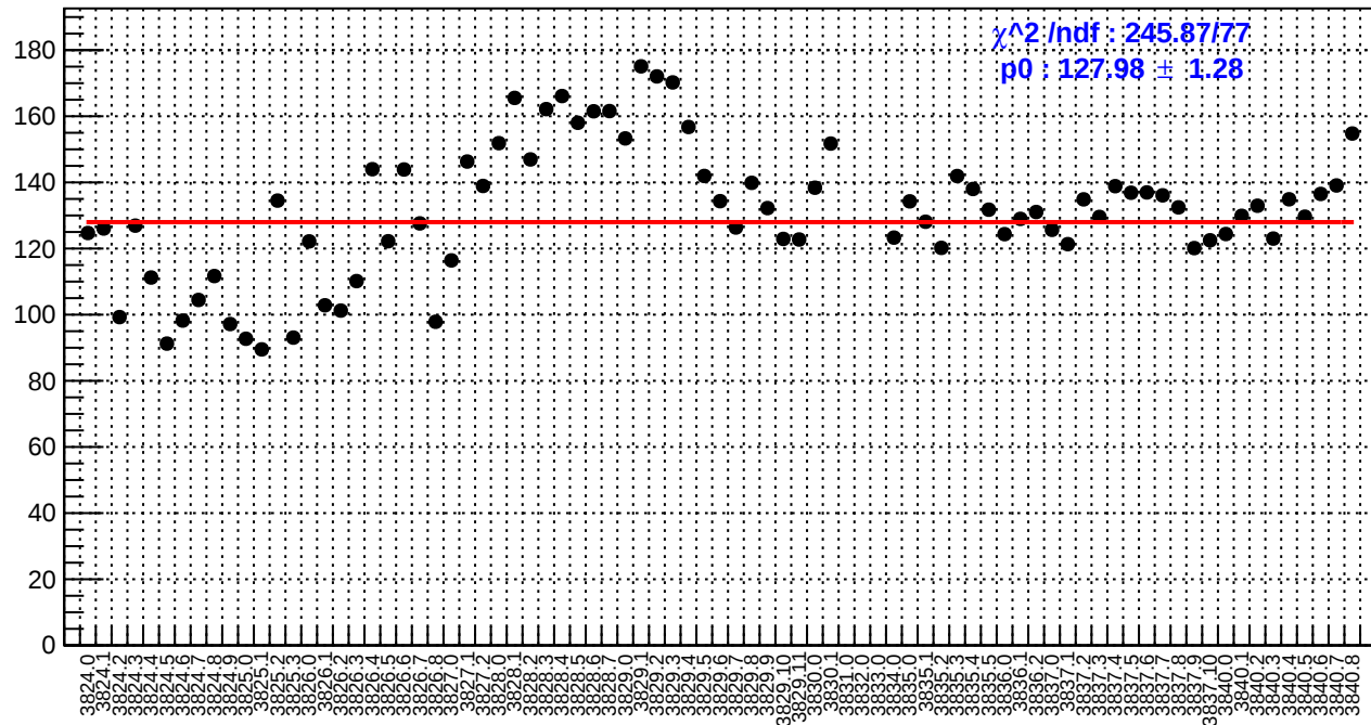
slug28: asym_bcm_an_us.rms/ppm
