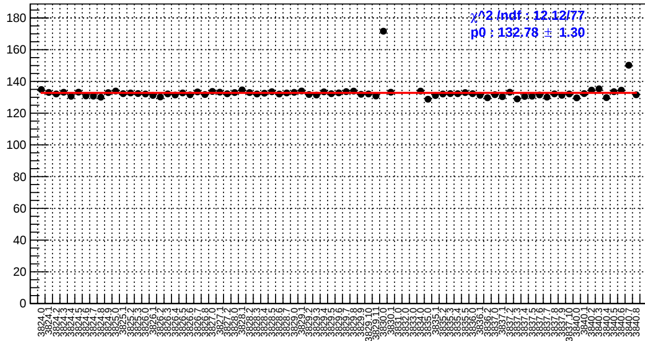
slug28: reg_asym_right_avg.rms/ppm
