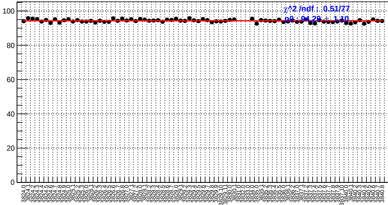
slug28: reg_asym_ds_dd.rms/ppm
