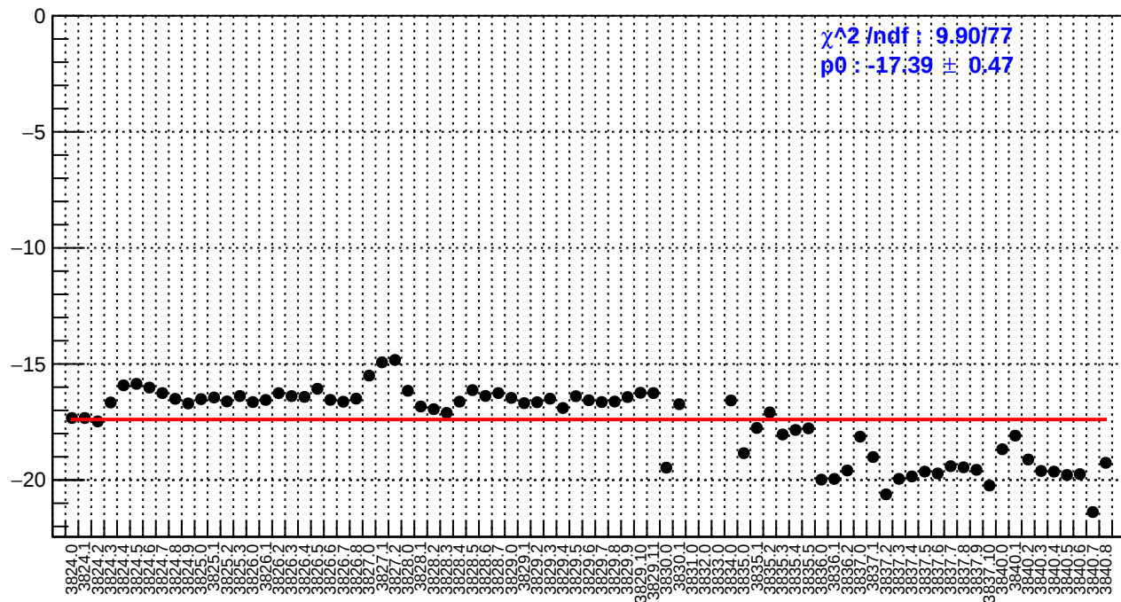
slug28: ds_avg_bpm4eX/(ppb/nm)
