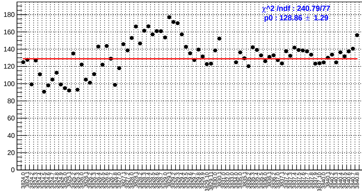
slug28: asym_bcm_an_ds.rms/ppm
