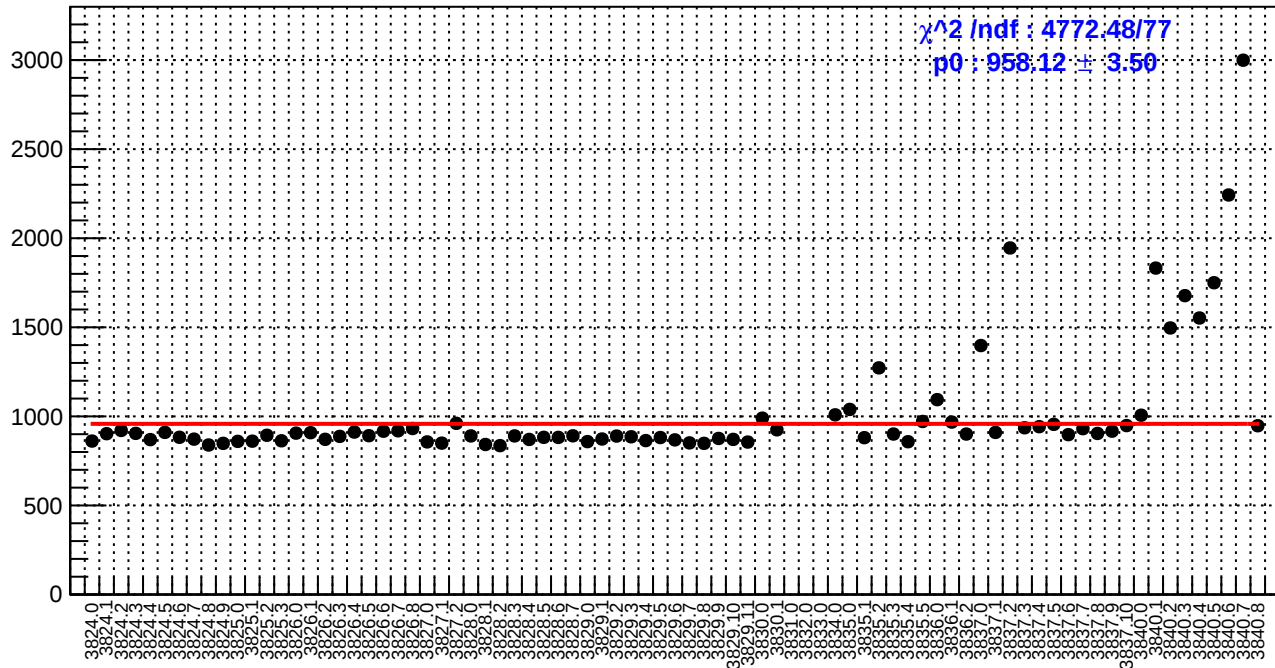
slug28: reg_asym_sam3.rms/ppm
