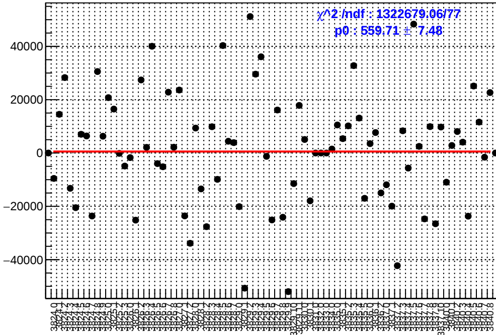
slug28: asym_sam7.mean/ppb-reg_asym_sam7.mean/ppb
