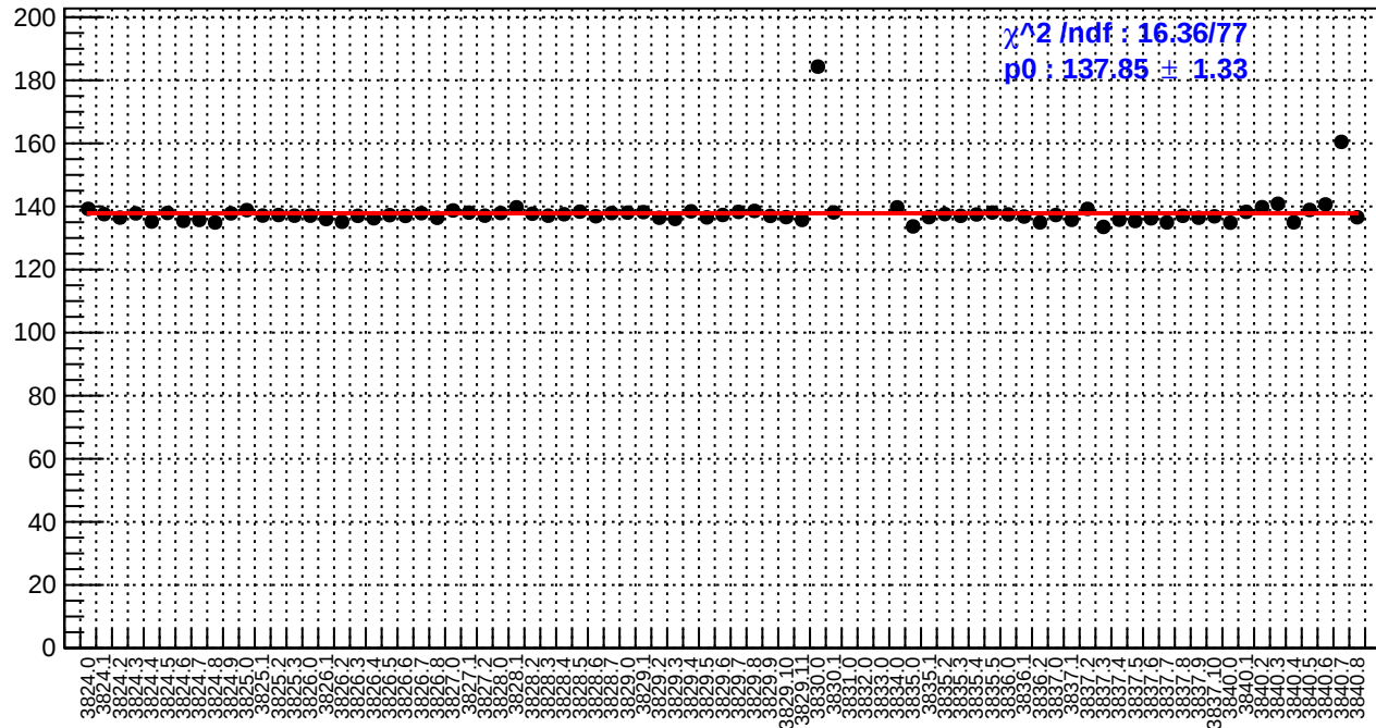
slug28: reg_asym_dsr.rms/ppm
