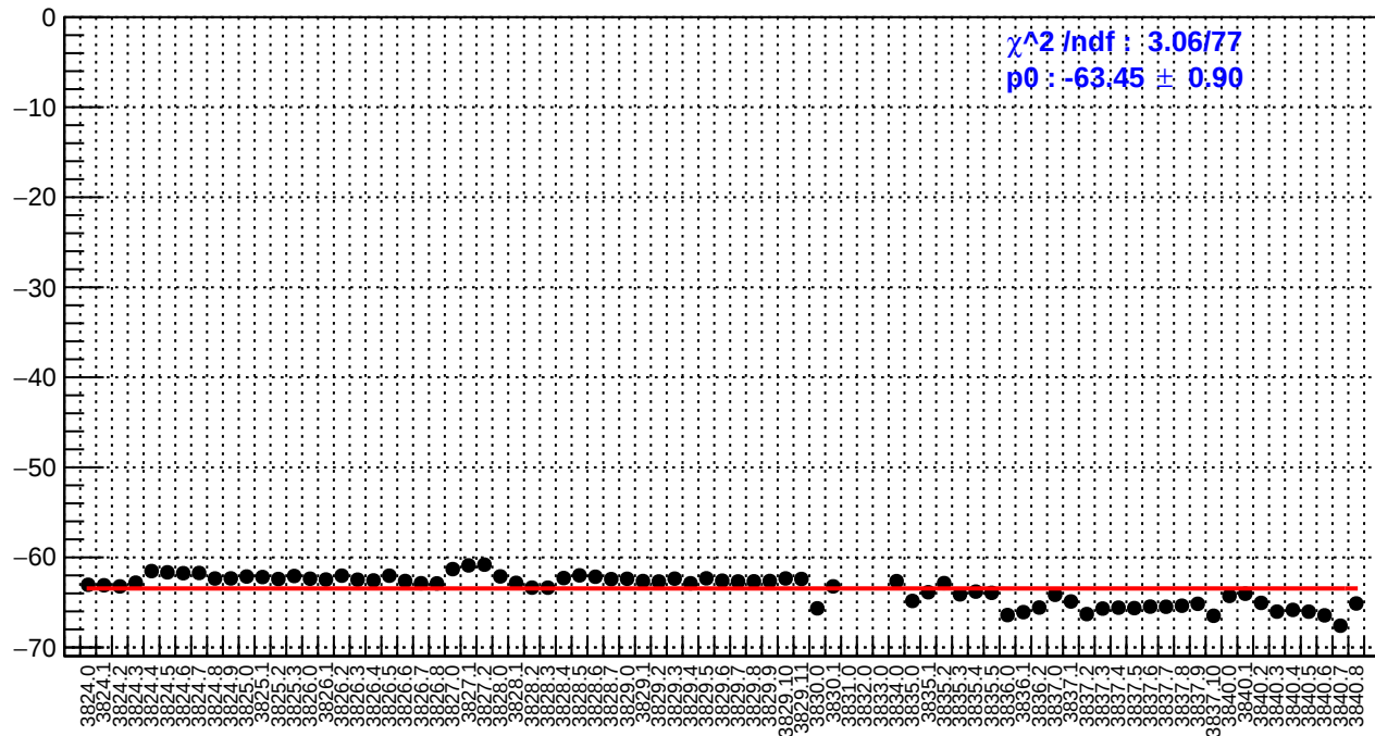
slug28: left_avg_bpm4eX/(ppb/nm)
