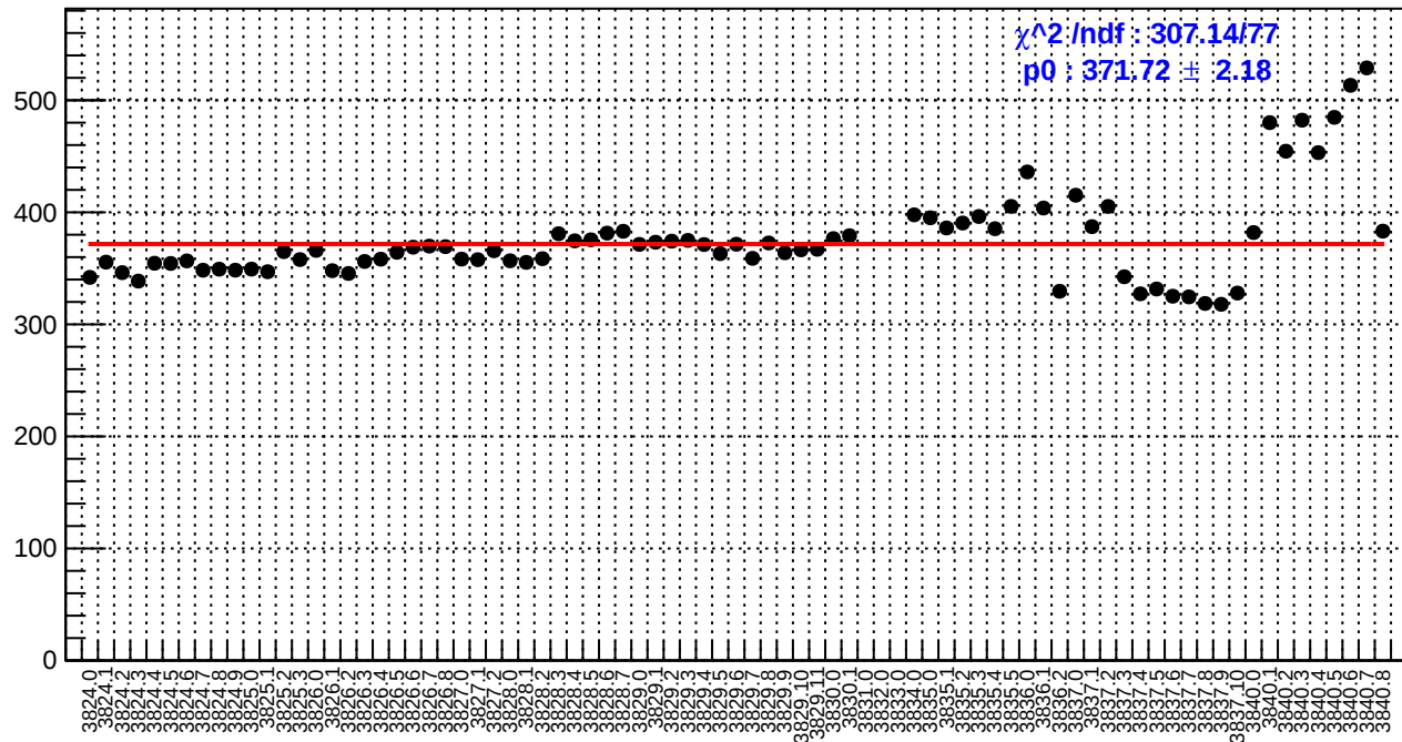
slug28: reg_asym_sam1.rms/ppm
