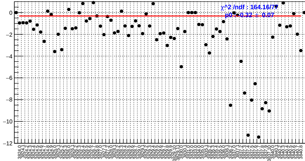
slug28: usl_bpm4aY/(ppb/nm)
