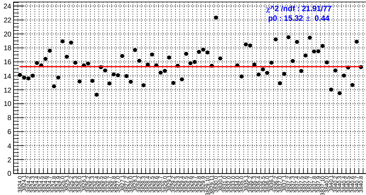
slug28: dsl_bpm4eY/(ppb/nm)
