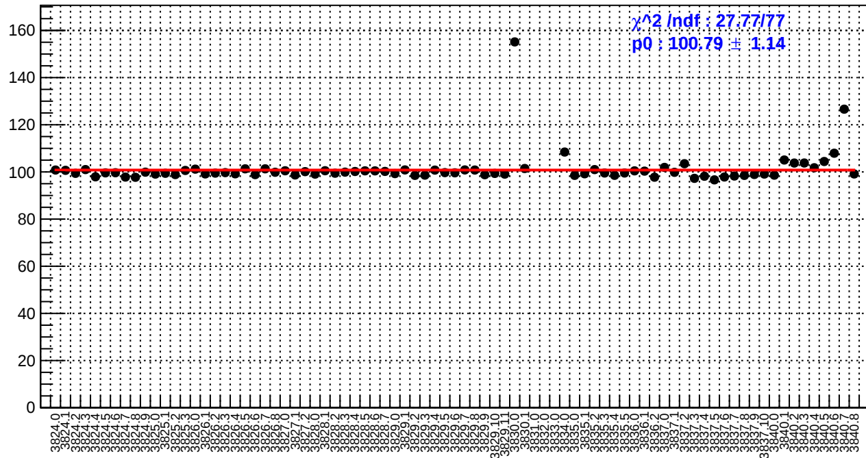
slug28: reg_asym_ds_avg.rms/ppm
