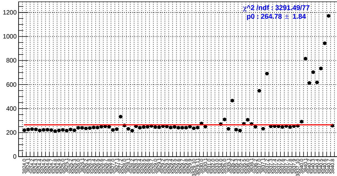
slug28: reg_asym_sam7.rms/ppm
