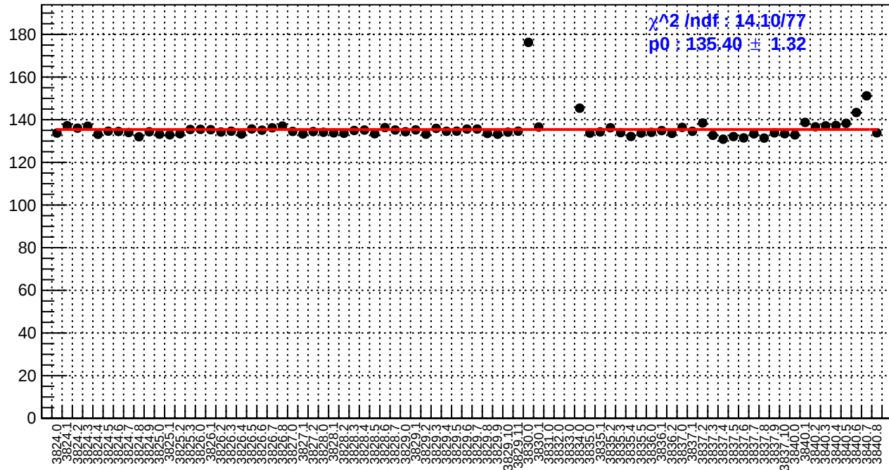
slug28: reg_asym_left_avg.rms/ppm
