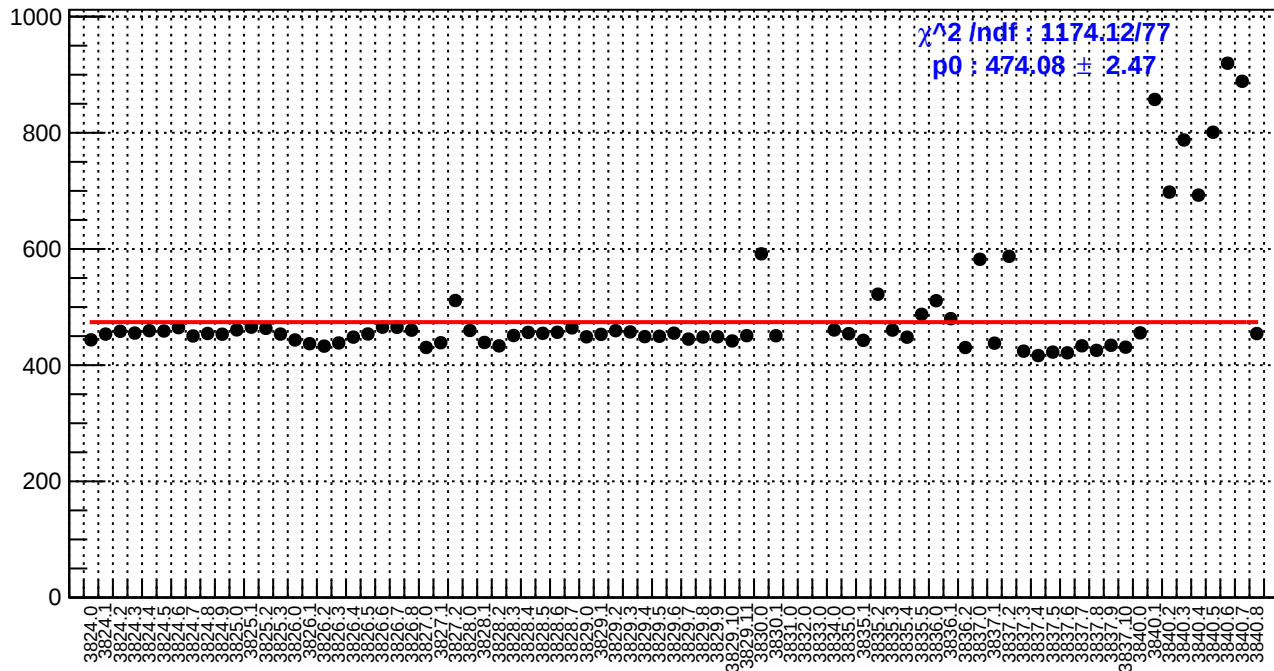
slug28: reg_asym_sam6.rms/ppm
