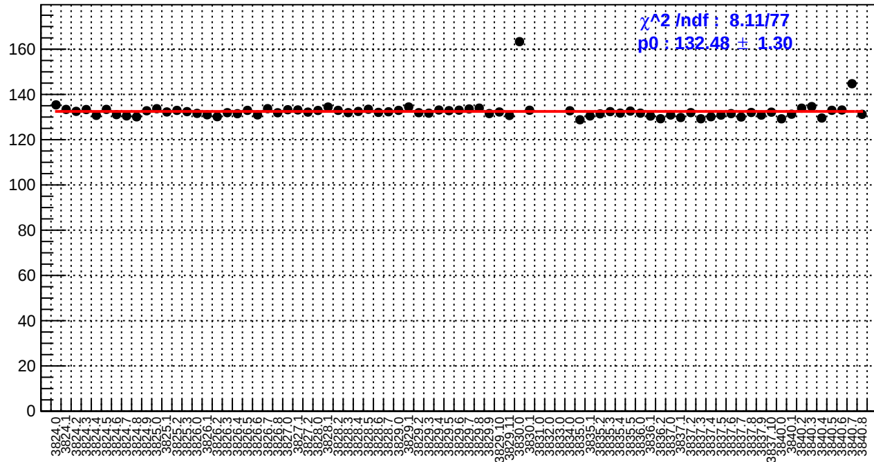
slug28: reg_asym_usr.rms/ppm
