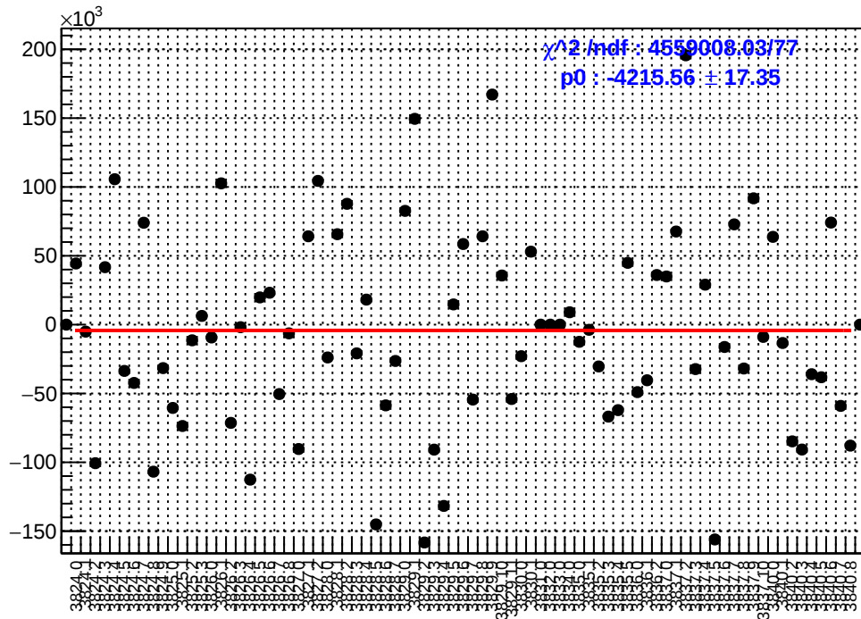
slug28: asym_sam4.mean/ppb-reg_asym_sam4.mean/ppb
