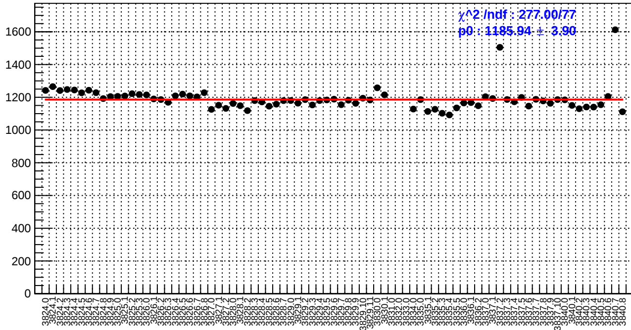
slug28: reg_asym_sam4.rms/ppm
