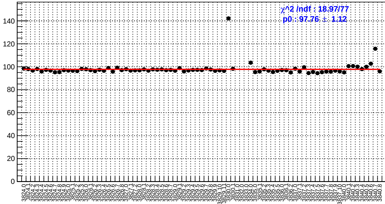
slug28: reg_asym_us_avg.rms/ppm
