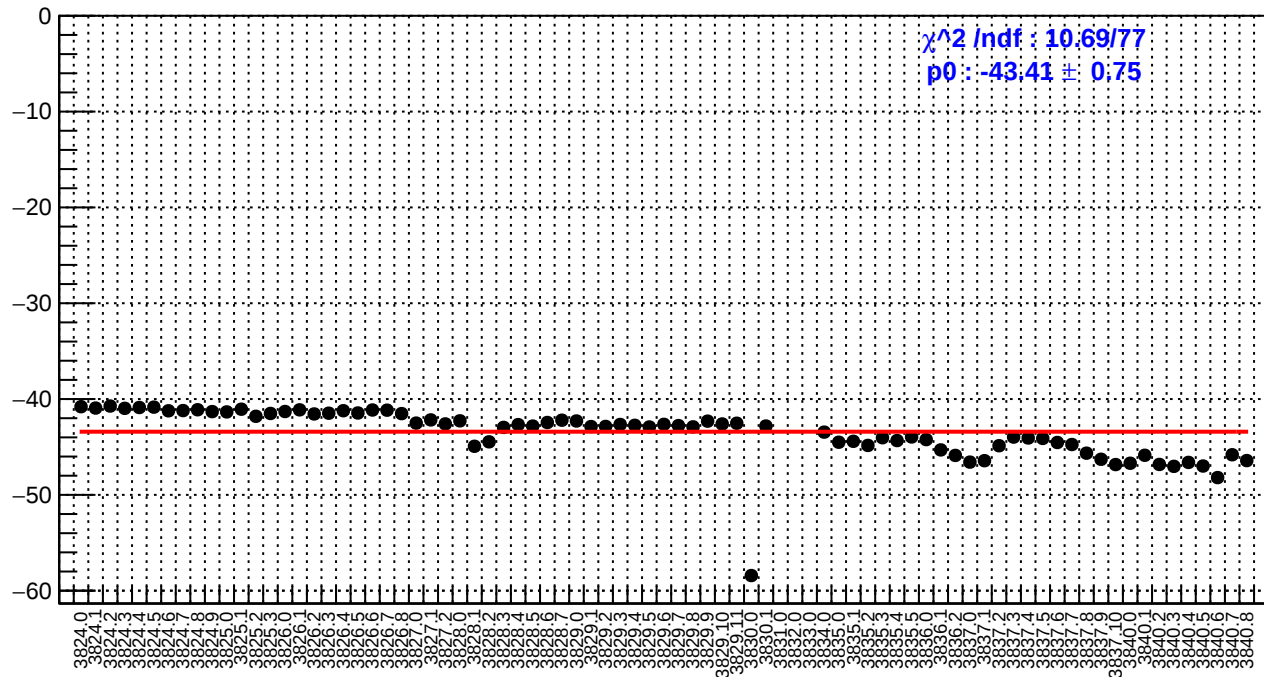
slug28: right_avg_bpm12X/(ppb/nm)
