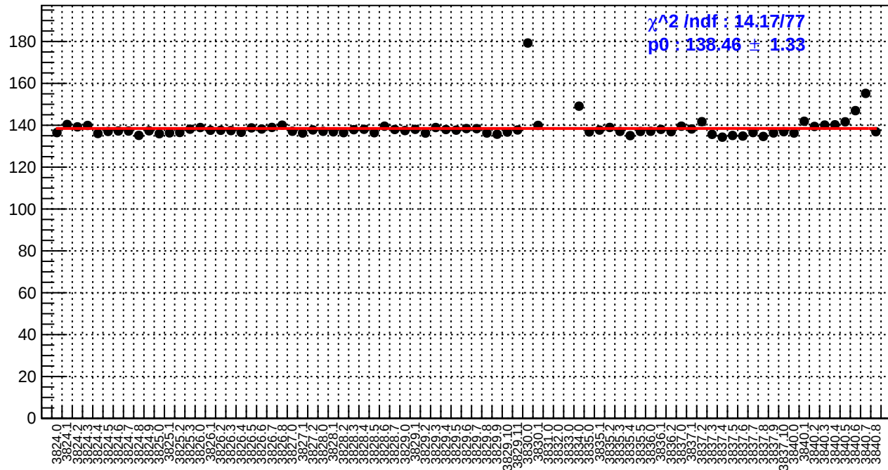
slug28: reg_asym_dsl.rms/ppm
