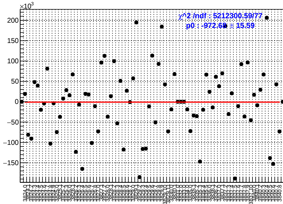
slug28: asym_sam2.mean/ppb-reg_asym_sam2.mean/ppb
