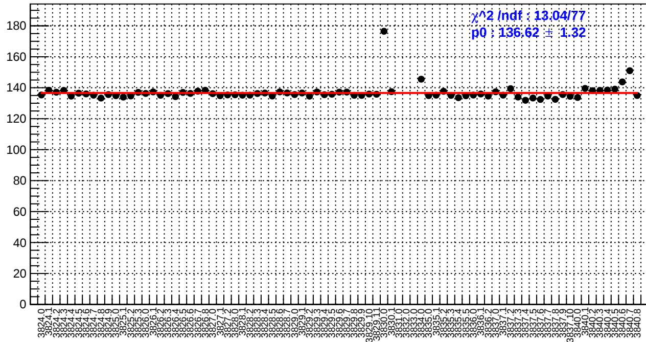
slug28: reg_asym_usl.rms/ppm
