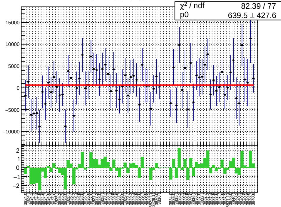
slug28: reg_asym_sam1.mean/ppb
