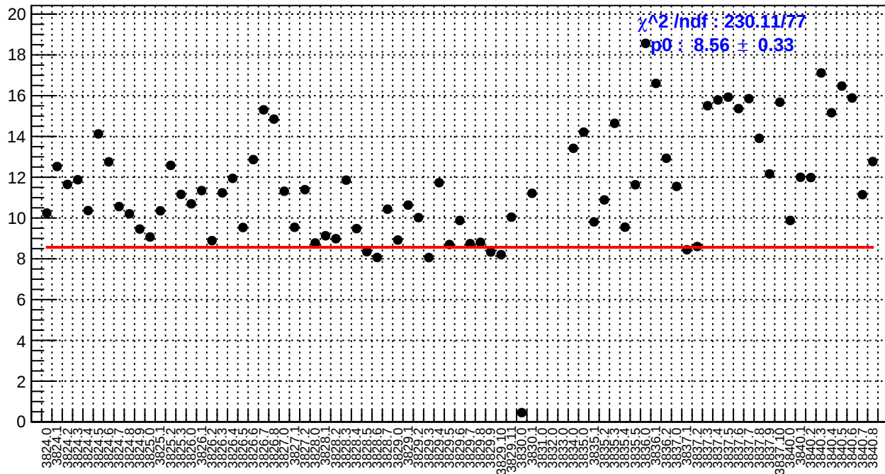
slug28: usl_bpm4aX/(ppb/nm)
