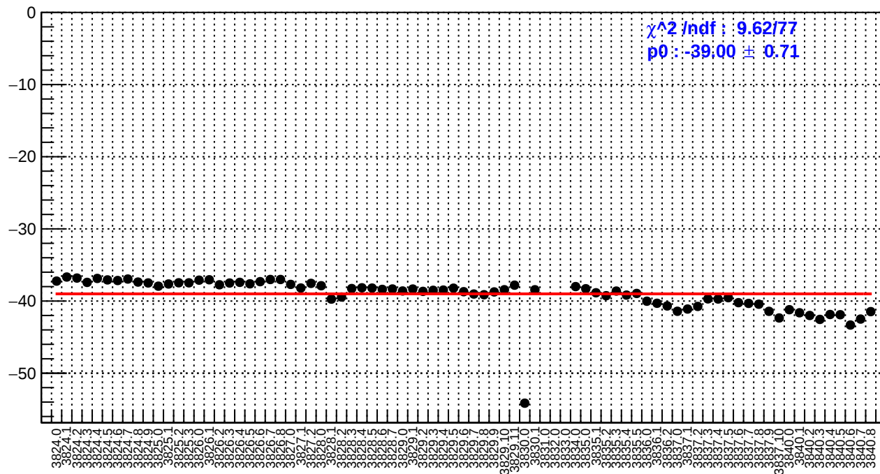
slug28: usl_bpm12X/(ppb/nm)
