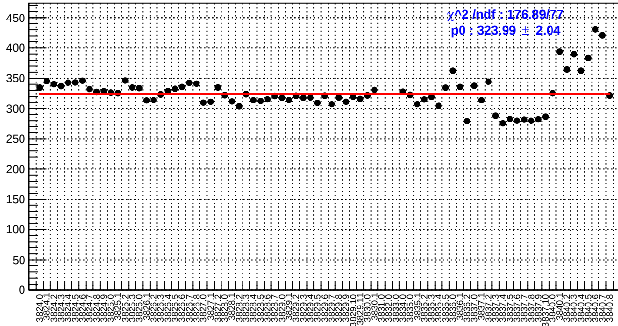
slug28: reg_asym_sam5.rms/ppm
