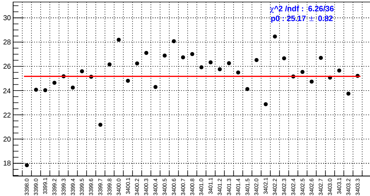
slug3: right_avg_bpm4aY/(ppb/nm)
