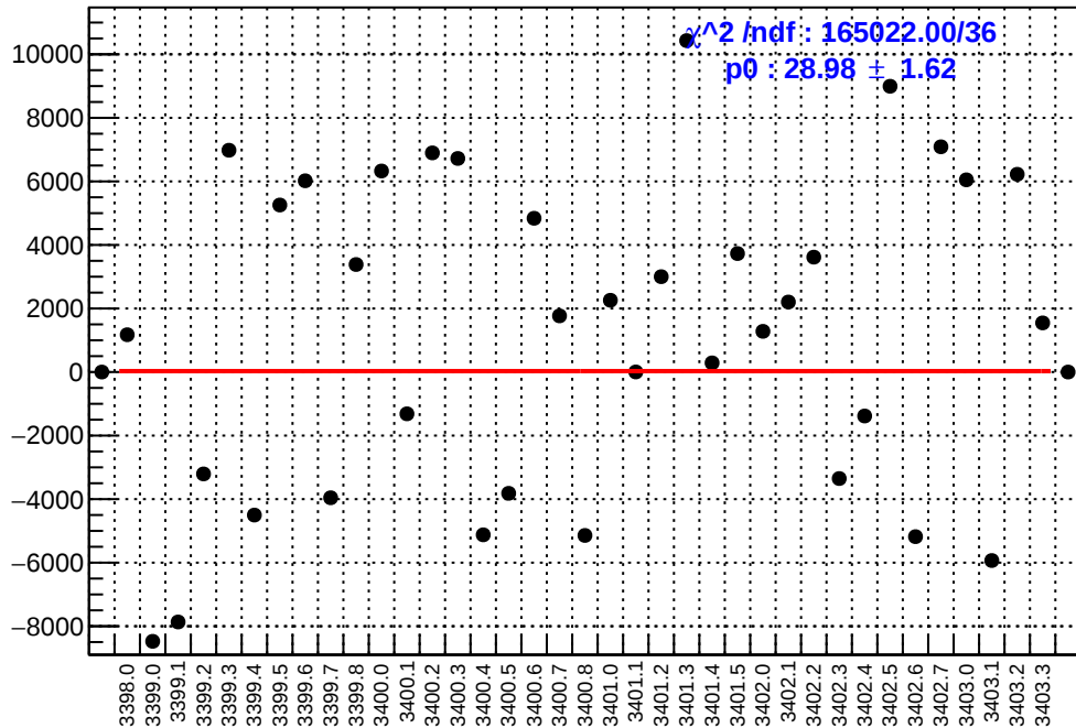
slug3: asym_usl.mean/ppb-reg_asym_usl.mean/ppb
