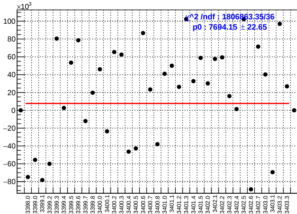
slug3: asym_sam4.mean/ppb-reg_asym_sam4.mean/ppb
