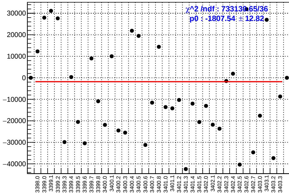
slug3: asym_sam7.mean/ppb-reg_asym_sam7.mean/ppb
