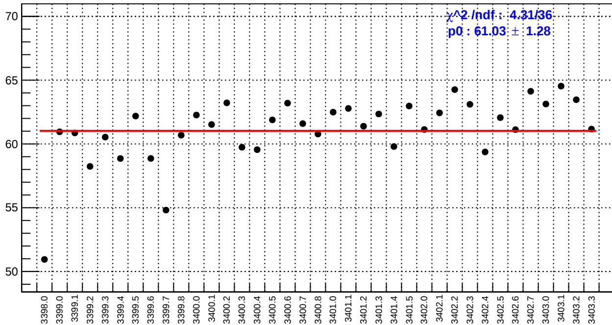
slug3: dsl_bpm4eY/(ppb/nm)
