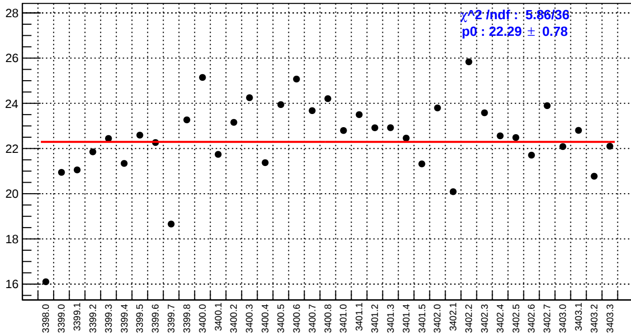
slug3: dsr_bpm4aY/(ppb/nm)
