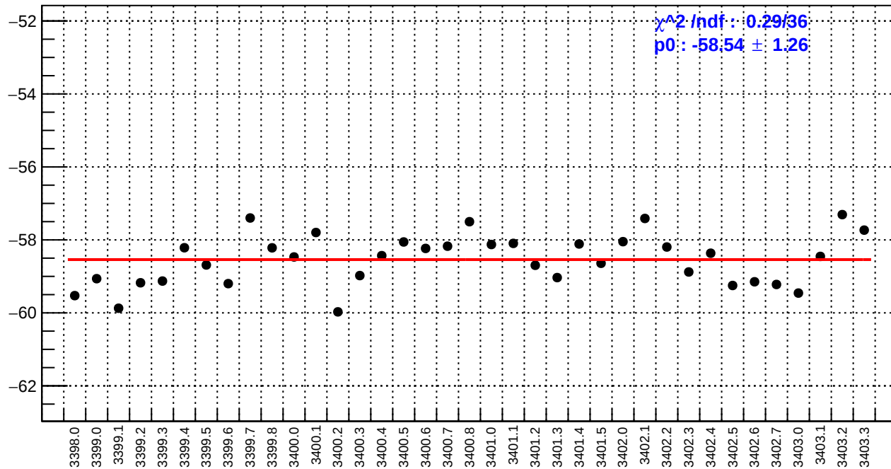
slug3: dsr_bpm12X/(ppb/nm)
