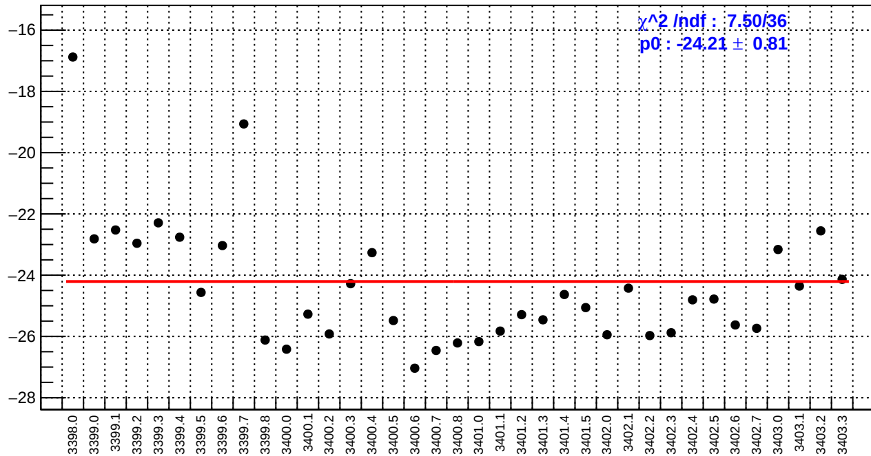
slug3: right_avg_bpm4eY/(ppb/nm)
