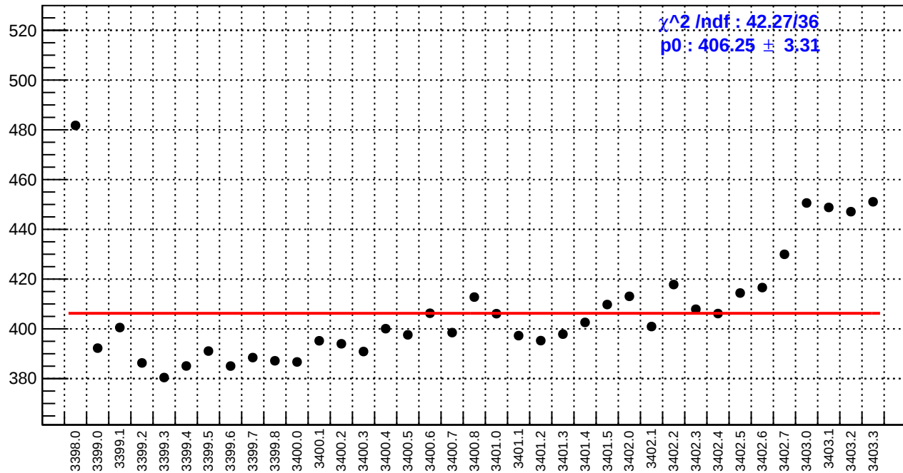
slug3: reg_asym_sam5.rms/ppm
