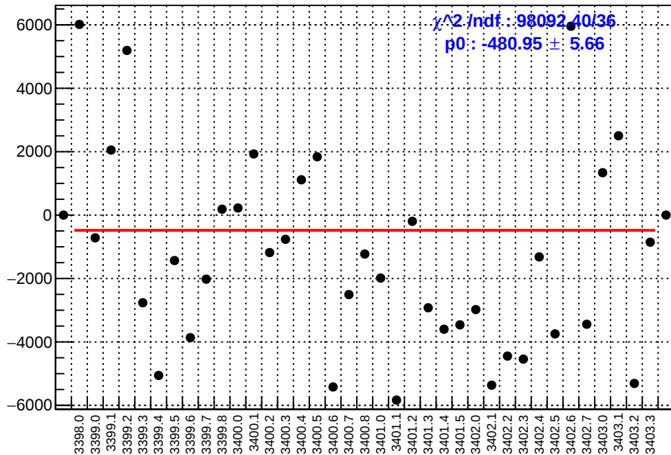
slug3: asym_dsr.mean/ppb-reg_asym_dsr.mean/ppb
