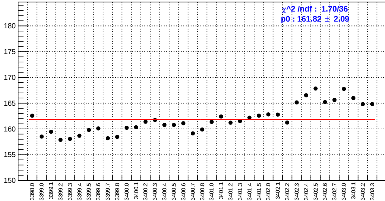
slug3: reg_asym_usl.rms/ppm
