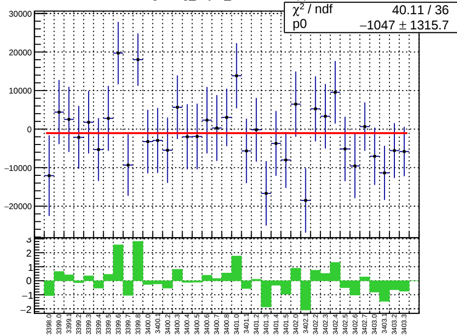
slug3: reg_asym_sam6.mean/ppb
