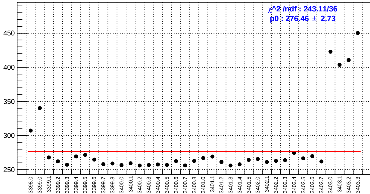
slug3: reg_asym_sam8.rms/ppm
