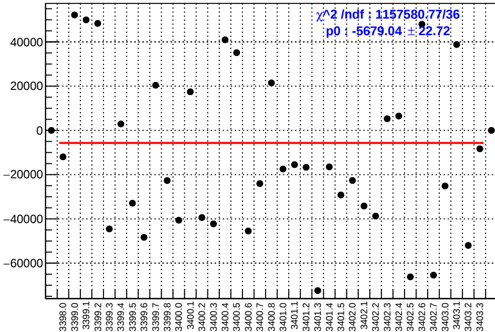
slug3: asym_sam6.mean/ppb-reg_asym_sam6.mean/ppb
