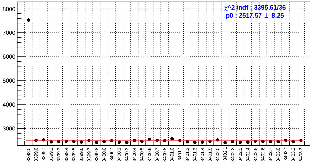
slug3: diff_bpm4aY.rms/nm
