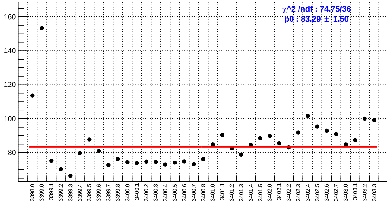
slug3: asym_bcm_an_ds.rms/ppm
