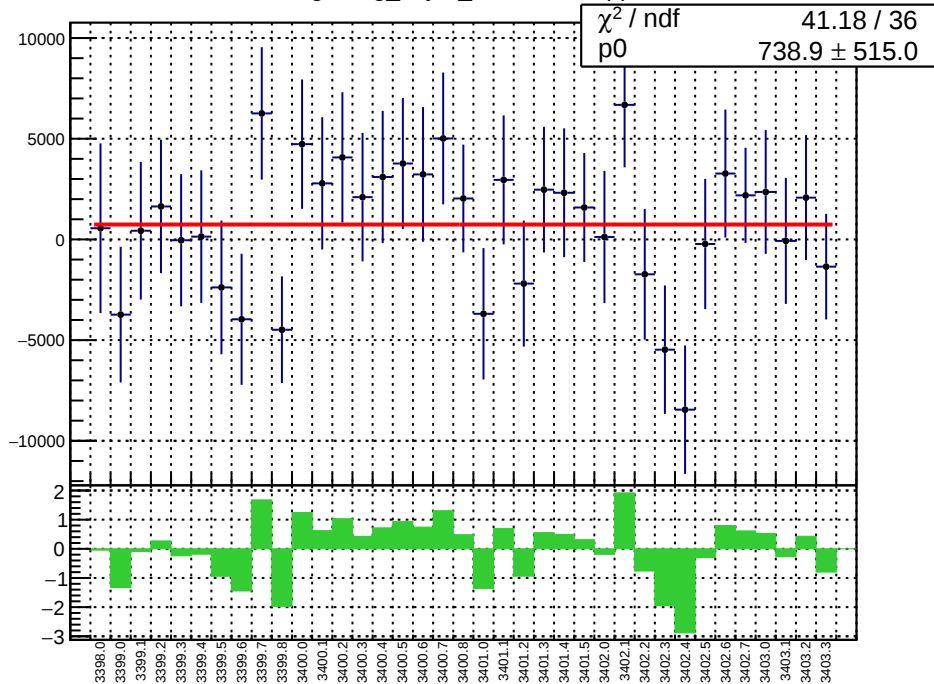
slug3: reg_asym_sam1.mean/ppb
