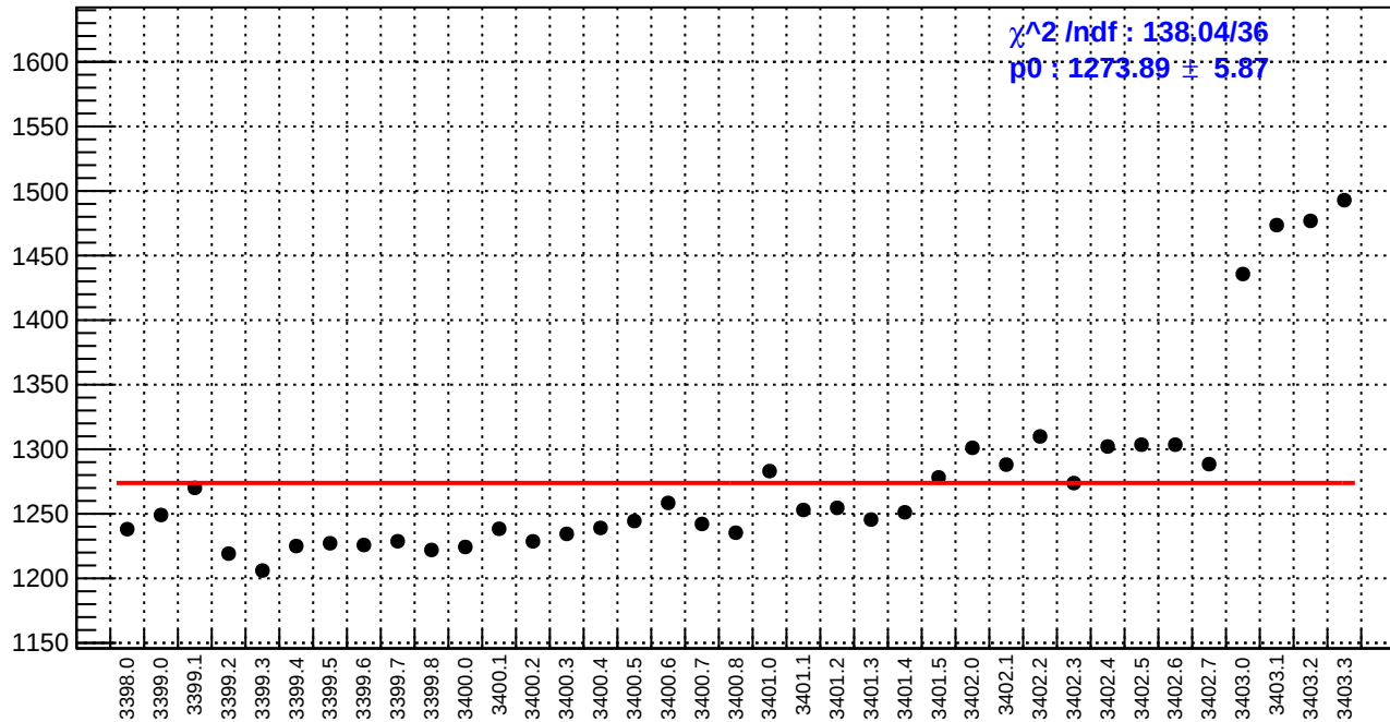
slug3: reg_asym_sam4.rms/ppm
