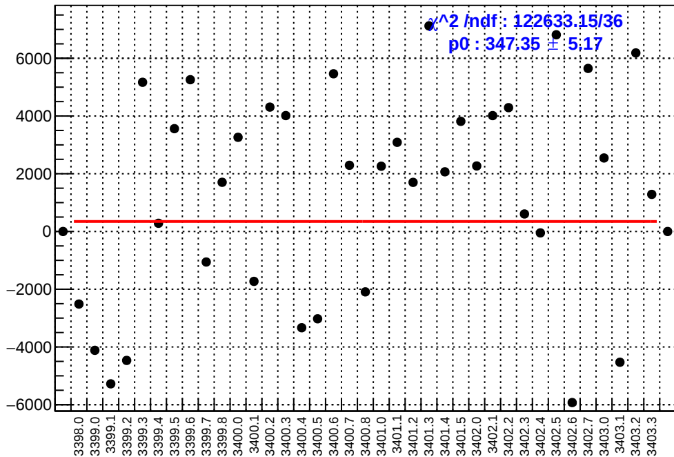
slug3: asym_ds_dd.mean/ppb-reg_asym_ds_dd.mean/ppb
