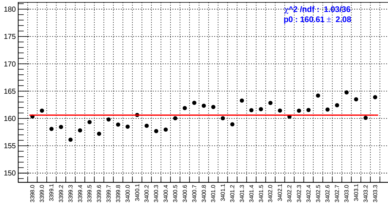
slug3: reg_asym_usr.rms/ppm
