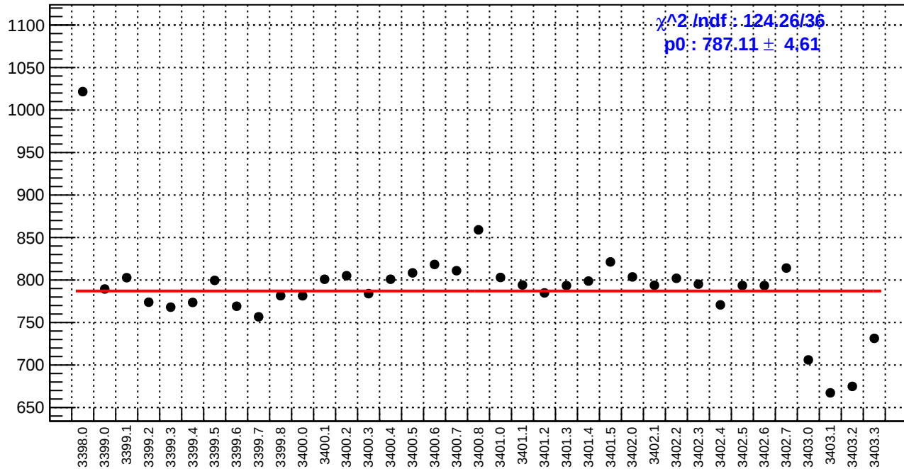
slug3: reg_asym_sam6.rms/ppm
