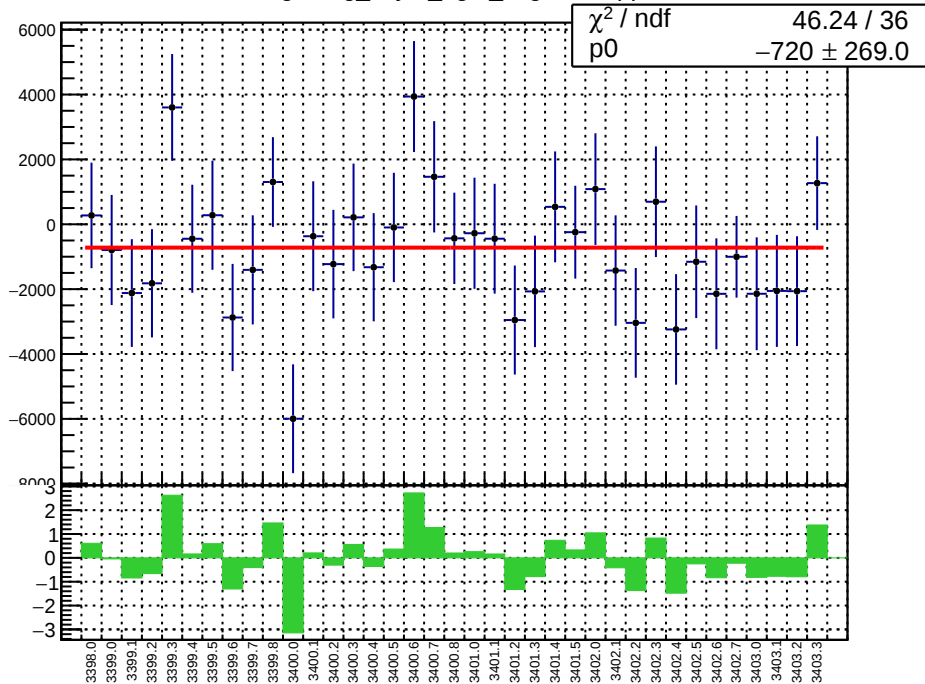
slug3: reg_asym_right_avg.mean/ppb
