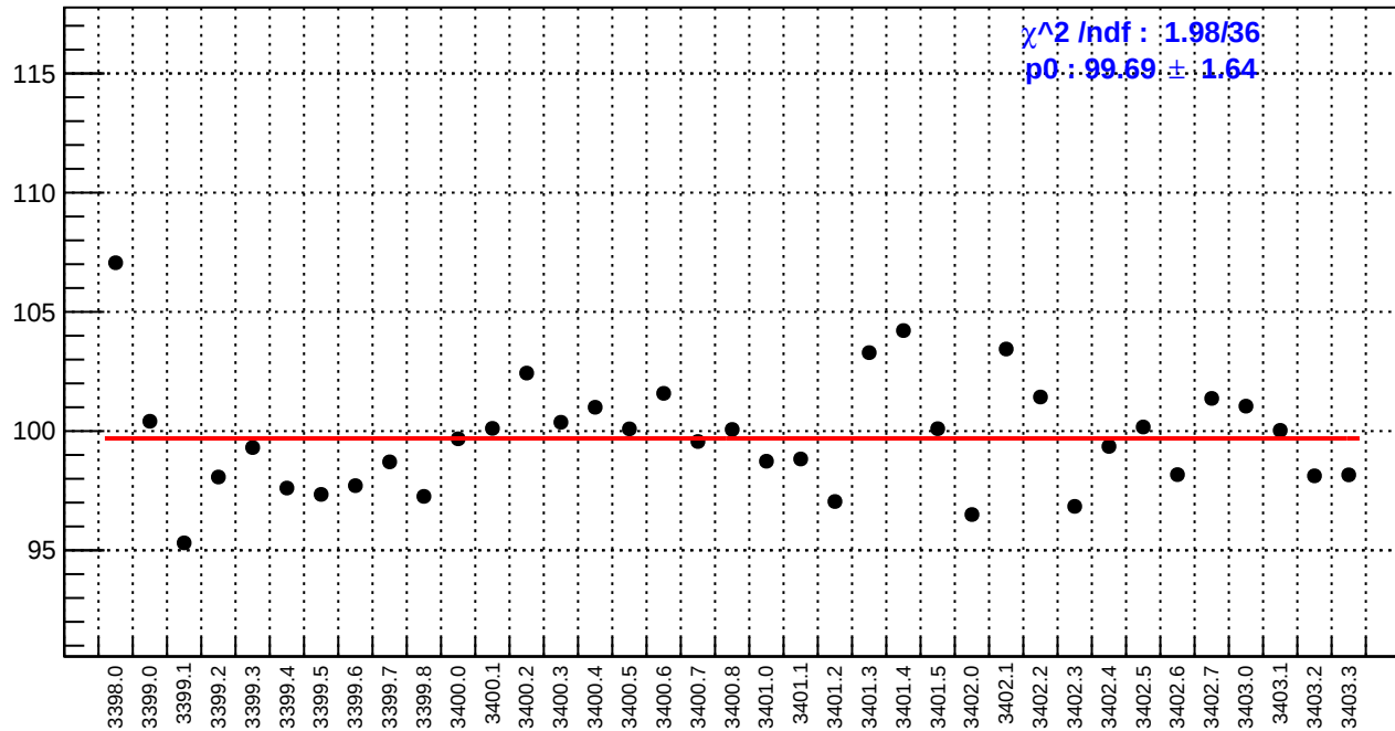
slug3: left_avg_bpm4aX/(ppb/nm)
