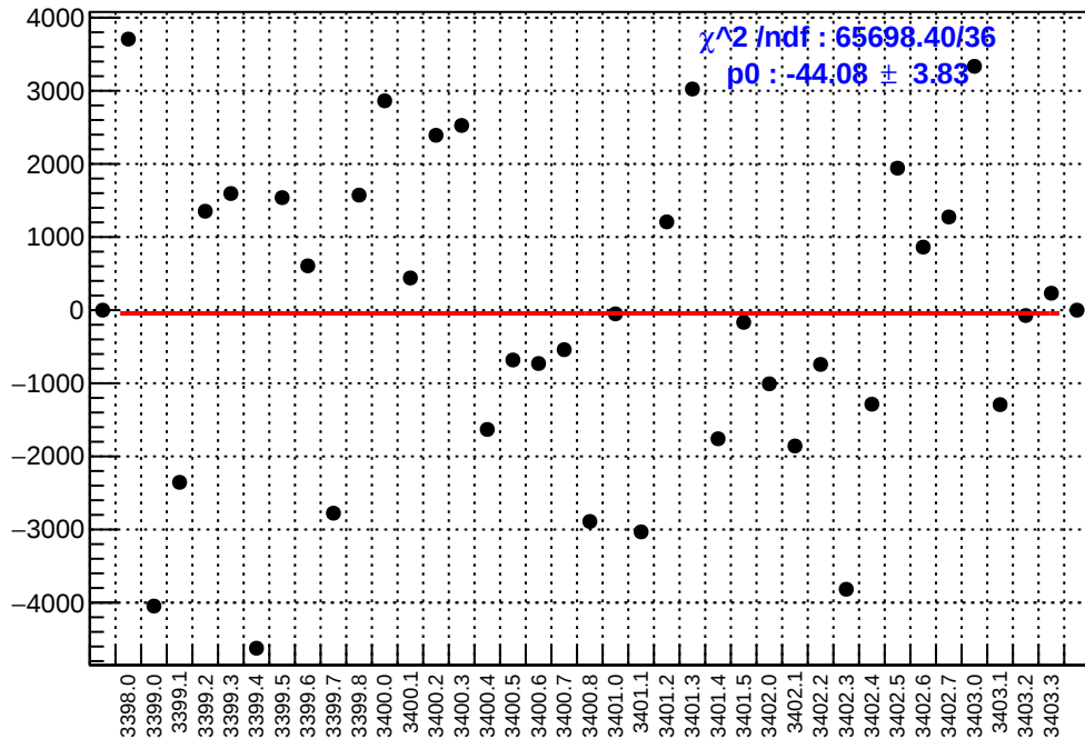
slug3: asym_us_avg.mean/ppb-reg_asym_us_avg.mean/ppb
