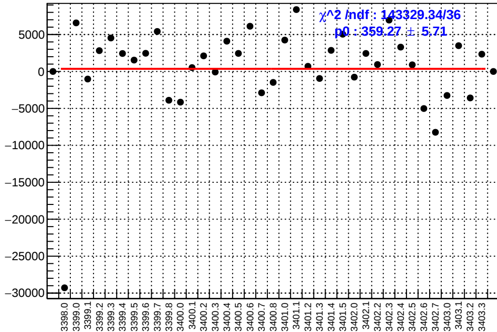
slug3: asym_sam5.mean/ppb-reg_asym_sam5.mean/ppb
