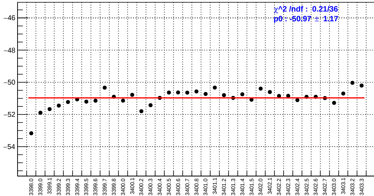
slug3: us_avg_bpm12X/(ppb/nm)
