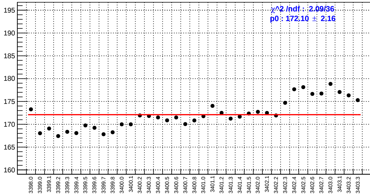
slug3: reg_asym_dsl.rms/ppm
