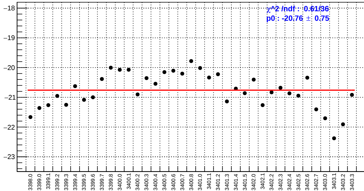
slug3: ds_avg_bpm4eX/(ppb/nm)
