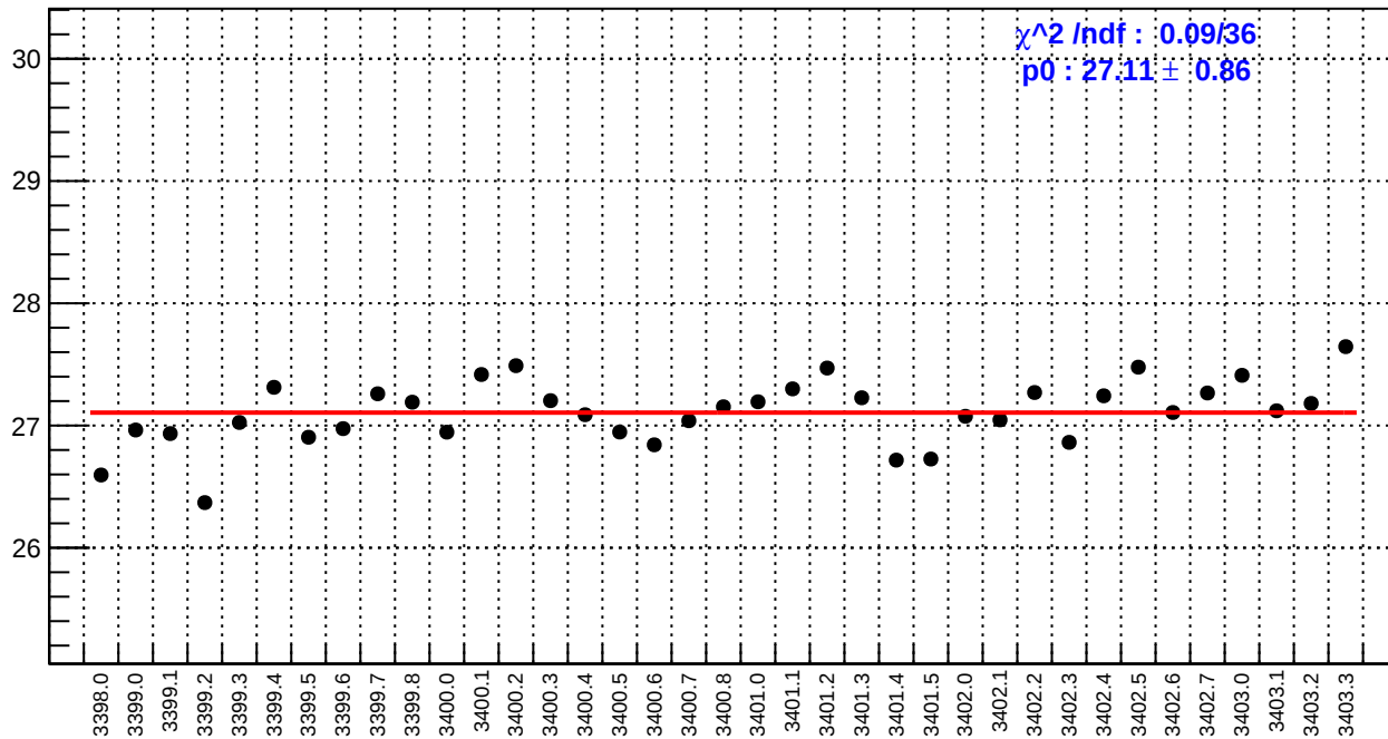
slug3: reg_asym_right_dd.rms/ppm
