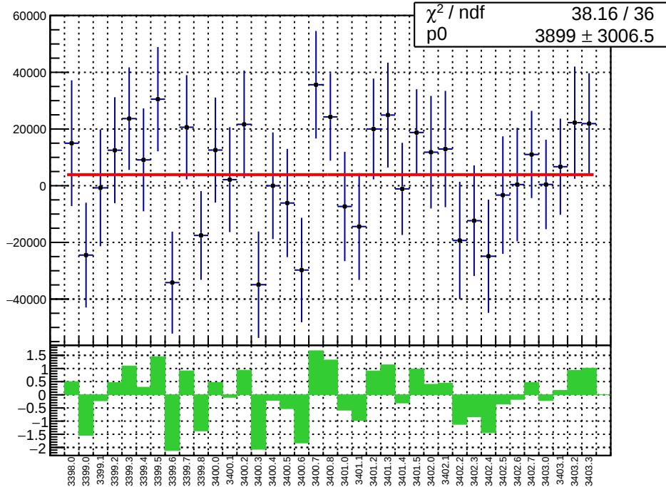
slug3: reg_asym_sam3.mean/ppb
