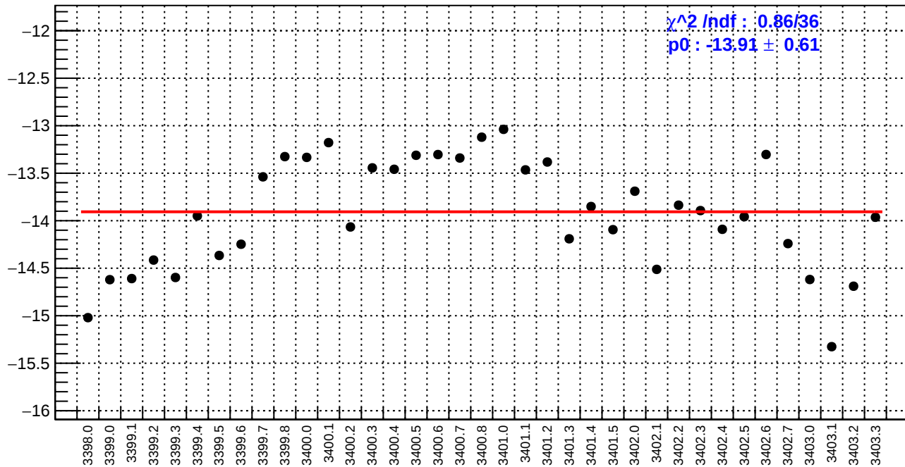
slug3: us_avg_bpm4eX/(ppb/nm)
