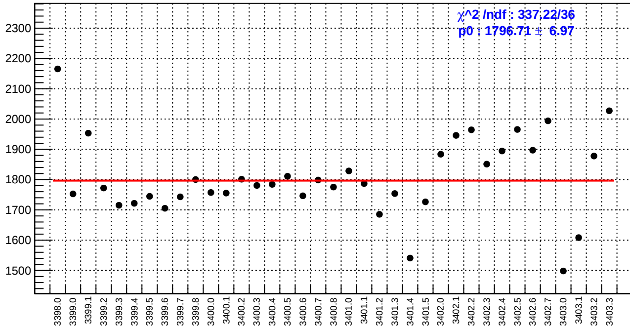
slug3: reg_asym_sam3.rms/ppm
