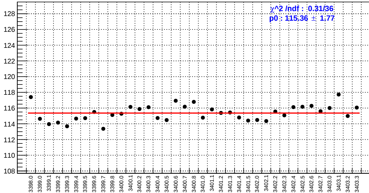
slug3: reg_asym_ds_dd.rms/ppm
