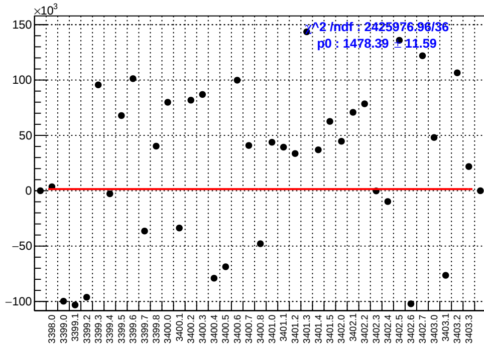
slug3: asym_sam2.mean/ppb-reg_asym_sam2.mean/ppb
