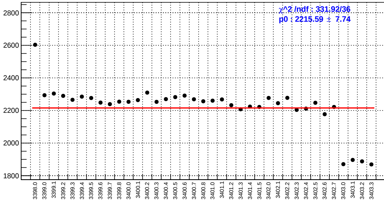
slug3: reg_asym_sam2.rms/ppm
