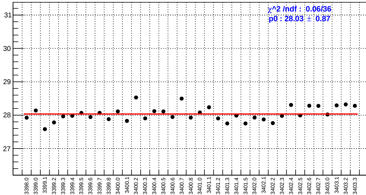
slug3: reg_asym_left_dd.rms/ppm
