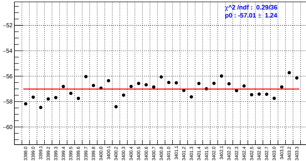
slug3: right_avg_bpm12X/(ppb/nm)
