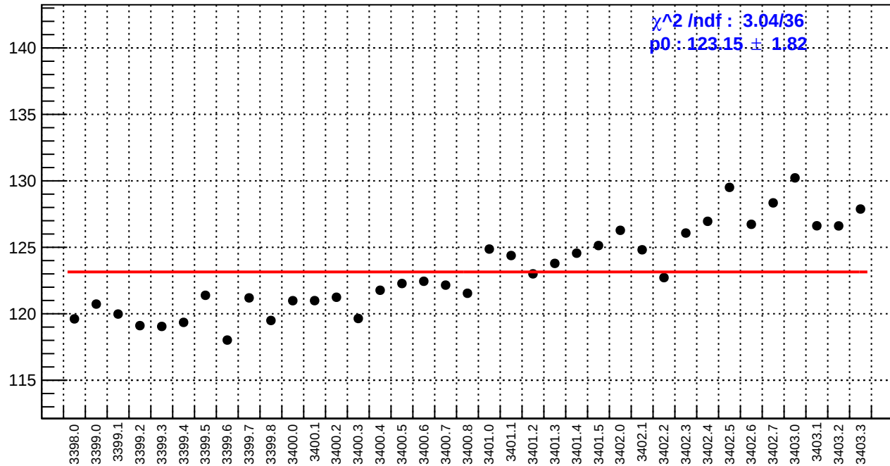
slug3: reg_asym_ds_avg.rms/ppm
