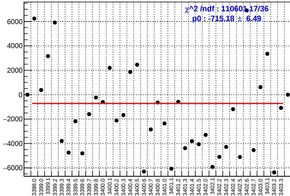
slug3: asym_usr.mean/ppb-reg_asym_usr.mean/ppb
