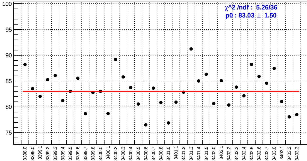
slug3: dsr_bpm4aX/(ppb/nm)
