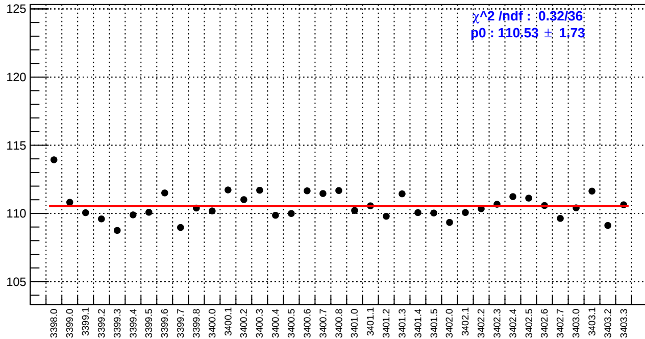
slug3: reg_asym_us_dd.rms/ppm
