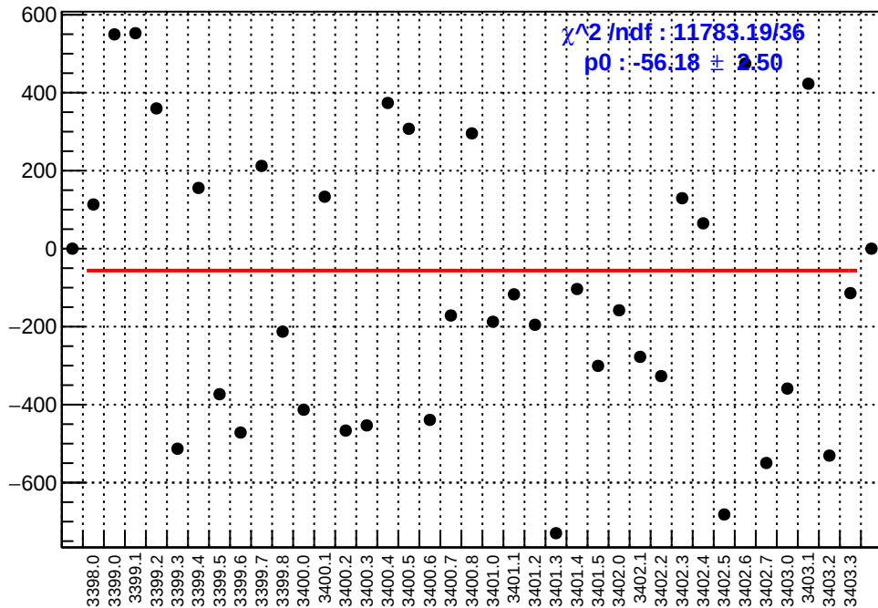
slug3: asym_right_dd.mean/ppb-reg_asym_right_dd.mean/ppb
