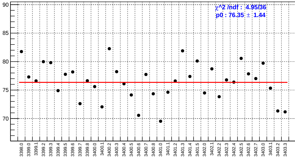
slug3: usr_bpm4aX/(ppb/nm)
