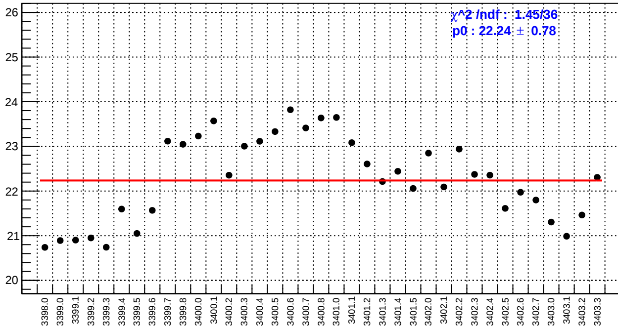
slug3: dsr_bpm4eX/(ppb/nm)
