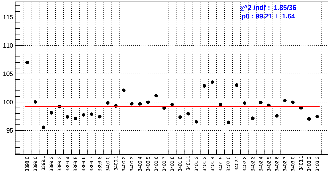
slug3: usl_bpm4aX/(ppb/nm)
