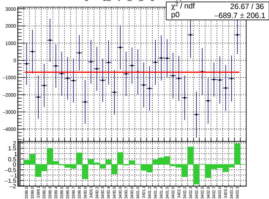
slug3: reg_asym_ds_avg.mean/ppb
