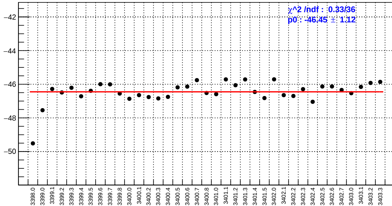
slug3: usl_bpm12X/(ppb/nm)
