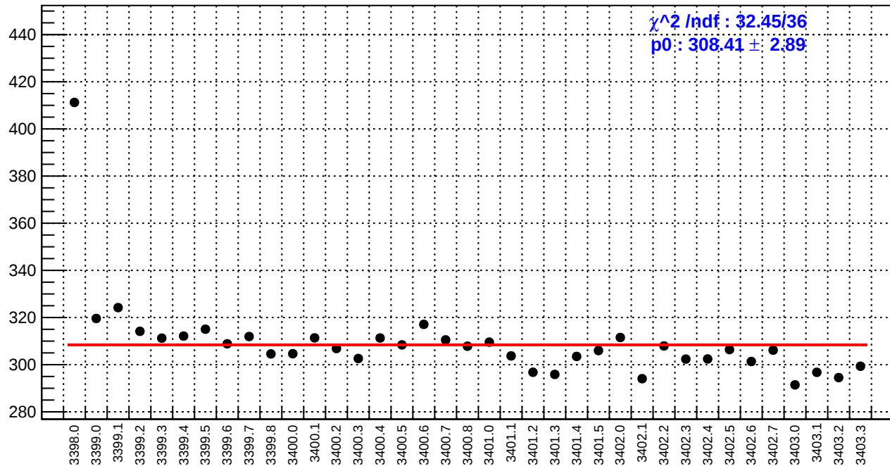
slug3: reg_asym_sam1.rms/ppm
