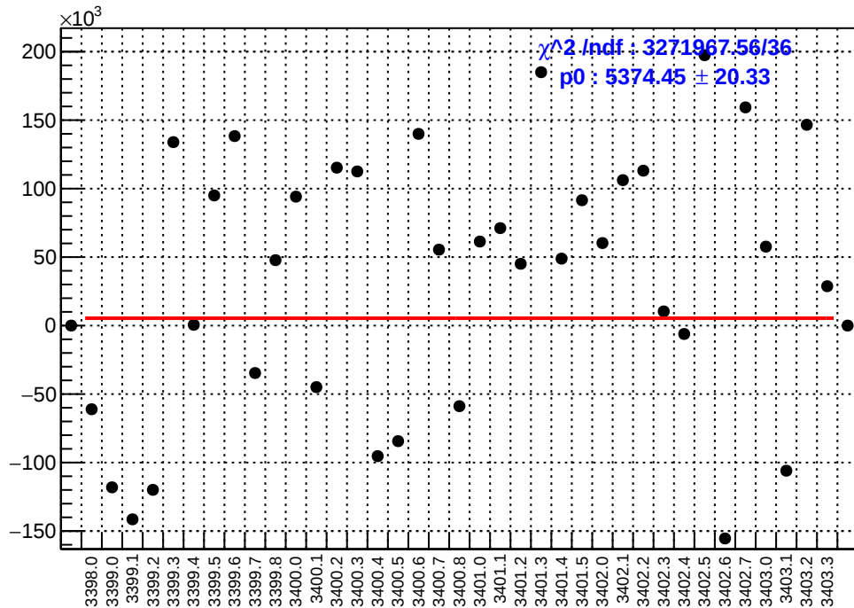
slug3: asym_sam3.mean/ppb-reg_asym_sam3.mean/ppb
