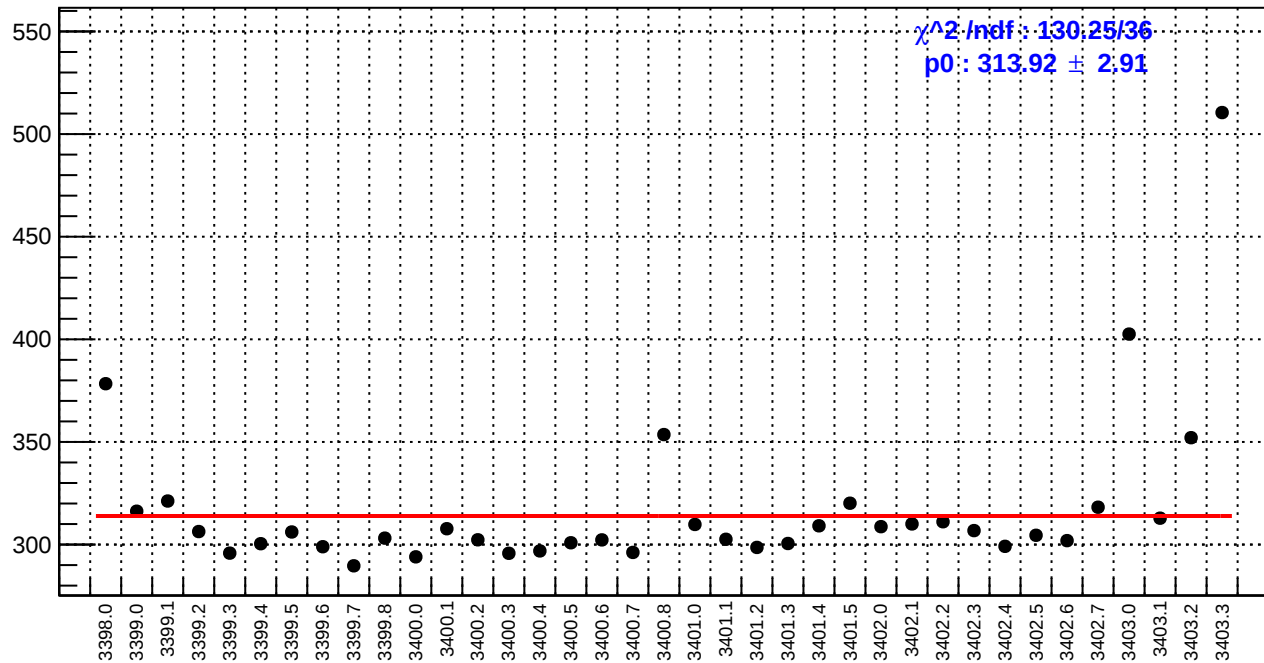
slug3: reg_asym_sam7.rms/ppm
