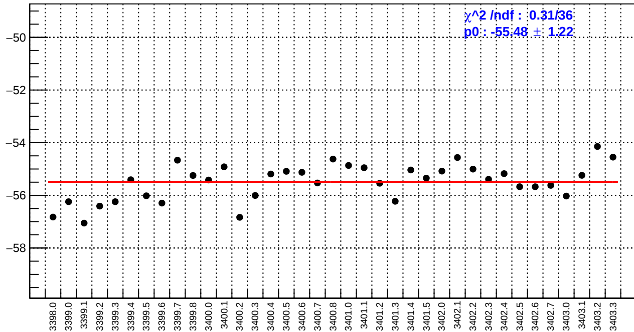
slug3: usr_bpm12X/(ppb/nm)
