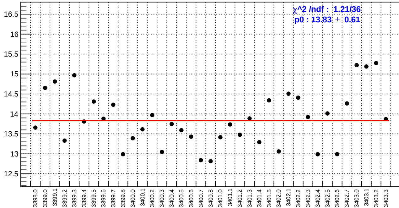
slug3: us_avg_bpm4eY/(ppb/nm)
