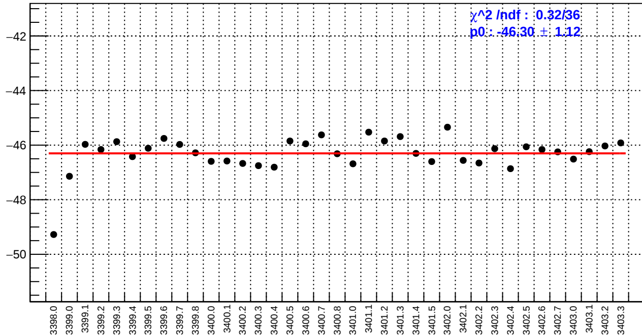
slug3: left_avg_bpm12X/(ppb/nm)
