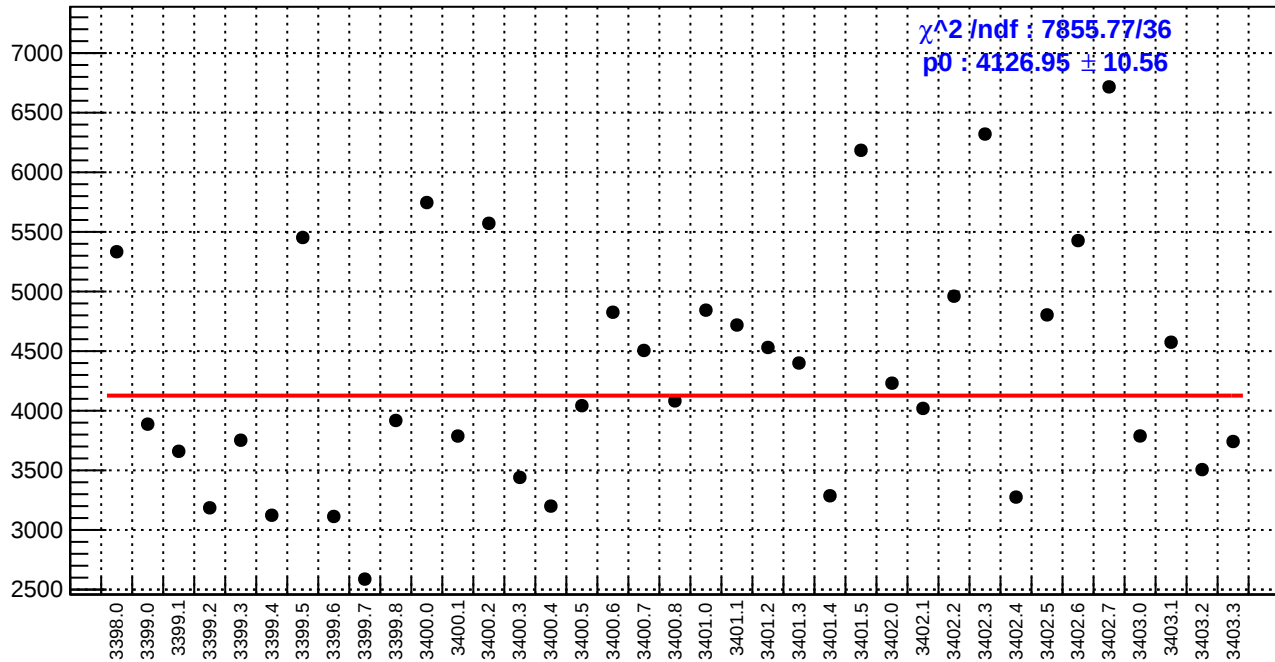
slug3: diff_bpm4eY.rms/nm
