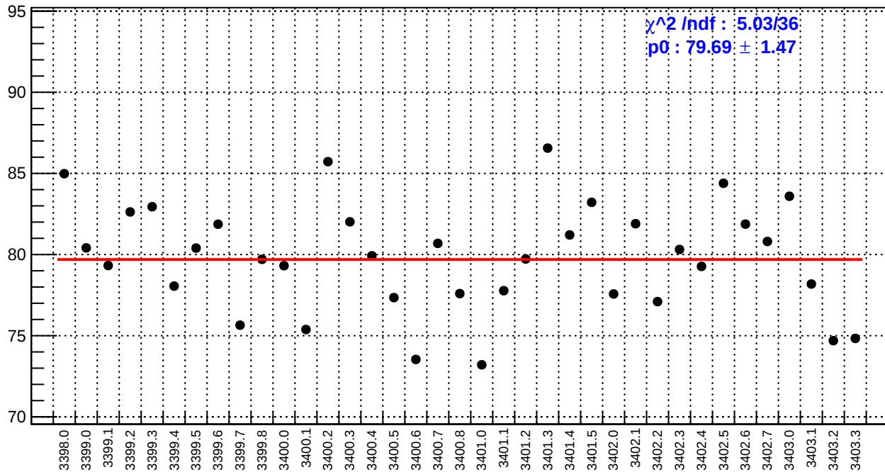
slug3: right_avg_bpm4aX/(ppb/nm)
