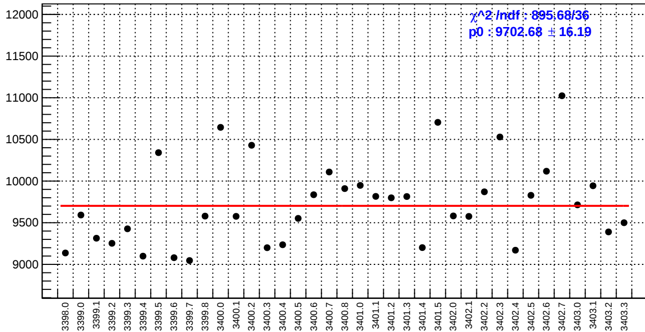
slug3: diff_bpm4eX.rms/nm
