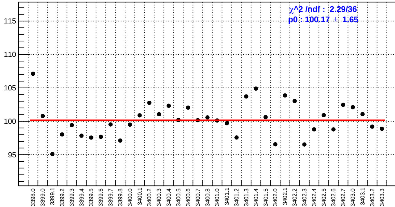
slug3: dsl_bpm4aX/(ppb/nm)
