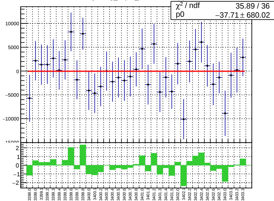
slug3: reg_asym_sam5.mean/ppb
