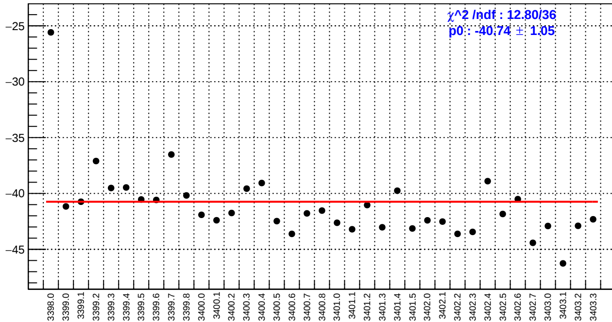
slug3: dsl_bpm4aY/(ppb/nm)
