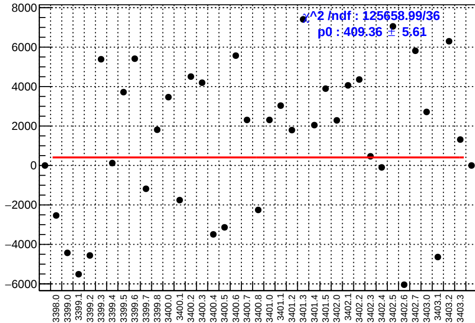
slug3: asym_us_dd.mean/ppb-reg_asym_us_dd.mean/ppb
