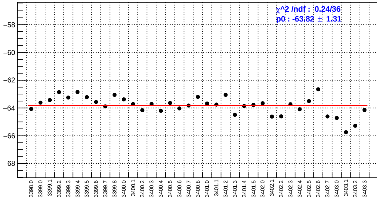
slug3: dsl_bpm4eX/(ppb/nm)
