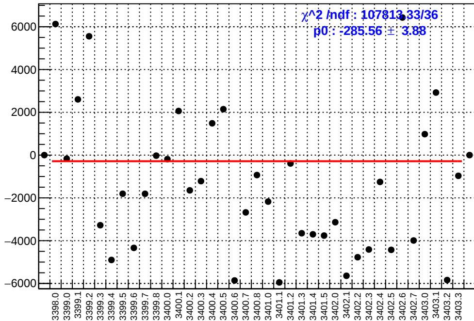
slug3: asym_right_avg.mean/ppb-reg_asym_right_avg.mean/ppb
