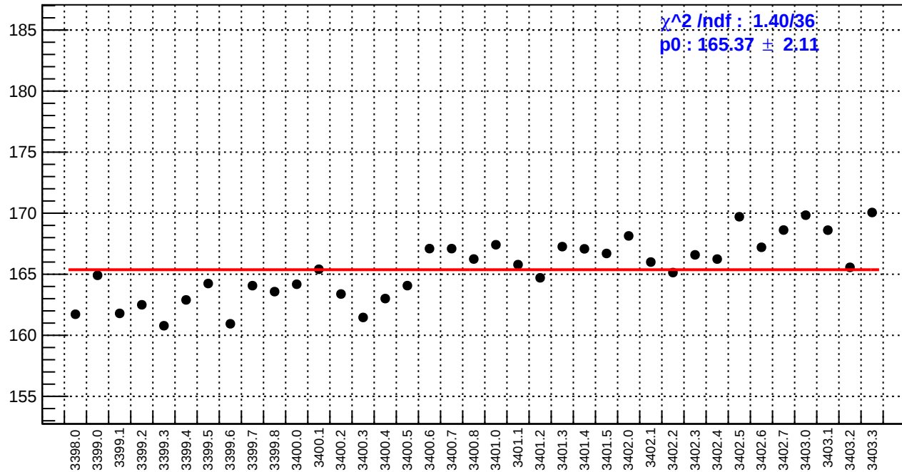
slug3: reg_asym_dsr.rms/ppm
