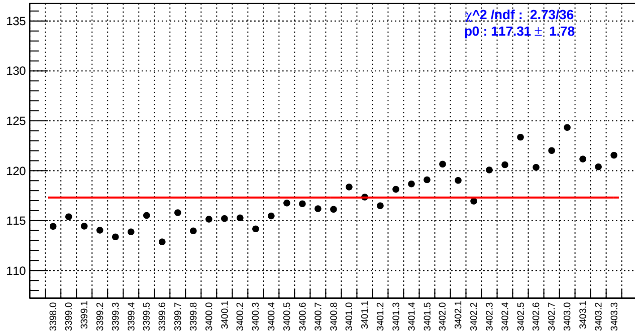
slug3: reg_asym_us_avg.rms/ppm
