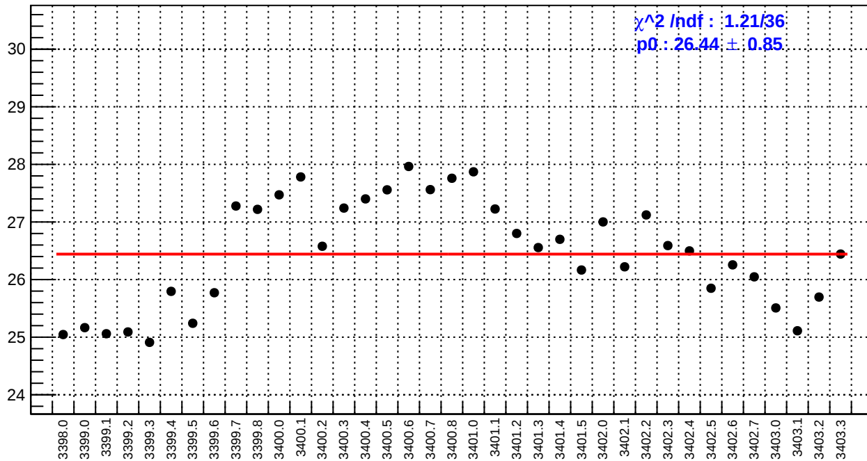
slug3: right_avg_bpm4eX/(ppb/nm)
