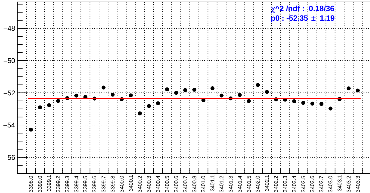
slug3: ds_avg_bpm12X/(ppb/nm)
