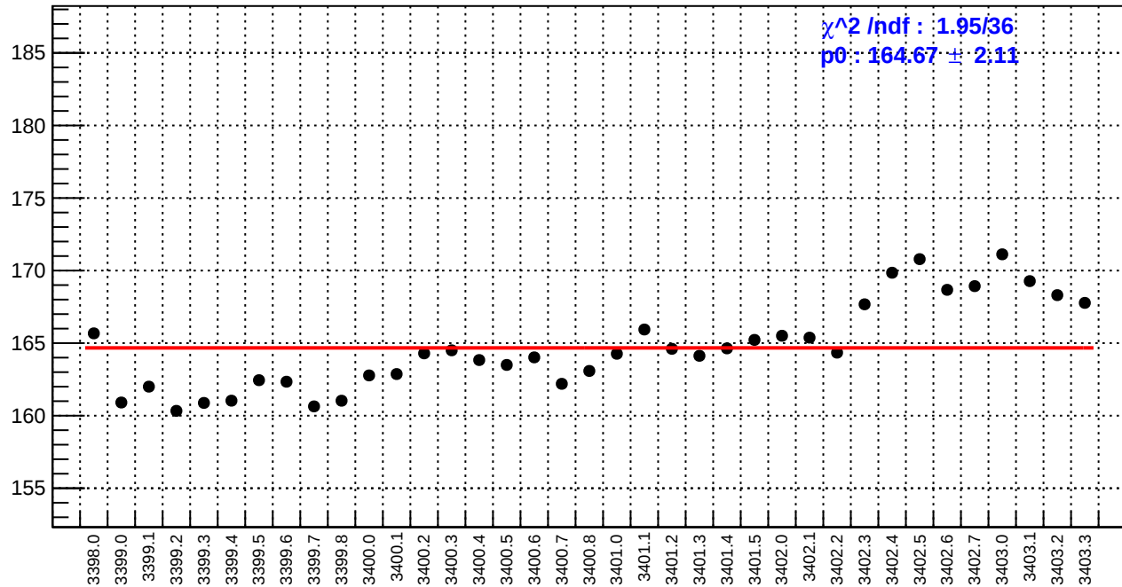
slug3: reg_asym_left_avg.rms/ppm
