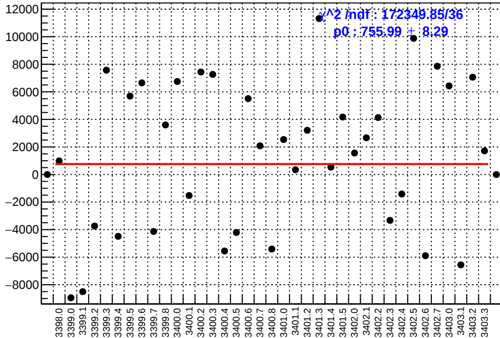
slug3: asym_dsl.mean/ppb-reg_asym_dsl.mean/ppb
