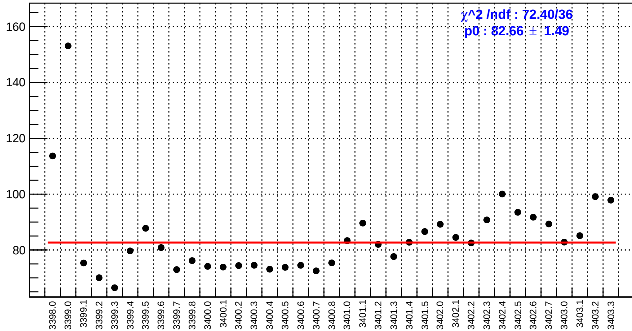
slug3: asym_bcm_an_us.rms/ppm
