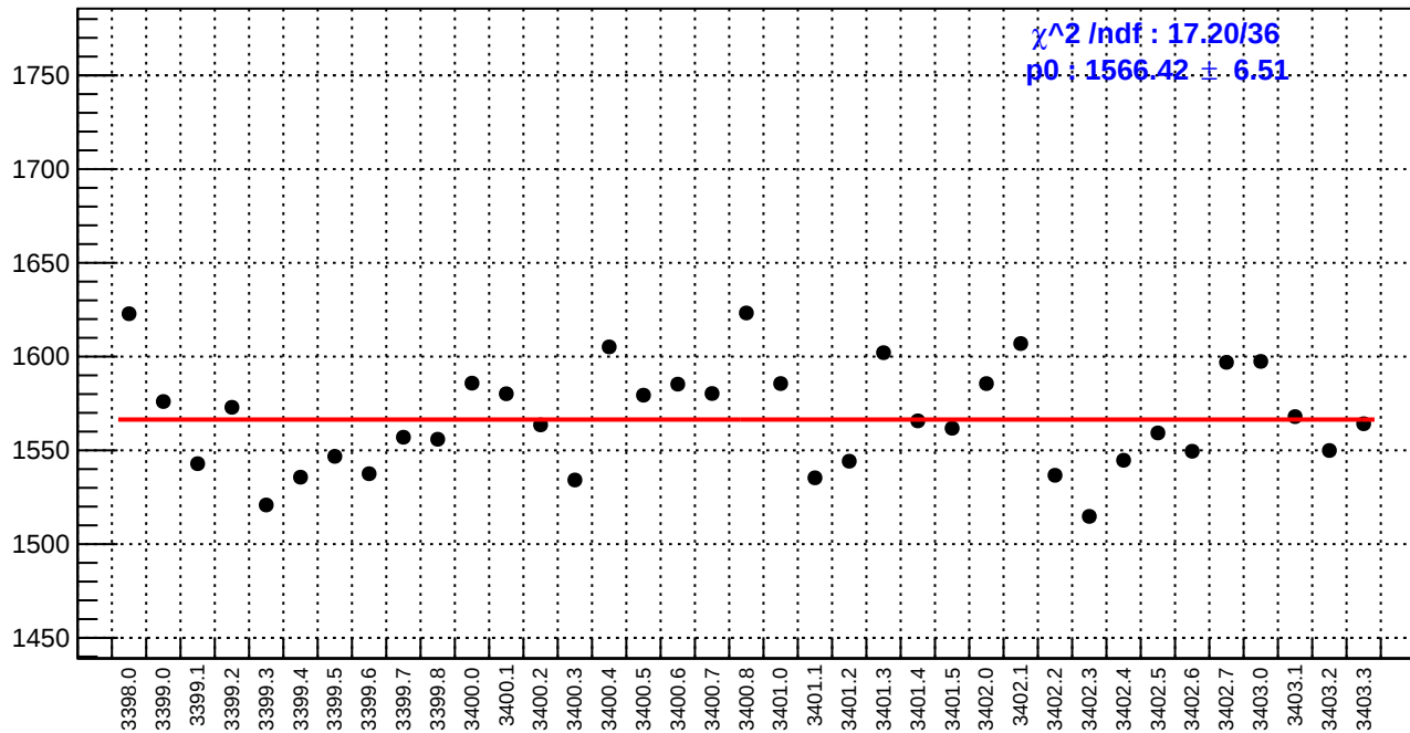
slug3: diff_bpm4aX.rms/nm
