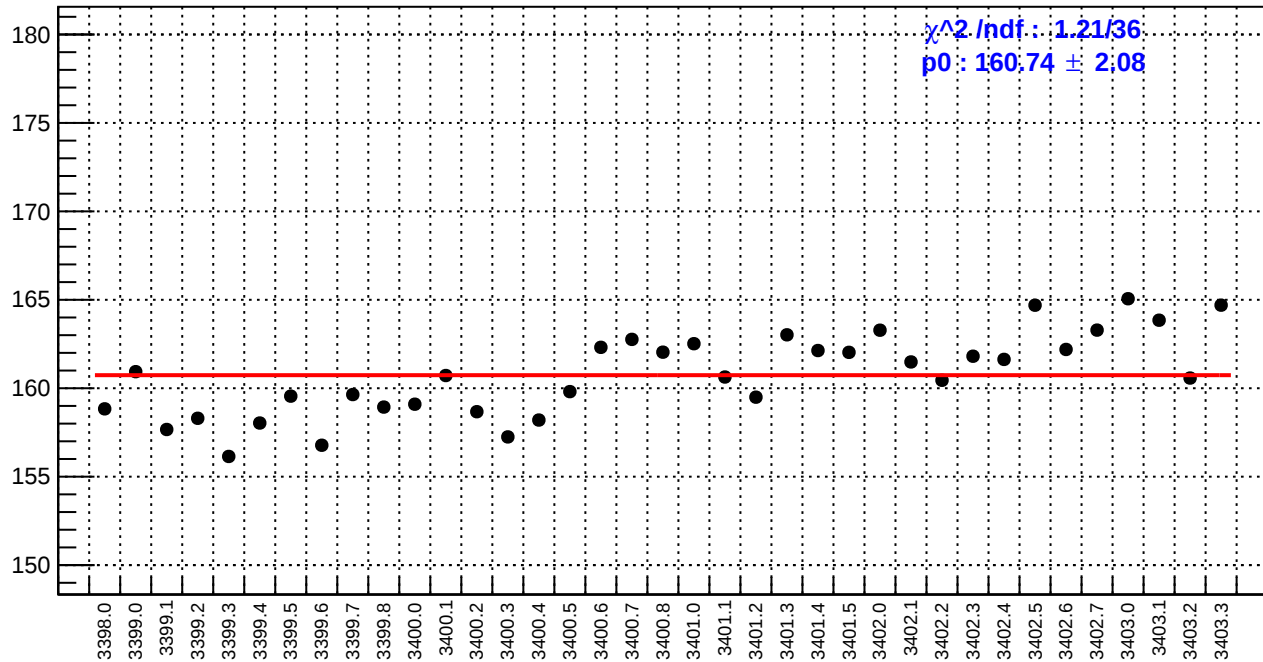
slug3: reg_asym_right_avg.rms/ppm
