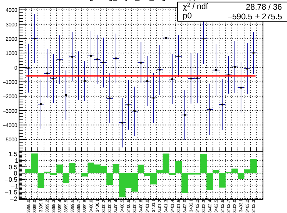
slug3: reg_asym_left_avg.mean/ppb
