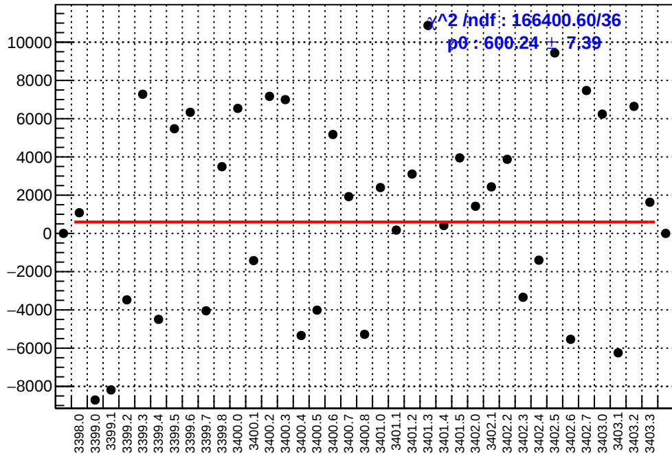
slug3: asym_left_avg.mean/ppb-reg_asym_left_avg.mean/ppb
