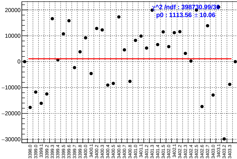
slug3: asym_sam8.mean/ppb-reg_asym_sam8.mean/ppb
