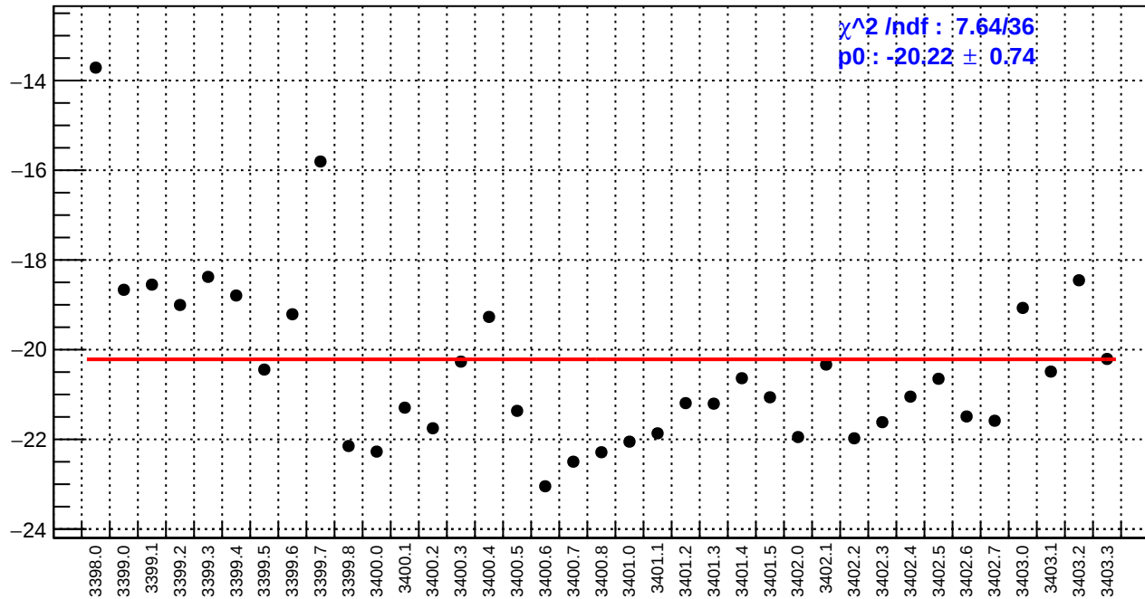
slug3: dsr_bpm4eY/(ppb/nm)
