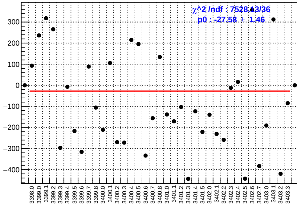
slug3: asym_left_dd.mean/ppb-reg_asym_left_dd.mean/ppb
