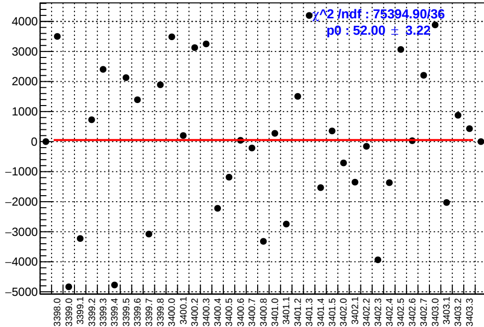
slug3: asym_ds_avg.mean/ppb-reg_asym_ds_avg.mean/ppb
