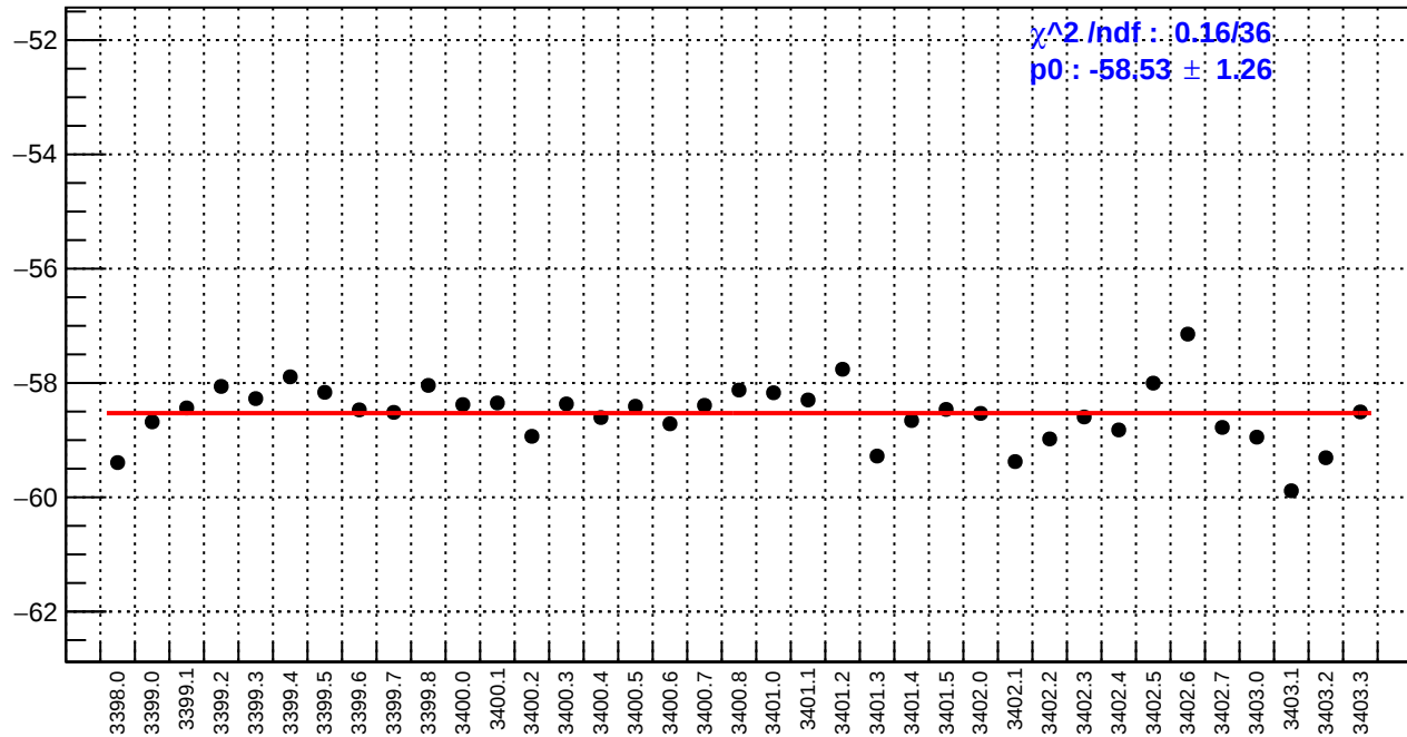
slug3: usl_bpm4eX/(ppb/nm)
