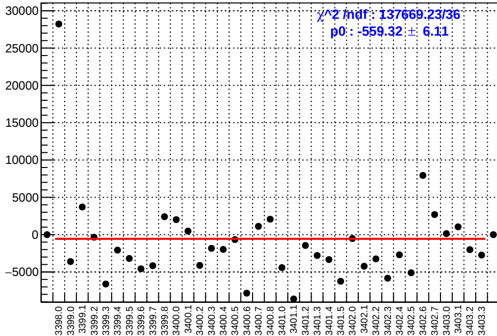
slug3: asym_sam1.mean/ppb-reg_asym_sam1.mean/ppb
