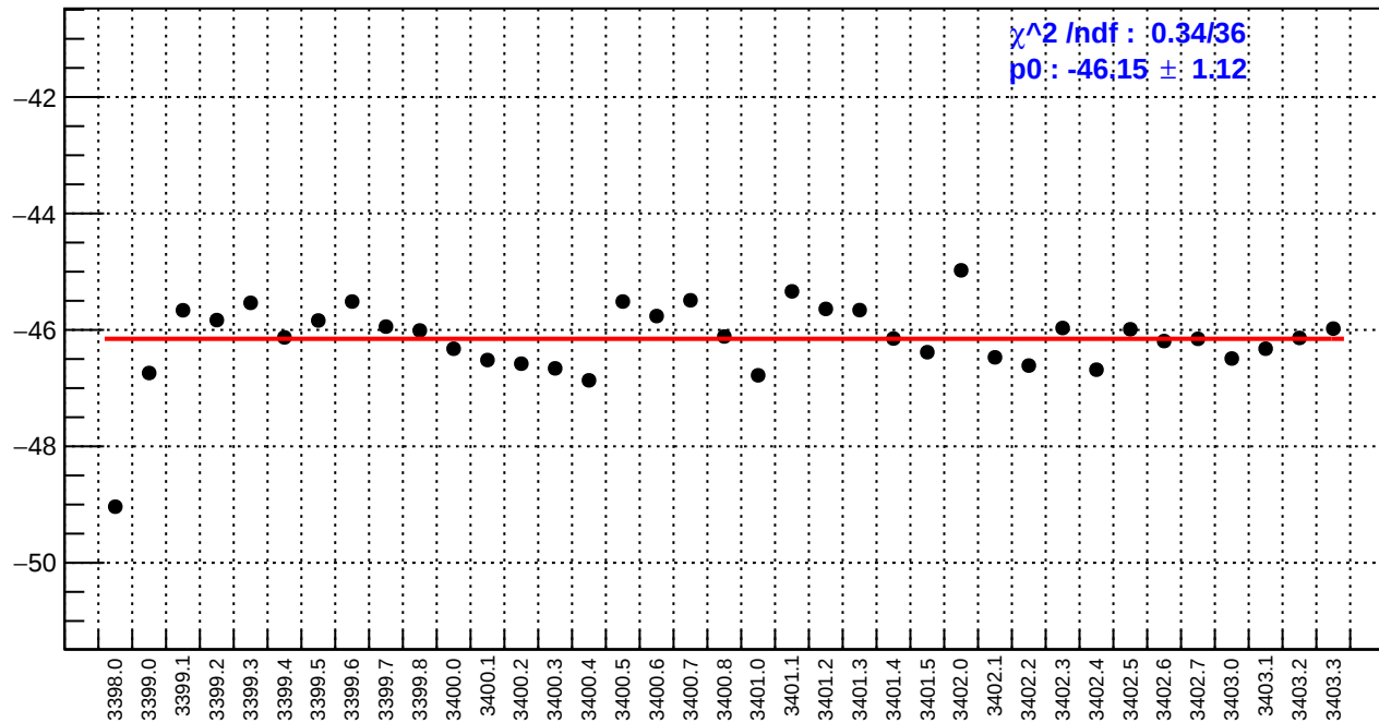
slug3: dsl_bpm12X/(ppb/nm)
