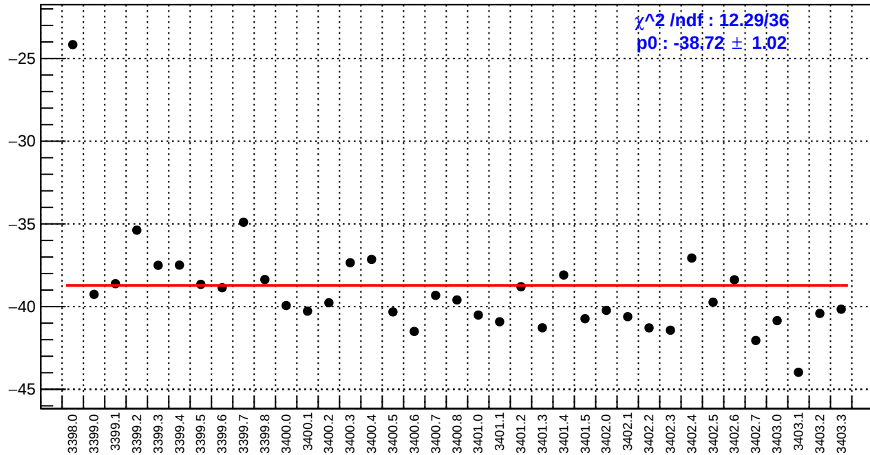
slug3: left_avg_bpm4aY/(ppb/nm)
