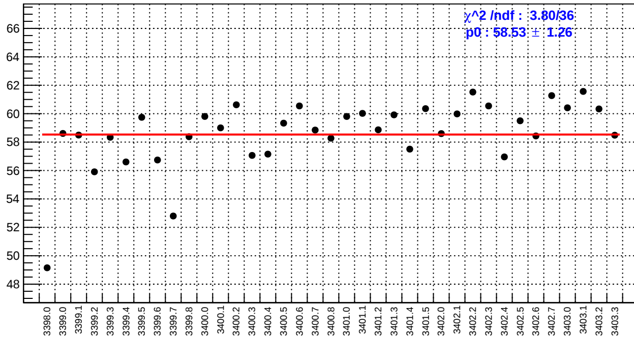
slug3: left_avg_bpm4eY/(ppb/nm)
