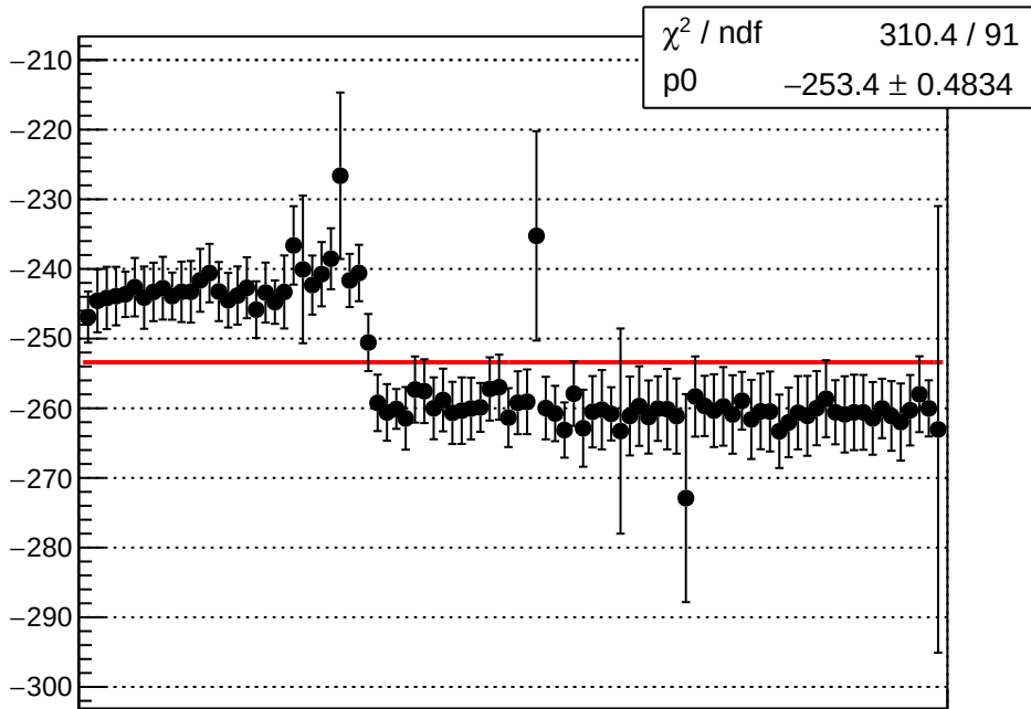
reg_asym_atr1l2_avg_diff_bpm11X_slope vs run
