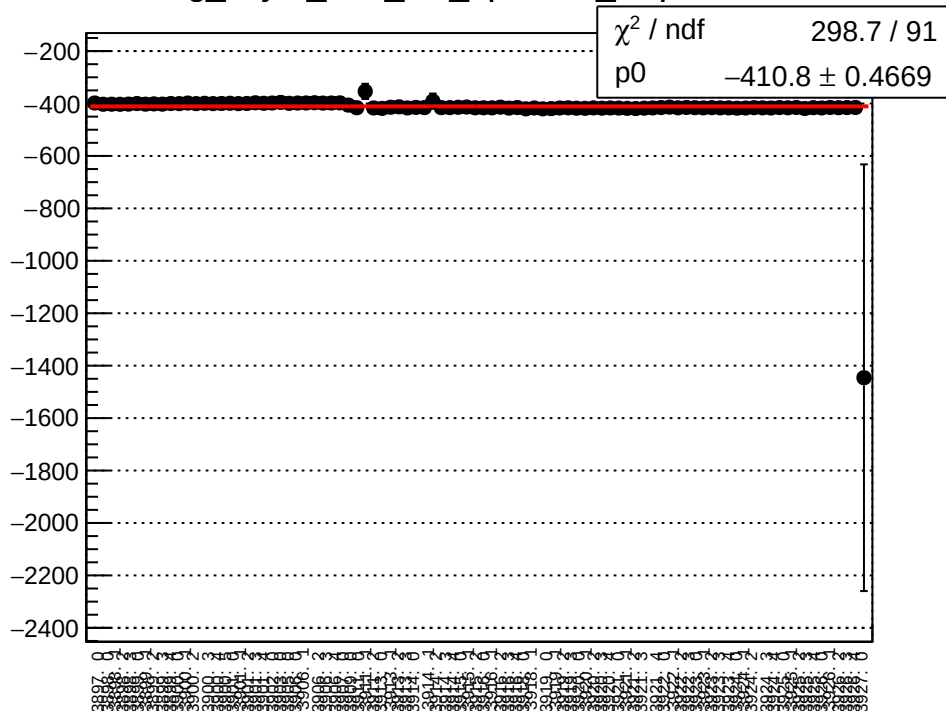
reg_asym_atr2_diff_bpm11X_slope vs run
