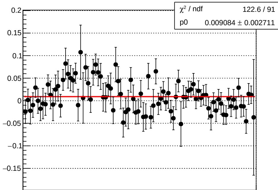
reg_bcm_dg_us_ds_dd_diff_bpm4eX_slope vs run
