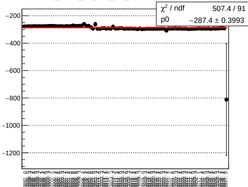
reg_asym_atr_avg_diff_bpm11X_slope vs run
