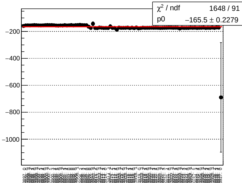
reg_asym_atl1r2_avg_diff_bpm11X_slope vs run
