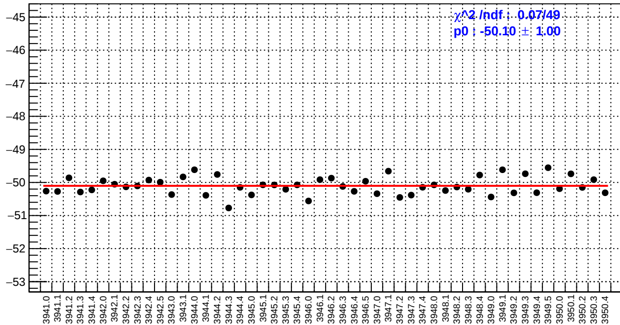
slug34: ds_avg_bpm12X/(ppb/nm)
