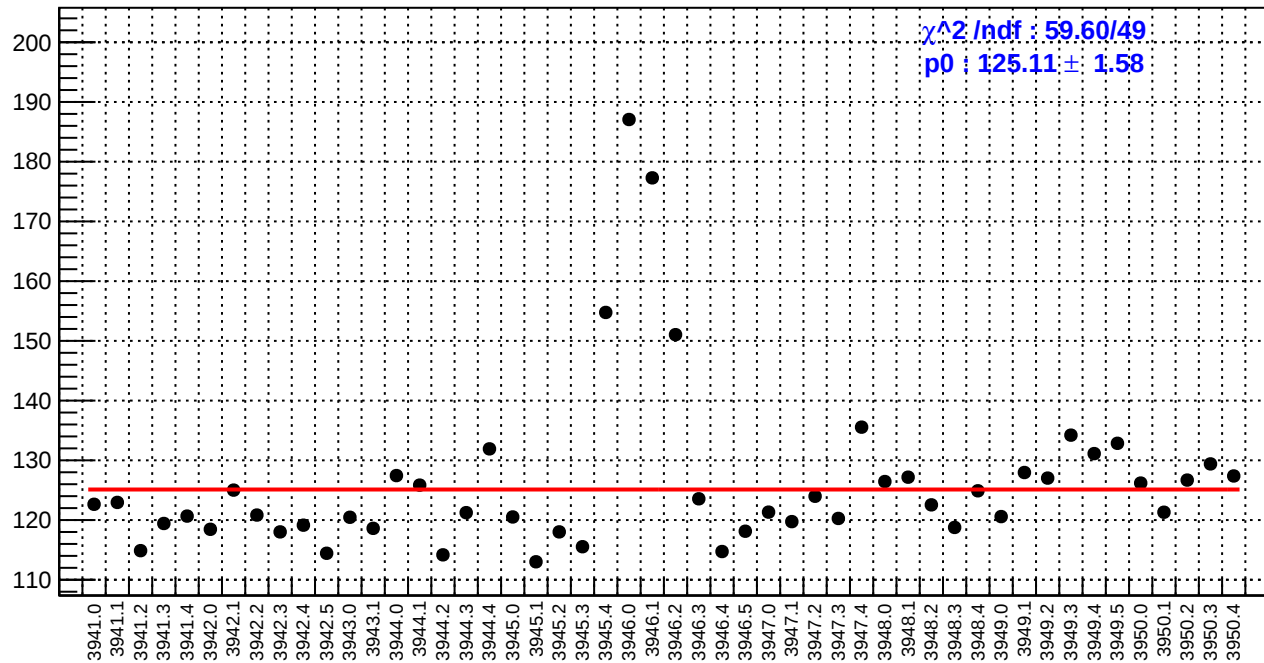
slug34: asym_bcm_an_ds3.rms/ppm
