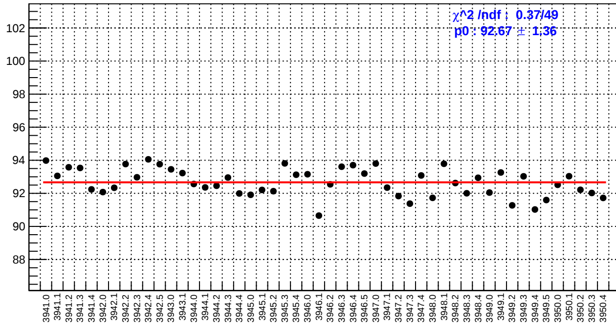
slug34: reg_asym_us_dd.rms/ppm
