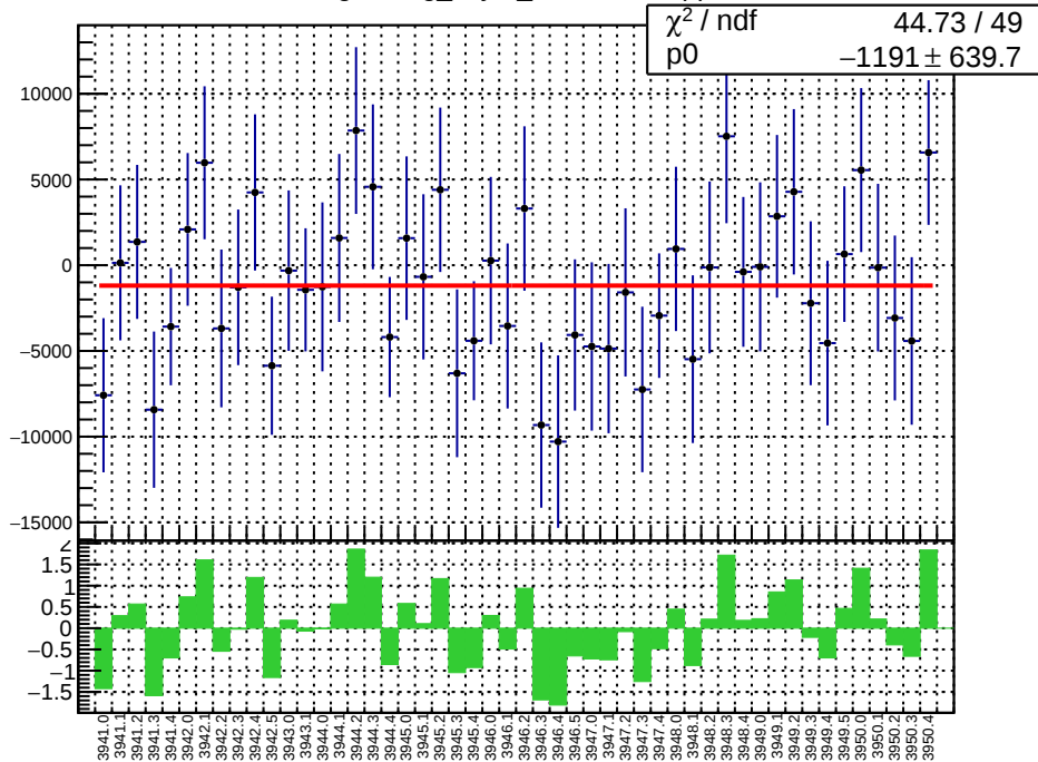
slug34: reg_asym_sam8.mean/ppb
