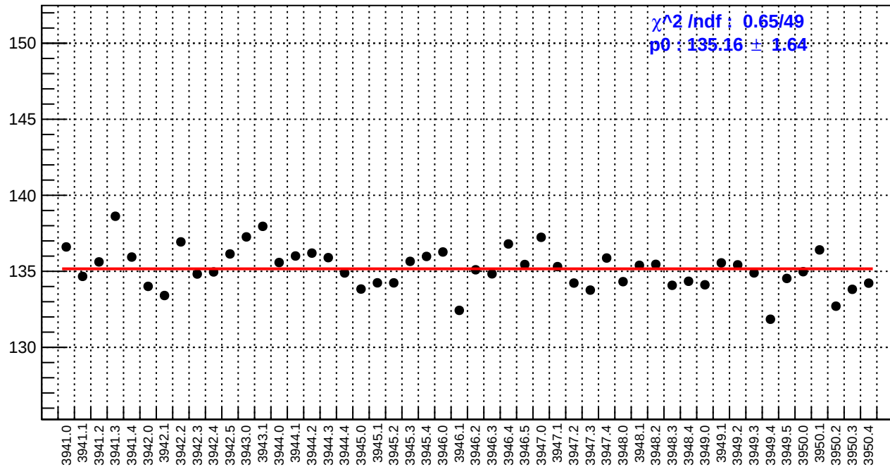
slug34: reg_asym_left_avg.rms/ppm
