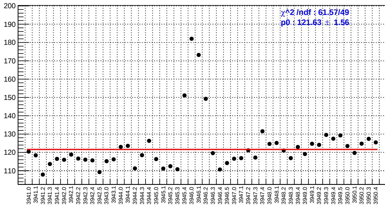
slug34: asym_bcm_an_us.rms/ppm
