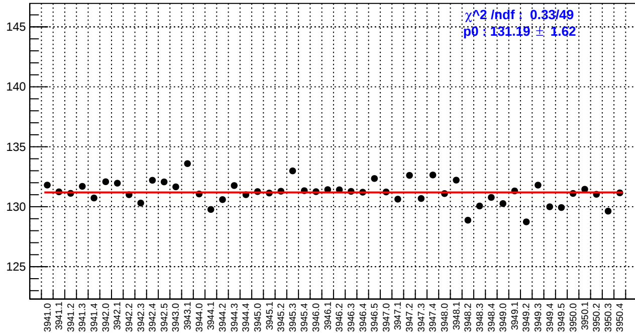
slug34: reg_asym_usr.rms/ppm
