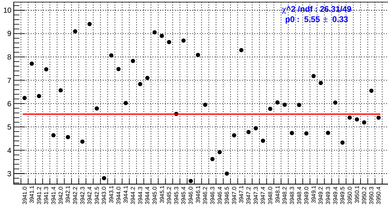
slug34: left_avg_bpm4eY/(ppb/nm)
