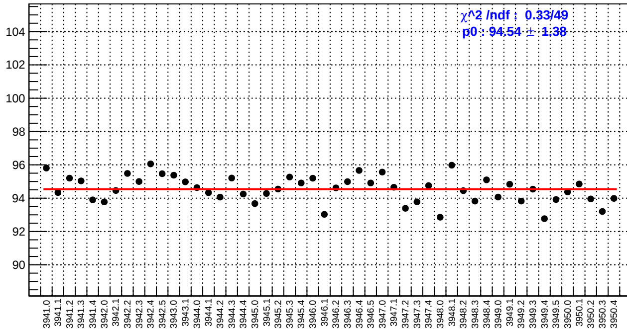
slug34: reg_asym_ds_dd.rms/ppm
