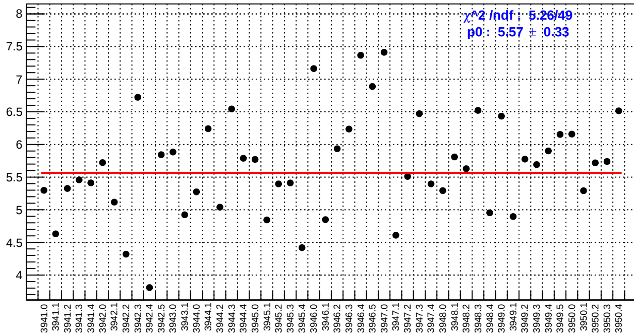
slug34: ds_avg_bpm4aY/(ppb/nm)
