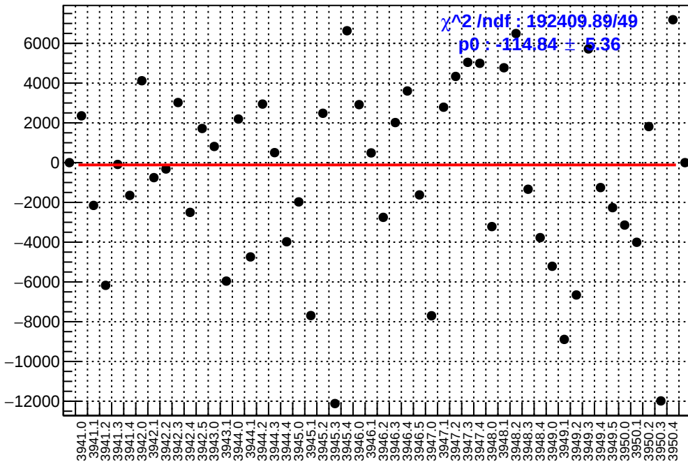
slug34: asym_usr.mean/ppb-reg_asym_usr.mean/ppb
