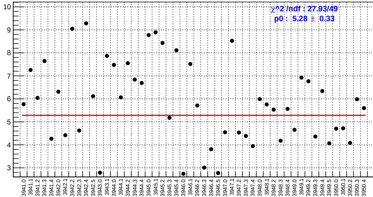
slug34: usl_bpm4eY/(ppb/nm)
