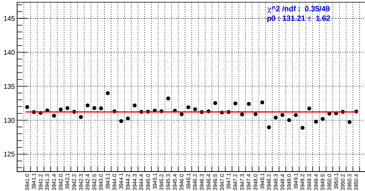
slug34: reg_asym_right_avg.rms/ppm
