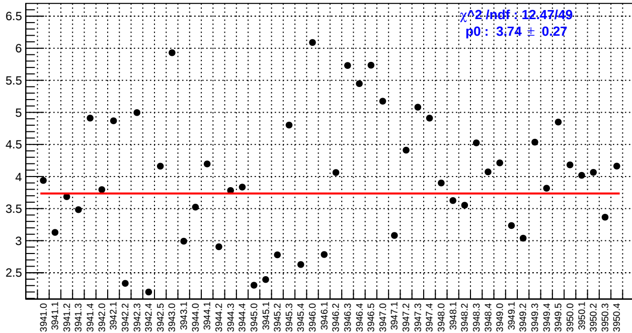
slug34: left_avg_bpm4aY/(ppb/nm)
