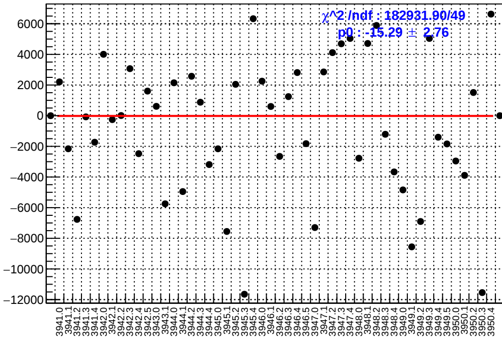
slug34: asym_right_avg.mean/ppb-reg_asym_right_avg.mean/ppb
