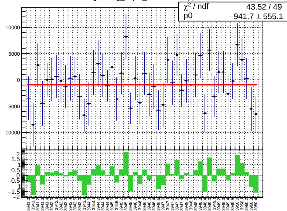
slug34: reg_asym_sam1.mean/ppb
