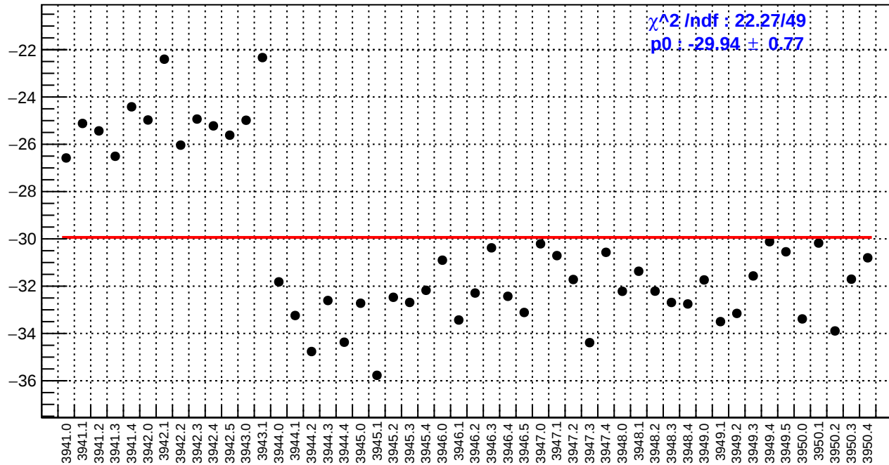
slug34: dsr_bpm4aX/(ppb/nm)
