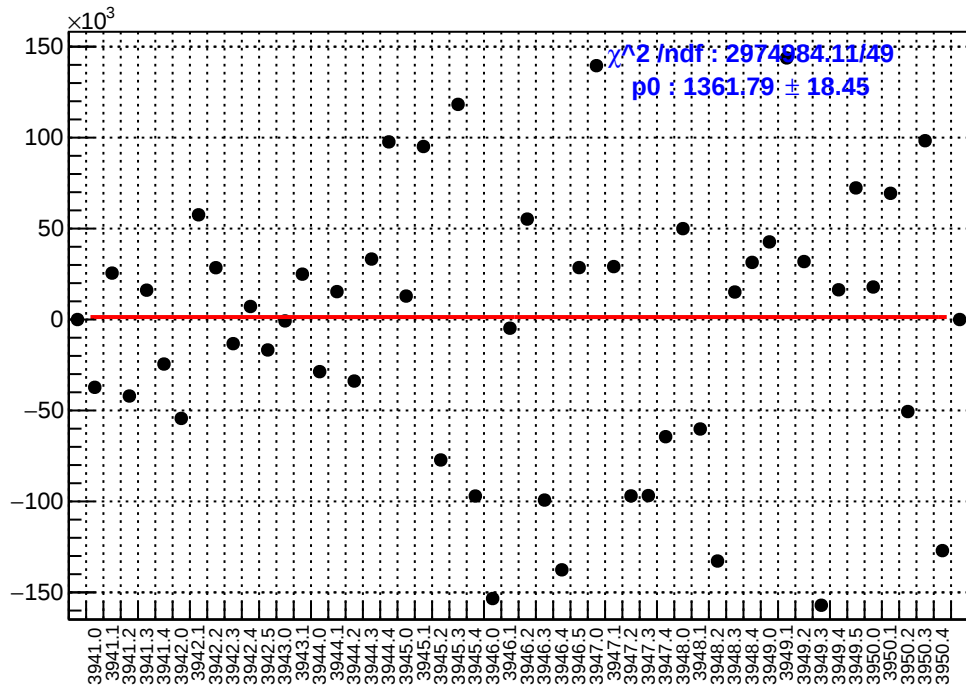
slug34: asym_sam2.mean/ppb-reg_asym_sam2.mean/ppb
