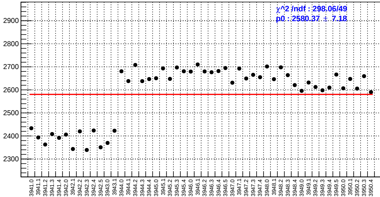
slug34: reg_asym_sam2.rms/ppm
