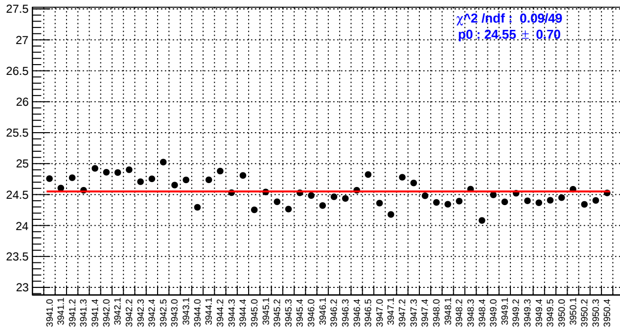
slug34: reg_asym_left_dd.rms/ppm
