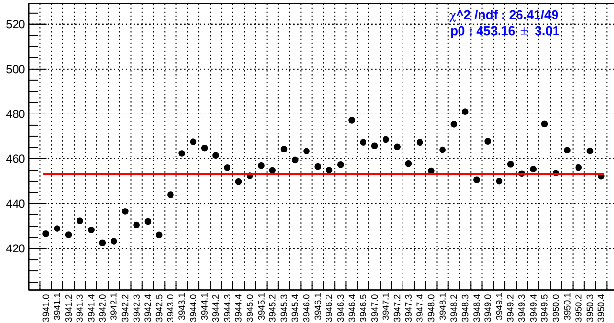
slug34: reg_asym_sam8.rms/ppm
