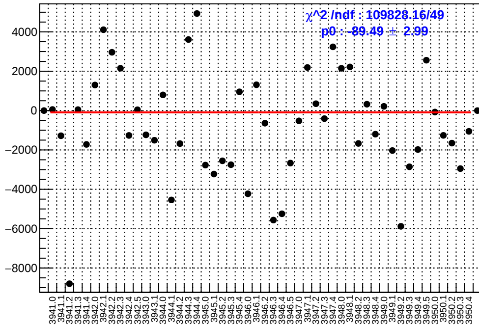
slug34: asym_us_avg.mean/ppb-reg_asym_us_avg.mean/ppb
