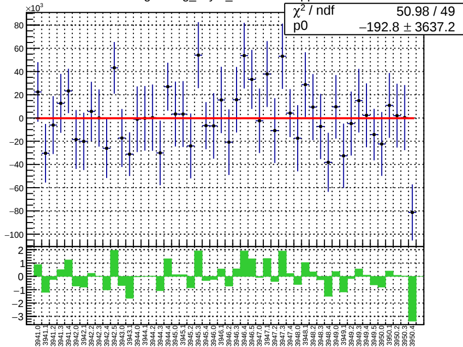
slug34: reg_asym_sam2.mean/ppb
