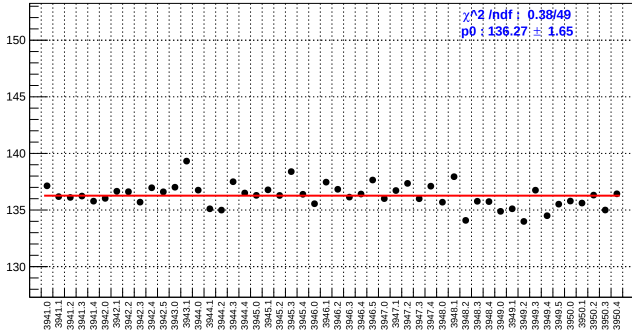
slug34: reg_asym_dsr.rms/ppm
