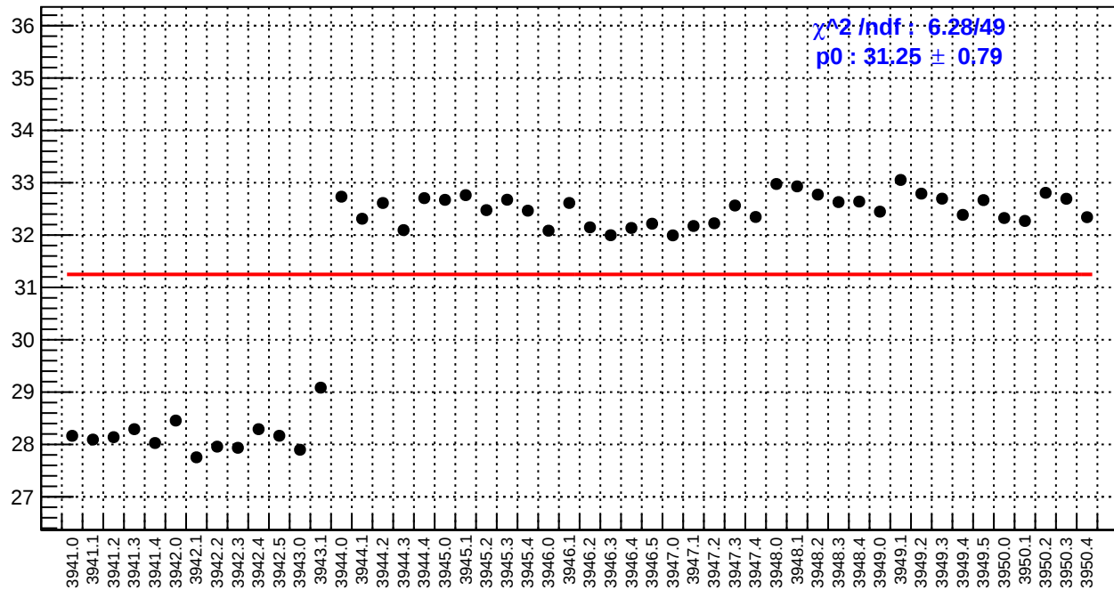
slug34: right_avg_bpm4eX/(ppb/nm)
