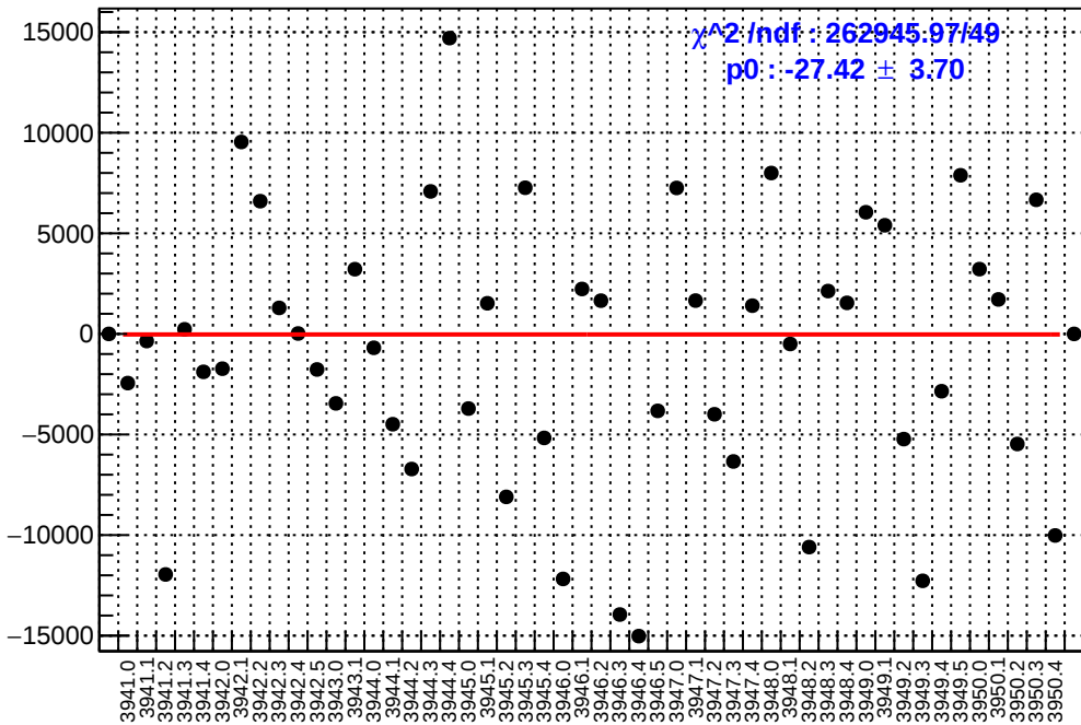
slug34: asym_dsl.mean/ppb-reg_asym_dsl.mean/ppb
