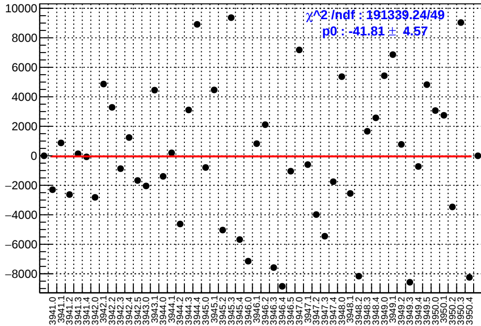
slug34: asym_us_dd.mean/ppb-reg_asym_us_dd.mean/ppb
