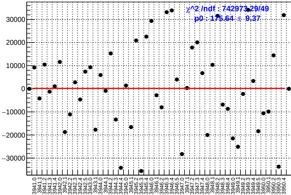
slug34: asym_sam7.mean/ppb-reg_asym_sam7.mean/ppb
