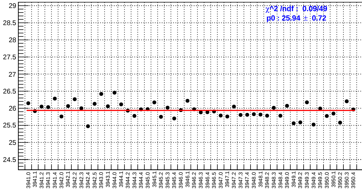
slug34: reg_asym_right_dd.rms/ppm
