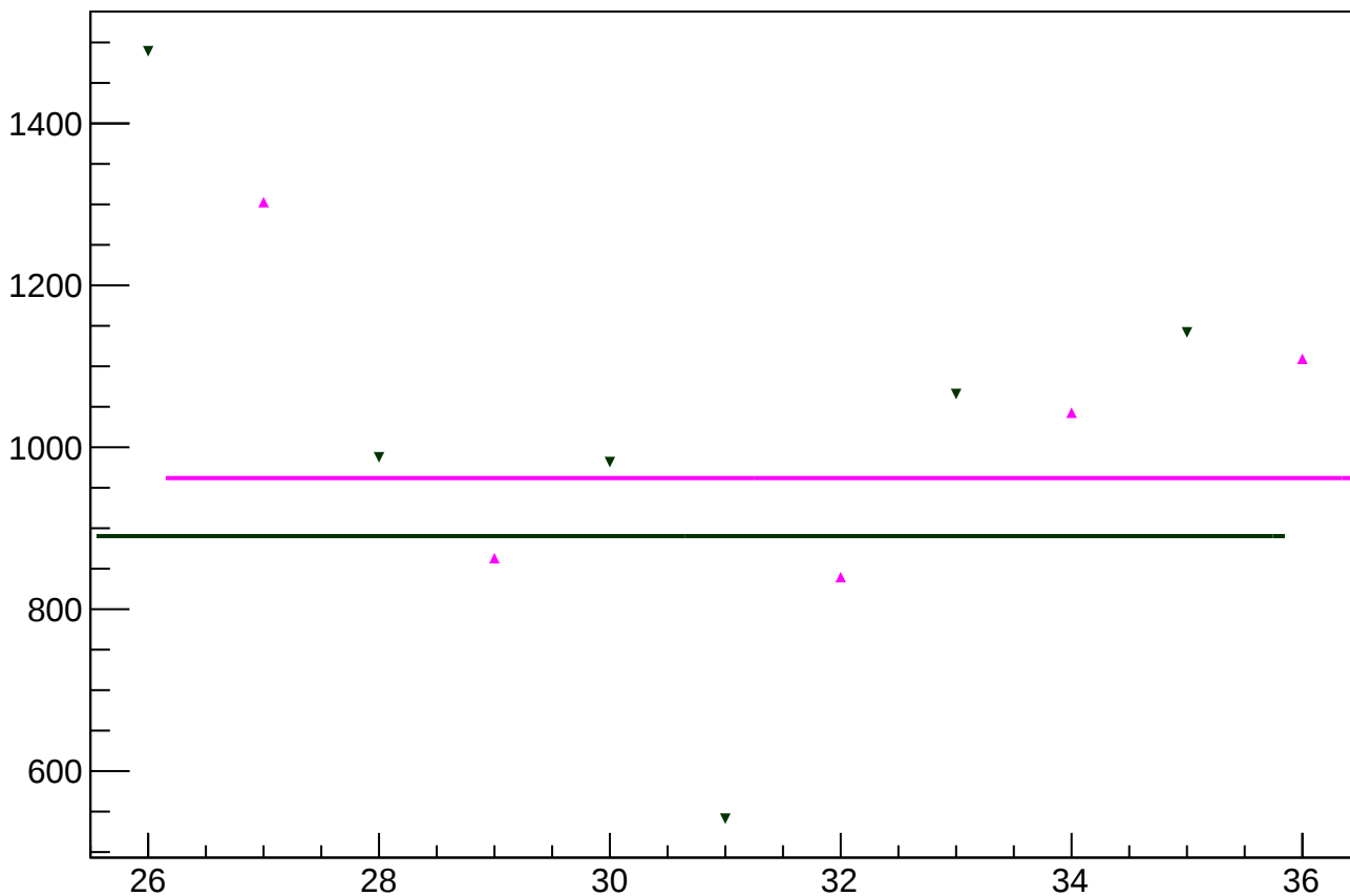
asym_atl1r2_avg_correction_rms vs slug
