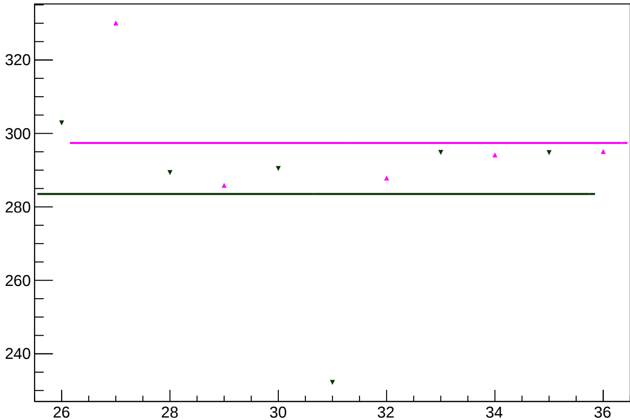
reg_asym_atl1r2_avg_rms vs slug
