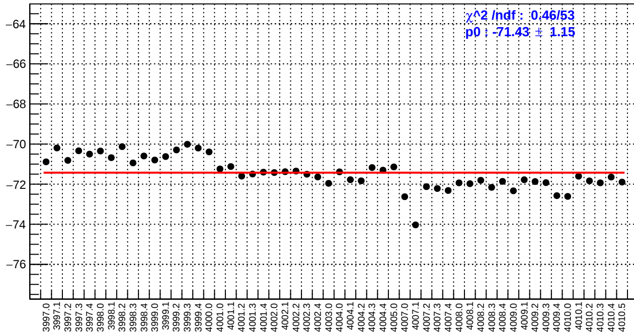
slug38: dsl_bpm4eX/(ppb/nm)
