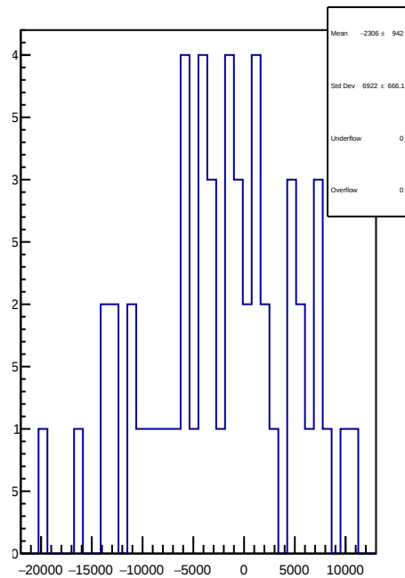
slug38: 1D Corr asym_usl.mean/ppb-reg_asym_usl.mean/ppb
