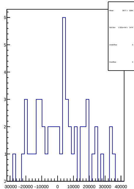
slug38: 1D Corr asym_sam1.mean/ppb-reg_asym_sam1.mean/ppb
