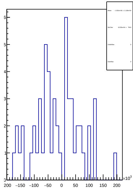
slug38: 1D Corr asym_sam2.mean/ppb-reg_asym_sam2.mean/ppb
