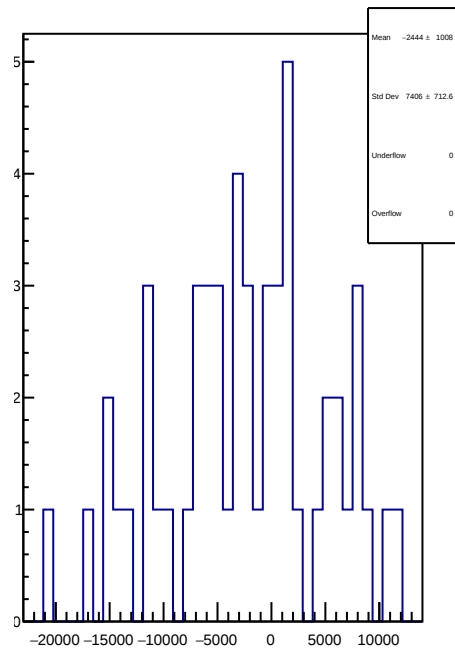
slug38: 1D Corr asym_dsl.mean/ppb-reg_asym_dsl.mean/ppb
