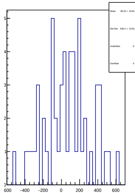
slug38: 1D Corr asym_left_dd.mean/ppb-reg_asym_left_dd.mean/ppb
