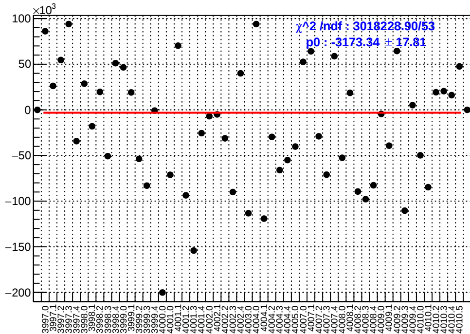
slug38: asym_sam4.mean/ppb-reg_asym_sam4.mean/ppb
