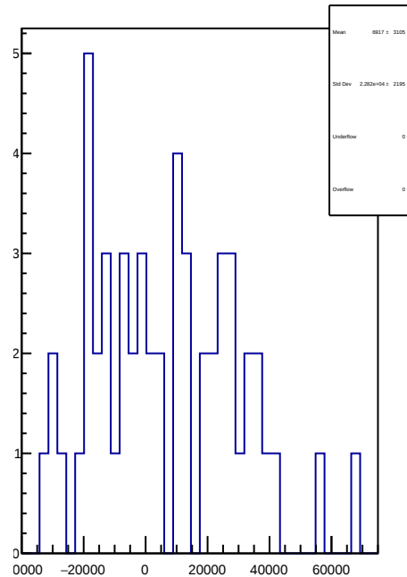
slug38: 1D Corr asym_sam8.mean/ppb-reg_asym_sam8.mean/ppb
