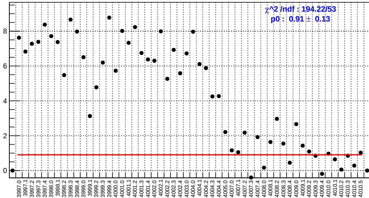
slug38: right_avg_bpm4aY/(ppb/nm)
