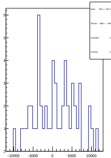
slug38: 1D Corr asym_usr.mean/ppb-reg_asym_usr.mean/ppb
