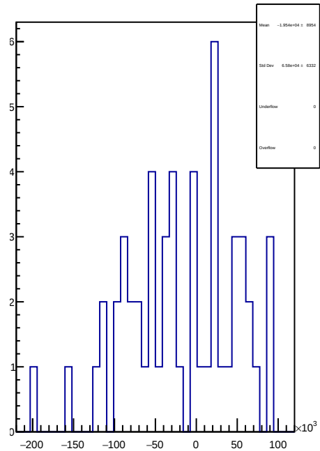
slug38: 1D Corr asym_sam4.mean/ppb-reg_asym_sam4.mean/ppb
