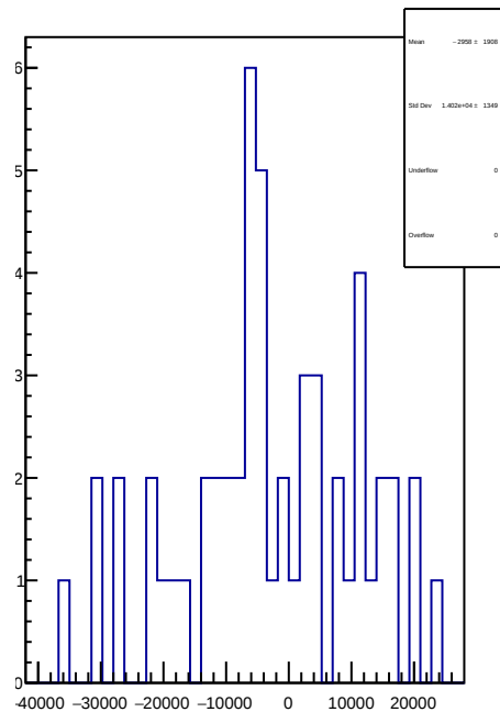
slug38: 1D Corr asym_sam5.mean/ppb-reg_asym_sam5.mean/ppb
