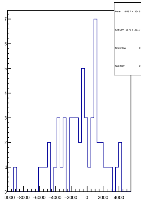
slug38: 1D Corr asym_us_avg.mean/ppb-reg_asym_us_avg.mean/ppb
