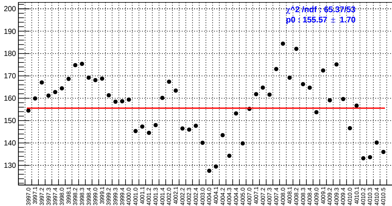
slug38: asym_bcm_an_ds.rms/ppm
