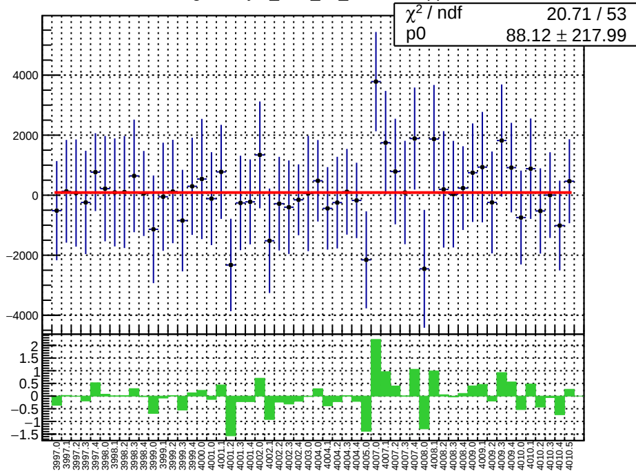
slug38: asym_bcm_an_ds3.mean/ppb
