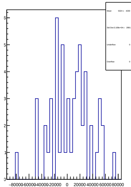
slug38: 1D Corr asym_sam6.mean/ppb-reg_asym_sam6.mean/ppb
