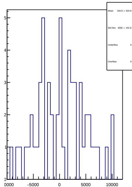
slug38: 1D Corr asym_dsr.mean/ppb-reg_asym_dsr.mean/ppb
