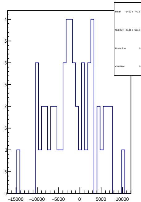
slug38: 1D Corr asym_us_dd.mean/ppb-reg_asym_us_dd.mean/ppb
