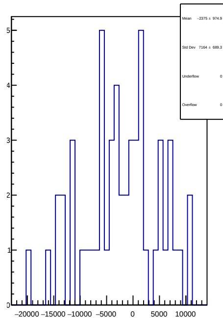
slug38: 1D Corr asym_left_avg.mean/ppb-reg_asym_left_avg.mean/ppb
