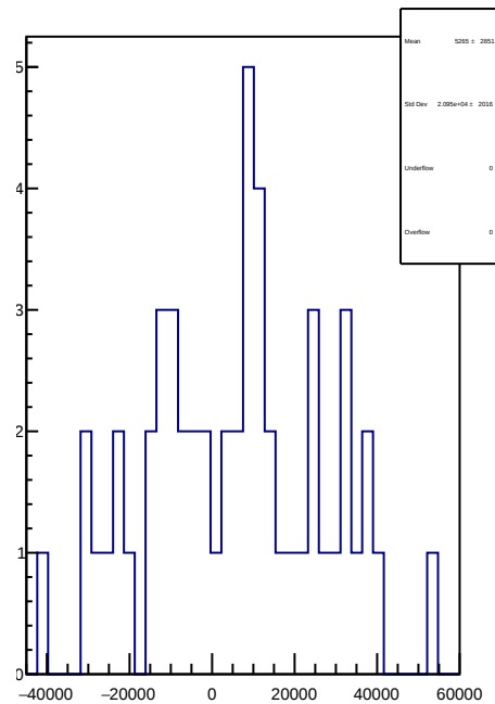
slug38: 1D Corr asym_sam7.mean/ppb-reg_asym_sam7.mean/ppb
