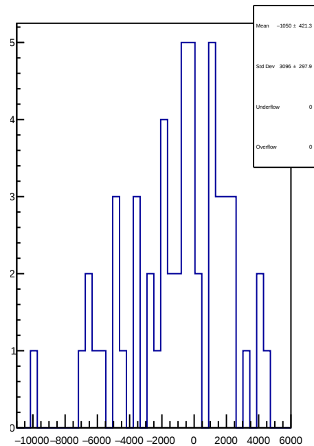
slug38: 1D Corr asym_ds_avg.mean/ppb-reg_asym_ds_avg.mean/ppb
