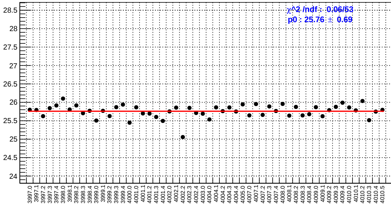
slug38: reg_asym_right_dd.rms/ppm
