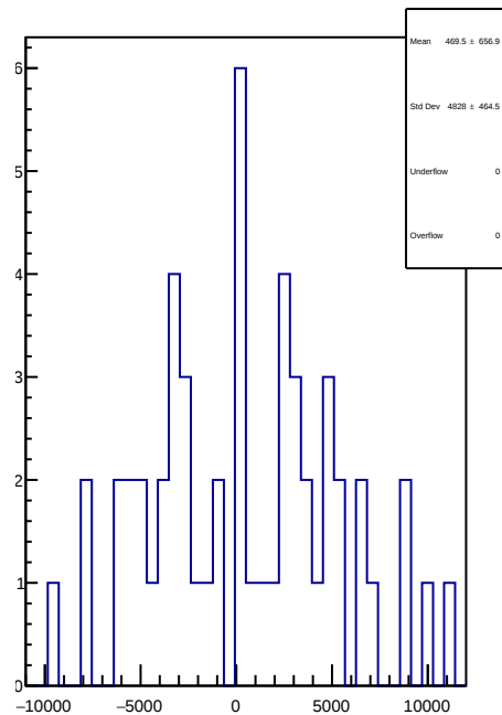
slug38: 1D Corr asym_right_avg.mean/ppb-reg_asym_right_avg.mean/ppb
