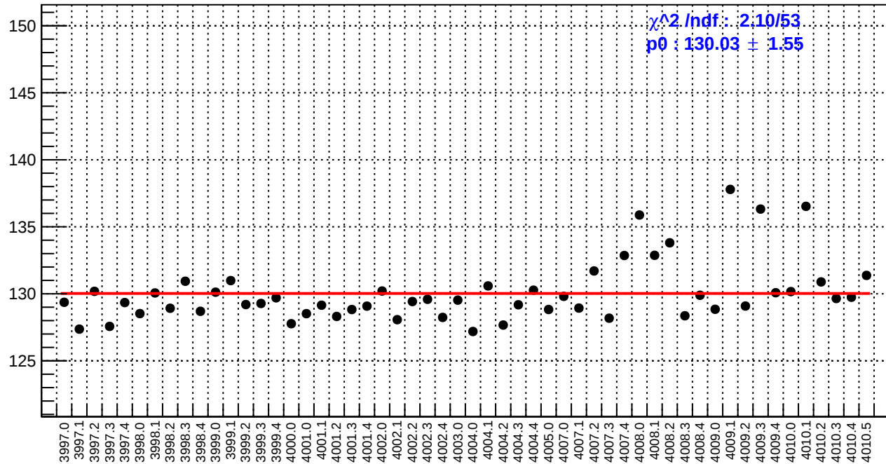
slug38: reg_asym_usr.rms/ppm
