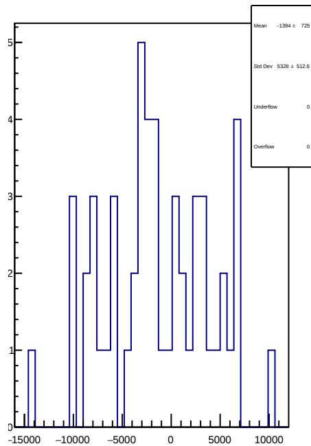
slug38: 1D Corr asym_ds_dd.mean/ppb-reg_asym_ds_dd.mean/ppb
