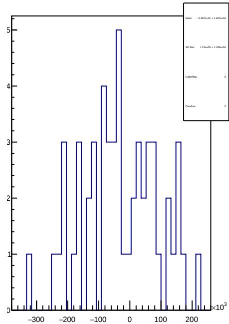
slug38: 1D Corr asym_sam3.mean/ppb-reg_asym_sam3.mean/ppb
