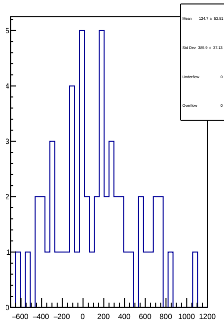
slug38: 1D Corr asym_right_dd.mean/ppb-reg_asym_right_dd.mean/ppb
