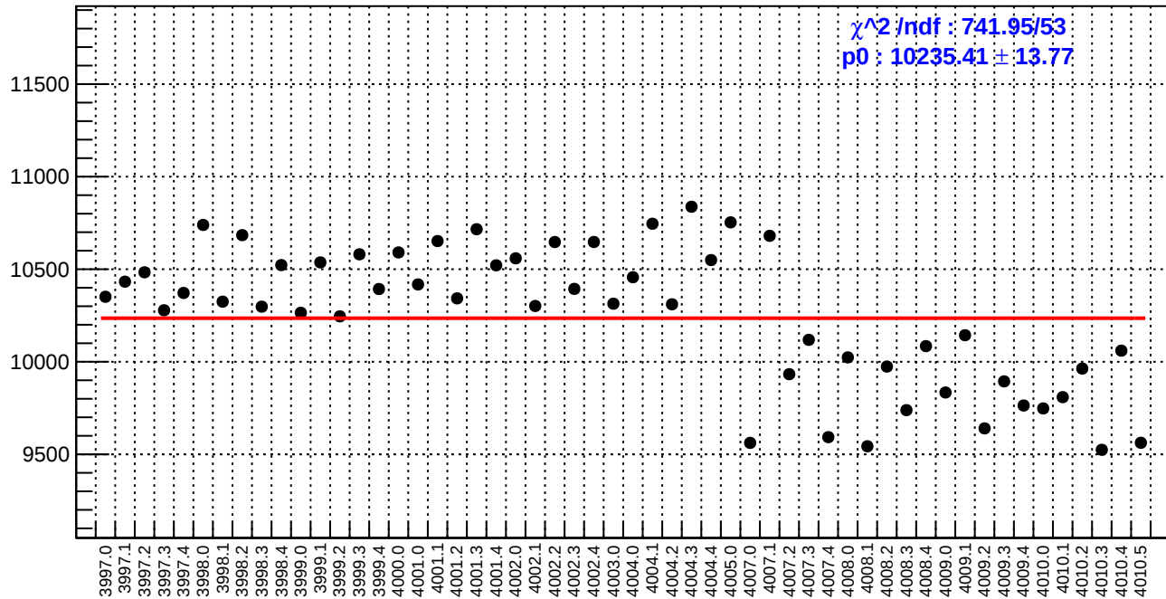
slug38: diff_bpm4eX.rms/nm
