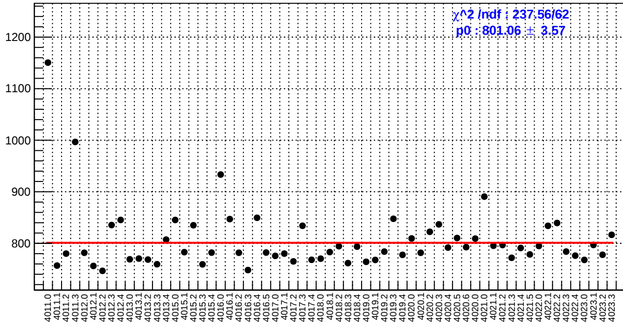
slug39: reg_asym_sam3.rms/ppm
