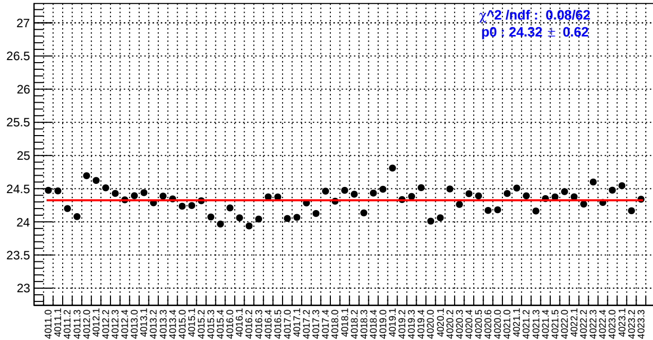
slug39: reg_asym_left_dd.rms/ppm
