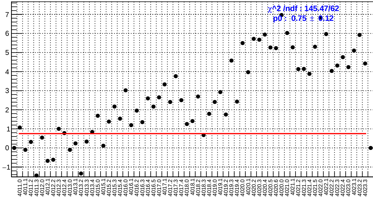
slug39: ds_avg_bpm4aY/(ppb/nm)
