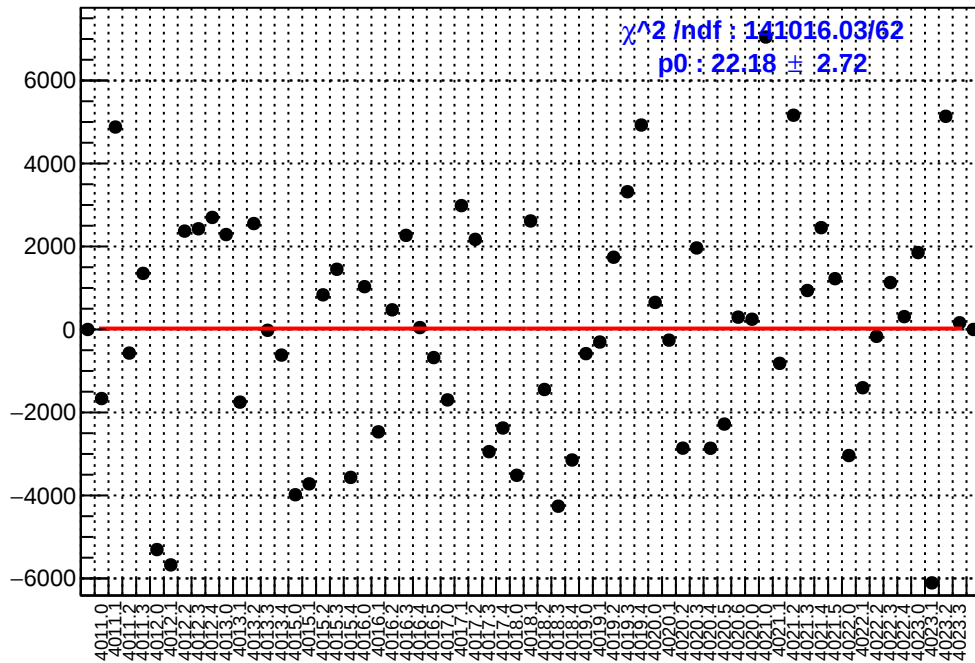
slug39: asym_us_avg.mean/ppb-reg_asym_us_avg.mean/ppb
