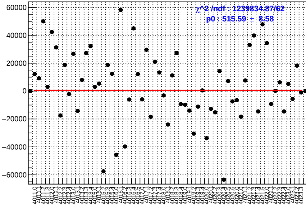
slug39: asym_sam6.mean/ppb-reg_asym_sam6.mean/ppb
