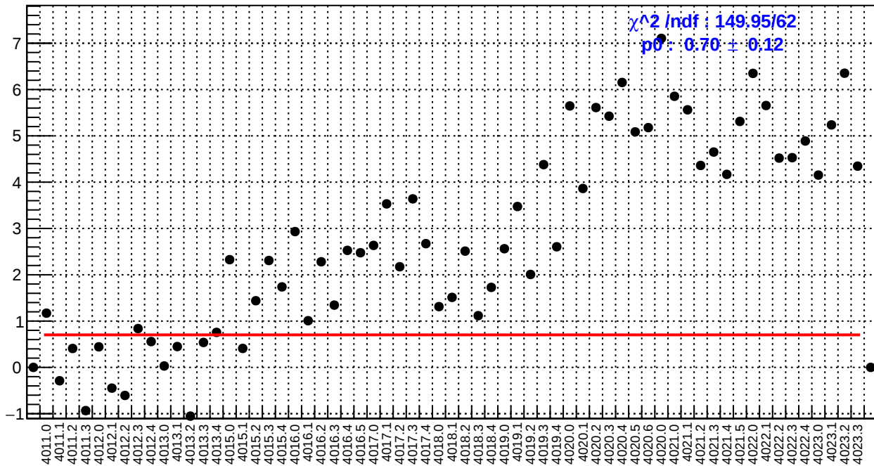
slug39: us_avg_bpm4aY/(ppb/nm)
