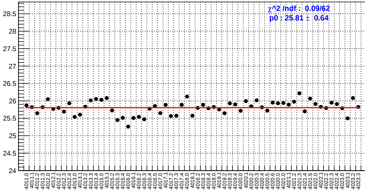
slug39: reg_asym_right_dd.rms/ppm
