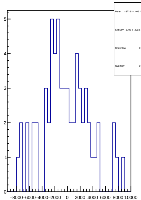
slug39: 1D Corr asym_ds_dd.mean/ppb-reg_asym_ds_dd.mean/ppb
