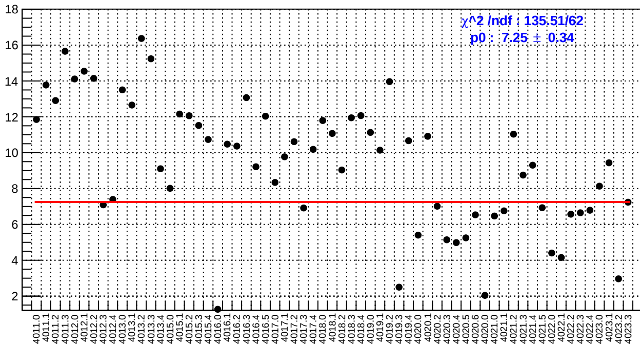
slug39: left_avg_bpm4eY/(ppb/nm)
