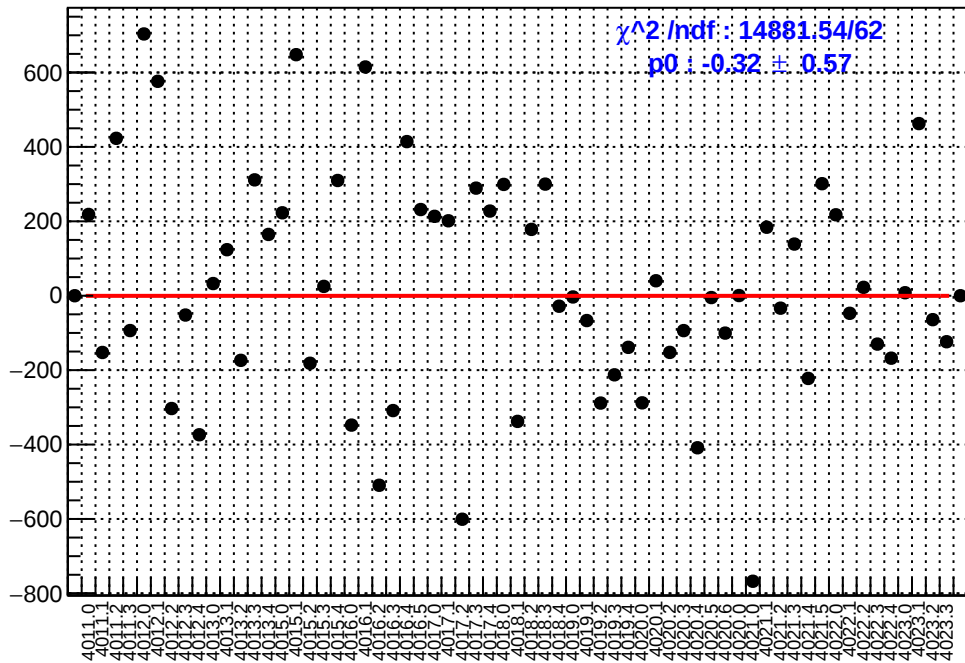
slug39: asym_right_dd.mean/ppb-reg_asym_right_dd.mean/ppb
