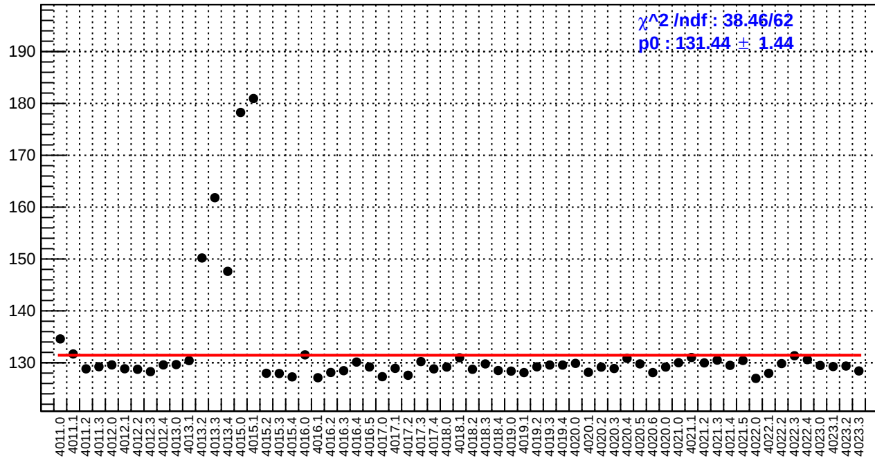
slug39: reg_asym_usr.rms/ppm
