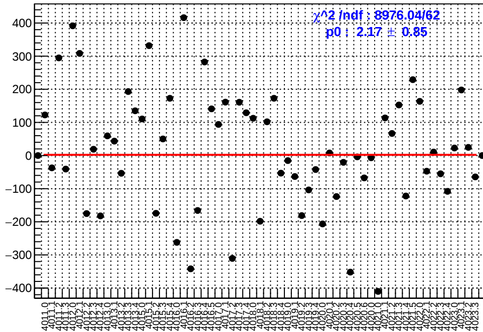
slug39: asym_left_dd.mean/ppb-reg_asym_left_dd.mean/ppb
