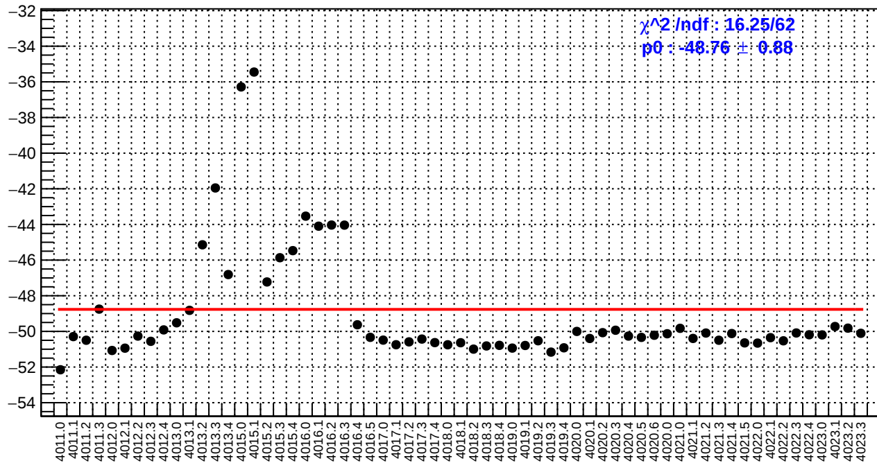
slug39: ds_avg_bpm12X/(ppb/nm)
