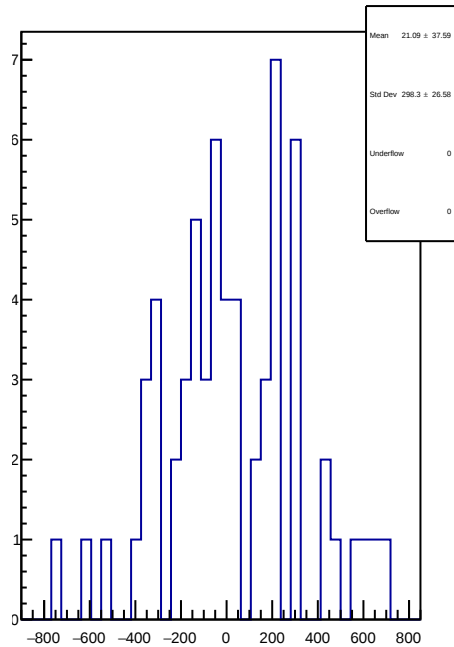
slug39: 1D Corr asym_right_dd.mean/ppb-reg_asym_right_dd.mean/ppb
