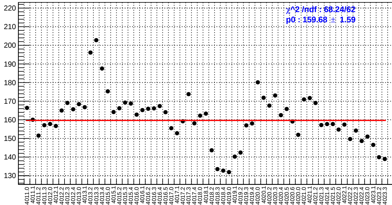
slug39: asym_bcm_an_ds3.rms/ppm
