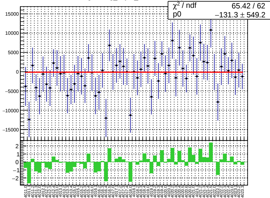
slug39: reg_asym_sam8.mean/ppb
