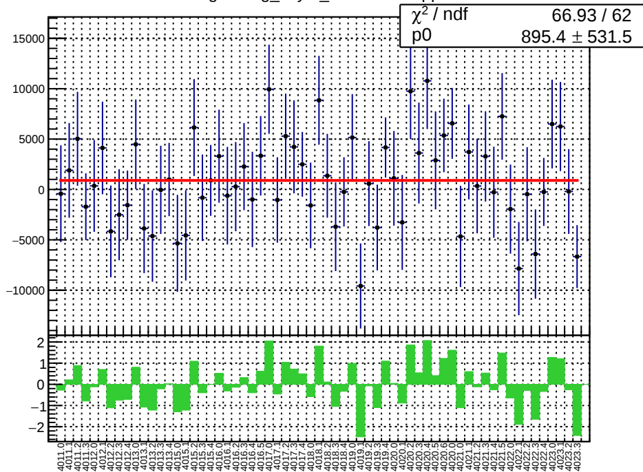
slug39: reg_asym_sam1.mean/ppb
