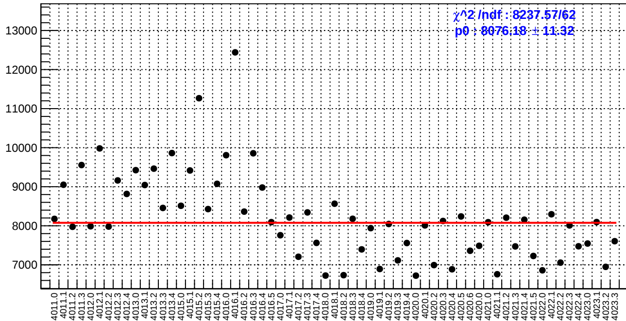
slug39: diff_bpm4aY.rms/nm
