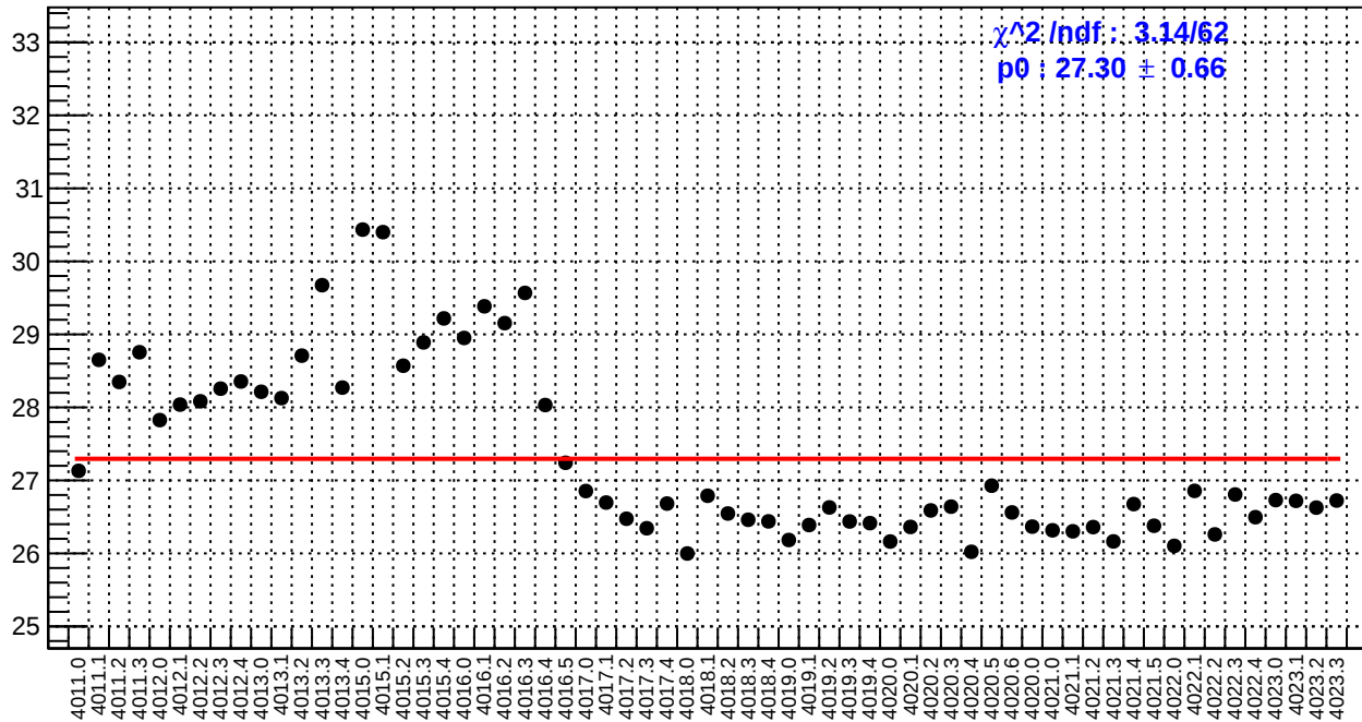
slug39: right_avg_bpm4eX/(ppb/nm)
