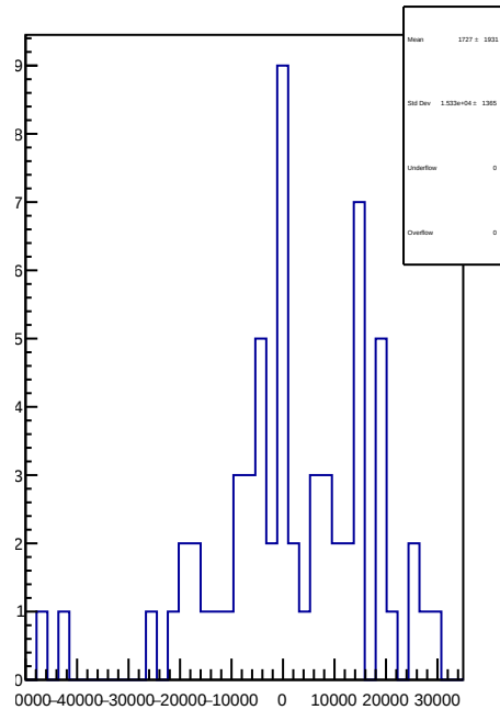
slug39: 1D Corr asym_sam5.mean/ppb-reg_asym_sam5.mean/ppb
