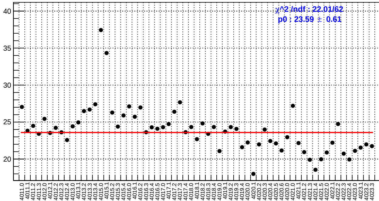
slug39: left_avg_bpm4aX/(ppb/nm)
