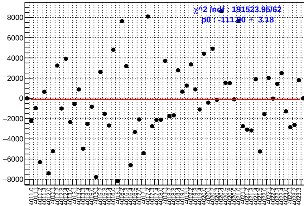
slug39: asym_us_dd.mean/ppb-reg_asym_us_dd.mean/ppb
