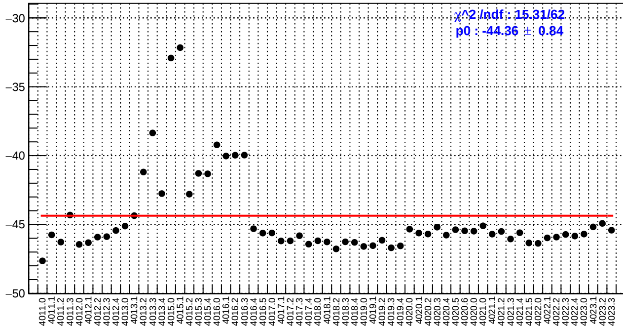
slug39: left_avg_bpm12X/(ppb/nm)
