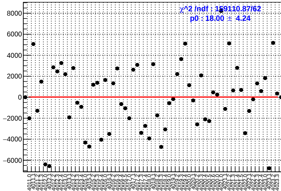
slug39: asym_ds_avg.mean/ppb-reg_asym_ds_avg.mean/ppb
