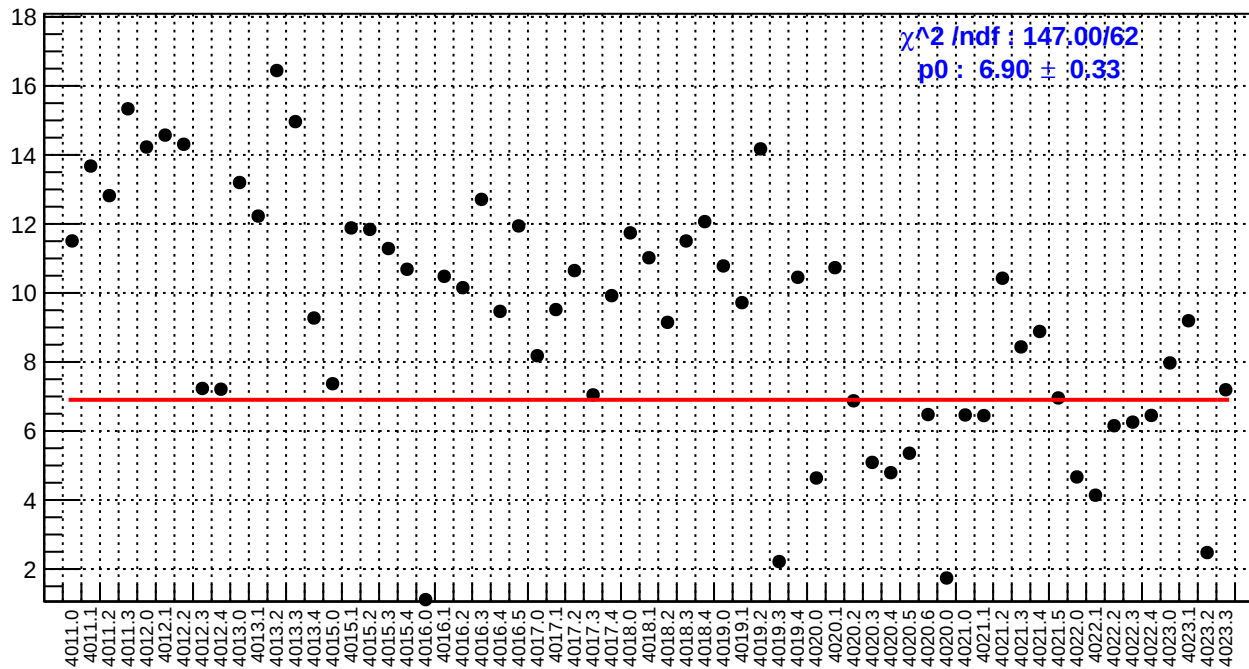
slug39: usl_bpm4eY/(ppb/nm)
