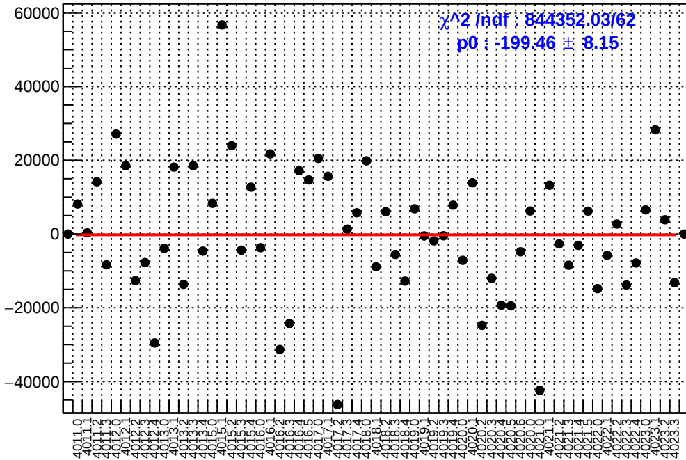
slug39: asym_sam8.mean/ppb-reg_asym_sam8.mean/ppb
