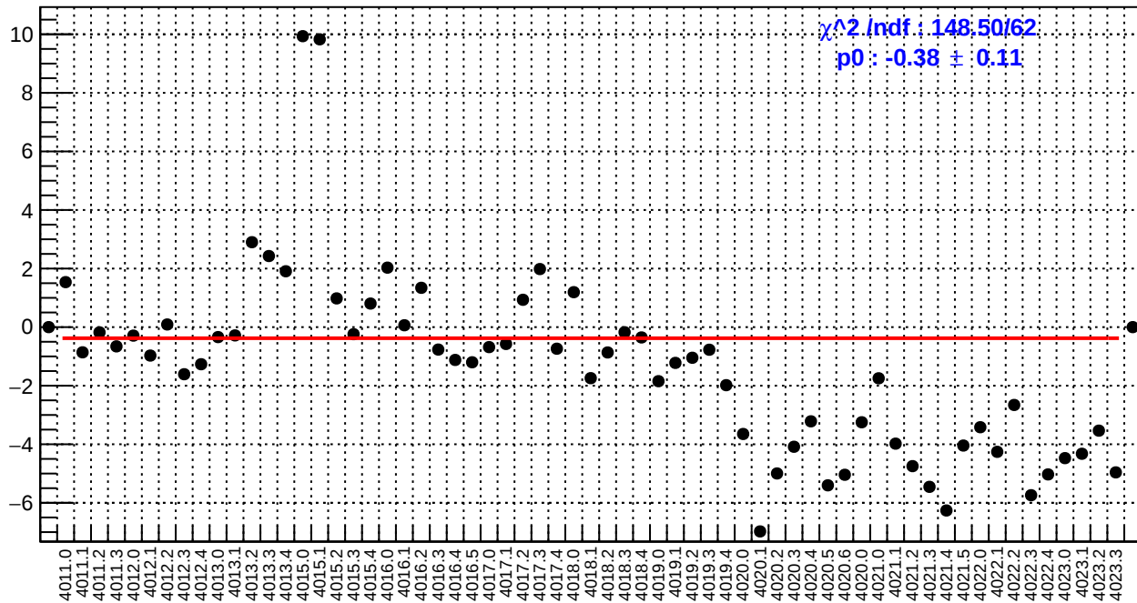
slug39: us_avg_bpm4aX/(ppb/nm)
