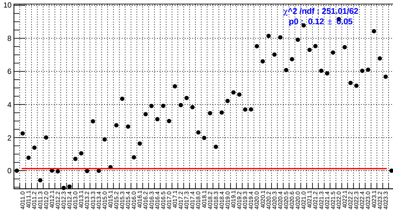
slug39: dsr_bpm4aY/(ppb/nm)
