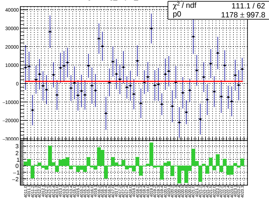
slug39: reg_asym_sam3.mean/ppb
