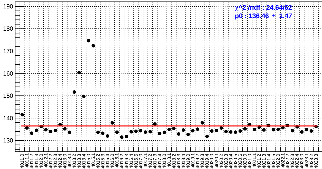
slug39: reg_asym_usl.rms/ppm
