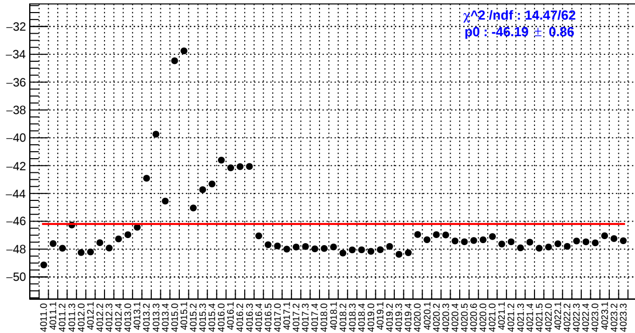
slug39: us_avg_bpm12X/(ppb/nm)
