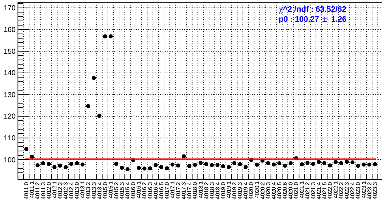
slug39: reg_asym_ds_avg.rms/ppm
