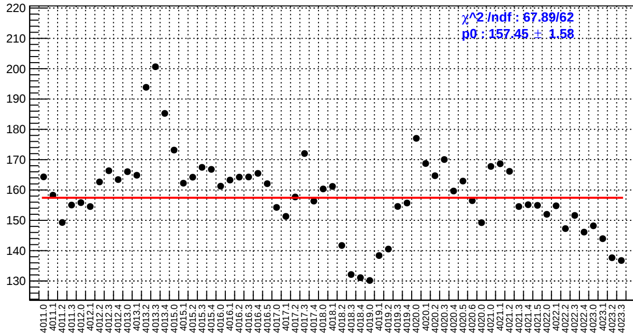
slug39: asym_bcm_an_ds.rms/ppm
