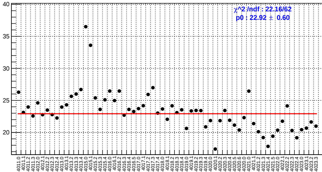
slug39: usl_bpm4aX/(ppb/nm)
