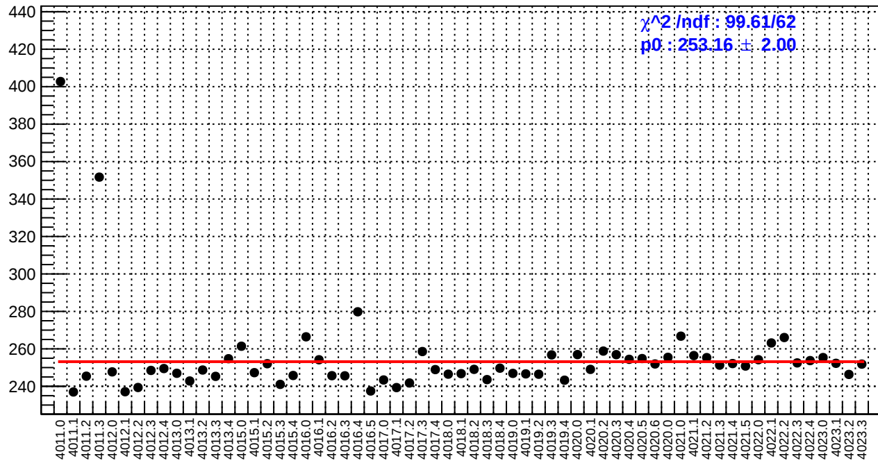
slug39: reg_asym_sam7.rms/ppm
