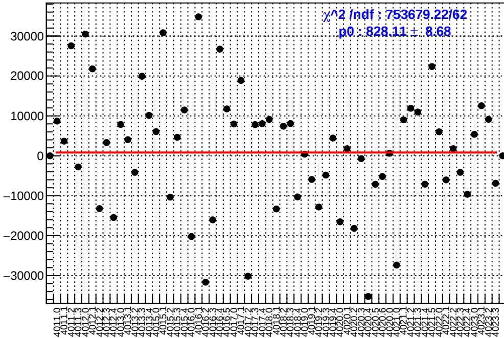
slug39: asym_sam7.mean/ppb-reg_asym_sam7.mean/ppb
