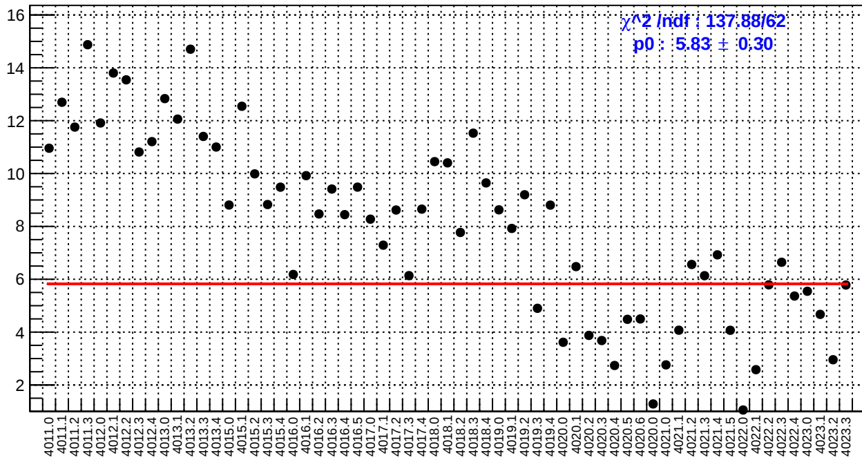
slug39: ds_avg_bpm4eY/(ppb/nm)
