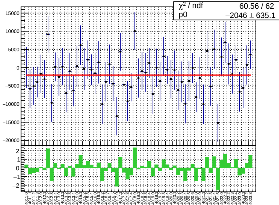
slug39: reg_asym_sam6.mean/ppb
