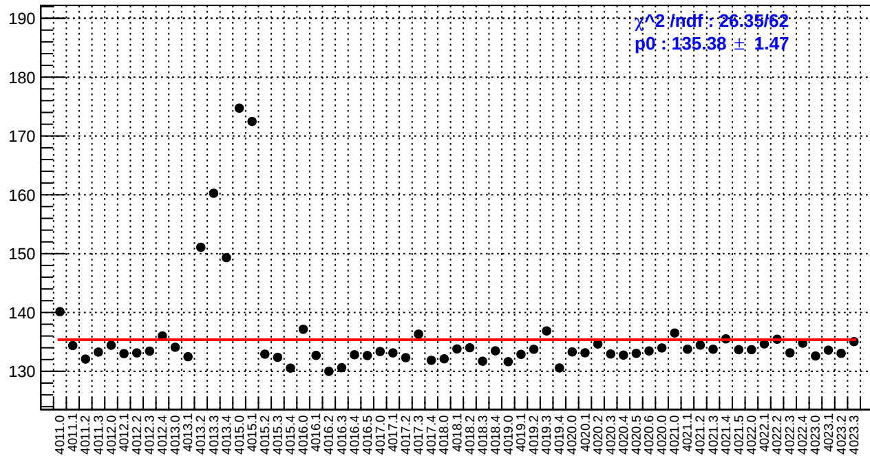
slug39: reg_asym_left_avg.rms/ppm
