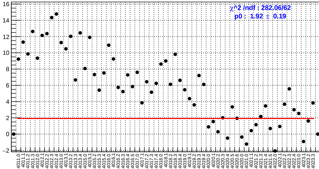
slug39: right_avg_bpm4eY/(ppb/nm)
