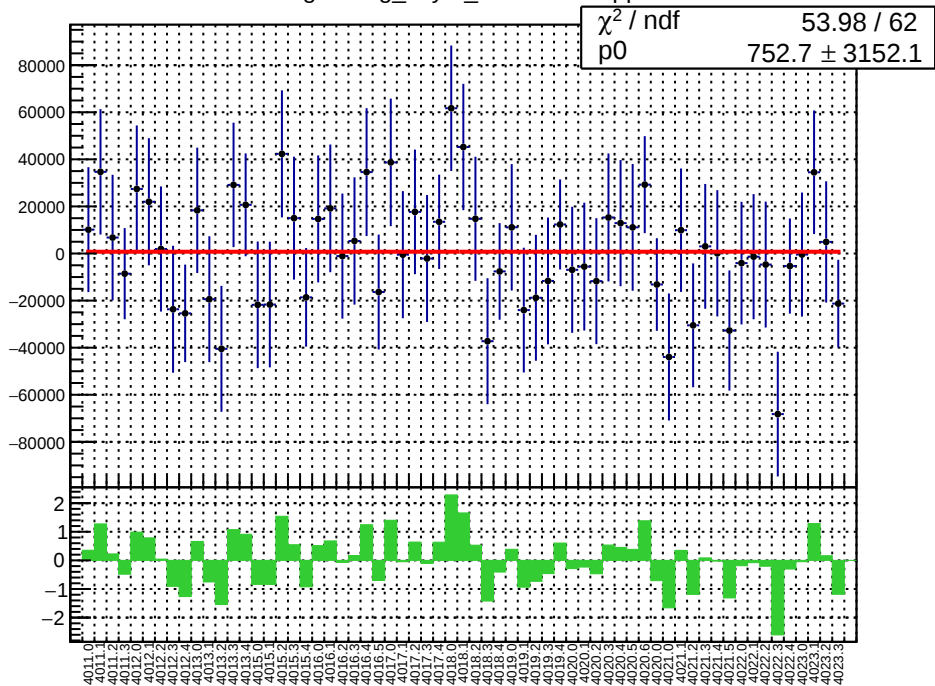
slug39: reg_asym_sam2.mean/ppb
