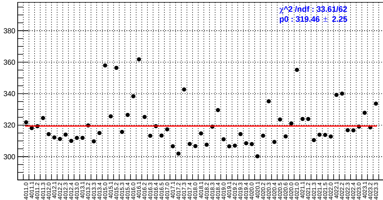
slug39: reg_asym_sam5.rms/ppm
