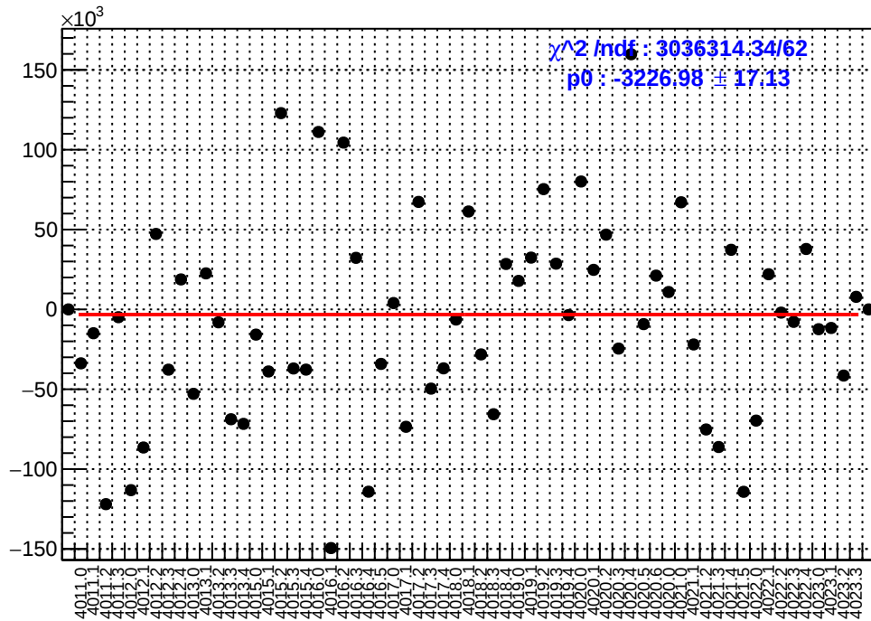
slug39: asym_sam2.mean/ppb-reg_asym_sam2.mean/ppb
