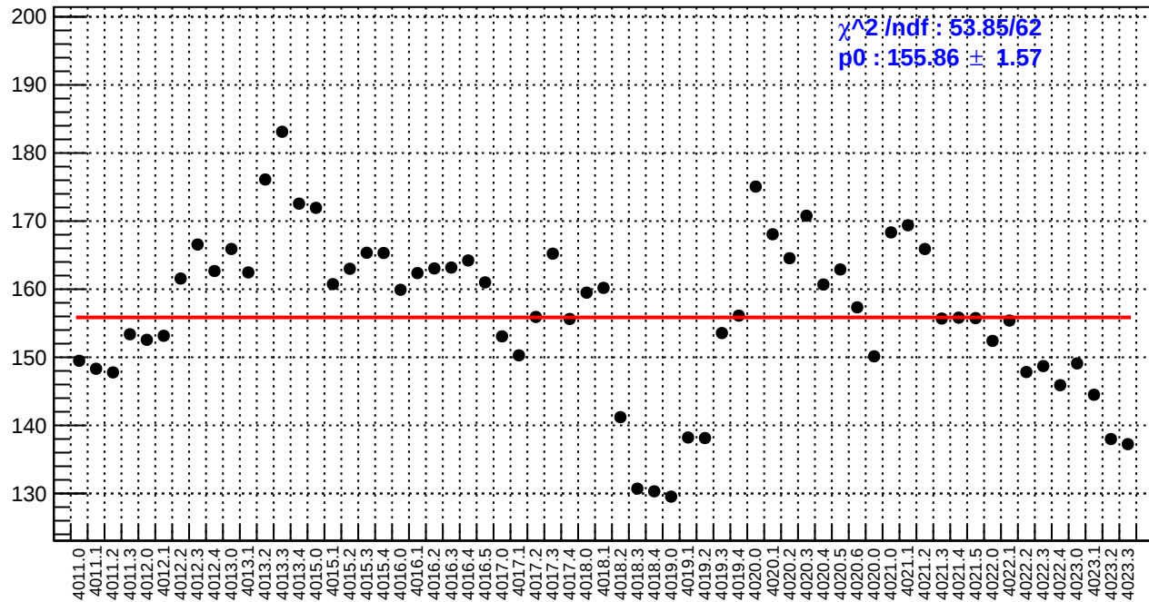
slug39: asym_bcm_an_us.rms/ppm
