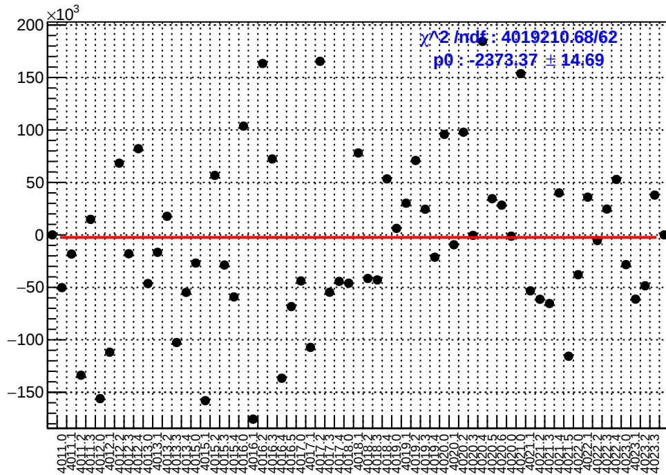
slug39: asym_sam3.mean/ppb-reg_asym_sam3.mean/ppb
