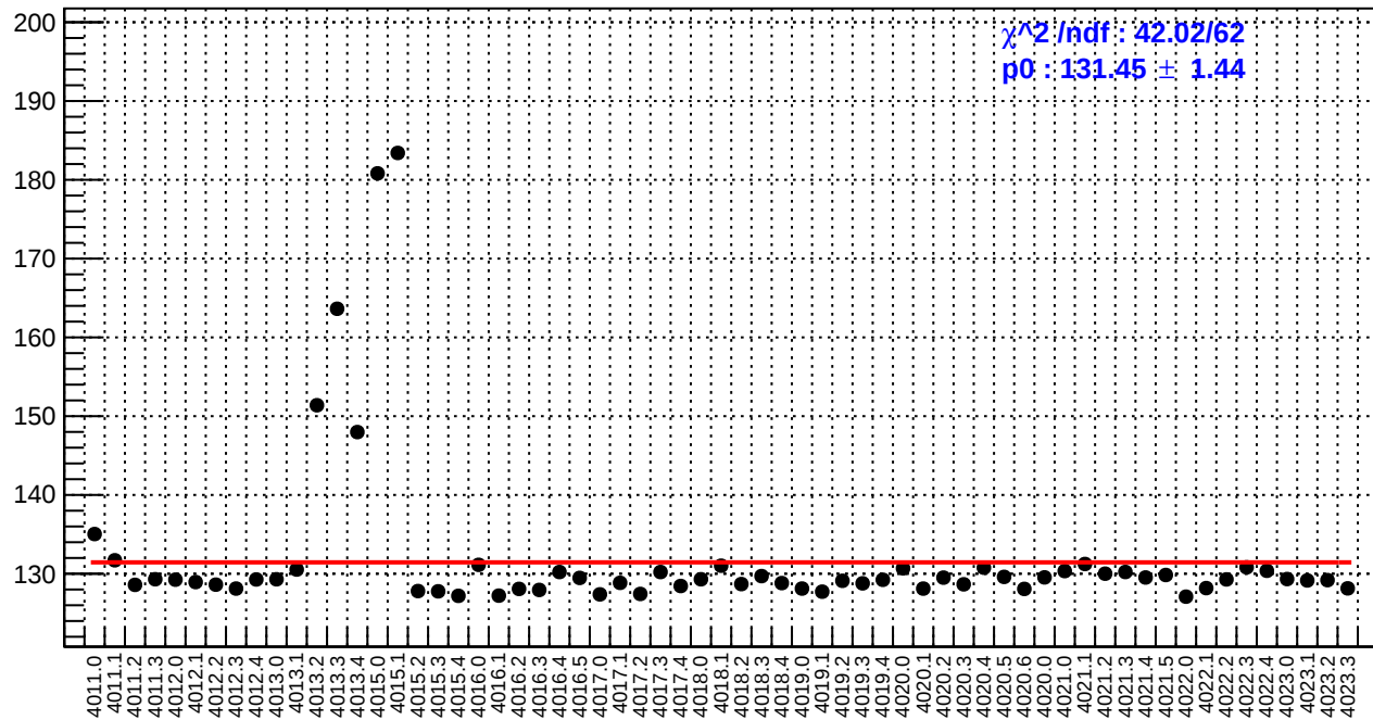
slug39: reg_asym_right_avg.rms/ppm
