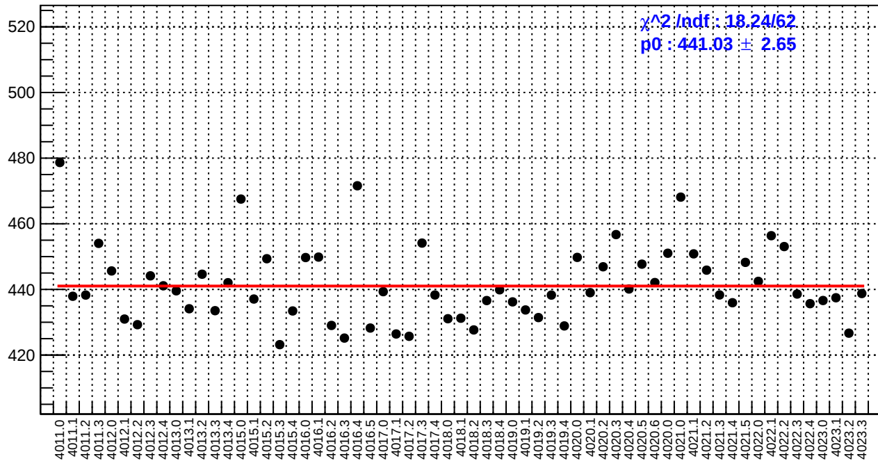
slug39: reg_asym_sam8.rms/ppm
