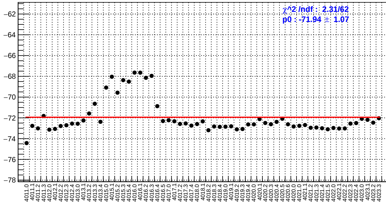
slug39: dsl_bpm4eX/(ppb/nm)
