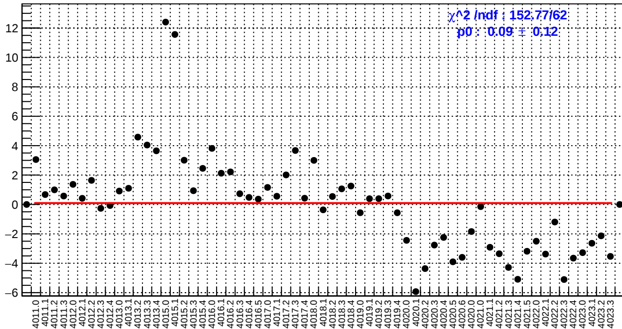
slug39: ds_avg_bpm4aX/(ppb/nm)
