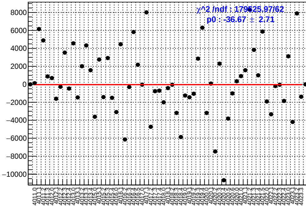
slug39: asym_dsr.mean/ppb-reg_asym_dsr.mean/ppb
