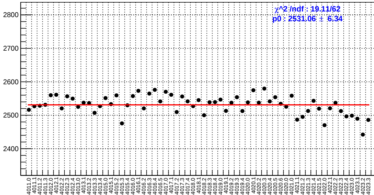
slug39: reg_asym_sam2.rms/ppm
