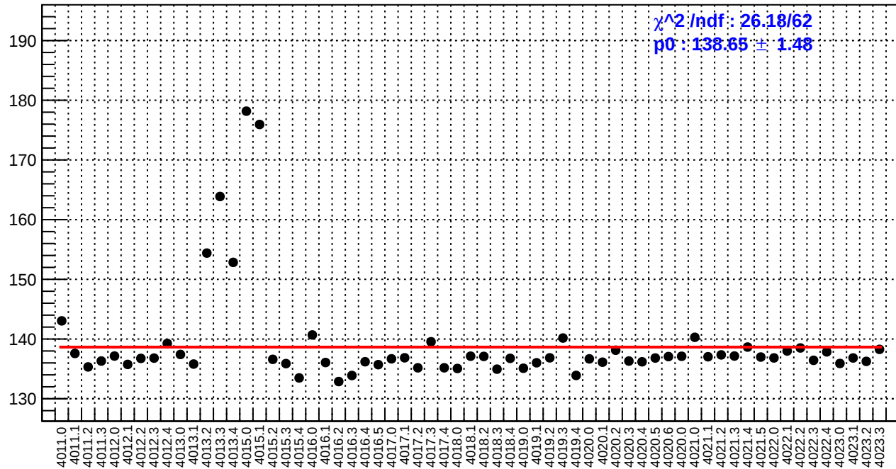
slug39: reg_asym_dsl.rms/ppm
