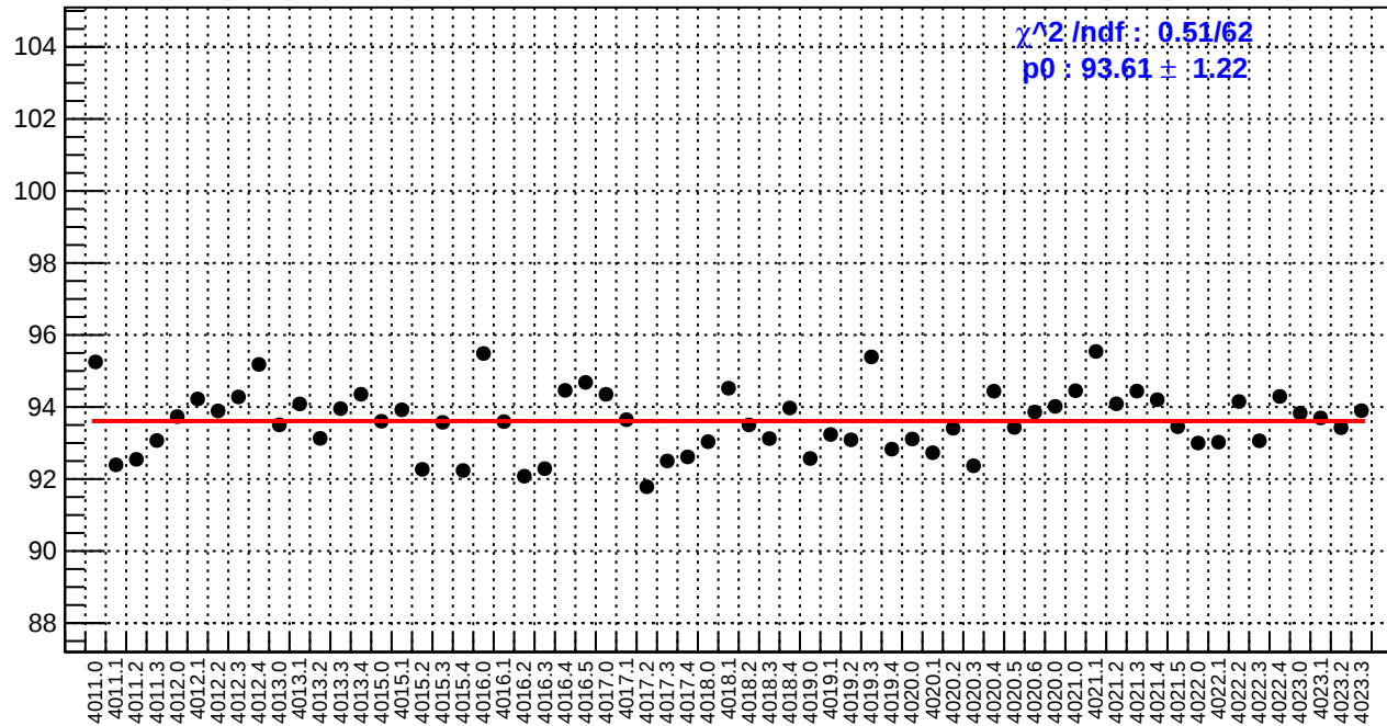
slug39: reg_asym_ds_dd.rms/ppm
