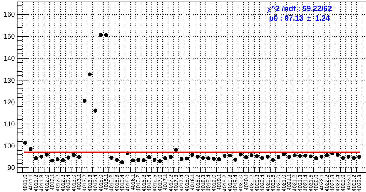
slug39: reg_asym_us_avg.rms/ppm
