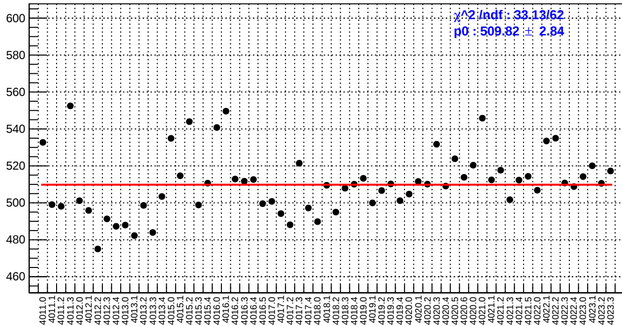
slug39: reg_asym_sam6.rms/ppm
