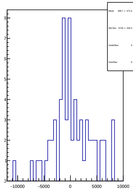
slug39: 1D Corr asym_dsr.mean/ppb-reg_asym_dsr.mean/ppb
