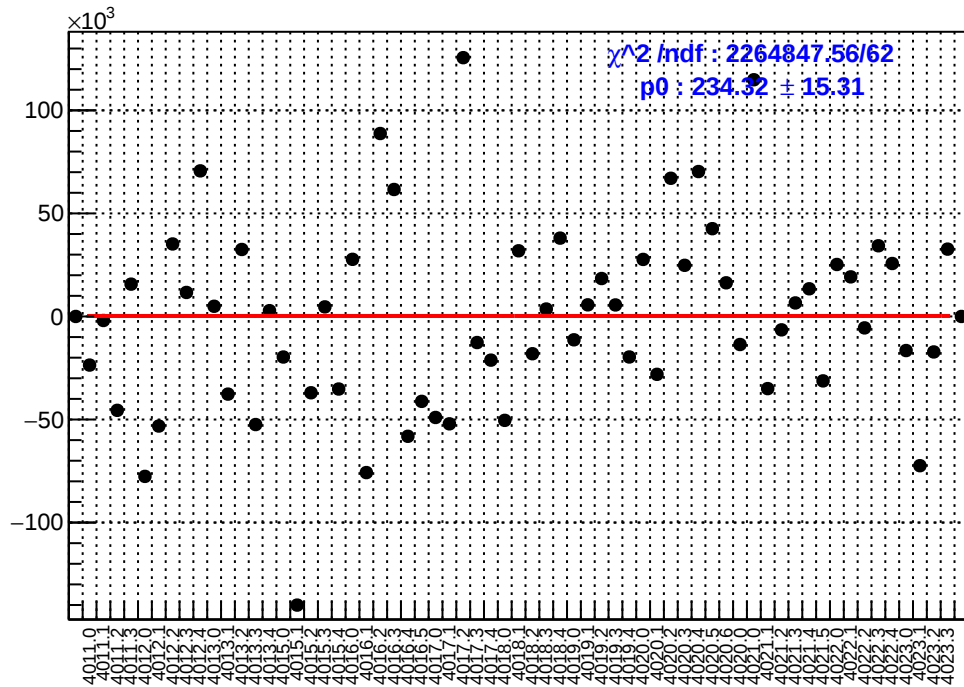
slug39: asym_sam4.mean/ppb-reg_asym_sam4.mean/ppb
