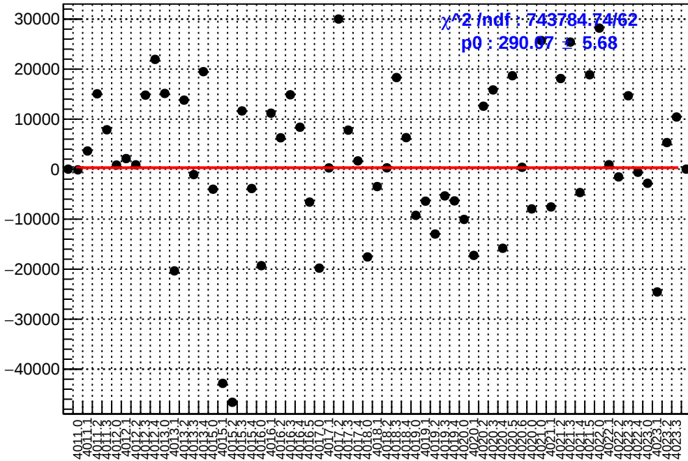
slug39: asym_sam5.mean/ppb-reg_asym_sam5.mean/ppb
