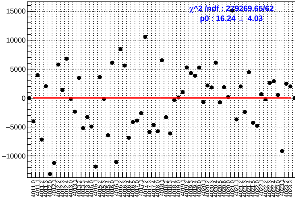
slug39: asym_left_avg.mean/ppb-reg_asym_left_avg.mean/ppb
