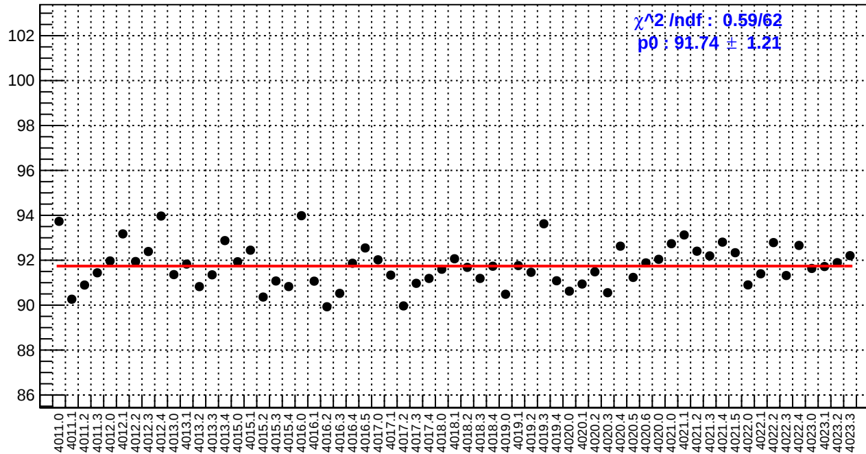
slug39: reg_asym_us_dd.rms/ppm
