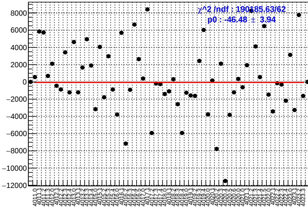
slug39: asym_usr.mean/ppb-reg_asym_usr.mean/ppb
