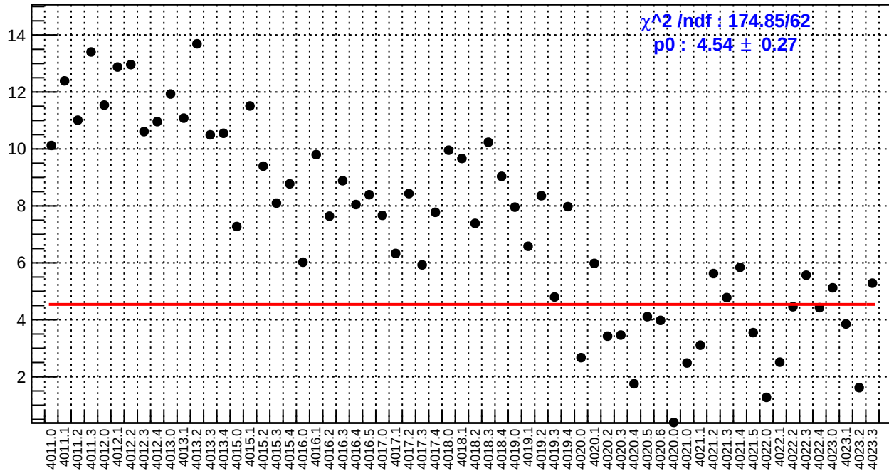
slug39: us_avg_bpm4eY/(ppb/nm)
