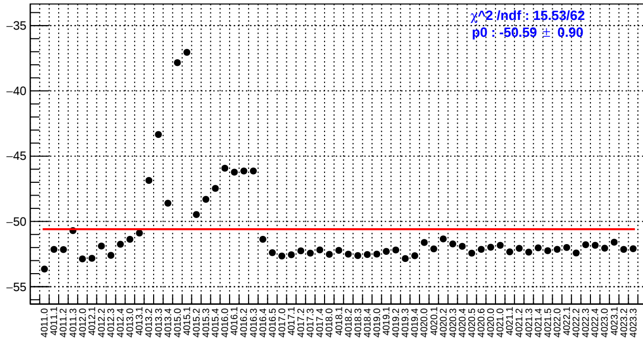
slug39: right_avg_bpm12X/(ppb/nm)
