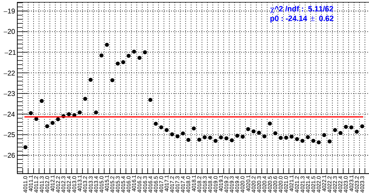
slug39: ds_avg_bpm4eX/(ppb/nm)
