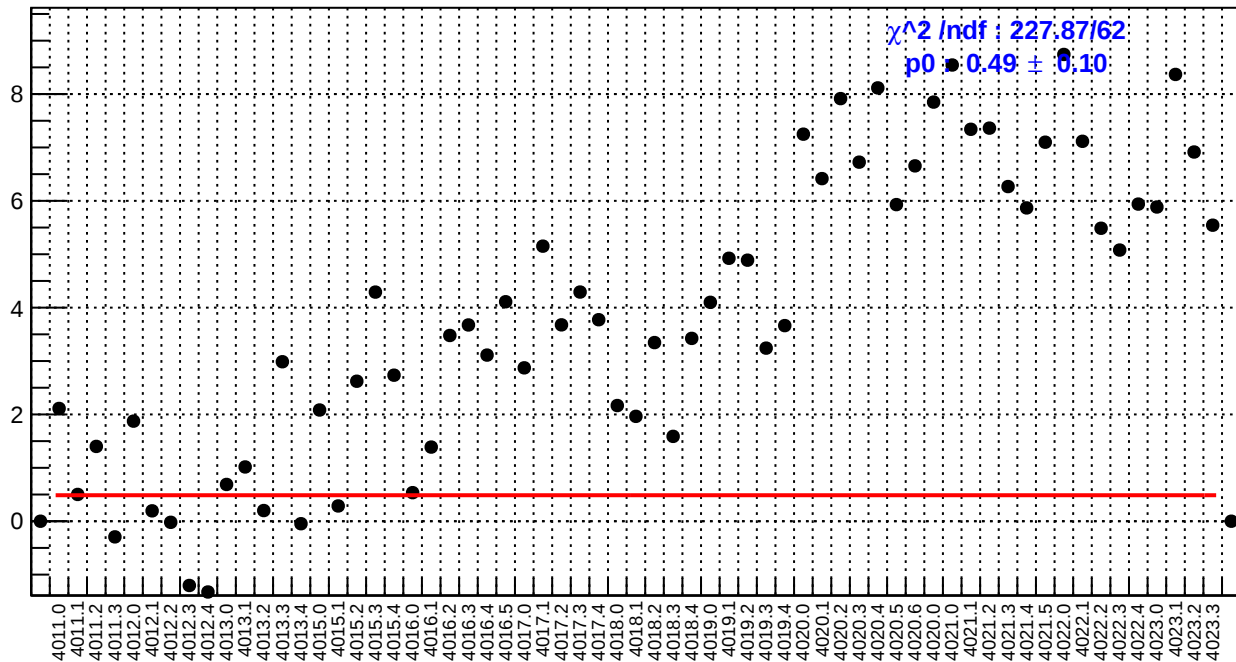
slug39: right_avg_bpm4aY/(ppb/nm)
