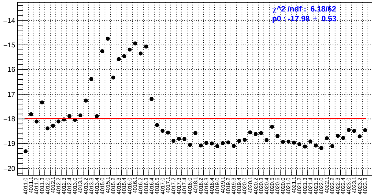
slug39: us_avg_bpm4eX/(ppb/nm)
