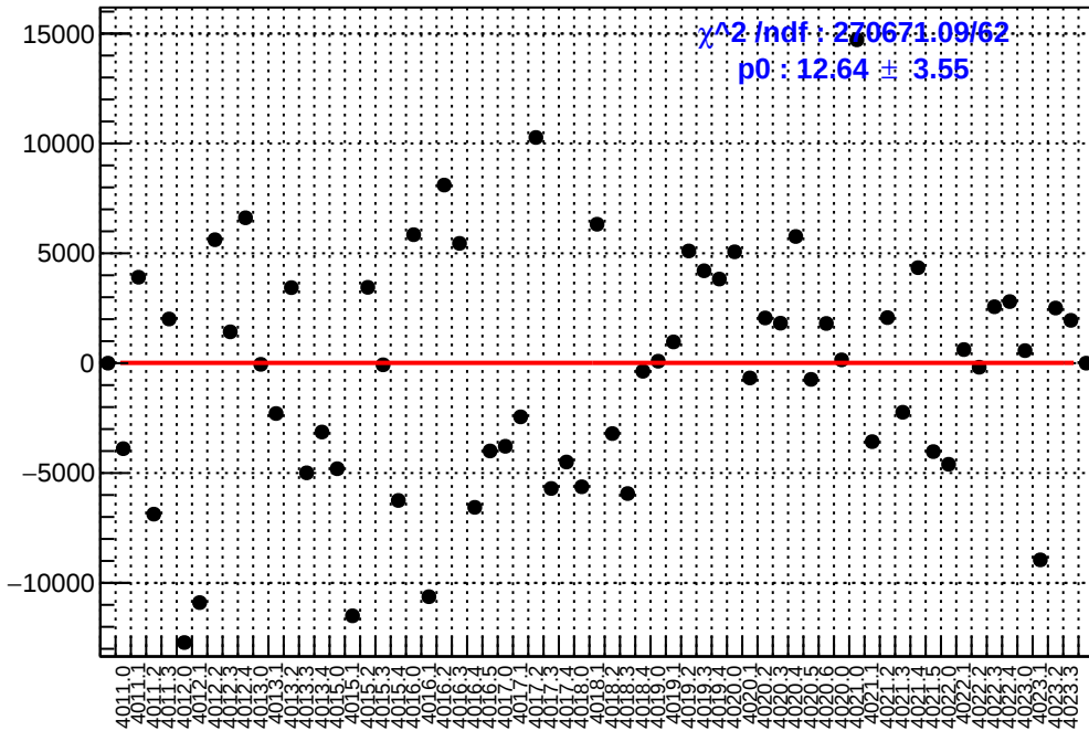
slug39: asym_usl.mean/ppb-reg_asym_usl.mean/ppb
