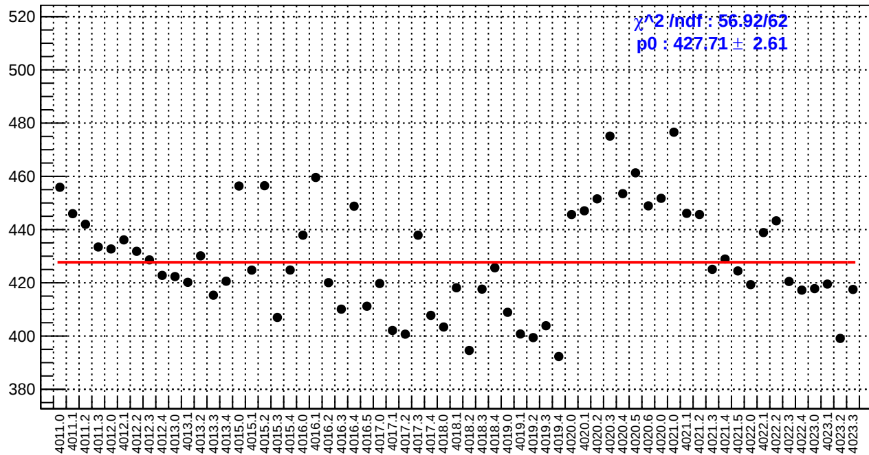
slug39: reg_asym_sam1.rms/ppm
