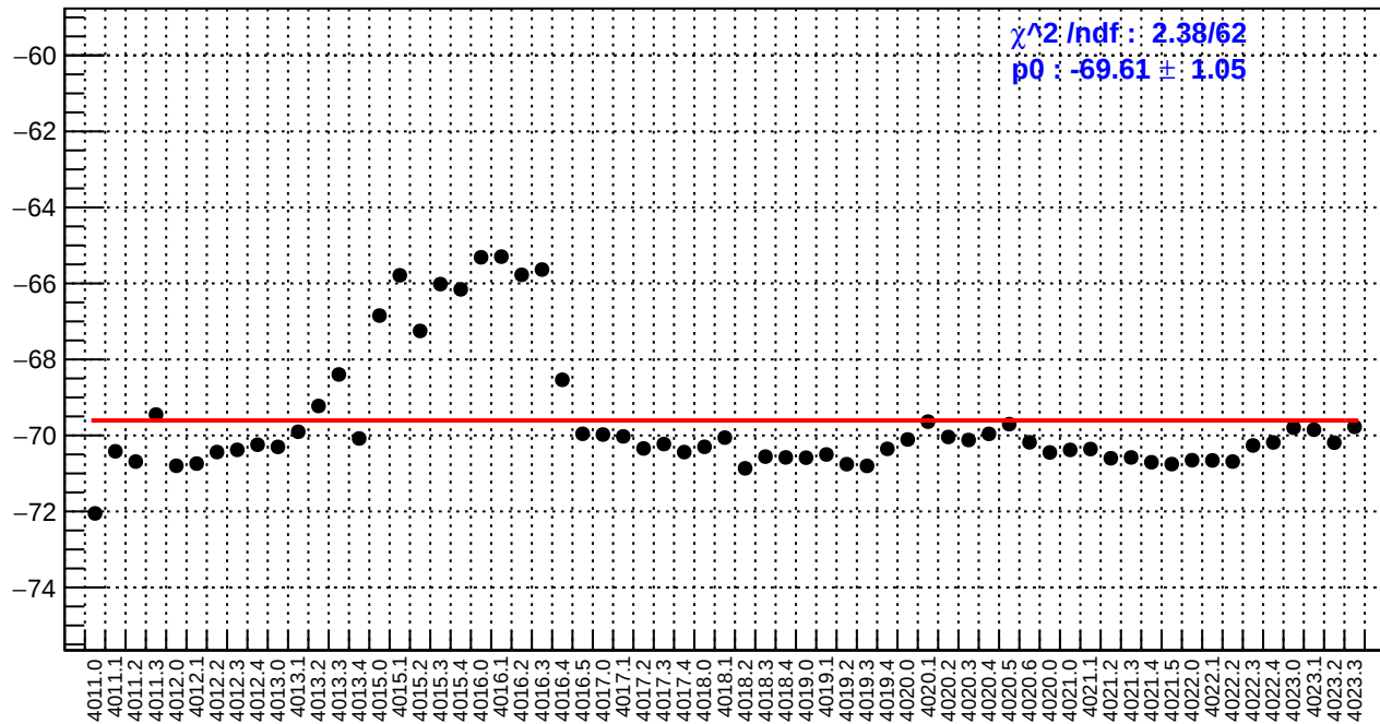
slug39: left_avg_bpm4eX/(ppb/nm)
