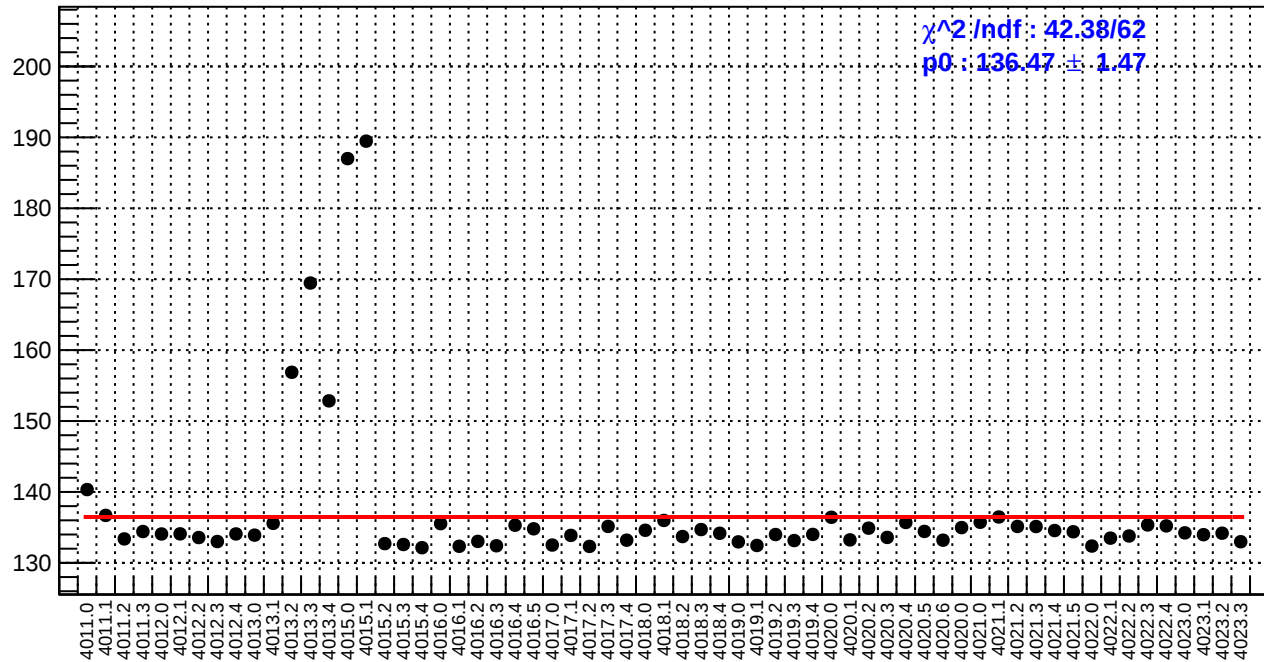
slug39: reg_asym_dsr.rms/ppm
