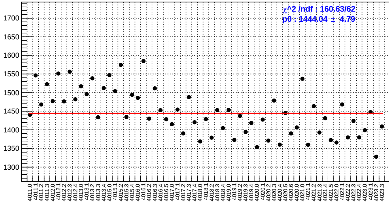
slug39: diff_bpm4aX.rms/nm
