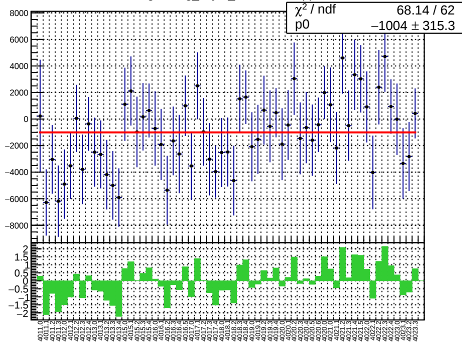
slug39: reg_asym_sam7.mean/ppb
