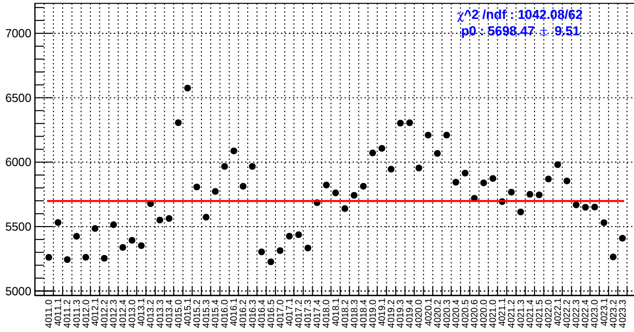
slug39: diff_bpm11X.rms/nm
