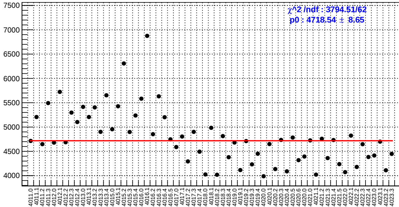
slug39: diff_bpm4eY.rms/nm
