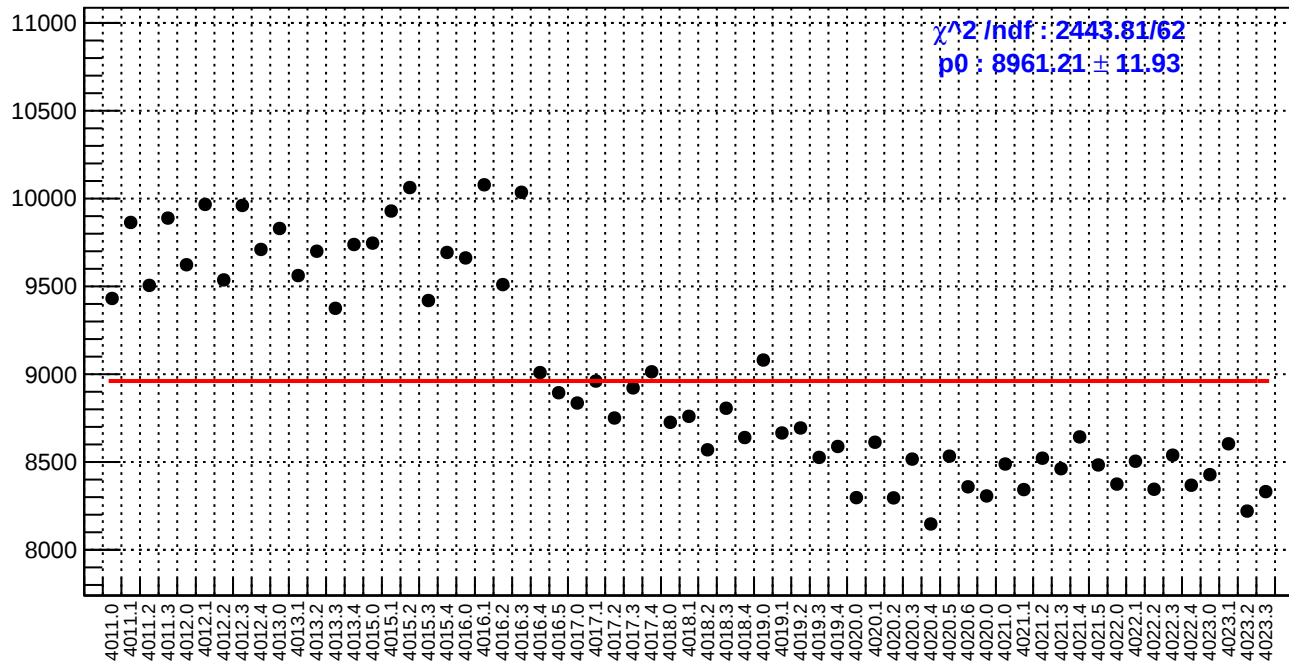
slug39: diff_bpm4eX.rms/nm
