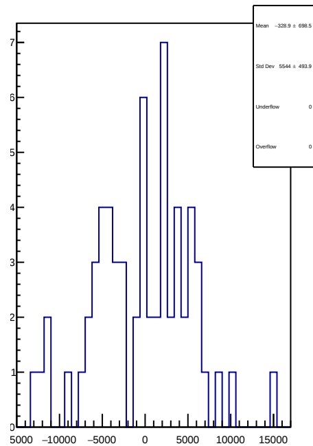
slug39: 1D Corr asym_left_avg.mean/ppb-reg_asym_left_avg.mean/ppb
