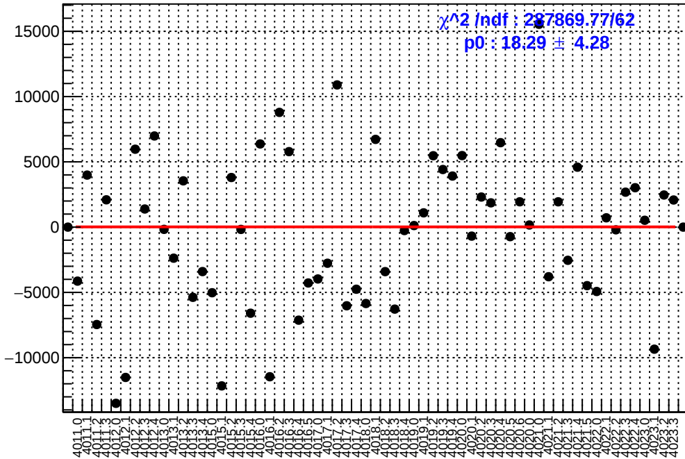
slug39: asym_dsl.mean/ppb-reg_asym_dsl.mean/ppb
