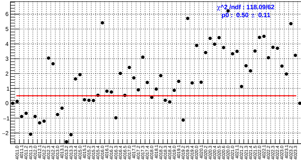
slug39: left_avg_bpm4aY/(ppb/nm)
