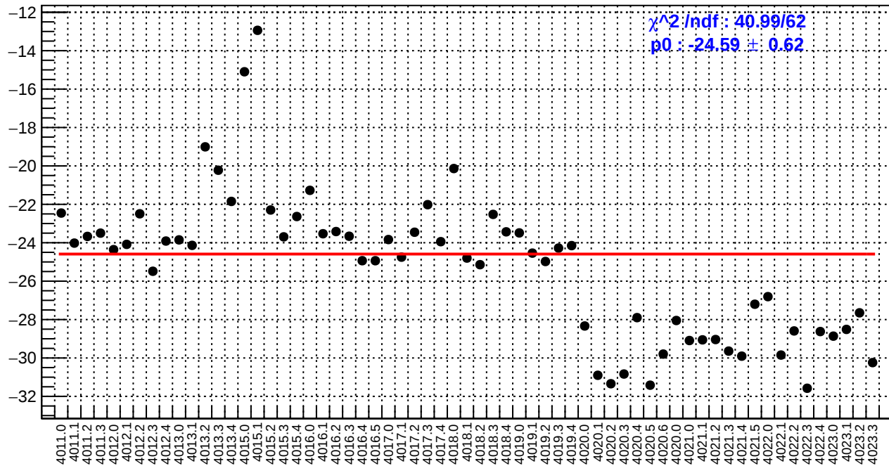
slug39: right_avg_bpm4aX/(ppb/nm)
