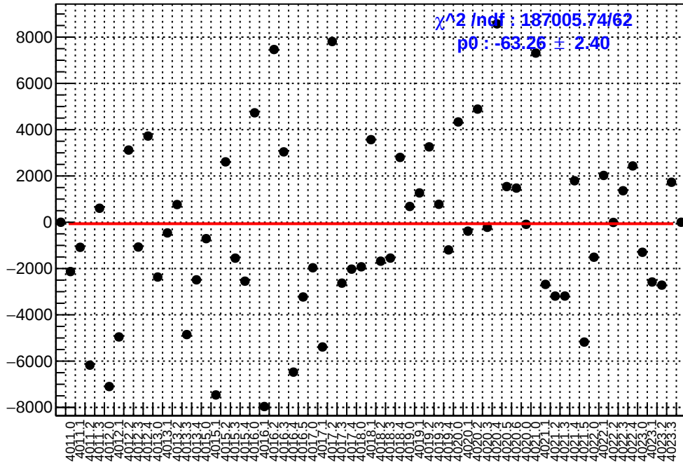
slug39: asym_ds_dd.mean/ppb-reg_asym_ds_dd.mean/ppb
