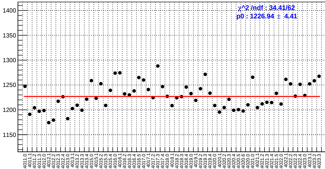
slug39: reg_asym_sam4.rms/ppm
