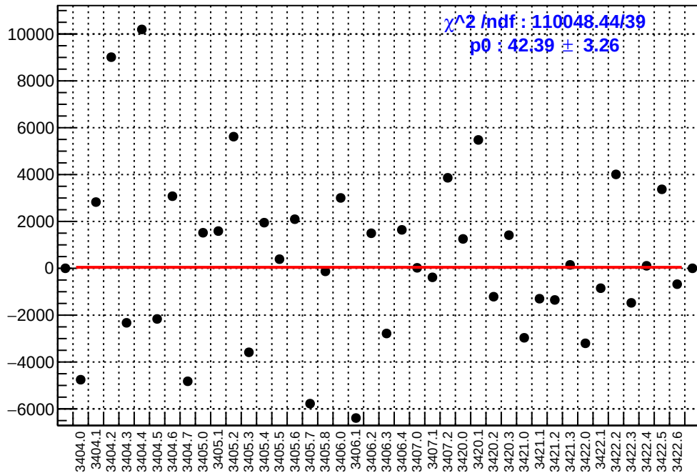
slug4: asym_right_avg.mean/ppb-reg_asym_right_avg.mean/ppb
