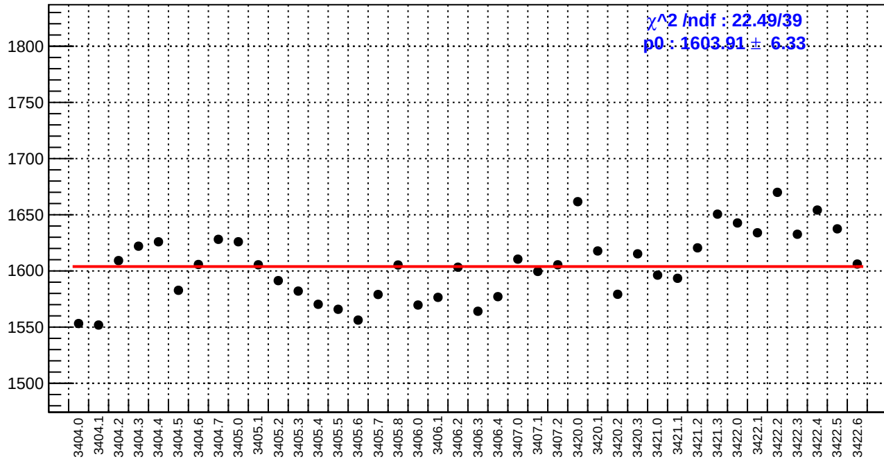
slug4: diff_bpm4aX.rms/nm
