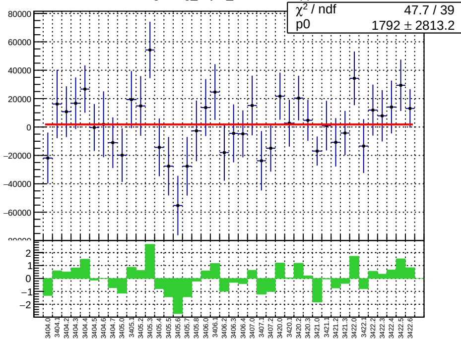
slug4: reg_asym_sam3.mean/ppb
