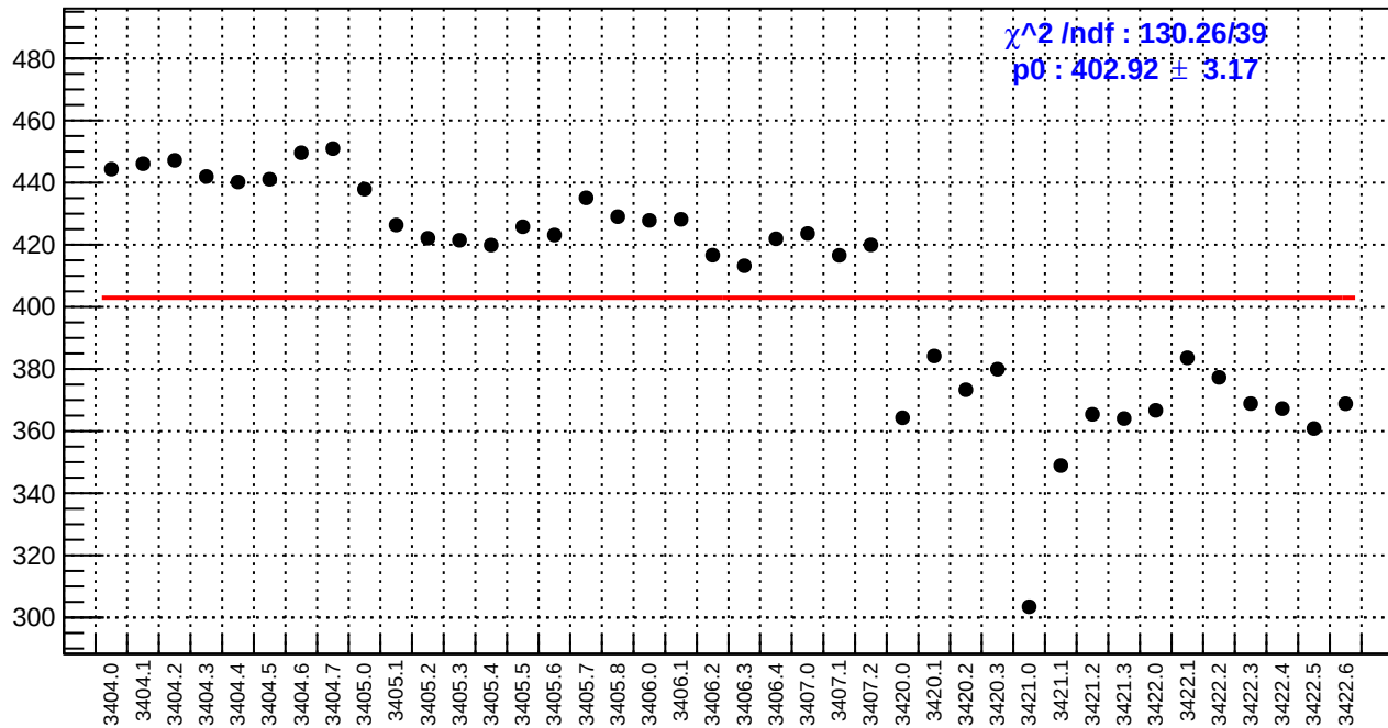
slug4: reg_asym_sam5.rms/ppm
