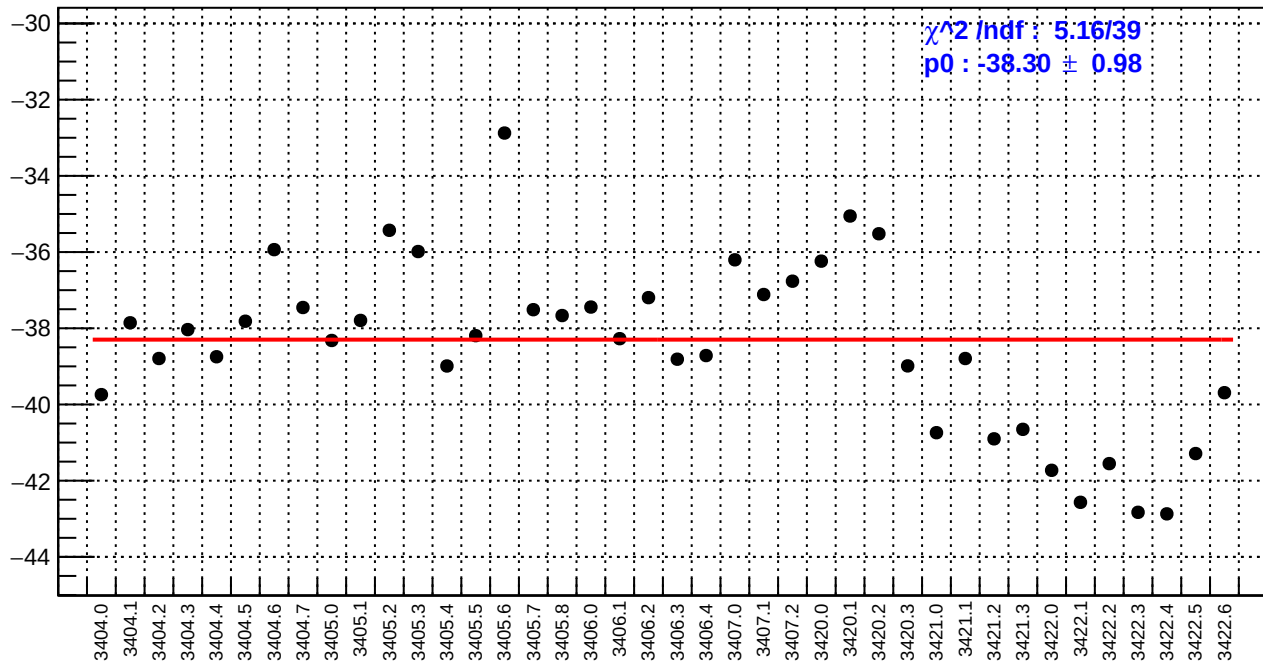
slug4: usl_bpm4aY/(ppb/nm)
