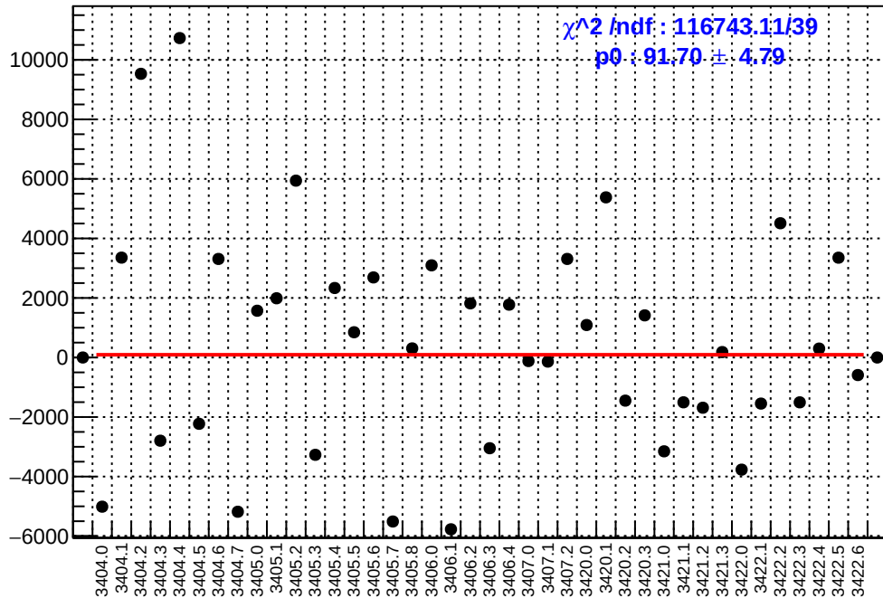
slug4: asym_usr.mean/ppb-reg_asym_usr.mean/ppb
