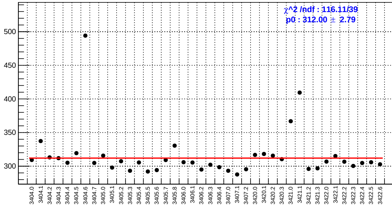
slug4: reg_asym_sam7.rms/ppm
