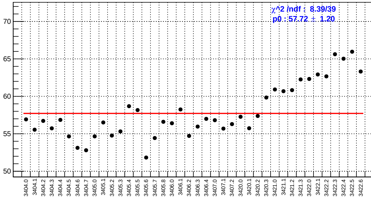
slug4: usl_bpm4eY/(ppb/nm)
