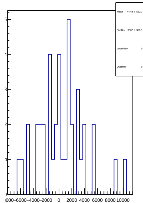
slug4: 1D Corr asym_right_avg.mean/ppb-reg_asym_right_avg.mean/ppb
