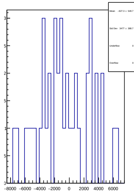
slug4: 1D Corr asym_ds_dd.mean/ppb-reg_asym_ds_dd.mean/ppb
