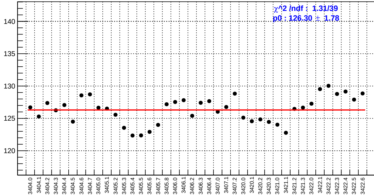
slug4: reg_asym_ds_avg.rms/ppm
