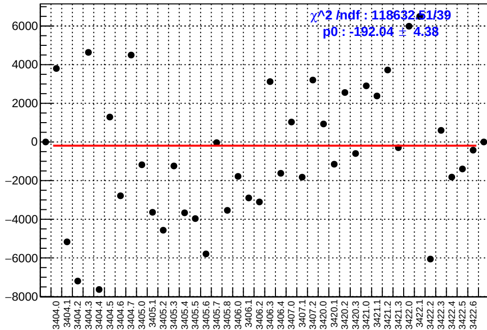
slug4: asym_us_dd.mean/ppb-reg_asym_us_dd.mean/ppb
