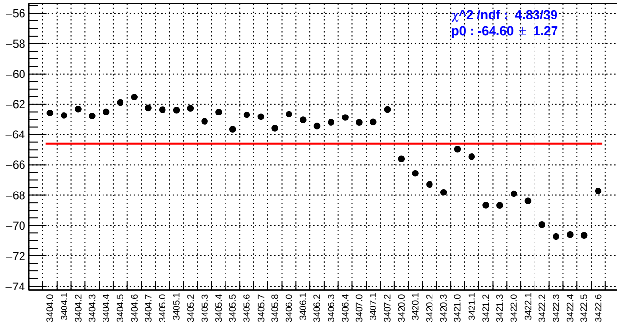
slug4: left_avg_bpm4eX/(ppb/nm)
