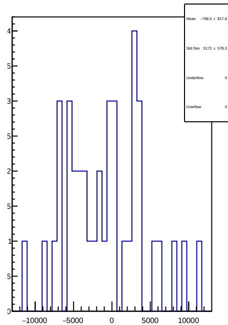
slug4: 1D Corr asym_usl.mean/ppb-reg_asym_usl.mean/ppb
