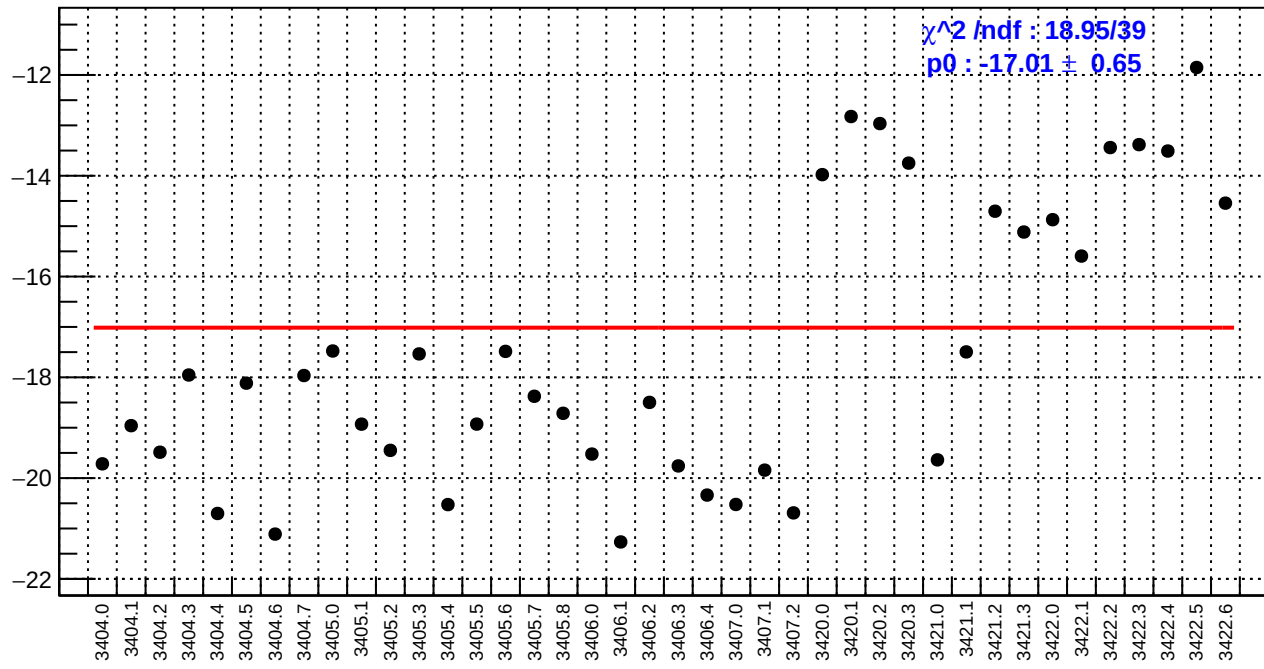
slug4: dsr_bpm4eY/(ppb/nm)
