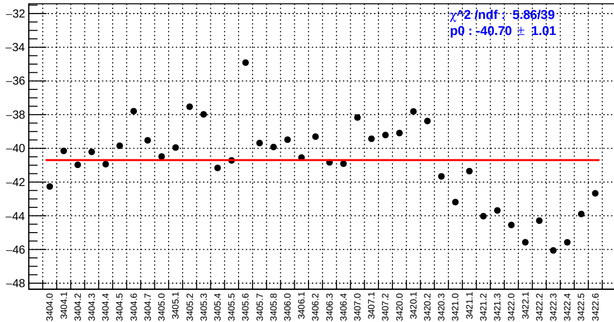
slug4: left_avg_bpm4aY/(ppb/nm)
