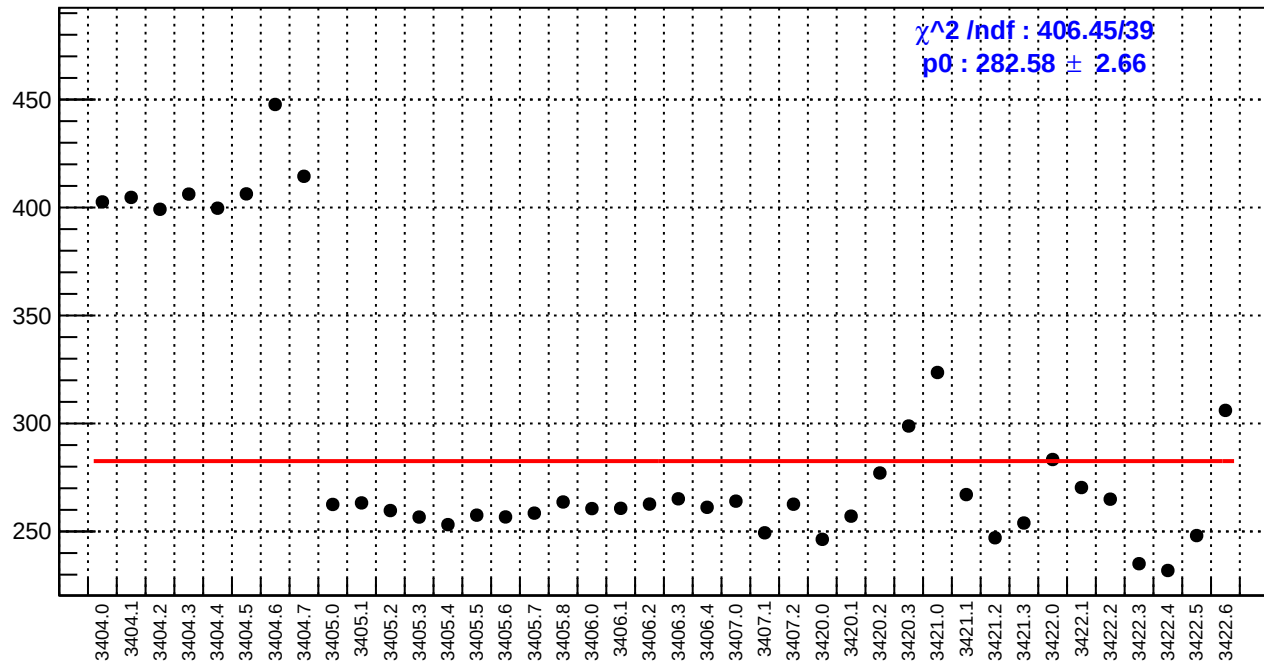
slug4: reg_asym_sam8.rms/ppm
