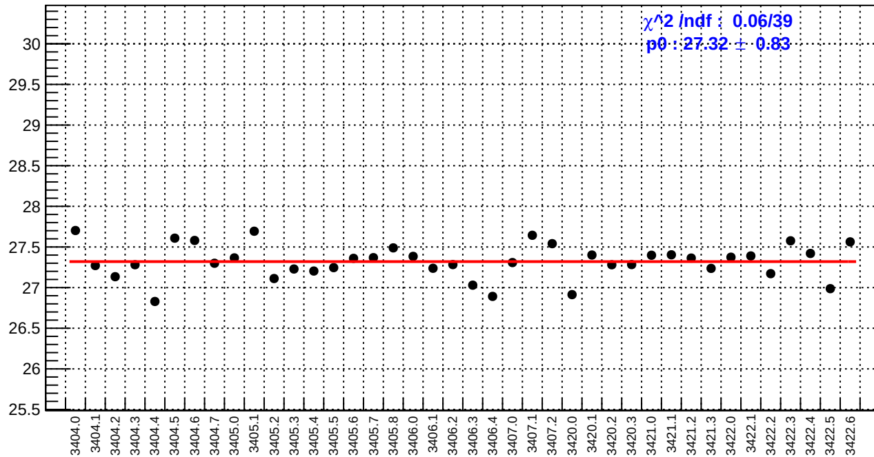
slug4: reg_asym_right_dd.rms/ppm
