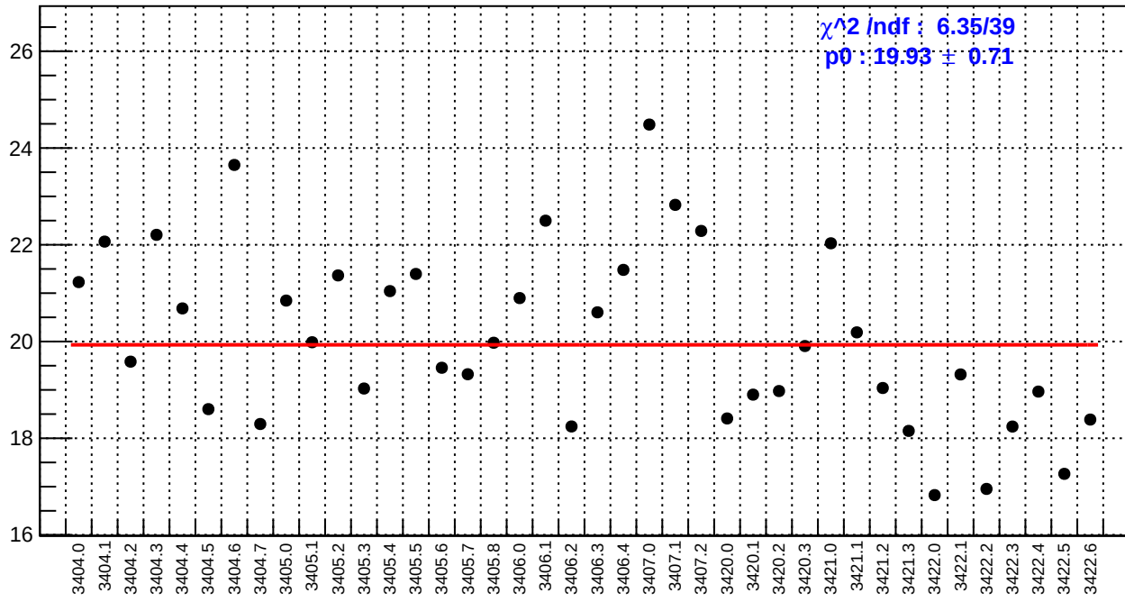
slug4: dsr_bpm4aY/(ppb/nm)
