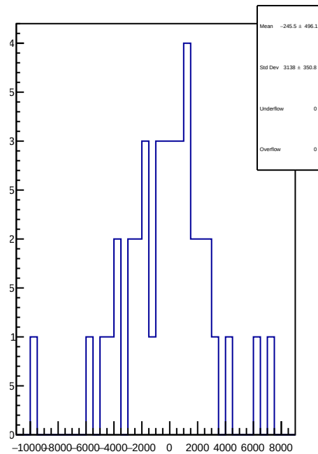
slug4: 1D Corr asym_ds_avg.mean/ppb-reg_asym_ds_avg.mean/ppb
