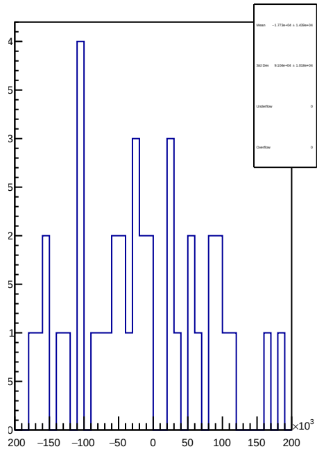
slug4: 1D Corr asym_sam3.mean/ppb-reg_asym_sam3.mean/ppb
