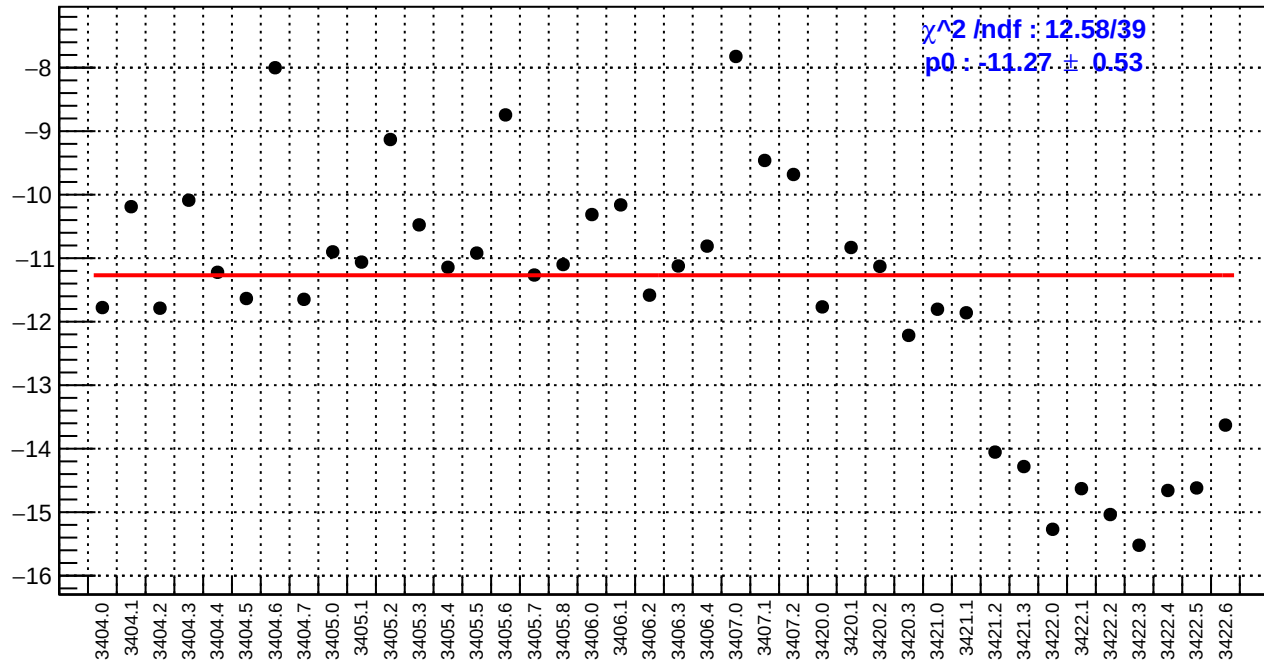
slug4: ds_avg_bpm4aY/(ppb/nm)
