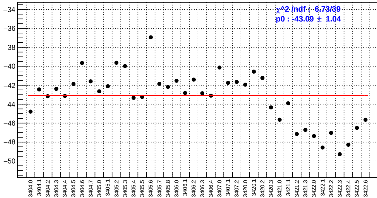
slug4: dsl_bpm4aY/(ppb/nm)
