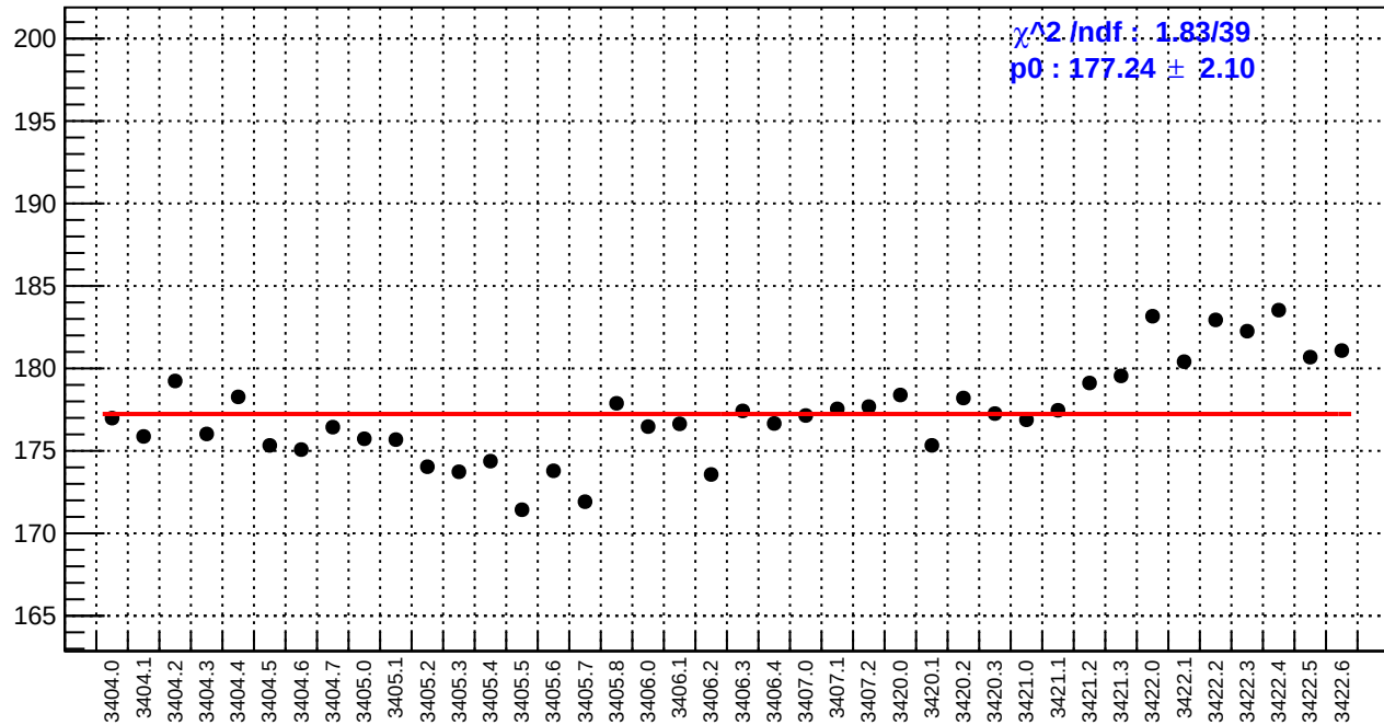
slug4: reg_asym_dsl.rms/ppm
