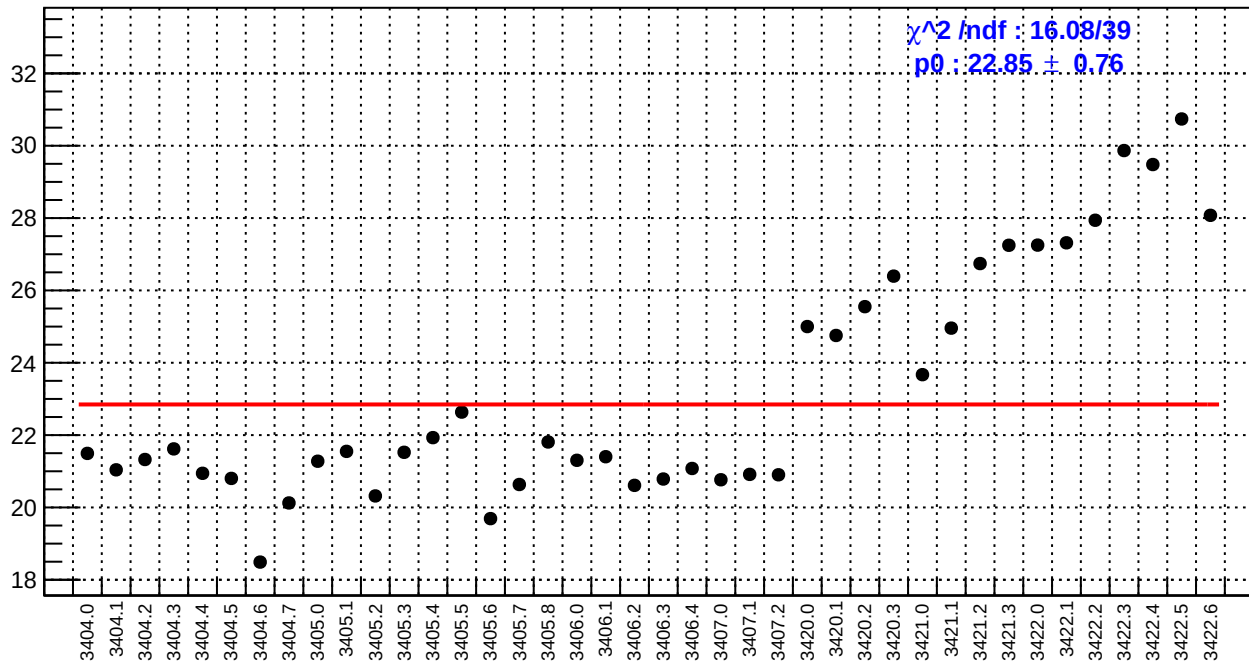
slug4: ds_avg_bpm4eY/(ppb/nm)
