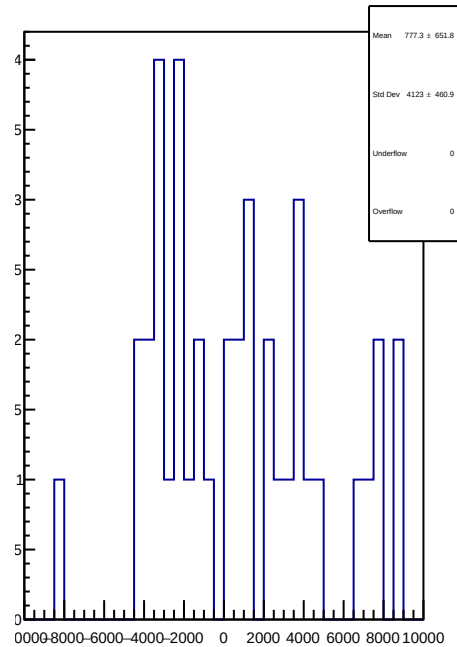
slug4: 1D Corr asym_sam1.mean/ppb-reg_asym_sam1.mean/ppb
