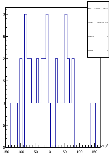
slug4: 1D Corr asym_sam2.mean/ppb-reg_asym_sam2.mean/ppb
