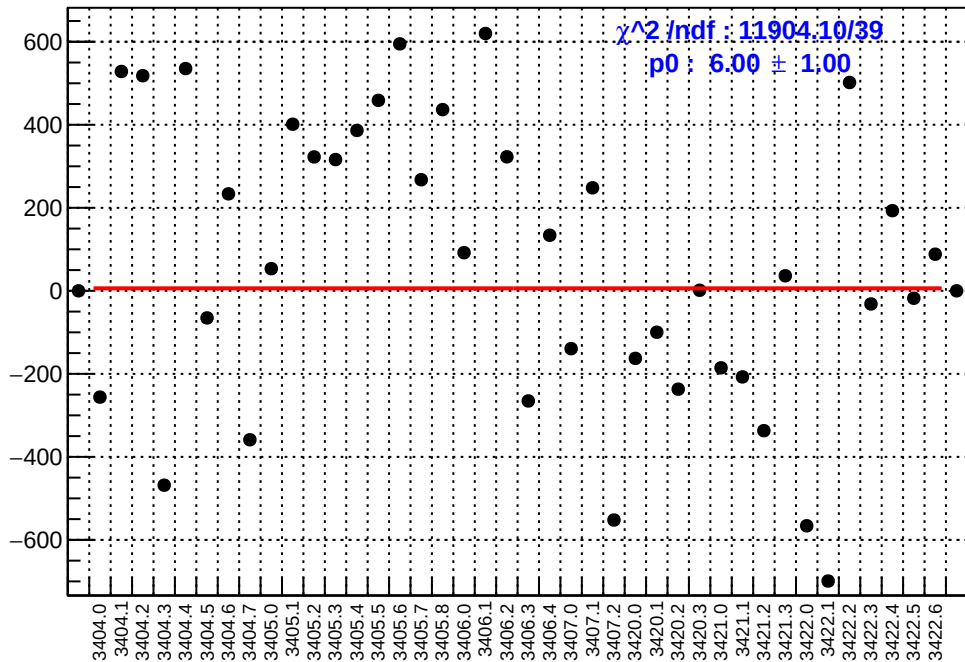
slug4: asym_right_dd.mean/ppb-reg_asym_right_dd.mean/ppb
