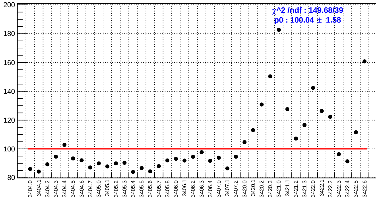
slug4: asym_bcm_an_us.rms/ppm
