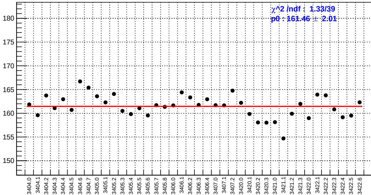
slug4: reg_asym_right_avg.rms/ppm
