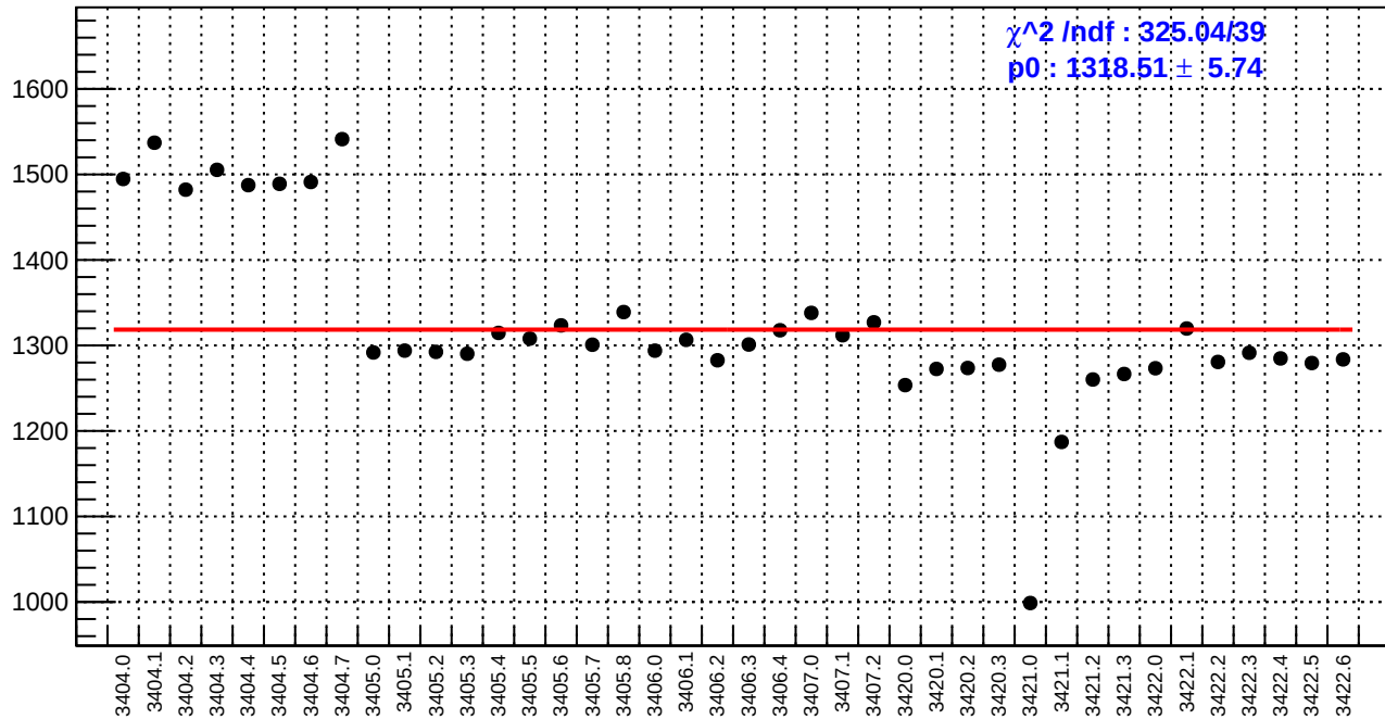
slug4: reg_asym_sam4.rms/ppm
