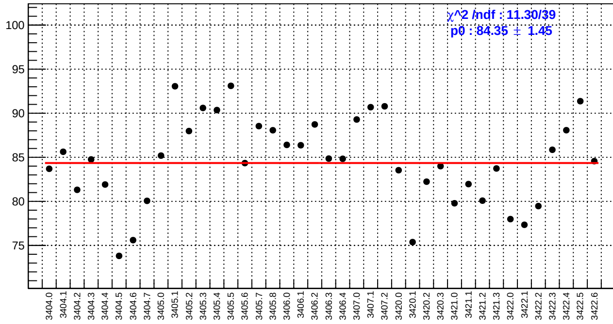
slug4: dsr_bpm4aX/(ppb/nm)
