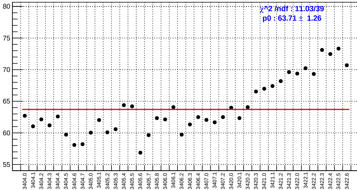
slug4: dsl_bpm4eY/(ppb/nm)
