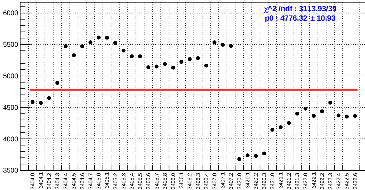
slug4: diff_bpm12X.rms/nm
