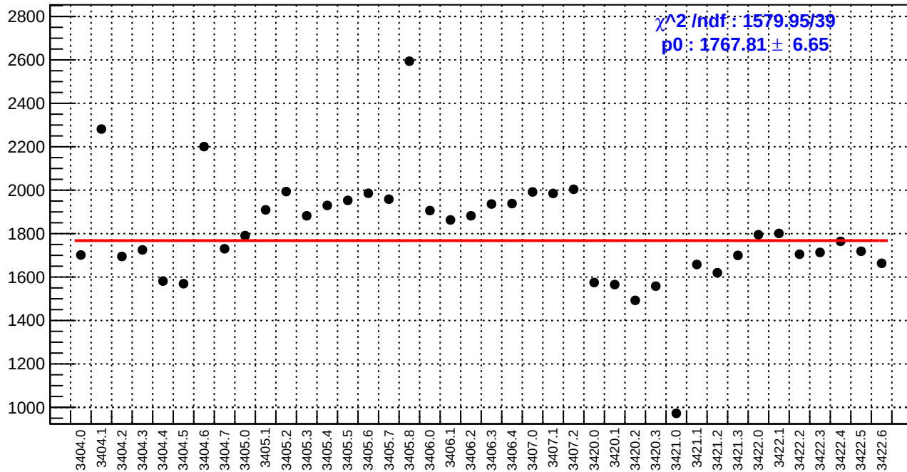
slug4: reg_asym_sam3.rms/ppm
