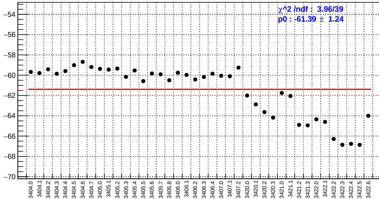
slug4: usl_bpm4eX/(ppb/nm)
