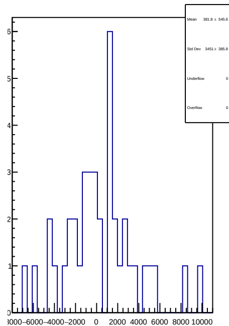
slug4: 1D Corr asym_dsr.mean/ppb-reg_asym_dsr.mean/ppb
