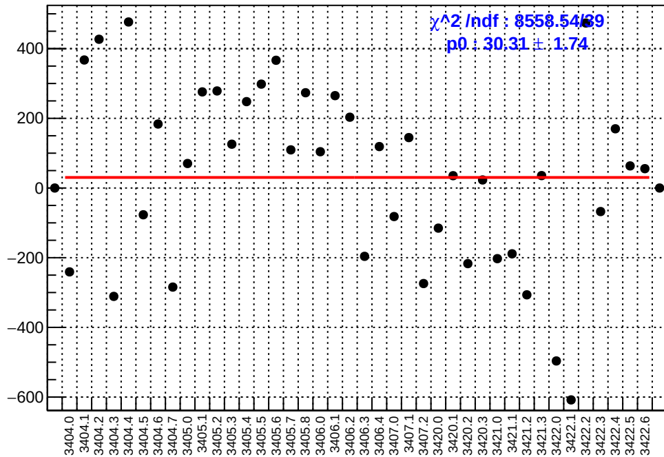
slug4: asym_left_dd.mean/ppb-reg_asym_left_dd.mean/ppb
