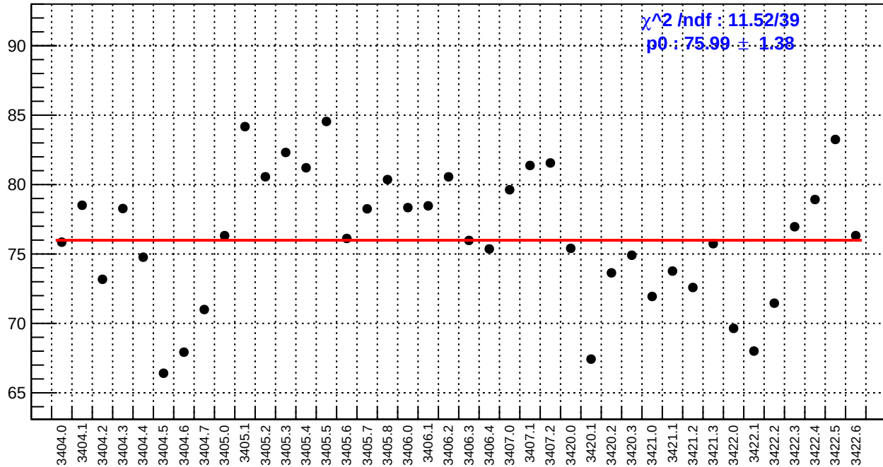
slug4: usr_bpm4aX/(ppb/nm)
