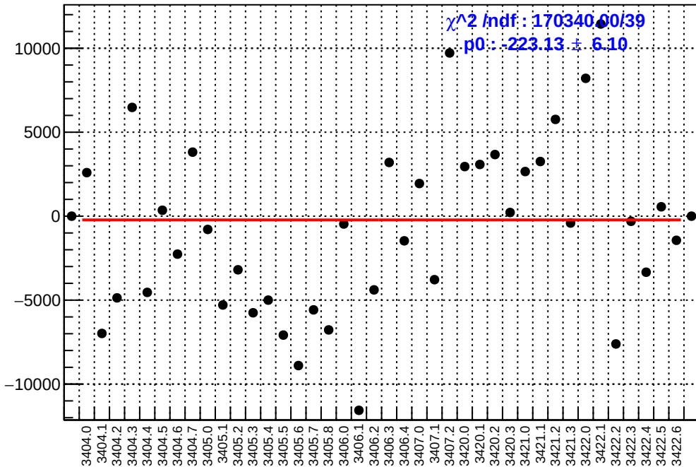
slug4: asym_usl.mean/ppb-reg_asym_usl.mean/ppb
