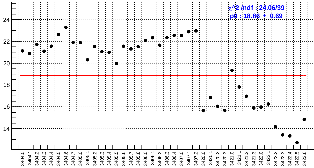
slug4: dsr_bpm4eX/(ppb/nm)
