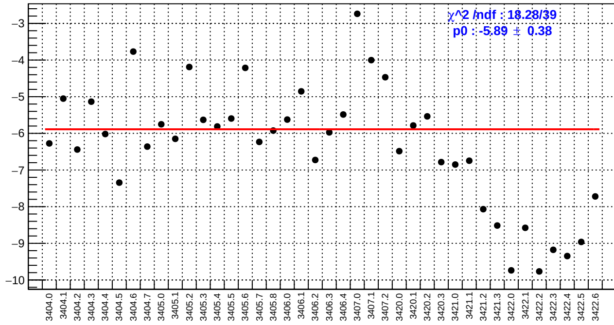
slug4: us_avg_bpm4aY/(ppb/nm)
