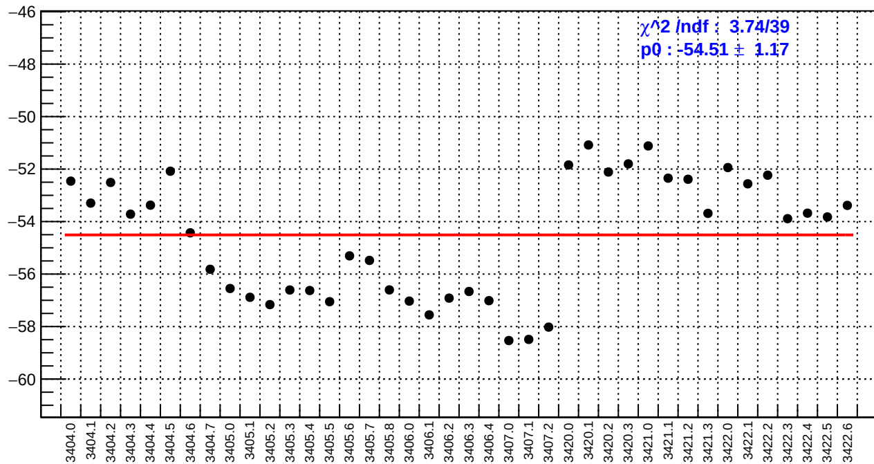
slug4: ds_avg_bpm12X/(ppb/nm)
