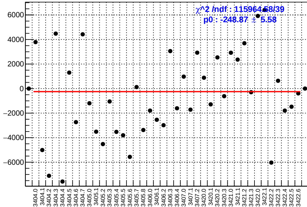
slug4: asym_ds_dd.mean/ppb-reg_asym_ds_dd.mean/ppb
