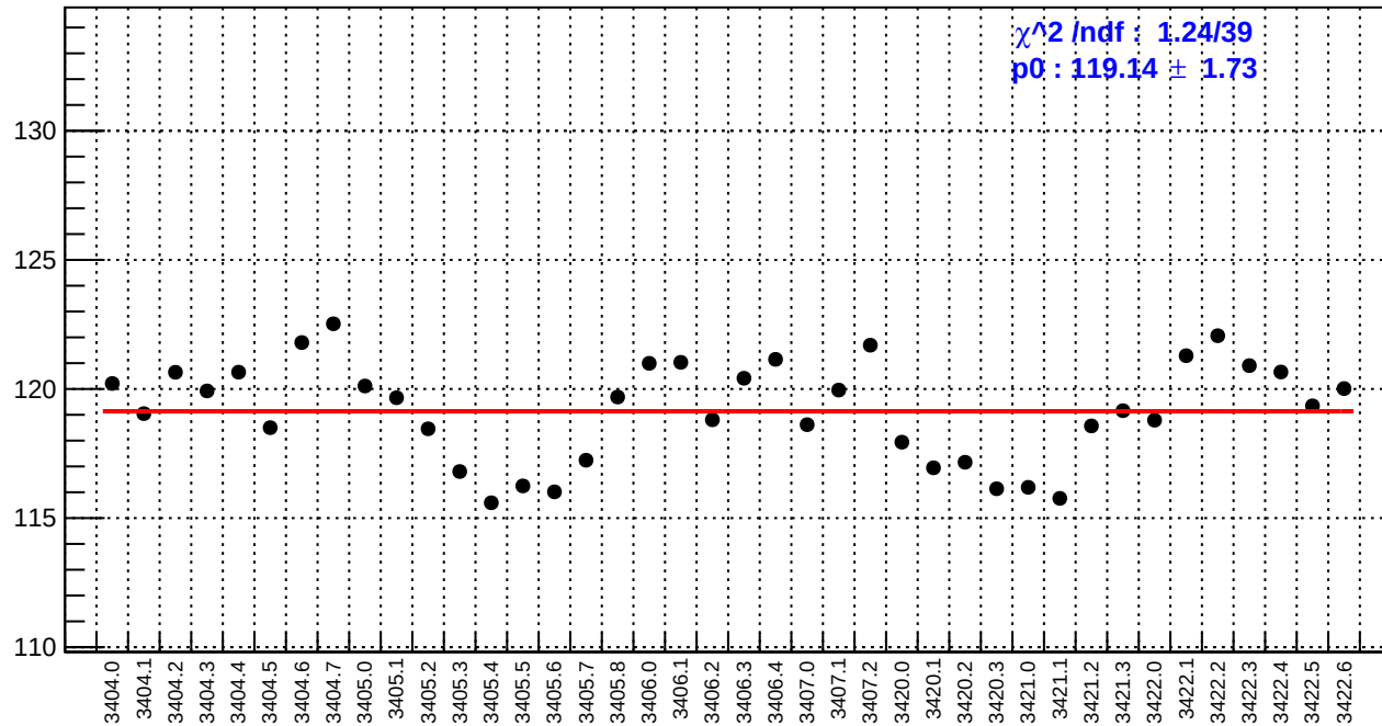
slug4: reg_asym_us_avg.rms/ppm
