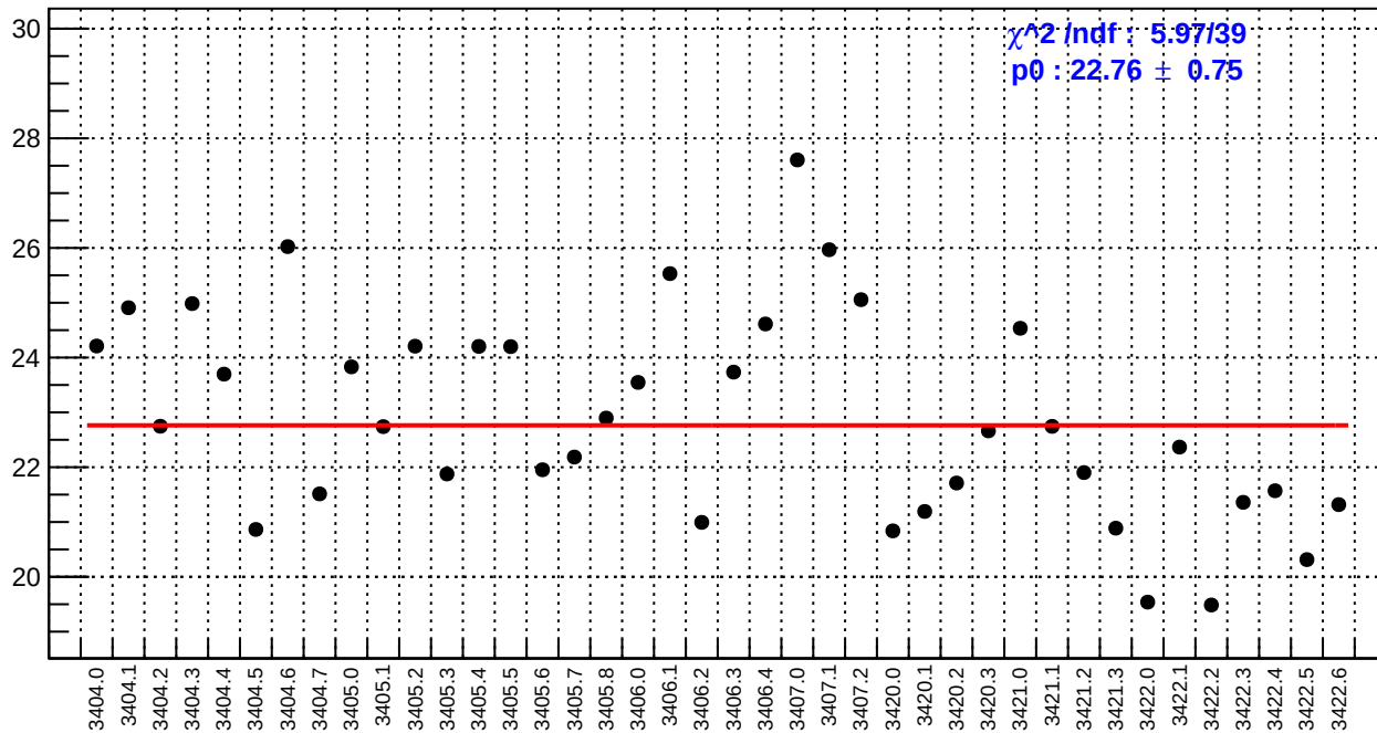
slug4: right_avg_bpm4aY/(ppb/nm)
