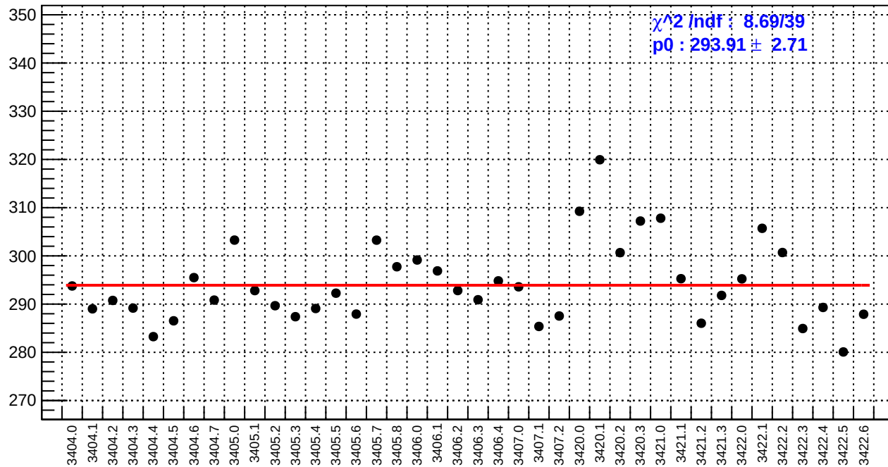
slug4: reg_asym_sam1.rms/ppm
