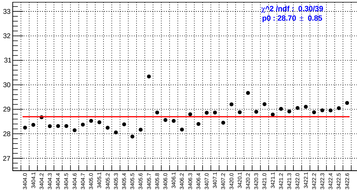
slug4: reg_asym_left_dd.rms/ppm
