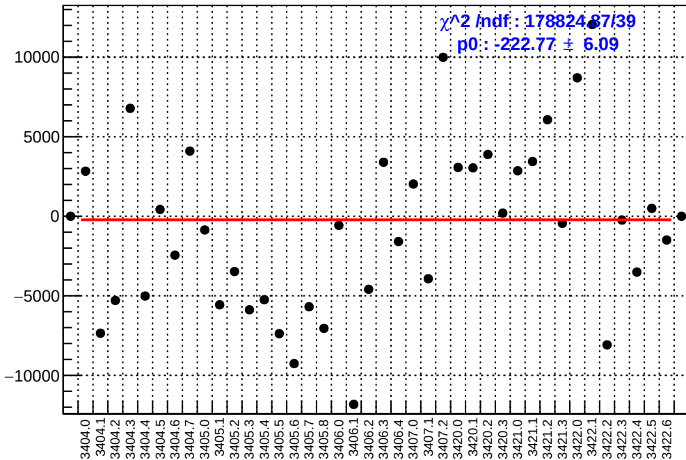
slug4: asym_left_avg.mean/ppb-reg_asym_left_avg.mean/ppb
