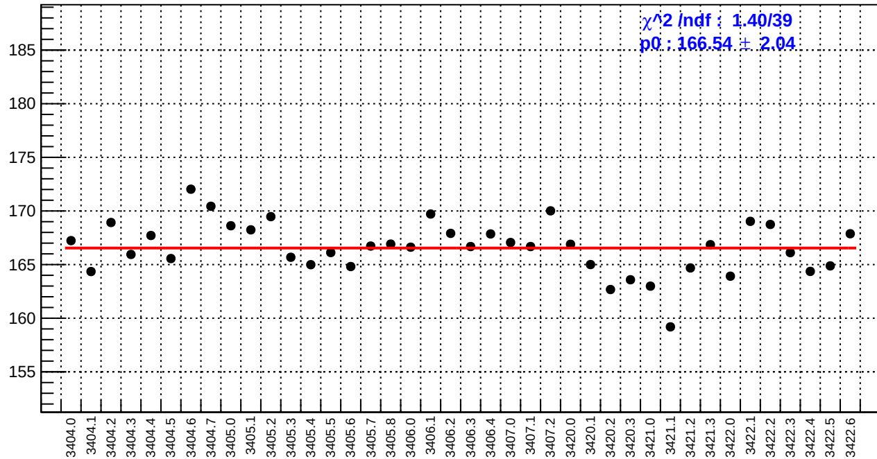
slug4: reg_asym_dsr.rms/ppm
