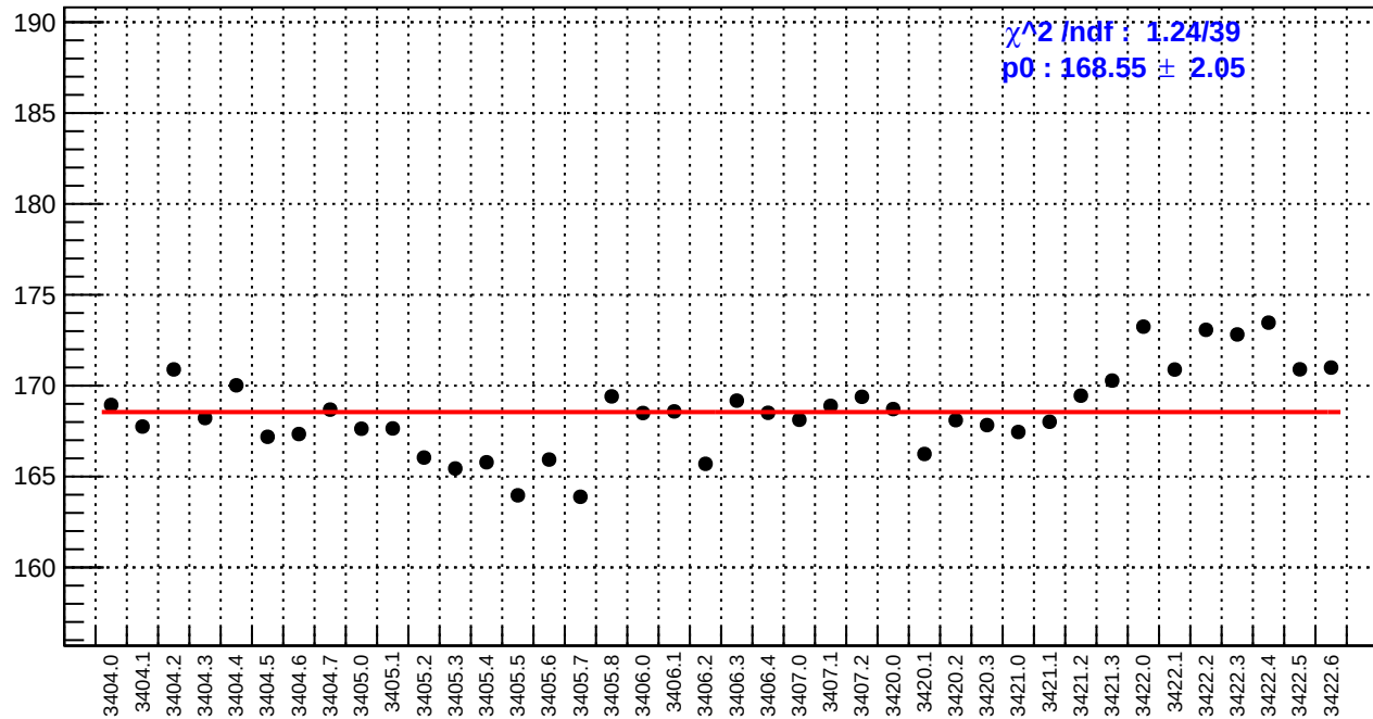
slug4: reg_asym_left_avg.rms/ppm
