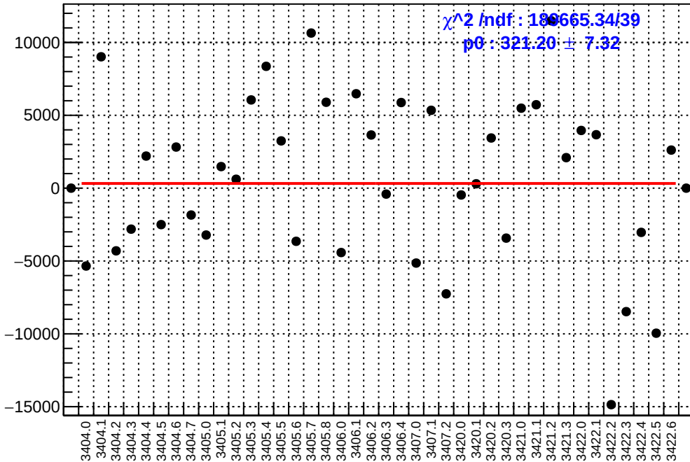
slug4: asym_sam5.mean/ppb-reg_asym_sam5.mean/ppb
