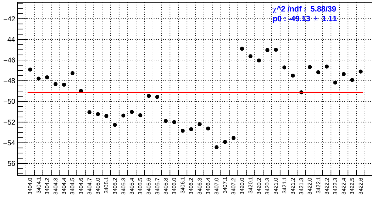
slug4: dsl_bpm12X/(ppb/nm)
