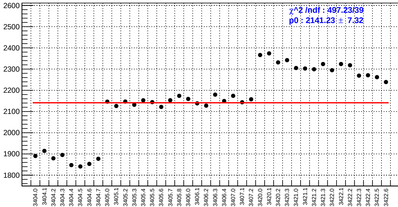
slug4: reg_asym_sam2.rms/ppm
