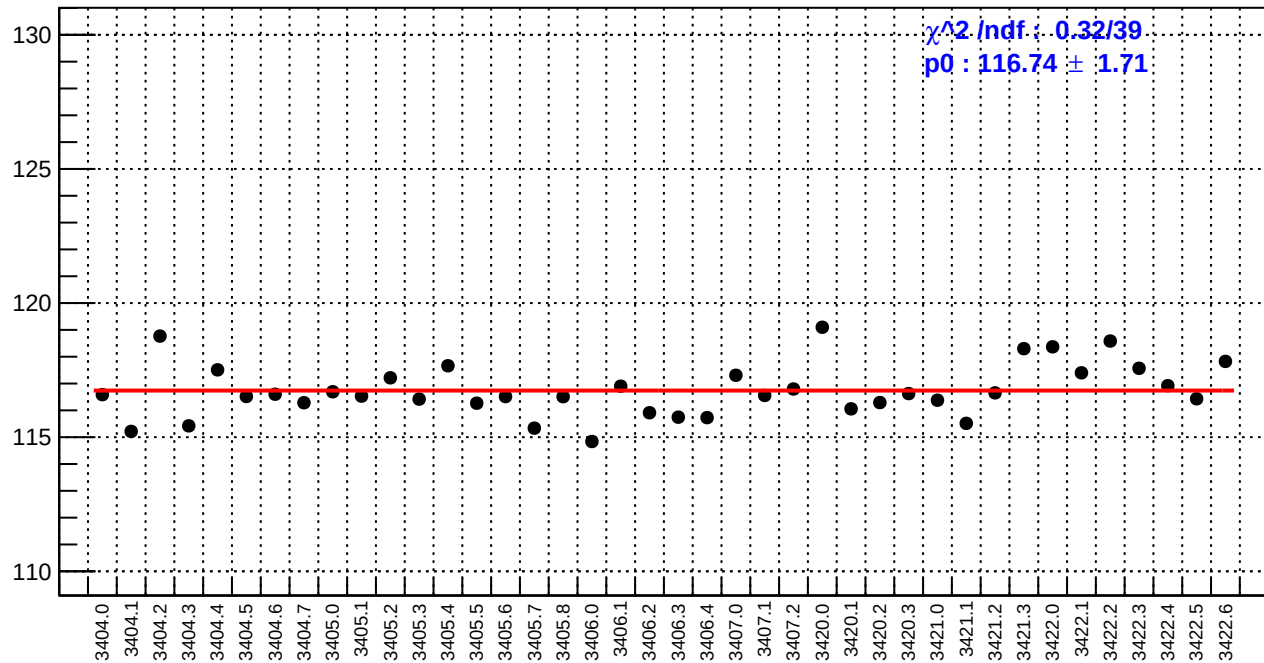
slug4: reg_asym_ds_dd.rms/ppm
