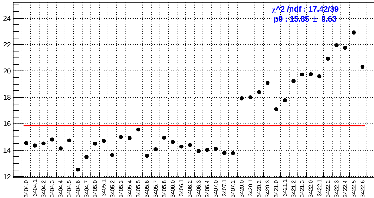
slug4: us_avg_bpm4eY/(ppb/nm)
