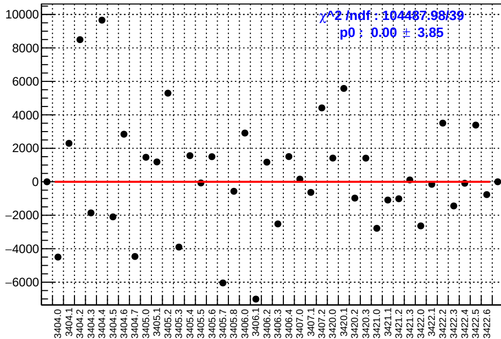
slug4: asym_dsr.mean/ppb-reg_asym_dsr.mean/ppb
