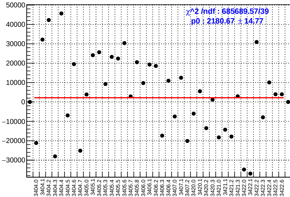
slug4: asym_sam7.mean/ppb-reg_asym_sam7.mean/ppb
