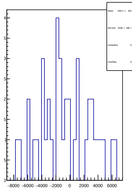
slug4: 1D Corr asym_us_dd.mean/ppb-reg_asym_us_dd.mean/ppb
