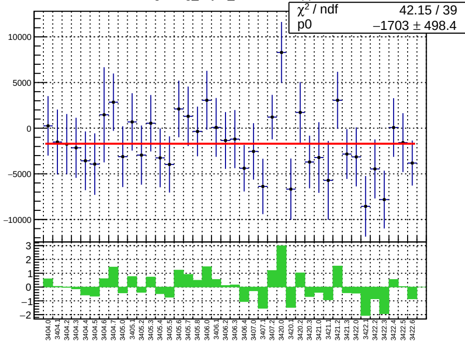
slug4: reg_asym_sam7.mean/ppb
