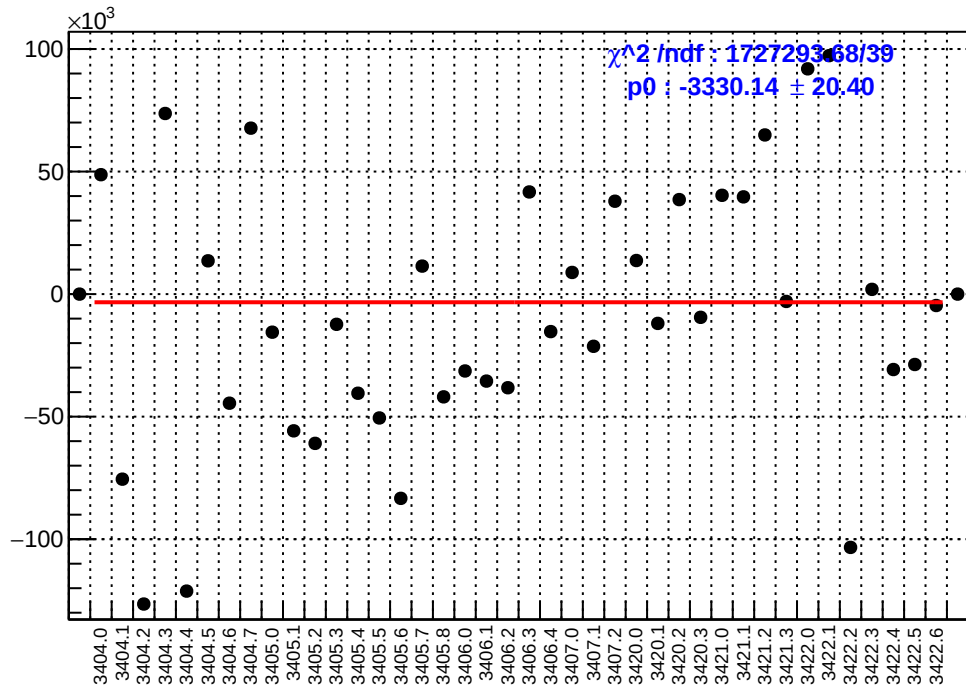
slug4: asym_sam4.mean/ppb-reg_asym_sam4.mean/ppb
