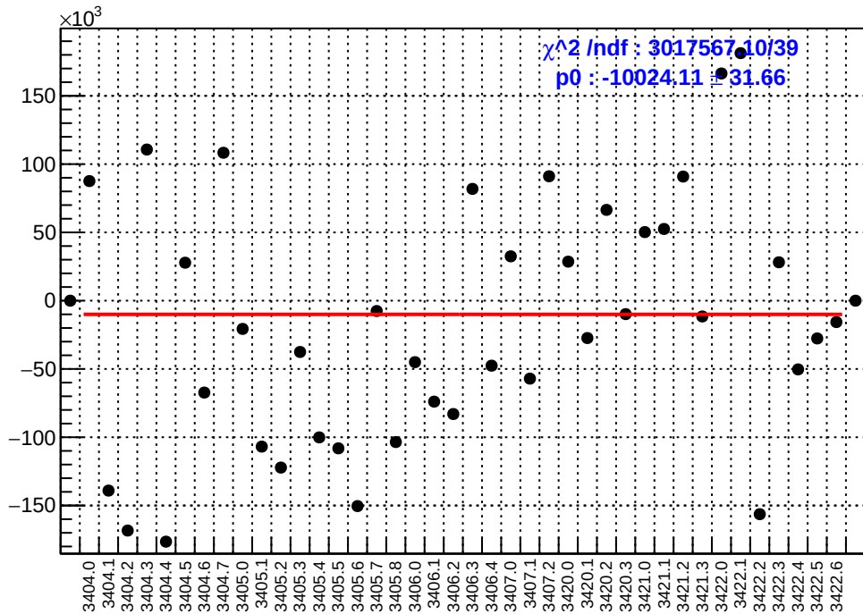
slug4: asym_sam3.mean/ppb-reg_asym_sam3.mean/ppb
