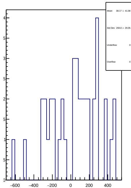
slug4: 1D Corr asym_left_dd.mean/ppb-reg_asym_left_dd.mean/ppb
