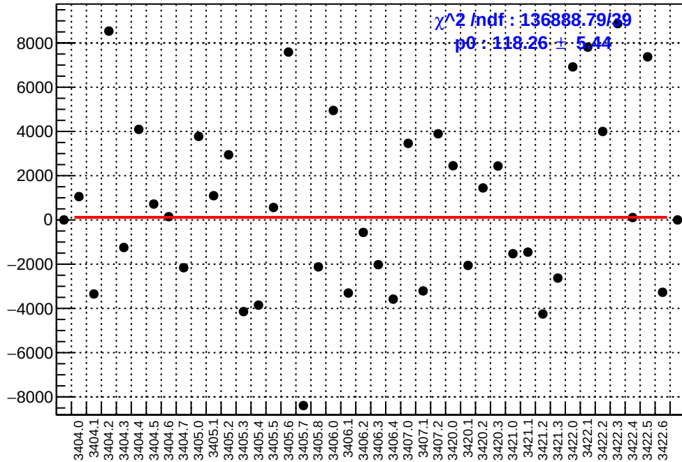
slug4: asym_sam1.mean/ppb-reg_asym_sam1.mean/ppb
