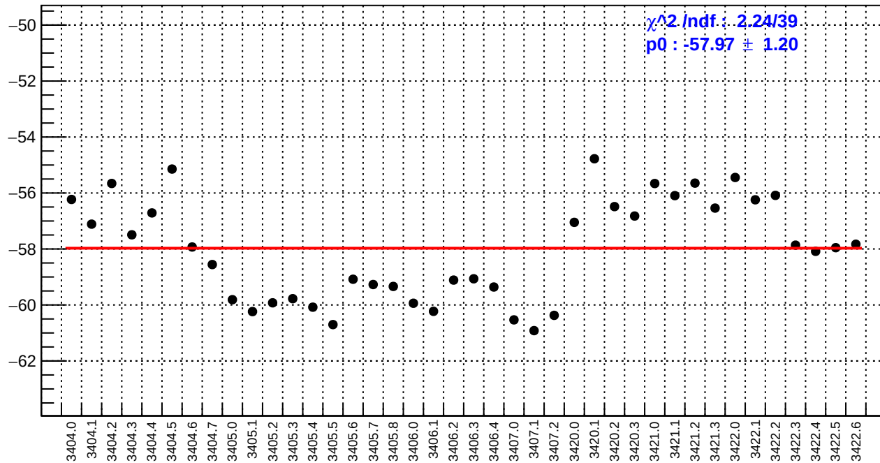
slug4: right_avg_bpm12X/(ppb/nm)
