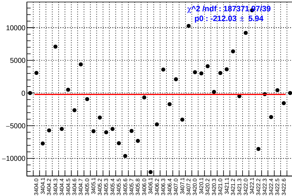
slug4: asym_dsl.mean/ppb-reg_asym_dsl.mean/ppb
