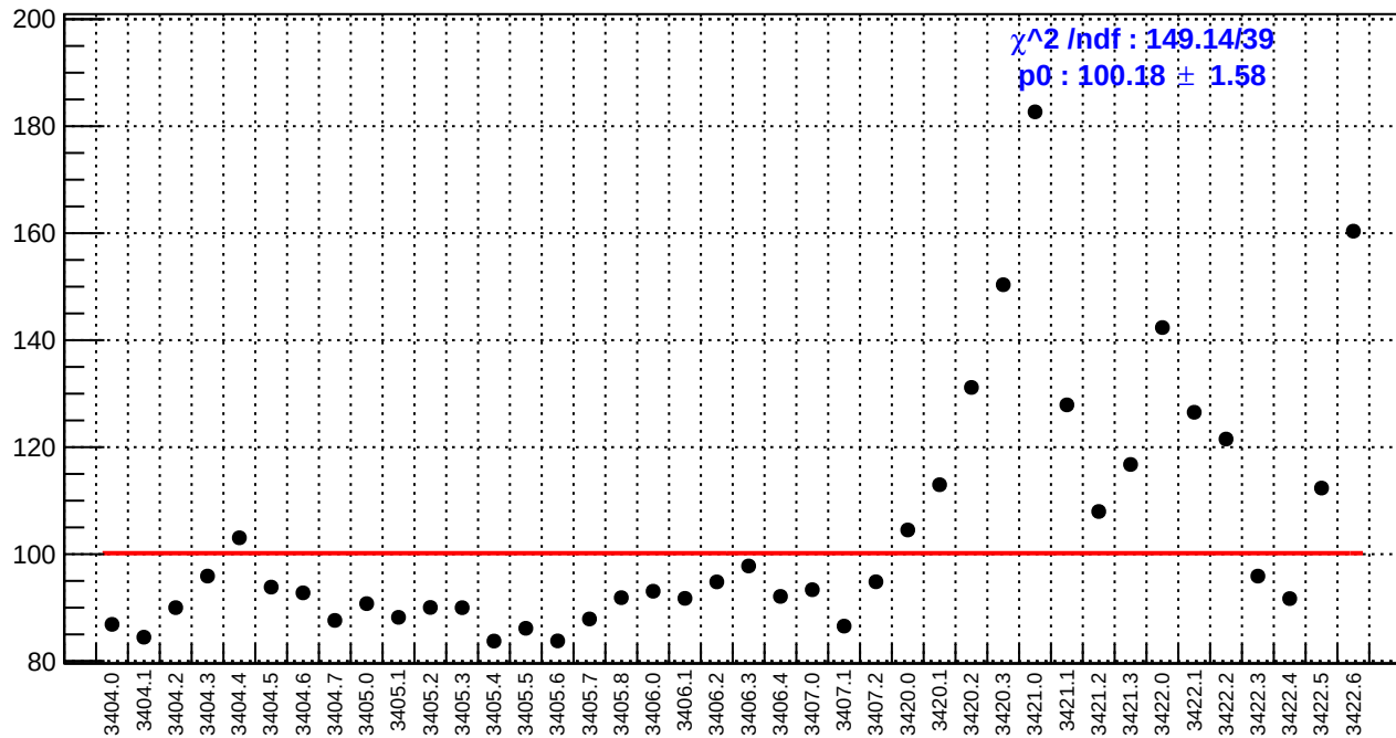
slug4: asym_bcm_an_ds3.rms/ppm
