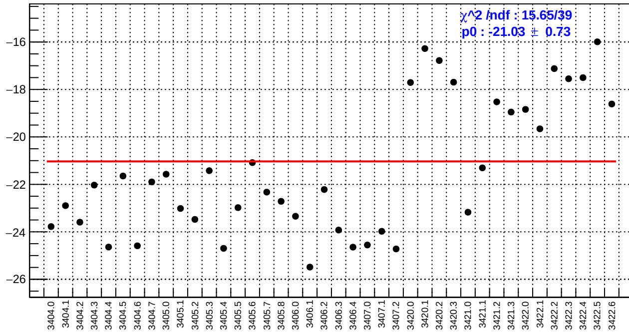
slug4: right_avg_bpm4eY/(ppb/nm)
