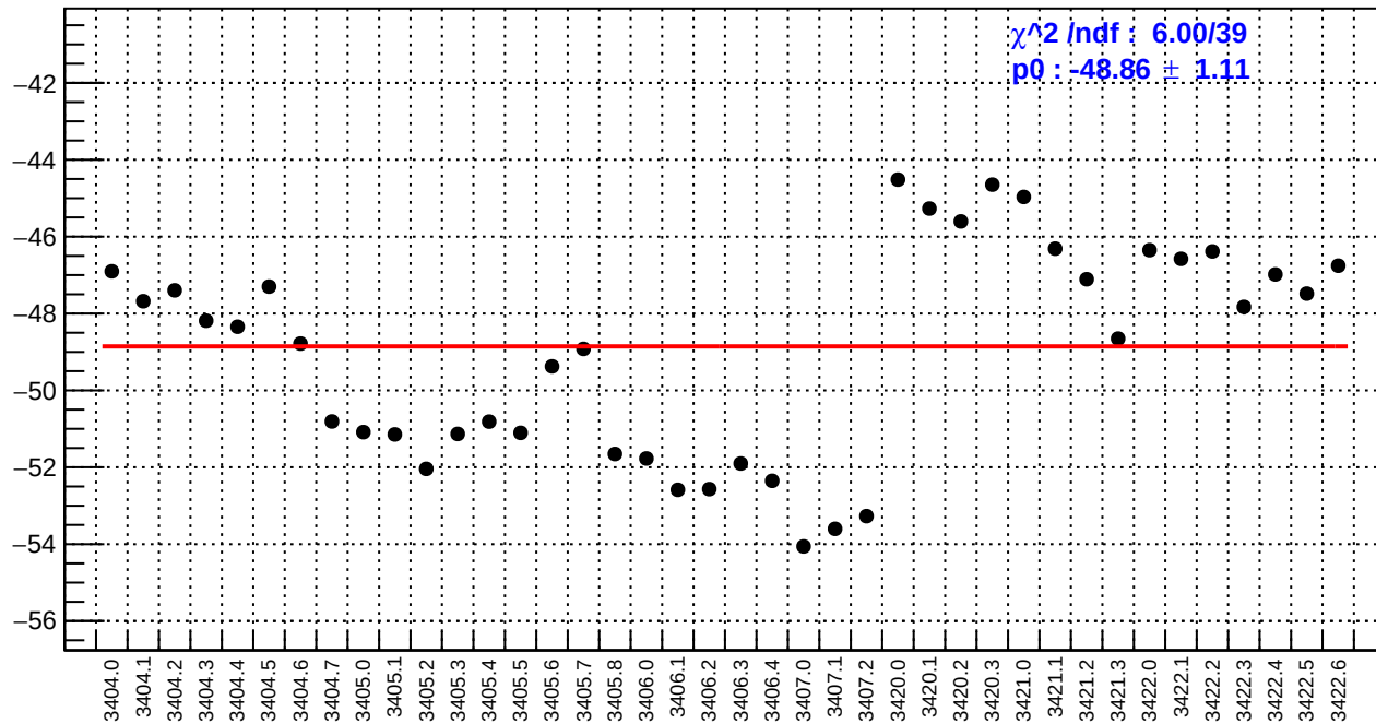
slug4: left_avg_bpm12X/(ppb/nm)
