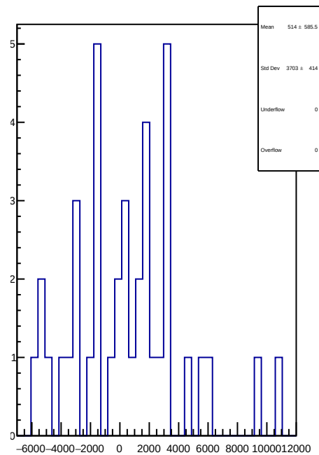
slug4: 1D Corr asym_usr.mean/ppb-reg_asym_usr.mean/ppb
