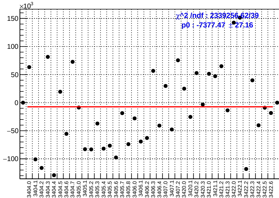
slug4: asym_sam2.mean/ppb-reg_asym_sam2.mean/ppb
