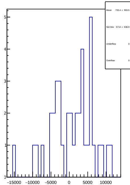
slug4: 1D Corr asym_sam5.mean/ppb-reg_asym_sam5.mean/ppb
