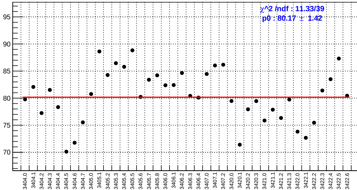
slug4: right_avg_bpm4aX/(ppb/nm)
