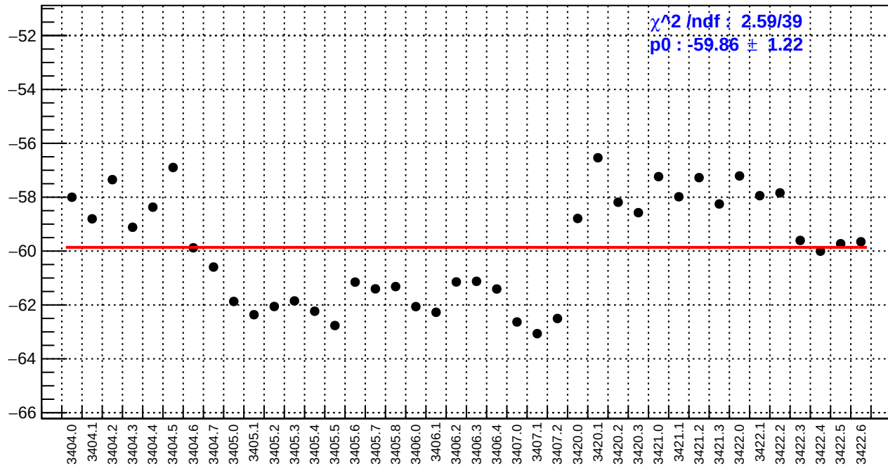
slug4: dsr_bpm12X/(ppb/nm)
