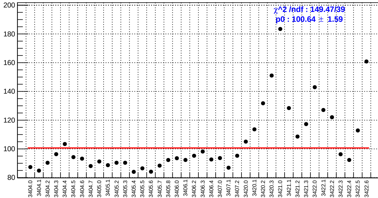
slug4: asym_bcm_an_ds.rms/ppm
