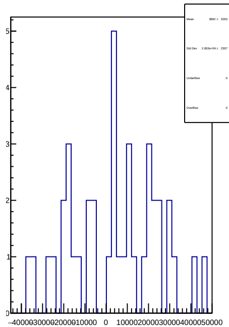
slug4: 1D Corr asym_sam7.mean/ppb-reg_asym_sam7.mean/ppb
