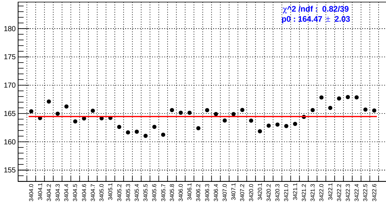
slug4: reg_asym_usl.rms/ppm
