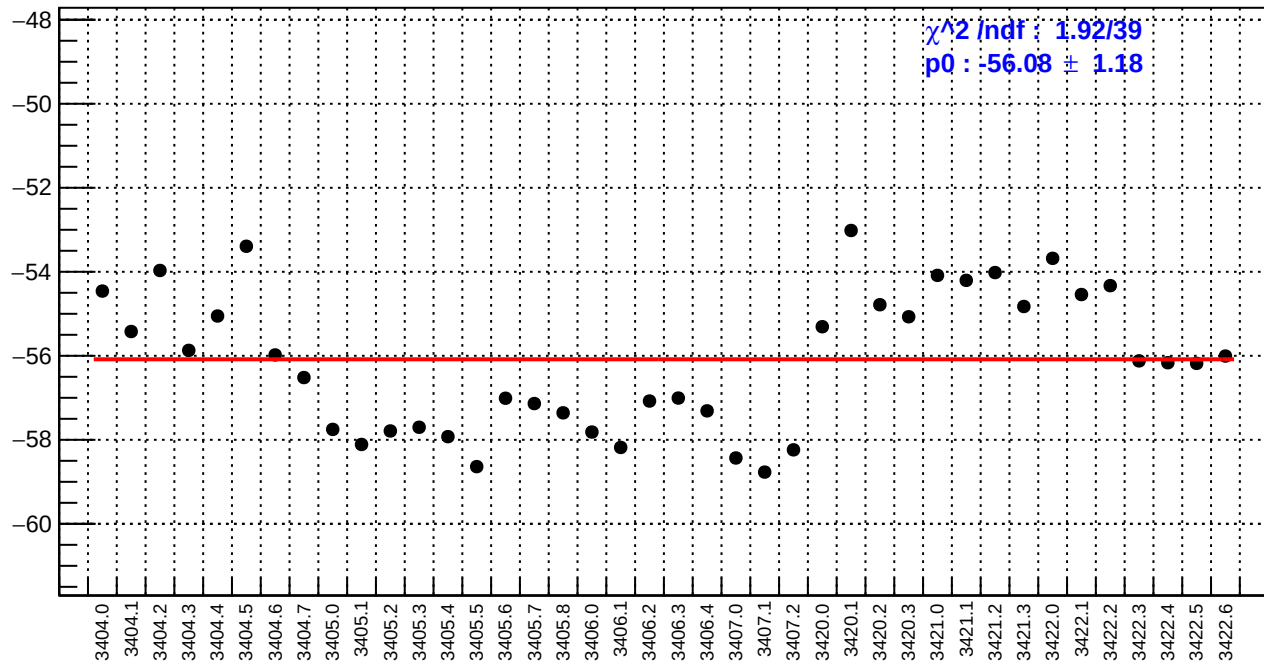
slug4: usr_bpm12X/(ppb/nm)
