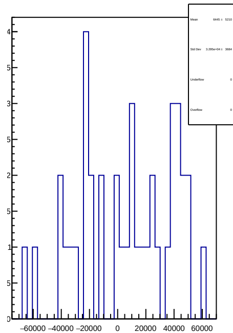
slug4: 1D Corr asym_sam6.mean/ppb-reg_asym_sam6.mean/ppb
