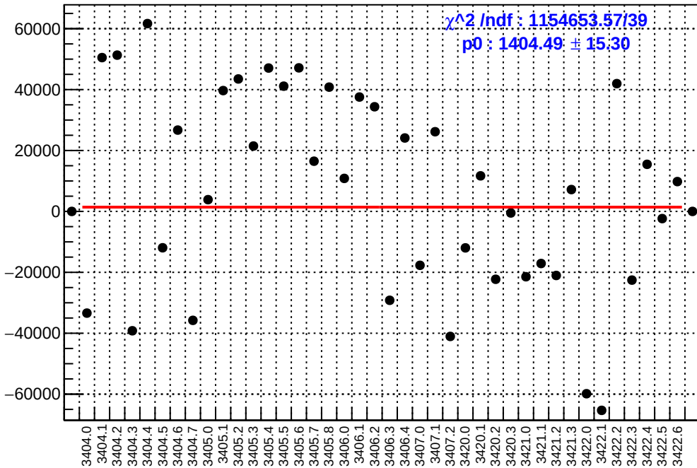
slug4: asym_sam6.mean/ppb-reg_asym_sam6.mean/ppb
