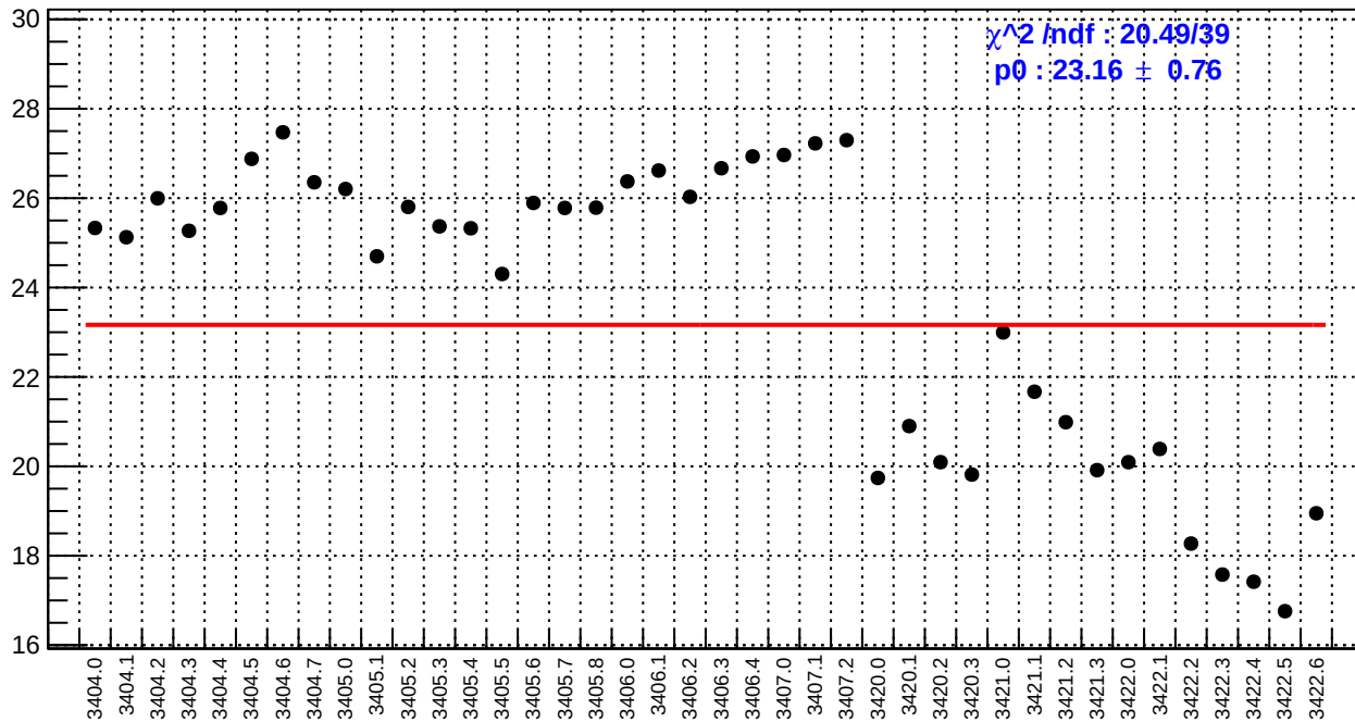
slug4: right_avg_bpm4eX/(ppb/nm)
