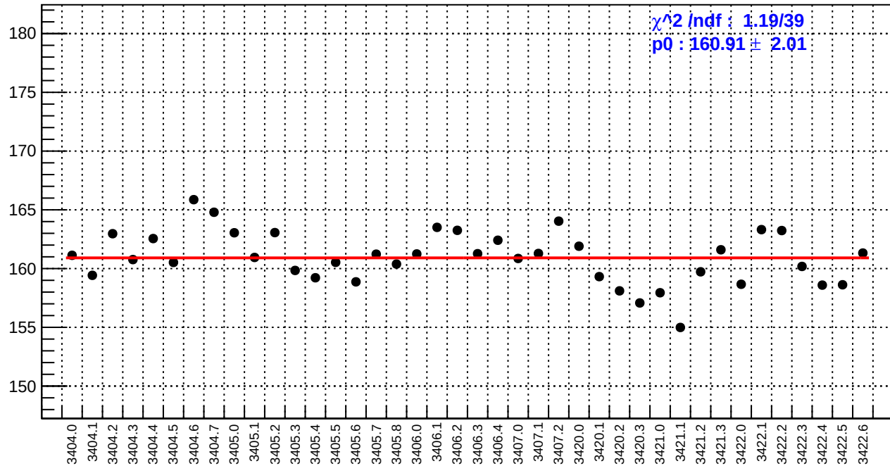
slug4: reg_asym_usr.rms/ppm
