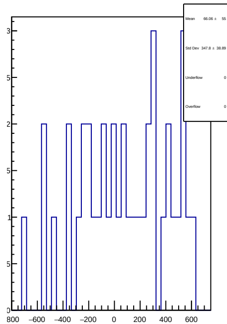
slug4: 1D Corr asym_right_dd.mean/ppb-reg_asym_right_dd.mean/ppb
