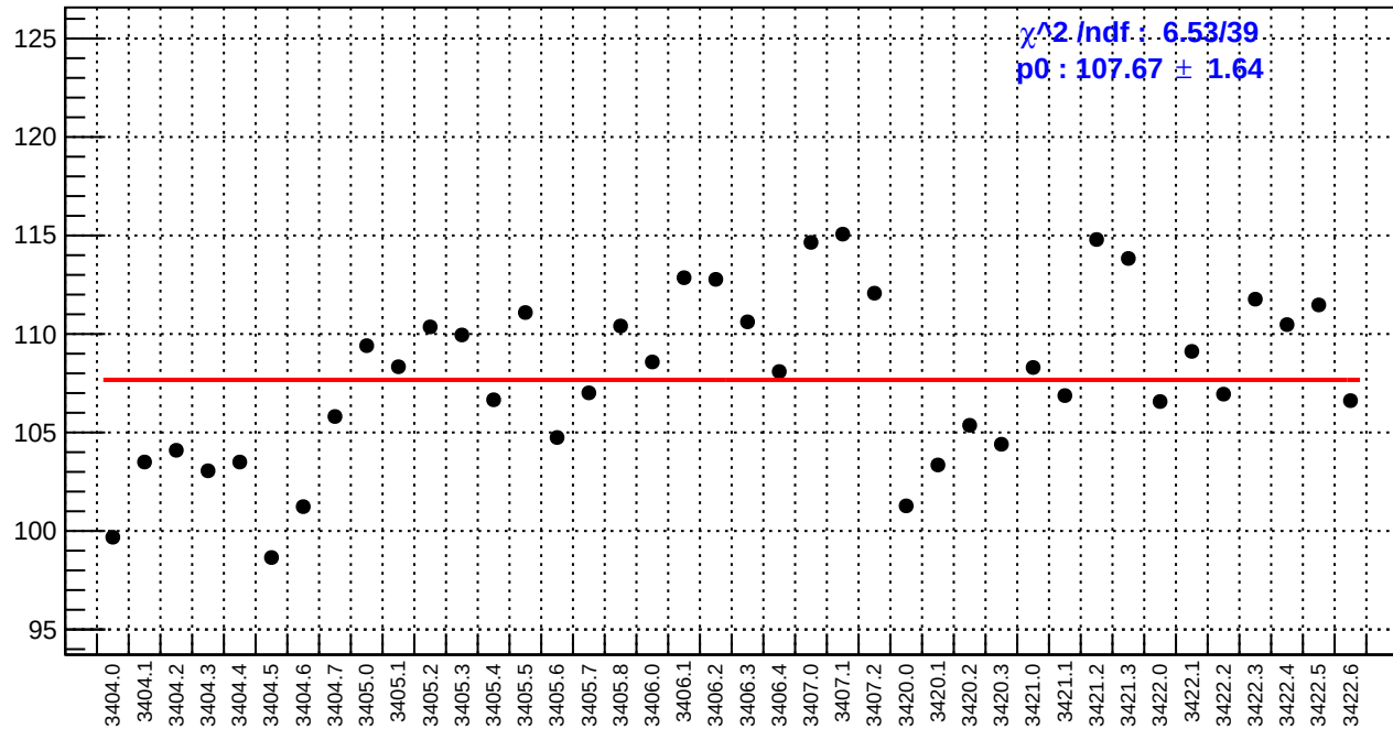
slug4: left_avg_bpm4aX/(ppb/nm)
