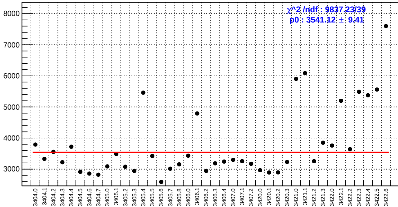
slug4: diff_bpm4eY.rms/nm
