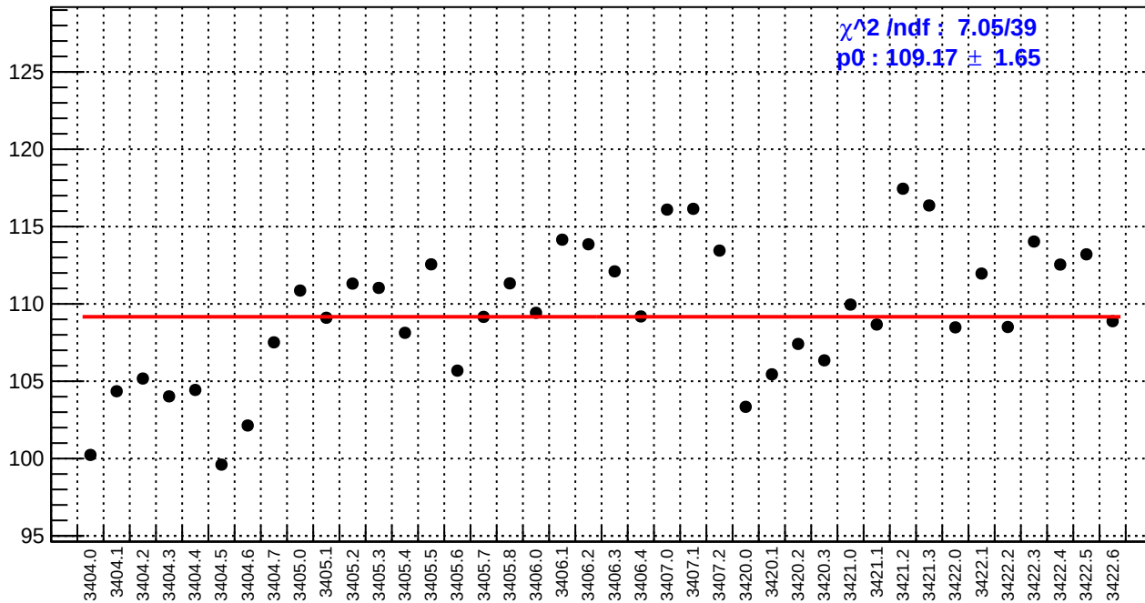
slug4: dsl_bpm4aX/(ppb/nm)
