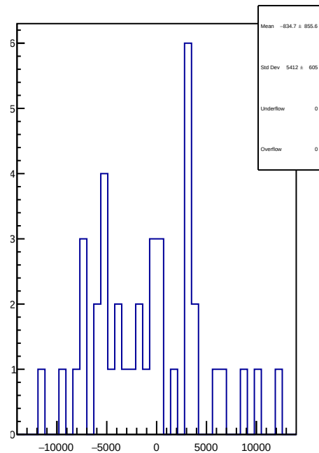
slug4: 1D Corr asym_left_avg.mean/ppb-reg_asym_left_avg.mean/ppb
