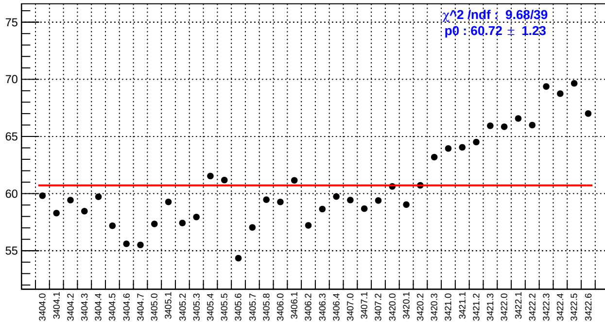
slug4: left_avg_bpm4eY/(ppb/nm)
