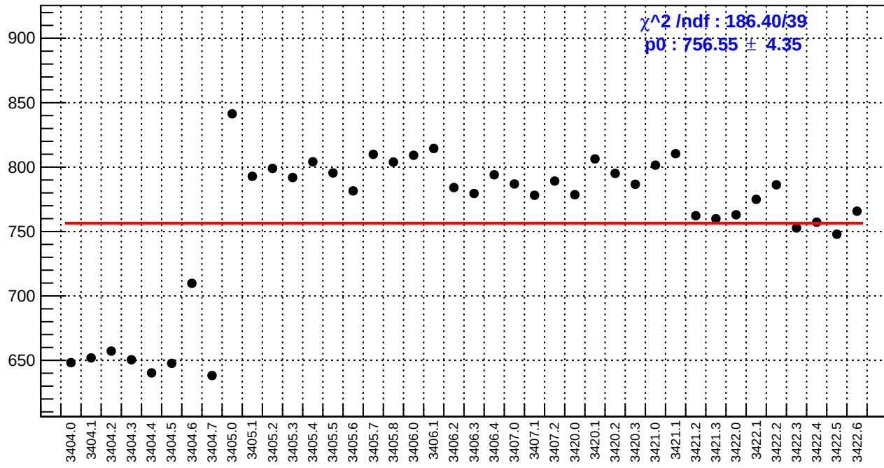
slug4: reg_asym_sam6.rms/ppm
