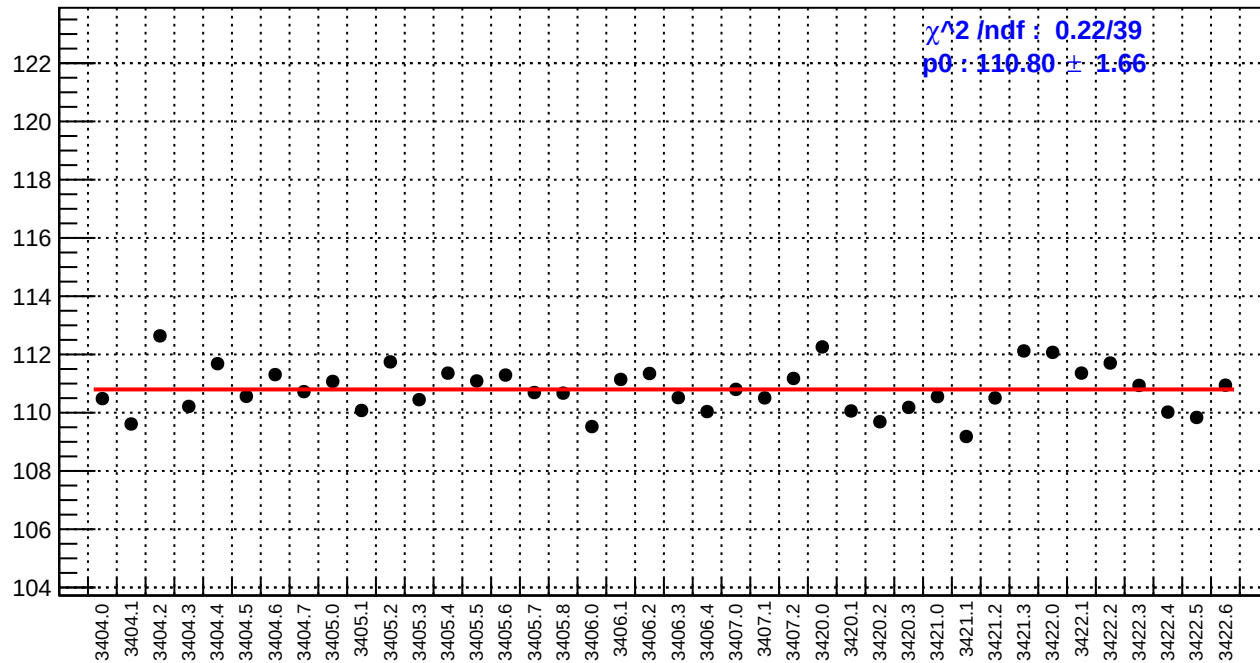
slug4: reg_asym_us_dd.rms/ppm
