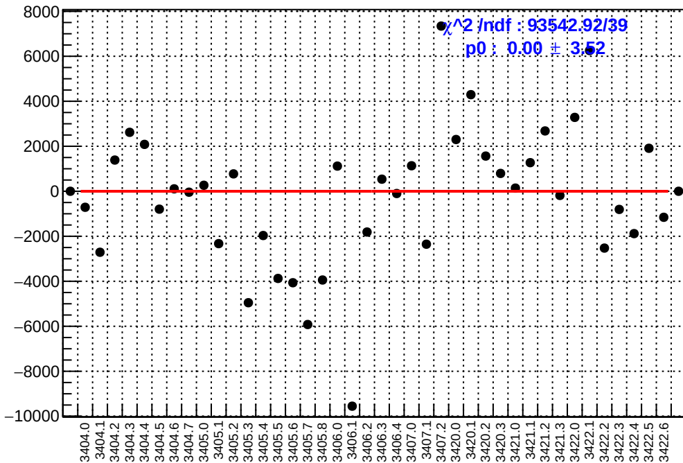
slug4: asym_ds_avg.mean/ppb-reg_asym_ds_avg.mean/ppb
