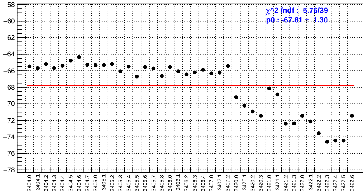
slug4: dsl_bpm4eX/(ppb/nm)
