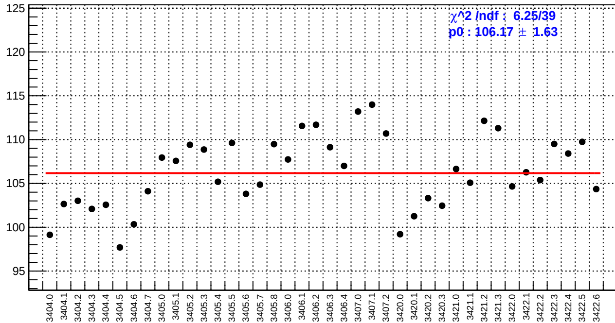
slug4: usl_bpm4aX/(ppb/nm)
