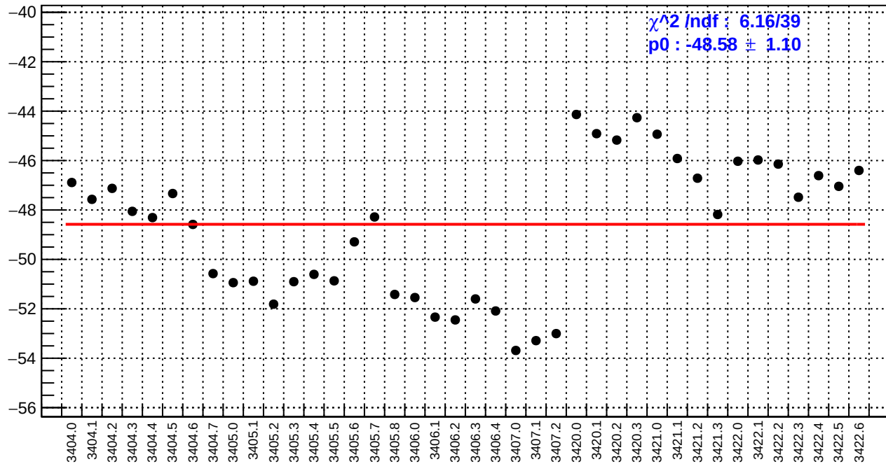
slug4: usl_bpm12X/(ppb/nm)
