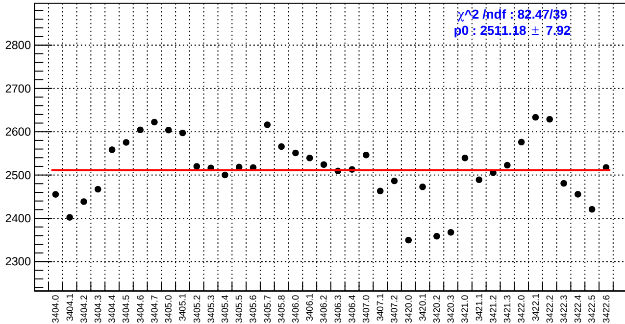
slug4: diff_bpm4aY.rms/nm
