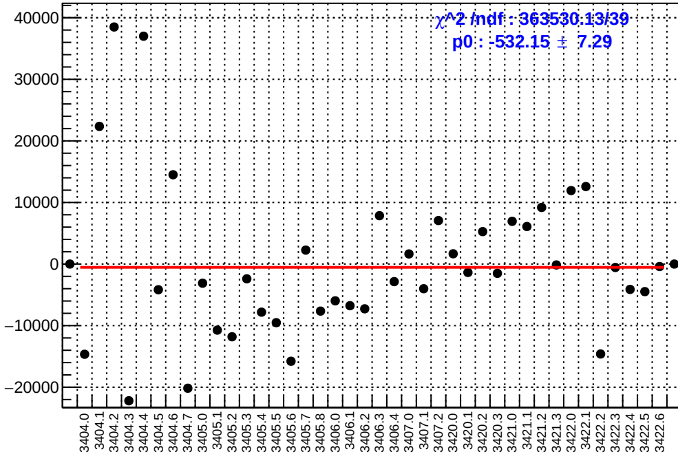
slug4: asym_sam8.mean/ppb-reg_asym_sam8.mean/ppb
