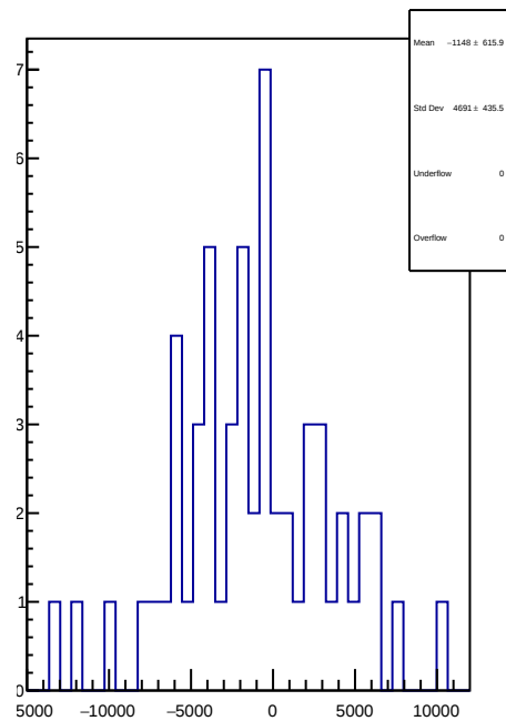
slug41: 1D Corr asym_usr.mean/ppb-reg_asym_usr.mean/ppb
