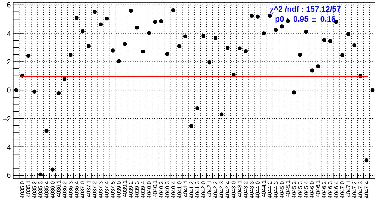
slug41: us_avg_bpm4eY/(ppb/nm)
