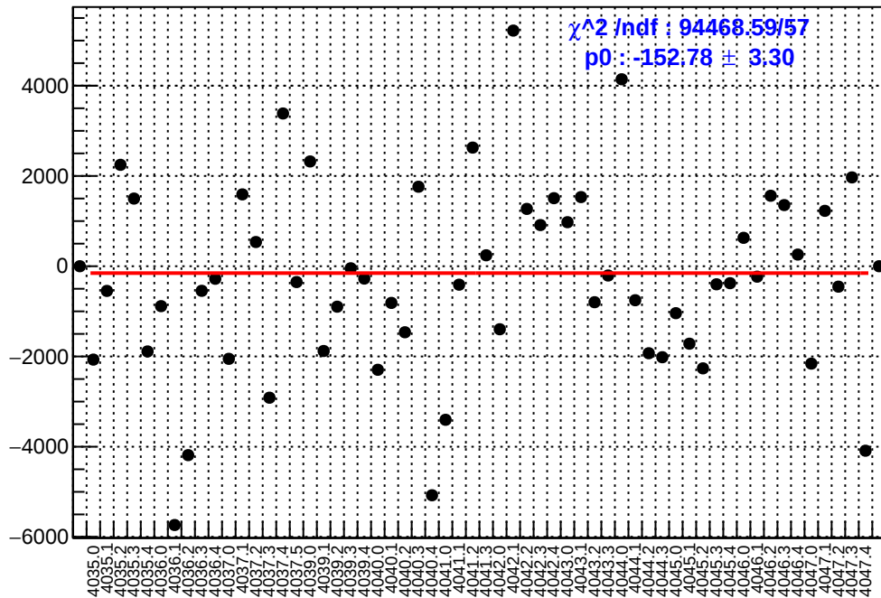
slug41: asym_us_avg.mean/ppb-reg_asym_us_avg.mean/ppb
