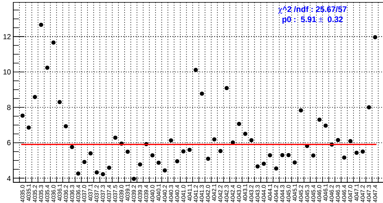
slug41: ds_avg_bpm4aY/(ppb/nm)
