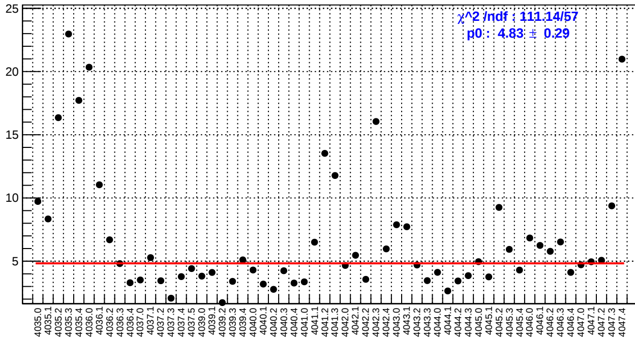
slug41: dsl_bpm4aY/(ppb/nm)
