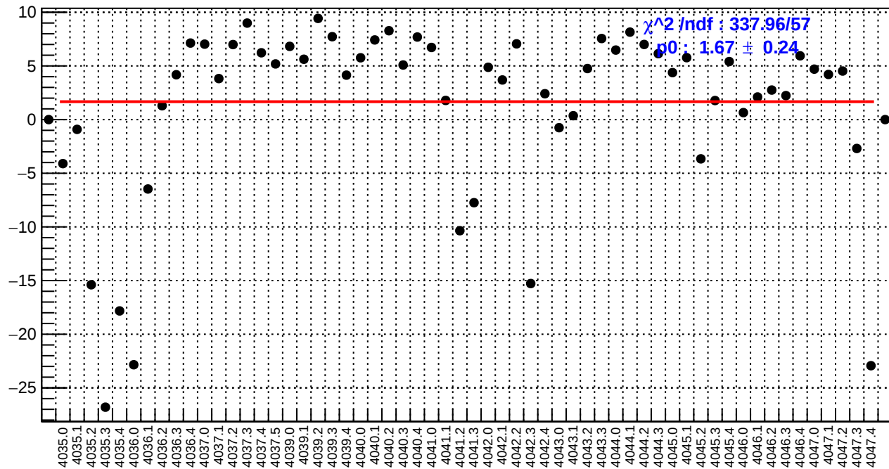
slug41: dsl_bpm4eY/(ppb/nm)
