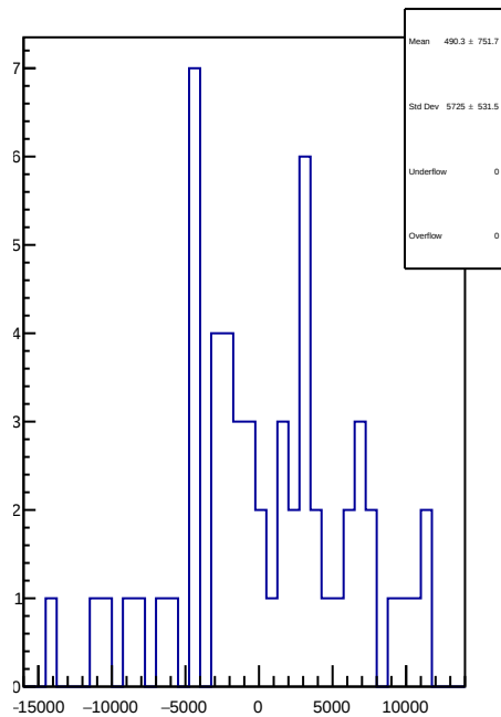
slug41: 1D Corr asym_usl.mean/ppb-reg_asym_usl.mean/ppb
