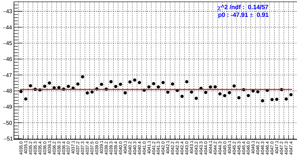
slug41: us_avg_bpm12X/(ppb/nm)
