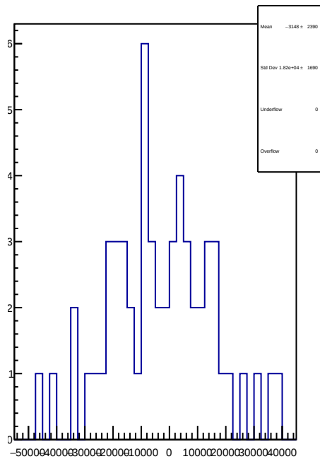
slug41: 1D Corr asym_sam7.mean/ppb-reg_asym_sam7.mean/ppb
