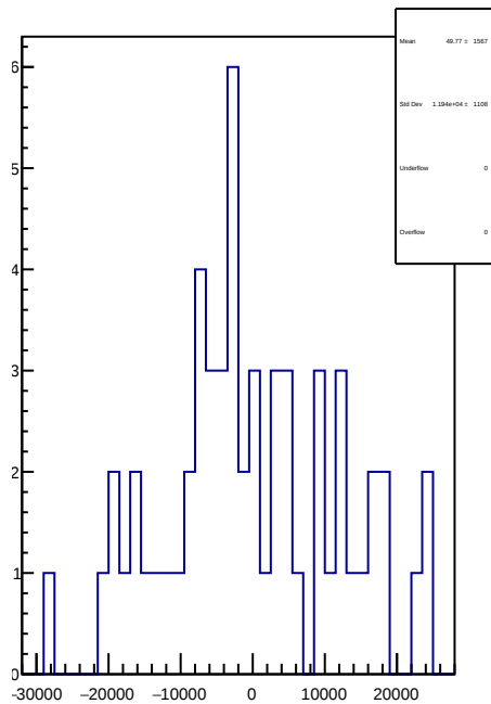
slug41: 1D Corr asym_sam5.mean/ppb-reg_asym_sam5.mean/ppb
