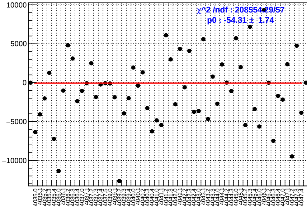
slug41: asym_right_avg.mean/ppb-reg_asym_right_avg.mean/ppb
