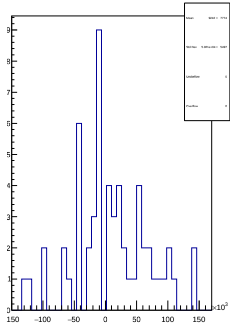
slug41: 1D Corr asym_sam4.mean/ppb-reg_asym_sam4.mean/ppb
