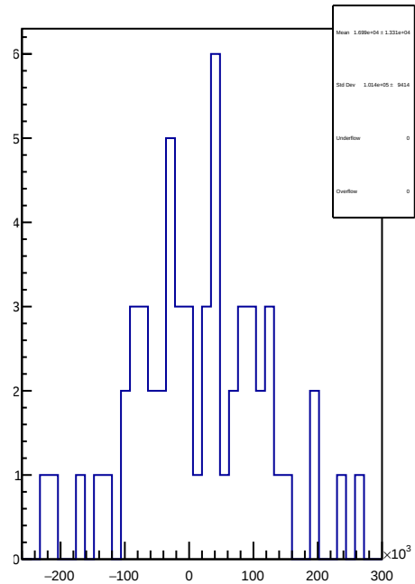
slug41: 1D Corr asym_sam3.mean/ppb-reg_asym_sam3.mean/ppb
