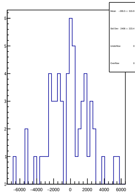
slug41: 1D Corr asym_ds_avg.mean/ppb-reg_asym_ds_avg.mean/ppb
