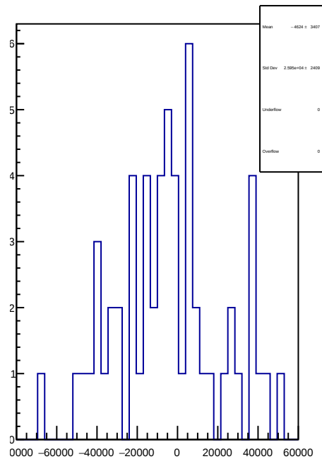
slug41: 1D Corr asym_sam6.mean/ppb-reg_asym_sam6.mean/ppb
