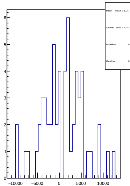
slug41: 1D Corr asym_ds_dd.mean/ppb-reg_asym_ds_dd.mean/ppb
