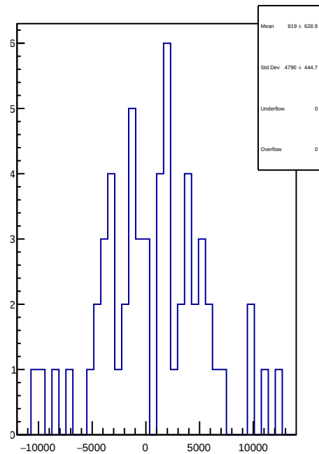
slug41: 1D Corr asym_us_dd.mean/ppb-reg_asym_us_dd.mean/ppb
