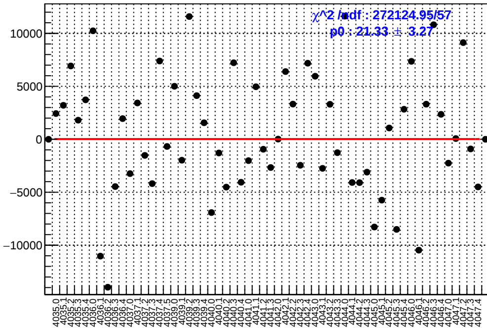
slug41: asym_usl.mean/ppb-reg_asym_usl.mean/ppb
