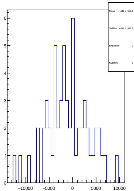
slug41: 1D Corr asym_right_avg.mean/ppb-reg_asym_right_avg.mean/ppb
