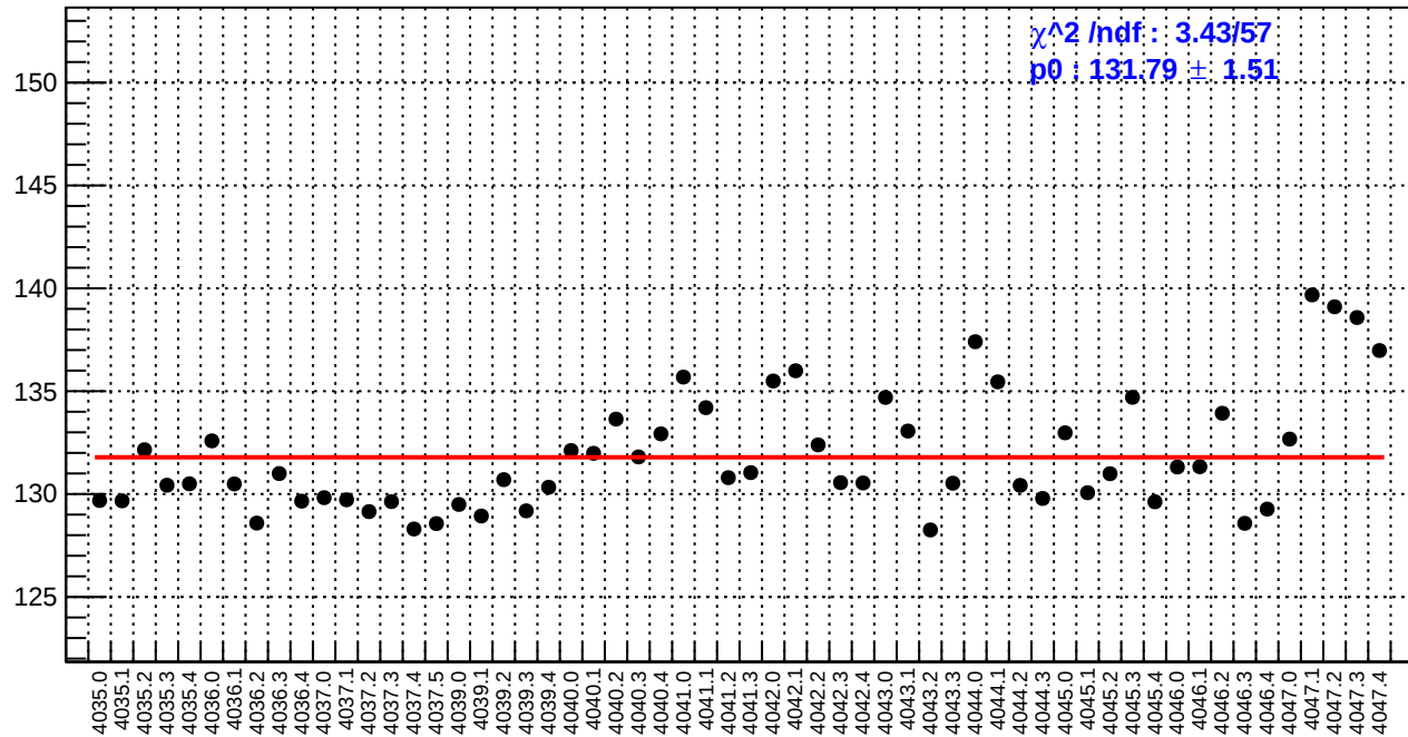
slug41: reg_asym_right_avg.rms/ppm
