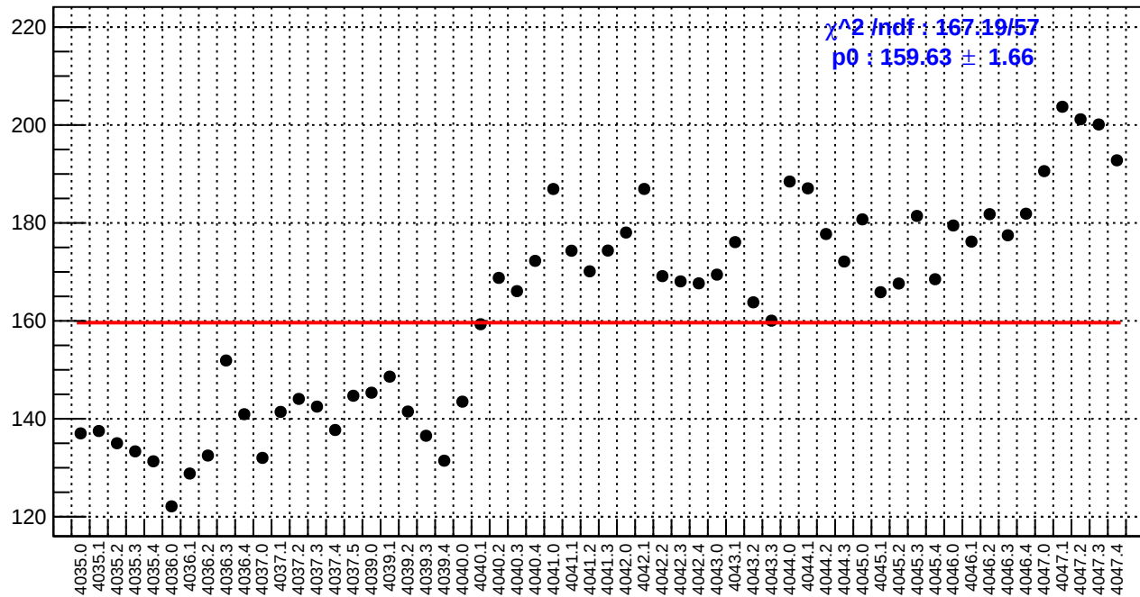
slug41: asym_bcm_an_ds.rms/ppm
