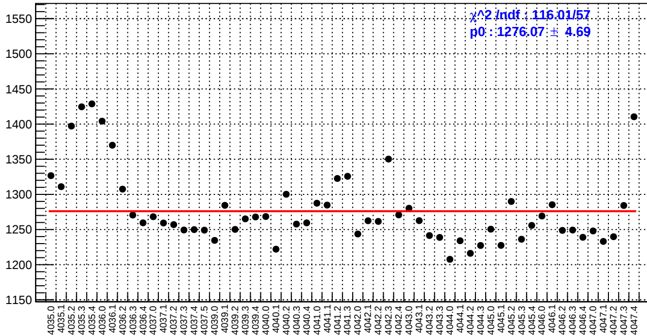
slug41: reg_asym_sam4.rms/ppm
