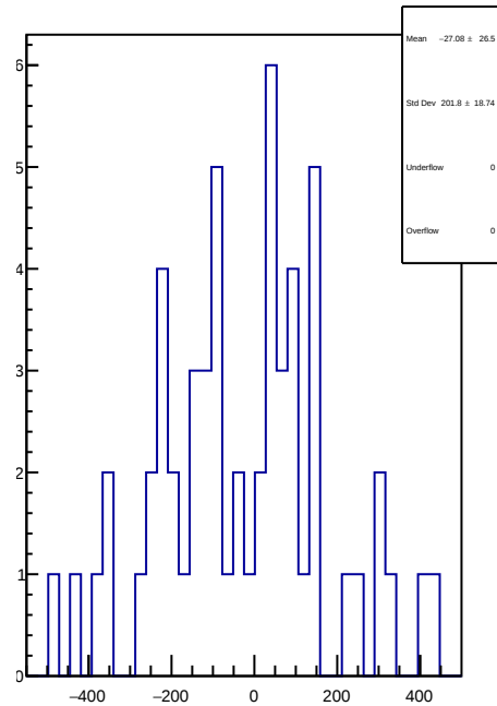
slug41: 1D Corr asym_left_dd.mean/ppb-reg_asym_left_dd.mean/ppb
