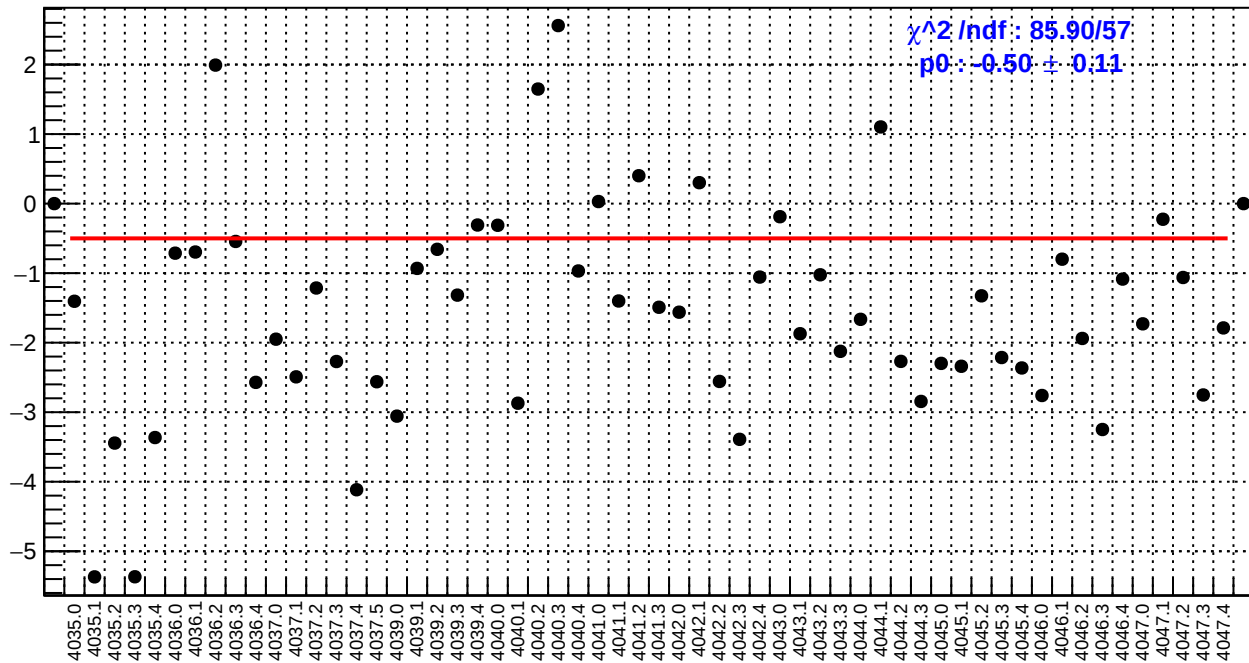
slug41: ds_avg_bpm4aX/(ppb/nm)
