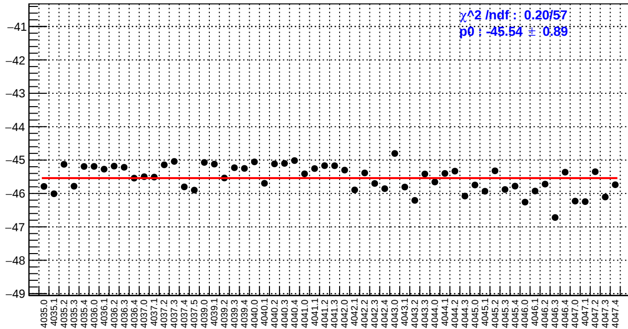
slug41: left_avg_bpm12X/(ppb/nm)
