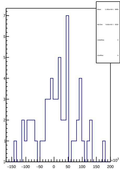
slug41: 1D Corr asym_sam2.mean/ppb-reg_asym_sam2.mean/ppb
