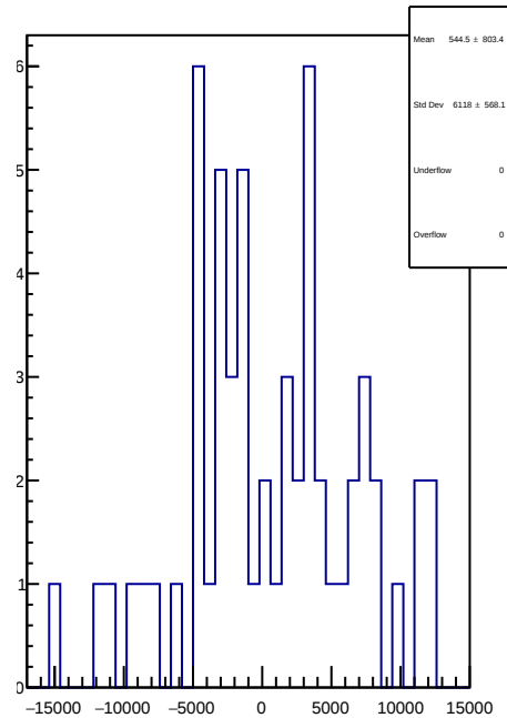
slug41: 1D Corr asym_dsl.mean/ppb-reg_asym_dsl.mean/ppb
