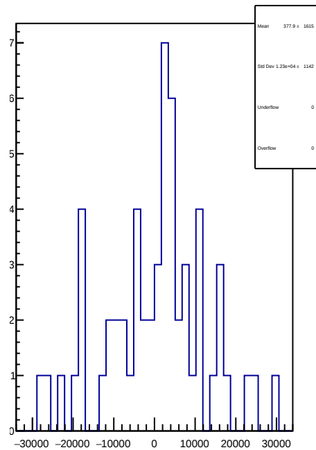
slug41: 1D Corr asym_sam1.mean/ppb-reg_asym_sam1.mean/ppb
