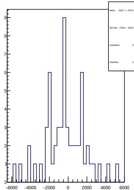
slug41: 1D Corr asym_us_avg.mean/ppb-reg_asym_us_avg.mean/ppb
