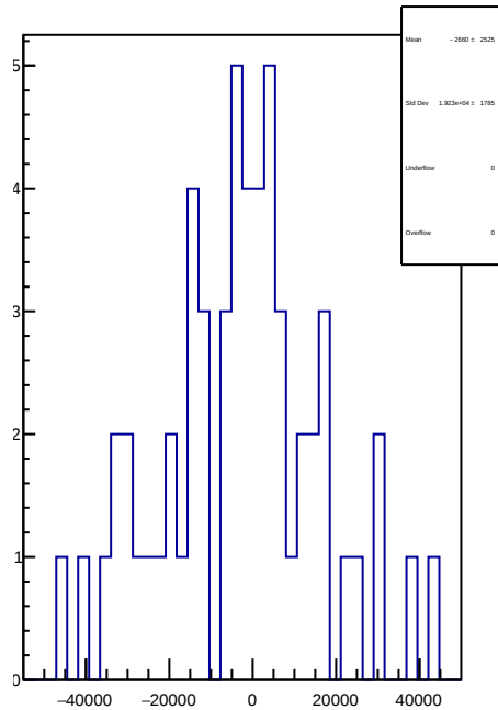
slug41: 1D Corr asym_sam8.mean/ppb-reg_asym_sam8.mean/ppb
