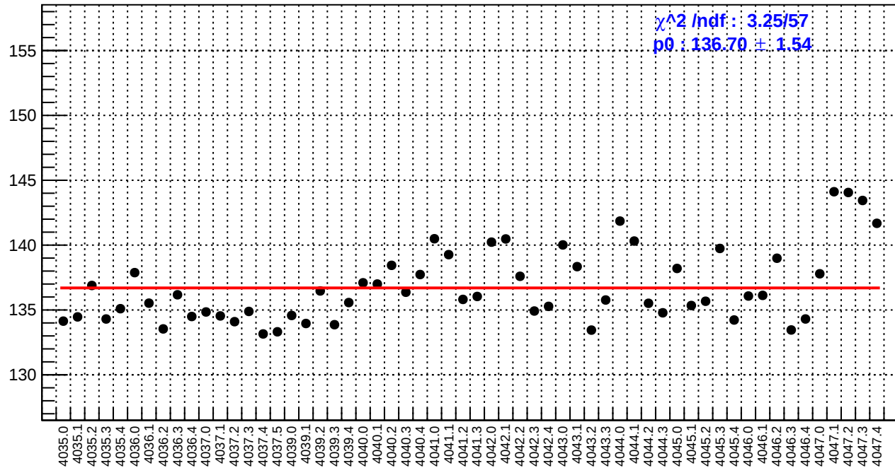
slug41: reg_asym_dsr.rms/ppm
