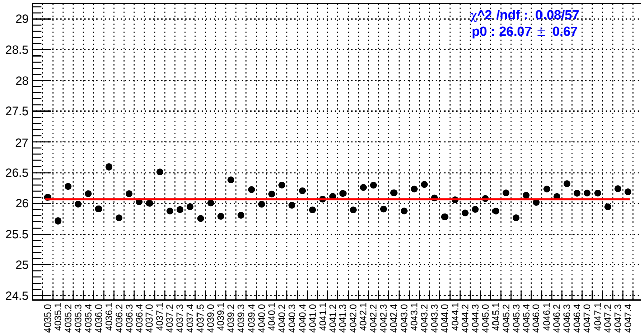
slug41: reg_asym_right_dd.rms/ppm
