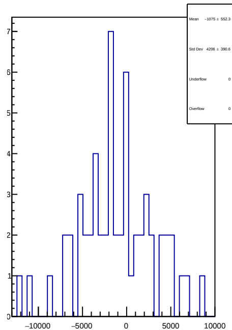
slug41: 1D Corr asym_dsr.mean/ppb-reg_asym_dsr.mean/ppb
