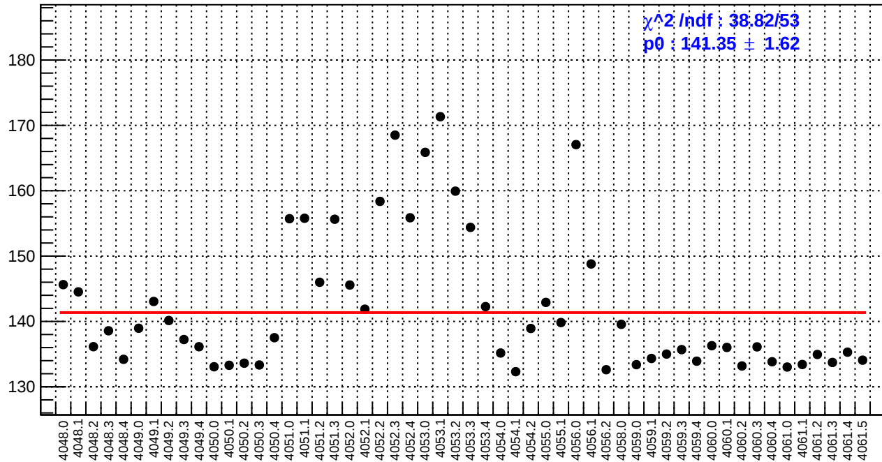
slug42: reg_asym_left_avg.rms/ppm
