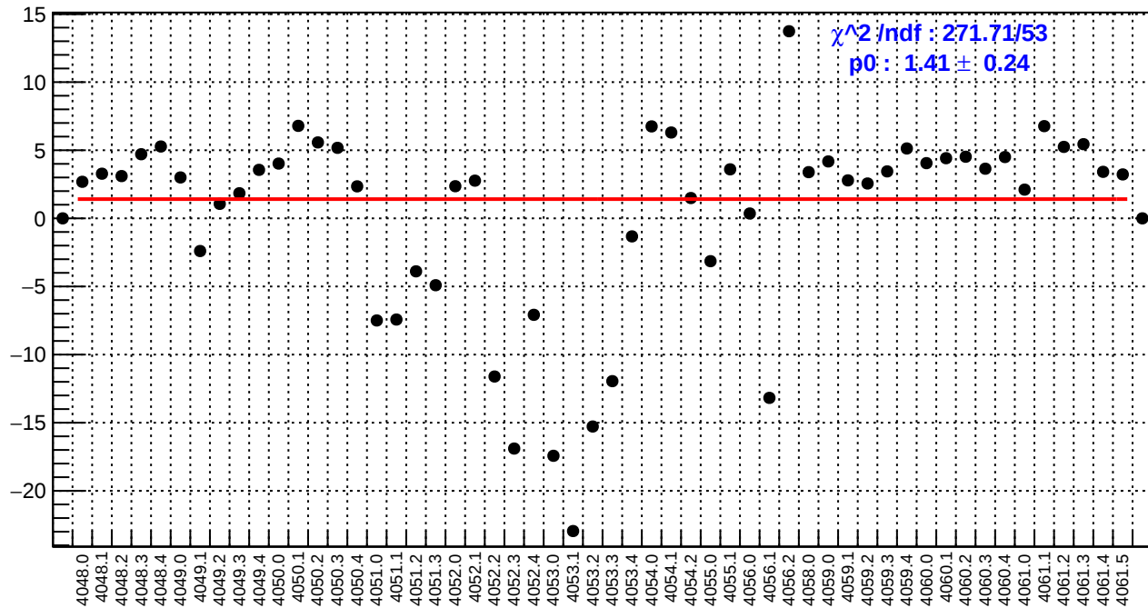
slug42: us_avg_bpm4eY/(ppb/nm)
