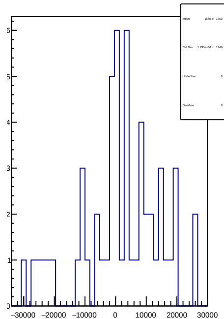
slug42: 1D Corr asym_sam1.mean/ppb-reg_asym_sam1.mean/ppb
