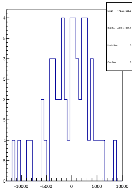
slug42: 1D Corr asym_us_dd.mean/ppb-reg_asym_us_dd.mean/ppb
