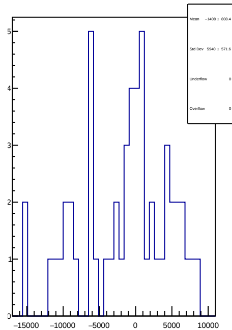
slug42: 1D Corr asym_dsl.mean/ppb-reg_asym_dsl.mean/ppb
