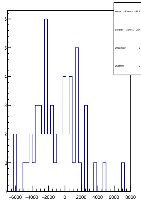
slug42: 1D Corr asym_us_avg.mean/ppb-reg_asym_us_avg.mean/ppb
