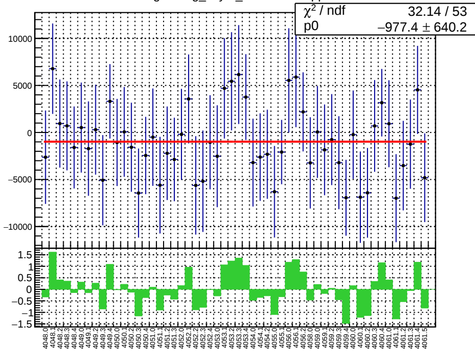
slug42: reg_asym_sam8.mean/ppb
