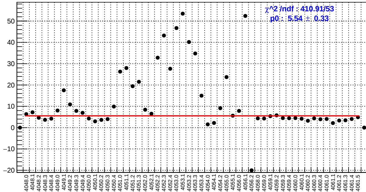
slug42: left_avg_bpm4aY/(ppb/nm)
