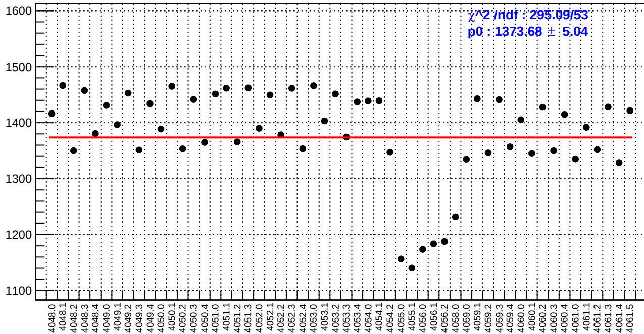
slug42: diff_bpm4aX.rms/nm
