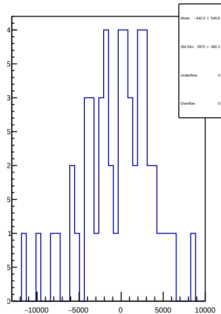
slug42: 1D Corr asym_ds_dd.mean/ppb-reg_asym_ds_dd.mean/ppb
