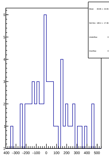
slug42: 1D Corr asym_left_dd.mean/ppb-reg_asym_left_dd.mean/ppb
