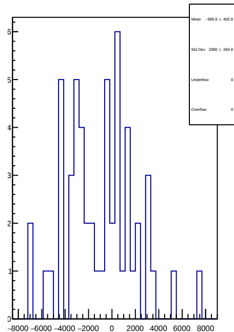
slug42: 1D Corr asym_ds_avg.mean/ppb-reg_asym_ds_avg.mean/ppb
