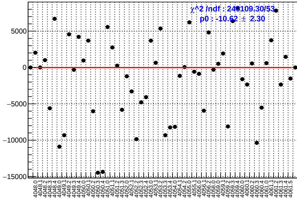
slug42: asym_usl.mean/ppb-reg_asym_usl.mean/ppb
