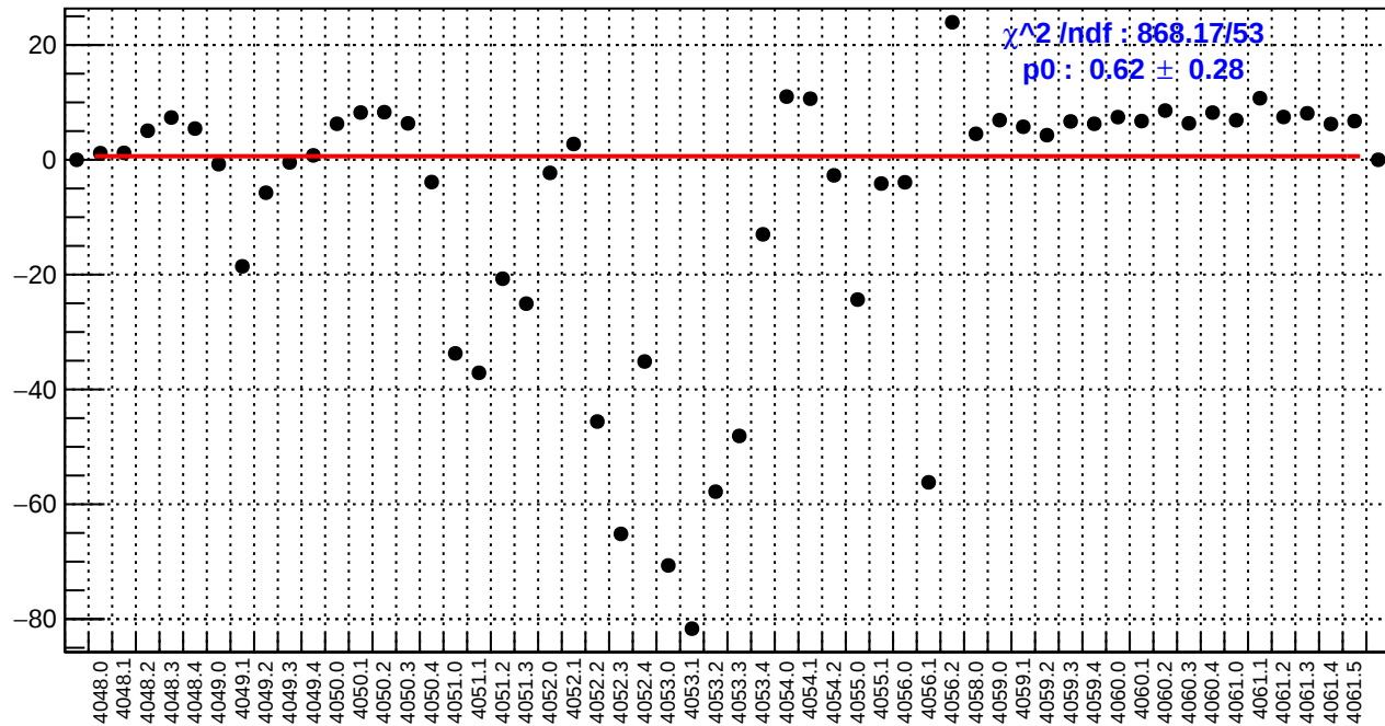
slug42: dsl_bpm4eY/(ppb/nm)
