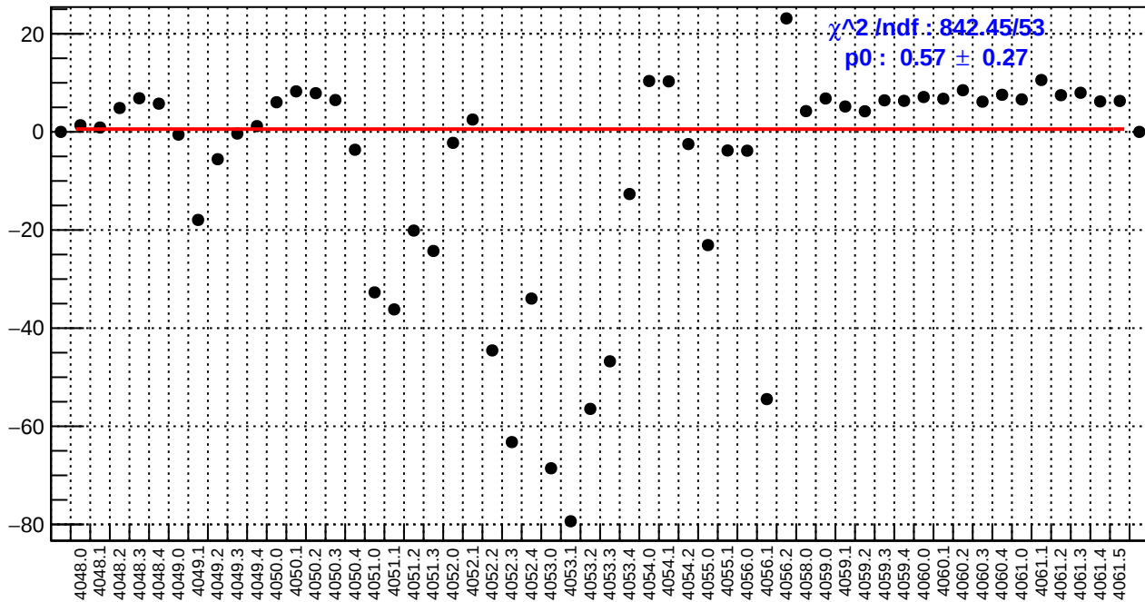
slug42: left_avg_bpm4eY/(ppb/nm)
