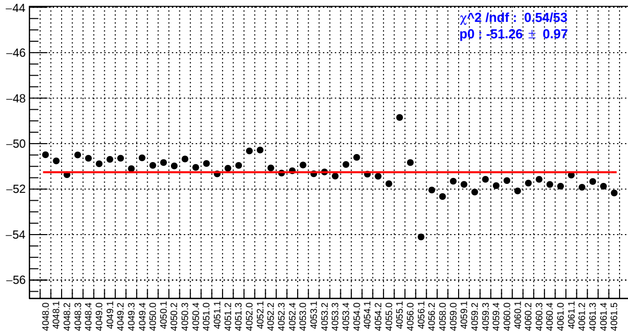
slug42: ds_avg_bpm12X/(ppb/nm)
