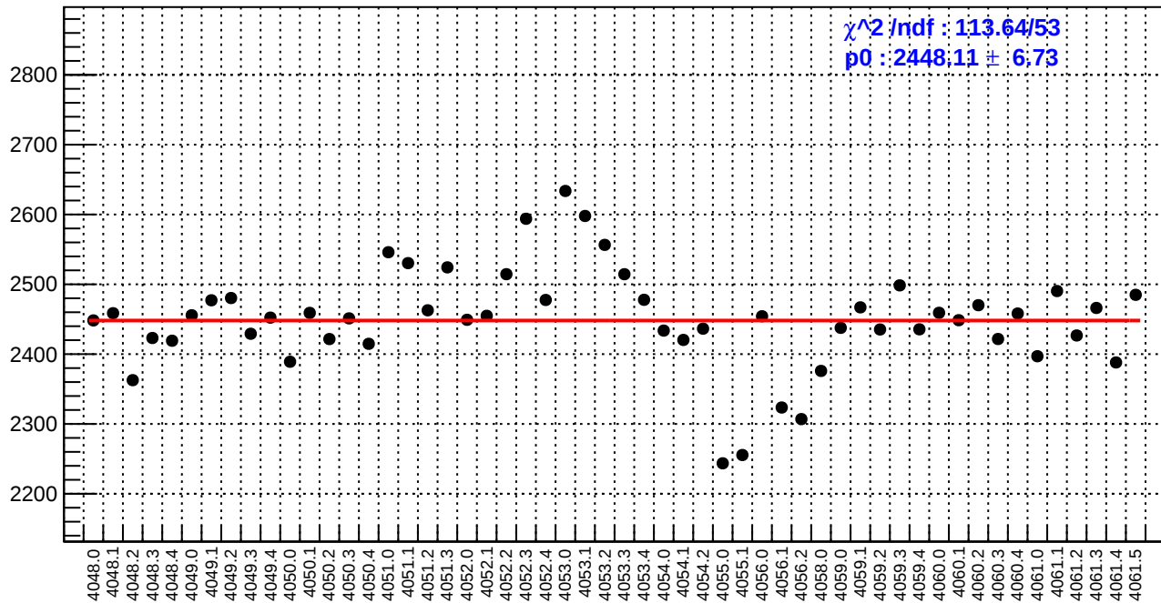
slug42: reg_asym_sam2.rms/ppm
