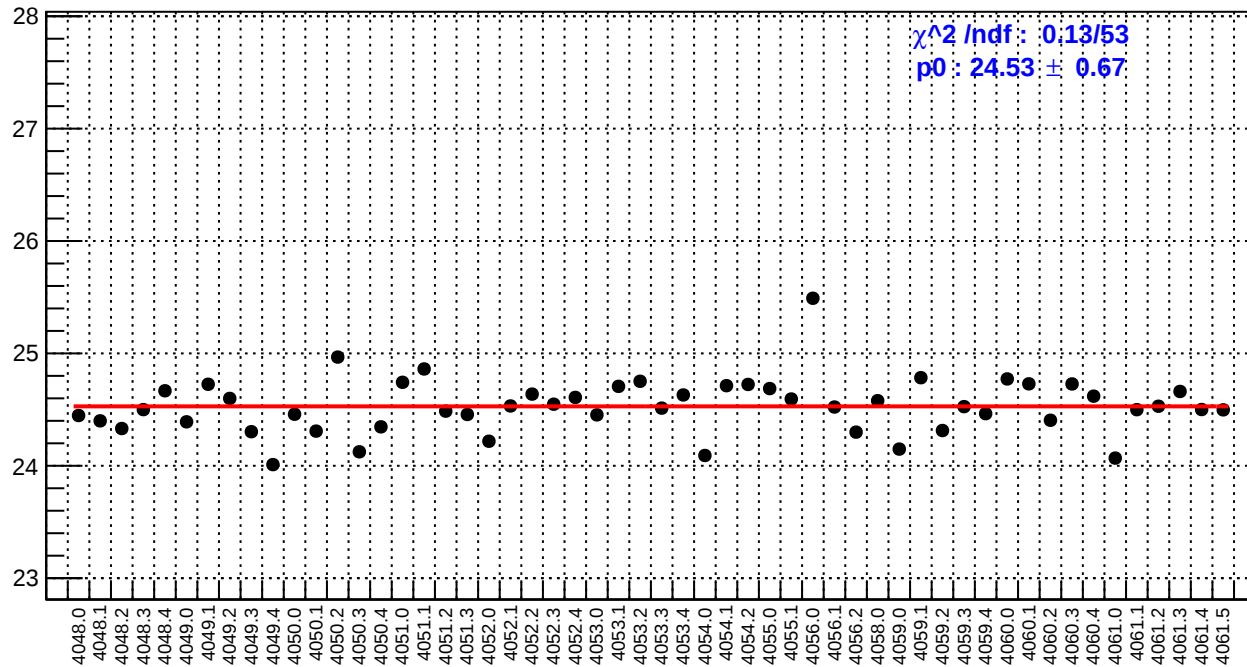
slug42: reg_asym_left_dd.rms/ppm
