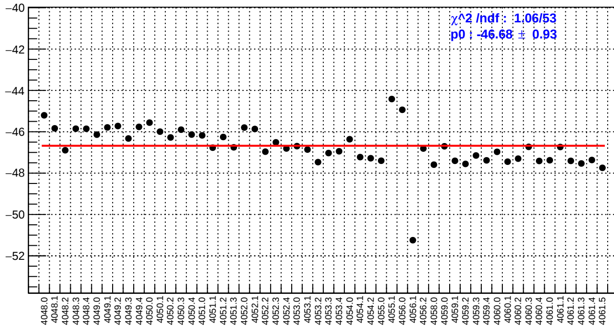
slug42: left_avg_bpm12X/(ppb/nm)
