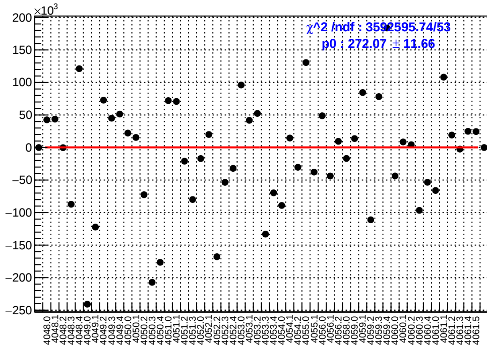
slug42: asym_sam3.mean/ppb-reg_asym_sam3.mean/ppb
