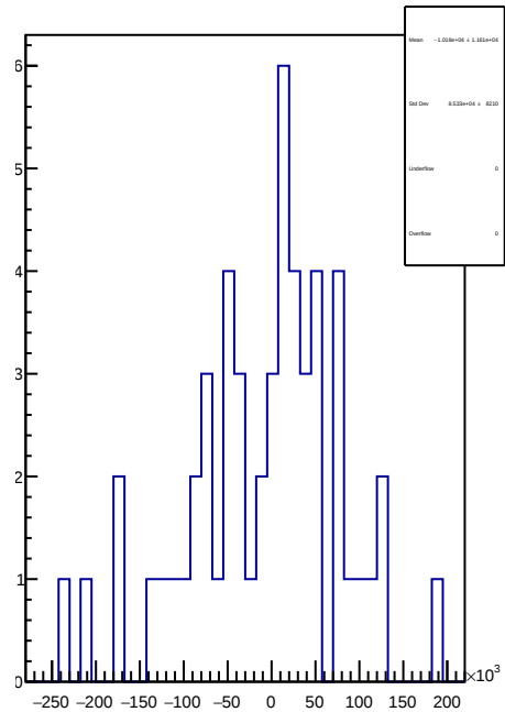
slug42: 1D Corr asym_sam3.mean/ppb-reg_asym_sam3.mean/ppb
