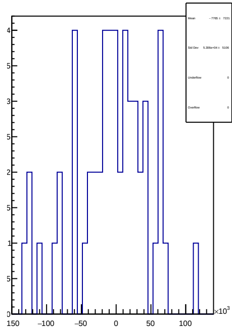
slug42: 1D Corr asym_sam4.mean/ppb-reg_asym_sam4.mean/ppb
