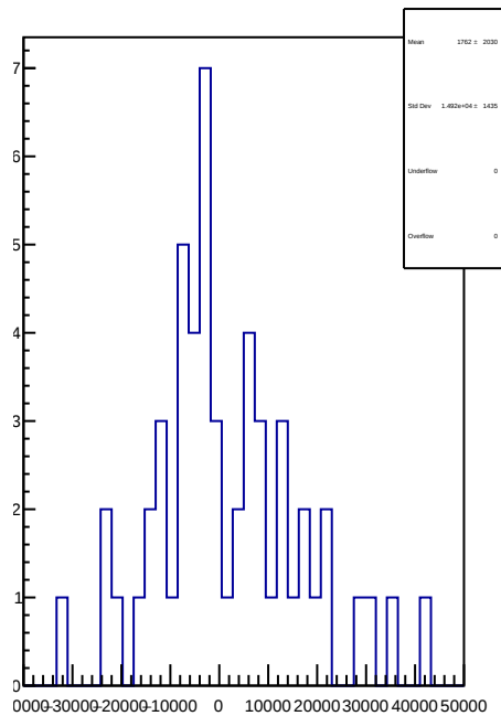
slug42: 1D Corr asym_sam7.mean/ppb-reg_asym_sam7.mean/ppb
