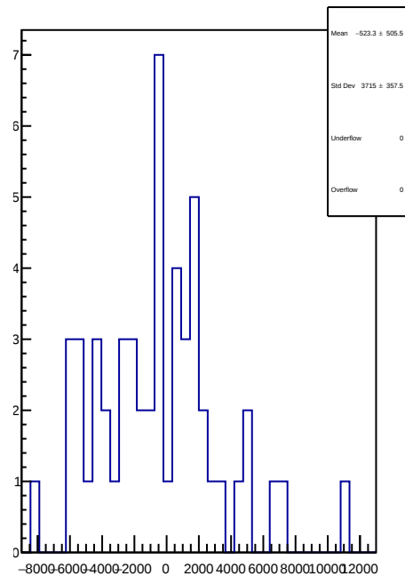
slug42: 1D Corr asym_dsr.mean/ppb-reg_asym_dsr.mean/ppb
