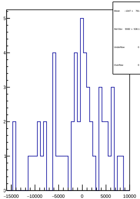
slug42: 1D Corr asym_usl.mean/ppb-reg_asym_usl.mean/ppb
