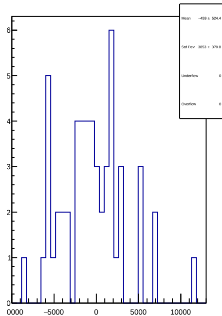
slug42: 1D Corr asym_right_avg.mean/ppb-reg_asym_right_avg.mean/ppb
