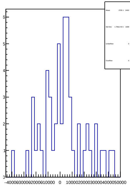
slug42: 1D Corr asym_sam8.mean/ppb-reg_asym_sam8.mean/ppb
