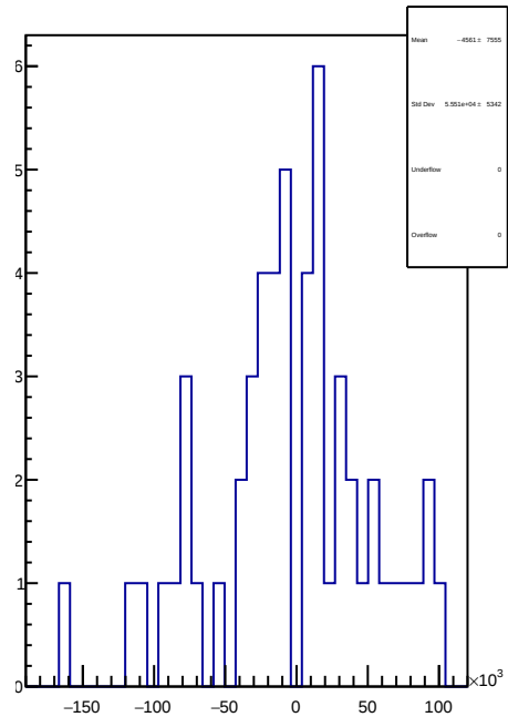
slug42: 1D Corr asym_sam2.mean/ppb-reg_asym_sam2.mean/ppb
