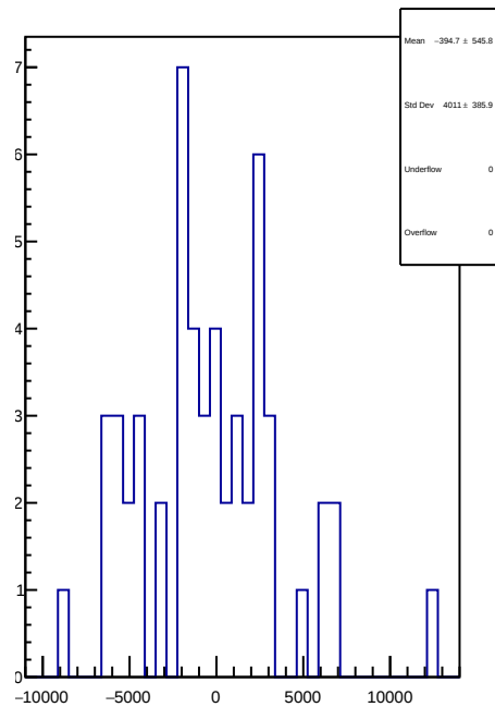
slug42: 1D Corr asym_usr.mean/ppb-reg_asym_usr.mean/ppb
