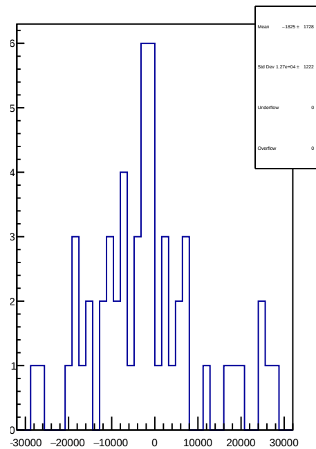
slug42: 1D Corr asym_sam5.mean/ppb-reg_asym_sam5.mean/ppb
