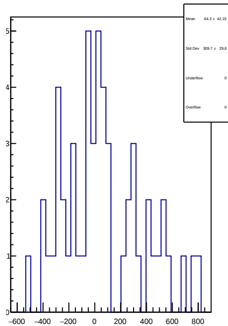
slug42: 1D Corr asym_right_dd.mean/ppb-reg_asym_right_dd.mean/ppb
