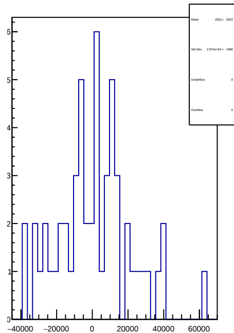
slug42: 1D Corr asym_sam6.mean/ppb-reg_asym_sam6.mean/ppb
