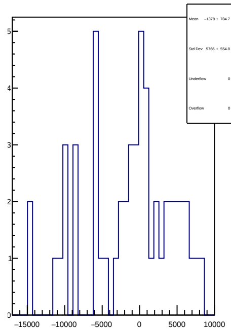
slug42: 1D Corr asym_left_avg.mean/ppb-reg_asym_left_avg.mean/ppb
