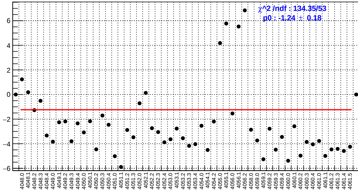
slug42: ds_avg_bpm4aX/(ppb/nm)
