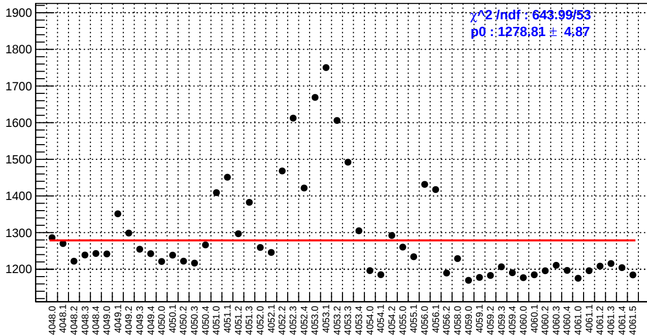
slug42: reg_asym_sam4.rms/ppm
