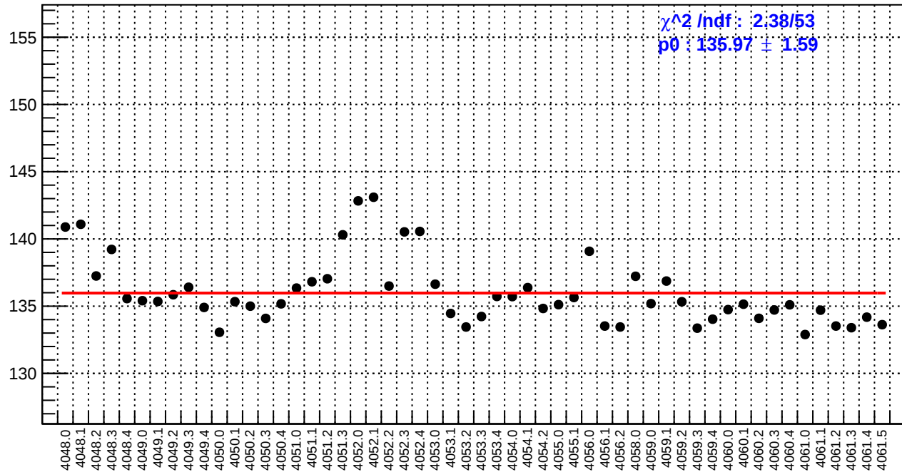
slug42: reg_asym_dsr.rms/ppm
