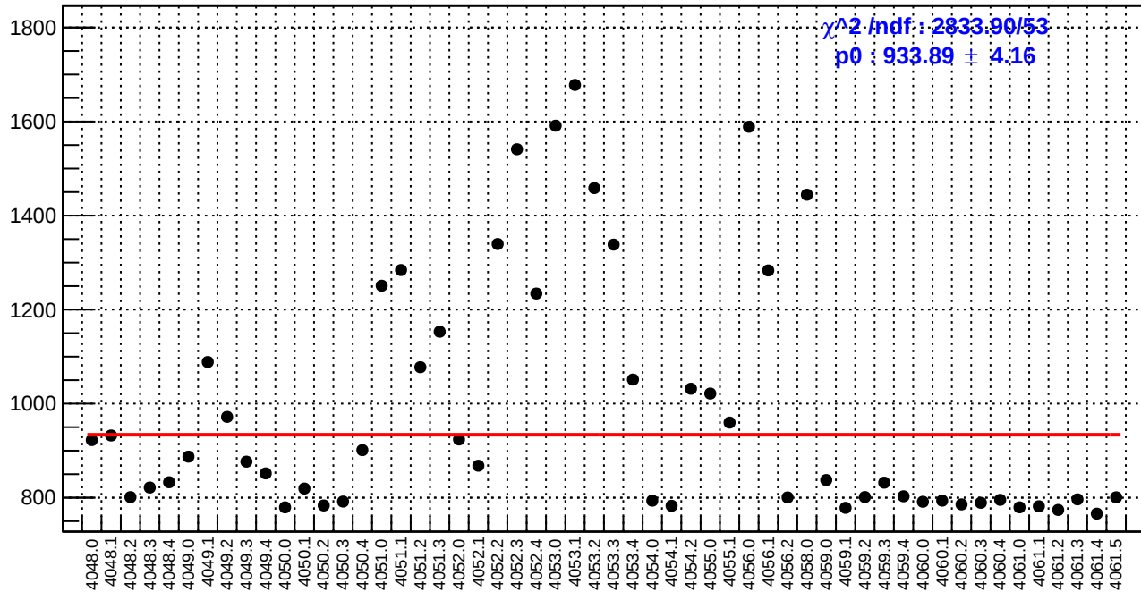
slug42: reg_asym_sam3.rms/ppm
