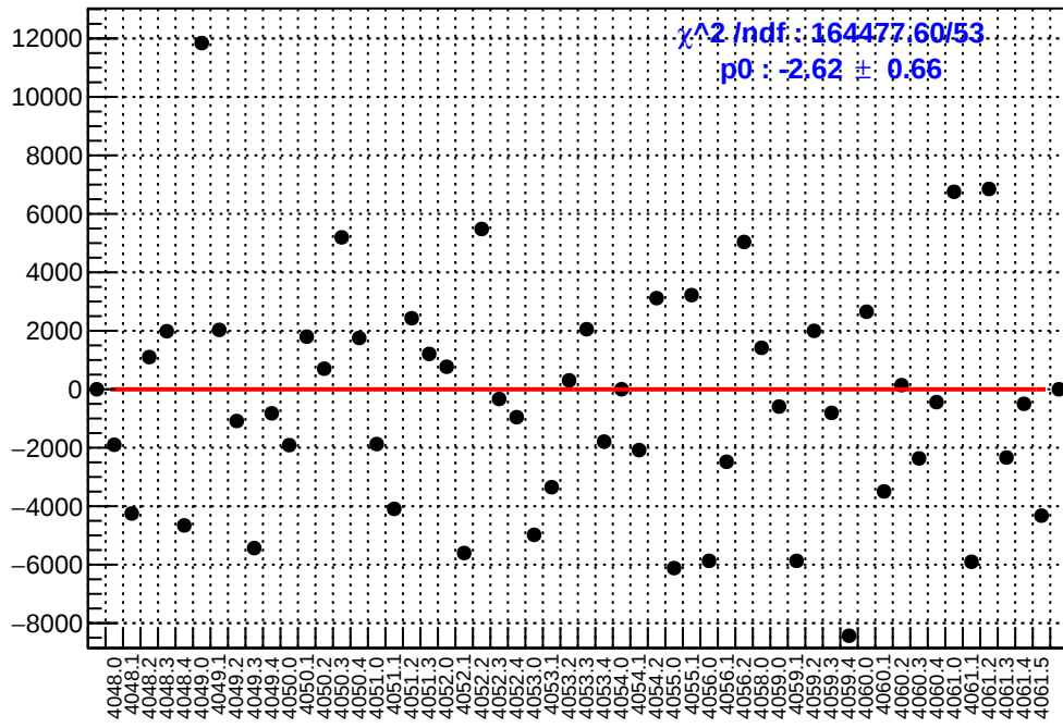
slug42: asym_right_avg.mean/ppb-reg_asym_right_avg.mean/ppb
