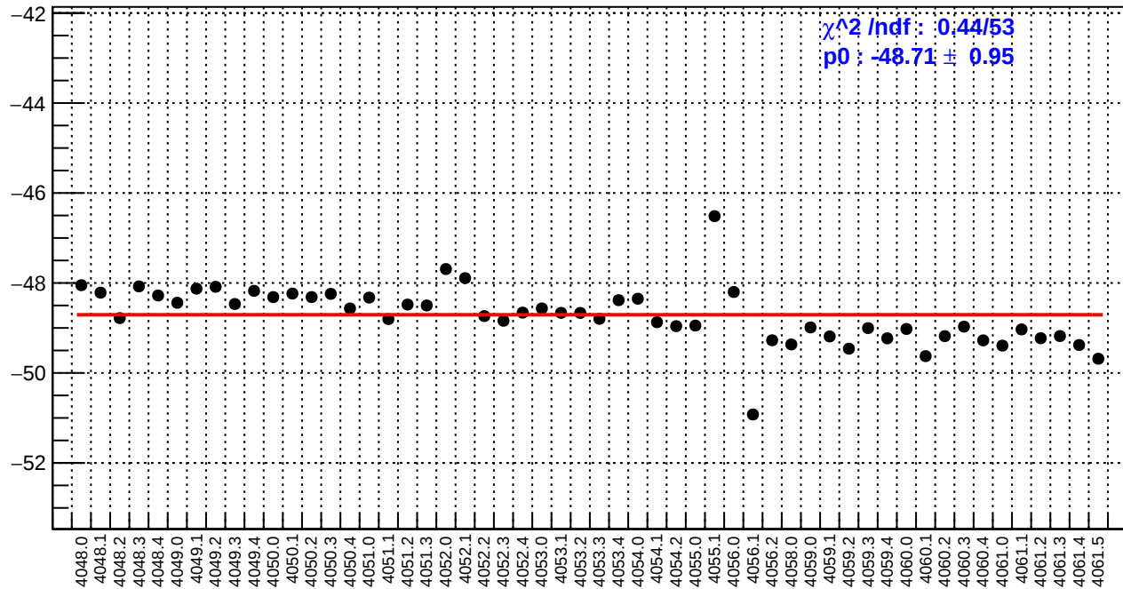
slug42: us_avg_bpm12X/(ppb/nm)
