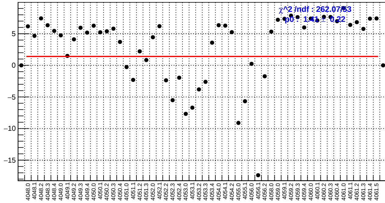
slug42: right_avg_bpm4aY/(ppb/nm)
