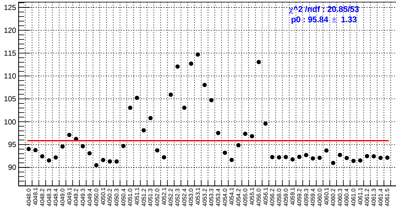
slug42: reg_asym_us_dd.rms/ppm
