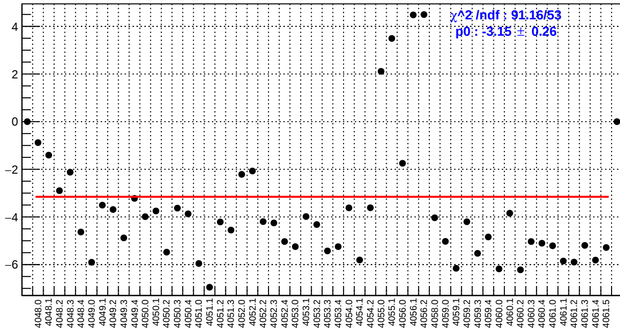
slug42: us_avg_bpm4aX/(ppb/nm)
