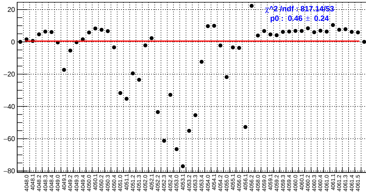
slug42: usl_bpm4eY/(ppb/nm)
