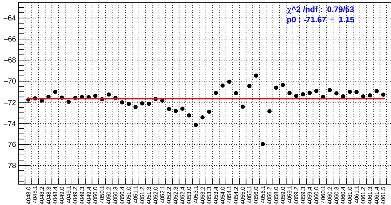
slug42: left_avg_bpm4eX/(ppb/nm)
