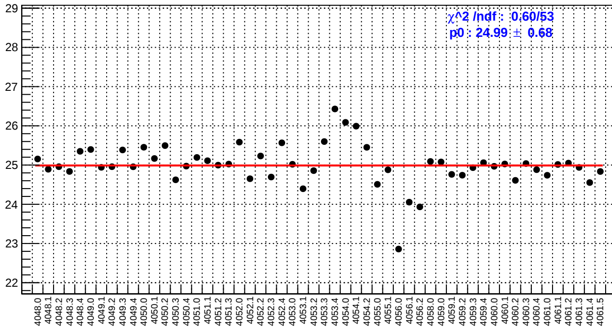
slug42: right_avg_bpm4eX/(ppb/nm)
