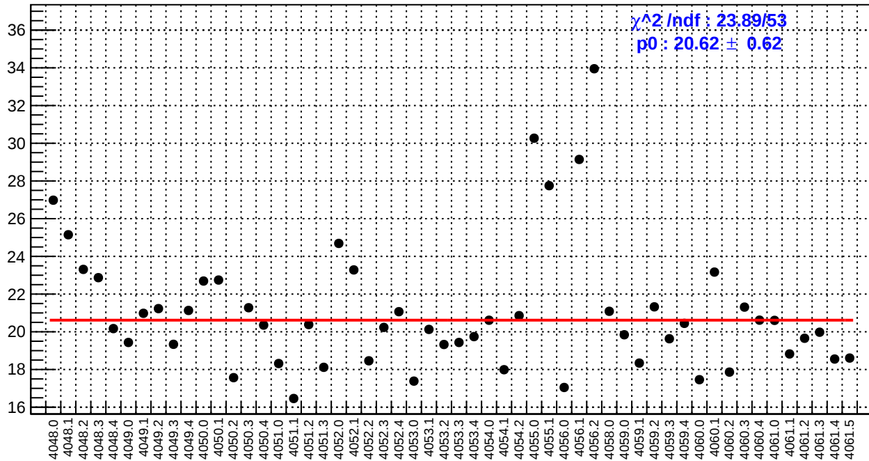
slug42: left_avg_bpm4aX/(ppb/nm)
